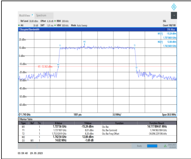
NTNV_N66_PC3_15_15_M_TID6_Ant1#1
