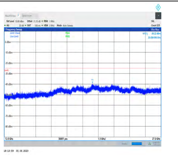
1-N41-PC3-30-100-M-1-N/A-DFT-PI2BPSK-Inner_1R B_Left-1@1-12000-27000-Ant1-20438.00--39.22--25- PASS
