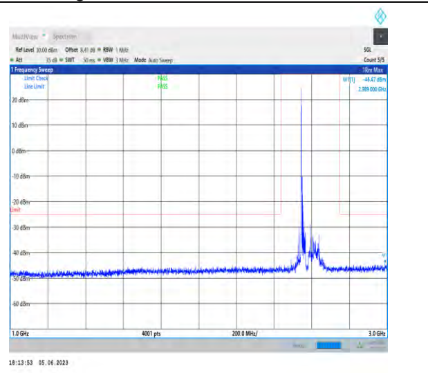
1-N41-PC3-30-100-M-1-N/A-DFT-PI2BPSK-Inner_1R B_Left-1@1-1000-3000-Ant1-2989.00--44.47--25-PA SS
