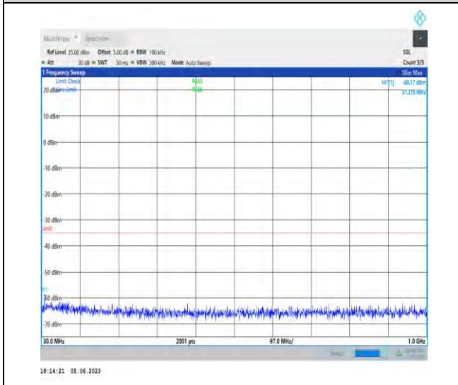
1-N41-PC3-30-100-H-1-N/A-DFT-PI2BPSK-Inner_1 RB_Left-1@1-30-1000-Ant1-37.28--60.17--35-PASS
