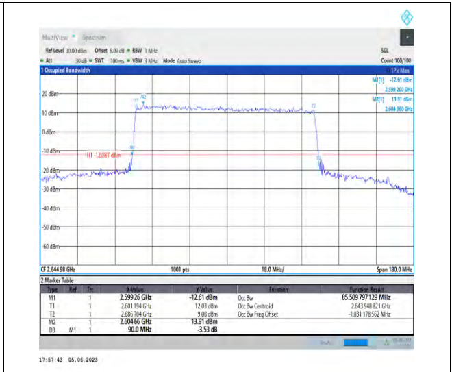
1-N41-PC3-30-90-H-4-DFT-64QAM-Outer_Full-240 @0-Ant1-85.51-90.000-<90-PASS
