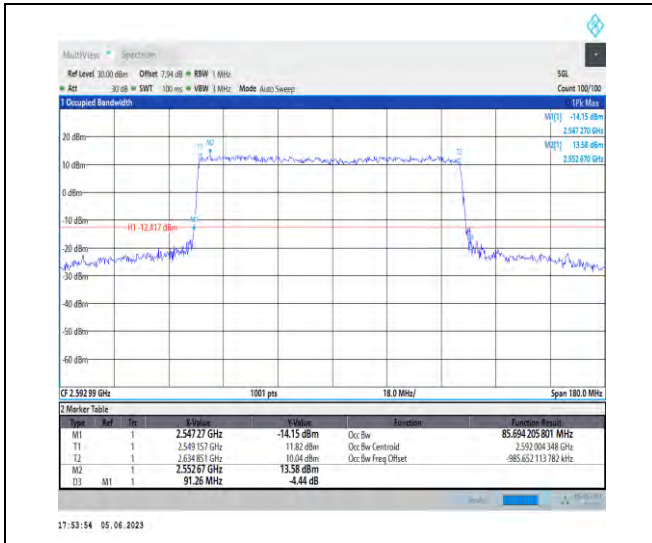
1-N41-PC3-30-90-M-4-DFT-64QAM-Outer_Full-240 @0-Ant1-85.694-91.260-<90-PASS
