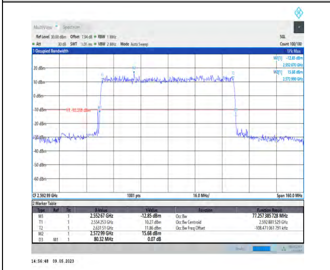
1-N41-PC3-30-80-M-2-DFT-PI2BPSK-Outer_Full-216 @0-Ant1-77.257-80.320-<80-PASS
