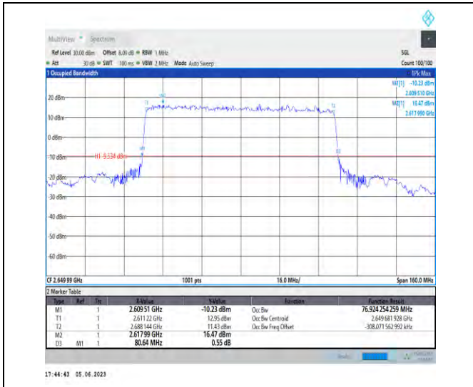
1-N41-PC3-30-80-H-2-DFT-PI2BPSK-Outer_Full-216 @0-Ant1-76.924-80.640-<80-PASS
