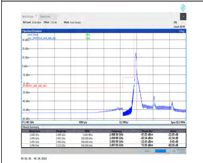
1-N41-PC3-30-20-L-4-CP-QPSK-Edge_1RB_Left-1@0-Ant1-1--PASS-see graph
