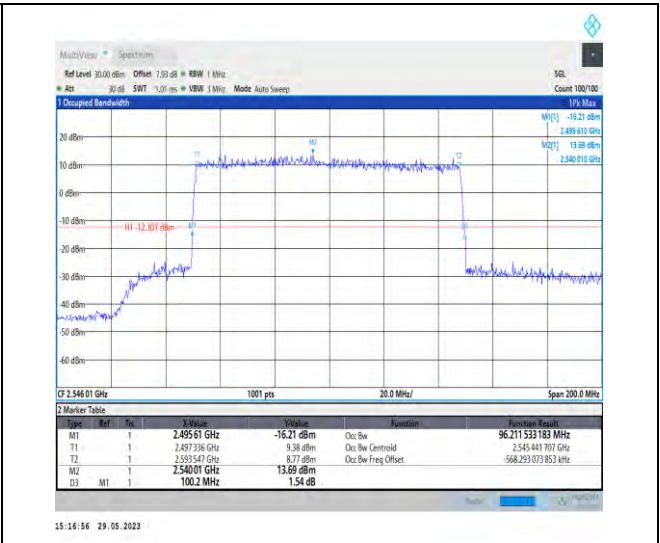
1-N41-PC3-30-100-L-3-DFT-16QAM-Outer_Full-270 @0-Ant1-96.212-100.20-≤100-PASS
