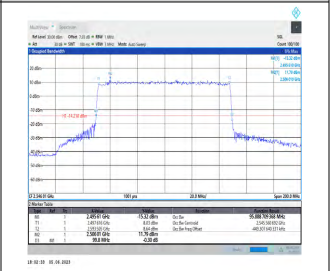
1-N41-PC3-30-100-L-5-DFT-256QAM-Outer_Full-27 @0-Ant1-95.889-99.800-≤100-PASS
