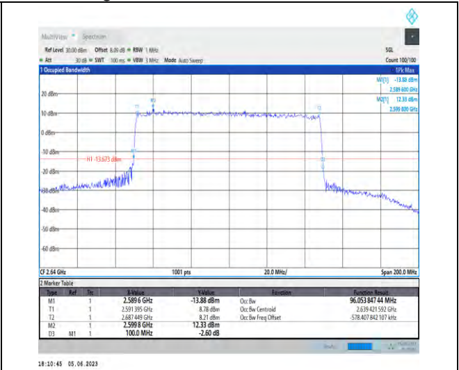
1-N41-PC3-30-100-H-5-DFT-256QAM-Outer_Full-270 @0-Ant1-96.054-100.000-≤100-PASS
