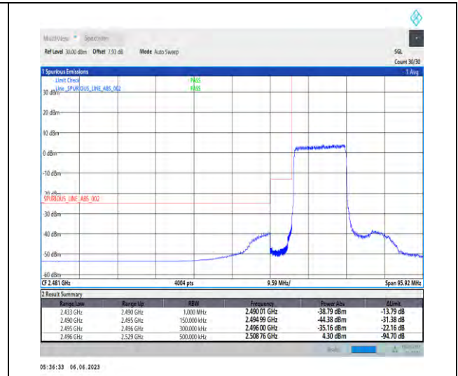
1-N41-PC3-30-15-L-3-DFT-PI2BPSK-Outer_Full-36@0-Ant1-1--PASS-see graph
