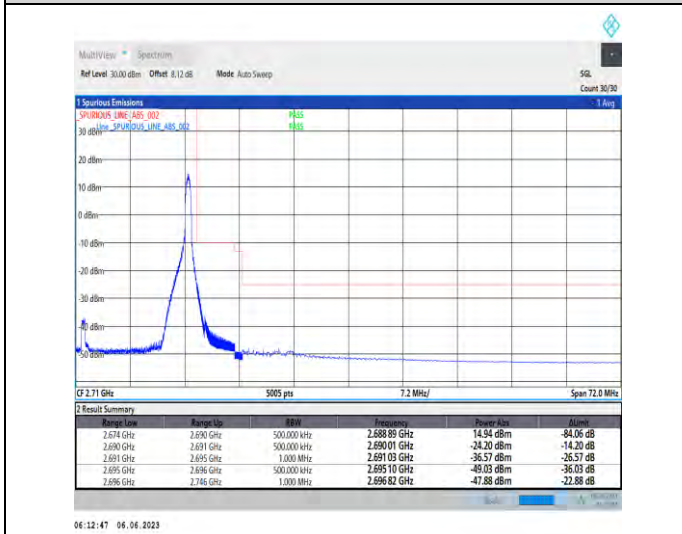
1-N41-PC3-30-30-H-5-CP-QPSK-Edge_1RB_Right-1@77-Ant1-1--PASS-see graph
