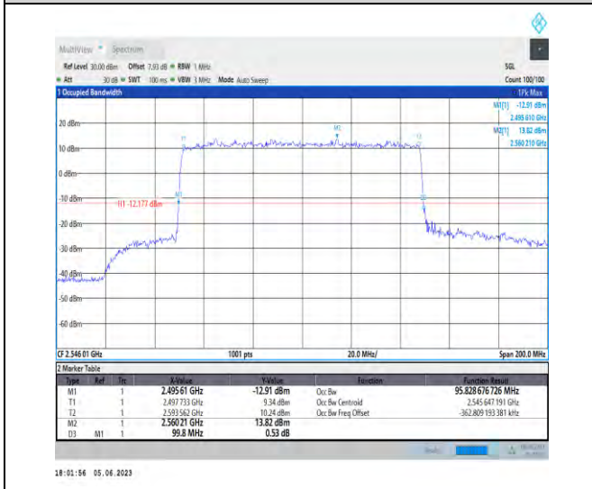
1-N41-PC3-30-100-L-4-DFT-64QAM-Outer_Full-270 @0-Ant1-95.829-99.800-≤100-PASS
