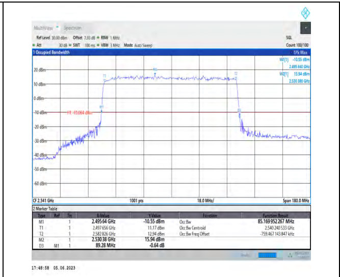
1-N41-PC3-30-90-L-2-DFT-PI2BPSK-Outer_Full-240 @0-Ant1-85.17-89.280-≤90-PASS
