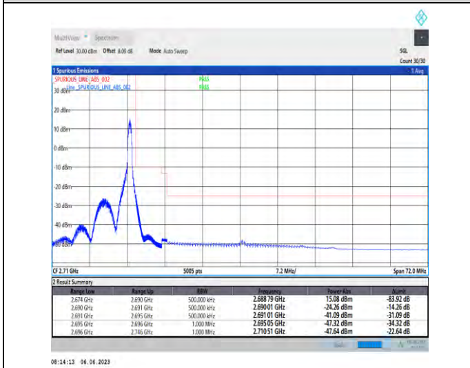
1-N41-PC3-30-80-H-5-CP-QPSK-Edge_1RB_Right-1@216-Ant1-1--PASS-see graph
