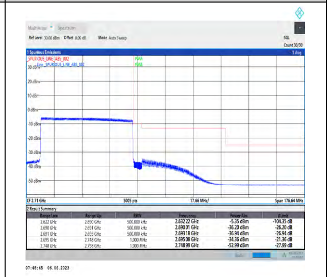
1-N41-PC3-30-60-H-6-CP-QPSK-Outer_Full-162@0-Ant1-1--PASS-see graph
