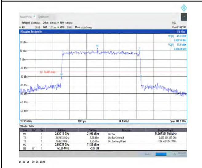
1-N41-PC3-30-70-H-4-DFT-64QAM-Outer_Full-180 @0-Ant1-64.007-66.360-<=70-PASS
