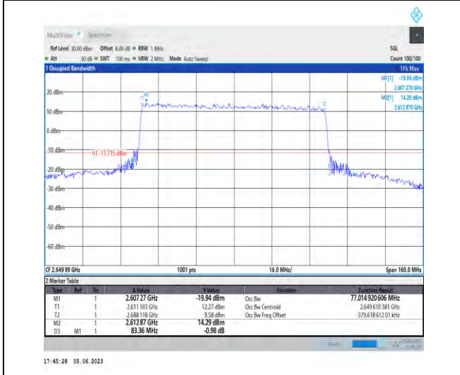
1-N41-PC3-30-80-H-4-DFT-64QAM-Outer_Full-216 @0-Ant1-77.015-83.360-<80-PASS
