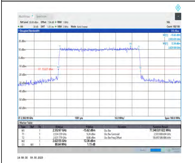
1-N41-PC3-30-80-M-6-CP-QPSK-Outer_Full-217@0 -Ant1-77.54-80.640-≤80-PASS
