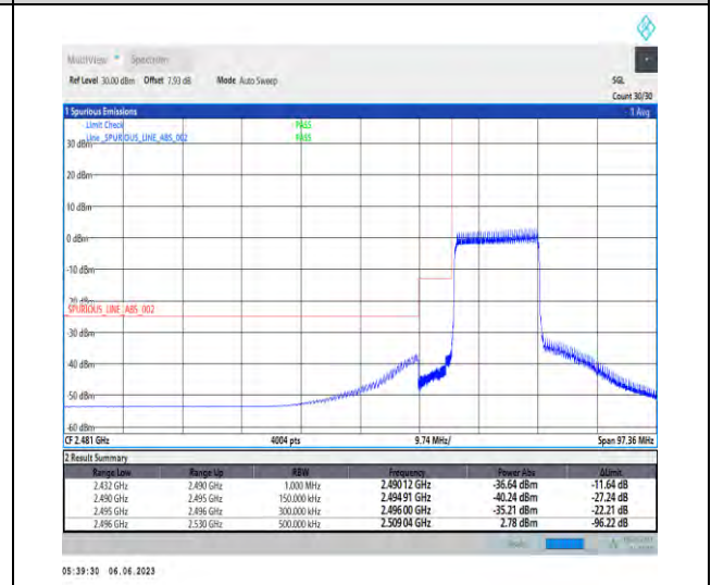
1-N41-PC3-30-15-L-6-CP-QPSK-Outer_Full-38@0-Ant1-1--PASS-see graph
