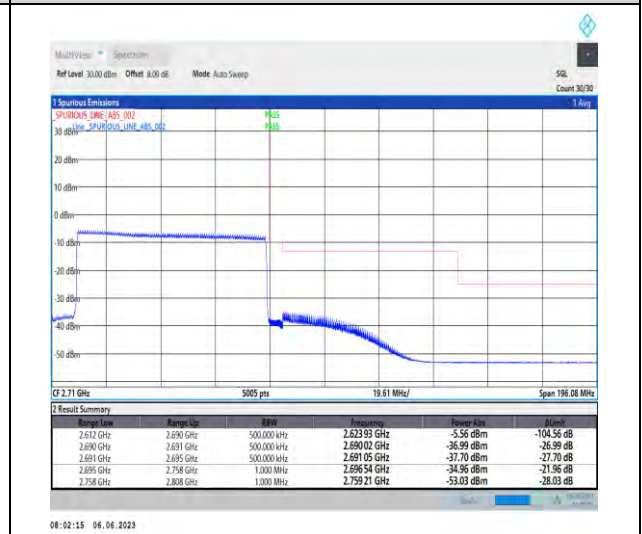
1-N41-PC3-30-70-H-6-CP-QPSK-Outer_Full-189@0-Ant1-1--PASS-see graph
