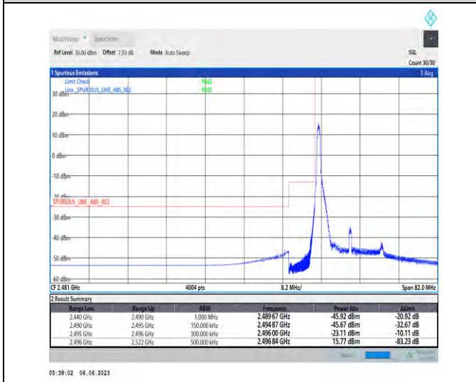
1-N41-PC3-30-15-L-4-CP-QPSK-Edge_1RB_Left-1@0-Ant1-1--PASS-see graph
