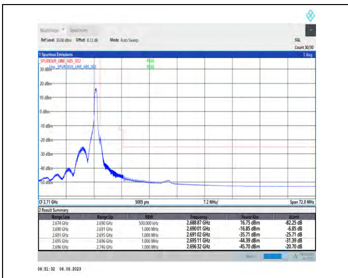
1-N41-PC3-30-40-H-2-DFT-PI2BPSK-Edge_1RB_Right-t-1@105-Ant1-1--PASS-see graph
