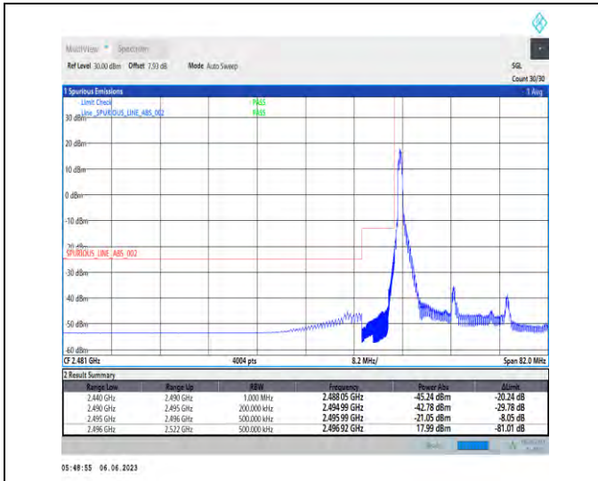
1-N41-PC3-30-20-L-1-DFT-PI2BPSK-Edge_1RB_Left-1@0-Ant1-1--PASS-see graph
