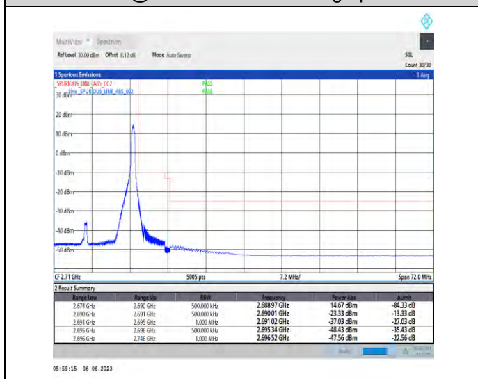
1-N41-PC3-30-20-H-5-CP-QPSK-Edge_1RB_Right-1@50-Ant1-1--PASS-see graph
