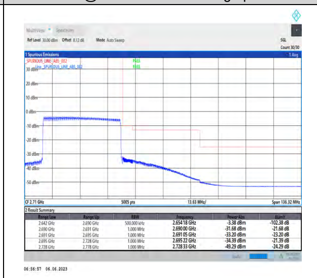
1-N41-PC3-30-40-H-6-CP-QPSK-Outer_Full-106@0-Ant1-1--PASS-see graph
