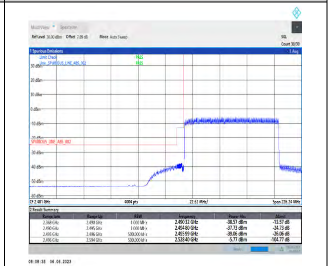
1-N41-PC3-30-80-L-6-CP-QPSK-Outer_Full-217@0-Ant1-1--PASS-see graph
