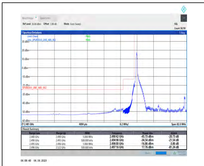
1-N41-PC3-30-50-L-1-DFT-PI2BPSK-Edge_1RB_Left-1@0-Ant1-1--PASS-see graph
