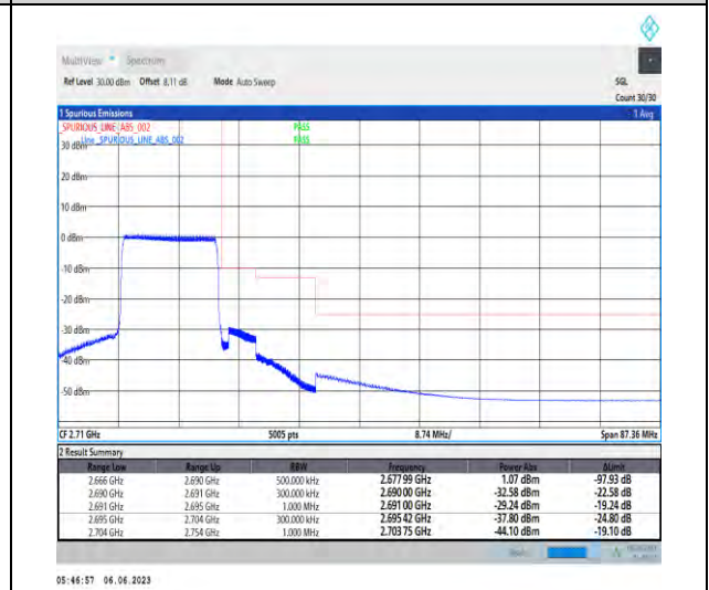
1-N41-PC3-30-15-H-6-CP-QPSK-Outer_Full-38@0-Ant1-1--PASS-see graph
