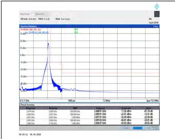
1-N41-PC3-30-30-H-2-DFT-PI2BPSK-Edge_1RB_Right-t1@77-Ant1-1--PASS-see graph
