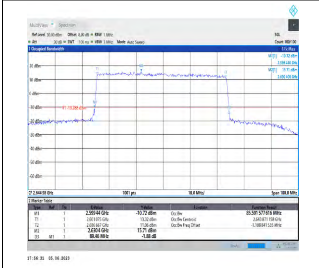
1-N41-PC3-30-90-H-1-DFT-QPSK-Outer_Full-240 @0-Ant1-85.592-89.460-<90-PASS
