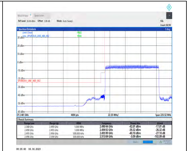
1-N41-PC3-30-80-L-3-DFT-PI2BPSK-Outer_Full-216@0-Ant1-1--PASS-see graph
