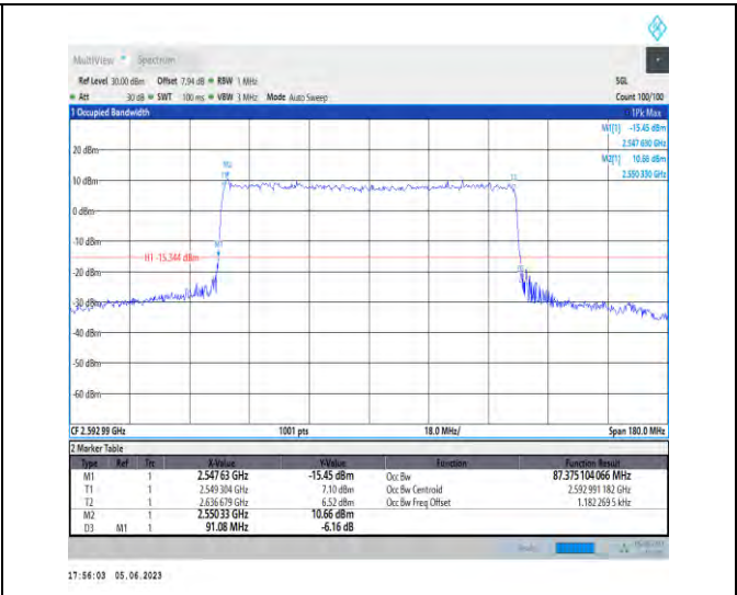
1-N41-PC3-30-90-M-9-CP-256QAM-Outer_Full-245 @0-Ant1-87.375-91.080-<90-PASS
