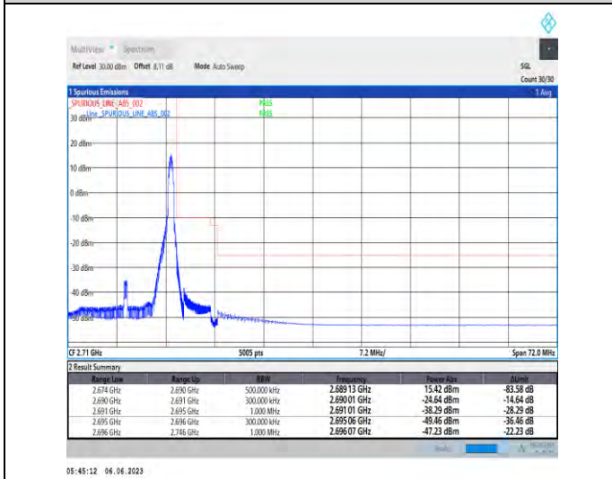
1-N41-PC3-30-15-H-5-CP-QPSK-Edge_1RB_Right-1@37-Ant1-1--PASS-see graph
