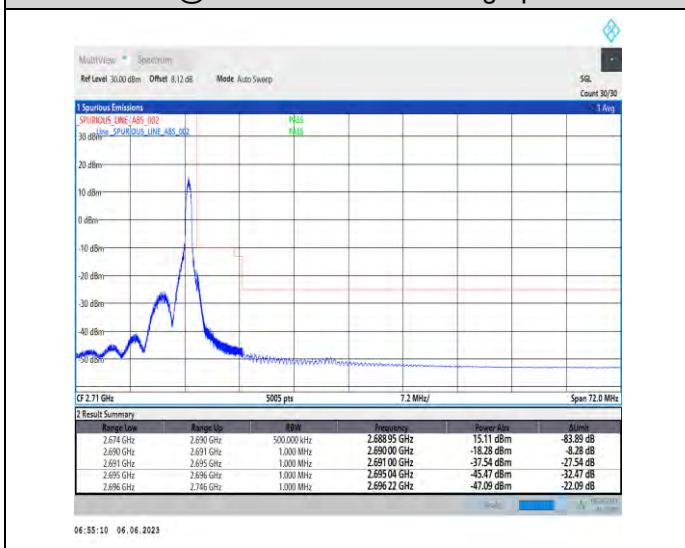
1-N41-PC3-30-40-H-5-CP-QPSK-Edge_1RB_Right-1@105-Ant1-1--PASS-see graph
