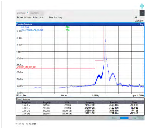
1-N41-PC3-30-70-L-1-DFT-PI2BPSK-Edge_1RB_Left-1@0-Ant1-1--PASS-see graph
