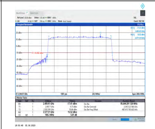
1-N41-PC3-30-100-L-1-DFT-QPSK-Outer_Full-270 @0-Ant1-95.644-100.200-≤100-PASS
