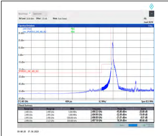
1-N41-PC3-30-30-L-1-DFT-PI2BPSK-Edge_1RB_Left-1@0-Ant1-1--PASS-see graph
