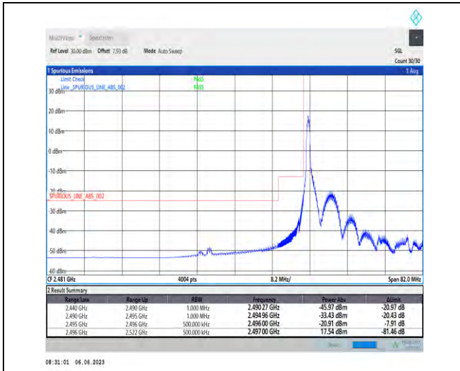
1-N41-PC3-30-100-L-1-DFT-PI2BPSK-Edge_1RB_Le ft-1@0-Ant1-1--PASS-see graph
