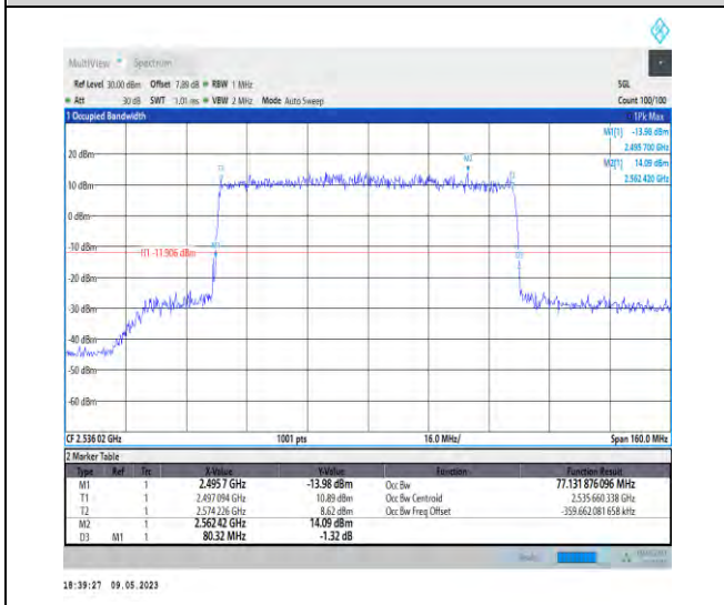
1-N41-PC3-30-80-L-3-DFT-16QAM-Outter_Full-216 @0-Ant1-77.132-80.320-≤80-PASS
