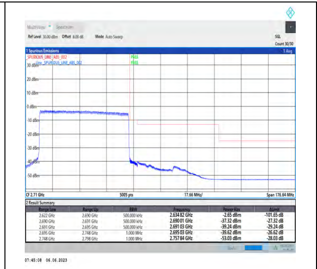
1-N41-PC3-30-60-H-3-DFT-PI2BPSK-Outer_Full-162@0-Ant1-1--PASS-see graph
