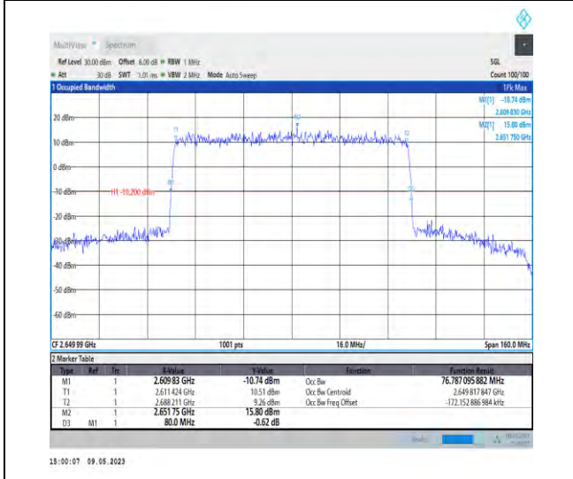
1-N41-PC3-30-80-H-1-DFT-QPSK-Outer_Full-216@ 0-Ant1-76.787-80.000-<80-PASS
