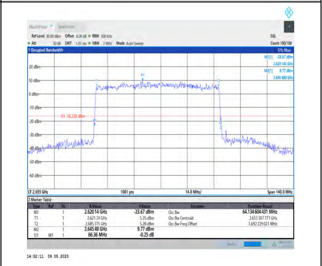
1-N41-PC3-30-70-H-5-DFT-256QAM-Outer_Full-180 @0-Ant1-64.135-66.360-<=70-PASS
