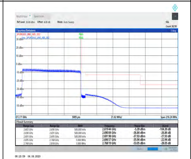
1-N41-PC3-30-80-H-6-CP-QPSK-Outer_Full-217@0-Ant1-1--PASS-see graph
