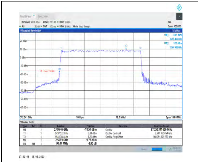
1-N41-PC3-30-90-L-9-CP-256QAM-Outer_Full-245@ 0-Ant1-87.256-91.440-<90-PASS
