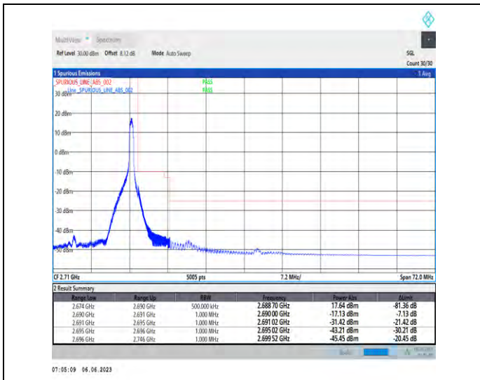
1-N41-PC3-30-50-H-2-DFT-PI2BPSK-Edge_1RB_Right-t-1@132-Ant1-1--PASS-see graph
