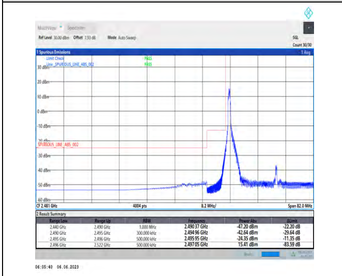
1-N41-PC3-30-30-L-4-CP-QPSK-Edge_1RB_Left-1@0-Ant1-1--PASS-see graph
