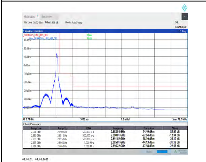
1-N41-PC3-30-70-H-5-CP-QPSK-Edge_1RB_Right-1@188-Ant1-1--PASS-see graph
