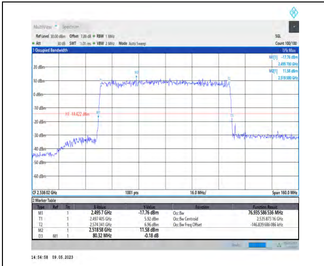
1-N41-PC3-30-80-L-5-DFT-256QAM-Outer_Full-216 @0-Ant1-76.936-80.320-≤80-PASS
