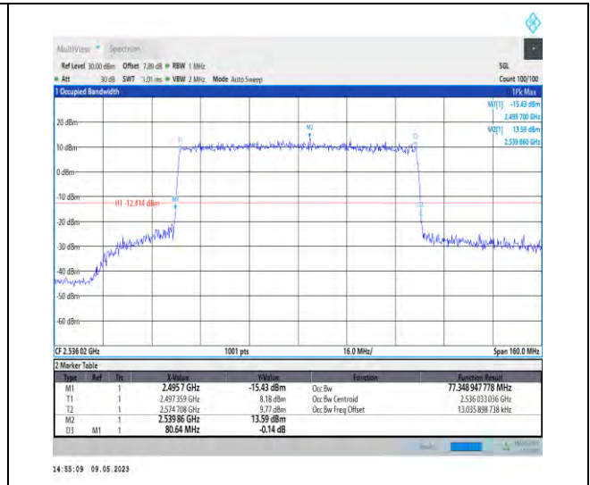
1-N41-PC3-30-80-L-6-CP-QPSK-Outer_Full-217@0 -Ant1-77.349-80.640-≤80-PASS
