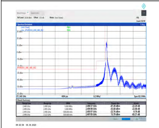
1-N41-PC3-30-100-L-4-CP-QPSK-Edge_1RB_Left-1 @0-Ant1-1--PASS-see graph
