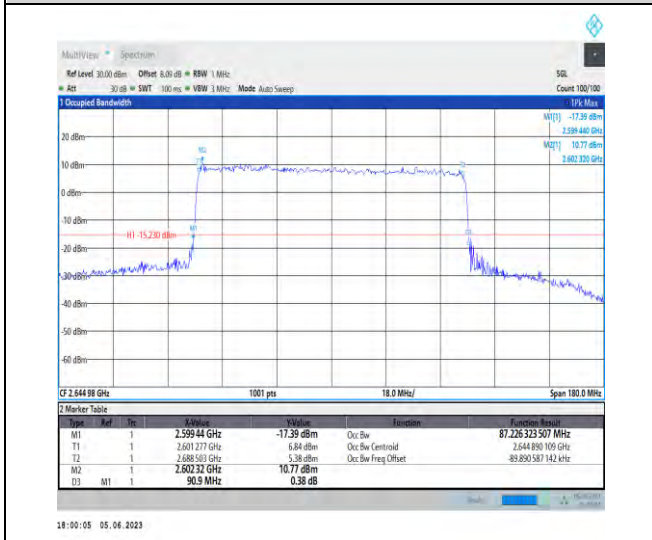
1-N41-PC3-30-90-H-9-CP-256QAM-Outer_Full-245 @0-Ant1-87.226-90.900-≤90-PASS
