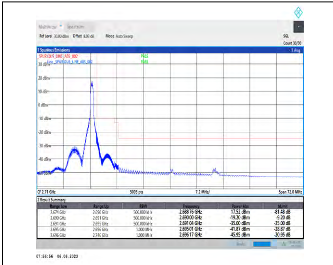
1-N41-PC3-30-70-H-2-DFT-PI2BPSK-Edge_1RB_Right-t-1@188-Ant1-1--PASS-see graph
