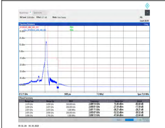
1-N41-PC3-30-10-H-5-CP-QPSK-Edge_1RB_Right-1@23-Ant1-1--PASS-see graph
