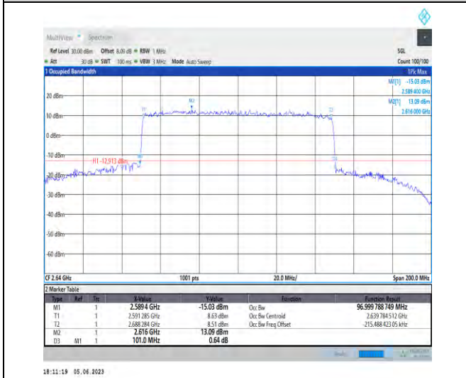
1-N41-PC3-30-100-H-6-CP-QPSK-Outer_Full-273 @0-Ant1-97-101.000-≤100-PASS
