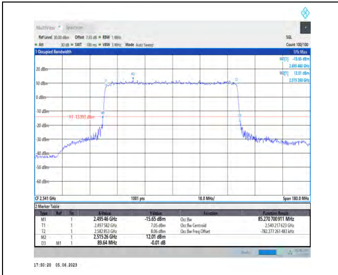
1-N41-PC3-30-90-L-5-DFT-256QAM-Outer_Full-240 @0-Ant1-85.271-89.640-<90-PASS
