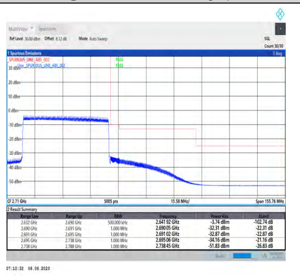
1-N41-PC3-30-50-H-6-CP-QPSK-Outer_Full-133@0-Ant1-1--PASS-see graph
