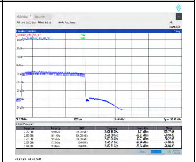
1-N41-PC3-30-100-H-6-CP-QPSK-Outer_Full-273 @0-Ant1-1--PASS-see graph
