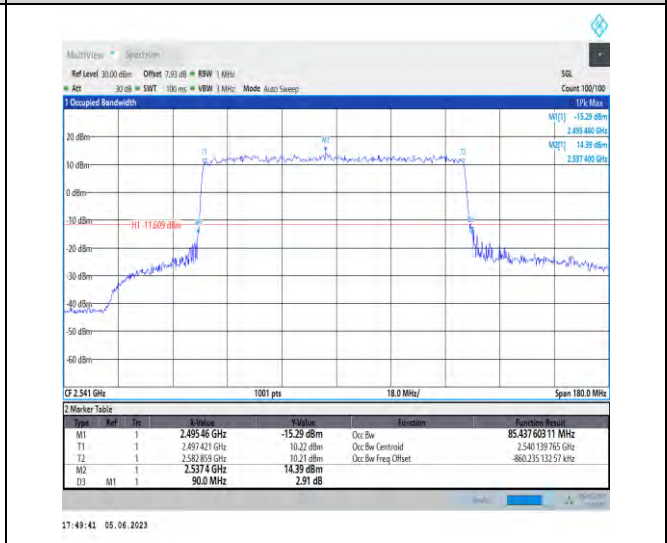
1-N41-PC3-30-90-L-4-DFT-64QAM-Outer_Full-240 @0-Ant1-85.438-90.000-≤90-PASS
