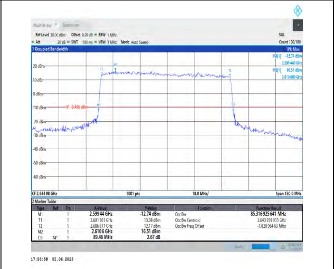
1-N41-PC3-30-90-H-2-DFT-PI2BPSK-Outer_Full-240 @0-Ant1-85.317-89.460-<90-PASS
