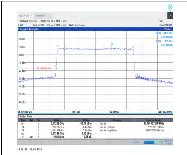
1-N41-PC3-30-100-M-9-CP-256QAM-Outer_Full-273 @0-Ant1-97.185-101.000-<=100-PASS
