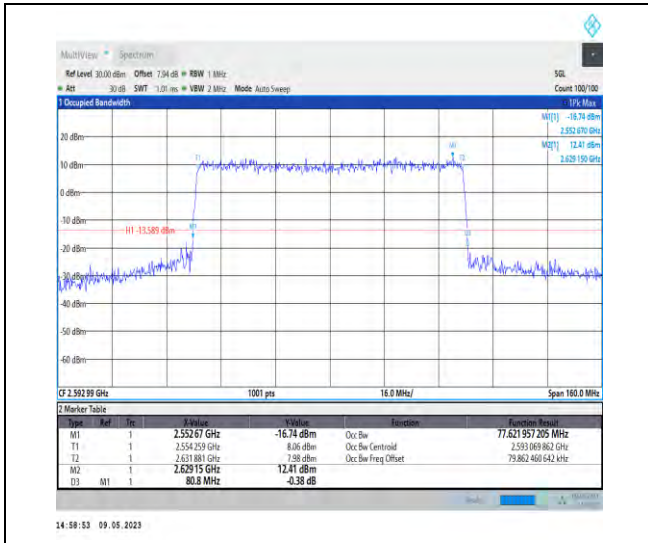
1-N41-PC3-30-80-M-8-CP-64QAM-Outer_Full-217 @0-Ant1-77.622-80.800-<80-PASS
