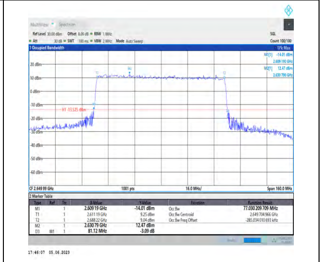
1-N41-PC3-30-80-H-5-DFT-256QAM-Outer_Full-216 @0-Ant1-77.03-81.120-<80-PASS
