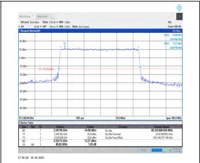
1-N41-PC3-30-90-M-5-DFT-256QAM-Outer_Full-240 @0-Ant1-85.536-89.820-<90-PASS
