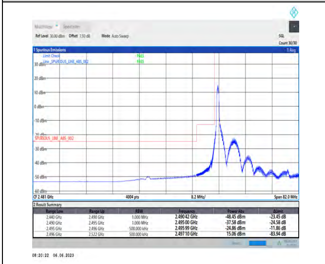
1-N41-PC3-30-90-L-4-CP-QPSK-Edge_1RB_Left-1@0-Ant1-1--PASS-see graph
