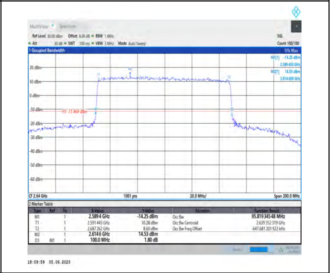
1-N41-PC3-30-100-H-3-DFT-16QAM-Outer_Full-270 @0-Ant1-95.819-100.000-<=100-PASS
