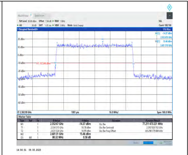
1-N41-PC3-30-80-M-1-DFT-QPSK-Outer_Full-216@ 0-Ant1-77.211-80.320-<80-PASS
