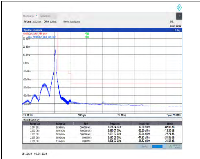
1-N41-PC3-30-80-H-2-DFT-PI2BPSK-Edge_1RB_Right-t-1@216-Ant1-1--PASS-see graph
