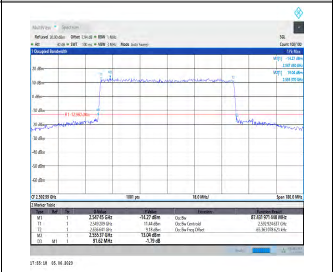
1-N41-PC3-30-90-M-7-CP-16QAM-Outer_Full-245@0 0-Ant1-87.432-91.620-<90-PASS
