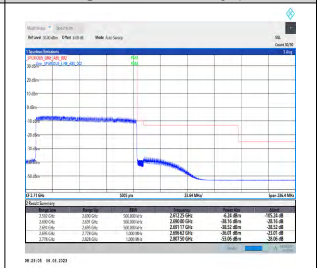
1-N41-PC3-30-90-H-6-CP-QPSK-Outer_Full-245@0-Ant1-1--PASS-see graph
