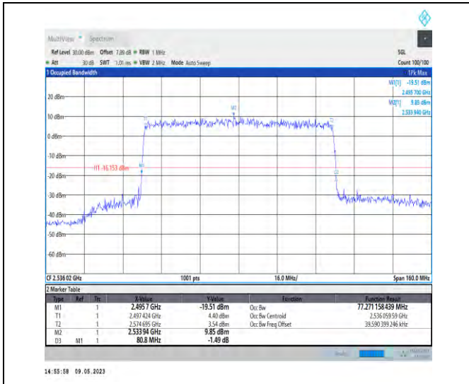
1-N41-PC3-30-80-L-9-CP-256QAM-Outer_Full-217@ 0-Ant1-77.271-80.800-<80-PASS
