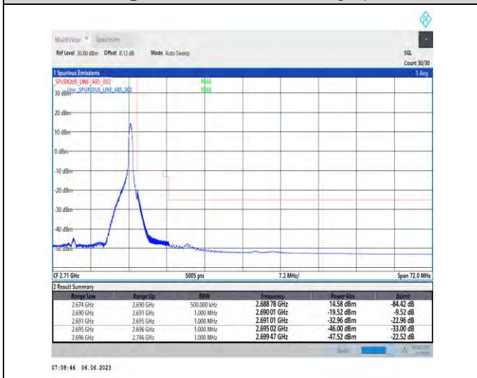
1-N41-PC3-30-50-H-5-CP-QPSK-Edge_1RB_Right-1@132-Ant1-1--PASS-see graph
