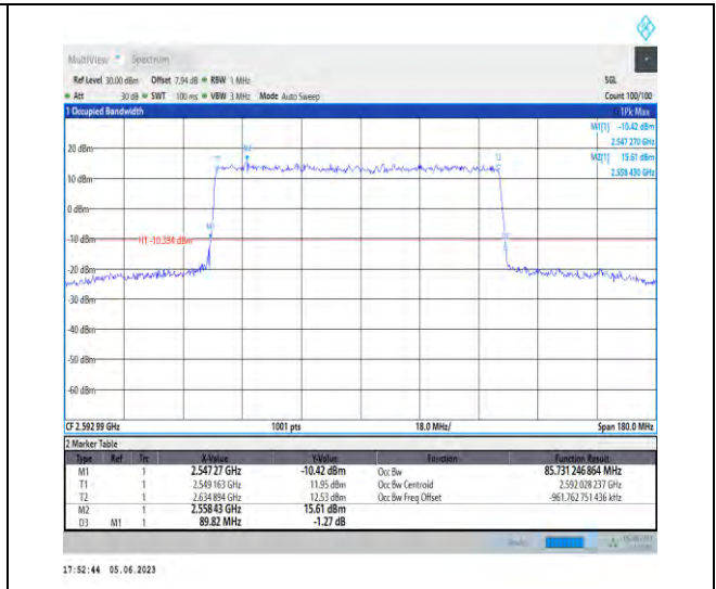
1-N41-PC3-30-90-M-1-DFT-QPSK-Outer_Full-240@ 0-Ant1-85.731-89.820-<90-PASS
