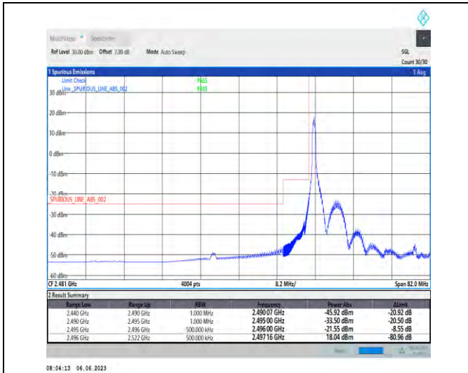
1-N41-PC3-30-80-L-1-DFT-PI2BPSK-Edge_1RB_Left-1@0-Ant1-1--PASS-see graph
