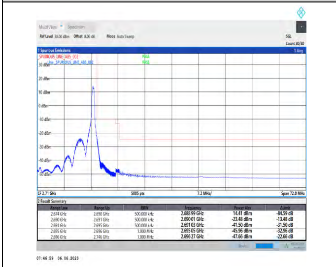
1-N41-PC3-30-60-H-5-CP-QPSK-Edge_1RB_Right-1@161-Ant1-1--PASS-see graph
