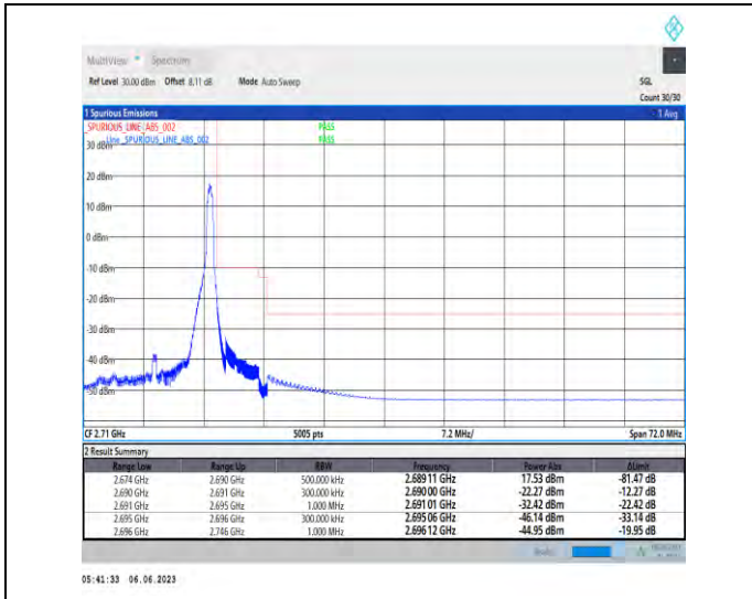
1-N41-PC3-30-15-H-2-DFT-PI2BPSK-Edge_1RB_Right-t1@37-Ant1-1--PASS-see graph
