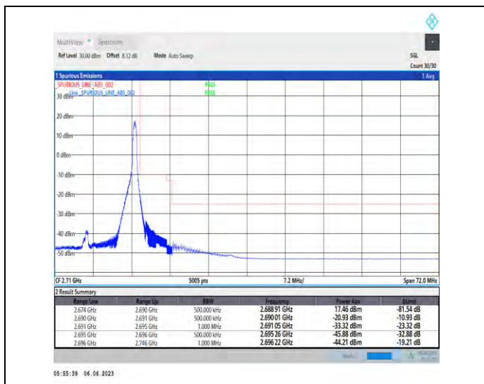
1-N41-PC3-30-20-H-2-DFT-PI2BPSK-Edge_1RB_Right-t-1@50-Ant1-1--PASS-see graph
