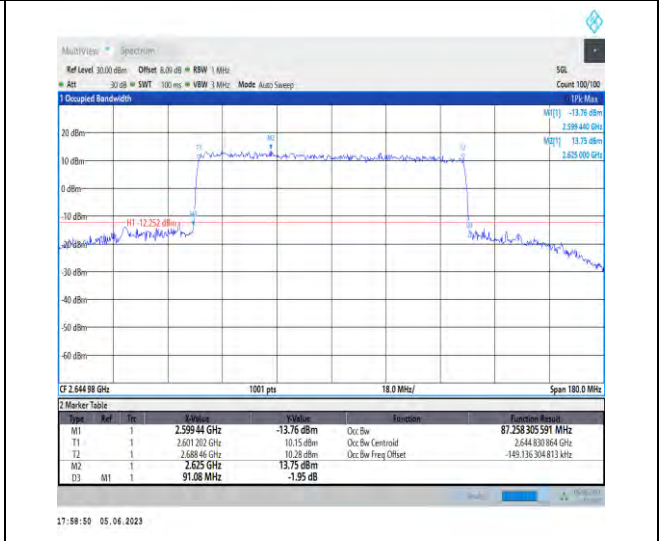
1-N41-PC3-30-90-H-6-CP-QPSK-Outer_Full-245@0 -Ant1-87.258-91.080-<90-PASS
