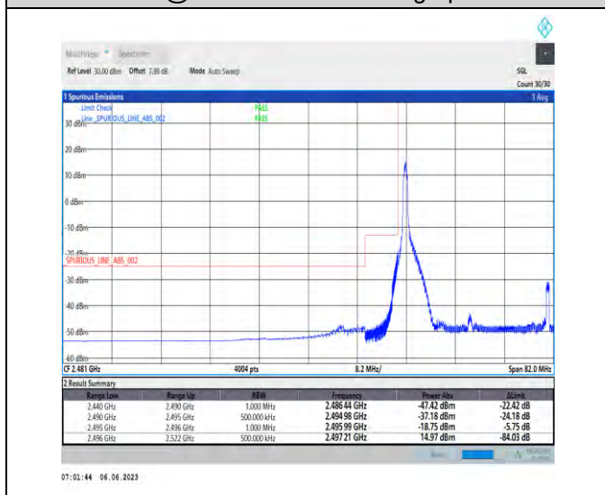
1-N41-PC3-30-50-L-4-CP-QPSK-Edge_1RB_Left-1@0-Ant1-1--PASS-see graph
