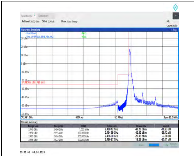
1-N41-PC3-30-15-L-1-DFT-PI2BPSK-Edge_1RB_Left-1@0-Ant1-1--PASS-see graph
