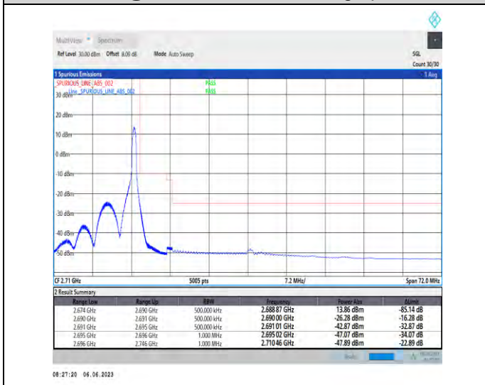
1-N41-PC3-30-90-H-5-CP-QPSK-Edge_1RB_Right-1@244-Ant1-1--PASS-see graph
