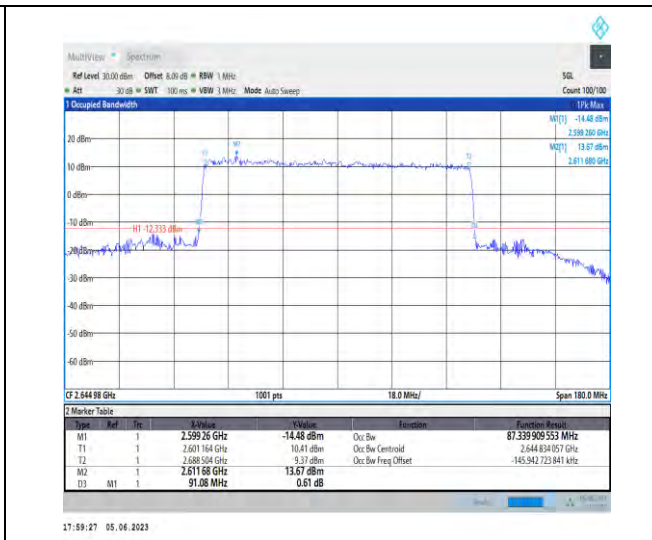
1-N41-PC3-30-90-H-8-CP-64QAM-Outer_Full-245 @0-Ant1-87.34-91.080-≤90-PASS
