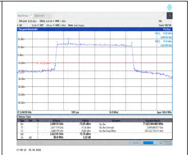
1-N41-PC3-30-80-H-3-DFT-16QAM-Outer_Full-216 @0-Ant1-77.025-80.800-<80-PASS
