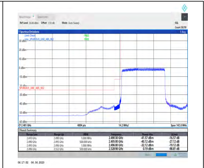
1-N41-PC3-30-40-L-3-DFT-PI2BPSK-Outer_Full-100@0-Ant1-1--PASS-see graph
