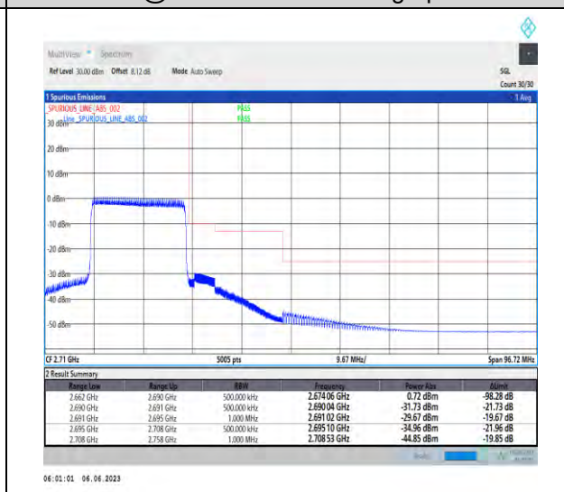
1-N41-PC3-30-20-H-6-CP-QPSK-Outer_Full-51@0-Ant1-1--PASS-see graph
