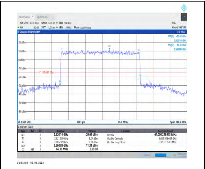
1-N41-PC3-30-70-H-3-DFT-16QAM-Outer_Full-180 @0-Ant1-64.66.360-<=70-PASS
