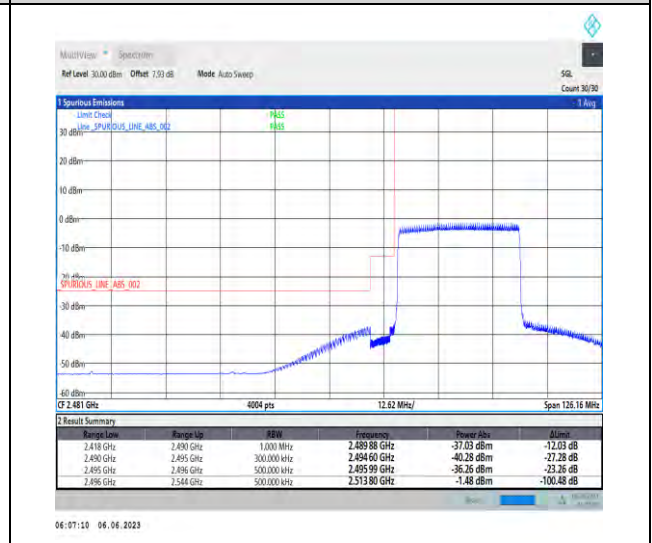
1-N41-PC3-30-30-L-6-CP-QPSK-Outer_Full-78@0-Ant1-1--PASS-see graph
