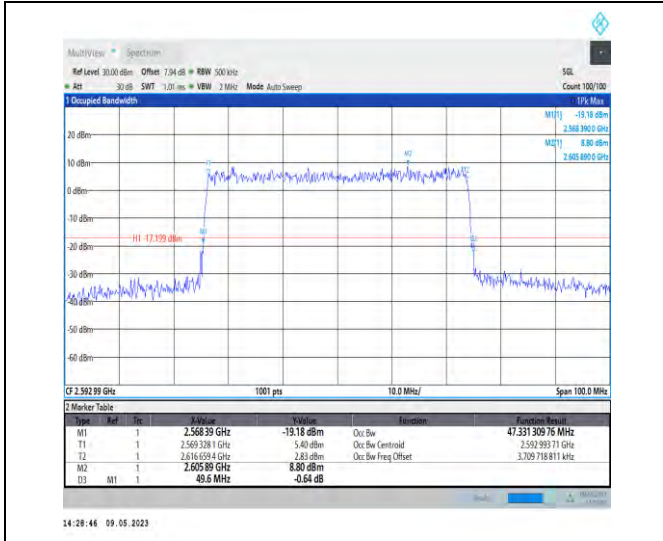
1-N41-PC3-30-50-M-9-CP-256QAM-Outer_Full-133 @0-Ant1-47.331-49.600-<50-PASS
