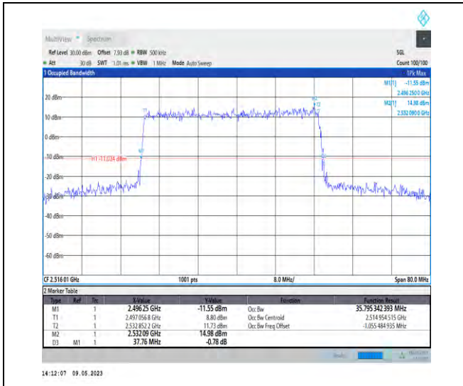
1-N41-PC3-30-40-L-1-DFT-QPSK-Outer_Full-100@ 0-Ant1-35.795-37.760-<40-PASS
