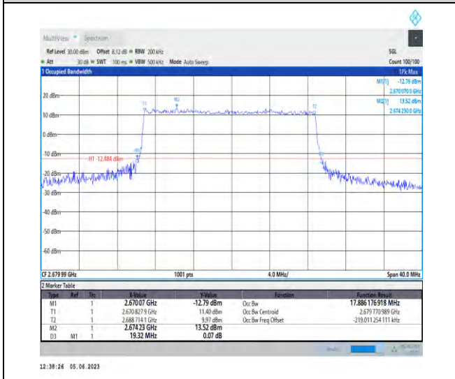
1-N41-PC3-30-20-H-3-DFT-16QAM-Outter_Full-50@ 0-Ant1-17.886-19.320-<20-PASS
