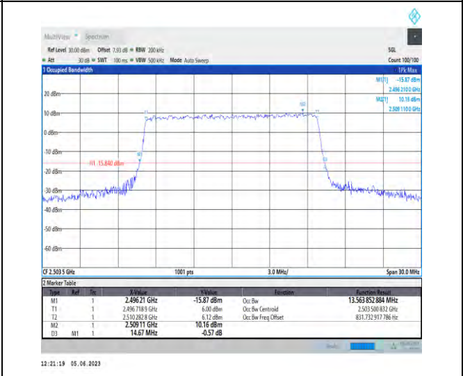
1-N41-PC3-30-15-L-9-CP-256QAM-Outer_Full-38@0-Ant1-13.564-14.670-≤15-PASS
