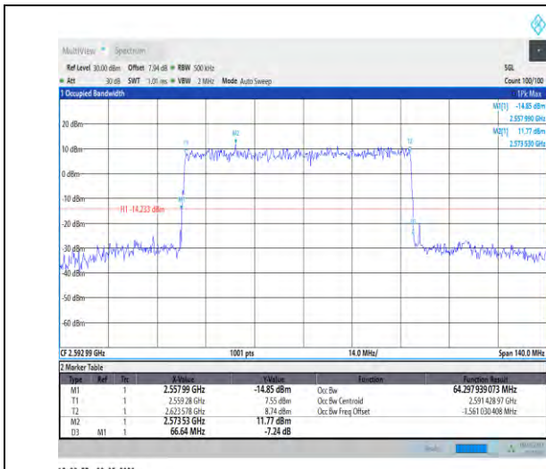
1-N41-PC3-30-70-M-3-DFT-16QAM-Outer_Full-180 @0-Ant1-64.298-66.640-<70-PASS
