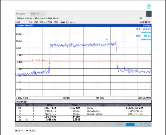
1-N41-PC3-30-60-M-9-CP-256QAM-Outer_Full-162 @0-Ant1-57.895-59.880-≤60-PASS
