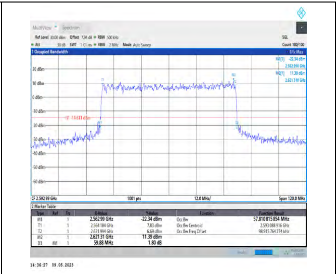
1-N41-PC3-30-60-M-7-CP-16QAM-Outer_Full-162@0-Ant1-57.811-59.880-≤60-PASS
