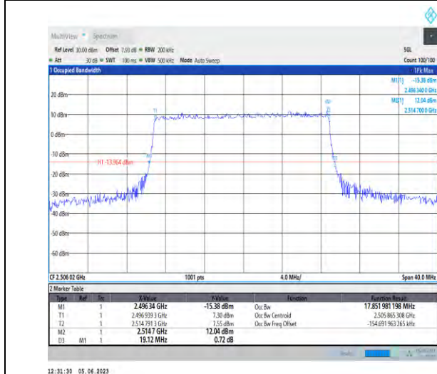
1-N41-PC3-30-20-L-5-DFT-256QAM-Outer_Full-50@0-Ant1-17.852-19.120-≤20-PASS
