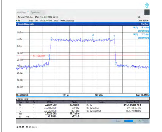
1-N41-PC3-30-50-M-7-CP-16QAM-Outer_Full-133@ 0-Ant1-47.425-49.800-<50-PASS
