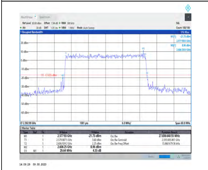
1-N41-PC3-30-30-M-9-CP-256QAM-Outer_Full-78@0 0-Ant1-27.837-29.640-≤30-PASS
