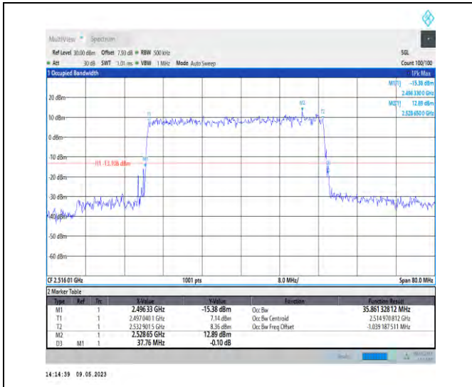
1-N41-PC3-30-40-L-5-DFT-256QAM-Outer_Full-100 @0-Ant1-35.861-37.760-<40-PASS
