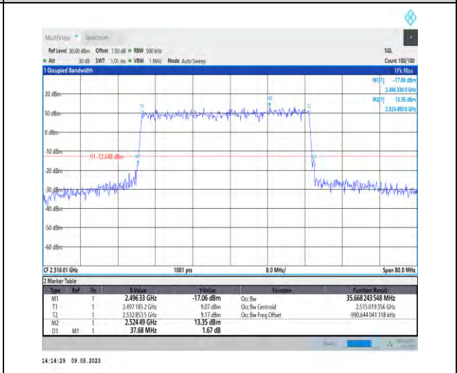
1-N41-PC3-30-40-L-4-DFT-64QAM-Outer_Full-100 @0-Ant1-35.668-37.680-<40-PASS
