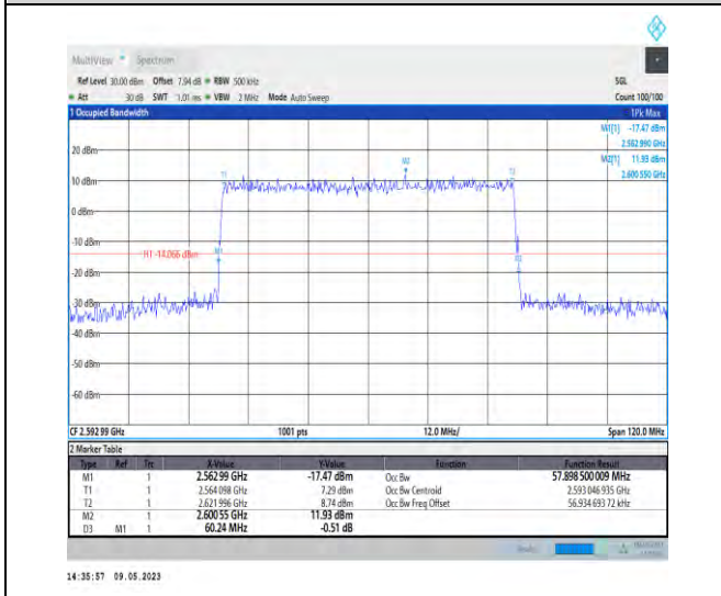
1-N41-PC3-30-60-M-4-DFT-64QAM-Outer_Full-162 @0-Ant1-57.899-60.240-<60-PASS
