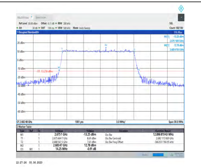
1-N41-PC3-30-15-H-5-DFT-256QAM-Outer_Full-36 @0-Ant1-12.897-14.250-≤15-PASS
