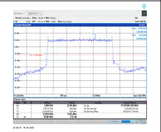
1-N41-PC3-30-60-L-2-DFT-PI2BPSK-Outer_Full-162 @0-Ant1-57.68-59.880-<=60-PASS
