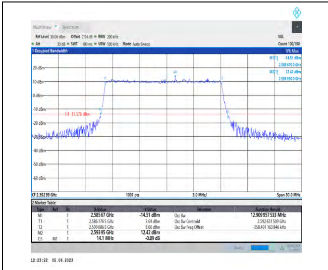
1-N41-PC3-30-15-M-5-DFT-256QAM-Outer_Full-36 @0-Ant1-12.91-14.100-≤15-PASS
