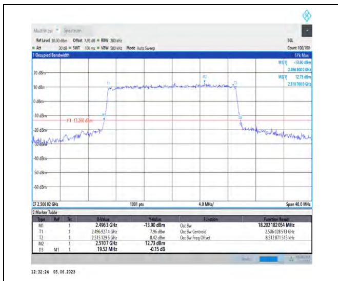
1-N41-PC3-30-20-L-7-CP-16QAM-Outer_Full-51@0-Ant1-18.202-19.520-≤20-PASS
