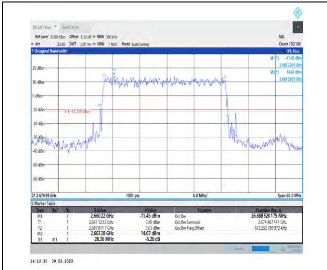
1-N41-PC3-30-30-H-2-DFT-PI2BPSK-Outer_Full-75 @0-Ant1-26.689-28.260-<30-PASS
