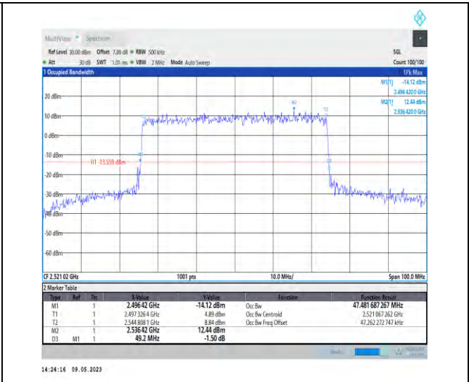
1-N41-PC3-30-50-L-7-CP-16QAM-Outer_Full-133@0 -Ant1-47.482-49.200-≤50-PASS
