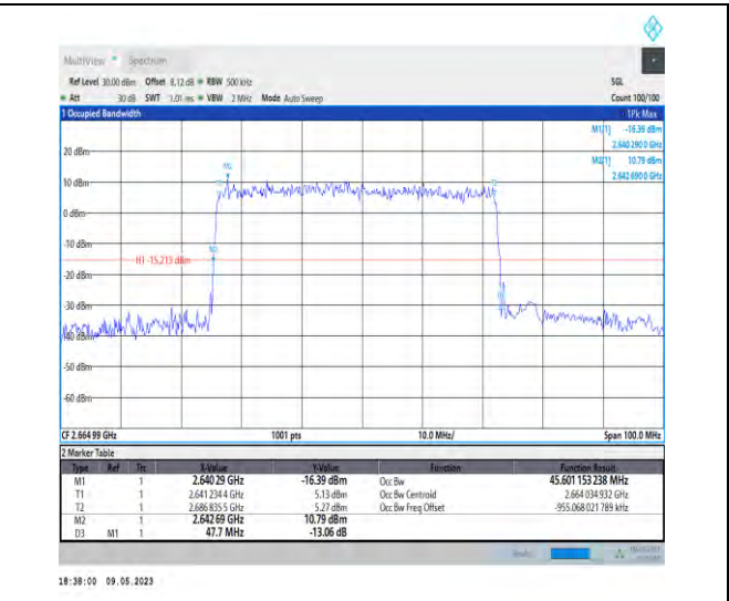
1-N41-PC3-30-50-H-5-DFT-256QAM-Outer_Full-128 @0-Ant1-45.601-47.700-<=50-PASS
