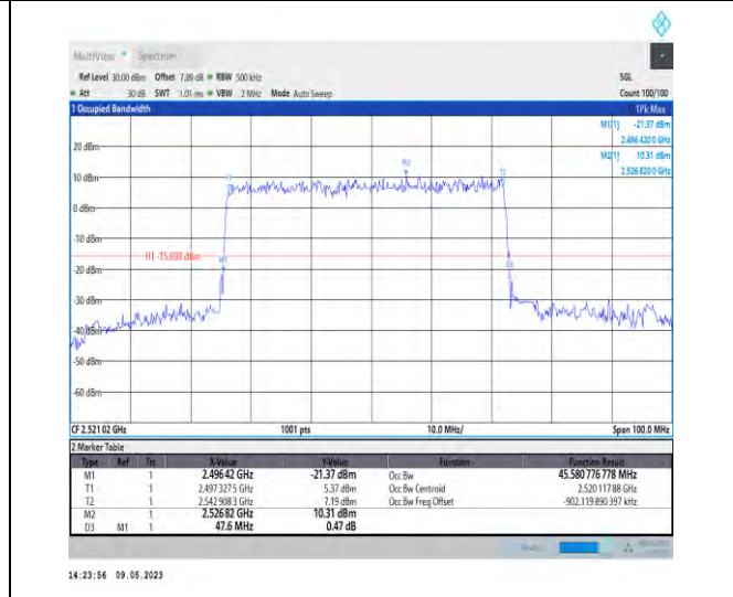
1-N41-PC3-30-50-L-5-DFT-256QAM-Outer_Full-128 @0-Ant1-45.581-47.600-≤50-PASS
