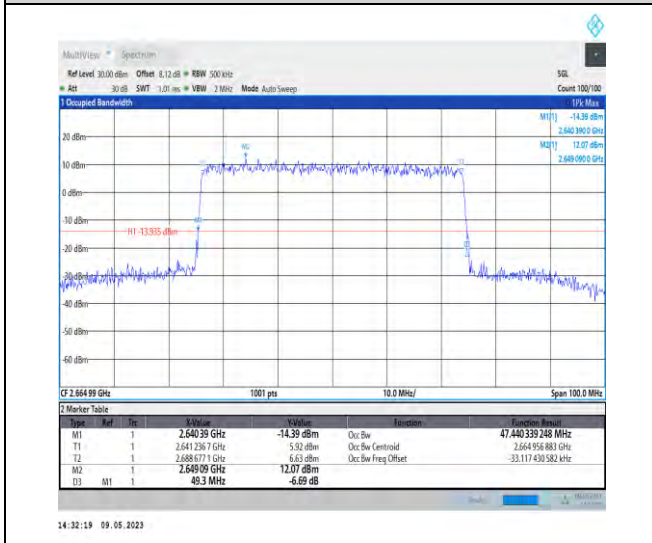
1-N41-PC3-30-50-H-6-CP-QPSK-Outer_Full-133@0 -Ant1-47.44-49.300-<=50-PASS
