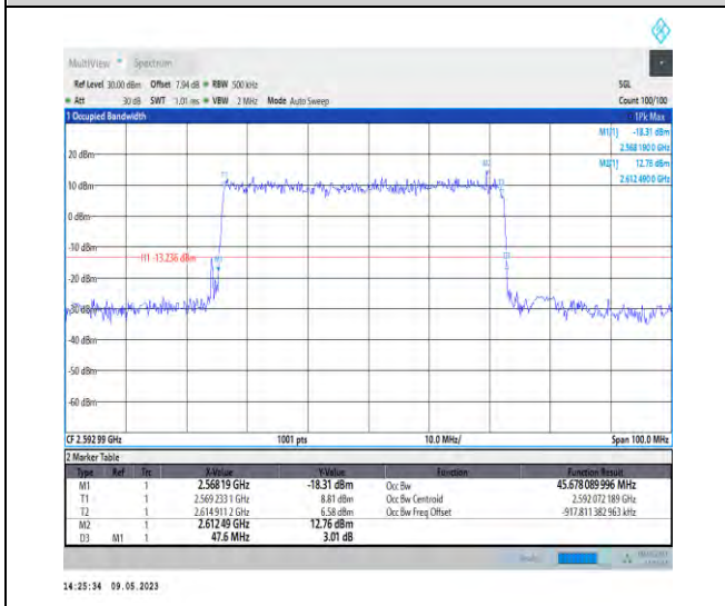
1-N41-PC3-30-50-M-3-DFT-16QAM-Outer_Full-128 @0-Ant1-45.678-47.600-≤50-PASS
