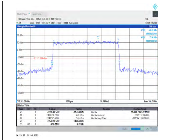
1-N41-PC3-30-50-L-3-DFT-16QAM-Outer_Full-128 @0-Ant1-45.667-47.600-≤50-PASS
