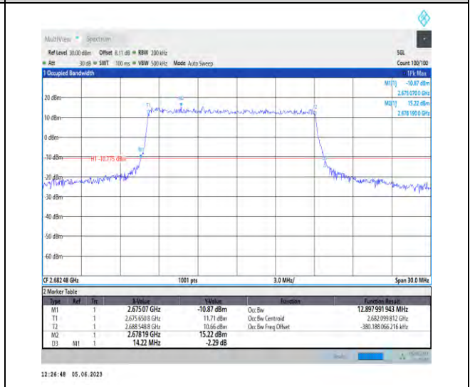
1-N41-PC3-30-15-H-3-DFT-16QAM-Outer_Full-36@ 0-Ant1-12.898-14.220-≤15-PASS
