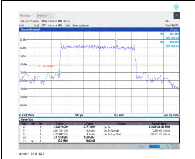
1-N41-PC3-30-50-H-2-DFT-PI2BPSK-Outer_Full-128 @0-Ant1-45.682-47.900-<50-PASS
