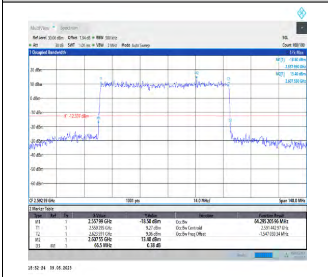
1-N41-PC3-30-70-M-1-DFT-QPSK-Outer_Full-180 @0-Ant1-64.295-66.500-<math>\leq 70</math>-PASS
