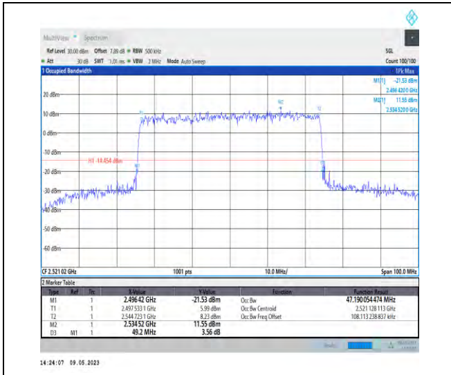
1-N41-PC3-30-50-L-6-CP-QPSK-Outer_Full-133@0 -Ant1-47.19-49.200-≤50-PASS
