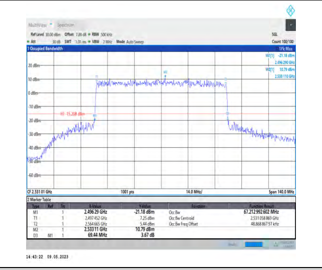
1-N41-PC3-30-70-L-7-CP-16QAM-Outer_Full-189@0 -Ant1-67.213-69.440-<=70-PASS
