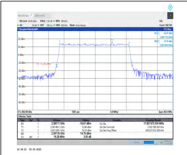
1-N41-PC3-30-20-M-2-DFT-PI2BPSK-Outer_Full-50 @0-Ant1-17.838-19.280-<=20-PASS
