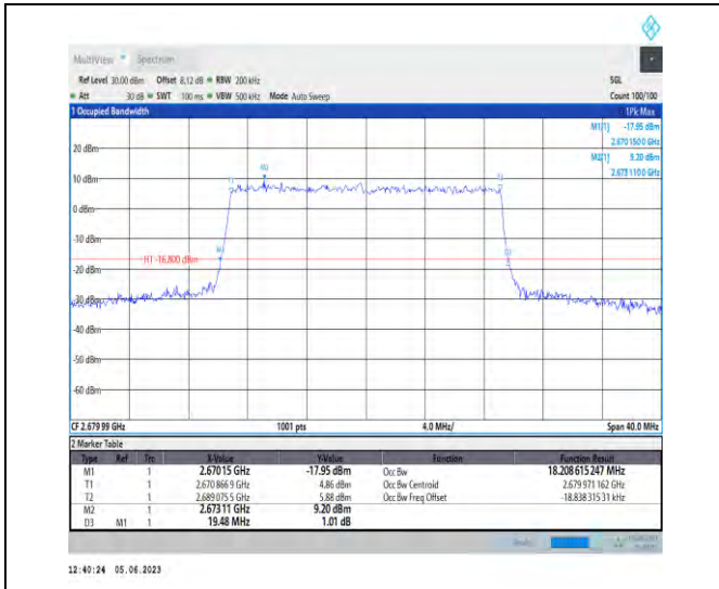
1-N41-PC3-30-20-H-9-CP-256QAM-Outer_Full-51@ 0-Ant1-18.209-19.480-<20-PASS
