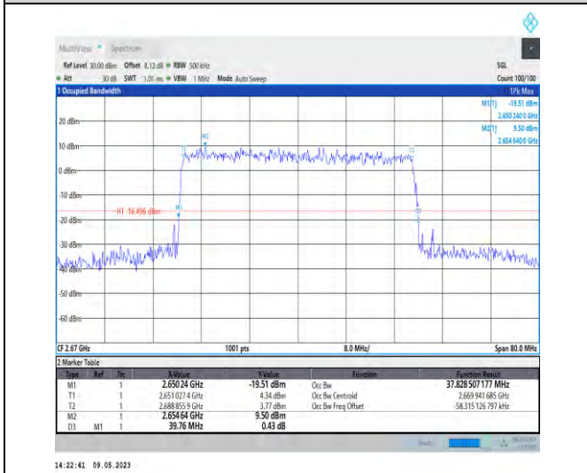
1-N41-PC3-30-40-H-9-CP-256QAM-Outer_Full-106@ @0-Ant1-37.829-39.760-<40-PASS
