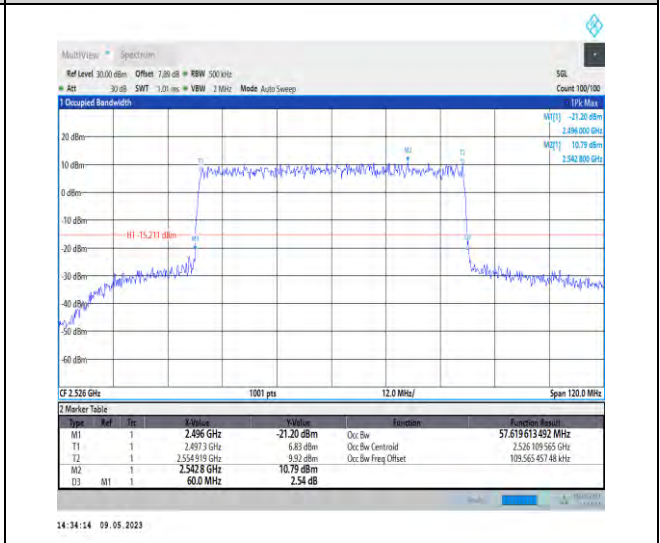
1-N41-PC3-30-60-L-6-CP-QPSK-Outer_Full-162@0 -Ant1-57.62-60.000-≤60-PASS
