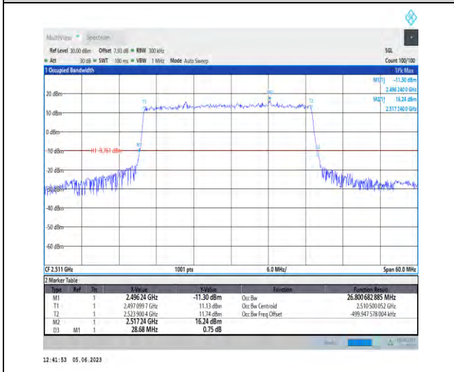
1-N41-PC3-30-30-L-2-DFT-PI2BPSK-Outer_Full-75 @0-Ant1-26.801-28.680-<30-PASS
