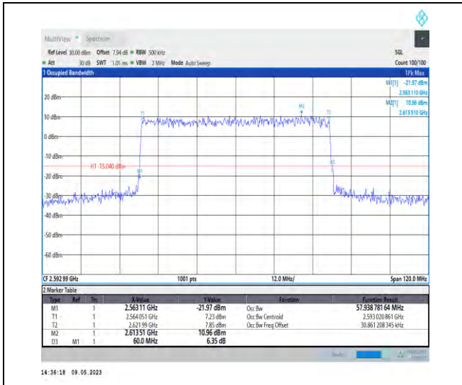
1-N41-PC3-30-60-M-6-CP-QPSK-Outer_Full-162@0 -Ant1-57.939-60.000-≤60-PASS
