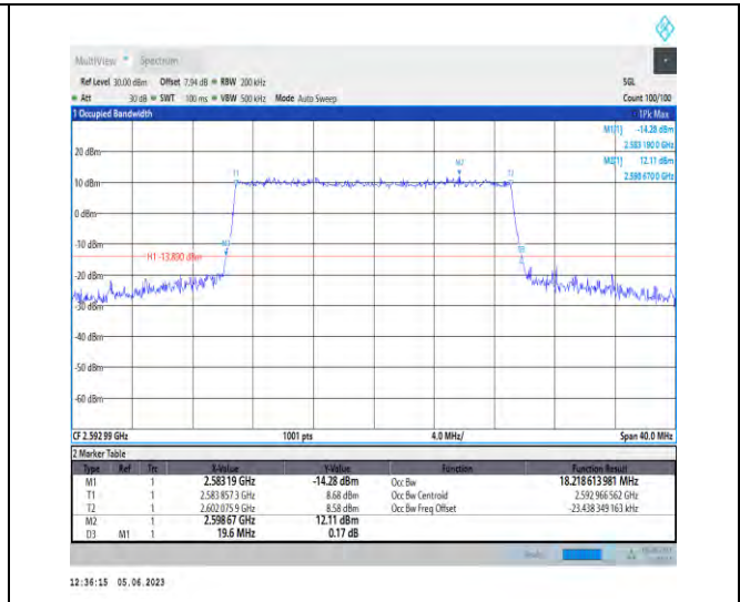
1-N41-PC3-30-20-M-7-CP-16QAM-Outer_Full-51@0-Ant1-18.219-19.600-≤20-PASS
