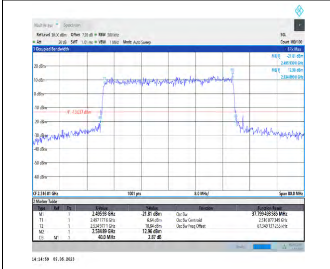
1-N41-PC3-30-40-L-7-CP-16QAM-Outer_Full-106@0-Ant1-37.799-40.000-<40-PASS
