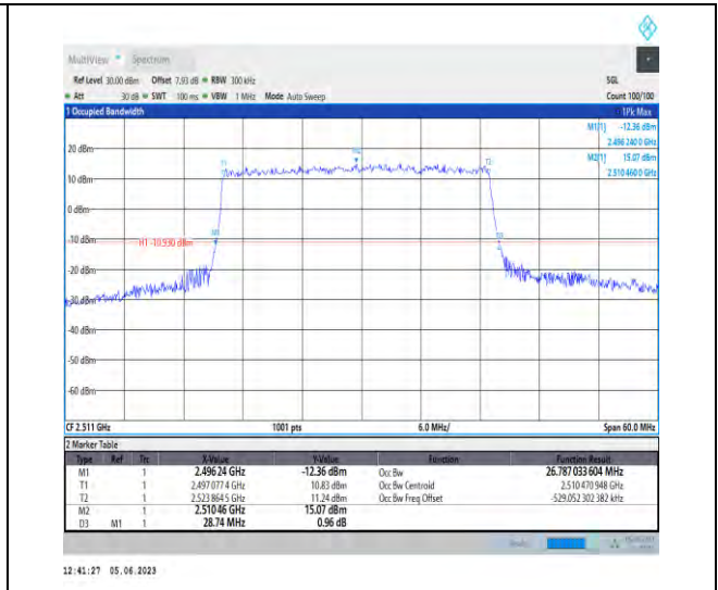
1-N41-PC3-30-30-L-1-DFT-QPSK-Outer_Full-75@0 -Ant1-26.787-28.740-<30-PASS
