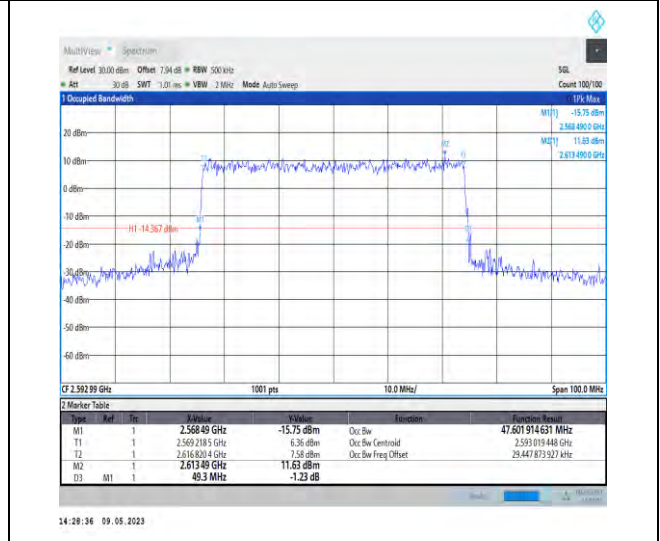
1-N41-PC3-30-50-M-8-CP-64QAM-Outer_Full-133 @0-Ant1-47.602-49.300-<50-PASS
