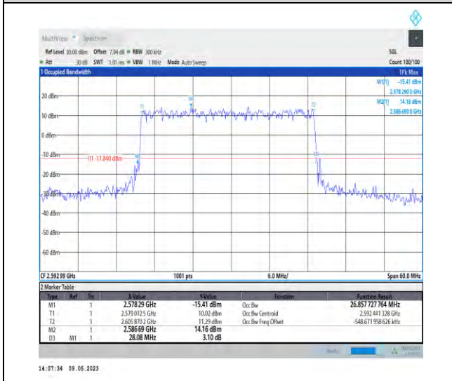
1-N41-PC3-30-30-M-1-DFT-QPSK-Outer_Full-75@ 0-Ant1-26.858-28.080-≤30-PASS
