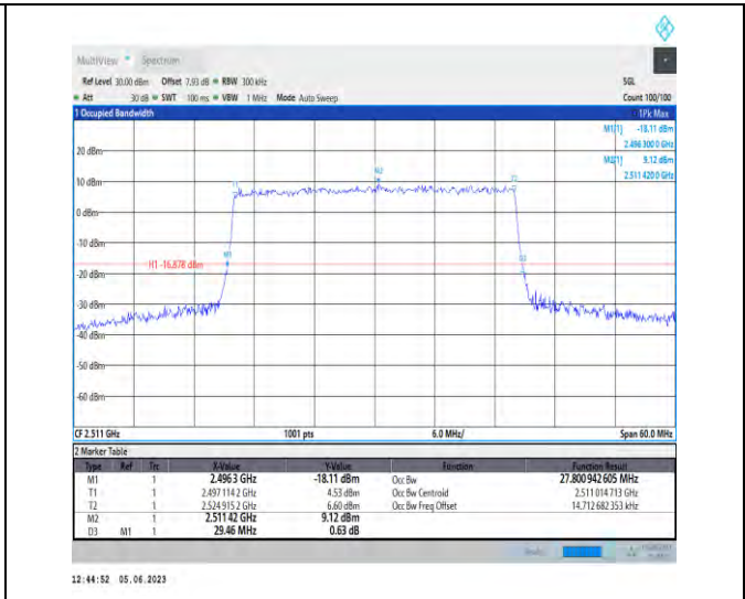
1-N41-PC3-30-30-L-9-CP-256QAM-Outer_Full-78@ -Ant1-27.801-29.460-≤30-PASS
