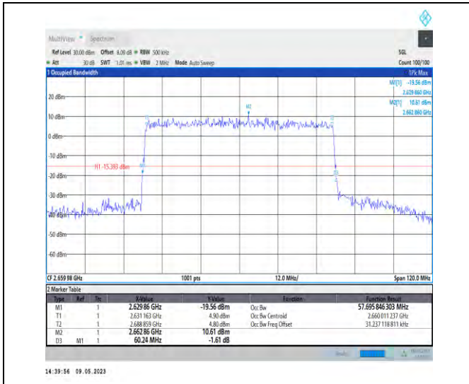
1-N41-PC3-30-60-H-5-DFT-256QAM-Outer_Full-162 @0-Ant1-57.696-60.240-≤60-PASS
