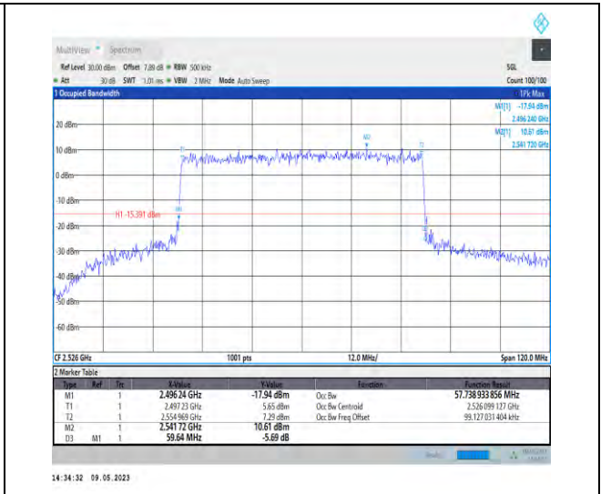
1-N41-PC3-30-60-L-8-CP-64QAM-Outer_Full-162@0 0-Ant1-57.739-59.640-≤60-PASS
