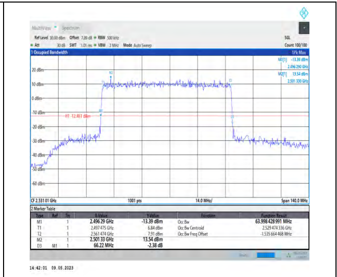
1-N41-PC3-30-70-L-1-DFT-QPSK-Outer_Full-180@ 0-Ant1-63.998-66.220-<=70-PASS
