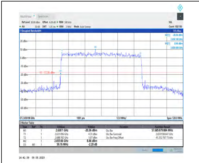
1-N41-PC3-30-60-H-9-CP-256QAM-Outer_Full-162 @0-Ant1-57.686-59.760-<=60-PASS
