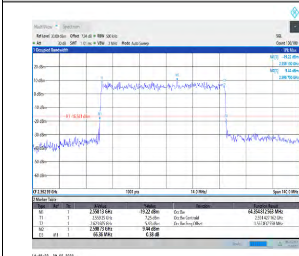
1-N41-PC3-30-70-M-5-DFT-256QAM-Outer_Full-180 @0-Ant1-64.355-66.360-<70-PASS
