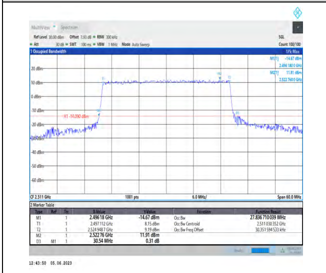
1-N41-PC3-30-30-L-6-CP-QPSK-Outer_Full-78@0- Ant1-27.837-30.540-≤30-PASS
