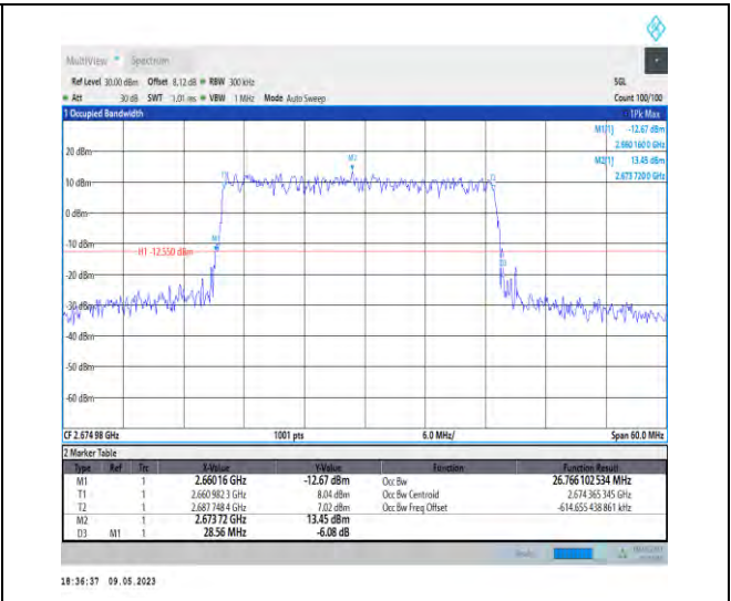
1-N41-PC3-30-30-H-3-DFT-16QAM-Outer_Full-75 @0-Ant1-26.766-28.560-<30-PASS
