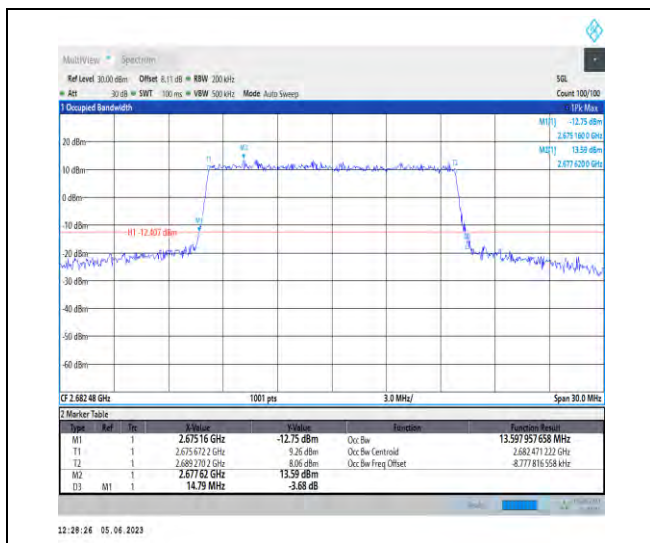
1-N41-PC3-30-15-H-8-CP-64QAM-Outer_Full-38@ -Ant1-13.598-14.790-≤15-PASS
