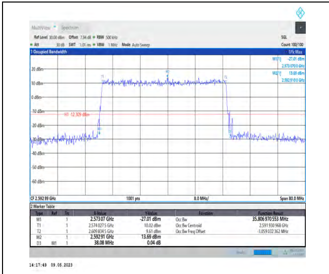
1-N41-PC3-30-40-M-4-DFT-64QAM-Outer_Full-100 @0-Ant1-35.807-38.080-<40-PASS
