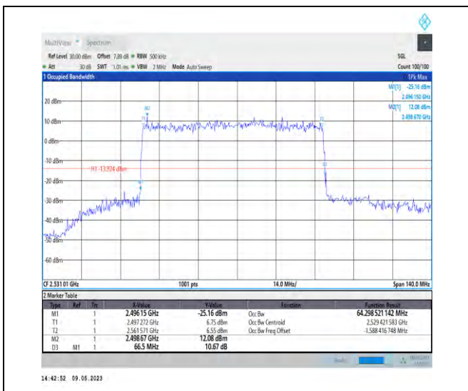
1-N41-PC3-30-70-L-4-DFT-64QAM-Outer_Full-180 @0-Ant1-64.299-66.500-<=70-PASS
