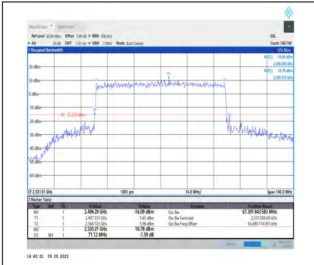
1-N41-PC3-30-70-L-8-CP-64QAM-Outer_Full-189 @0-Ant1-67.392-71.120-<math>\leq 70</math>-PASS
