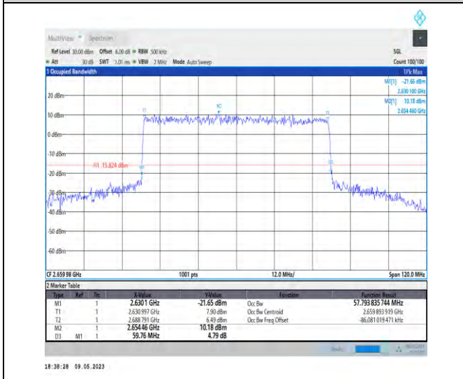
1-N41-PC3-30-60-H-7-CP-16QAM-Outer_Full-162 @0-Ant1-57.794-59.760-≤60-PASS
