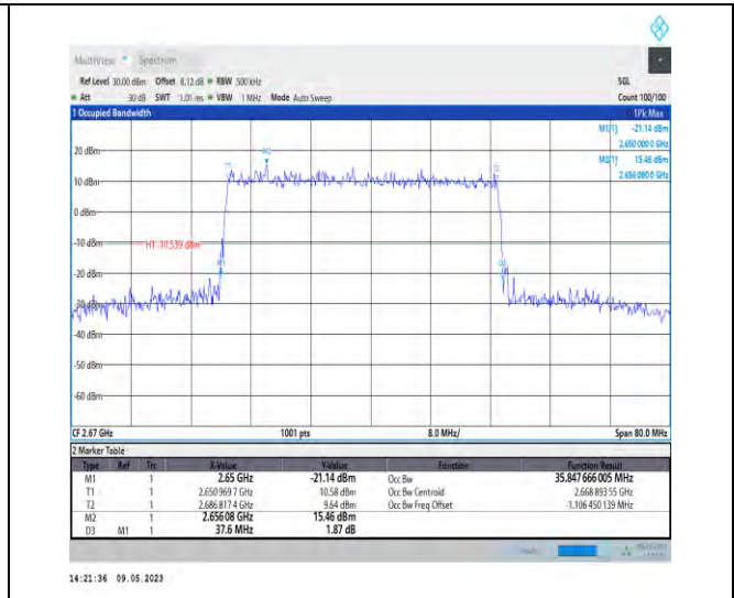
1-N41-PC3-30-40-H-4-DFT-64QAM-Outer_Full-100 @0-Ant1-35.848-37.600-<40-PASS
