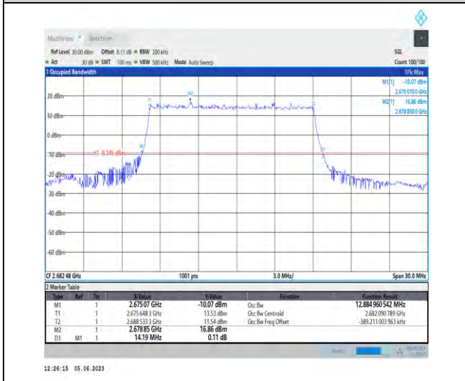
1-N41-PC3-30-15-H-2-DFT-PI2BPSK-Outer_Full-36@ 0-Ant1-12.885-14.190-≤15-PASS
