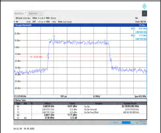
1-N41-PC3-30-30-H-5-DFT-256QAM-Outer_Full-75 @0-Ant1-26.731-27.960-<30-PASS
