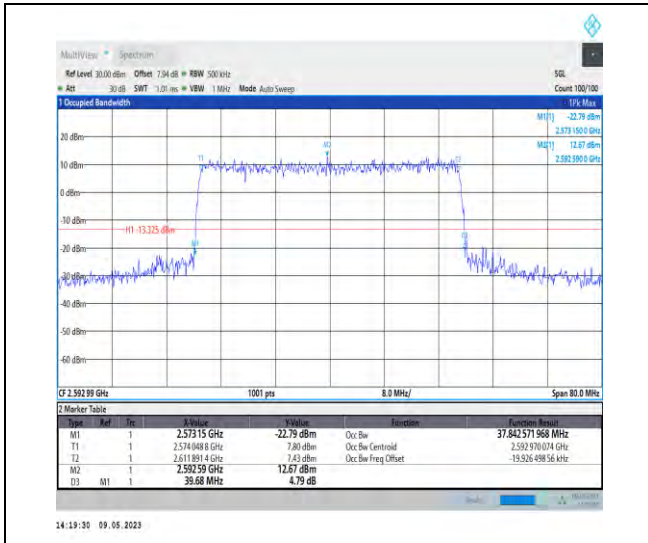
1-N41-PC3-30-40-M-8-CP-64QAM-Outer_Full-106 @0-Ant1-37.843-39.680-<40-PASS
