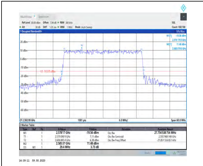
1-N41-PC3-30-30-M-7-CP-16QAM-Outer_Full-78@0 -Ant1-27.755-29.400-≤30-PASS
