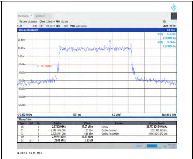
1-N41-PC3-30-30-M-4-DFT-64QAM-Outer_Full-75@ 0-Ant1-26.778-28.020-≤30-PASS
