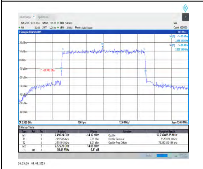
1-N41-PC3-30-60-L-1-DFT-QPSK-Outer_Full-162@ 0-Ant1-57.737-59.640-<=60-PASS
