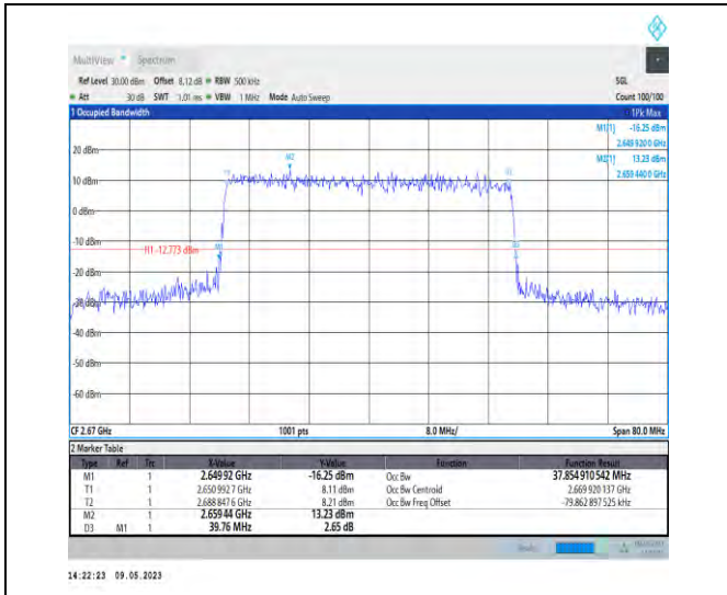
1-N41-PC3-30-40-H-7-CP-16QAM-Outer_Full-106@ 0-Ant1-37.855-39.760-<40-PASS
