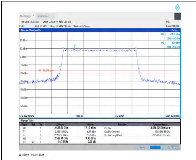
1-N41-PC3-30-15-M-9-CP-256QAM-Outer_Full-38@ 0-Ant1-13.569-14.700-≤15-PASS
