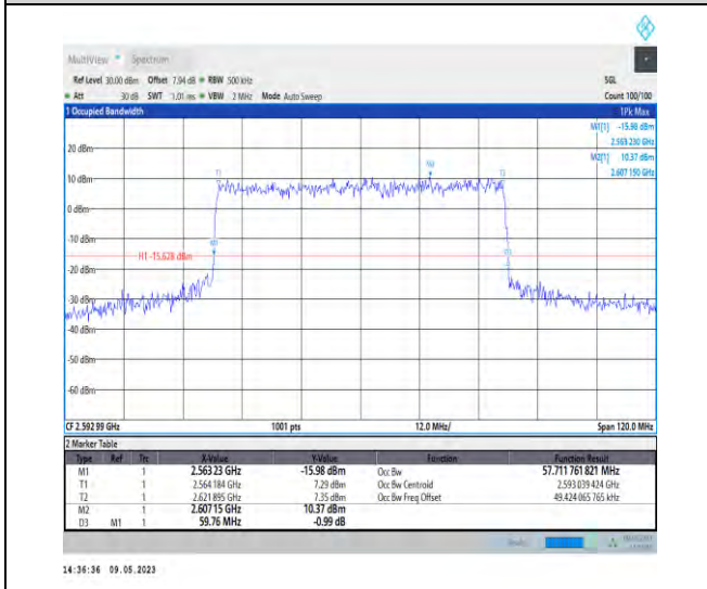
1-N41-PC3-30-60-M-8-CP-64QAM-Outer_Full-162 @0-Ant1-57.712-59.760-≤60-PASS
