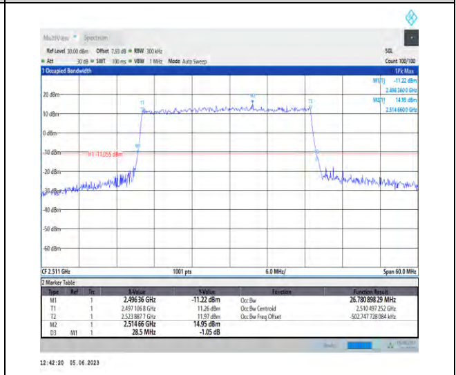
1-N41-PC3-30-30-L-3-DFT-16QAM-Outer_Full-75@ 0-Ant1-26.781-28.500-<30-PASS
