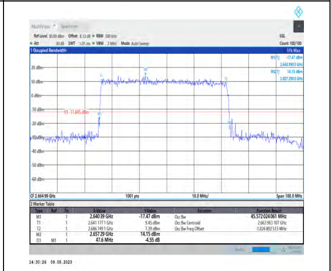
1-N41-PC3-30-50-H-3-DFT-16QAM-Outer_Full-128 @0-Ant1-45.572-47.600-<50-PASS
