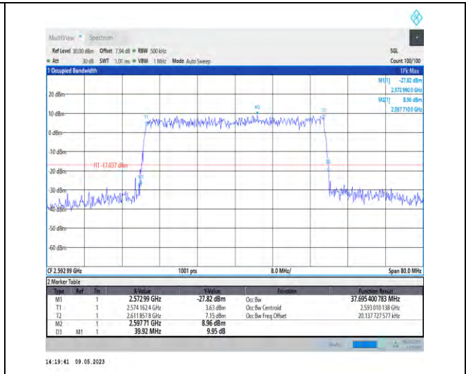
1-N41-PC3-30-40-M-9-CP-256QAM-Outer_Full-106 @0-Ant1-37.695-39.920-<40-PASS
