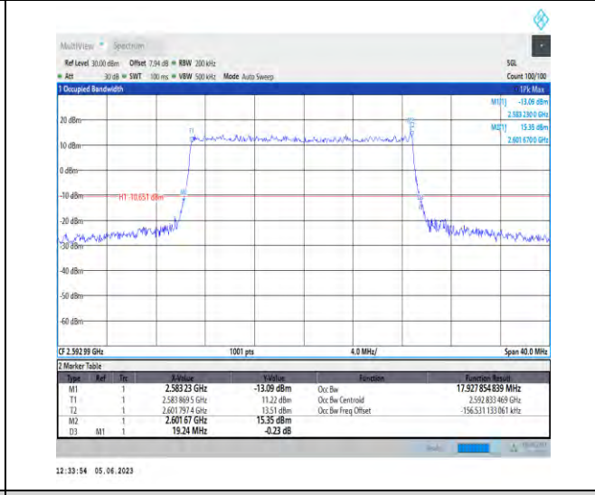
1-N41-PC3-30-20-M-1-DFT-QPSK-Outer_Full-50@0-Ant1-17.928-19.240-≤20-PASS
