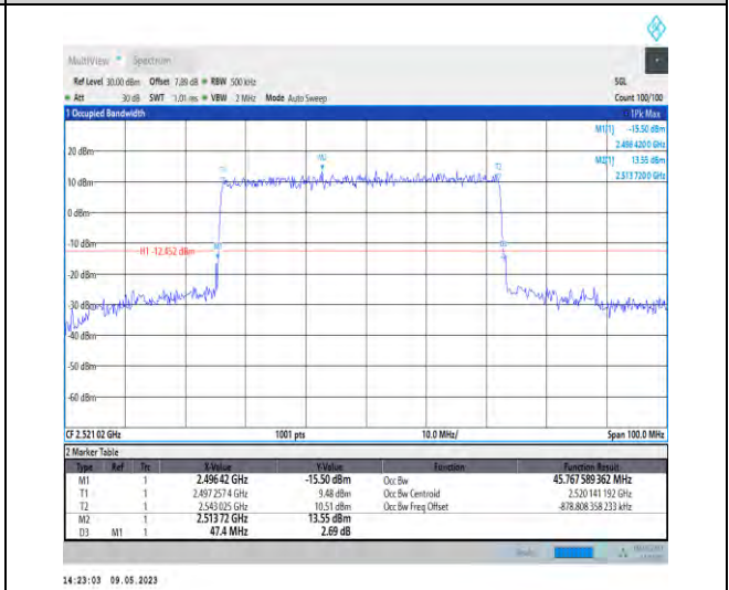
1-N41-PC3-30-50-L-1-DFT-QPSK-Outer_Full-128@ 0-Ant1-45.768-47.400-<50-PASS
