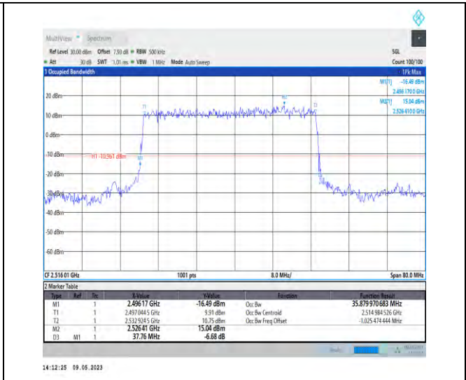
1-N41-PC3-30-40-L-2-DFT-PI2BPSK-Outer_Full-100 @0-Ant1-35.88-37.760-<40-PASS
