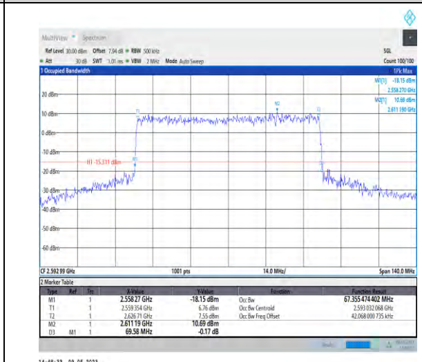
1-N41-PC3-30-70-M-6-CP-QPSK-Outer_Full-180@ 0-Ant1-67.355-69.580-<70-PASS
