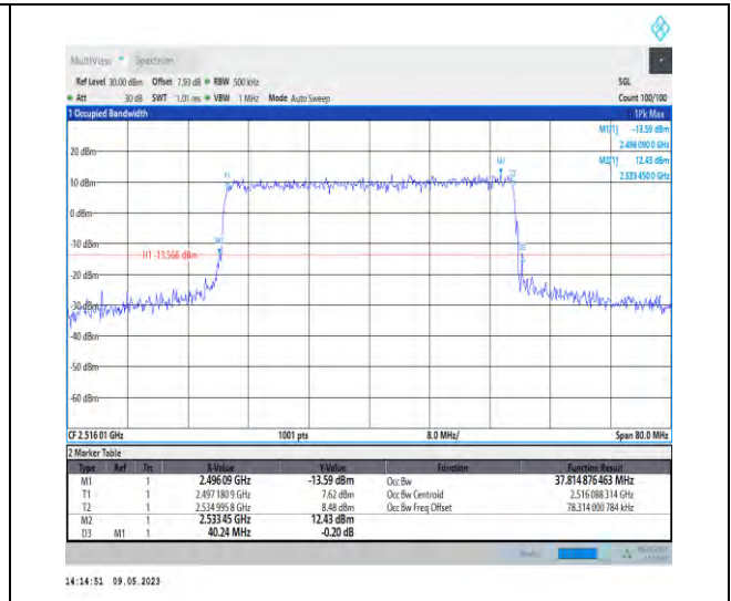
1-N41-PC3-30-40-L-6-CP-QPSK-Outer_Full-106@0-Ant1-37.815-40.240-<40-PASS
