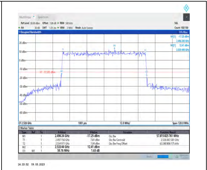
1-N41-PC3-30-60-L-4-DFT-64QAM-Outer_Full-162 @0-Ant1-57.816-59.760-≤60-PASS
