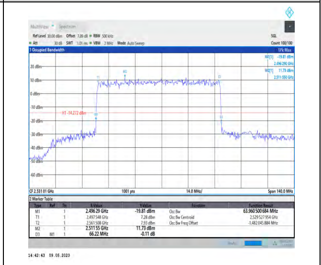
1-N41-PC3-30-70-L-3-DFT-16QAM-Outer_Full-180 @0-Ant1-63.961-66.220-<=70-PASS
