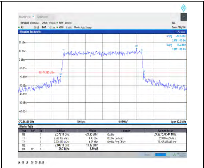
1-N41-PC3-30-30-M-8-CP-64QAM-Outer_Full-78@0 0-Ant1-27.828-29.700-≤30-PASS
