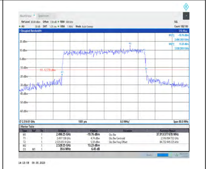
1-N41-PC3-30-40-L-8-CP-64QAM-Outer_Full-106@0-Ant1-37.913-39.600-<40-PASS
