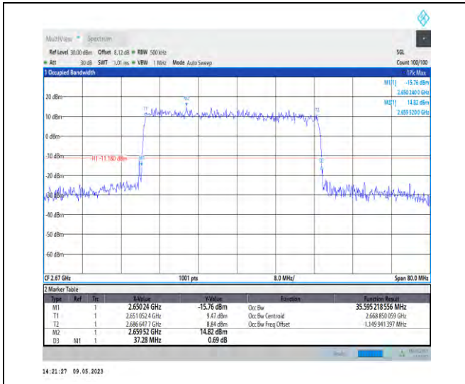
1-N41-PC3-30-40-H-3-DFT-16QAM-Outer_Full-100 @0-Ant1-35.595-37.280-<40-PASS
