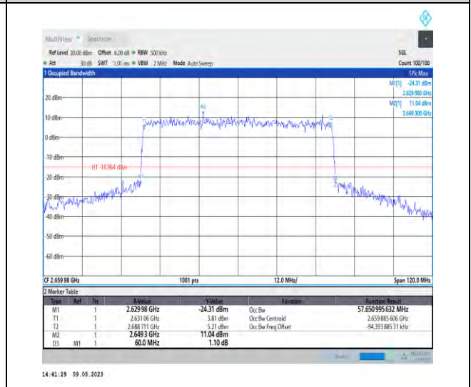
1-N41-PC3-30-60-H-8-CP-64QAM-Outer_Full-162 @0-Ant1-57.651-60.000-≤60-PASS
