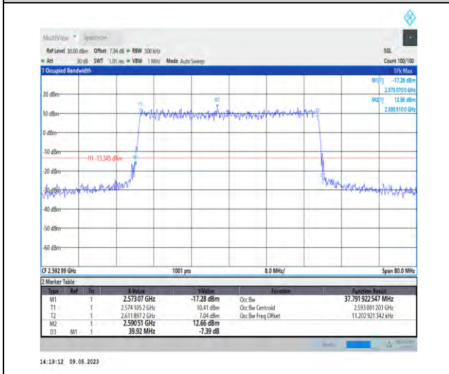
1-N41-PC3-30-40-M-6-CP-QPSK-Outer_Full-106@0 -Ant1-37.792-39.920-<40-PASS
