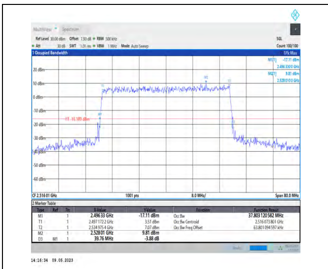
1-N41-PC3-30-40-L-9-CP-256QAM-Outer_Full-106@ 0-Ant1-37.803-39.760-<40-PASS
