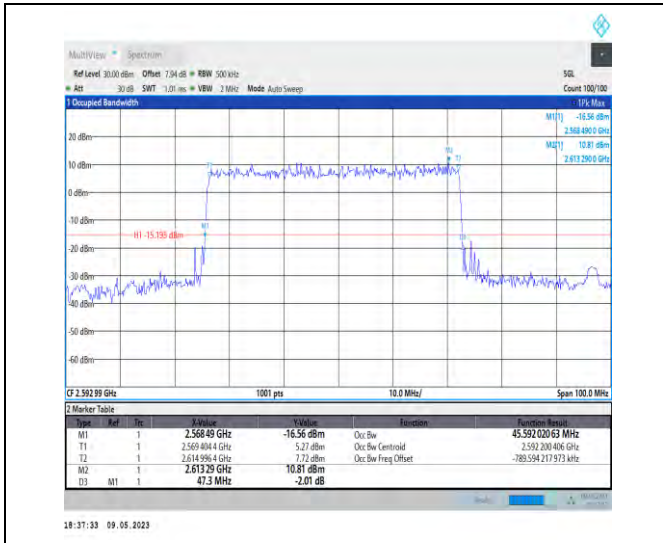
1-N41-PC3-30-50-M-5-DFT-256QAM-Outer_Full-128 @0-Ant1-45.592-47.300-<50-PASS
