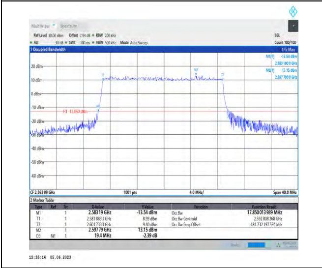
1-N41-PC3-30-20-M-4-DFT-64QAM-Outer_Full-50 @0-Ant1-17.85-19.400-<=20-PASS
