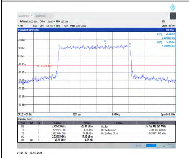
1-N41-PC3-30-40-L-3-DFT-16QAM-Outer_Full-100 @0-Ant1-35.762-37.760-<40-PASS
