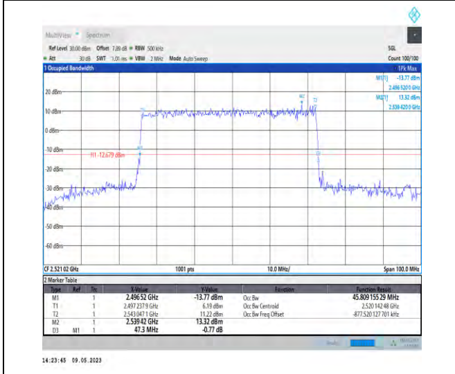
1-N41-PC3-30-50-L-4-DFT-64QAM-Outer_Full-128 @0-Ant1-45.809-47.300-≤50-PASS
