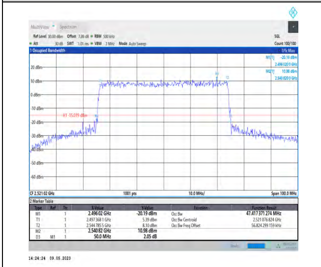
1-N41-PC3-30-50-L-8-CP-64QAM-Outer_Full-133@0 0-Ant1-47.417-50.000-≤50-PASS
