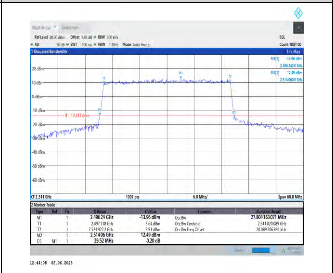
1-N41-PC3-30-30-L-7-CP-16QAM-Outer_Full-78@0- Ant1-27.804-29.520-≤30-PASS
