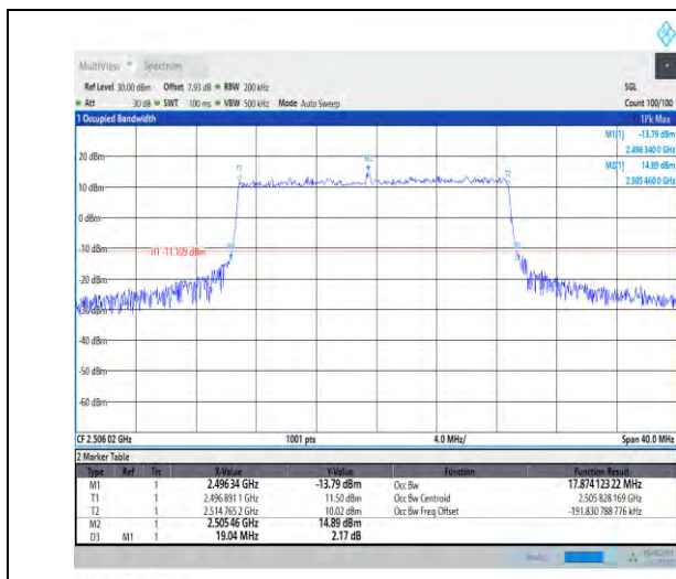
1-N41-PC3-30-20-L-3-DFT-16QAM-Outer_Full-50@0-Ant1-17.874-19.040-≤20-PASS
