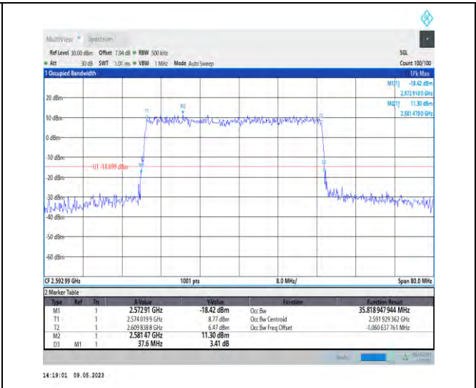
1-N41-PC3-30-40-M-5-DFT-256QAM-Outer_Full-100 @0-Ant1-35.819-37.600-<40-PASS
