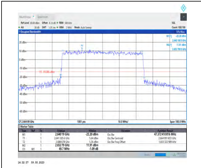
1-N41-PC3-30-50-H-8-CP-64QAM-Outer_Full-133@ 0-Ant1-47.372-49.700-<=50-PASS
