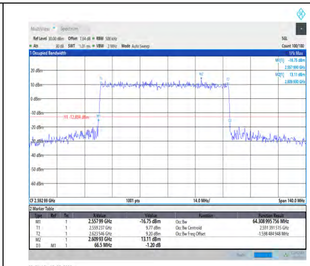
1-N41-PC3-30-70-M-4-DFT-64QAM-Outer_Full-180 @0-Ant1-64.309-66.50-<70-PASS
