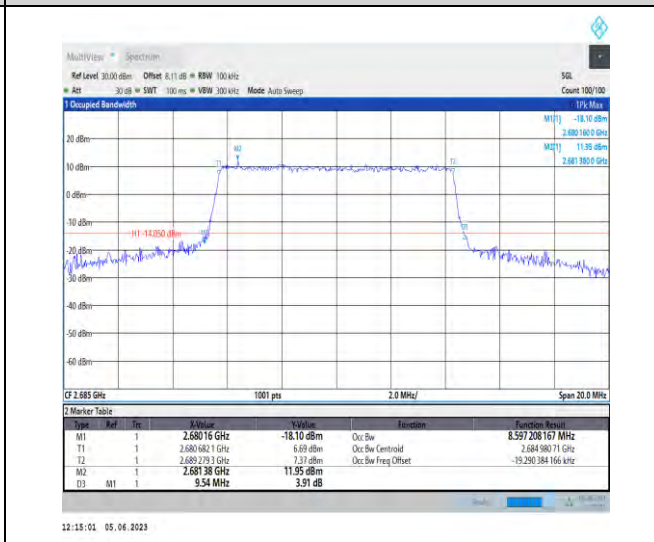
1-N41-PC3-30-10-H-6-CP-QPSK-Outer_Full-24@0-A nt1-8.597-9.540-<=10-PASS
