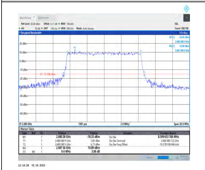
1-N41-PC3-30-10-H-5-DFT-256QAM-Outer_Full-24 @0-Ant1-8.6-9.400-<=10-PASS
