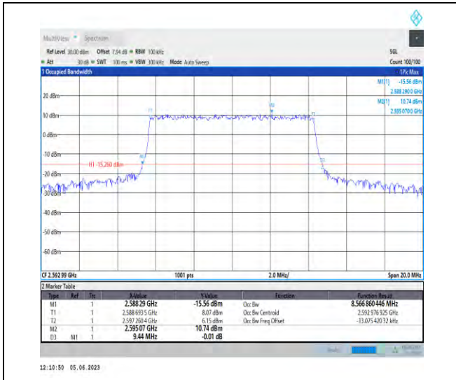
1-N41-PC3-30-10-M-8-CP-64QAM-Outer_Full-24@ 0-Ant1-8.567-9.440-≤10-PASS
