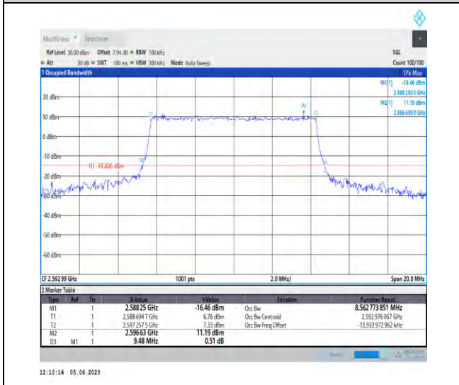
1-N41-PC3-30-10-M-6-CP-QPSK-Outer_Full-24@0- Ant1-8.563-9.480-≤10-PASS
