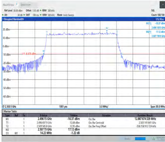
1-N41-PC3-30-15-L-2-DFT-PI2BPSK-Outer_Full-36 @0-Ant1-12.888-14.220-<=15-PASS
