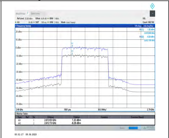
1-N41-PC3-30-100-H-2-CP-256QAM-Outer_Full-273 0@0-Ant1-9.60-100%-0.00-9.60-PASS-≤13
