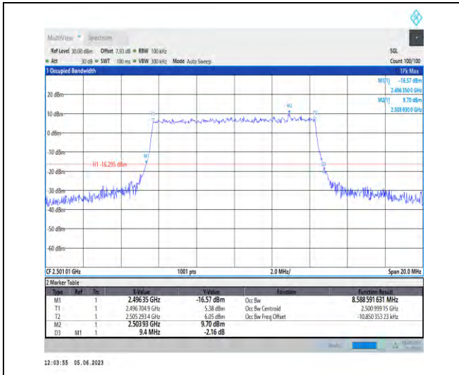
1-N41-PC3-30-10-L-9-CP-256QAM-Outer_Full-24@0 -Ant1-8.589-9.400-≤10-PASS
