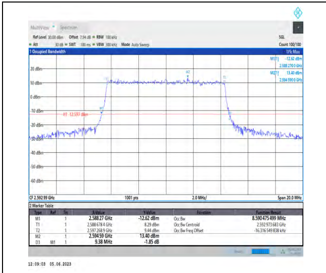
1-N41-PC3-30-10-M-4-DFT-64QAM-Outer_Full-24 @0-Ant1-8.59-9.380-≤10-PASS
