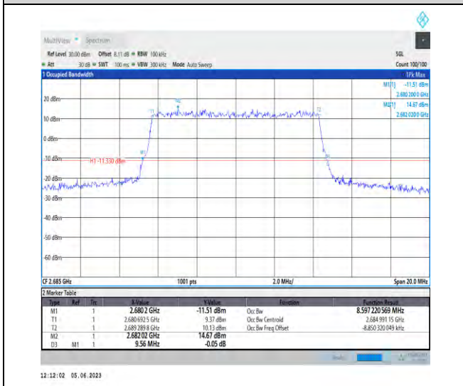
1-N41-PC3-30-10-H-1-DFT-QPSK-Outer_Full-24@0 -Ant1-8.597-9.560-≤10-PASS
