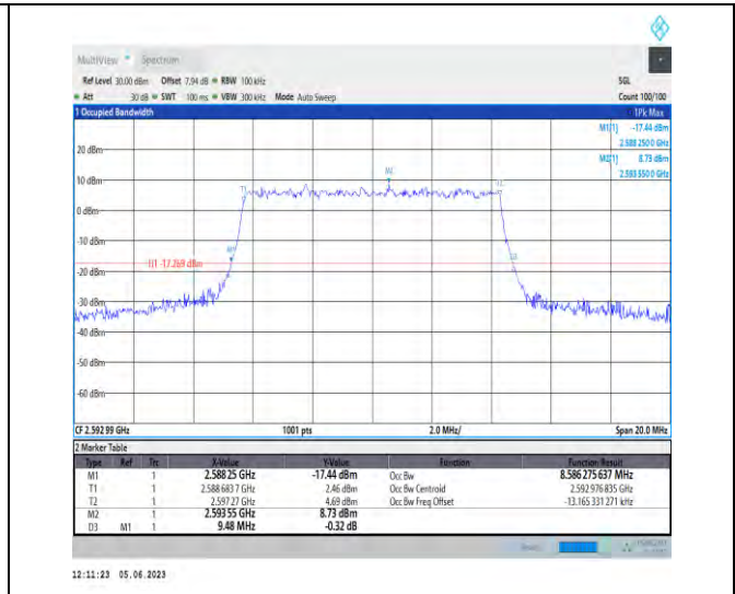
1-N41-PC3-30-10-M-9-CP-256QAM-Outer_Full-24@ 0-Ant1-8.586-9.480-≤10-PASS
