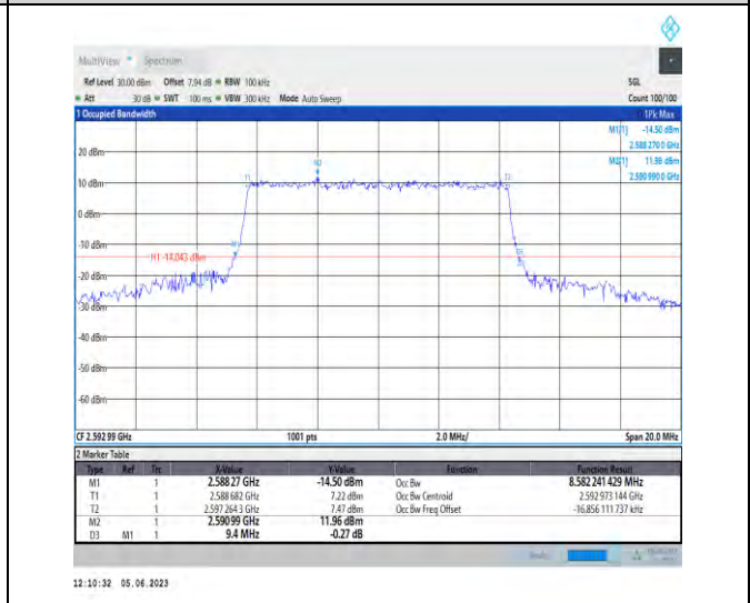
1-N41-PC3-30-10-M-7-CP-16QAM-Outer_Full-24@0- Ant1-8.582-9.400-≤10-PASS
