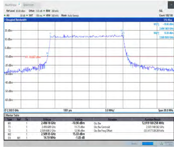
1-N41-PC3-30-15-L-3-DFT-16QAM-Outer_Full-36@ 0-Ant1-12.919-14.190-<=15-PASS
