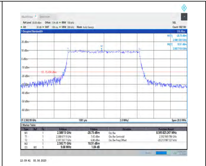
1-N41-PC3-30-10-M-5-DFT-256QAM-Outer_Full-24 @0-Ant1-8.596-9.680-≤10-PASS
