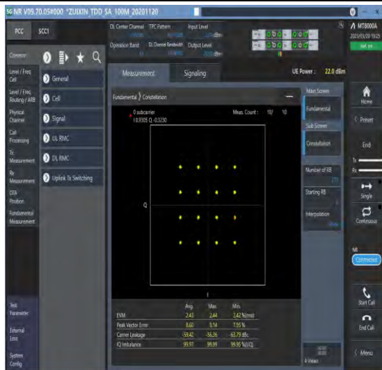
1-N41-30-100-M-7-CP-16QAM-Outer_Full-273@0-Ant1-see graph-PASS
