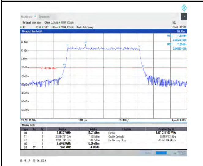
1-N41-PC3-30-10-M-2-DFT-PI2BPSK-Outer_Full-24 @0-Ant1-8.601-9.480-≤10-PASS
