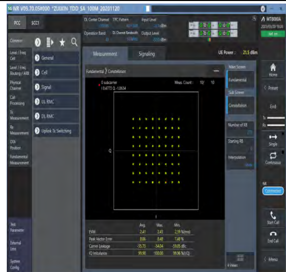
1-N41-30-100-M-8-CP-64QAM-Outer_Full-273@0-Ant1-see graph-PASS
