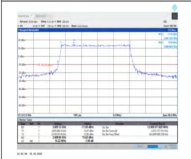
1-N38-PC3-30-15-H-3-DFT-16QAM-Outer_Full-36@ 0-Ant1-12.909-14.220-≤15-PASS
