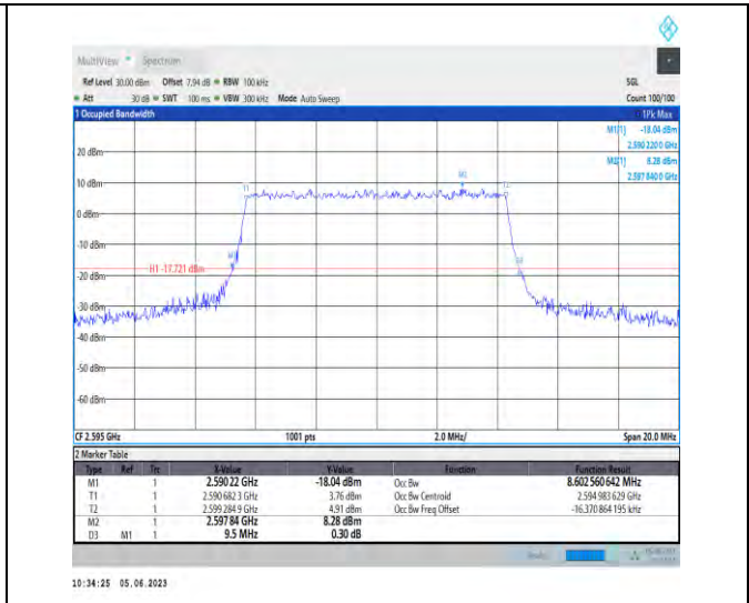
1-N38-PC3-30-10-M-9-CP-256QAM-Outer_Full-24@ 0-Ant1-8.603-9.500-≤10-PASS
