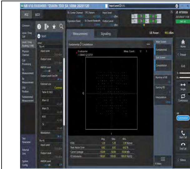
1-N38-PC3-30-20-M-5-DFT-256QAM-Outer_Full-50@0-Ant1-see graph-PASS
