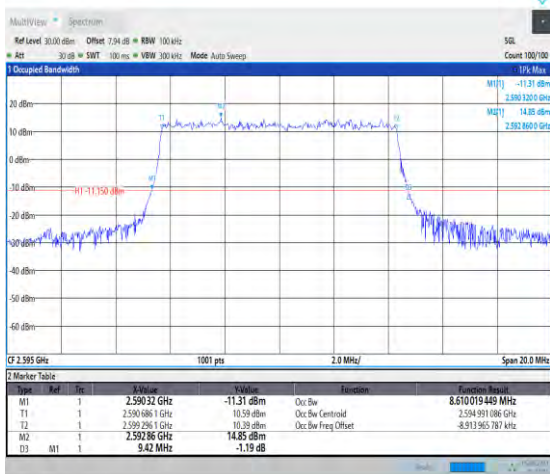
1-N38-PC3-30-10-M-2-DFT-PI2BPSK-Outer_Full-24 @0-Ant1-8.61-9.420-≤10-PASS
