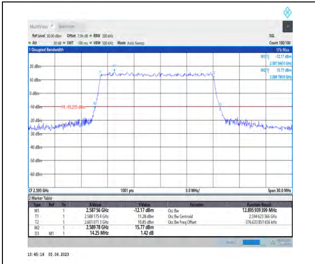
1-N38-PC3-30-15-M-1-DFT-QPSK-Outter_Full-36@0-Ant1-12.896-14.250-≤15-PASS
