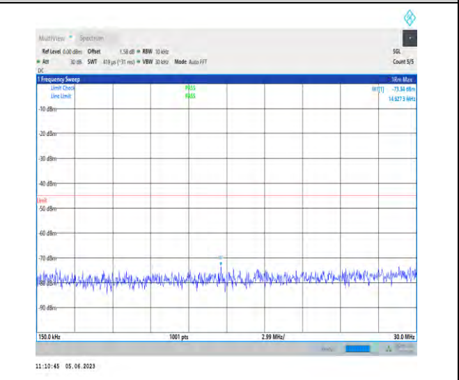
1-N38-PC3-30-20-M-1-N/A-DFT-PI2BPSK-Inner_1RB _Left-1@1-0.15-30-Ant1-14.63--73.34--45-PASS
