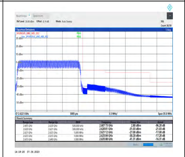
1-N38-PC3-30-15-H-6-CP-QPSK-Outer_Full-38@0-Ant1-1--PASS-see graph
