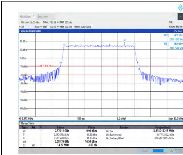
1-N38-PC3-30-15-L-2-DFT-PI2BPSK-Outer_Full-36 @0-Ant1-12.893-14.220-≤15-PASS
