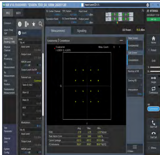
1-N38-PC3-30-20-M-7-CP-16QAM-Outer_Full-51@0-Ant1-see graph-PASS
