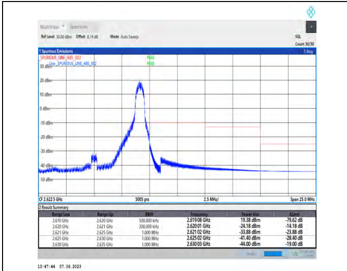
1-N38-PC3-30-10-H-2-DFT-PI2BPSK-Edge_1RB_Right-t-1@23-Ant1-1--PASS-see graph
