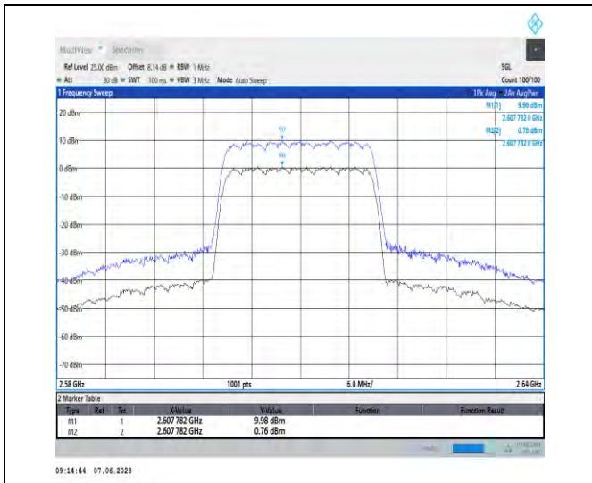
1-N38-PC3-30-20-H-1-DFT-256QAM-Outer_Full-50 @0-Ant1-9.22-100%-0.00-9.22-PASS≤13
