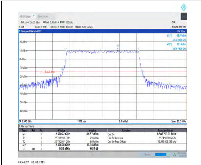
1-N38-PC3-30-10-L-5-DFT-256QAM-Outer_Full-24@0-Ant1-8.587-9.520-≤10-PASS
