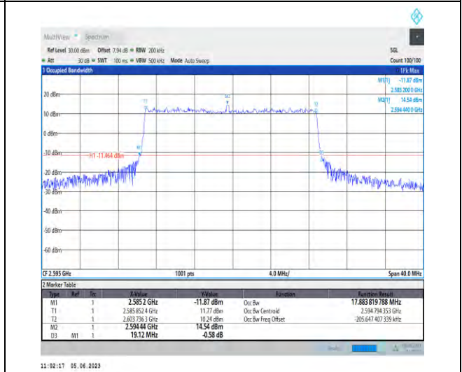
1-N38-PC3-30-20-M-3-DFT-16QAM-Outer_Full-50 @0-Ant1-17.884-19.120-<20-PASS
