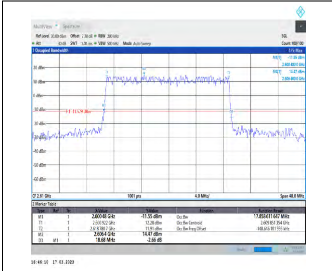
1-N38-PC3-30-20-H-3-DFT-16QAM-Outer_Full-50@ 0-Ant1-35.902-39.880-≤20-FAIL
