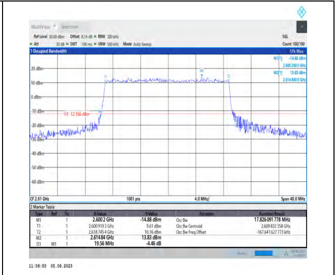
1-N38-PC3-30-20-H-4-DFT-64QAM-Outer_Full-50@ 0-Ant1-17.826-19.560-≤20-PASS
