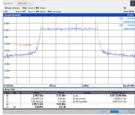
1-N38-PC3-30-10-M-1-DFT-QPSK-Outer_Full-24@ -Ant1-8.591-9.380-≤10-PASS
