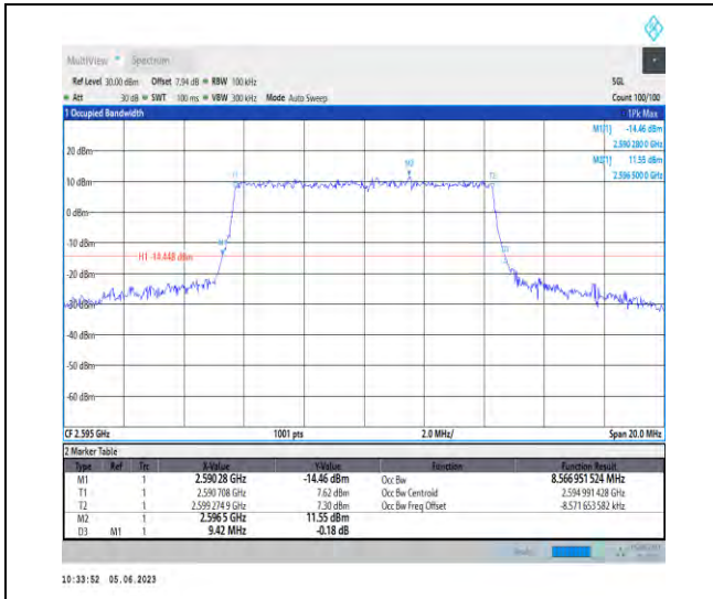
1-N38-PC3-30-10-M-8-CP-64QAM-Outer_Full-24@ 0-Ant1-8.567-9.420-≤10-PASS
