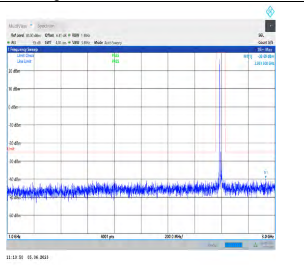
1-N38-PC3-30-20-M-1-N/A-DFT-PI2BPSK-Inner_1RB _Left-1@1-1000-3000-Ant1-2931.50--39.69--25-PASS S
