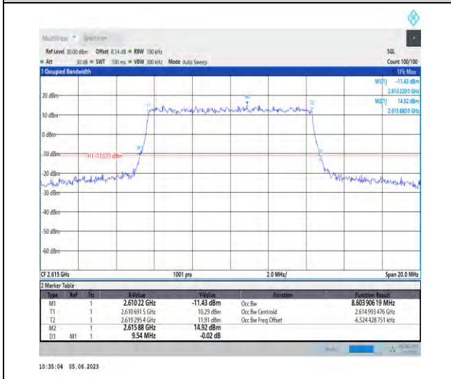
1-N38-PC3-30-10-H-1-DFT-QPSK-Outer_Full-24@ 0-Ant1-8.604-9.540-≤10-PASS
