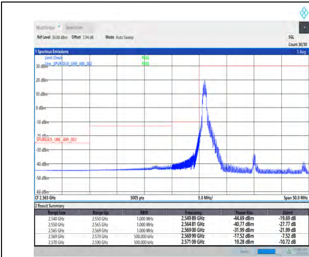
1-N38-PC3-30-20-L-1-DFT-PI2BPSK-Edge_1RB_Left-1@0-Ant1-1--PASS-see graph
