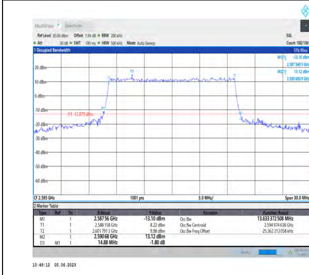
1-N38-PC3-30-15-M-7-CP-16QAM-Outer_Full-38@0- Ant1-13.633-14.880-≤15-PASS
