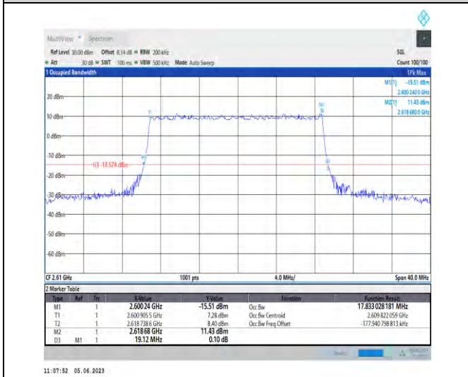
1-N38-PC3-30-20-H-5-DFT-256QAM-Outer_Full-50 @0-Ant1-17.833-19.120-≤20-PASS
