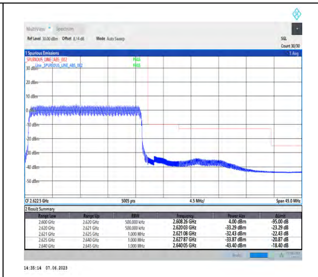
1-N38-PC3-30-20-H-3-DFT-PI2BPSK-Outer_Full-50@0-Ant1-1--PASS-see graph
