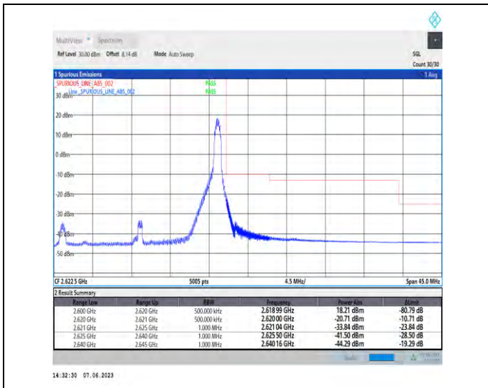
1-N38-PC3-30-20-H-2-DFT-PI2BPSK-Edge_1RB_Right-t-1@50-Ant1-1--PASS-see graph
