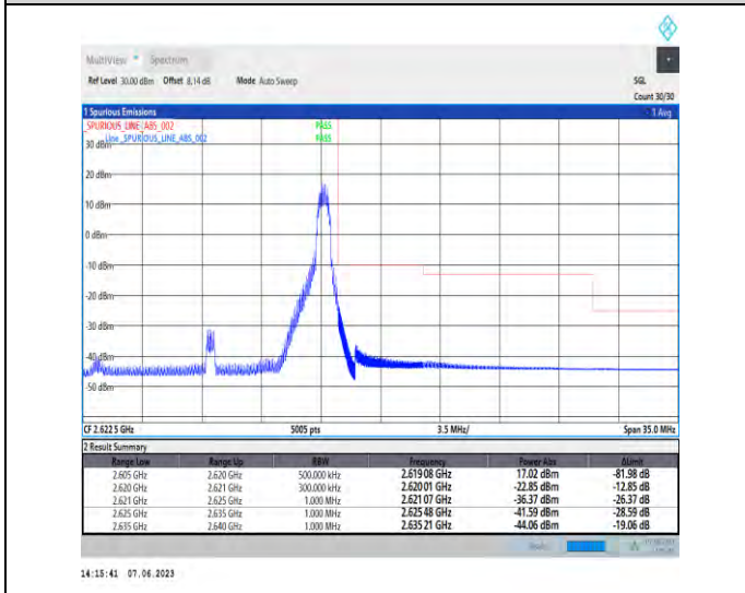
1-N38-PC3-30-15-H-5-CP-QPSK-Edge_1RB_Right-1@37-Ant1-1--PASS-see graph
