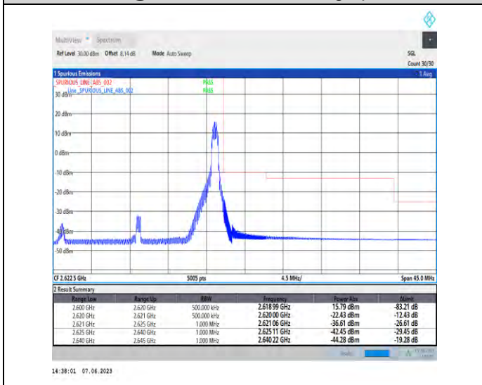
1-N38-PC3-30-20-H-5-CP-QPSK-Edge_1RB_Right-1@50-Ant1-1--PASS-see graph
