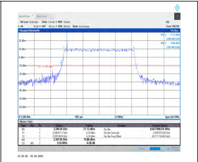
1-N38-PC3-30-10-M-5-DFT-256QAM-Outer_Full-24@ @0-Ant1-8.607-9.240-≤10-PASS
