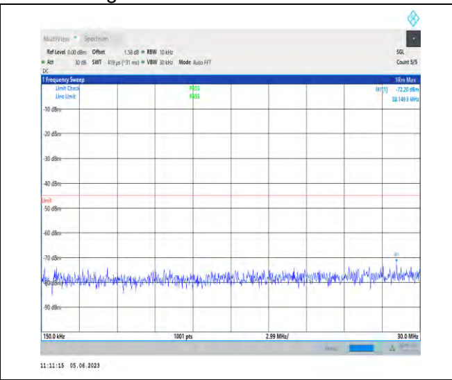
1-N38-PC3-30-20-H-1-N/A-DFT-PI2BPSK-Inner_1RB _Left-1@1-0.15-30-Ant1-28.15--72.20--45-PASS
