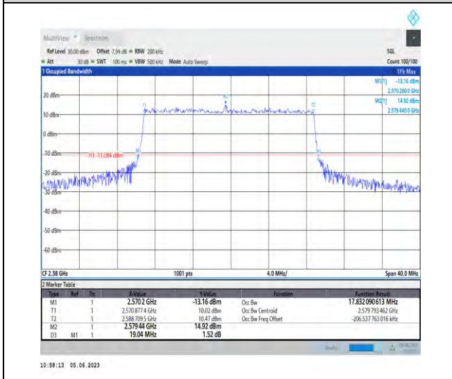
1-N38-PC3-30-20-L-3-DFT-16QAM-Outer_Full-50@ 0-Ant1-17.832-19.040-≤20-PASS
