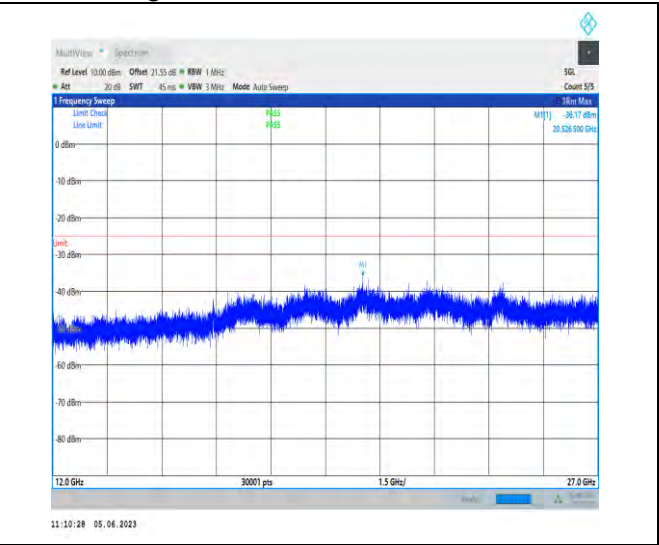
1-N38-PC3-30-20-L-1-N/A-DFT-PI2BPSK-Inner_1RB _Left-1@1-12000-27000-Ant1-20526.50--36.17--25-P ASS
