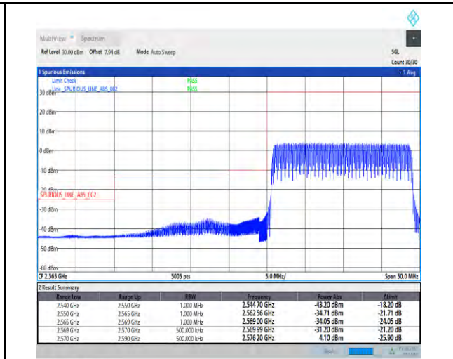
1-N38-PC3-30-20-L-3-DFT-PI2BPSK-Outer_Full-50@0-Ant1-1--PASS-see graph
