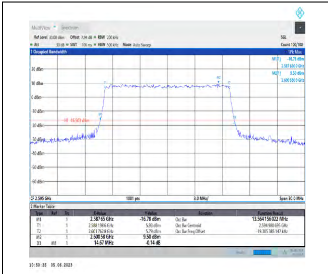
1-N38-PC3-30-15-M-9-CP-256QAM-Outer_Full-38 @0-Ant1-13.564-14.670-≤15-PASS
