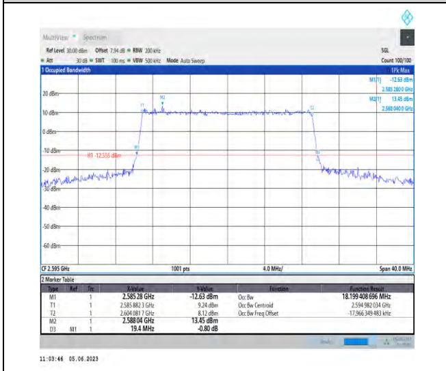
1-N38-PC3-30-20-M-6-CP-QPSK-Outer_Full-51@0- Ant1-18.199-19.400-≤20-PASS
