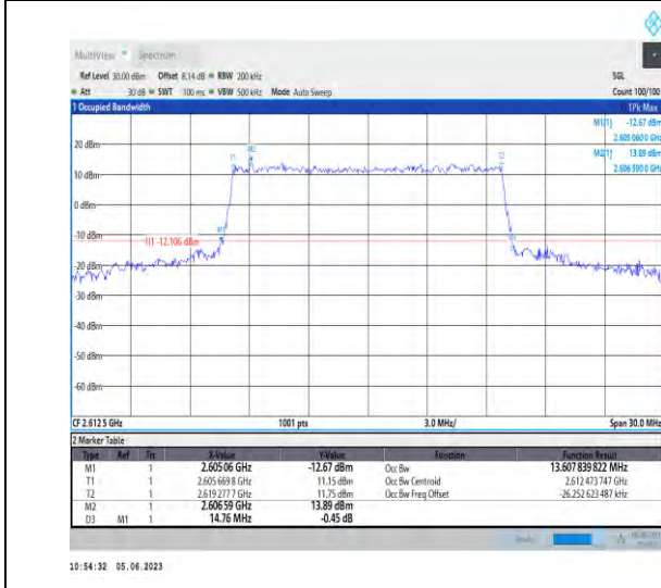
1-N38-PC3-30-15-H-7-CP-16QAM-Outer_Full-38@0-Ant1-13.608-14.760-≤15-PASS
