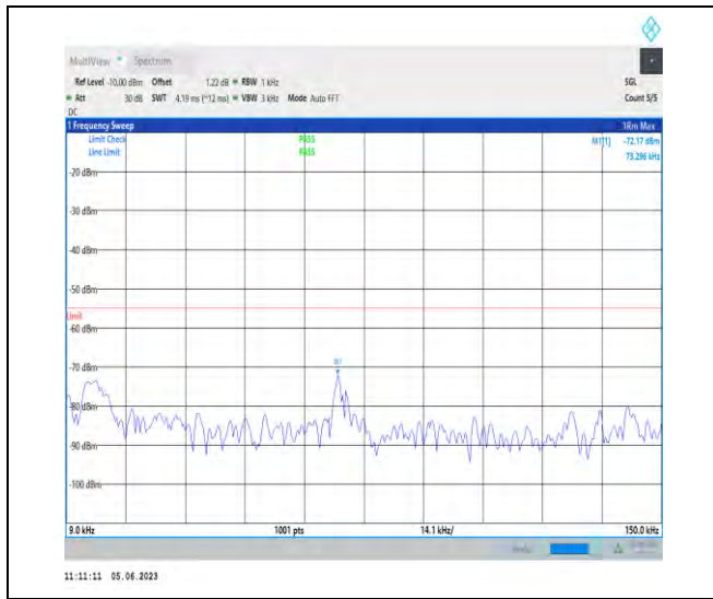
1-N38-PC3-30-20-H-1-N/A-DFT-PI2BPSK-Inner_1R B_Left-1@1-0.009-0.15-Ant1-0.07--72.17--55-PASS
