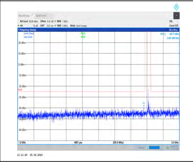
1-N38-PC3-30-20-H-1-N/A-DFT-PI2BPSK-Inner_1RB _Left-1@1-1000-3000-Ant1-2561.00--38.77--25-PASS
