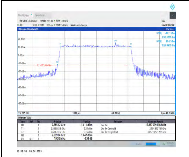
1-N38-PC3-30-20-M-4-DFT-64QAM-Outer_Full-50@ 0-Ant1-17.858-19.520-≤20-PASS
