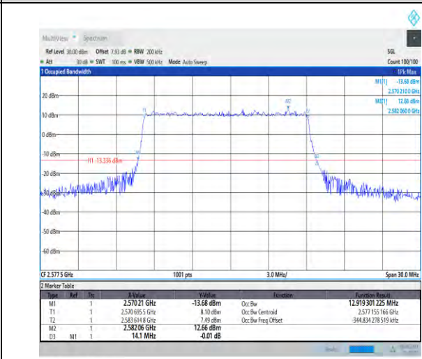
1-N38-PC3-30-15-L-3-DFT-16QAM-Outer_Full-36 @0-Ant1-12.921-14.280-≤15-PASS
