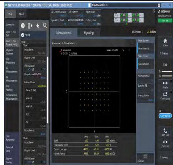
1-N38-PC3-30-20-M-8-CP-64QAM-Outer_Full-51@0-Ant1-see graph-PASS
