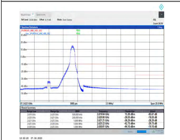
1-N38-PC3-30-10-H-5-CP-QPSK-Edge_1RB_Right-1@23-Ant1-1--PASS-see graph
