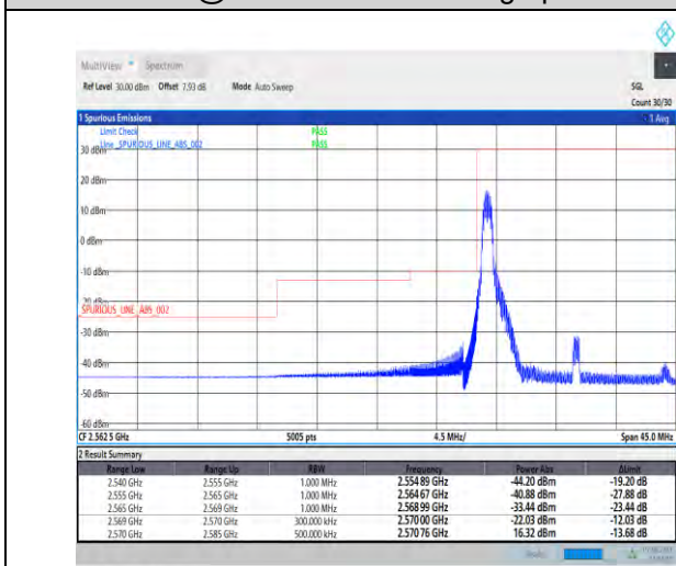
1-N38-PC3-30-15-L-1-DFT-PI2BPSK-Edge_1RB_Left-1@0-Ant1-1--PASS-see graph
