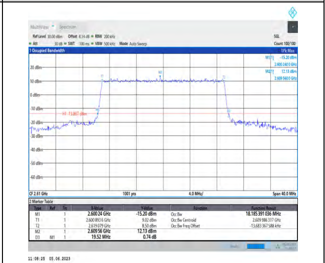
1-N38-PC3-30-20-H-6-CP-QPSK-Outer_Full-51@0- Ant1-18.185-19.520-≤20-PASS
