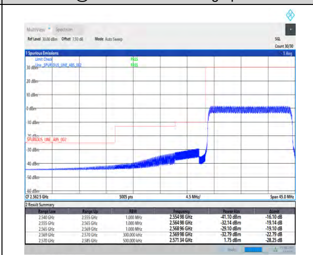
1-N38-PC3-30-15-L-3-DFT-PI2BPSK-Outer_Full-36@0-Ant1-1--PASS-see graph
