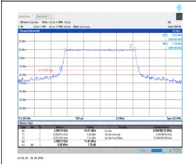
1-N38-PC3-30-10-M-6-CP-QPSK-Outer_Full-24@0- Ant1-8.585-9.580-≤10-PASS
