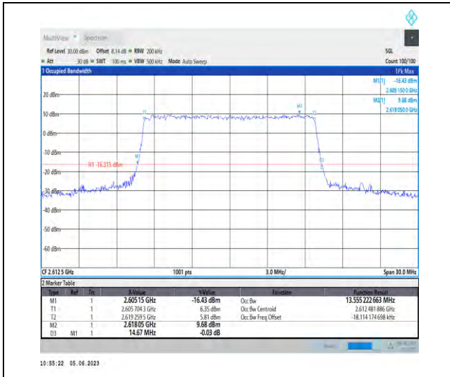
1-N38-PC3-30-15-H-9-CP-256QAM-Outer_Full-38@ 0-Ant1-13.555-14.670-≤15-PASS
