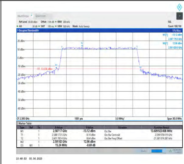
1-N38-PC3-30-15-M-6-CP-QPSK-Outer_Full-38@0- Ant1-13.61-15.240-≤15-PASS
