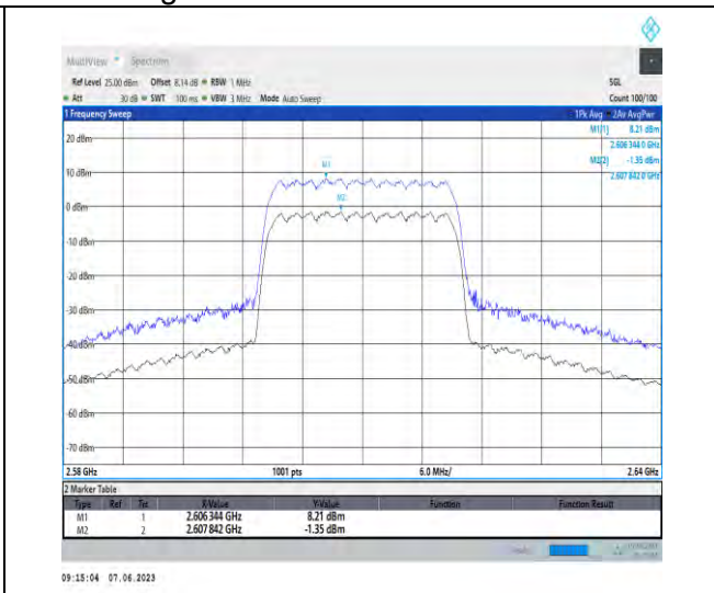
1-N38-PC3-30-20-H-2-CP-256QAM-Outer_Full-51@ 0-Ant1-9.56-100%-0.00-9.56-PASS≤13
