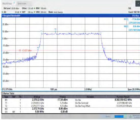
1-N38-PC3-30-10-L-9-CP-256QAM-Outer_Full-24@ 0-Ant1-8.582-9.560-≤10-PASS
