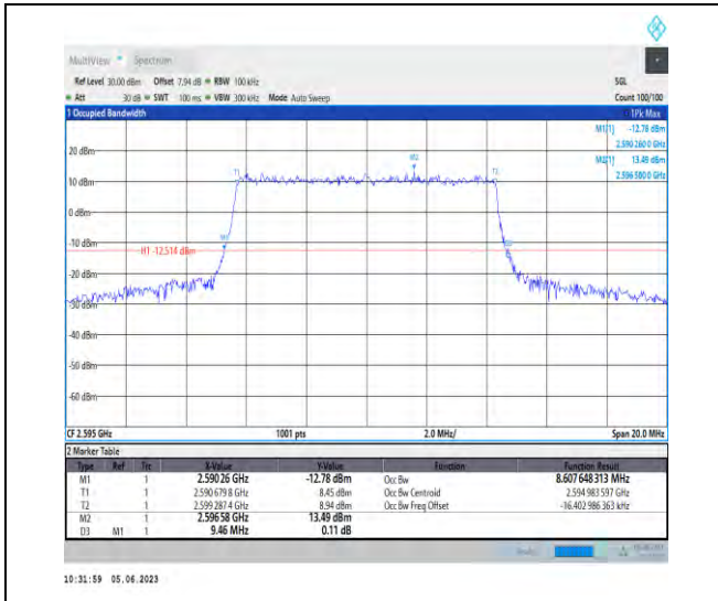
1-N38-PC3-30-10-M-4-DFT-64QAM-Outer_Full-24@ 0-Ant1-8.608-9.460-≤10-PASS
