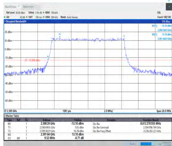
1-N38-PC3-30-10-M-3-DFT-16QAM-Outer_Full-24@ 0-Ant1-8.612-9.520-≤10-PASS
