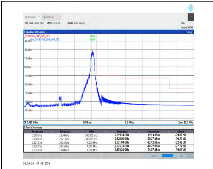
1-N38-PC3-30-15-H-2-DFT-PI2BPSK-Edge_1RB_Right-t-1@37-Ant1-1--PASS-see graph
