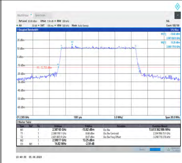
1-N38-PC3-30-15-M-8-CP-64QAM-Outer_Full-38@ 0-Ant1-13.613-14.820-≤15-PASS
