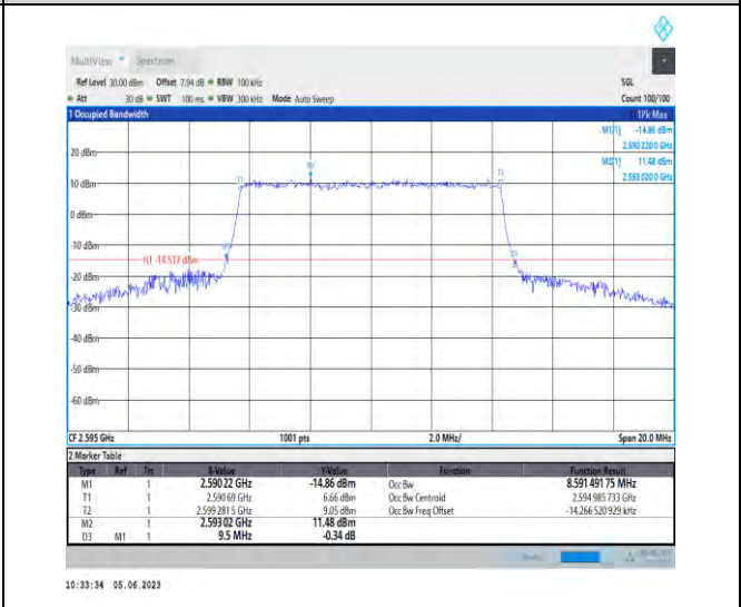
1-N38-PC3-30-10-M-7-CP-16QAM-Outer_Full-24@0 -Ant1-8.591-9.500-≤10-PASS
