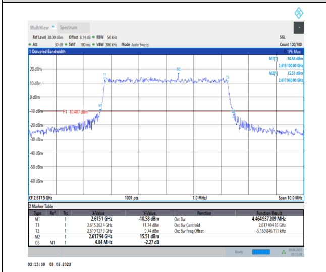
1-N38-PC3-15-5-H-1-DFT-QPSK-Outer_Full-25@0- Ant1-4.465-4.840-≤5-PASS
