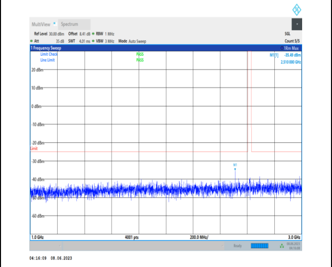
1-N38-PC3-15-5-H-1-N/A-DFT-PI2BPSK-Inner_1RB_Left-1@1-1000-3000-Ant1-2671.00--35.49--25-PASS
