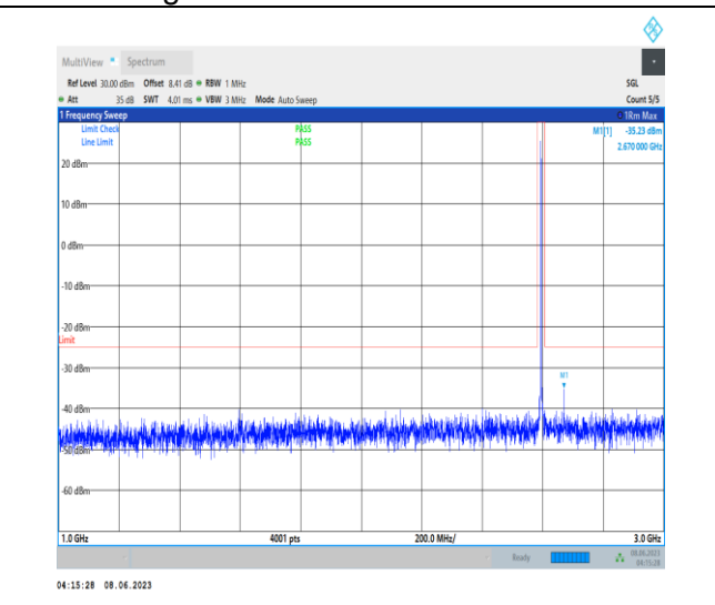
1-N38-PC3-15-5-M-1-N/A-DFT-PI2BPSK-Inner_1RB Left-1@1-1000-3000-Ant1-2608.50--35.23--25-PASS
