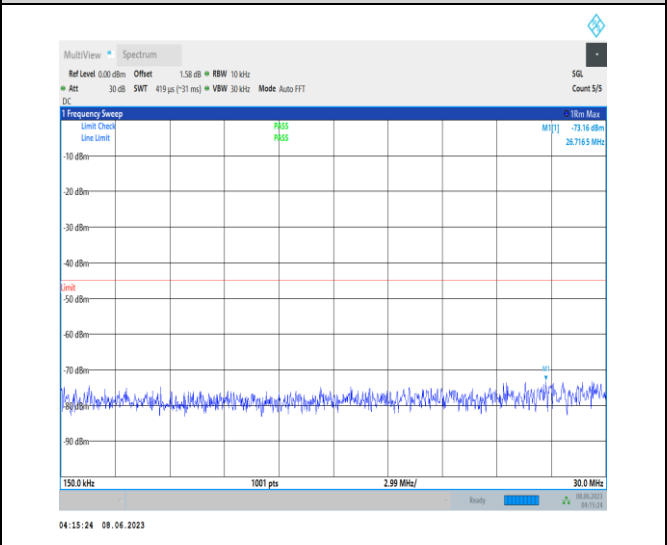
1-N38-PC3-15-5-M-1-N/A-DFT-PI2BPSK-Inner_1RB_ Left-1@1-0.15-30-Ant1-28.21--73.16--45-PASS
