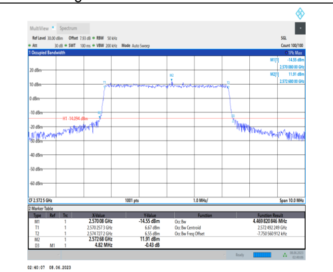
1-N38-PC3-15-5-L-6-CP-QPSK-Outer_Full-25@0-An t1-4.47-4.820-≤5-PASS
