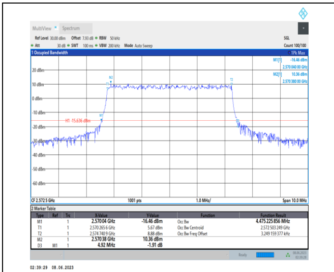
1-N38-PC3-15-5-L-5-DFT-256QAM-Outer_Full-25@0-Ant1-4.475-4.920-≤5-PASS
