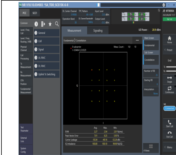
1-N38-PC3-15-5-M-7-CP-16QAM-Outer_Full-25@0-Ant1-see graph-PASS
