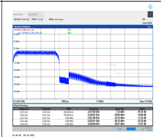
1-N38-PC3-15-5-H-6-CP-QPSK-Outer_Full-25@0-Ant1-1--PASS-see graph
