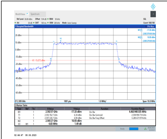
1-N38-PC3-15-5-M-8-CP-64QAM-Outer_Full-25@0 -Ant1-4.464-4.830-≤5-PASS
