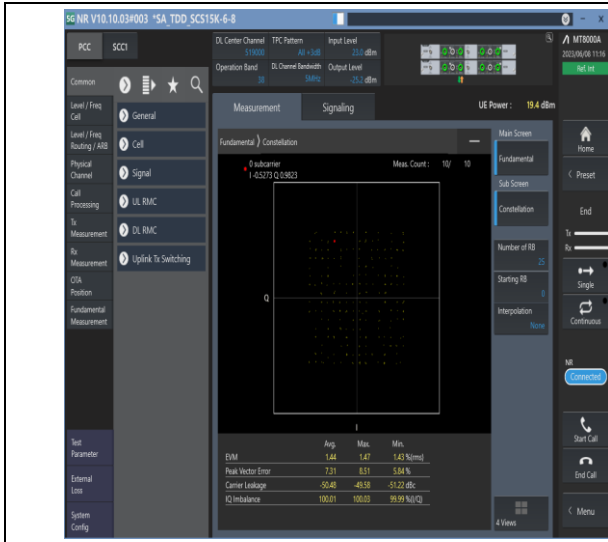
1-N38-PC3-15-5-M-5-DFT-256QAM-Outer_Full-25@0-Ant1-see graph-PASS
