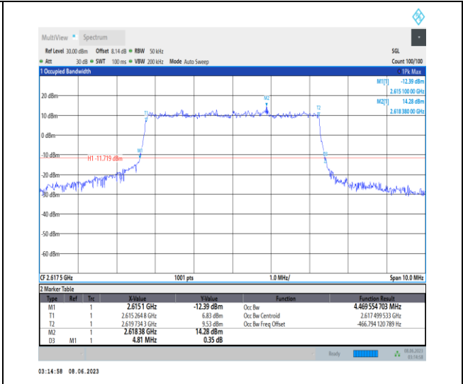
1-N38-PC3-15-5-H-4-DFT-64QAM-Outer_Full-25@0-Ant1-4.47-4.810-≤5-PASS
