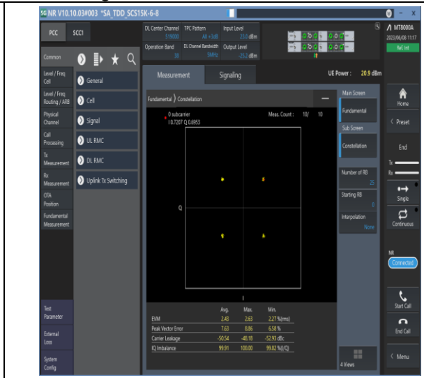
1-N38-PC3-15-5-M-6-CP-QPSK-Outer_Full-25@0-Ant1-see graph-PASS
