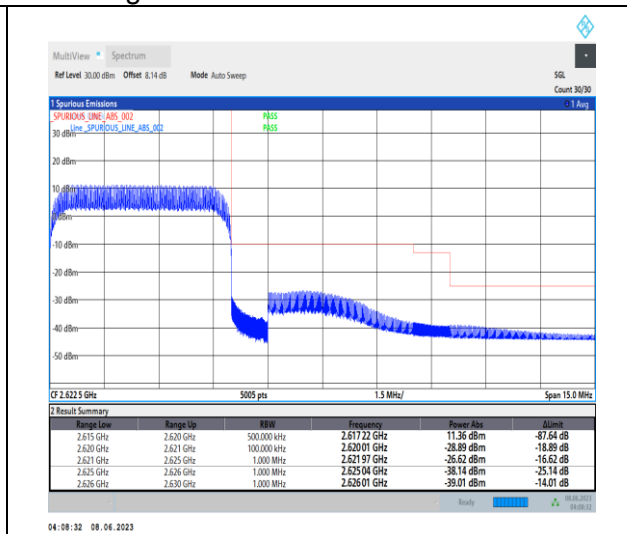
1-N38-PC3-15-5-H-3-DFT-PI2BPSK-Outer_Full-25@0-Ant1-1--PASS-see graph
