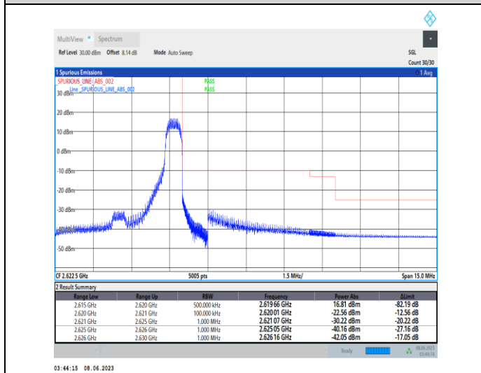
1-N38-PC3-15-5-H-5-CP-QPSK-Edge_1RB_Right-1@24-Ant1-1--PASS-see graph
