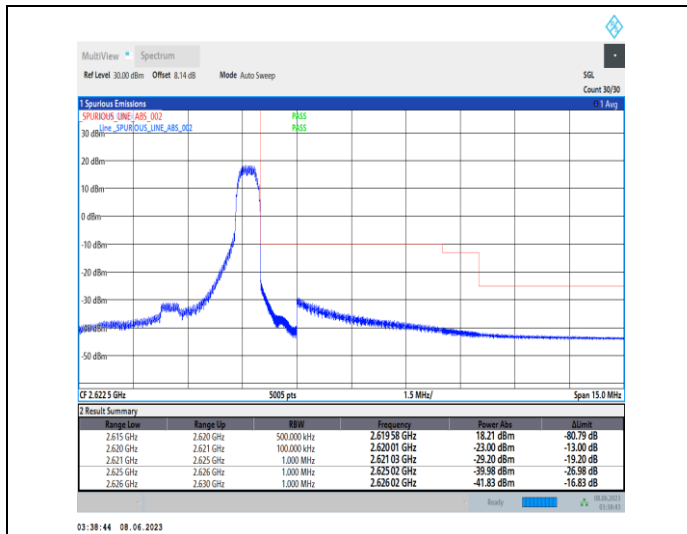
1-N38-PC3-15-5-H-2-DFT-PI2BPSK-Edge_1RB_Right-1@24-Ant1-1--PASS-see graph
