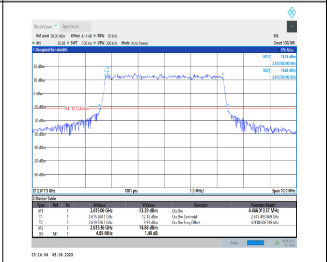
1-N38-PC3-15-5-H-2-DFT-PI2BPSK-Outer_Full-25@ 0-Ant1-4.466-4.850-≤5-PASS
