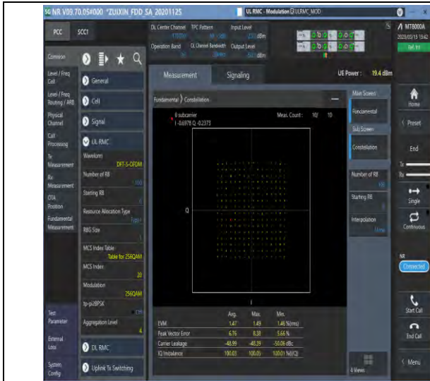
1-N26-824-849-PC3-15-20-M-5-DFT-256QAM-Outer_Fu ll-100@0-Ant1-see graph-PASS
