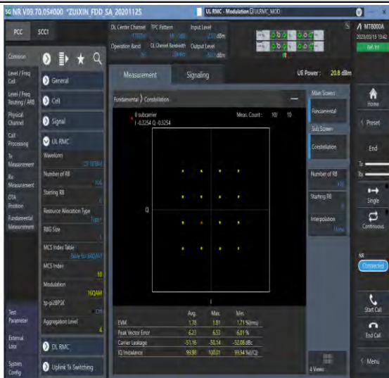
1-N26-824-849-PC3-15-20-M-7-CP-16QAM-Outer_Full- 106@0-Ant1-see graph-PASS
