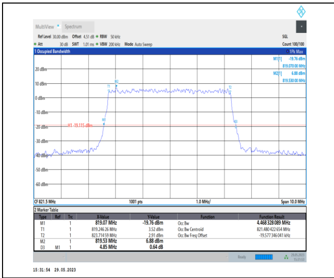
NTNV_N26-814-824_PC3_15_5_H_TID9_Ant1#1
