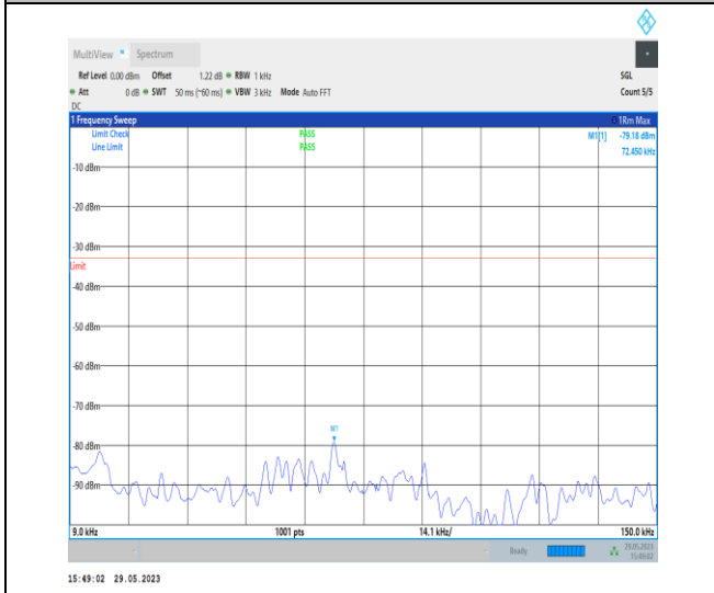
NTVN_N26-814-824_PC3_15_10_M_TID1_N/A_0.009_0_15_#1
