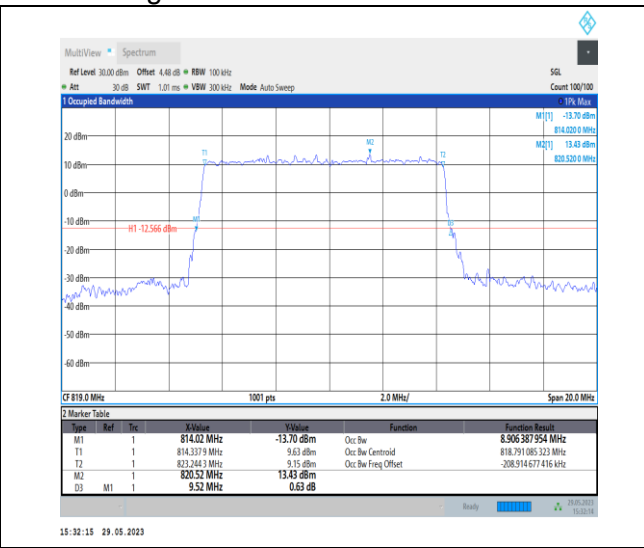
NTNV_N26-814-824_PC3_15_10_M_TID1_Ant1#1
