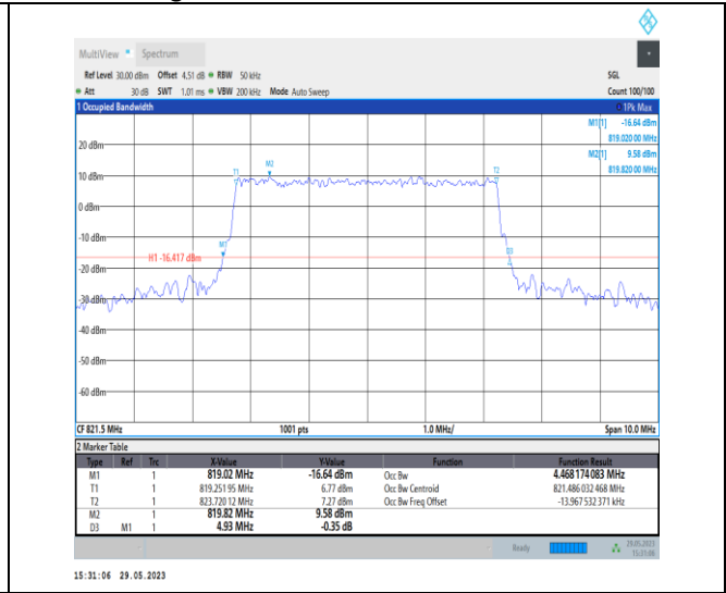
NTNV_N26-814-824_PC3_15_5_H_TID6_Ant1#1
