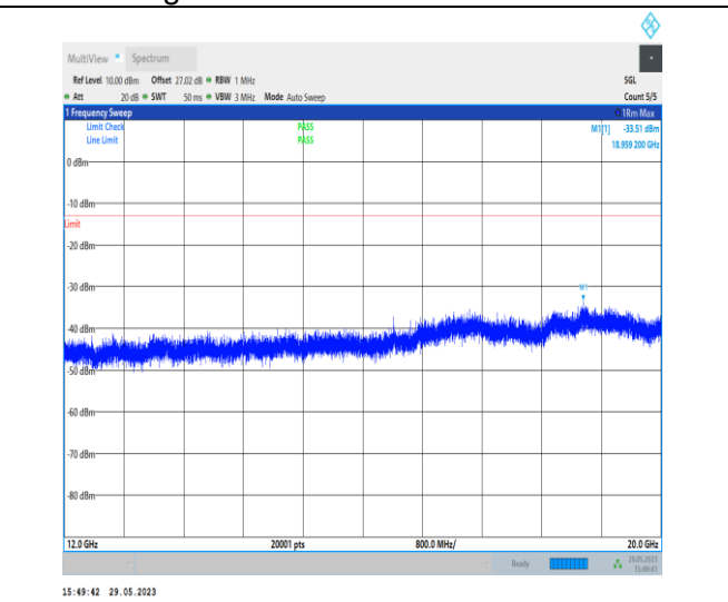
NTNV_N26-814-824_PC3_15_10_H_TID1_N/A_12000_20 000_#1
