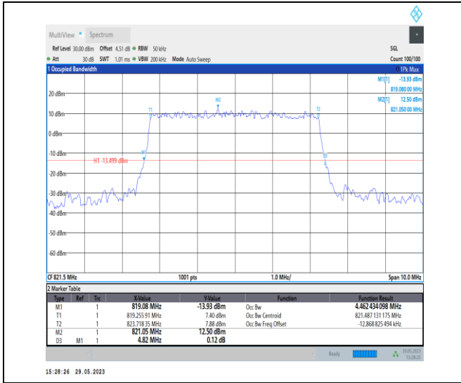
NTNV_N26-814-824_PC3_15_5_H_TID4_Ant1#1
