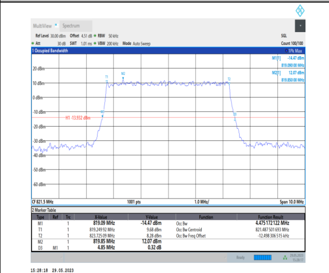
NTVN_N26-814-824_PC3_15_5_H_TID3_Ant1#1
