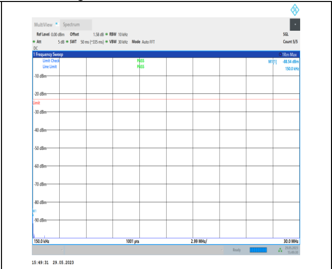
NTVN_N26-814-824_PC3_15_10_H_TID1_N/A_0.15_30_#1
