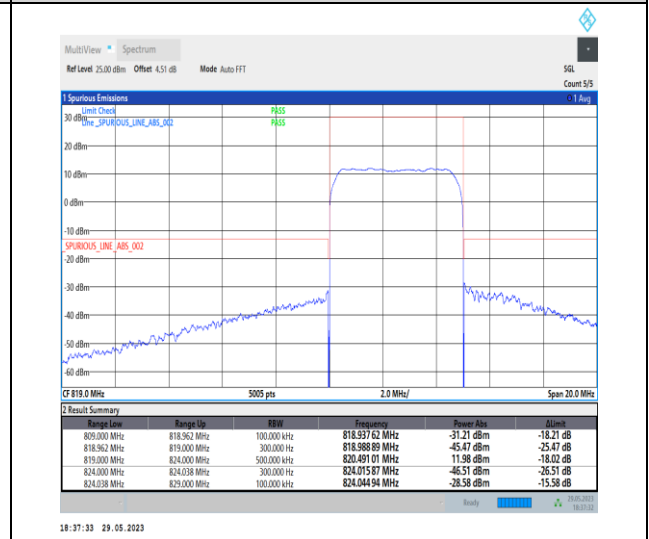
1-N26-814-824-PC3-15-5-H-6-CP-QPSK-Outer_Full-25@0-Ant1-1--PASS-see graph
