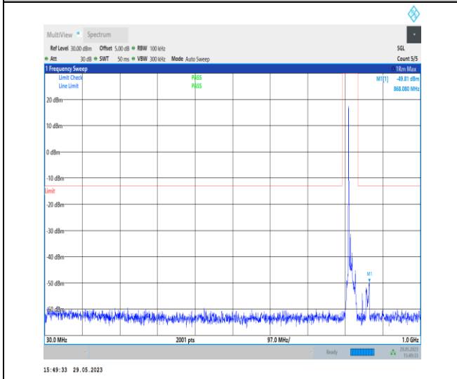
NTVN_N26-814-824_PC3_15_10_H_TID1_N/A_30_1000_#1
