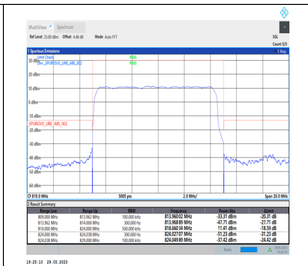
1-N26-814-824-PC3-15-10-H-3-DFT-PI2BPSK-Out er_Full-50@0-Ant1-1--PASS-see graph
