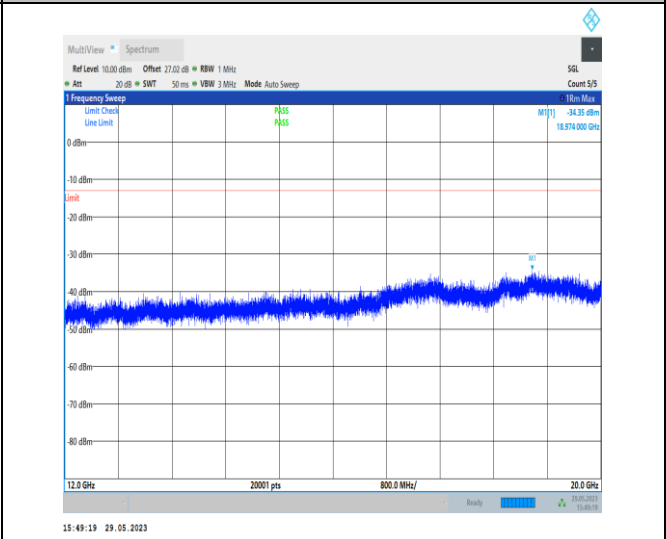
NTVN_N26-814-824_PC3_15_10_M_TID1_N/A_12000_20_000_#1
