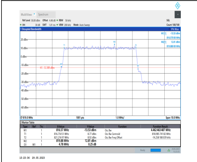
NTVN_N26-814-824_PC3_15_5_M_TID3_Ant1#1
