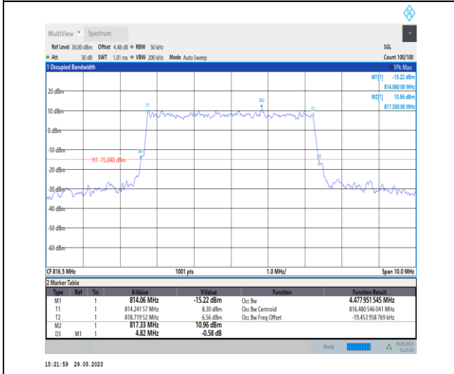
NTNV_N26-814-824_PC3_15_5_L_TID8_Ant1#1
