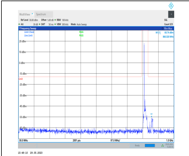
NTVN_N26-814-824_PC3_15_10_M_TID1_N/A_30_1000_#1
