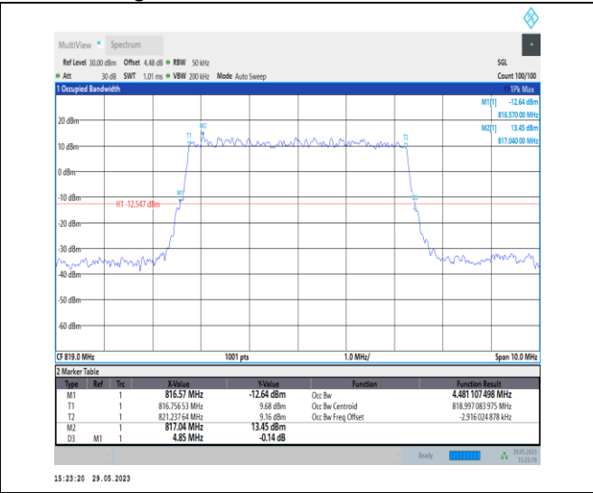
NTVN_N26-814-824_PC3_15_5_M_TID2_Ant1#1
