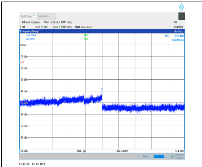
NTNV_N26-814-824_PC3_15_10_H_TID1_N/A_3000_12 000_#1
