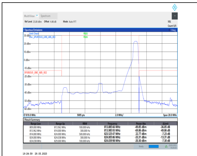
1-N26-814-824-PC3-15-10-H-2-DFT-PI2BPSK-Edge_1 RB_Right-1@51-Ant1-1--PASS-see graph
