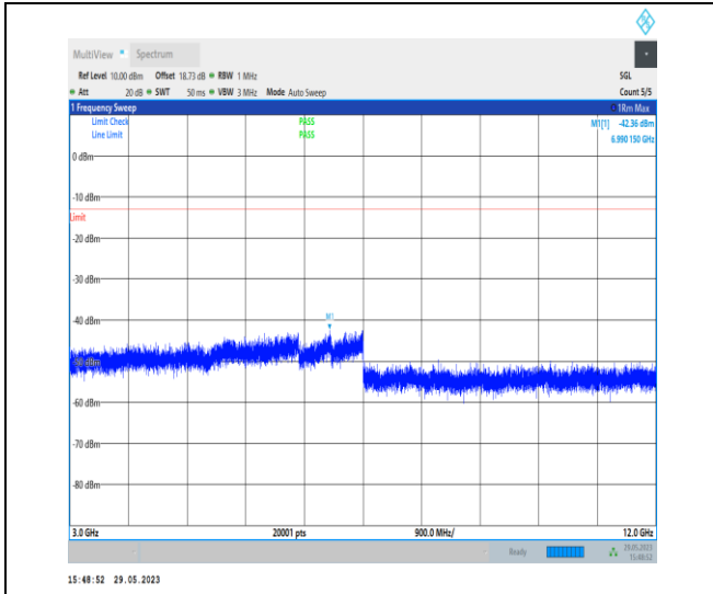
NTVN_N26-814-824_PC3_15_10_L_TID1_N/A_3000_12_000_#1
