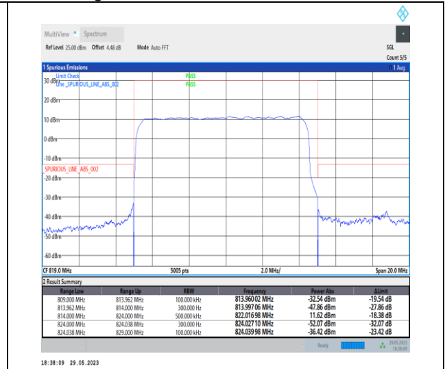
1-N26-814-824-PC3-15-10-L-3-DFT-PI2BPSK-Out er_Full-50@0-Ant1-1--PASS-see graph
