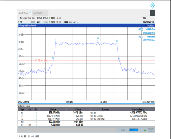
NTNV_N26-814-824_PC3_15_5_H_TID8_Ant1#1
