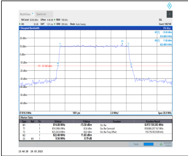
NTVN_N26-814-824_PC3_15_10_M_TID4_Ant1#1
