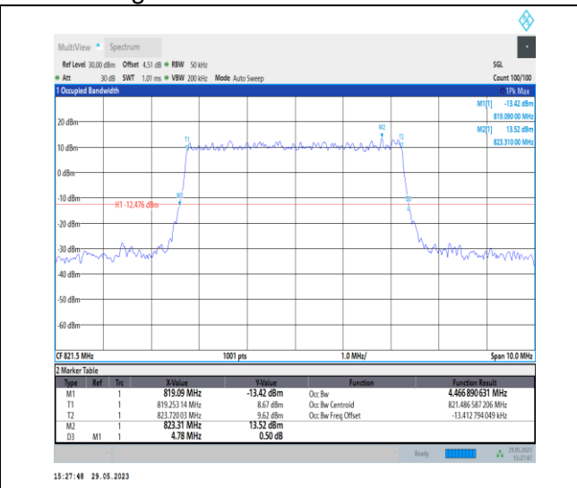
NTVN_N26-814-824_PC3_15_5_H_TID1_Ant1#1
