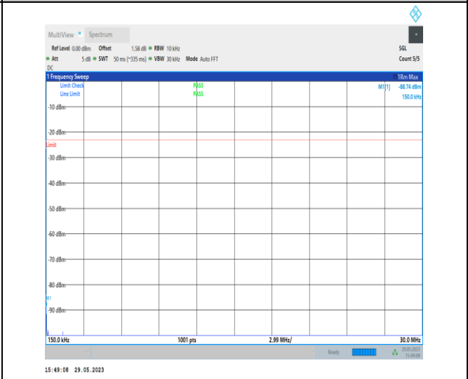
NTVN_N26-814-824_PC3_15_10_M_TID1_N/A_0.15_30_#1
