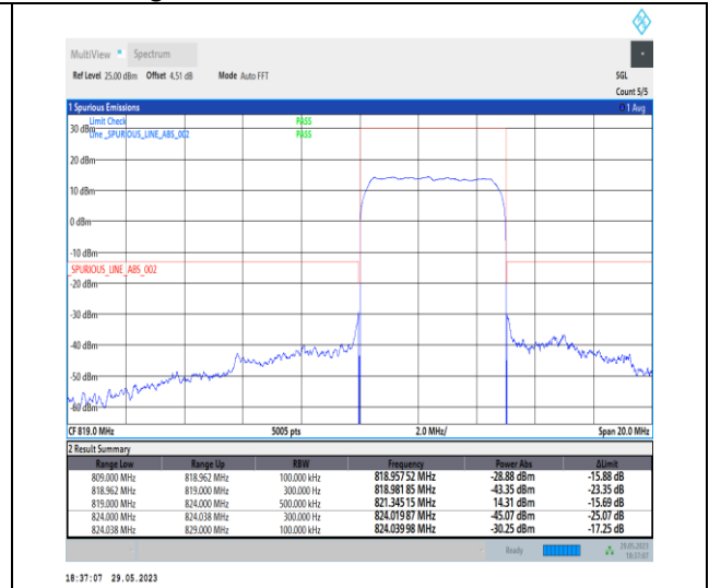
1-N26-814-824-PC3-15-5-H-3-DFT-PI2BPSK-Outer_Full-25@0-Ant1-1--PASS-see graph
