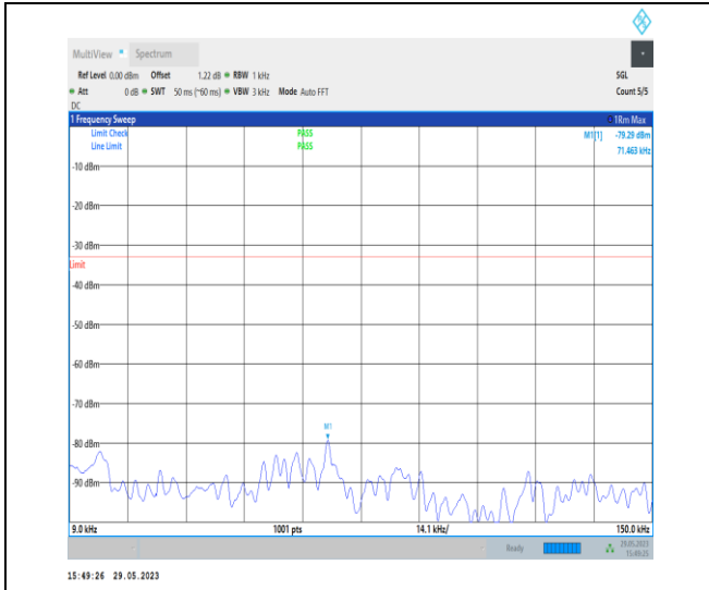
NTVN_N26-814-824_PC3_15_10_H_TID1_N/A_0.009_0.
