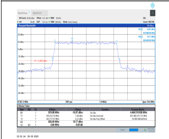
NTNV_N26-814-824_PC3_15_5_H_TID7_Ant1#1
