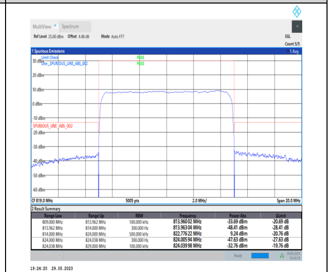
1-N26-814-824-PC3-15-10-L-6-CP-QPSK-Outer_F ull-52@0-Ant1-1--PASS-see graph
