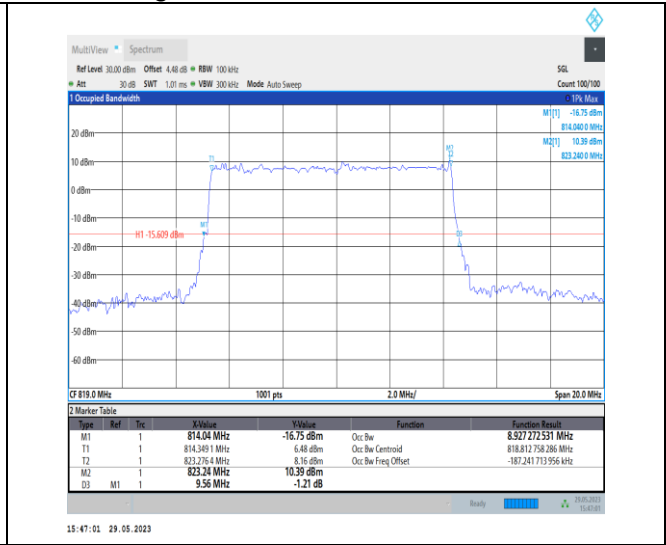
NTVN_N26-814-824_PC3_15_10_M_TID5_Ant1#1
