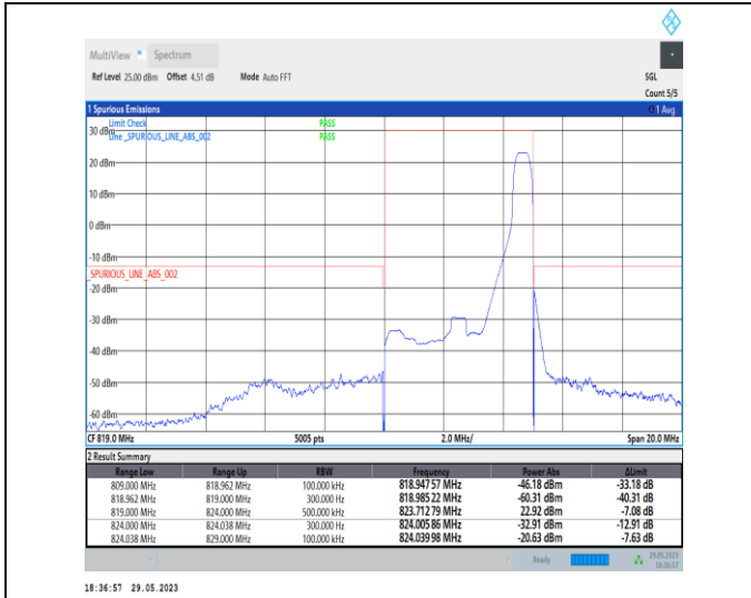
1-N26-814-824-PC3-15-5-H-2-DFT-PI2BPSK-Edge_1 RB_Right-1@24-Ant1-1--PASS-see graph
