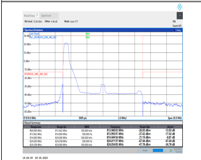
1-N26-814-824-PC3-15-10-L-4-CP-QPSK-Edge_1RB_Left-1@0-Ant1-1--PASS-see graph
