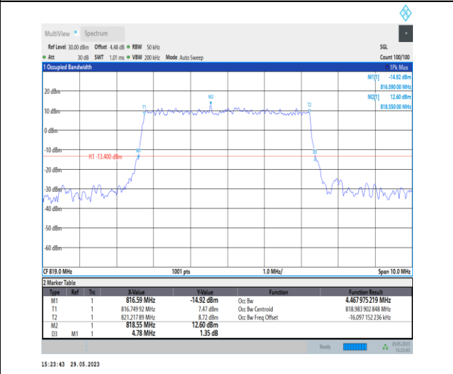
NTVN_N26-814-824_PC3_15_5_M_TID4_Ant1#1
