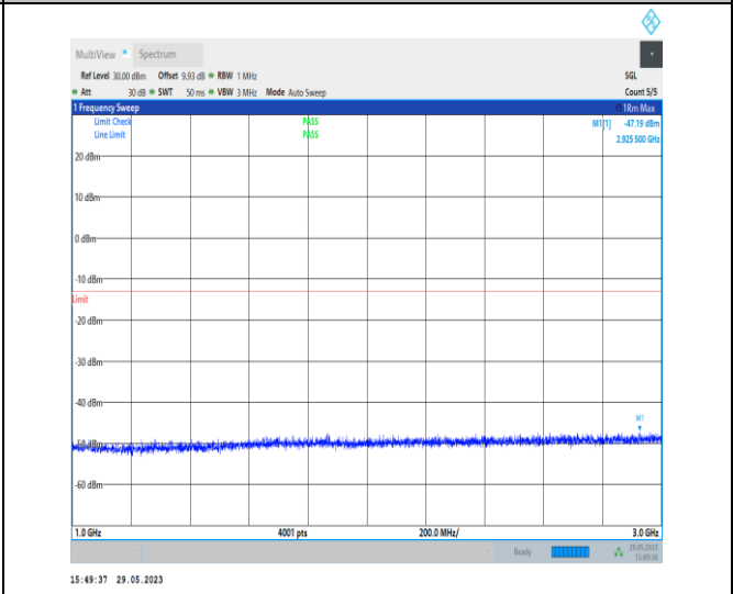
NTVN_N26-814-824_PC3_15_10_H_TID1_N/A_1000_300_0_#1
