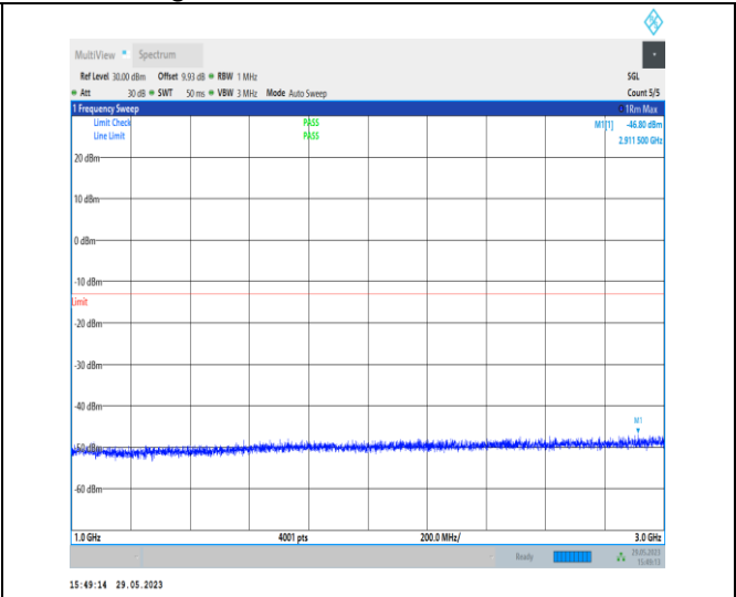
NTVN_N26-814-824_PC3_15_10_M_TID1_N/A_1000_300_0_#1
