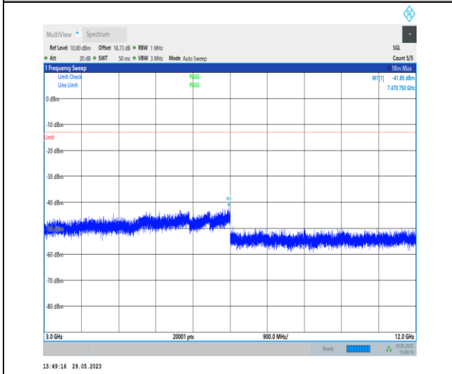
NTVN_N26-814-824_PC3_15_10_M_TID1_N/A_3000_12_000_#1
