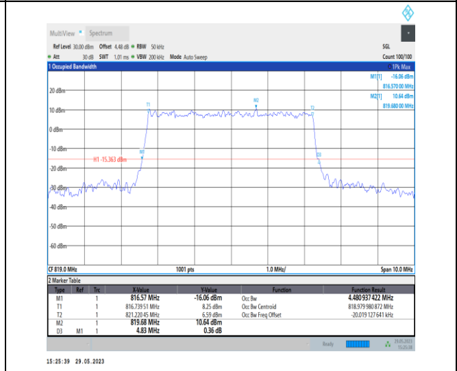
NTVN_N26-814-824_PC3_15_5_M_TID8_Ant1#1
