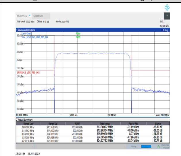
1-N26-814-824-PC3-15-10-H-6-CP-QPSK-Outer_1 Full-52@0-Ant1-1--PASS-see graph
