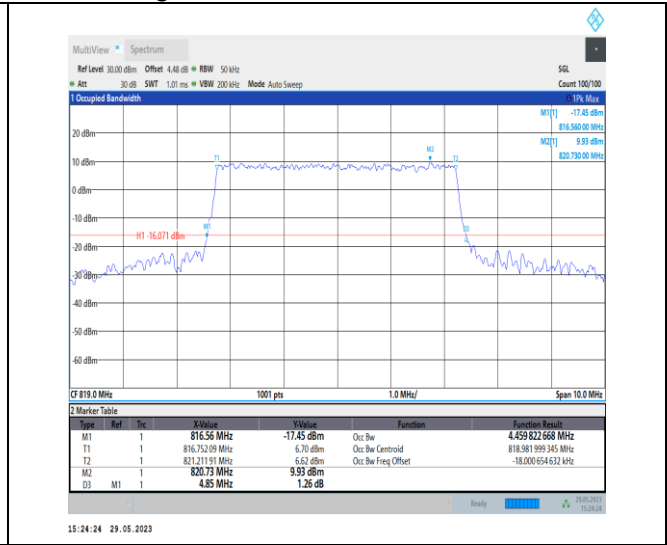
NTVN_N26-814-824_PC3_15_5_M_TID6_Ant1#1
