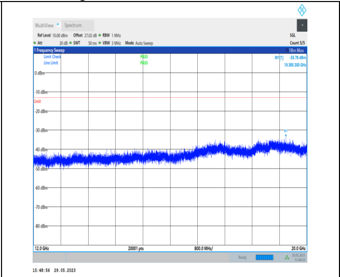
NTVN_N26-814-824_PC3_15_10_L_TID1_N/A_12000_20_000_#1
