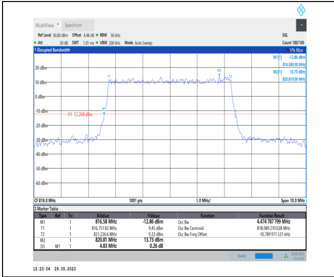
NTVN_N26-814-824_PC3_15_5_M_TID1_Ant1#1
