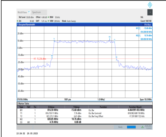
NTVN_N26-814-824_PC3_15_5_M_TID7_Ant1#1
