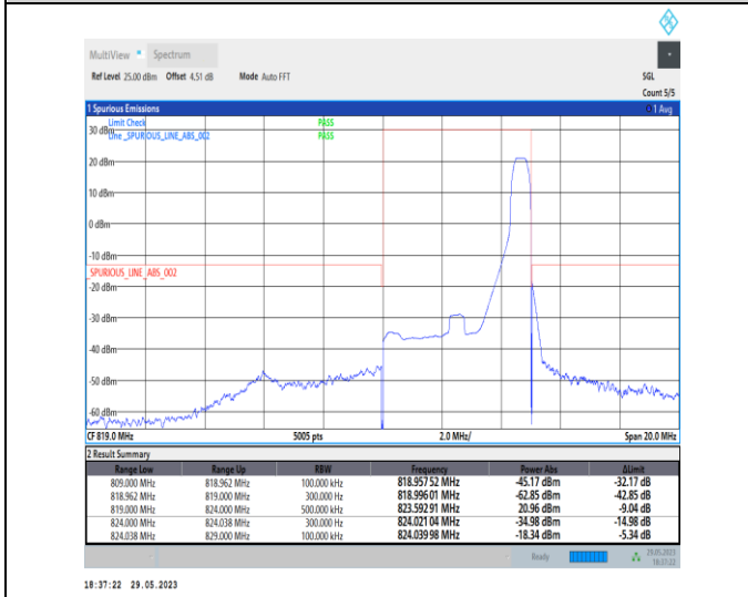
1-N26-814-824-PC3-15-5-H-5-CP-QPSK-Edge_1RB_Right-1@24-Ant1-1--PASS-see graph
