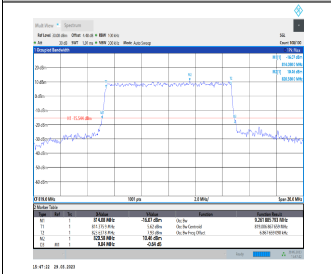
NTVN_N26-814-824_PC3_15_10_M_TID6_Ant1#1
