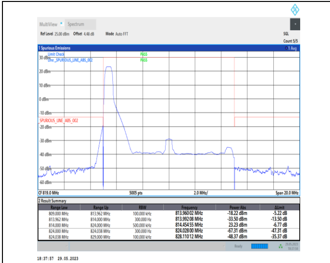
1-N26-814-824-PC3-15-10-L-1-DFT-PI2BPSK-Edge_1 RB_Left-1@0-Ant1-1--PASS-see graph
