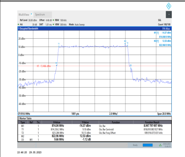
NTNV_N26-814-824_PC3_15_10_M_TID3_Ant1#1
