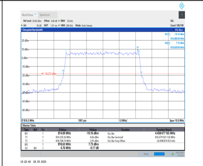
NTNV_N26-814-824_PC3_15_5_L_TID9_Ant1#1
