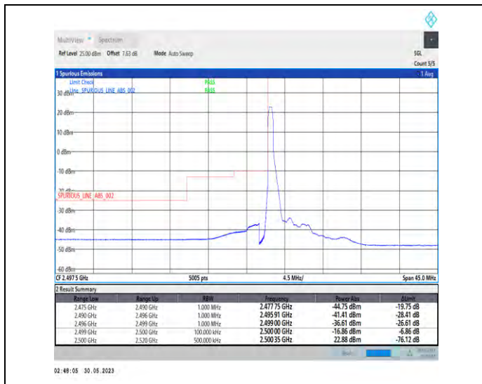
1-N7-PC3-15-5-L-1-DFT-PI2BPSK-Edge_1RB_Left-1@0-Ant1-1--PASS-see graph
