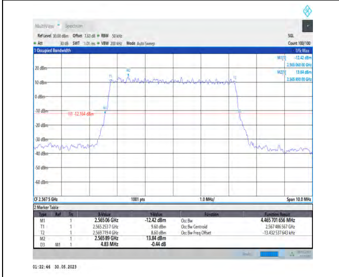
1-N7-PC3-15-5-H-2-DFT-PI2BPSK-Outer_Full-25@0-A Ant1-4.466-4.830-≤5-PASS
