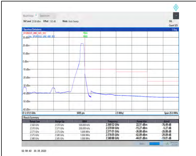
1-N7-PC3-15-10-H-2-DFT-PI2BPSK-Edge_1RB_Right-1@51-Ant1-1--PASS-see graph
