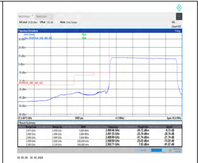
1-N7-PC3-15-20-L-3-DFT-PI2BPSK-Outer_Full-100@0-Ant1-1--PASS-see graph
