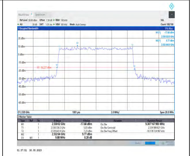
1-N7-PC3-15-10-M-8-CP-64QAM-Outer_Full-52@0- Ant1-9.307-9.880-≤10-PASS
