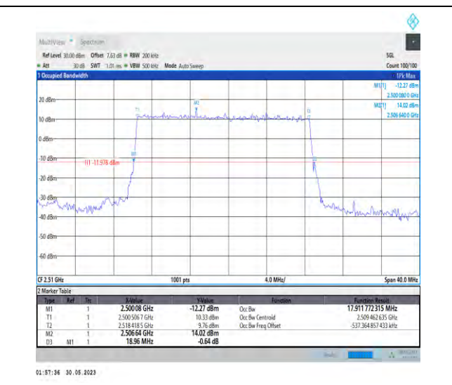
1-N7-PC3-15-20-L-2-DFT-PI2BPSK-Outer_Full-100 @0-Ant1-17.912-18.960-≤20-PASS
