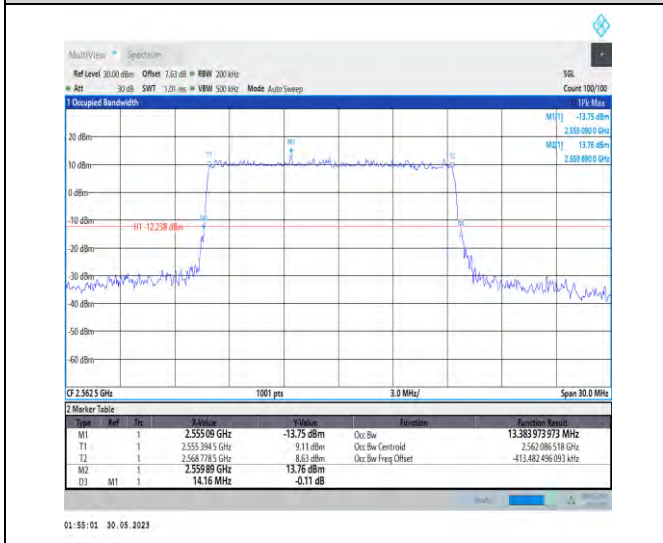
1-N7-PC3-15-15-H-4-DFT-64QAM-Outer_Full-75@0- Ant1-13.384-14.160-≤15-PASS
