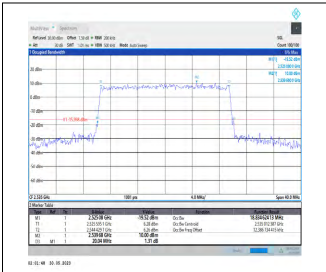
1-N7-PC3-15-20-M-8-CP-64QAM-Outer_Full-106@ 0-Ant1-18.835-20.040-≤20-PASS
