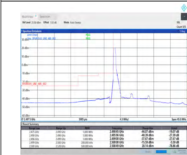
1-N7-PC3-15-10-L-1-DFT-PI2BPSK-Edge_1RB_Left-1 @0-Ant1-1--PASS-see graph
