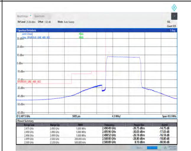
1-N7-PC3-15-10-L-3-DFT-PI2BPSK-Outer_Full-50 @0-Ant1-1--PASS-see graph
