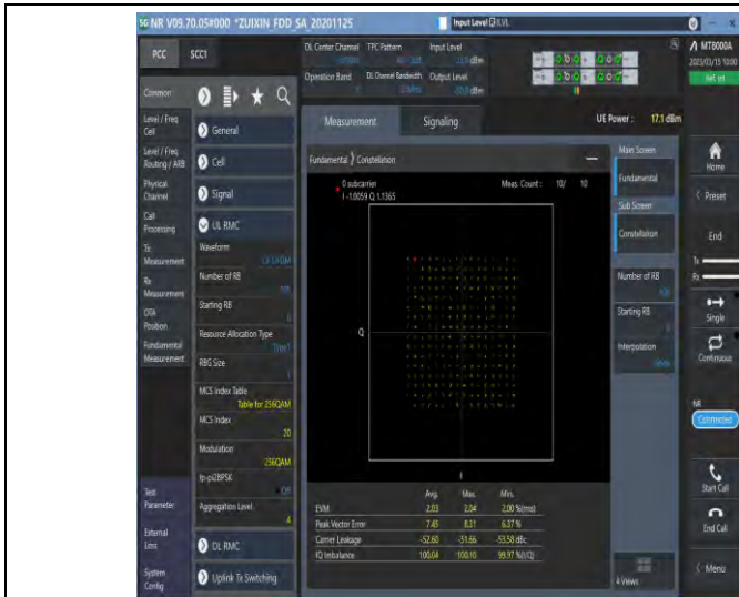
1-N7-PC3-15-20-M-9-CP-256QAM-Outer_Full-106@0-Ant1-see graph-PASS
