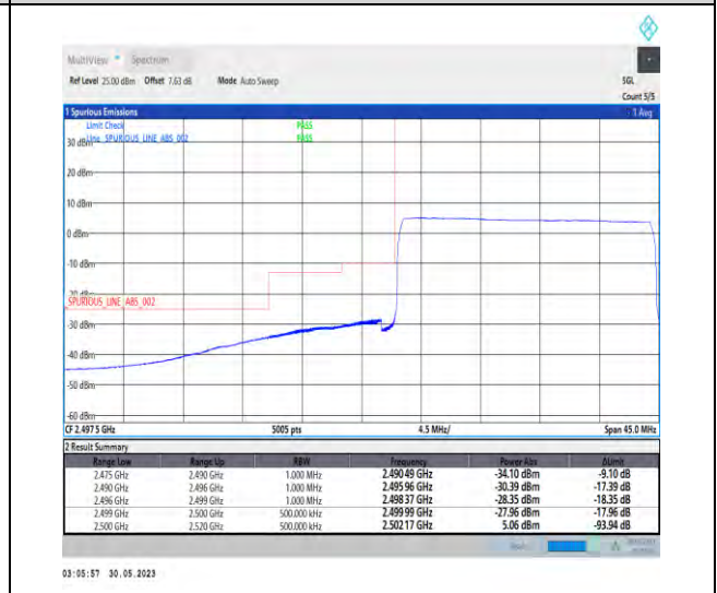
1-N7-PC3-15-20-L-6-CP-QPSK-Outer_Full-106@0-Ant1-1--PASS-see graph
