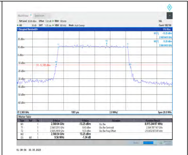
1-N7-PC3-15-10-H-1-DFT-QPSK-Outer_Full-50@0- Ant1-8.915-9.560-≤10-PASS
