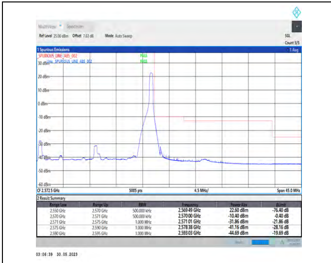
1-N7-PC3-15-20-H-2-DFT-PI2BPSK-Edge_1RB_Right-1@105-Ant1-1--PASS-see graph
