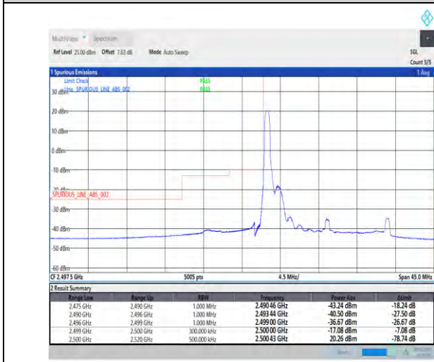
1-N7-PC3-15-15-L-1-DFT-PI2BPSK-Edge_1RB_Left-1 @0-Ant1-1--PASS-see graph
