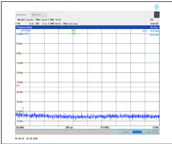
1-N7-PC3-15-20-M-1-N/A-DFT-PI2BPSK-Inner_1RB_Left-1@1-30-1000-Ant1-107.60--59.72--35-PASS
