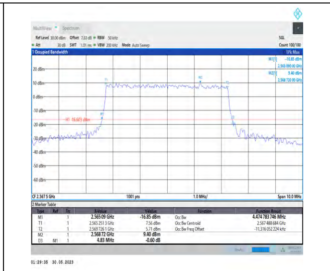
1-N7-PC3-15-5-H-7-CP-16QAM-Outer_Full-25@0-A Ant1-4.475-4.830-≤5-PASS
