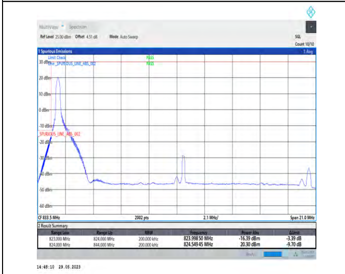
1-N5-PC3-15-20-L-4-CP-QPSK-Edge_1RB_Left-1@0-Ant1-1-seegraph-PASS-see graph
