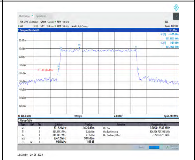
1-N5-PC3-15-10-M-8-CP-64QAM-Outer_Full-52@0- Ant1-9.305-9.860-≤10-PASS
