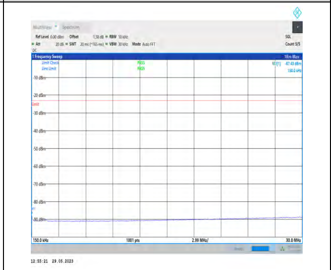
1-N5-PC3-15-20-H-1-N/A-DFT-PI2BPSK-Inner_1RB _Left-1@1-0.15-30-Ant1-0.15--87.43--23-PASS
