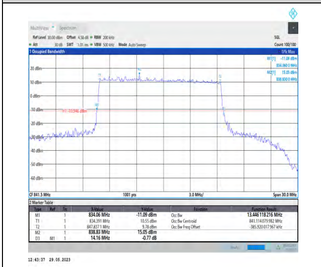
1-N5-PC3-15-15-H-3-DFT-16QAM-Outer_Full-75@0-Ant1-13.446-14.160-≤15-PASS
