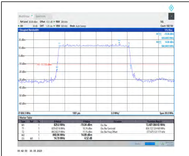
1-N5-PC3-15-15-M-2-DFT-PI2BPSK-Outer_Full-75@ 0-Ant1-13.401-14.190≤15-PASS
