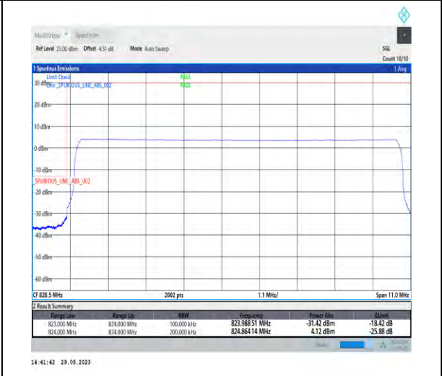
1-N5-PC3-15-10-L-6-CP-QPSK-Outer_Full-52@0-Ant1-1-seegraph-PASS-see graph
