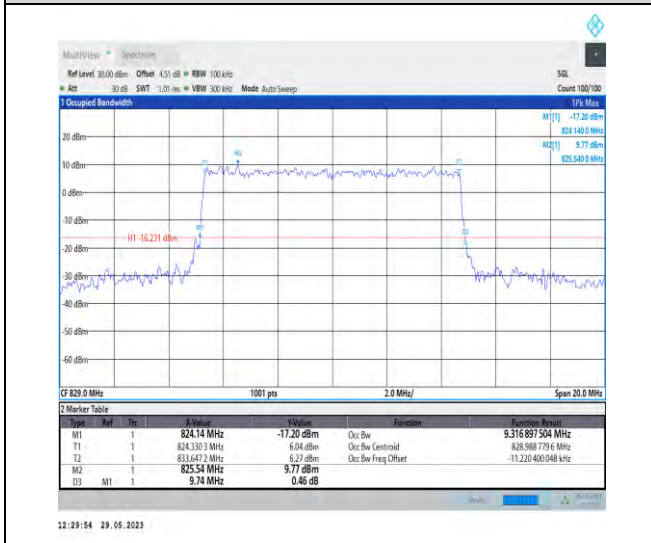
1-N5-PC3-15-10-L-8-CP-64QAM-Outer_Full-52@0-A Ant1-9.317-9.740-≤10-PASS
