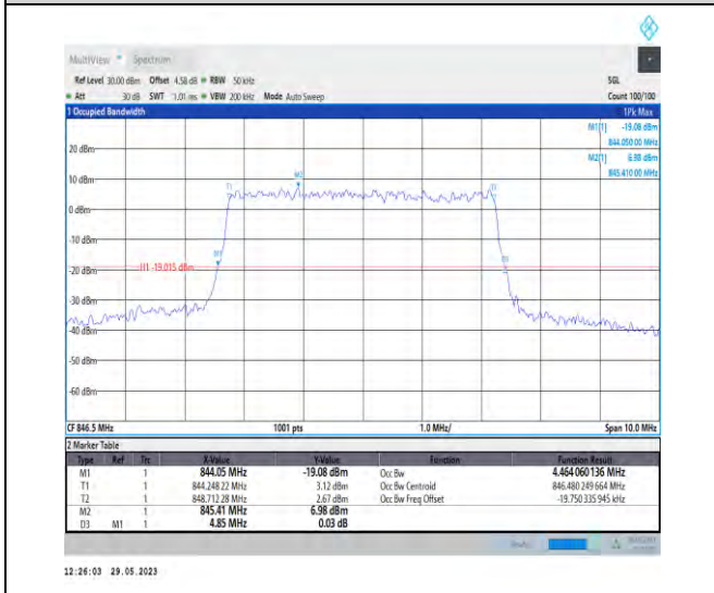
1-N5-PC3-15-5-H-9-CP-256QAM-Outer_Full-25@0-A Ant1-4.464-4.850-≤5-PASS
