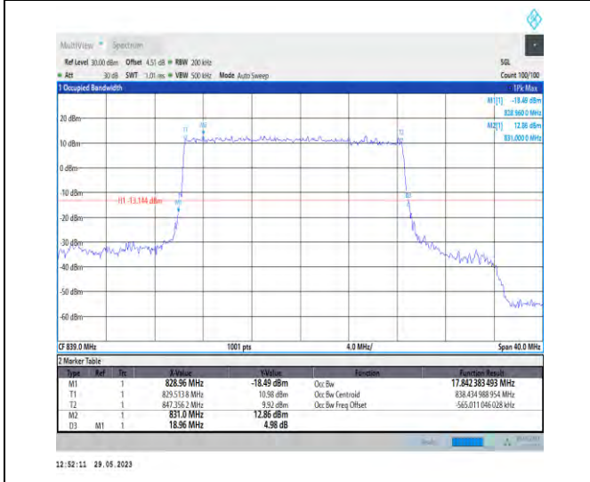
1-N5-PC3-15-20-H-2-DFT-PI2BPSK-Outer_Full-100 @0-Ant1-17.842-18.960-≤20-PASS
