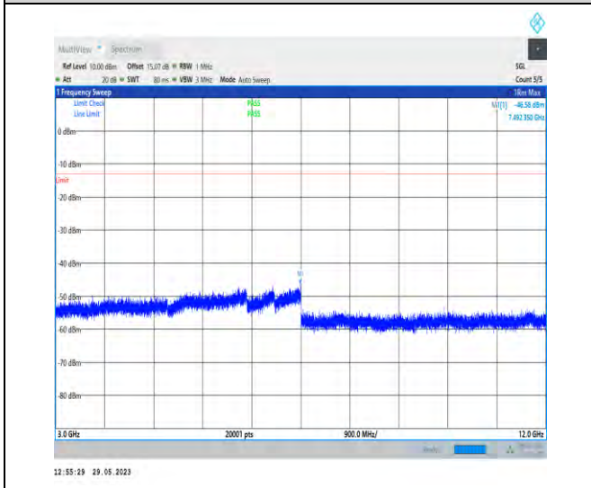
1-N5-PC3-15-20-H-1-N/A-DFT-PI2BPSK-Inner_1RB _Left-1@1-3000-12000-Ant1-7492.35--46.58--13-PA SS
