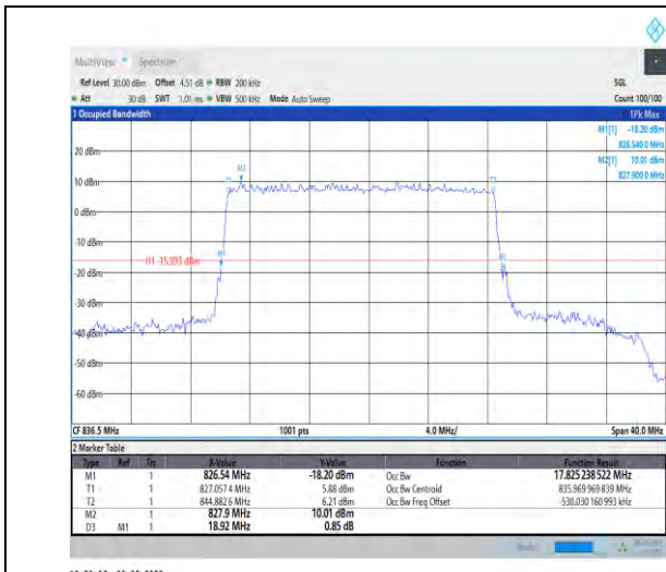
1-N5-PC3-15-20-M-5-DFT-256QAM-Outer_Full-100 @0-Ant1-17.825-18.920-≤20-PASS
