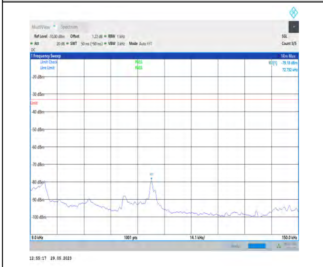
1-N5-PC3-15-20-H-1-N/A-DFT-PI2BPSK-Inner_1RB _Left-1@1-0.009-0.15-Ant1-0.07--79.18--33-PASS
