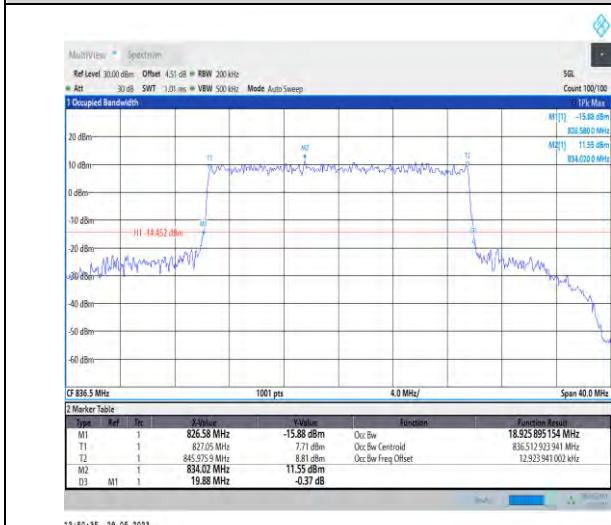
1-N5-PC3-15-20-M-7-CP-16QAM-Outer_Full-106@0- Ant1-18.926-19.880-≤20-PASS
