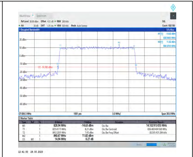
1-N5-PC3-15-15-M-7-CP-16QAM-Outer_Full-79@0- Ant1-14.103-14.940-≤15-PASS
