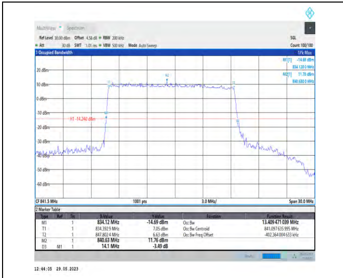
1-N5-PC3-15-15-H-5-DFT-256QAM-Outer_Full-75@0 -Ant1-13.409-14.100-≤15-PASS
