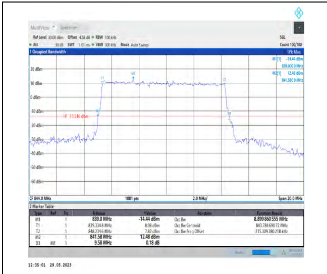
1-N5-PC3-15-10-H-4-DFT-64QAM-Outer_Full-50@ 0-Ant1-8.9-9.580-≤10-PASS
