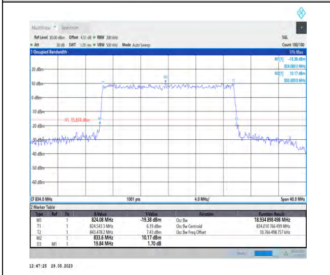
1-N5-PC3-15-20-L-8-CP-64QAM-Outer_Full-106@0-Ant1-18.935-19.840-≤20-PASS
