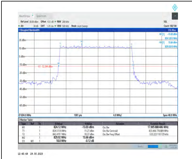
1-N5-PC3-15-20-L-2-DFT-PI2BPSK-Outer_Full-100 @0-Ant1-17.906-18.800-<=20-PASS
