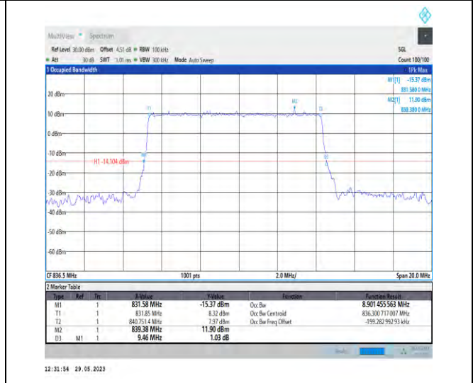
1-N5-PC3-15-10-M-4-DFT-64QAM-Outer_Full-50@0-Ant1-8.901-9.460-≤10-PASS
