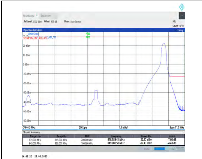
1-N5-PC3-15-10-H-2-DFT-PI2BPSK-Edge_1RB_Right-1@51-Ant1-1-seegraph-PASS-see graph
