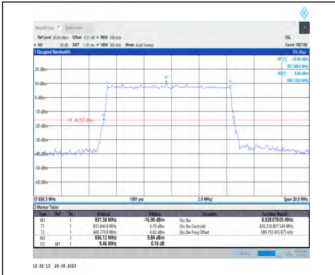
1-N5-PC3-15-10-M-5-DFT-256QAM-Outer_Full-50@ 0-Ant1-8.928-9.460-≤10-PASS
