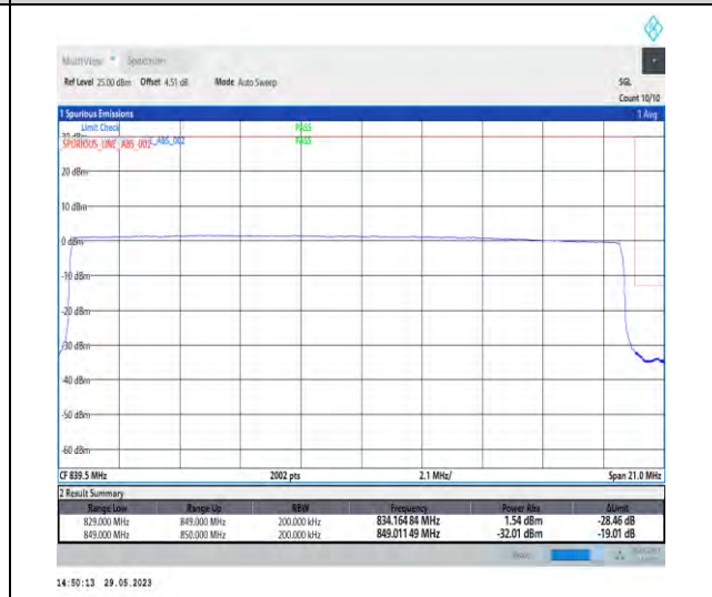
1-N5-PC3-15-20-H-6-CP-QPSK-Outer_Full-106@0-Ant1-1-seegraph-PASS-see graph
