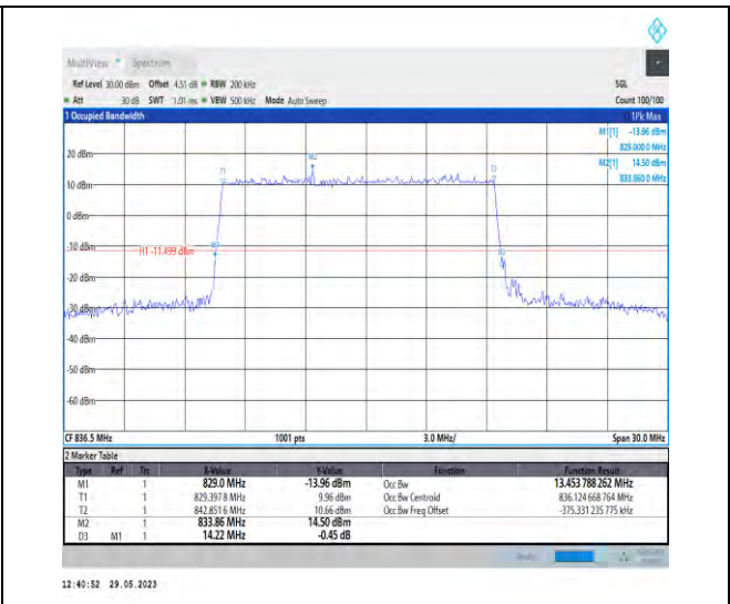
1-N5-PC3-15-15-M-3-DFT-16QAM-Outer_Full-75@ 0-Ant1-13.454-14.220≤15-PASS
