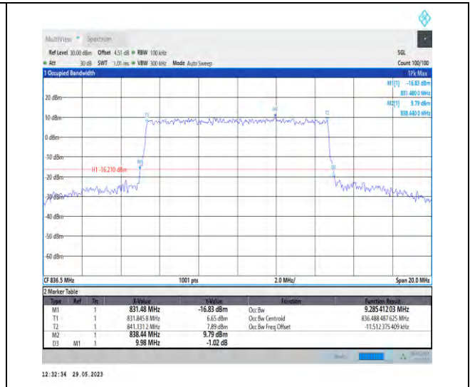
1-N5-PC3-15-10-M-6-CP-QPSK-Outer_Full-52@0- Ant1-9.285-9.980-≤10-PASS
