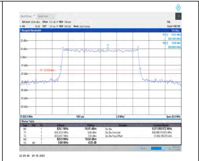
1-N5-PC3-15-10-L-7-CP-16QAM-Outer_Full-52@0-A Ant1-9.311-9.840-≤10-PASS
