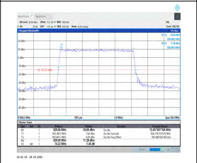
1-N5-PC3-15-15-M-5-DFT-256QAM-Outer_Full-75@ 0-Ant1-13.458-14.220≤15-PASS
