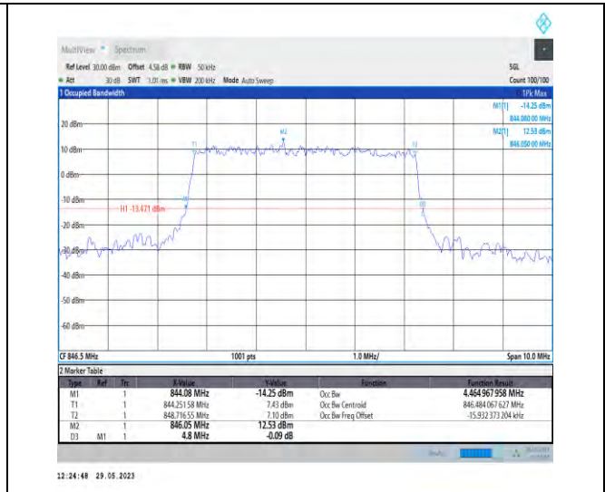
1-N5-PC3-15-5-H-4-DFT-64QAM-Outer_Full-25@0- Ant1-4.465-4.800-≤5-PASS
