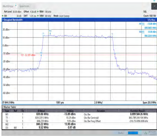
1-N5-PC3-15-10-H-2-DFT-PI2BPSK-Outer_Full-50@ 0-Ant1-8.9-9.520-≤10-PASS
