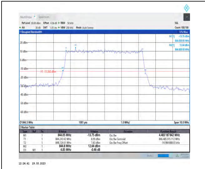
1-N5-PC3-15-5-H-3-DFT-16QAM-Outer_Full-25@0- Ant1-4.483-4.850-≤5-PASS
