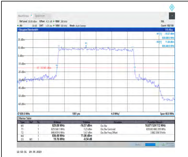
1-N5-PC3-15-20-H-8-CP-64QAM-Outer_Full-106@0 -Ant1-18.872-19.760-≤20-PASS
