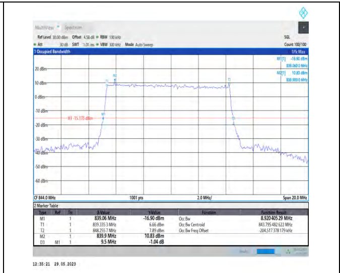
1-N5-PC3-15-10-H-5-DFT-256QAM-Outer_Full-50@0 -Ant1-8.92-9.500-≤10-PASS
