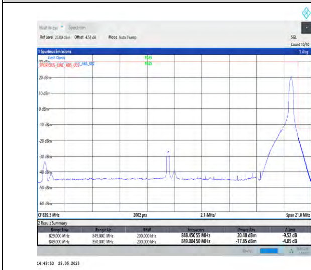
1-N5-PC3-15-20-H-5-CP-QPSK-Edge_1RB_Right-1@105-Ant1-1-seegraph-PASS-see graph
