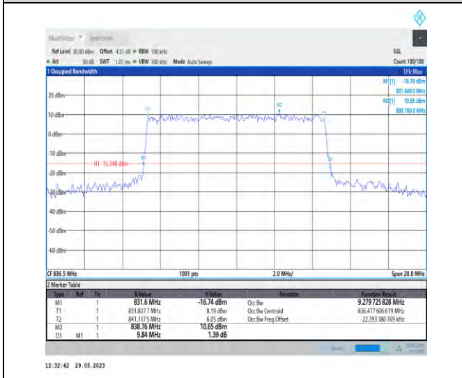
1-N5-PC3-15-10-M-7-CP-16QAM-Outer_Full-52@0-A nt1-9.28-9.840-≤10-PASS
