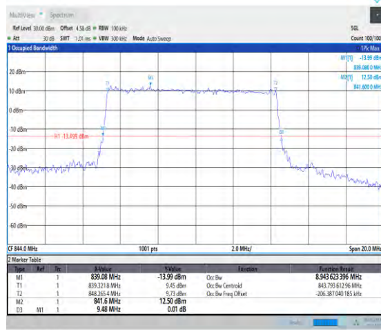
1-N5-PC3-15-10-H-3-DFT-16QAM-Outer_Full-50@0 -Ant1-8.944-9.480-≤10-PASS
