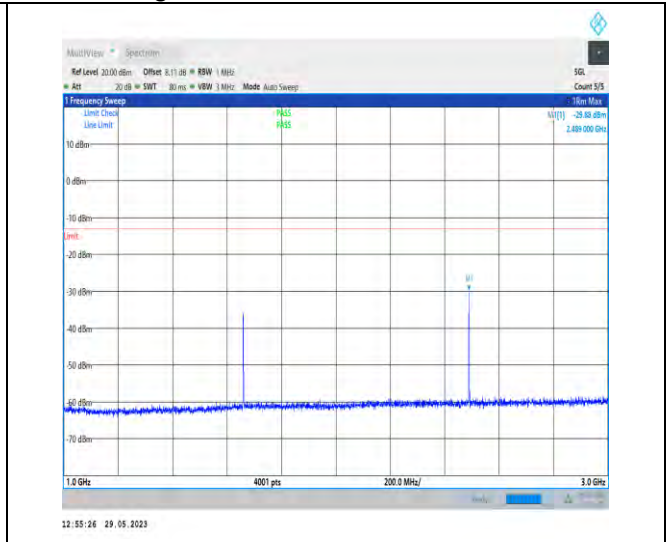
1-N5-PC3-15-20-H-1-N/A-DFT-PI2BPSK-Inner_1RB _Left-1@1-1000-3000-Ant1-2489.00--29.88--13-PAS S
