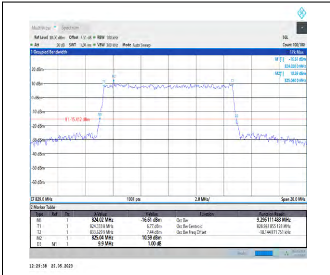
1-N5-PC3-15-10-L-6-CP-QPSK-Outer_Full-52@0-A Ant1-9.296-9.900-≤10-PASS
