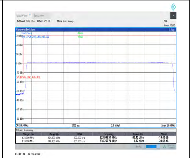
1-N5-PC3-15-20-L-6-CP-QPSK-Outer_Full-106@0-Ant1-1-seegraph-PASS-see graph
