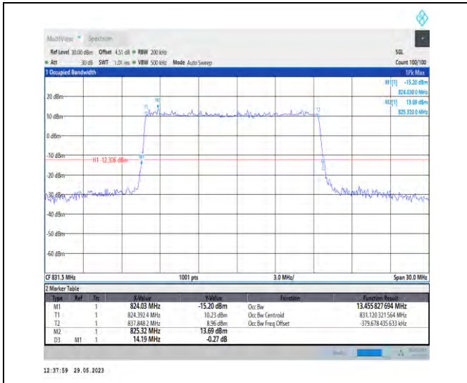
1-N5-PC3-15-15-L-3-DFT-16QAM-Outer_Full-75@0-Ant1-13.456-14.190-≤15-PASS
