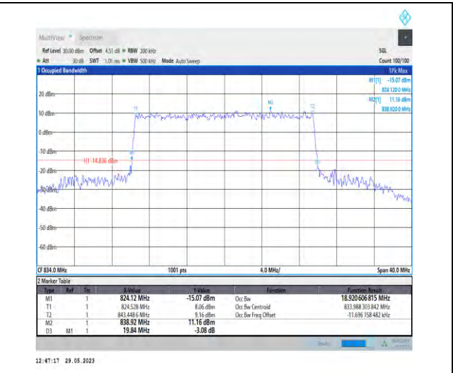
1-N5-PC3-15-20-L-7-CP-16QAM-Outer_Full-106@0-Ant1-18.921-19.840-≤20-PASS
