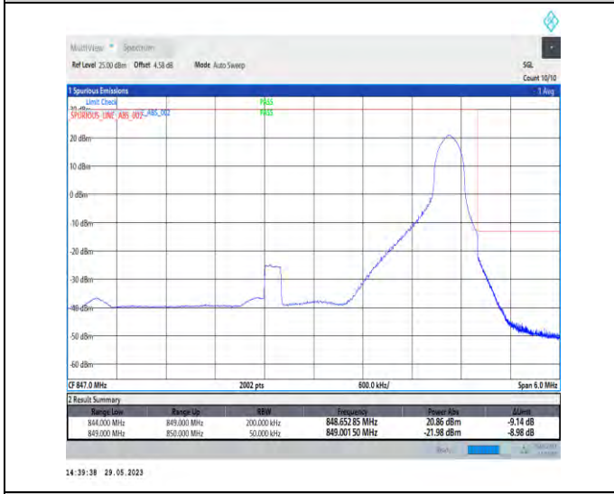
1-N5-PC3-15-5-H-5-CP-QPSK-Edge_1RB_Right-1@2 4-Ant1-1-seegraph-PASS-see graph
