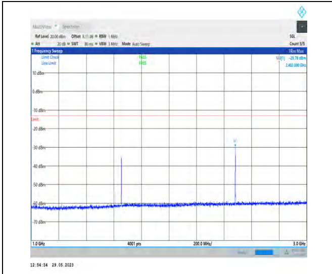
1-N5-PC3-15-20-M-1-N/A-DFT-PI2BPSK-Inner_1RB _Left-1@1-1000-3000-Ant1-2482.00--29.78--13-PAS S
