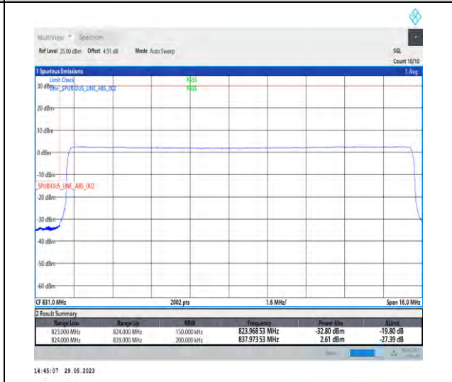
1-N5-PC3-15-15-L-6-CP-QPSK-Outer_Full-79@0-Ant1-1-seegraph-PASS-see graph
