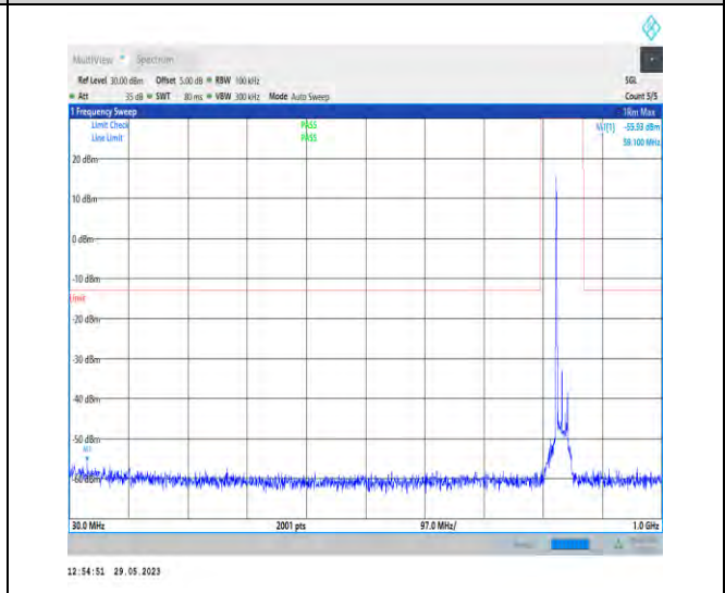
1-N5-PC3-15-20-M-1-N/A-DFT-PI2BPSK-Inner_1RB_Left-1@1-30-1000-Ant1-59.10--55.93--13-PASS
