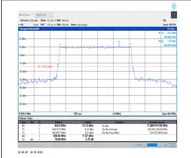
1-N5-PC3-15-20-L-4-DFT-64QAM-Outer_Full-100 @0-Ant1-17.889-18.960-<=20-PASS
