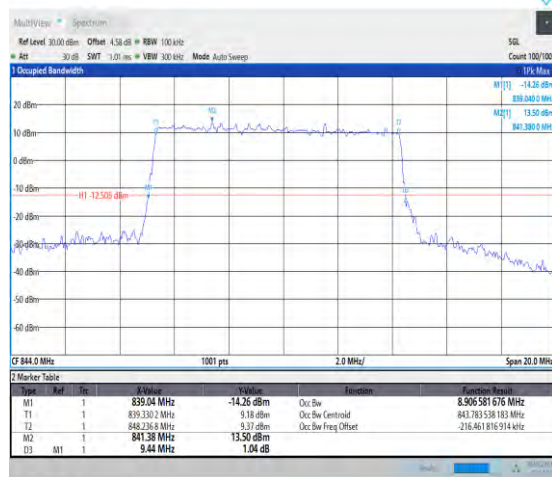
1-N5-PC3-15-10-H-1-DFT-QPSK-Outer_Full-50@0- Ant1-8.907-9.440-≤10-PASS
