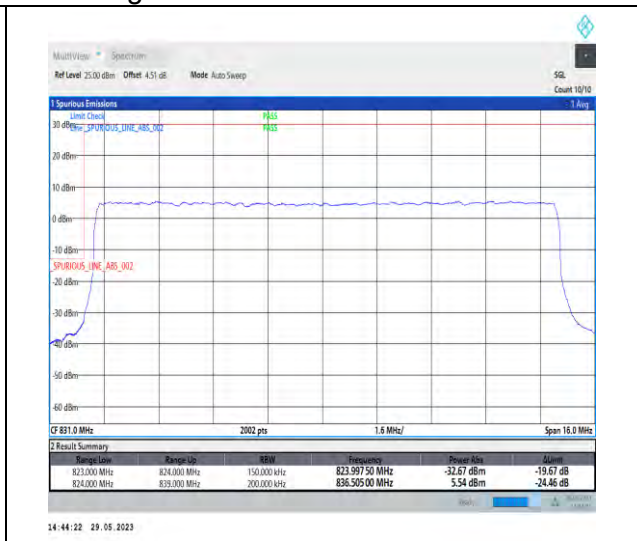
1-N5-PC3-15-15-L-3-DFT-PI2BPSK-Outer_Full-75 @0-Ant1-1-seegraph-PASS-see graph
