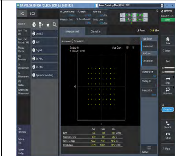
1-N5-PC3-15-20-M-8-CP-64QAM-Outer_Full-106@0-Ant1-see graph-PASS
