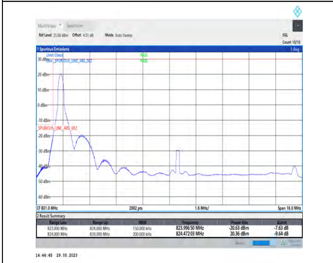
1-N5-PC3-15-15-L-4-CP-QPSK-Edge_1RB_Left-1@0-Ant1-1-seegraph-PASS-see graph
