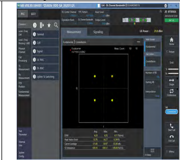
1-N5-PC3-15-20-M-6-CP-QPSK-Outer_Full-106@0-Ant1-see graph-PASS
