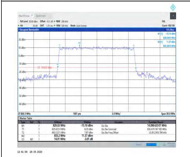
1-N5-PC3-15-15-M-8-CP-64QAM-Outer_Full-79@0- Ant1-14.097-14.910-≤15-PASS
