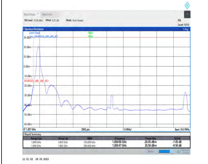
1-N2-PC3-15-15-L-4-CP-QPSK-Edge_1RB_Left-1@0-Ant1-1-seegraph-PASS-see graph
