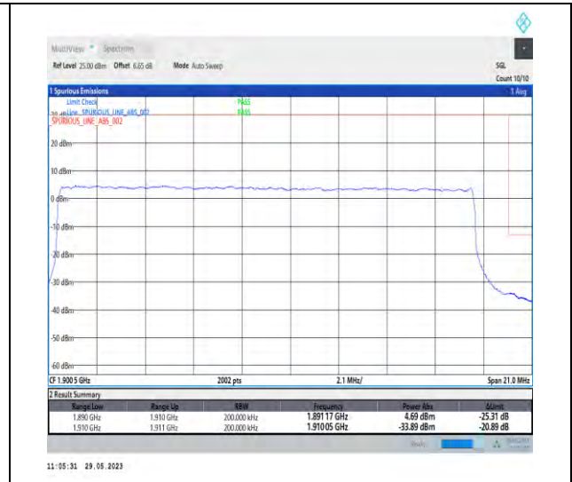
1-N2-PC3-15-20-H-3-DFT-PI2BPSK-Outer_Full-100@0-Ant1-1-seegraph-PASS-see graph
