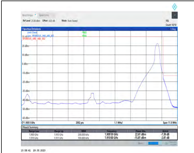
1-N2-PC3-15-10-H-2-DFT-PI2BPSK-Edge_1RB_Right-1@51-Ant1-1-seegraph-PASS-see graph
