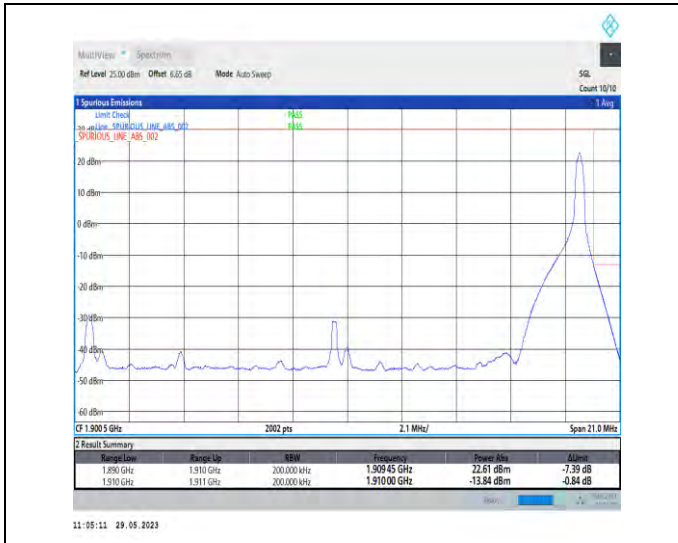
1-N2-PC3-15-20-H-2-DFT-PI2BPSK-Edge_1RB_Right-1@105-Ant1-1-seegraph-PASS-see graph
