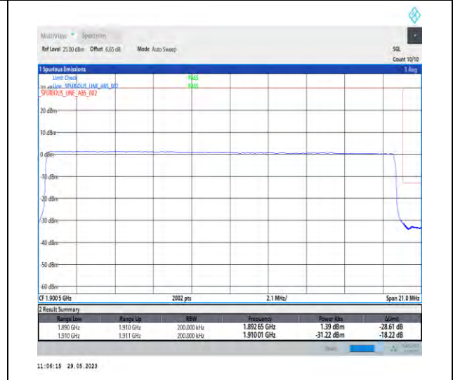
1-N2-PC3-15-20-H-6-CP-QPSK-Outer_Full-106@0-Ant1-1-seegraph-PASS-see graph
