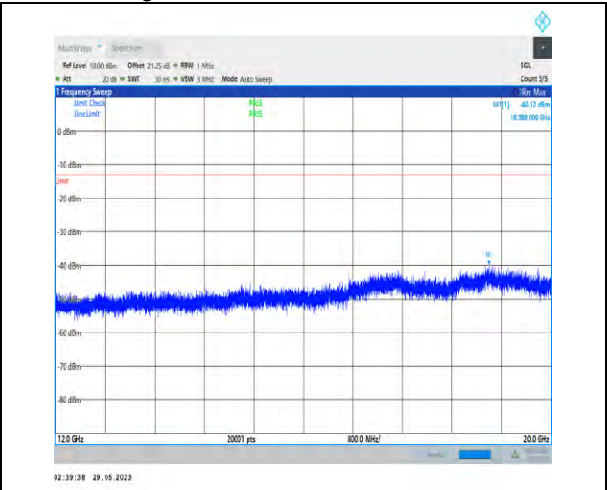
1-N2-PC3-15-20-H-1-N/A-DFT-PI2BPSK-Inner_1RB _Left-1@1-12000-20000-Ant1-18988.00--40.12--13-PA SS
