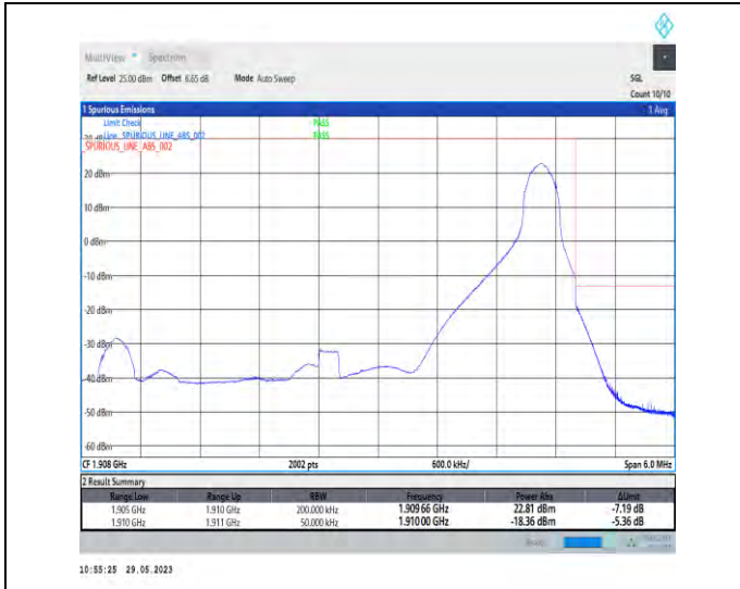
1-N2-PC3-15-5-H-2-DFT-PI2BPSK-Edge_1RB_Right-1 @24-Ant1-1-seegraph-PASS-see graph
