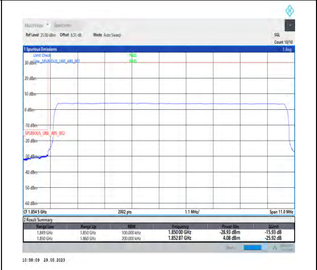
1-N2-PC3-15-10-L-6-CP-QPSK-Outer_Full-52@0-Ant1-1-seegraph-PASS-see graph
