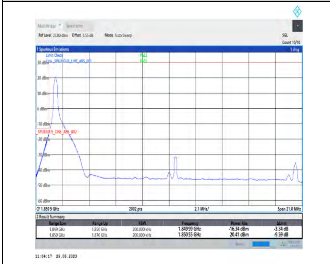
1-N2-PC3-15-20-L-4-CP-QPSK-Edge_1RB_Left-1@0-Ant1-1-seegraph-PASS-see graph
