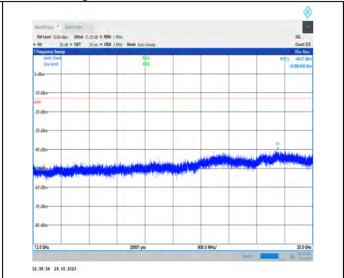
1-N2-PC3-15-20-L-1-N/A-DFT-PI2BPSK-Inner_1RB _Left-1@1-12000-20000-Ant1-18998.80--40.47--13-PA-SS
