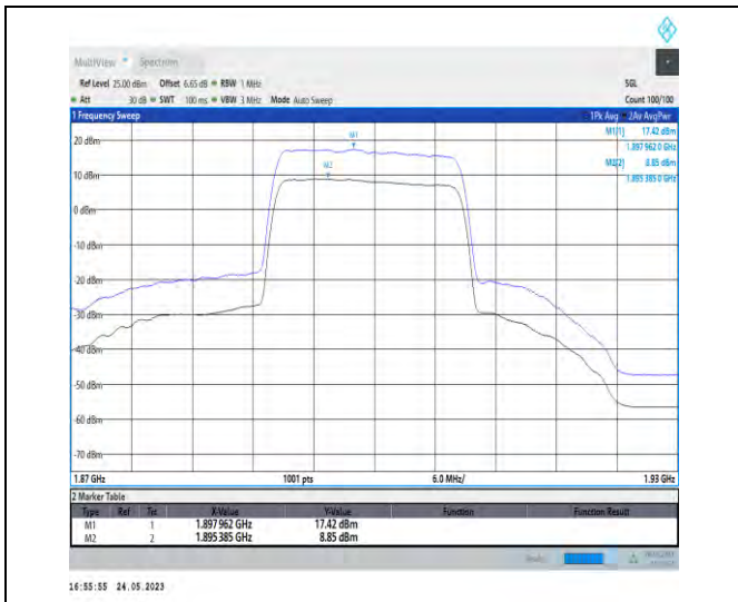
1-N2-PC3-15-20-H-1-DFT-256QAM-Outer_Full-100 @0-Ant1-8.57-100%-0.00-8.57-PASS-≤13
