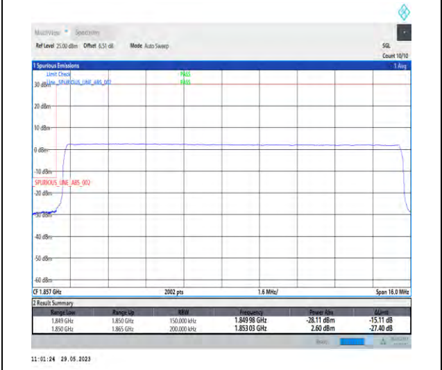
1-N2-PC3-15-15-L-6-CP-QPSK-Outer_Full-79@0-Ant1-1-seegraph-PASS-see graph
