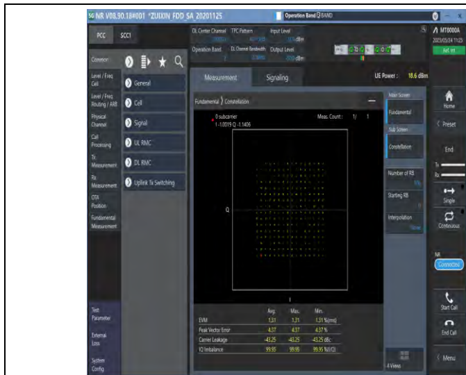
1-N2-PC3-15-20-M-9-CP-256QAM-Outer_Full-106@0-Ant1-see graph-PASS
