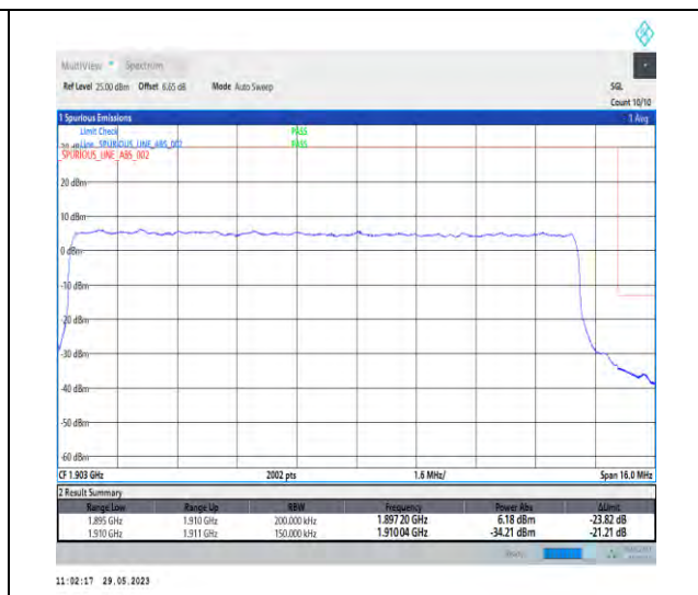
1-N2-PC3-15-15-H-3-DFT-PI2BPSK-Outer_Full-75 @0-Ant1-1-seegraph-PASS-see graph
