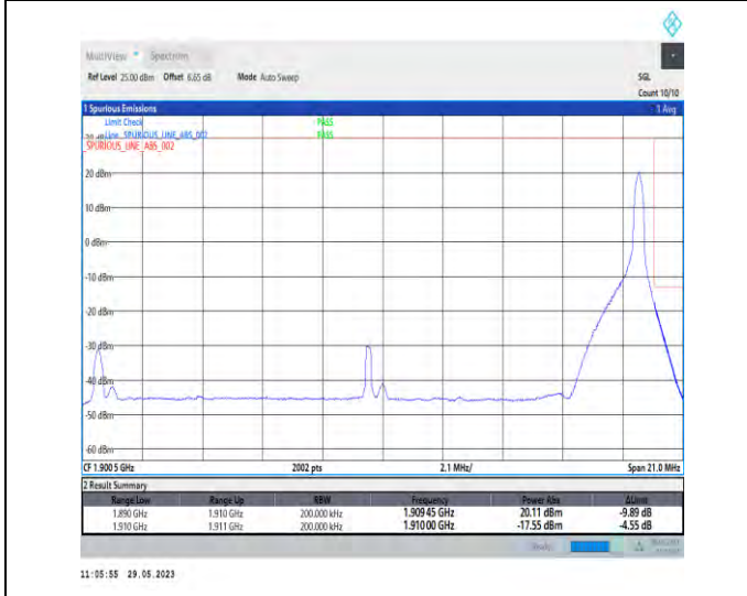
1-N2-PC3-15-20-H-5-CP-QPSK-Edge_1RB_Right-1@105-Ant1-1-seegraph-PASS-see graph
