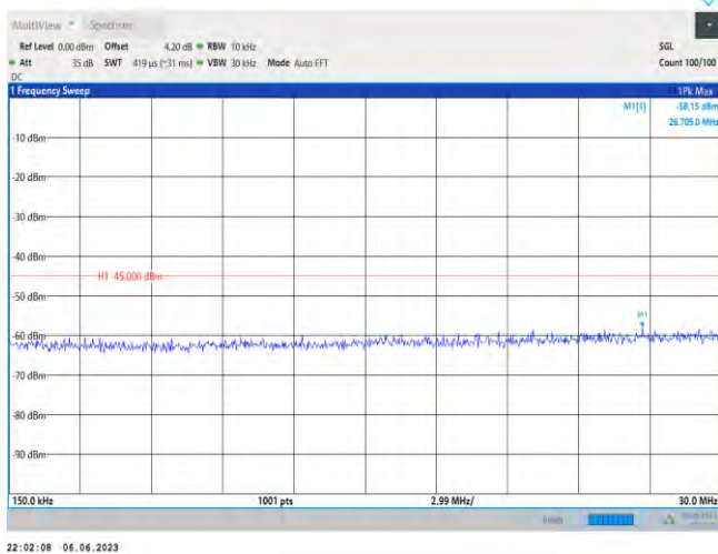
41-41-20MHz-20MHz-QPSK-QPSK-41292-41490-1RB#0-0RB#0-0.15~30MHz
