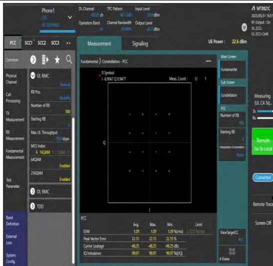
41-41-20MHz-20MHz-16QAM-16QAM-40521-40719-100RB#0-100RB#0
