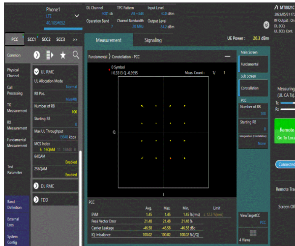
7-7-20MHz-20MHz-16QAM-16QAM-21001-21199-100RB#0-100RB#0
