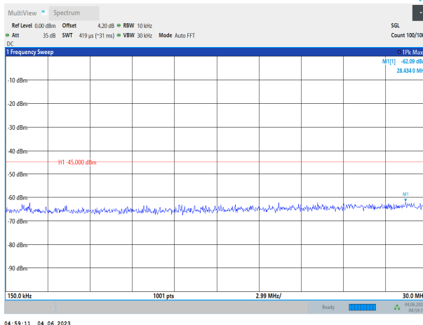
7-7-20MHz-20MHz-QPSK-QPSK-21001-21199-1RB#0-0RB#0-0.15~30MHz
