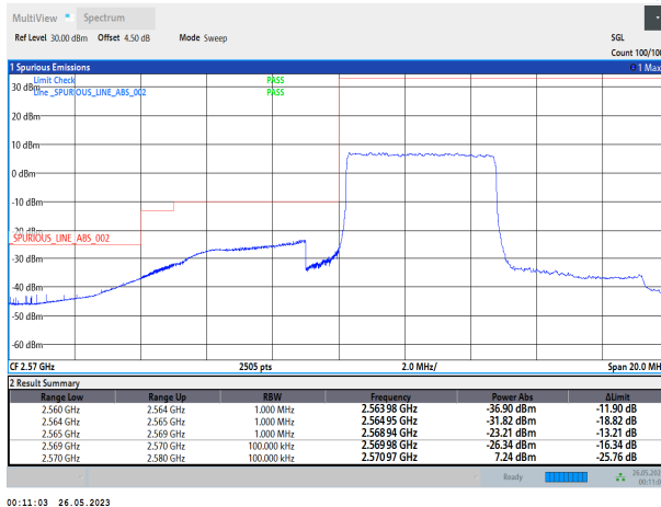
Band38-5MHz-QPSK-37775-25RB#0
