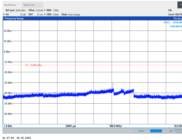
Band26-10MHz-QPSK-26740-1RB#0-Range4:1000~10000MHz
