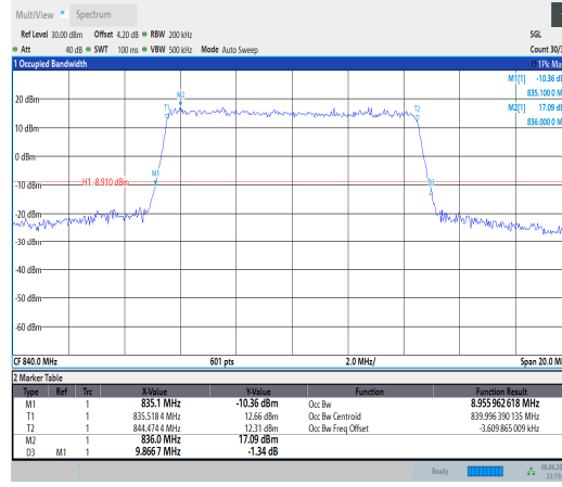
Band19-10MHz-16QAM-24100-50RB#0
