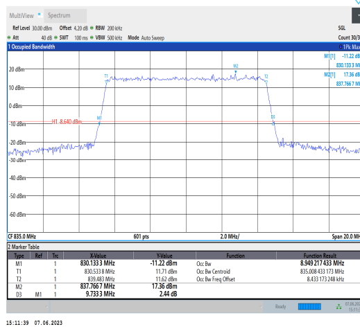
Band19-10MHz-64QAM-24050-50RB#0
