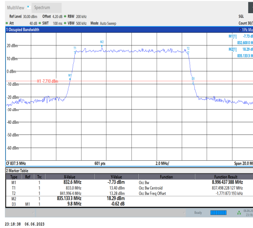
Band19-10MHz-QPSK-24075-50RB#0
