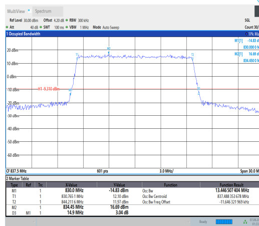
Band19-15MHz-16QAM-24075-75RB#0
