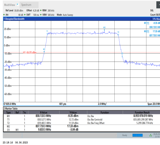
Band19-10MHz-16QAM-24050-50RB#0
