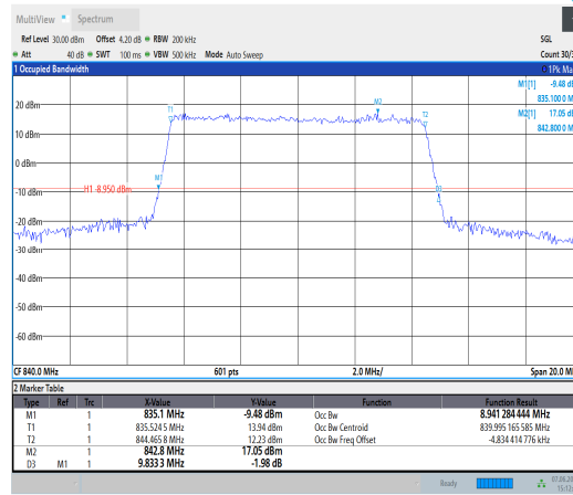
Band19-10MHz-64QAM-24100-50RB#0
