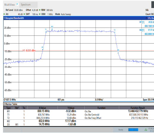
Band19-15MHz-QPSK-24075-75RB#0
