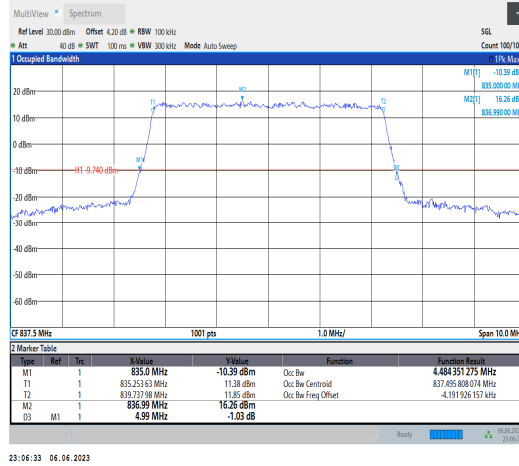
Band19-5MHz-16QAM-24075-25RB#0
