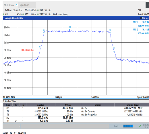
Band19-5MHz-64QAM-24075-25RB#0
