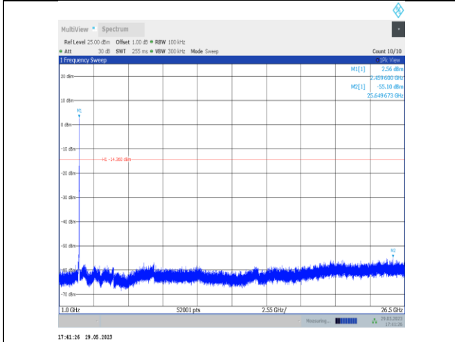
11VHT20SISO-Ant22-2462-1000~26500
