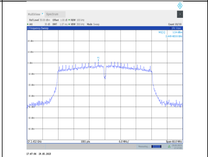
11VHT40SISO-Ant22-2452-0~Reference
