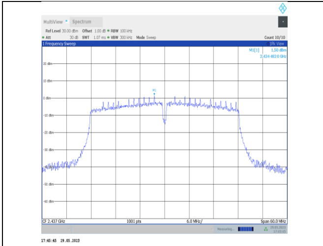
11VHT40SISO-Ant22-2437-0~Reference
