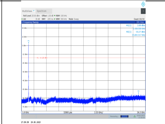
11VHT20SISO-Ant22-2437-1000~26500
