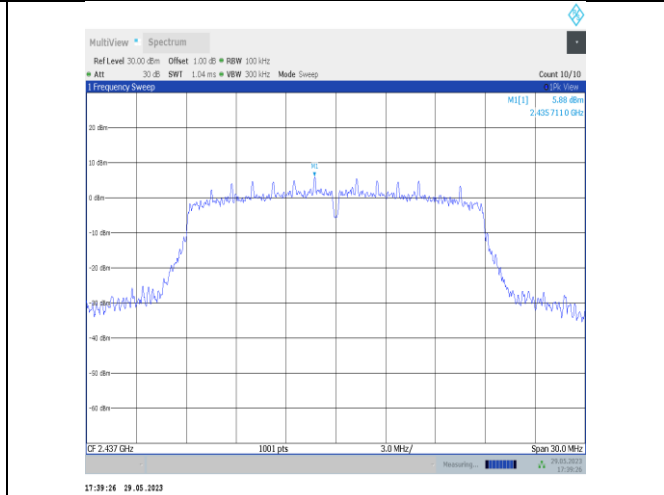
11VHT20SISO-Ant22-2437-0~Reference
