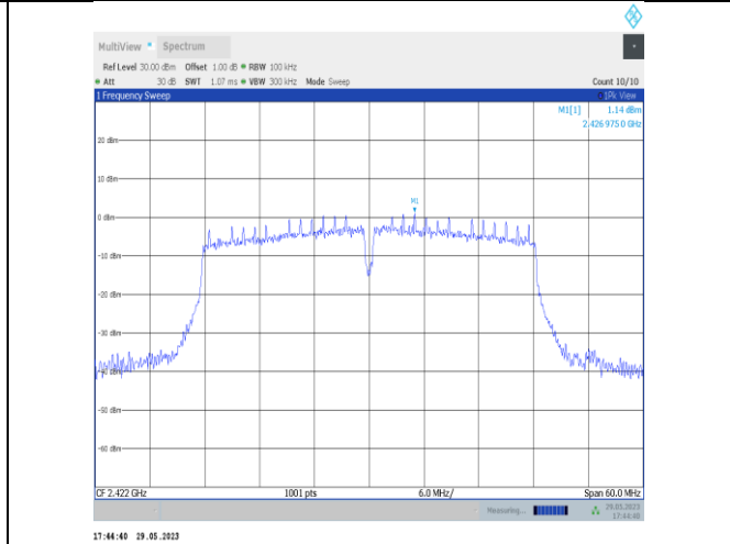
11VHT40SISO-Ant22-2422-0~Reference
