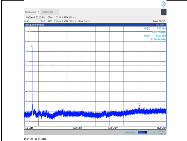
11VHT20SISO-Ant22-2412-1000~26500
