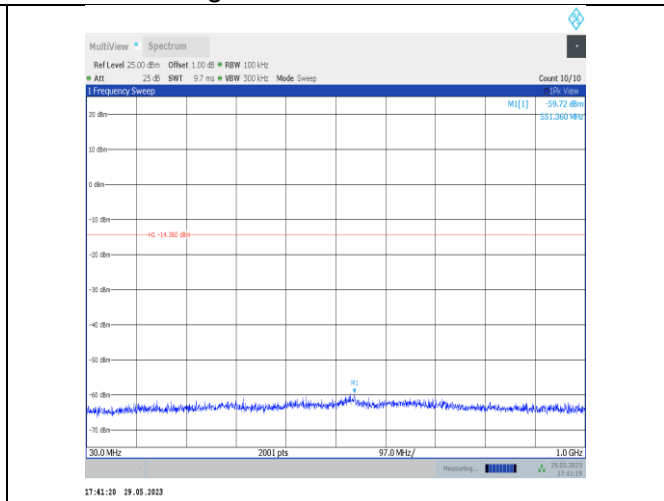
11VHT20SISO-Ant22-2462-30~1000
