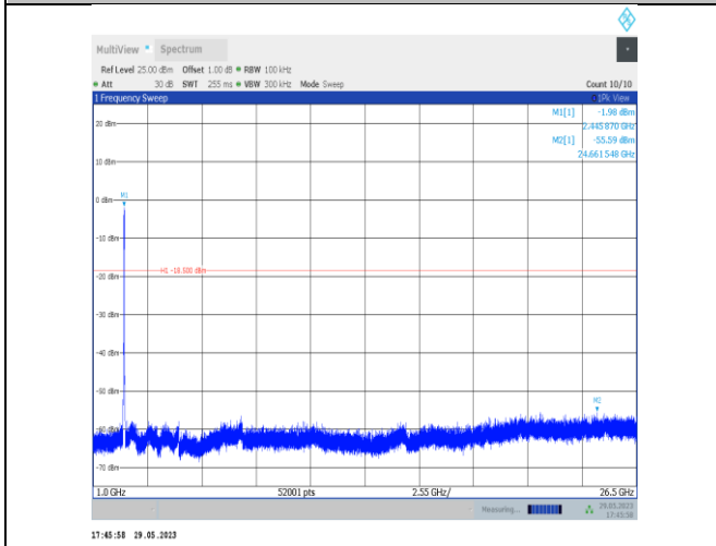
11VHT40SISO-Ant22-2437-1000~26500
