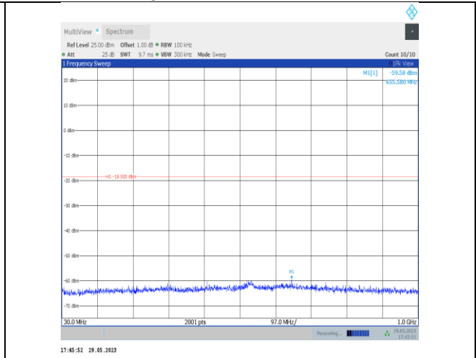
11VHT40SISO-Ant22-2437-30~1000
