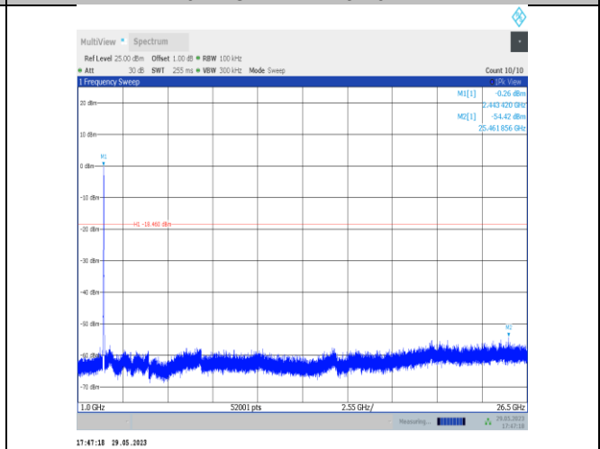
11VHT40SISO-Ant22-2452-1000~26500
