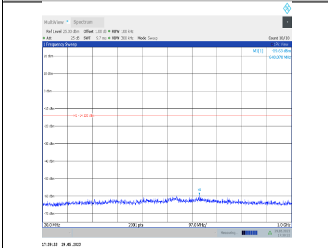
11VHT20SISO-Ant22-2437-30~1000
