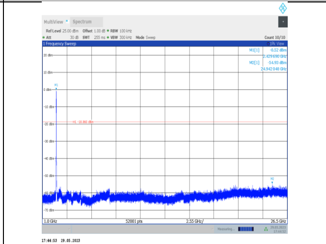
11VHT40SISO-Ant22-2422-1000~26500
