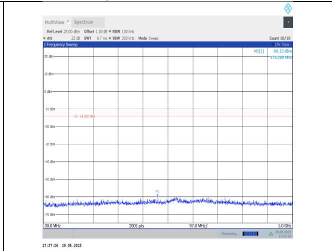
11VHT20SISO-Ant22-2412-30~1000
