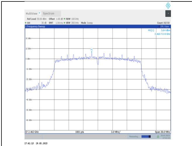
11VHT20SISO-Ant22-2462-0~Reference
