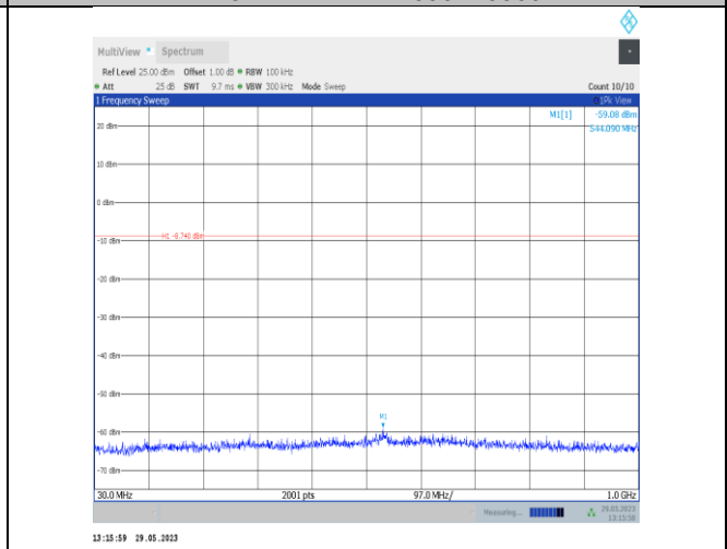
DH5-Ant22-2480-30~1000
