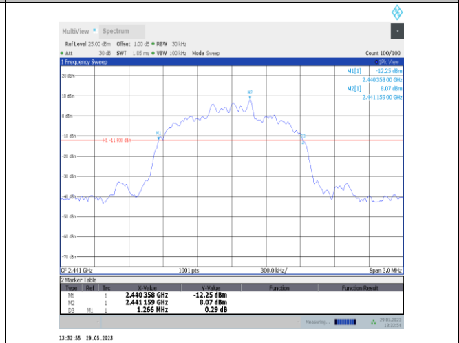
3DH5-Ant22-2441
