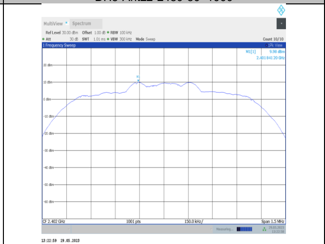
2DH5-Ant22-2402-0~Reference
