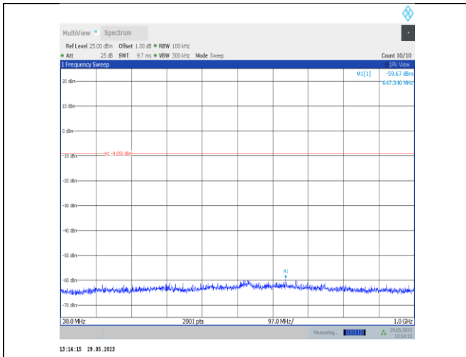
DH5-Ant22-2441-30~1000
