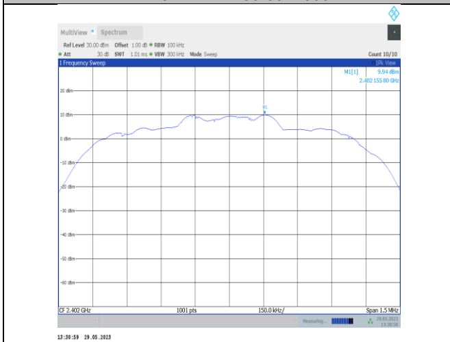
3DH5-Ant22-2402-0~Reference
