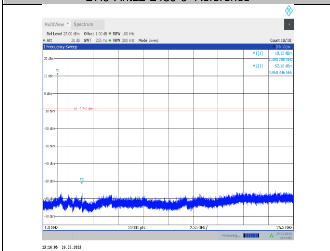
DH5-Ant22-2480-1000~26500
