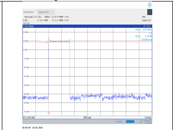
2DH3-Ant22-Hop
