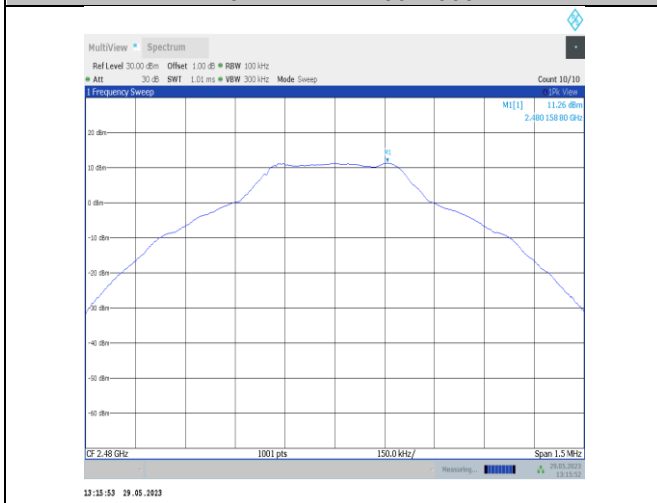
DH5-Ant22-2480-0~Reference
