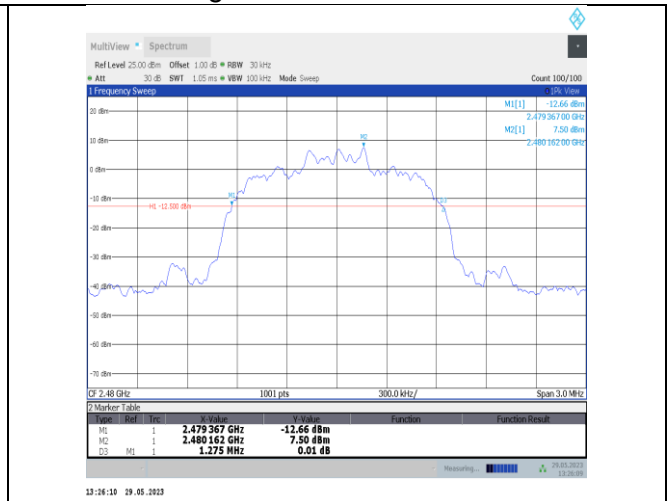
2DH5-Ant22-2480
