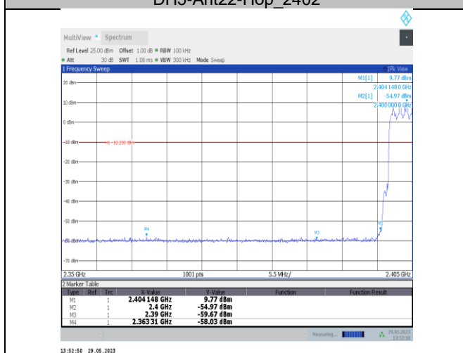
2DH5-Ant22-Hop_2402
