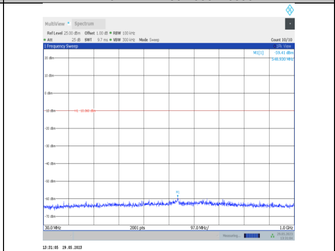
3DH5-Ant22-2402-30~1000
