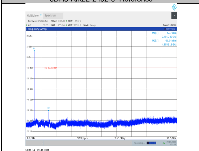
3DH5-Ant22-2402-1000~26500
