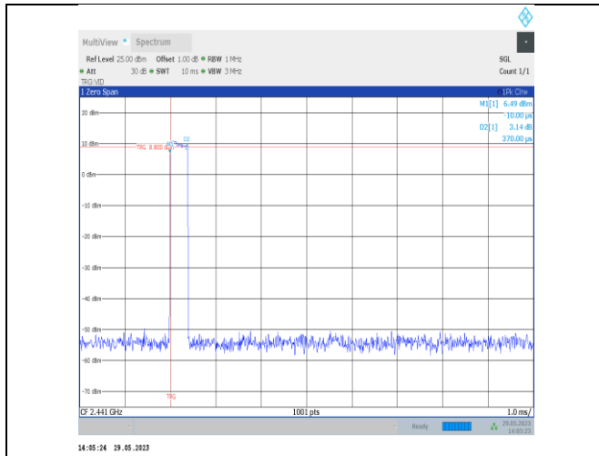
2DH1-Ant22-Hop
