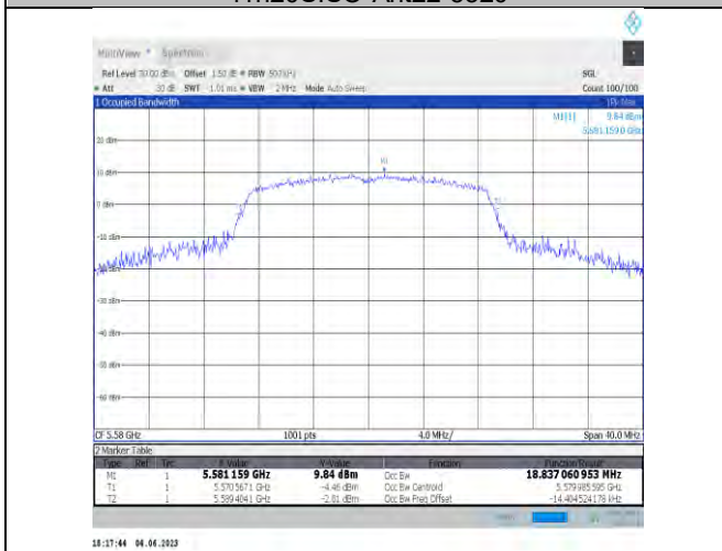
11n20SISO-Ant22-5580
