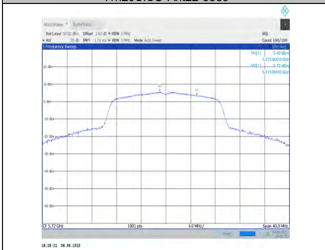
11n20SISO-Ant22-5720 UNII-2C
