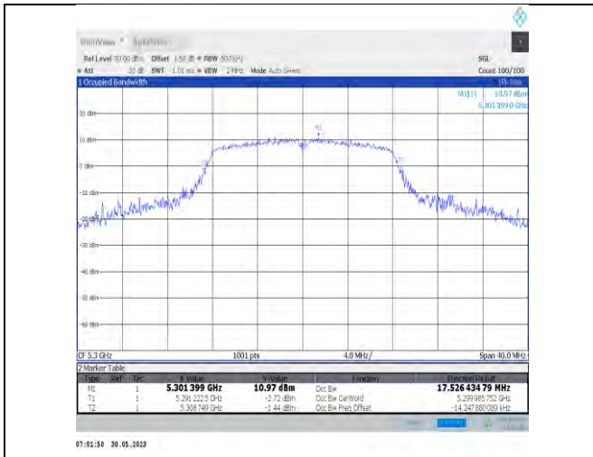
11a-Ant22-5300
