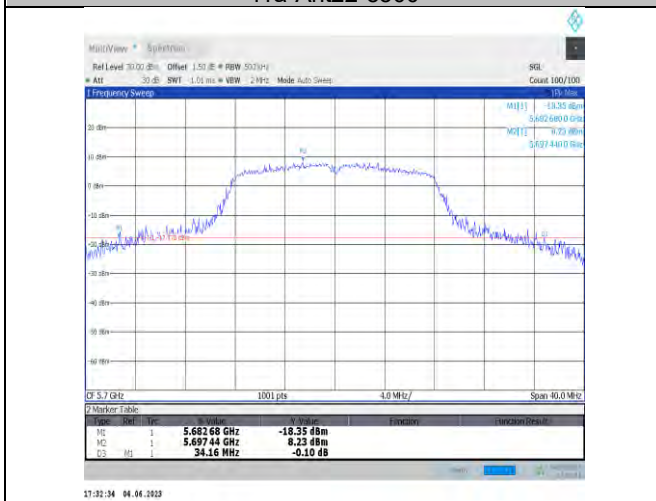
11a-Ant22-5700
