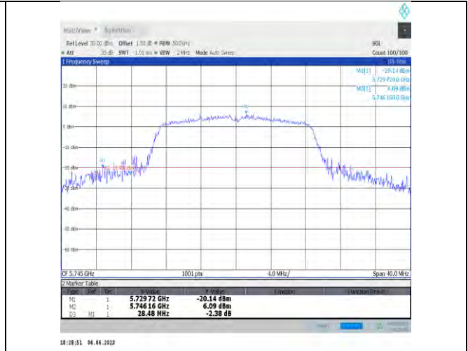
11n20SISO-Ant22-5745
