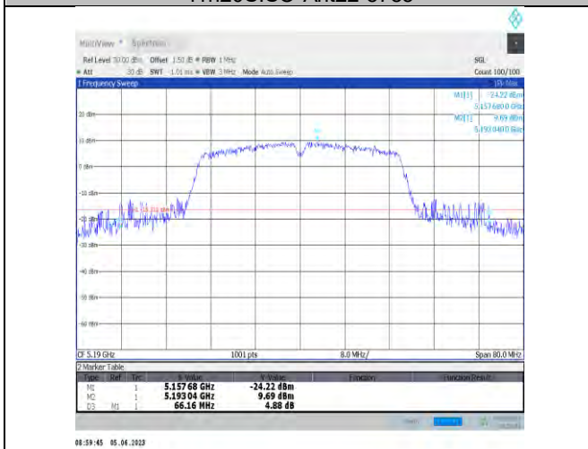
11n40SISO-Ant22-5190
