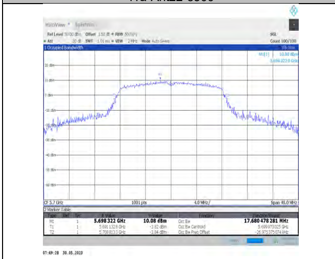
11a-Ant22-5700
