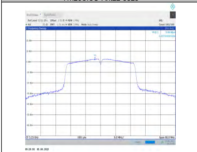
11n40SISO-Ant22-5230
