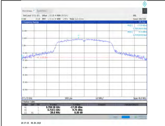
11n20SISO-Ant22-5720
