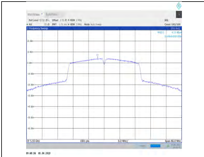
11n40SISO-Ant22-5550
