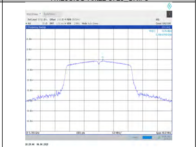
11n20SISO-Ant22-5785
