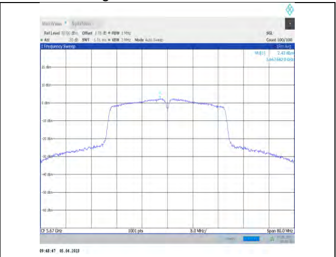
11n40SISO-Ant22-5670
