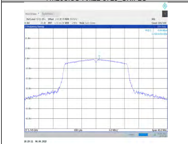
11n20SISO-Ant22-5745
