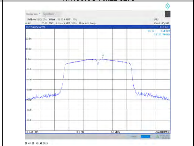
11n40SISO-Ant22-5510
