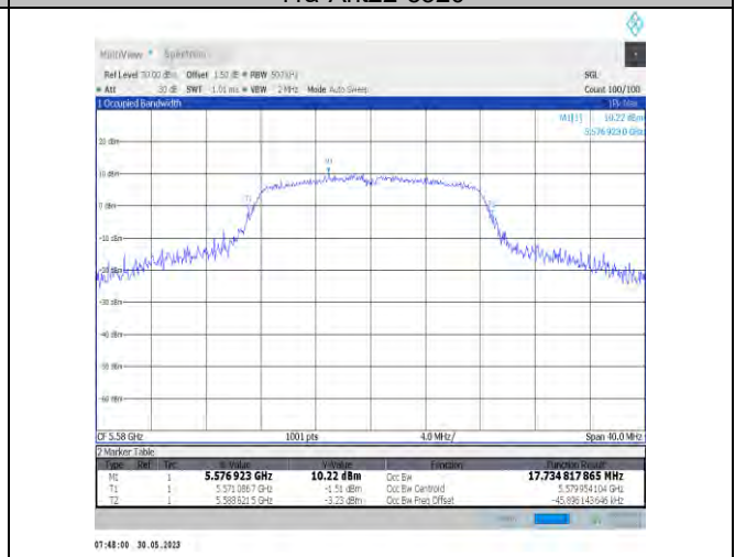
11a-Ant22-5580
