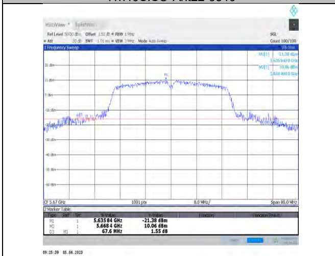
11n40SISO-Ant22-5670
