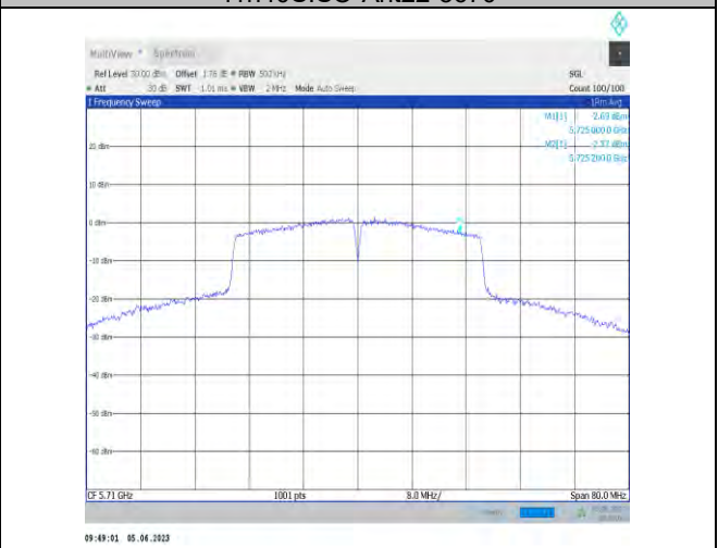
11n40SISO-Ant22-5710 UNII-3
