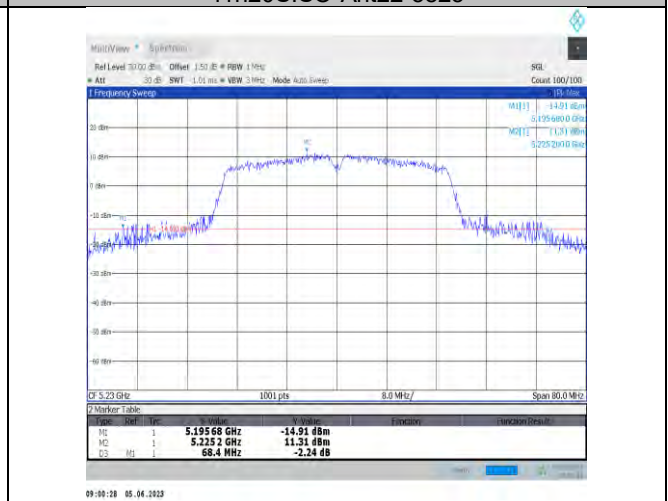
11n40SISO-Ant22-5230
