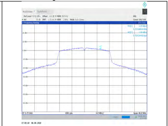
11a-Ant22-5720 UNII-3
