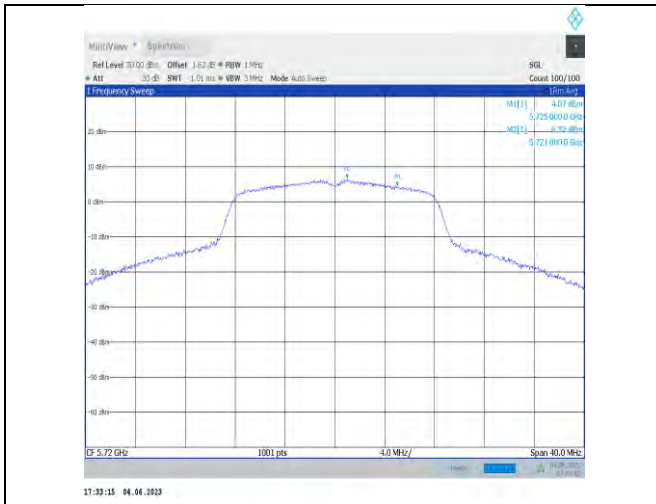
11a-Ant22-5720 UNII-2C
