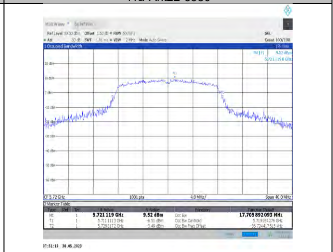
11a-Ant22-5720
