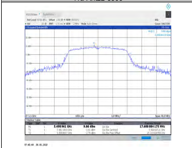
11a-Ant22-5500
