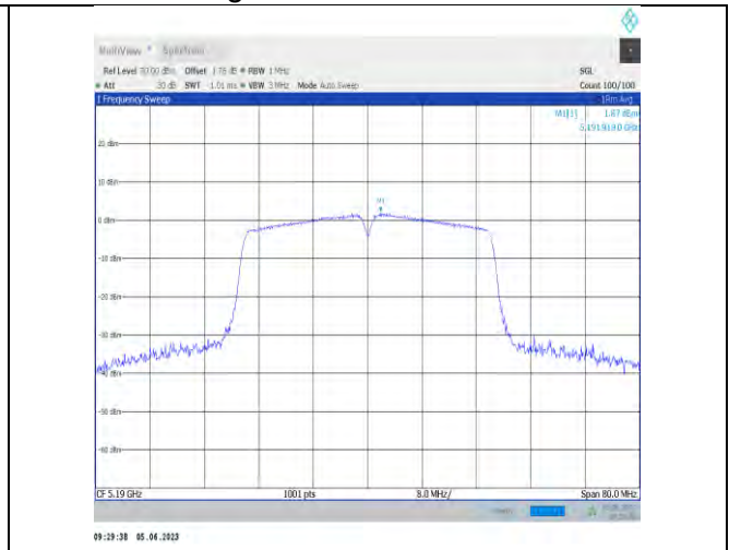
11n40SISO-Ant22-5190
