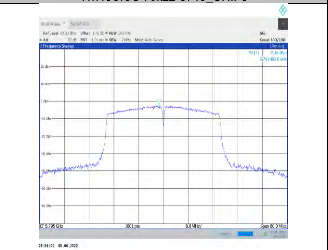
11n40SISO-Ant22-5795
