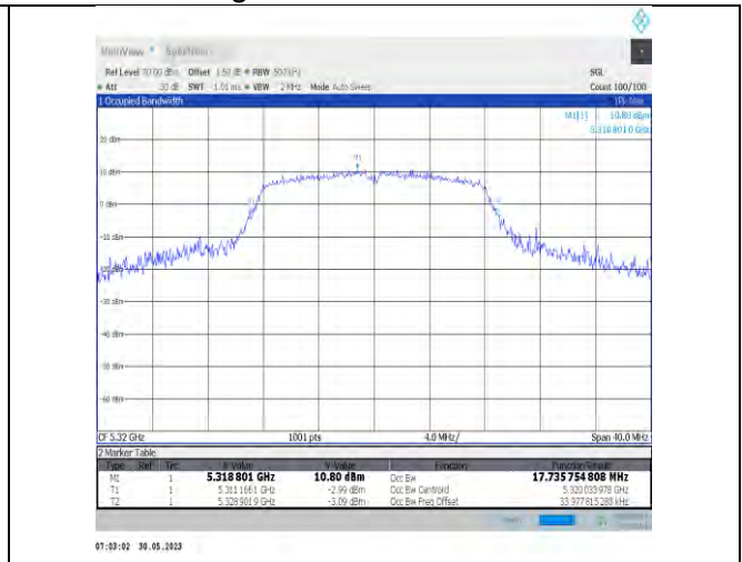
11a-Ant22-5320
