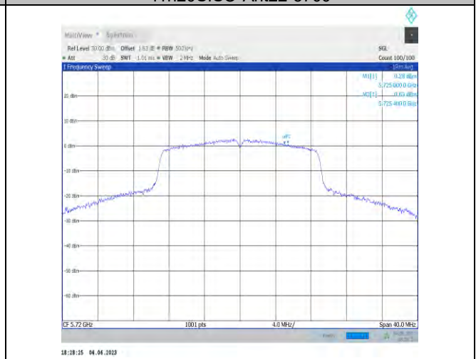
11n20SISO-Ant22-5720 UNII-3
