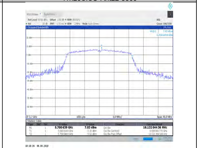
11n20SISO-Ant22-5700
