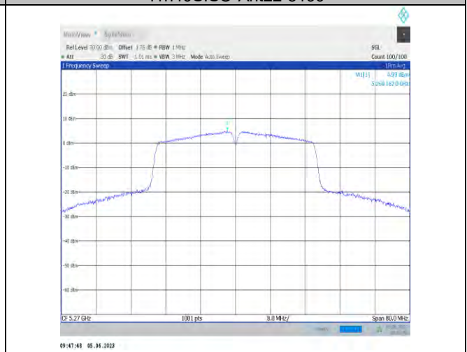
11n40SISO-Ant22-5270
