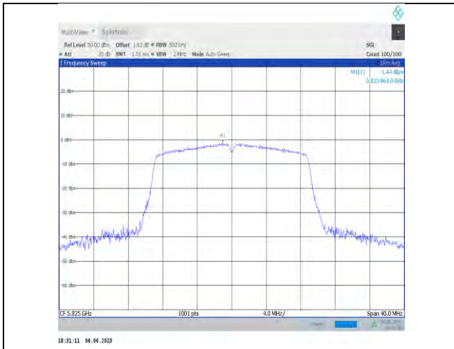
11n20SISO-Ant22-5825
