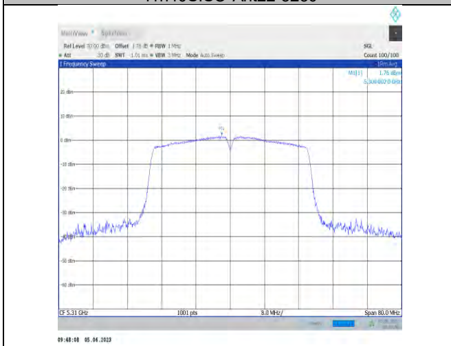
11n40SISO-Ant22-5310
