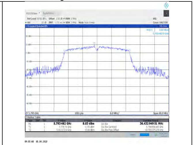
11n40SISO-Ant22-5795
