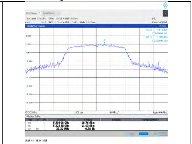
11a-Ant22-5320
