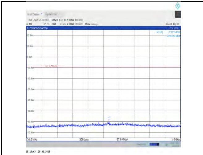
11b-Ant22-2437-30~1000
