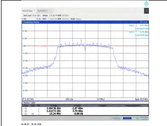
11n20SISO-Ant22-2412
