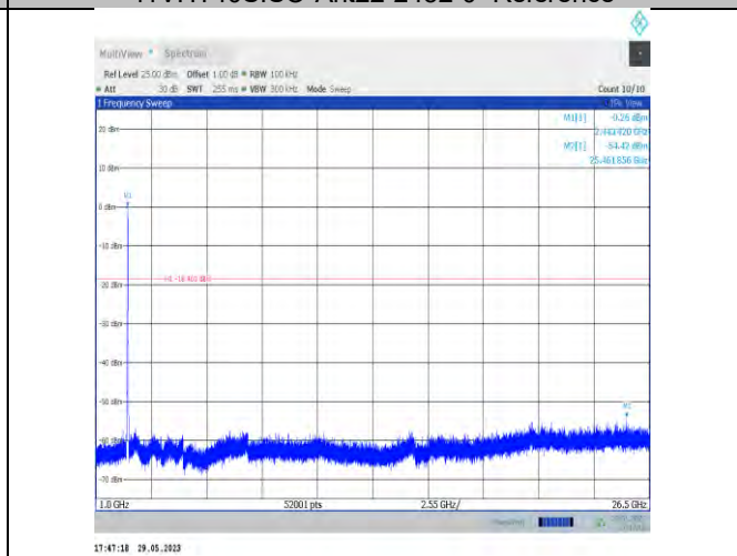
11VHT40SISO-Ant22-2452-1000~26500
