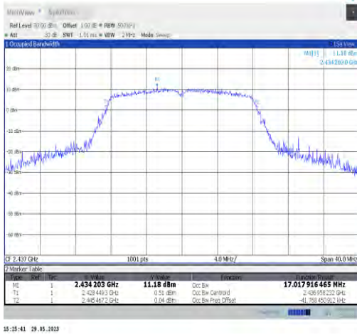
11g-Ant22-2437
