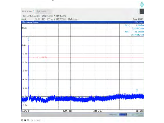
11n20SISO-Ant22-2437-1000~26500
