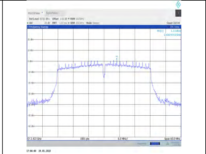
11VHT40SISO-Ant22-2422-0~Reference
