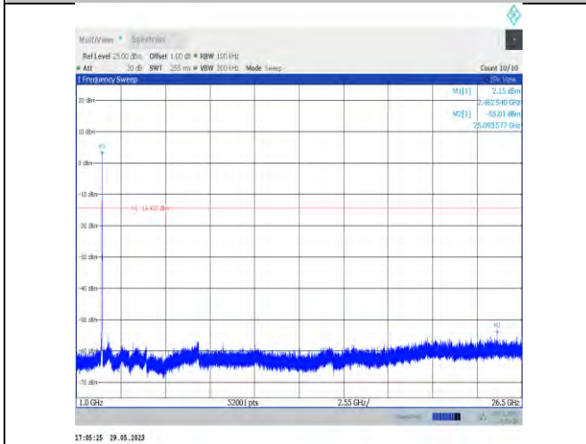
11n20SISO-Ant22-2462-1000~26500
