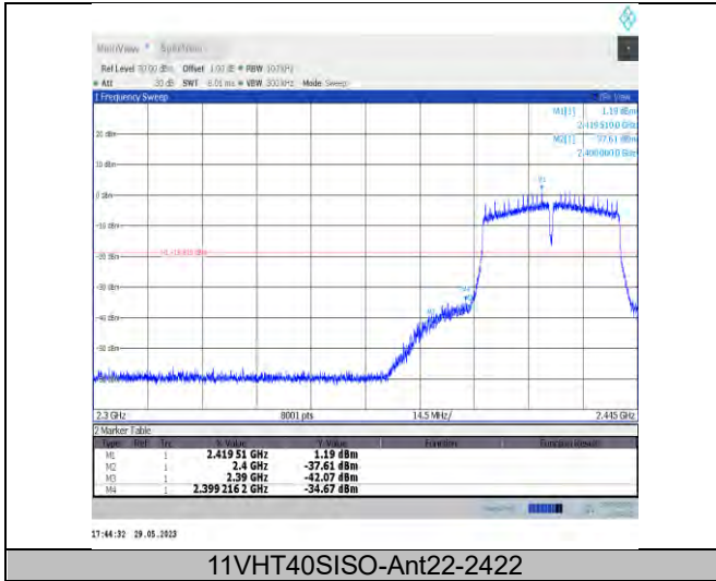
11VHT40SISO-Ant22-2422
