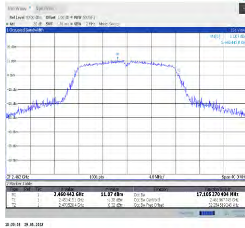
11g-Ant22-2462
