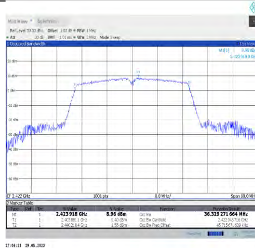
11n40SISO-Ant22-2422
