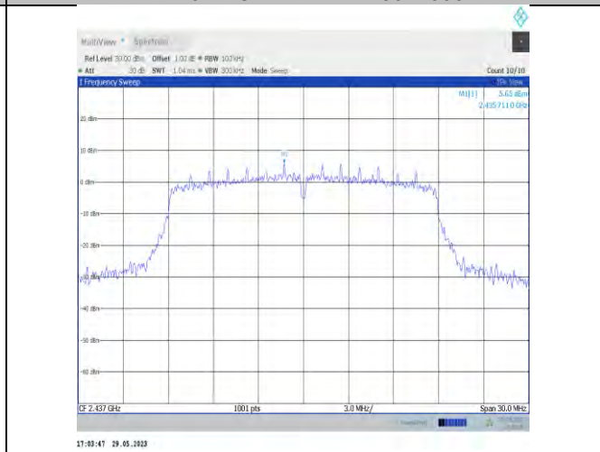
11n20SISO-Ant22-2437-0~Reference
