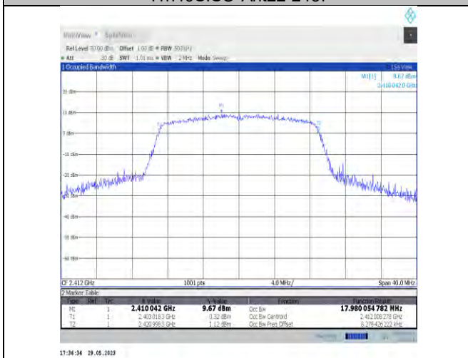
11VHT20SISO-Ant22-2412
