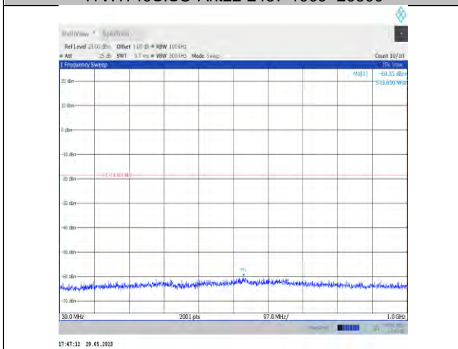
11VHT40SISO-Ant22-2452-30~1000
