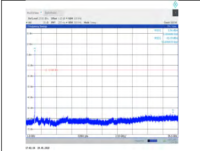
11VHT20SISO-Ant22-2462-1000~26500
