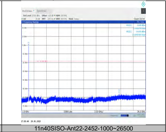
11n40SISO-Ant22-2452-1000~26500
