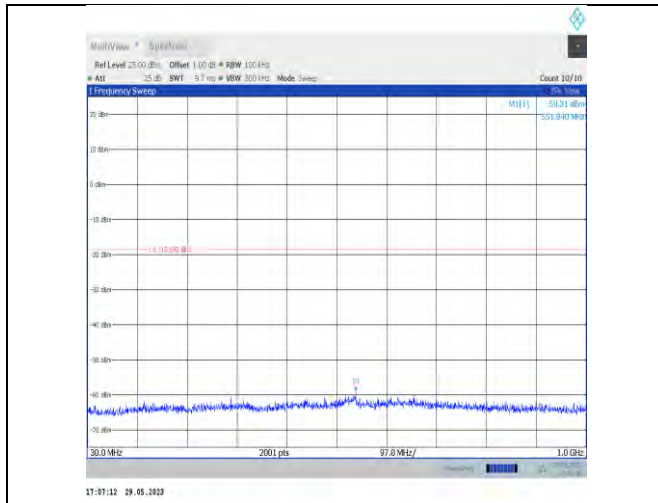
11n40SISO-Ant22-2422-30~1000
