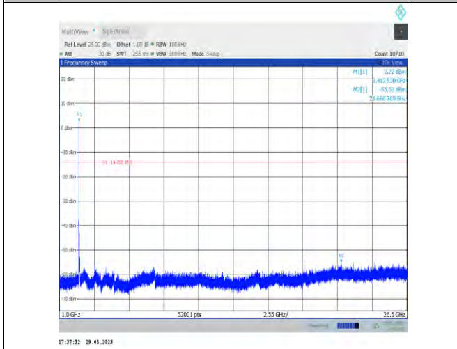
11VHT20SISO-Ant22-2412-1000~26500
