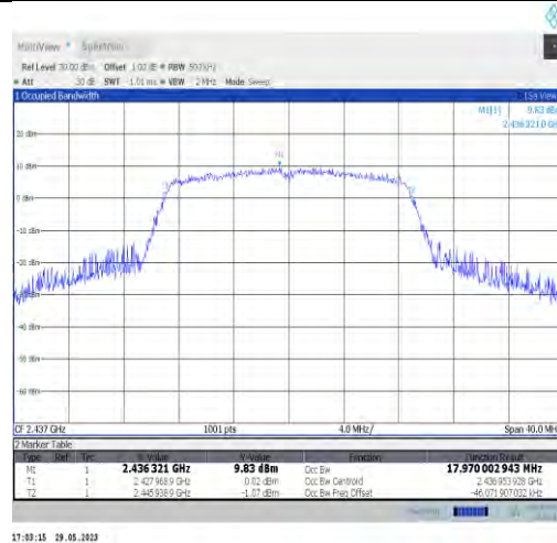
11n20SISO-Ant22-2437
