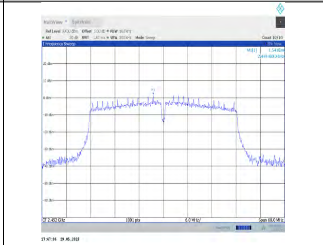
11VHT40SISO-Ant22-2452-0~Reference
