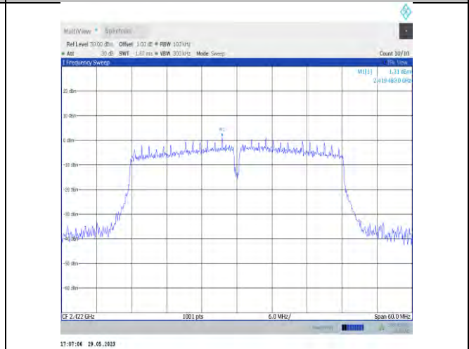
11n40SISO-Ant22-2422-0~Reference
