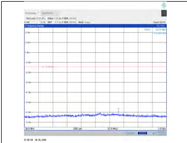
11n20SISO-Ant22-2437-30~1000
