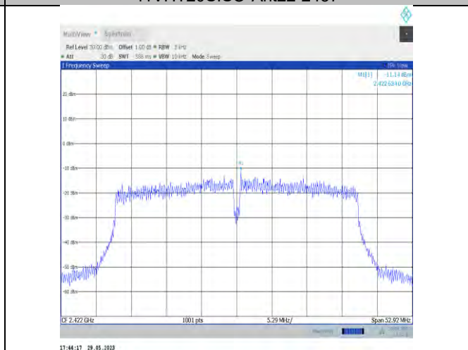
11VHT40SISO-Ant22-2422
