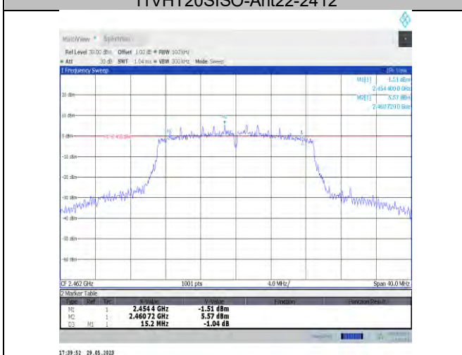
11VHT20SISO-Ant22-2462
