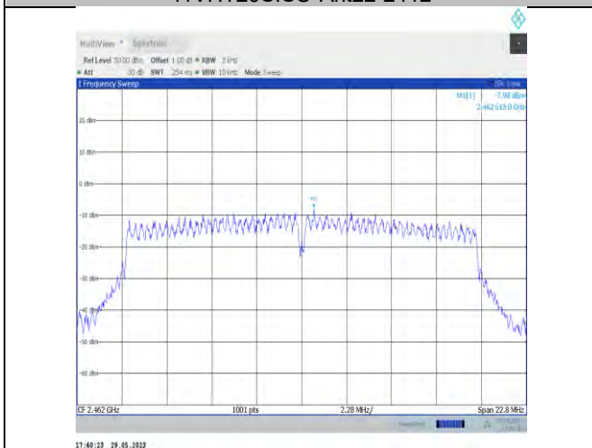
11VHT20SISO-Ant22-2462
