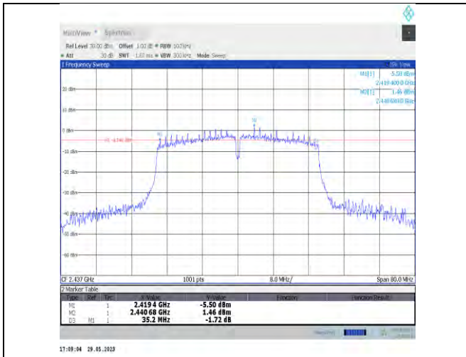
11n40SISO-Ant22-2437
