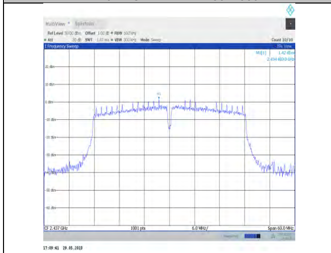
11n40SISO-Ant22-2437-0~Reference
