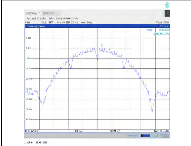
11b-Ant22-2462-0~Reference
