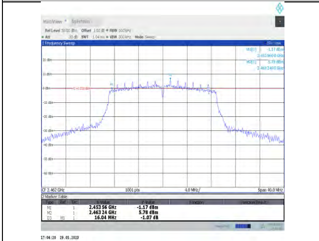
11n20SISO-Ant22-2462
