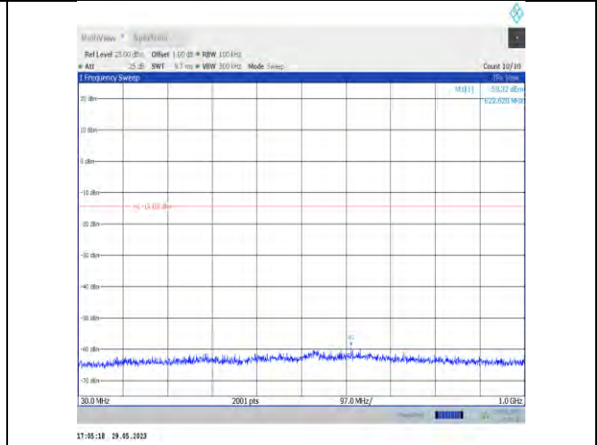
11n20SISO-Ant22-2462-30~1000
