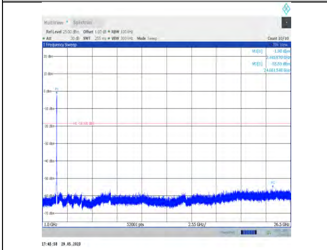
11VHT40SISO-Ant22-2437-1000~26500
