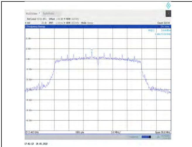
11VHT20SISO-Ant22-2462-0~Reference
