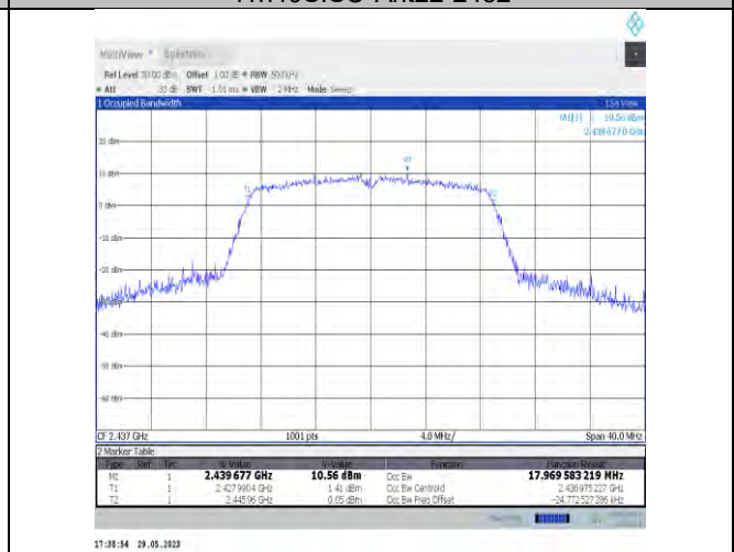
11VHT20SISO-Ant22-2437
