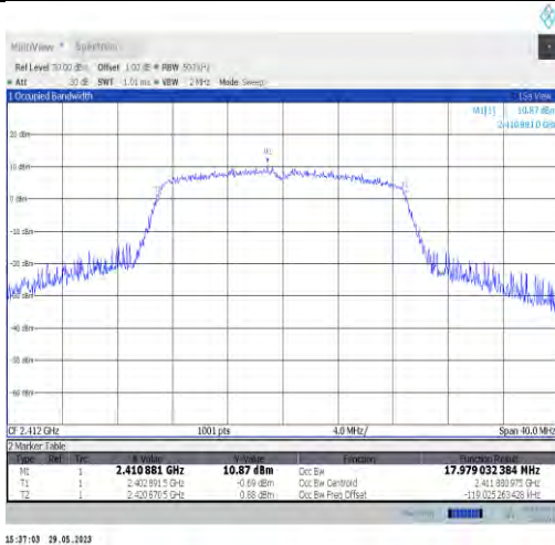
11n20SISO-Ant22-2412
