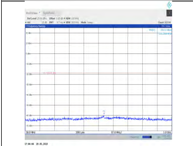
11VHT40SISO-Ant22-2422-30~1000
