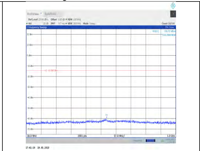
11VHT20SISO-Ant22-2462-30~1000
