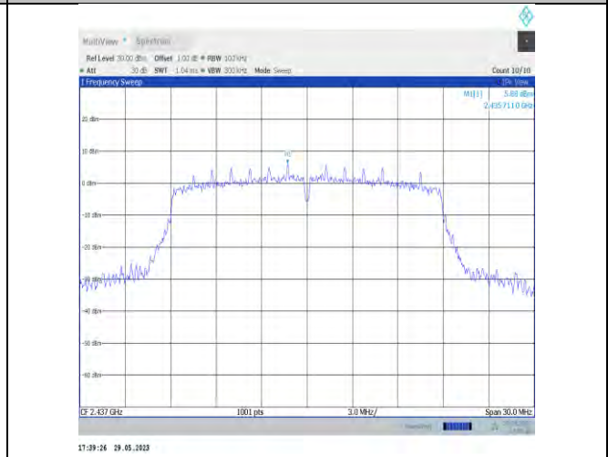
11VHT20SISO-Ant22-2437-0~Reference
