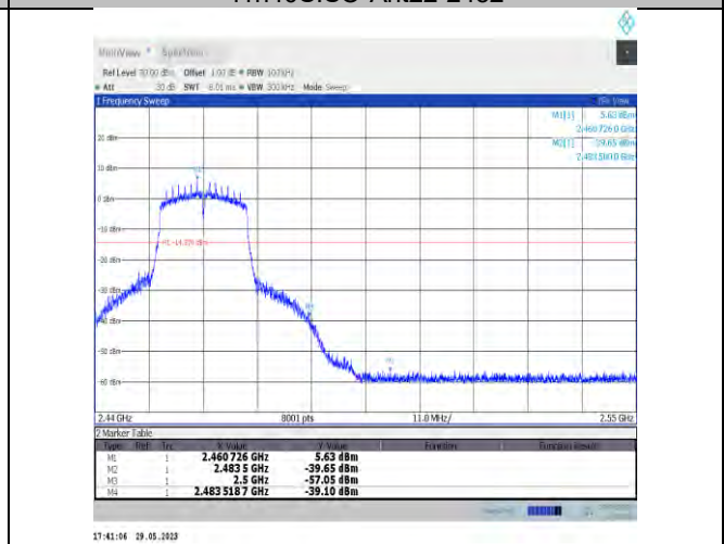
11VHT20SISO-Ant22-2462
