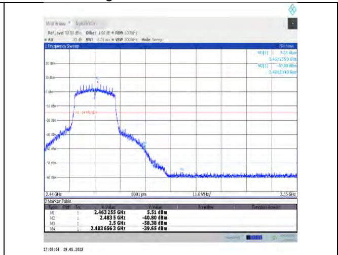
11n20SISO-Ant22-2462
