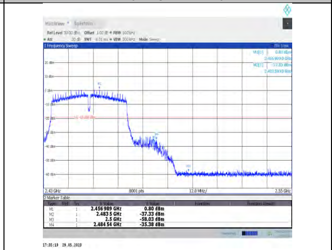
11n40SISO-Ant22-2452
