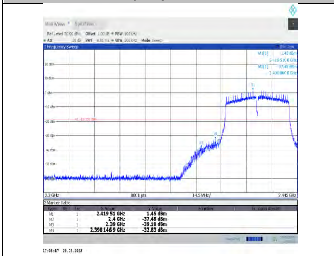
11n40SISO-Ant22-2422
