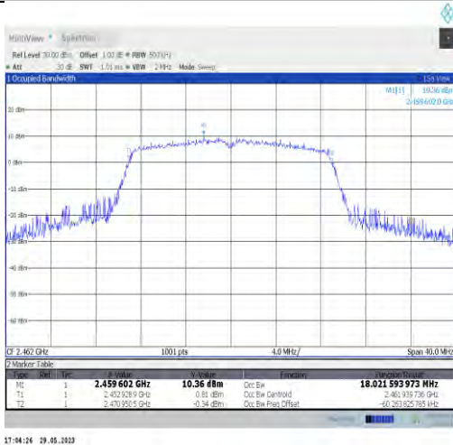
11n20SISO-Ant22-2462
