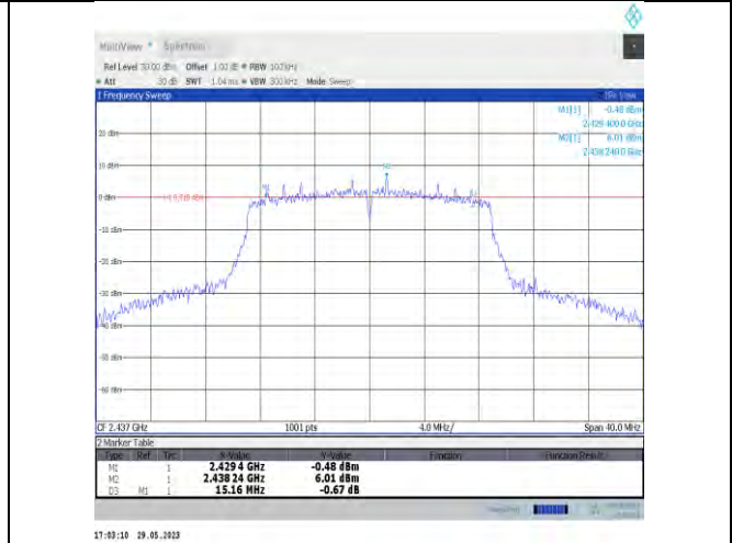
11n20SISO-Ant22-2437
