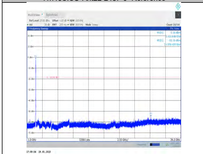
11n40SISO-Ant22-2437-1000~26500
