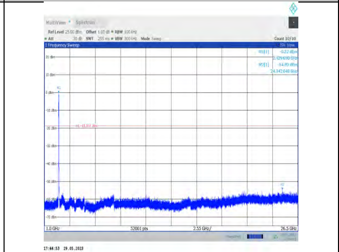
11VHT40SISO-Ant22-2422-1000~26500
