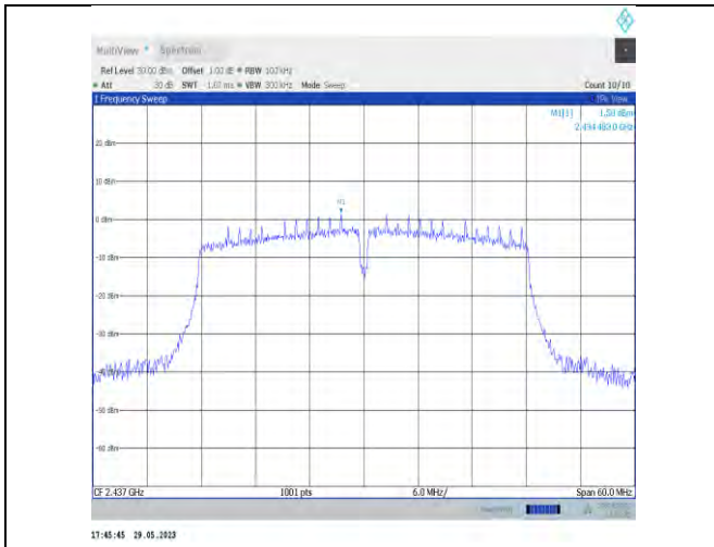
11VHT40SISO-Ant22-2437-0~Reference
