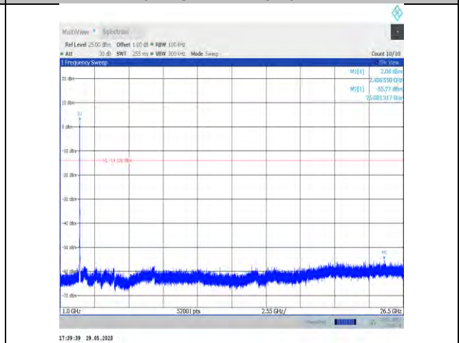
11VHT20SISO-Ant22-2437-1000~26500
