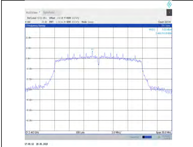
11n20SISO-Ant22-2462-0~Reference
