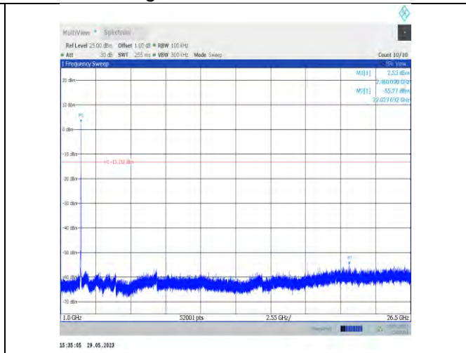
11g-Ant22-2462-1000~26500
