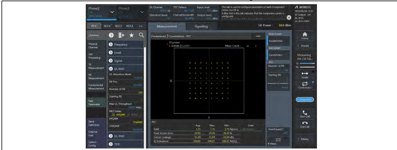
41-41-20MHz-20MHz-64QAM-64QAM-40521-40719-100RB#0-100RB#0
