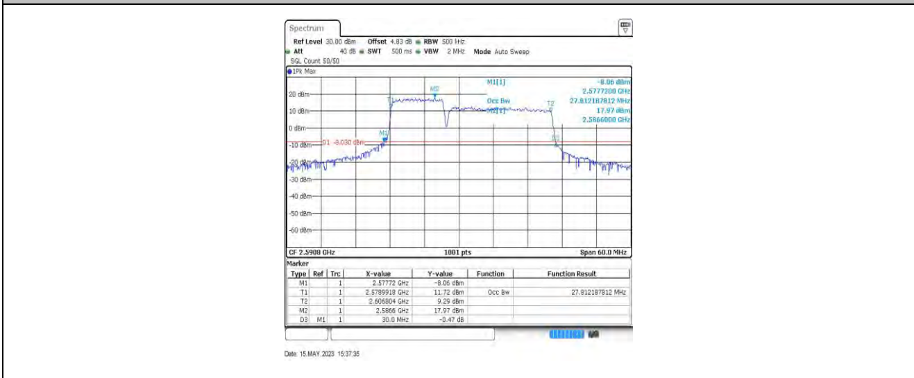
41-41-10MHz-20MHz-QPSK-QPSK-40526-40670-50RB#0-100RB#0-27.812
