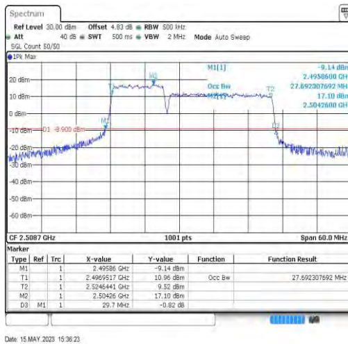
41-41-10MHz-20MHz-16QAM-16QAM-39705-39849-50RB#0-100RB#0-27.692
