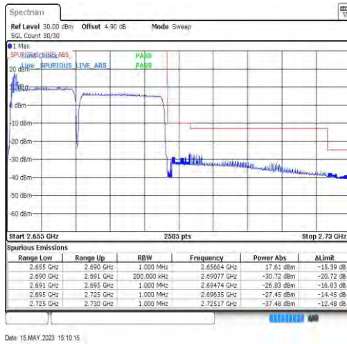
41-41-15MHz-20MHz-QPSK-QPSK-41319-41490-75RB#0-100RB#0
