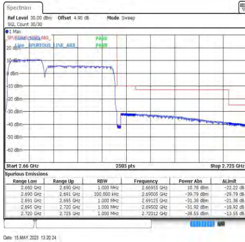
41-41-10MHz-20MHz-QPSK-QPSK-41346-41490-50RB#0-100RB#0
