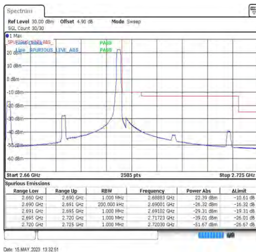
41-41-15MHz-15MHz-QPSK-QPSK-41365-41515-0RB#0-1RB#74
