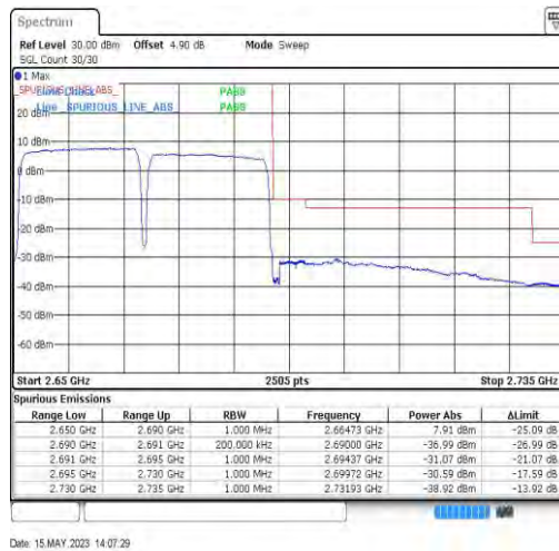
41-41-20MHz-20MHz-QPSK-QPSK-41292-41490-100RB#0-100RB#0
