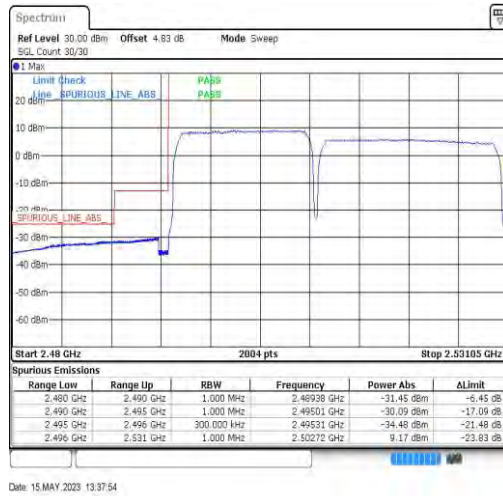
41-41-15MHz-20MHz-QPSK-QPSK-39728-39899-75RB#0-100RB#0
