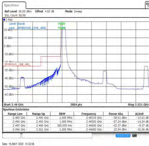
41-41-15MHz-10MHz-QPSK-QPSK-39725-39845-1RB#0-0RB#0
