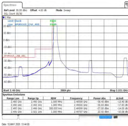
41-41-20MHz-5MHz-QPSK-QPSK-39750-39867-1RB#0-0RB#0
