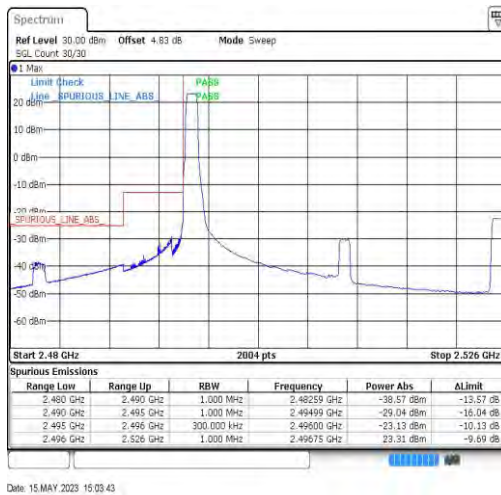
41-41-15MHz-15MHz-QPSK-QPSK-39725-39875-1RB#0-0RB#0
