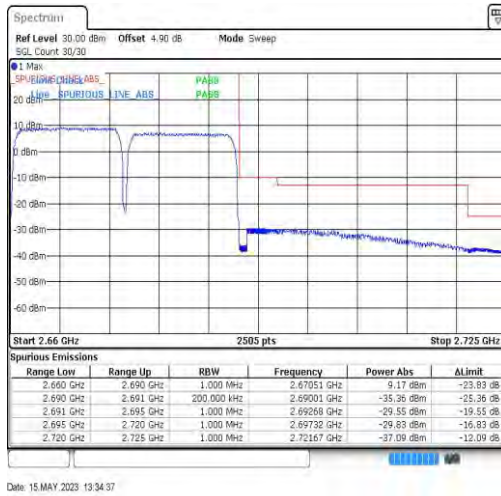
41-41-15MHz-15MHz-QPSK-QPSK-41365-41515-75RB#0-75RB#0
