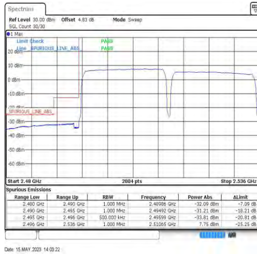
41-41-20MHz-20MHz-QPSK-QPSK-39750-39948-100RB#0-100RB#0
