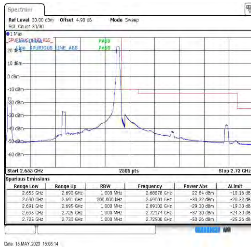
41-41-15MHz-20MHz-QPSK-QPSK-41319-41490-0RB#0-1RB#99
