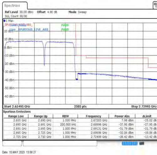
41-41-20MHz-15MHz-QPSK-QPSK-41341-41512-100RB#0-75RB#0
