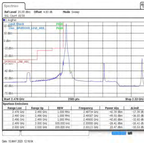
7-7-20MHz-10MHz-QPSK-QPSK-20850-20994-1RB#0-0RB#0
