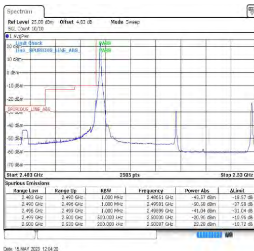
7-7-15MHz-15MHz-QPSK-QPSK-20825-20975-1RB#0-0RB#0
