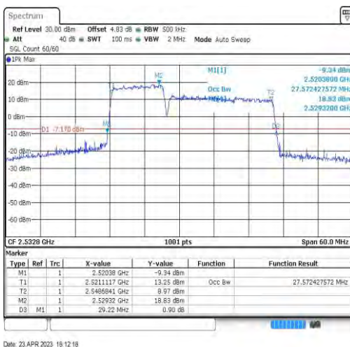
7-7-10MHz-20MHz-16QAM-16QAM-21006-21150-50RB#0-100RB#0-27.572
