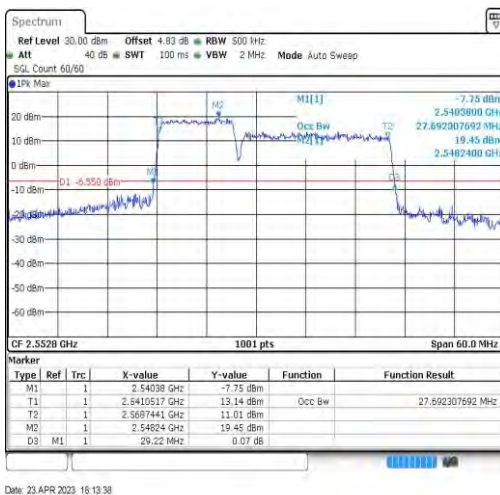
7-7-10MHz-20MHz-16QAM-16QAM-21206-21350-50RB#0-100RB#0-27.692
