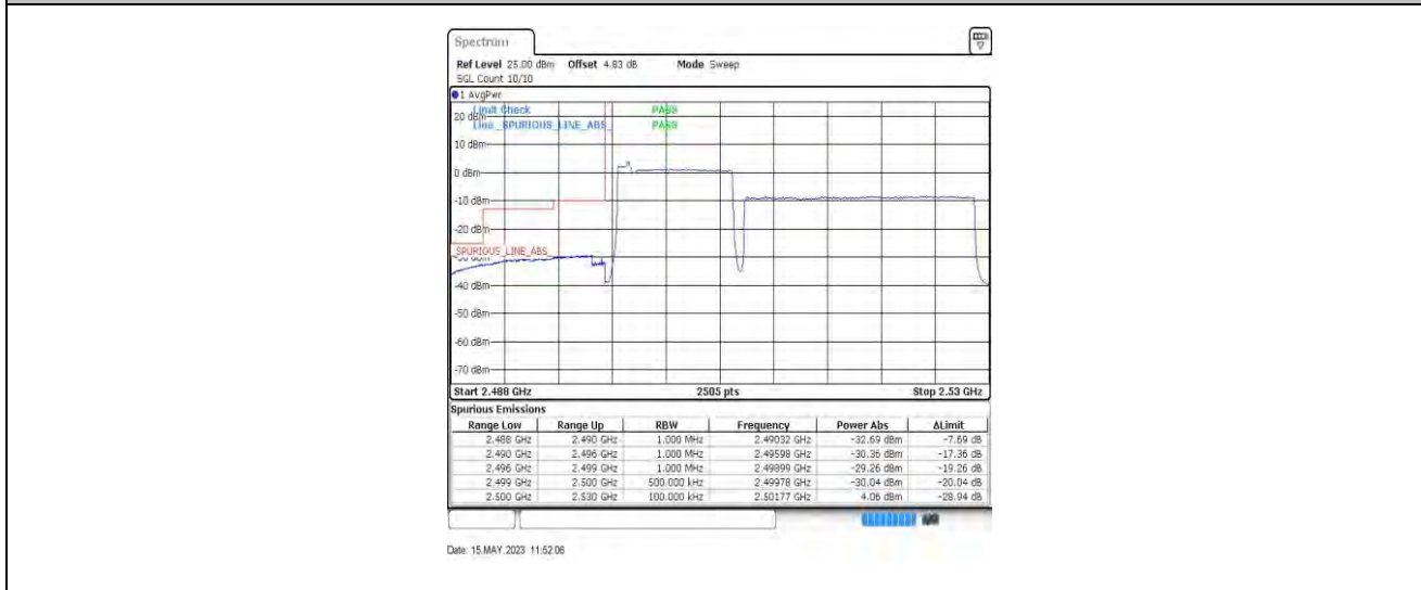
7-7-10MHz-20MHz-QPSK-QPSK-20805-20949-50RB#0-100RB#0
