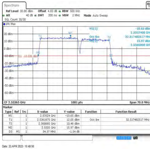
7-7-20MHz-15MHz-16QAM-16QAM-21201-21372-100RB#0-75RB#0-32.517
