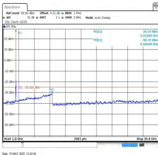
7-7-20MHz-20MHz-QPSK-QPSK-21152-21350-1RB#0-0RB#0-1000~20000MHz
