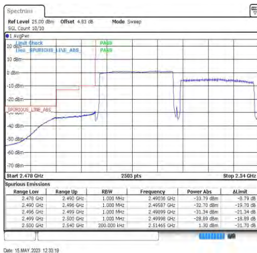
7-7-20MHz-20MHz-QPSK-QPSK-20850-21048-100RB#0-100RB#0
