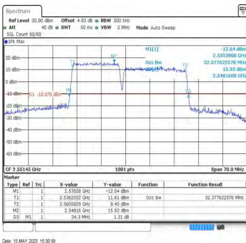
7-7-15MHz-20MHz-64QAM-64QAM-21179-21350-75RB#0-100RB#0-32.378
