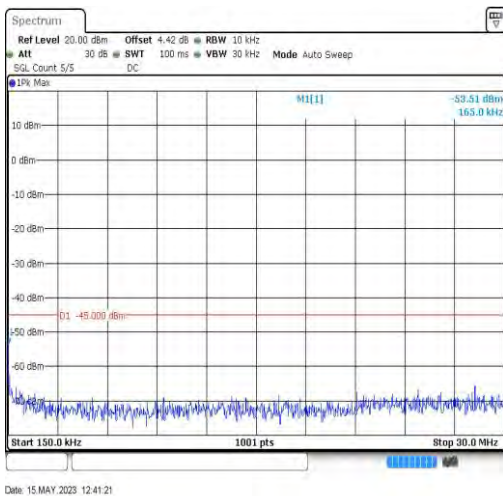
7-7-20MHz-20MHz-QPSK-QPSK-21152-21350-1RB#0-ORB#0-0.15~30MHz
