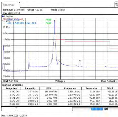
7-7-15MHz-15MHz-QPSK-QPSK-21225-21375-0RB#0-1RB#74
