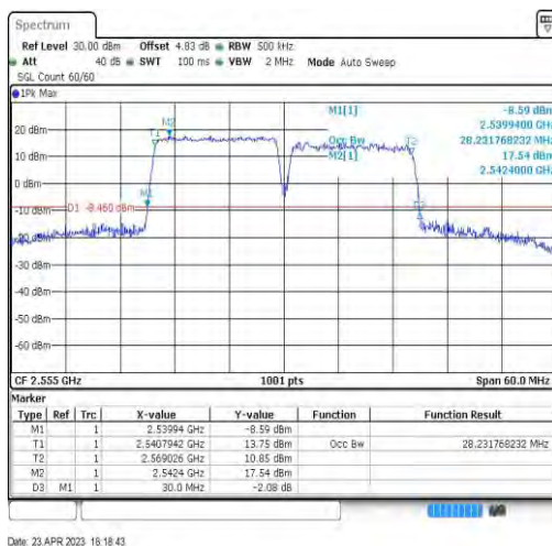
7-7-15MHz-15MHz-QPSK-QPSK-21225-21375-75RB#0-75RB#0-28.232
