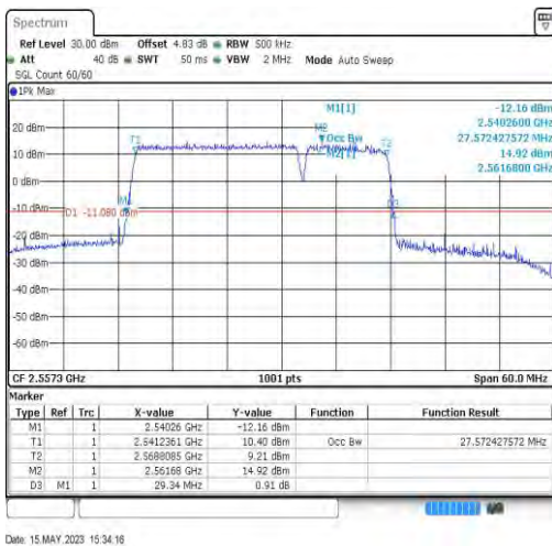
7-7-20MHz-10MHz-64QAM-64QAM-21251-21395-100RB#0-50RB#0-27.572
