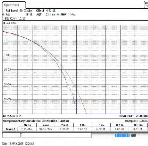
7-7-20MHz-20MHz-QPSK-QPSK-21001-21199-100RB#0-100RB#0
