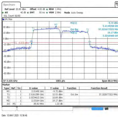
7-7-20MHz-20MHz-64QAM-64QAM-21001-21199-100RB#0-100RB#0-37.323
