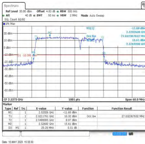
7-7-20MHz-10MHz-64QAM-64QAM-21051-21195-100RB#0-50RB#0-27.632
