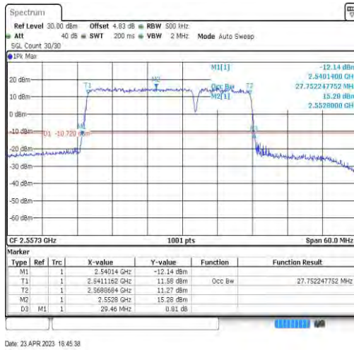
7-7-20MHz-10MHz-QPSK-QPSK-21251-21395-100RB#0-50RB#0-27.752
