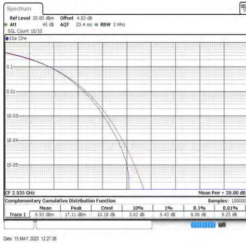
7-7-20MHz-20MHz-16QAM-16QAM-21001-21199-100RB#0-100RB#0
