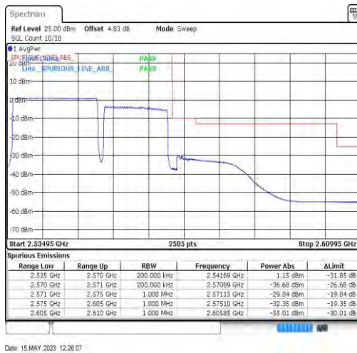
7-7-20MHz-15MHz-QPSK-QPSK-21201-21372-100RB#0-75RB#0
