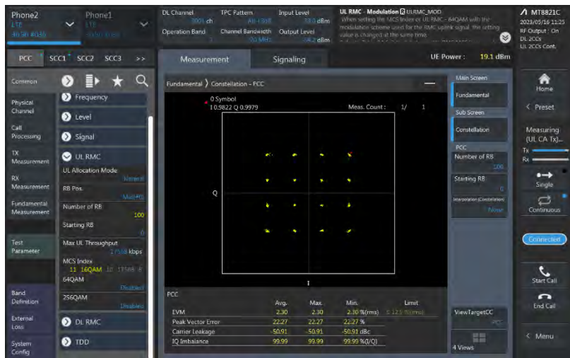
7-7-20MHz-20MHz-16QAM-16QAM -21001-21199-100RB#0-100RB#0
