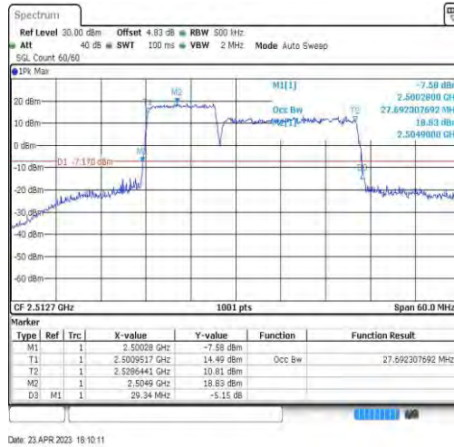
7-7-10MHz-20MHz-QPSK-QPSK-20805-20949-50RB#0-100RB#0-27.692
