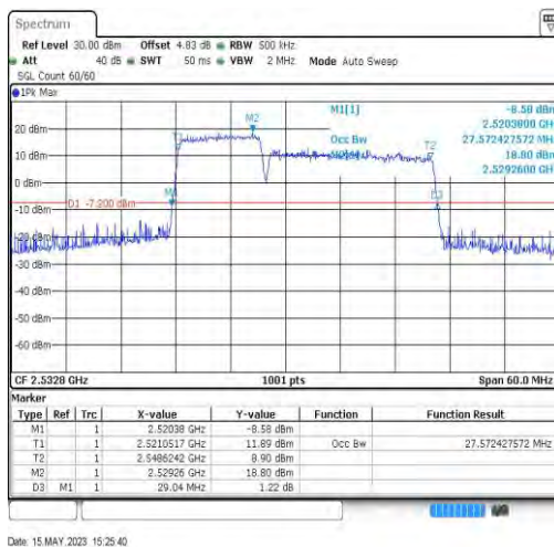
7-7-10MHz-20MHz-64QAM-64QAM-21006-21150-50RB#0-100RB#0-27.572
