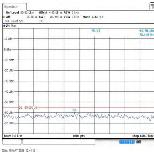
7-7-20MHz-20MHz-QPSK-QPSK-21152-21350-1RB#0-0RB#0-0.009~0.15MHz
