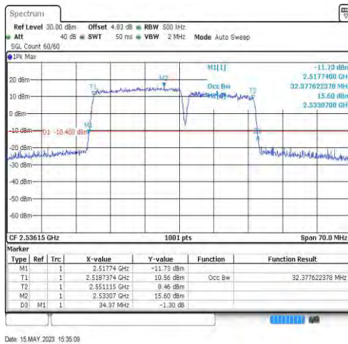
7-7-20MHz-15MHz-64QAM-64QAM-21026-21197-100RB#0-75RB#0-32.378
