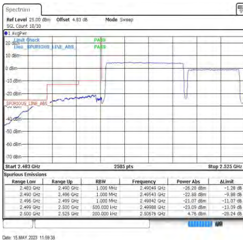
7-7-15MHz-10MHz-QPSK-QPSK-20825-20945-75RB#0-50RB#0
