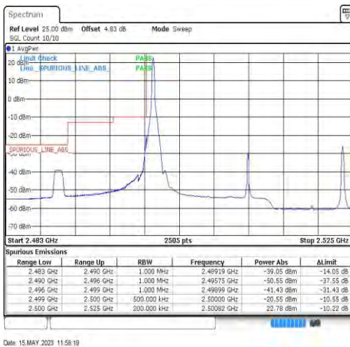
7-7-15MHz-10MHz-QPSK-QPSK-20825-20945-1RB#0-0RB#0
