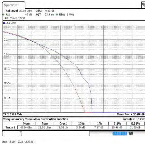
7-7-20MHz-20MHz-QPSK-QPSK-21152-21350-100RB#0-100RB#0
