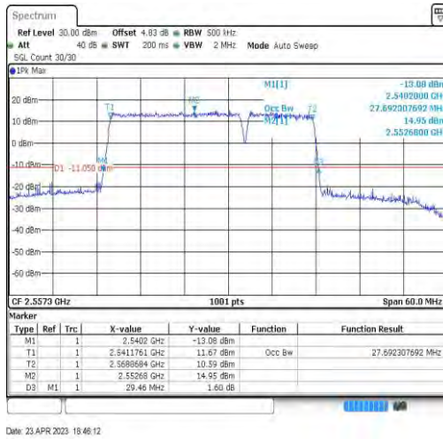
7-7-20MHz-10MHz-16QAM-16QAM-21251-21395-100RB#0-50RB#0-27.692
