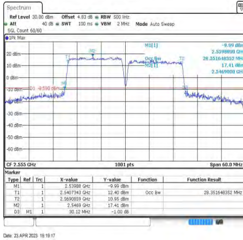
7-7-15MHz-15MHz-16QAM-16QAM-21225-21375-75RB#0-75RB#0-28.352
