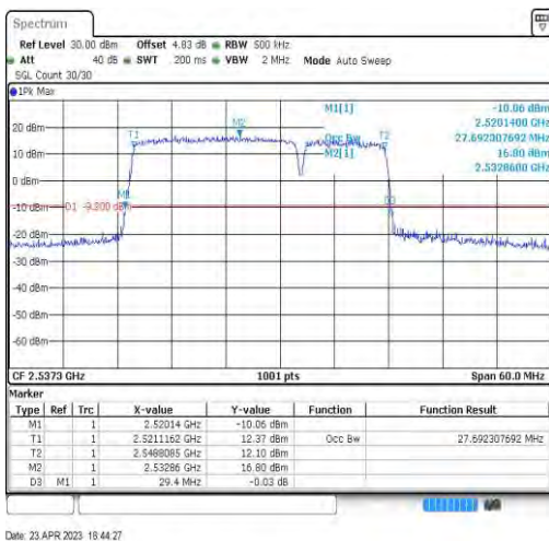
7-7-20MHz-10MHz-QPSK-QPSK-21051-21195-100RB#0-50RB#0-27.692
