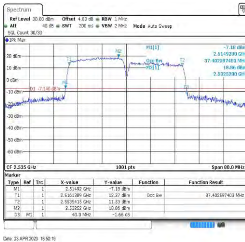
7-7-20MHz-20MHz-16QAM-16QAM-21001-21199-100RB#0-100RB#0-37.403
