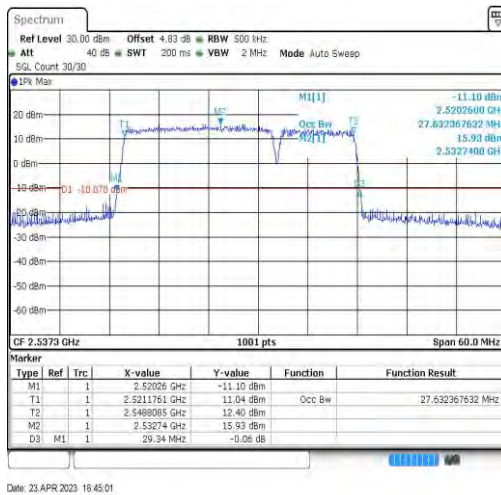
7-7-20MHz-10MHz-16QAM-16QAM-21051-21195-100RB#0-50RB#0-27.632
