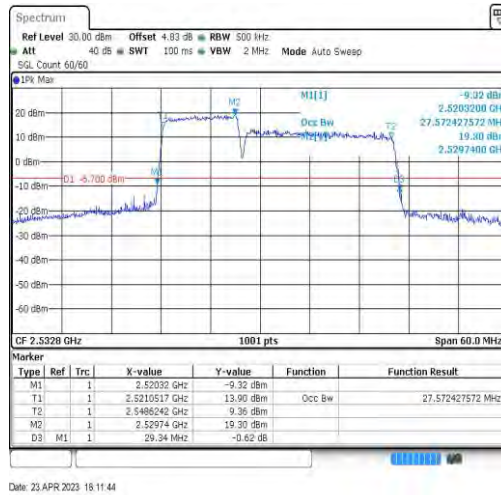
7-7-10MHz-20MHz-QPSK-QPSK-21006-21150-50RB#0-100RB#0-27.572
