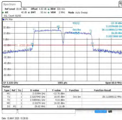
7-7-15MHz-15MHz-64QAM-64QAM-21025-21175-75RB#0-75RB#0-28.112
