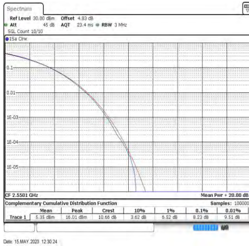
7-7-20MHz-20MHz-16QAM-16QAM-21152-21350-100RB#0-100RB#0
