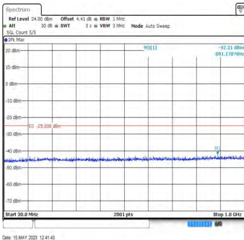
7-7-20MHz-20MHz-QPSK-QPSK-21152-21350-1RB#0-ORB#0-30~1000MHz
