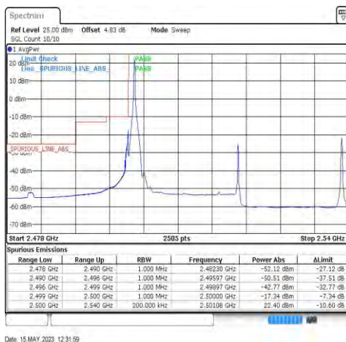
7-7-20MHz-20MHz-QPSK-QPSK-20850-21048-1RB#0-0RB#0
