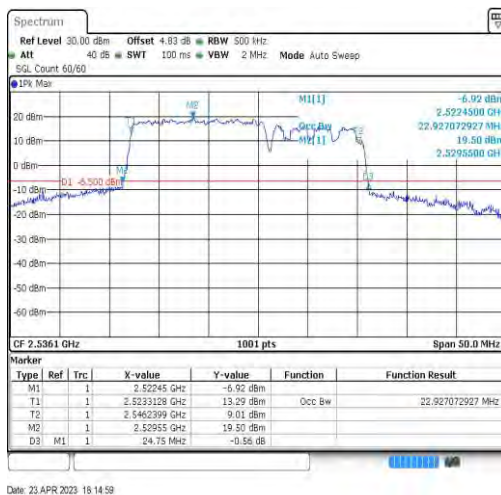
7-7-15MHz-10MHz-16QAM-16QAM-21051-21171-75RB#0-50RB#0-22.927
