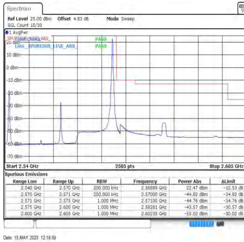
7-7-20MHz-10MHz-QPSK-QPSK-21251-21395-0RB#0-1RB#49
