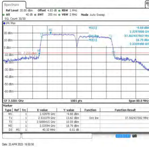
7-7-20MHz-20MHz-QPSK-QPSK-21152-21350-100RB#0-100RB#0-37.562
