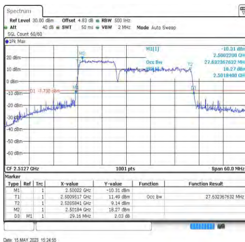
7-7-10MHz-20MHz-64QAM-64QAM-20805-20949-50RB#0-100RB#0-27.632
