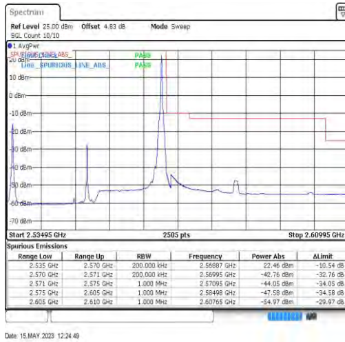
7-7-20MHz-15MHz-QPSK-QPSK-21201-21372-0RB#0-1RB#74
