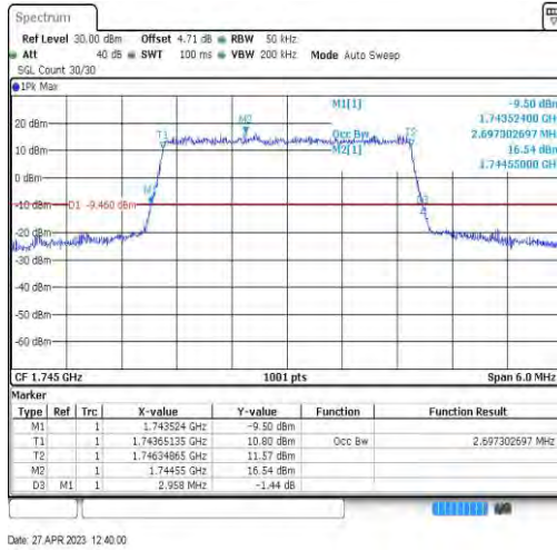
Band66-3MHz-QPSK-132322-15RB#0-2.697
