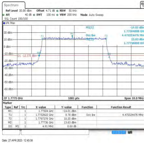
Band66-5MHz-QPSK-132647-25RB#0-4.476
