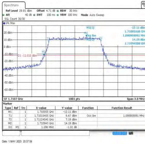
Band66-1.4MHz-64QAM-131979-6RB#0-1.091
