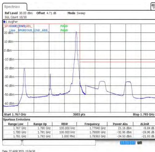
Band66-10MHz-QPSK-132622-1RB#49
