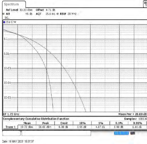
Band66-20MHz-16QAM-132072-100RB#0
