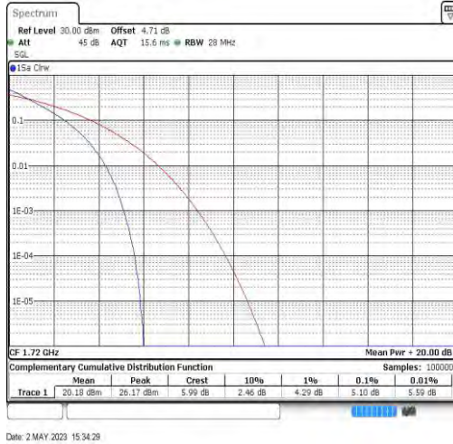
Band66-20MHz-QPSK-132072-100RB#0
