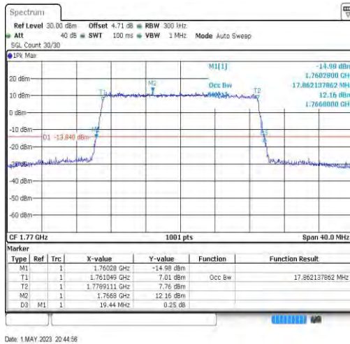
Band66-20MHz-64QAM-132572-100RB#0-17.862
