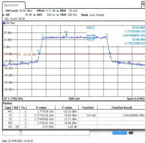
Band66-3MHz-QPSK-132657-15RB#0-2.691
