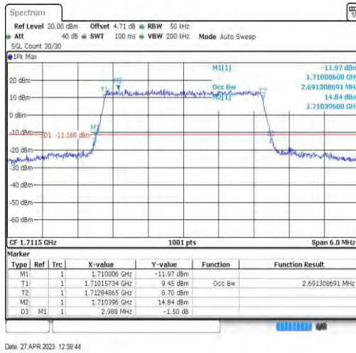
Band66-3MHz-16QAM-131987-15RB#0-2.691
