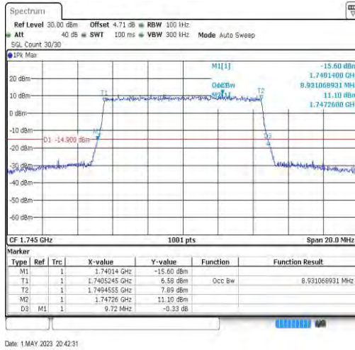
Band66-10MHz-64QAM-132322-50RB#0-8.931
