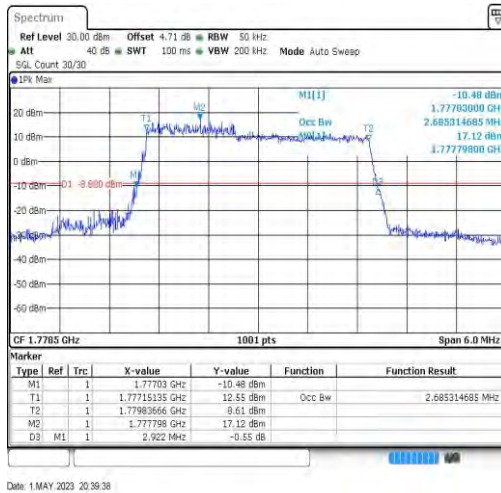
Band66-3MHz-64QAM-132657-15RB#0-2.685
