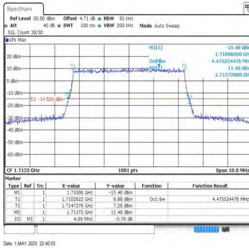
Band66-5MHz-64QAM-131997-25RB#0-4.476
