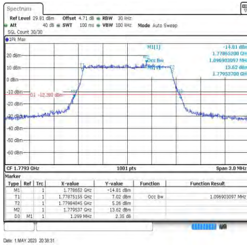
Band66-1.4MHz-64QAM-132665-6RB#0-1.097
