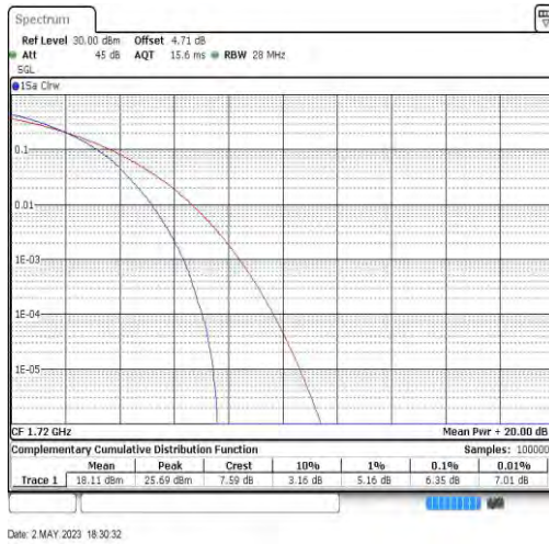
Band66-20MHz-64QAM-132072-100RB#0
