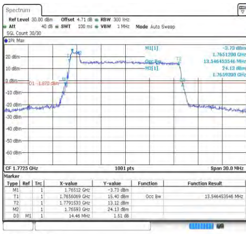
Band66-15MHz-QPSK-132597-75RB#0-13.546
