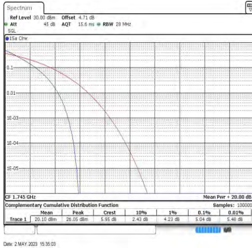
Band66-20MHz-QPSK-132322-100RB#0
