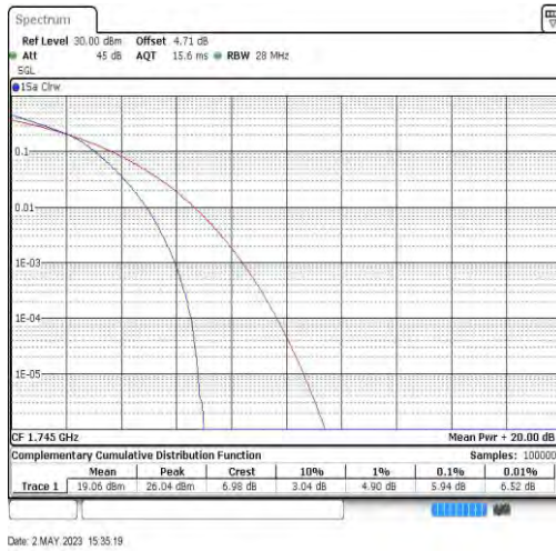
Band66-20MHz-16QAM-132322-100RB#0
