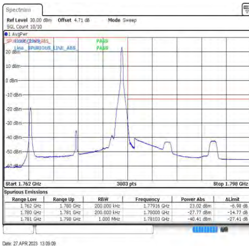
Band66-15MHz-QPSK-132597-1RB#74
