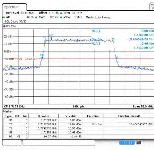
Band66-15MHz-QPSK-132047-75RB#0-13.457
