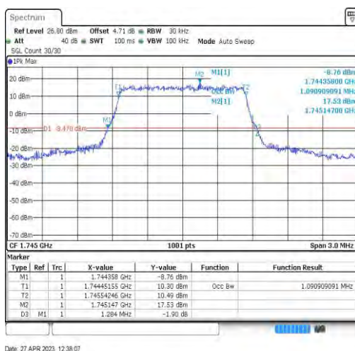
Band66-1.4MHz-QPSK-132322-6RB#0-1.091
