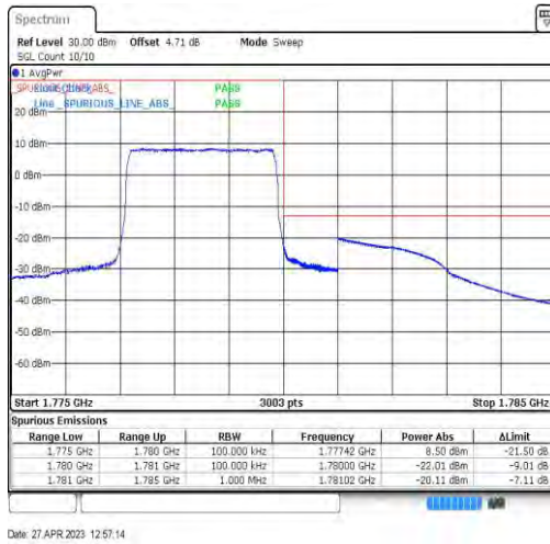
Band66-3MHz-QPSK-132657-15RB#0
