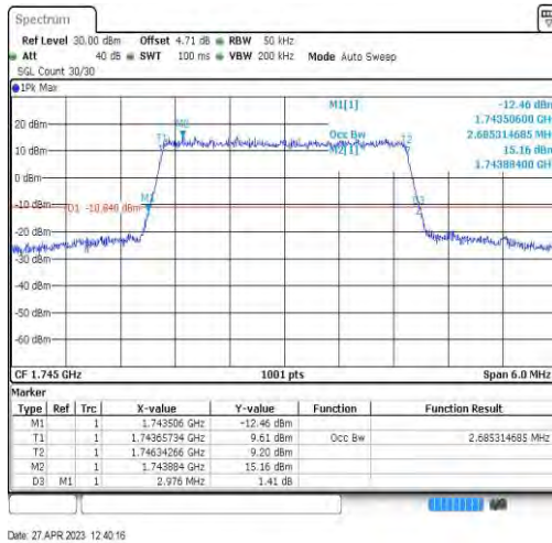
Band66-3MHz-16QAM-132322-15RB#0-2.685
