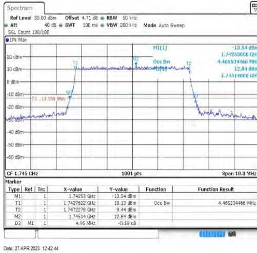
Band66-5MHz-16QAM-132322-25RB#0-4.466
