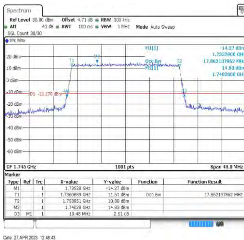
Band66-20MHz-16QAM-132322-100RB#0-17.862
