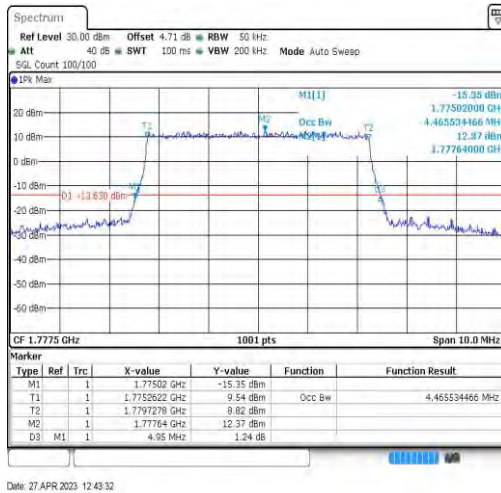
Band66-5MHz-16QAM-132647-25RB#0-4.466
