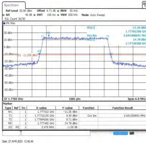
Band66-3MHz-16QAM-132657-15RB#0-2.691
