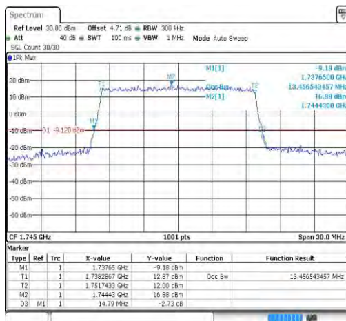
Band66-15MHz-QPSK-132047-75RB#0-13.457
