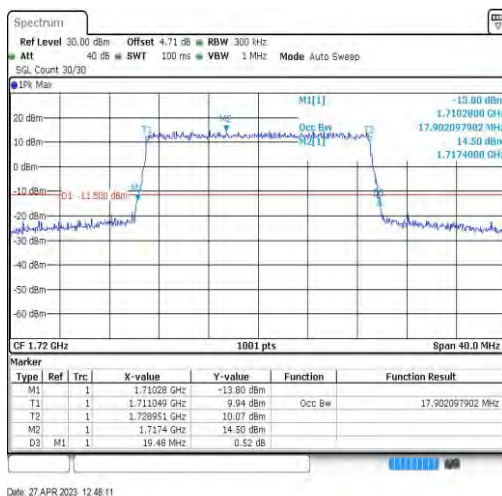
Band66-20MHz-16QAM-132072-100RB#0-17.902
