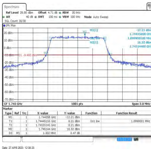
Band66-1.4MHz-16QAM-132322-6RB#0-1.1
