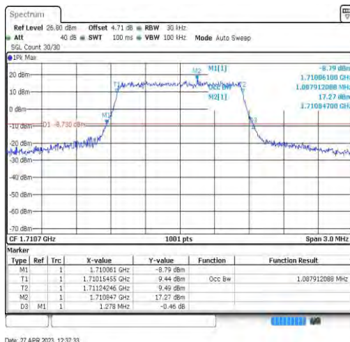
Band66-1.4MHz-QPSK-131979-6RB#0-1.088
