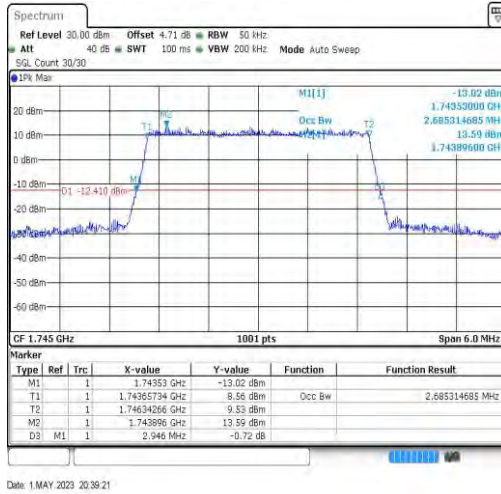
Band66-3MHz-64QAM-132322-15RB#0-2.685
