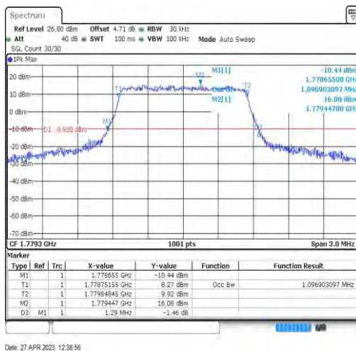
Band66-1.4MHz-16QAM-132665-6RB#0-1.097
