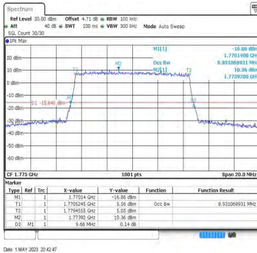
Band66-10MHz-64QAM-132622-50RB#0-8.931
