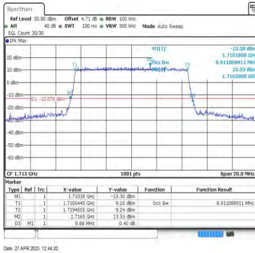
Band66-10MHz-16QAM-132022-50RB#0-8.911
