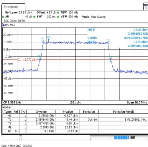
Band41-10MHz-64QAM-40620-50RB#0-8.911
