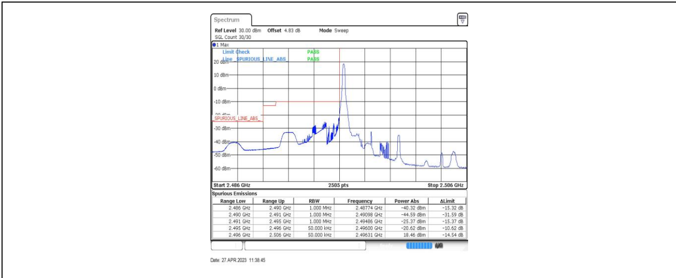
Band41-5MHz-QPSK-39675-1RB#0
