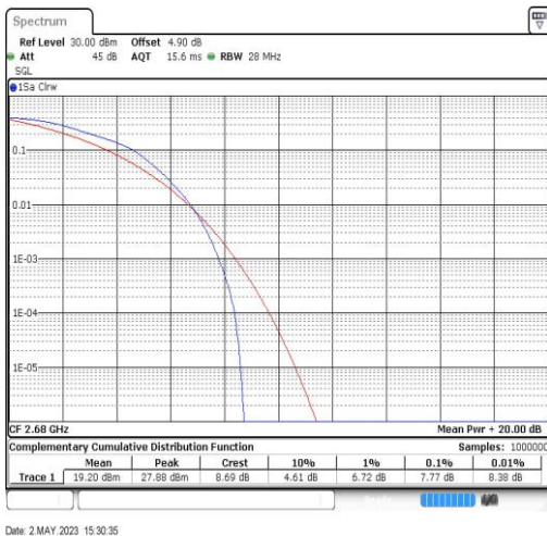
Band41-20MHz-16QAM-41490-100RB#0
