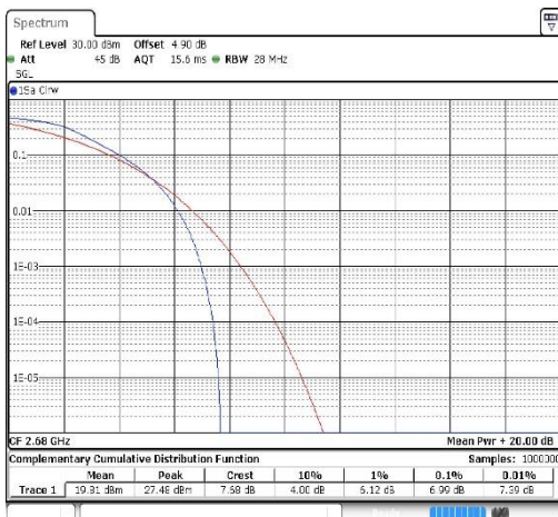
Band41-20MHz-QPSK-41490-100RB#0
