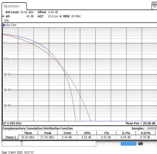
Band41-20MHz-64QAM-40620-100RB#0
