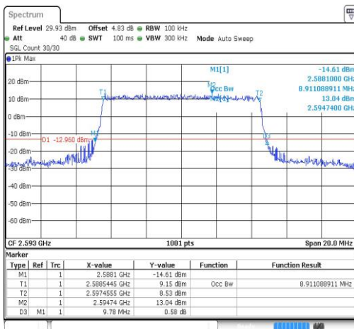
Band41-10MHz-QPSK-40620-50RB#0-8.911
