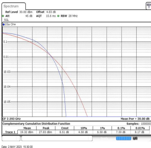
Band41-20MHz-16QAM-40620-100RB#0
