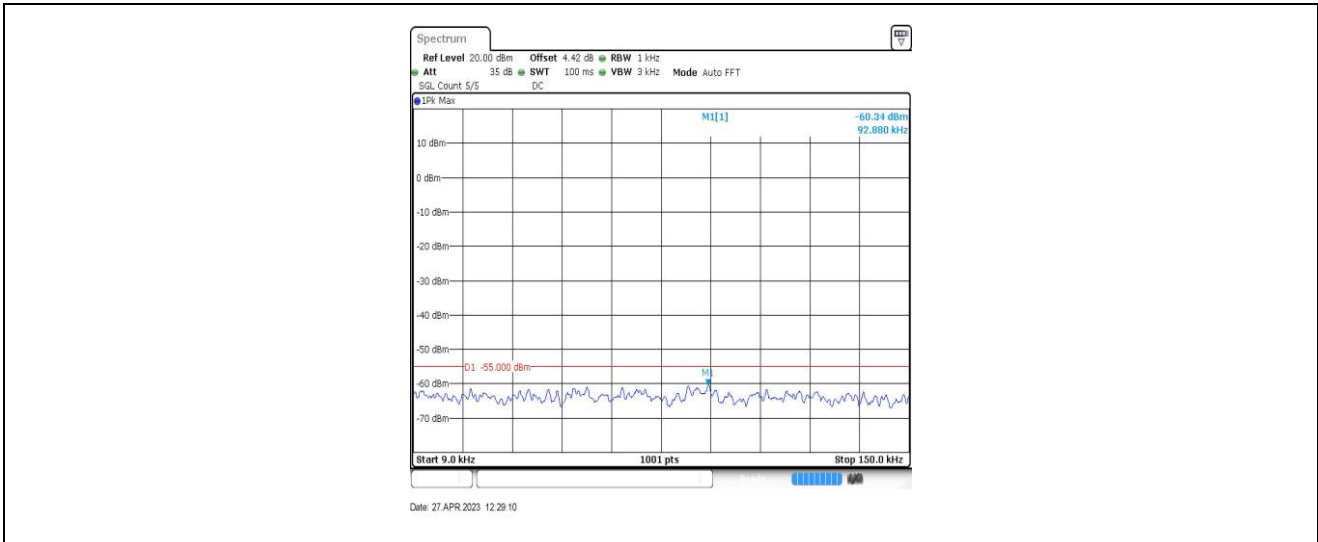
Band41-20MHz-QPSK-39750-1RB#0-Range1:0.009~0.15MHz
