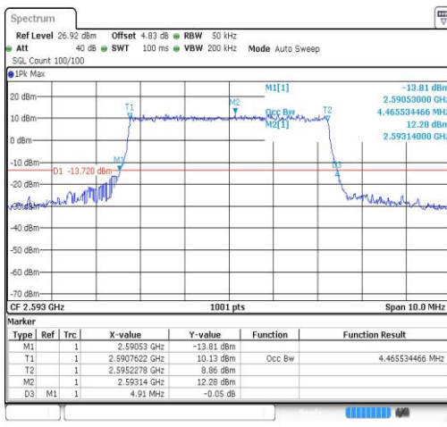
Band41-5MHz-16QAM-40620-25RB#0-4.466
