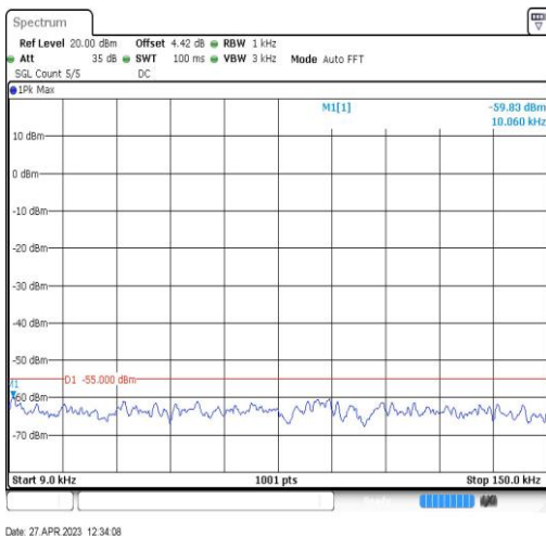
Band41-20MHz-QPSK-41490-1RB#0-Range1:0.009~0.15MHz
