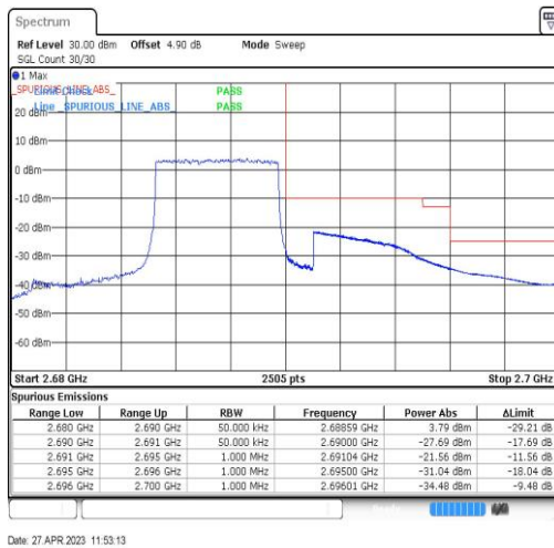
Band41-5MHz-QPSK-41565-25RB#0
