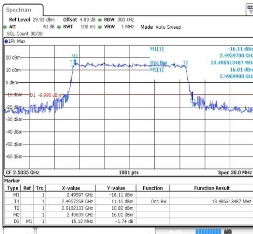
Band41-15MHz-QPSK-41515-75RB#0-13.487
