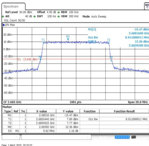
Band41-10MHz-64QAM-41540-50RB#0-8.911
