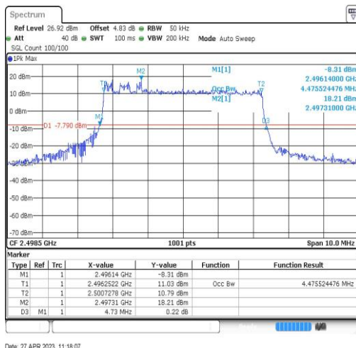
Band41-5MHz-QPSK-39675-25RB#0-4.476
