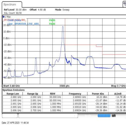
Band41-5MHz-QPSK-41565-1RB#24
