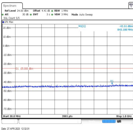
Band41-20MHz-QPSK-40620-1RB#0-Range3:30~1000MHz
