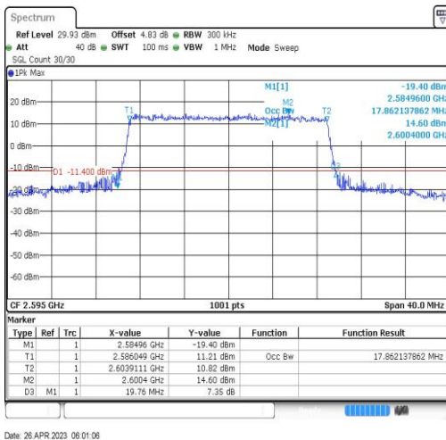
Band38-20MHz-16QAM-38000-100RB#0-17.862
