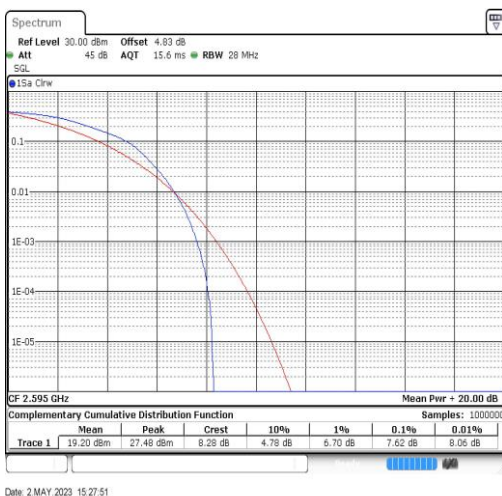
Band38-20MHz-16QAM-38000-100RB#0
