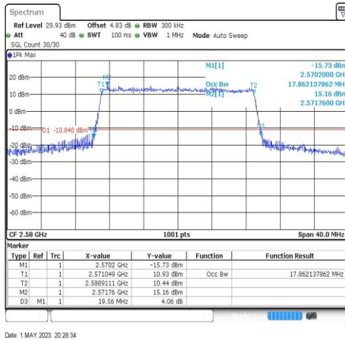
Band38-20MHz-64QAM-37850-100RB#0-17.862
