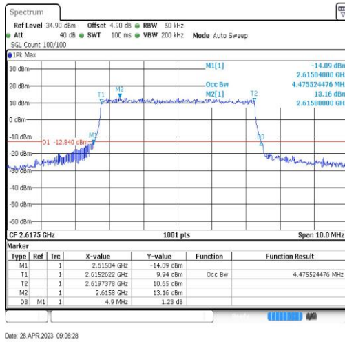
Band38-5MHz-QPSK-38225-25RB#0-4.476
