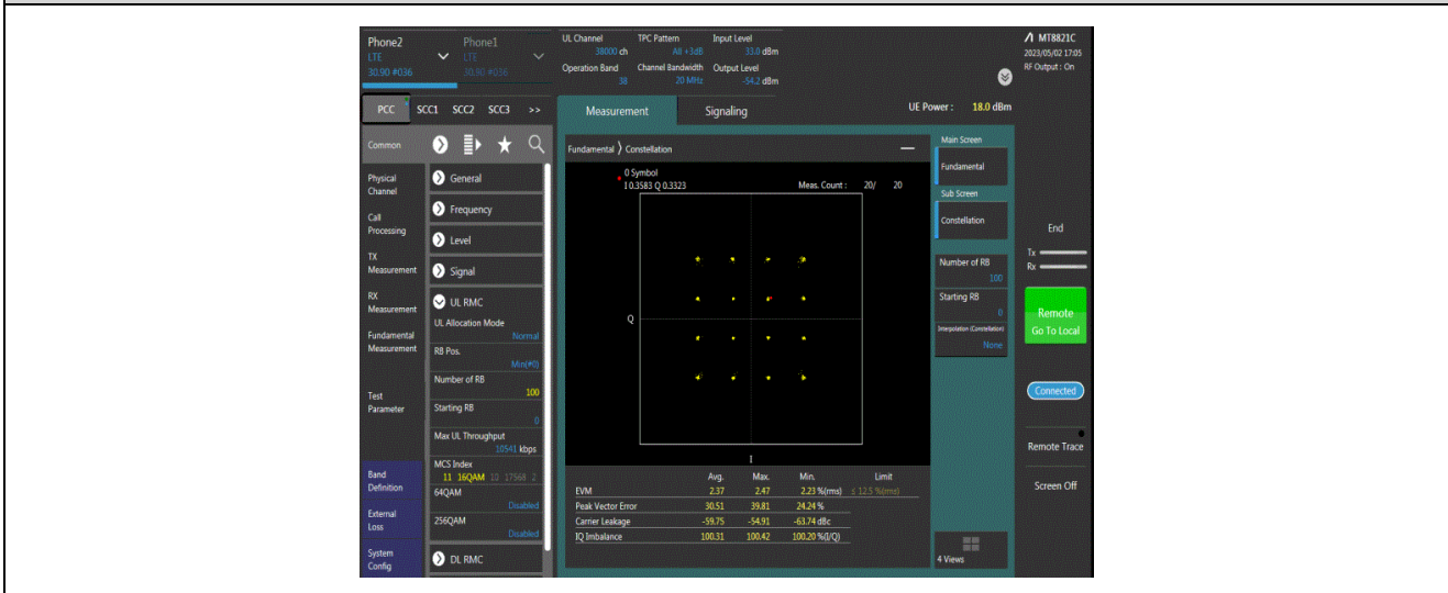
Band38-20MHz-16QAM-38000-100RB#0
