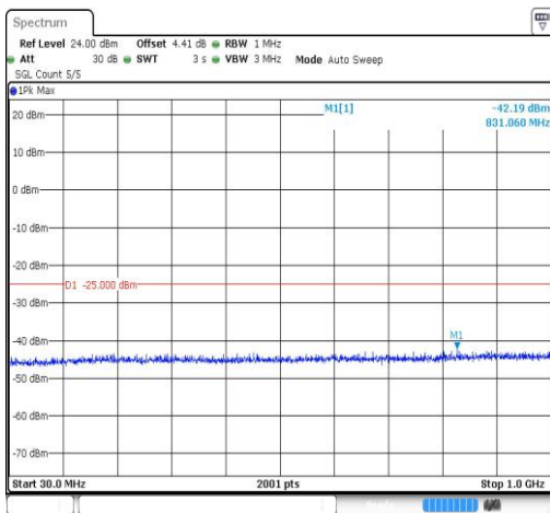
Band38-20MHz-QPSK-38150-1RB#0-Range3:30~1000MHz
