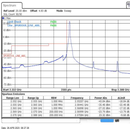
Band38-15MHz-QPSK-37825-1RB#0
