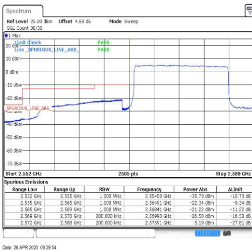
Band38-15MHz-QPSK-37825-75RB#0
