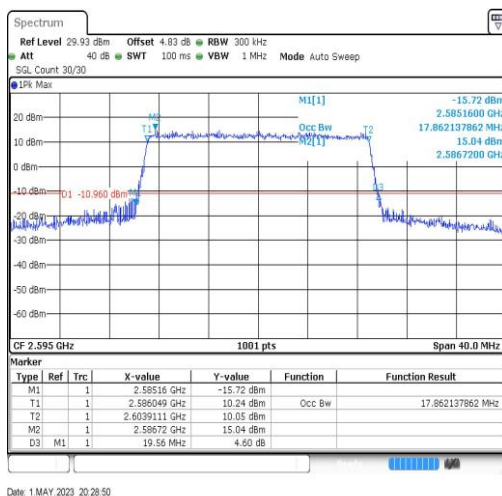
Band38-20MHz-64QAM-38000-100RB#0-17.862
