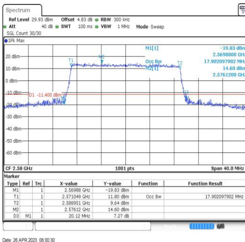
Band38-20MHz-16QAM-37850-100RB#0-17.902
