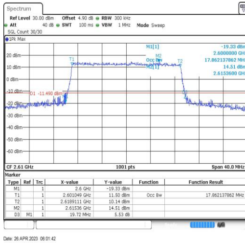
Band38-20MHz-16QAM-38150-100RB#0-17.862
