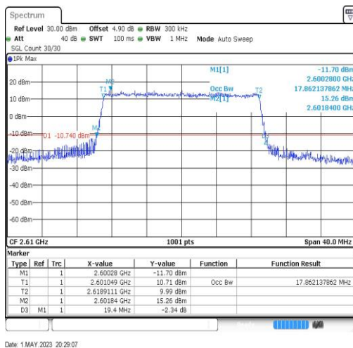
Band38-20MHz-64QAM-38150-100RB#0-17.862
