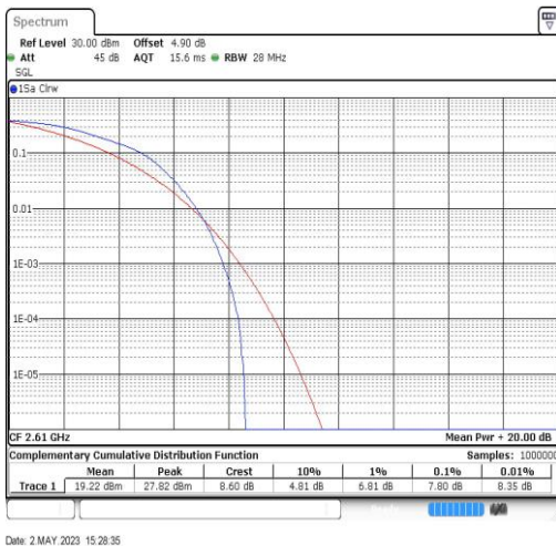
Band38-20MHz-16QAM-38150-100RB#0
