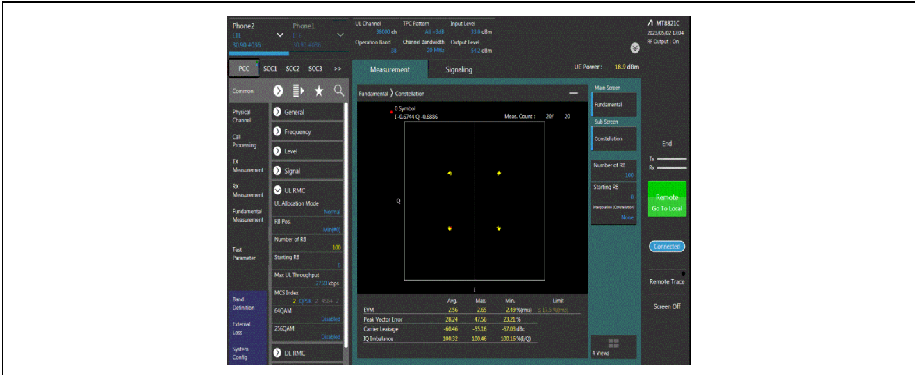
Band38-20MHz-QPSK-38000-100RB#0
