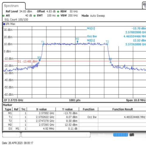
Band38-5MHz-16QAM-37775-25RB#0-4.466
