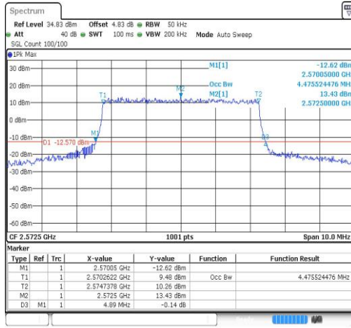
Band38-5MHz-QPSK-37775-25RB#0-4.476
