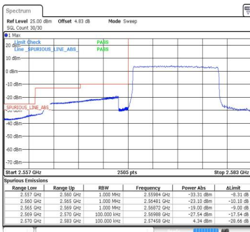
Band38-10MHz-QPSK-37800-1RB#0
