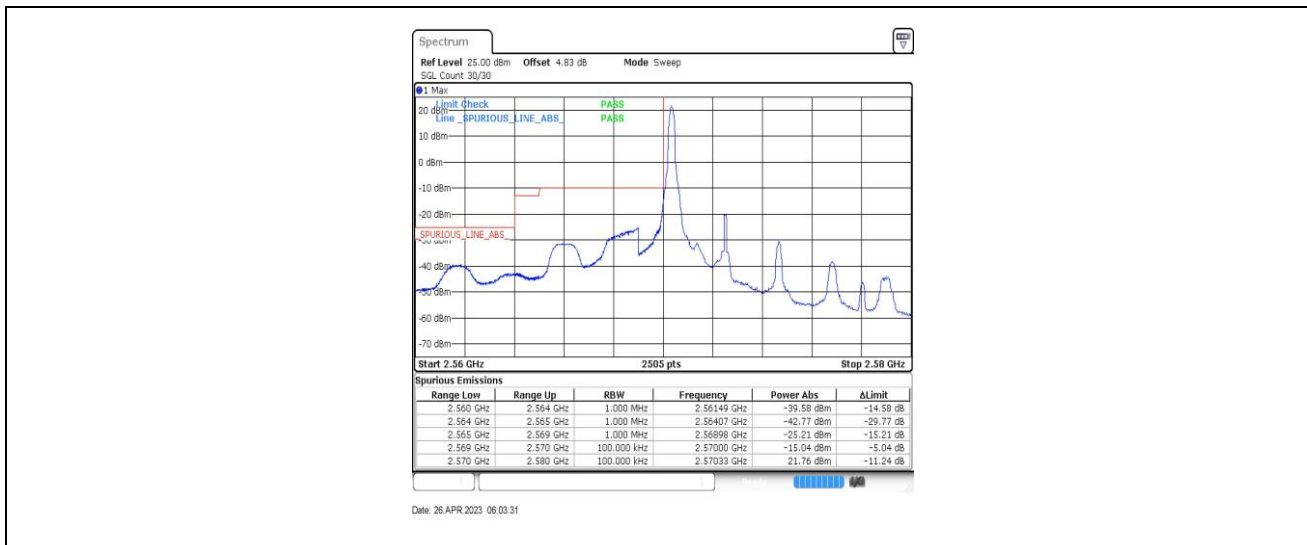
Band38-5MHz-QPSK-37775-1RB#0
