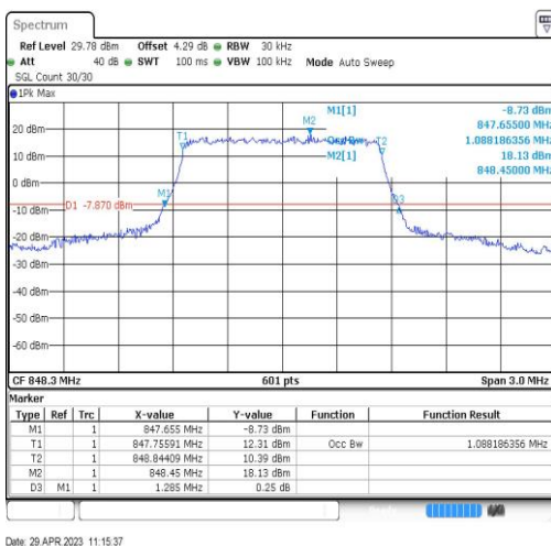
Band26-1.4MHz-QPSK-27033-6RB#0-1.088
