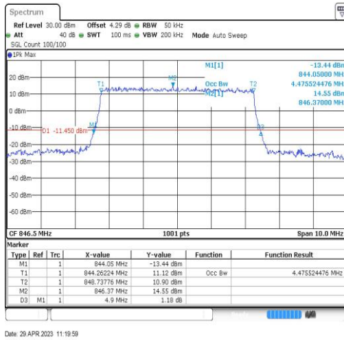
Band26-5MHz-QPSK-27015-25RB#0-4.476
