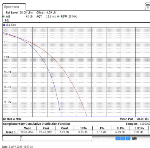
Band26-15MHz-64QAM-26865-75RB#0
