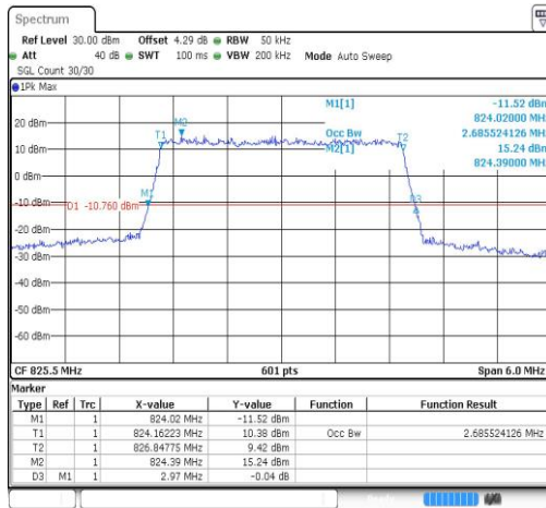
Band26-3MHz-16QAM-27025-15RB#0-2.686
