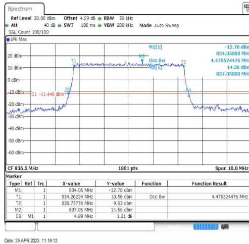
Band26-5MHz-QPSK-26915-25RB#0-4.476
