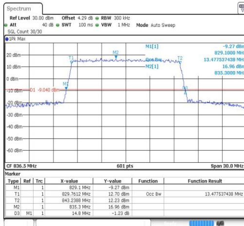
Band26-15MHz-16QAM-26915-75RB#0-13.478
