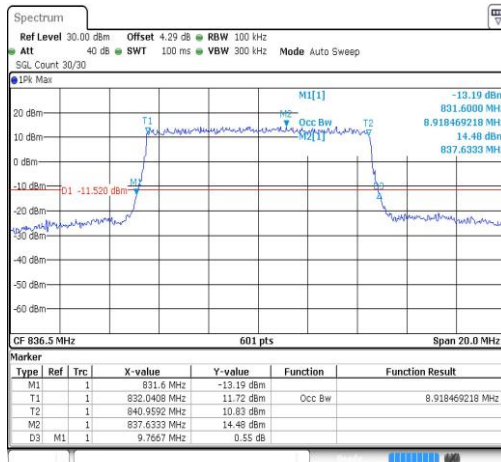
Band26-10MHz-QPSK-26915-50RB#0-8.918
