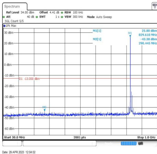
Band26-15MHz-QPSK-26915-1RB#0-Range3:30~1000MHz
