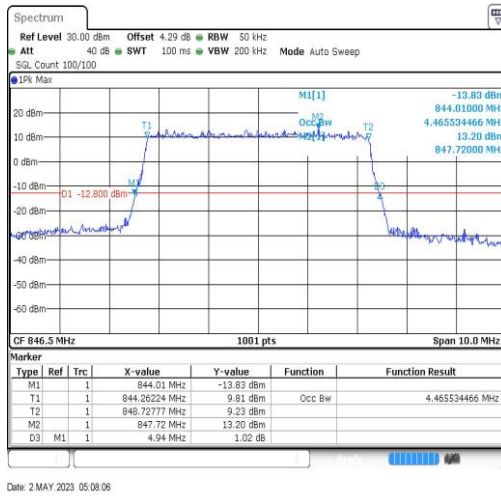
Band26-5MHz-64QAM-27015-25RB#0-4.466
