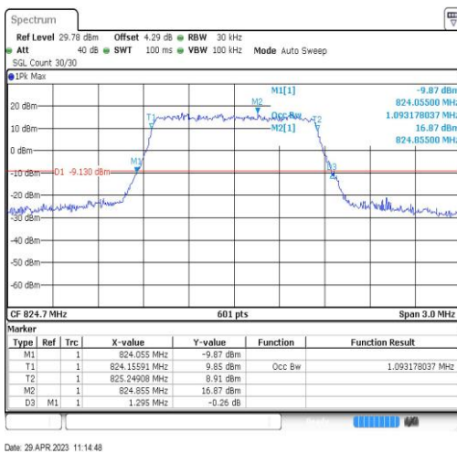
Band26-1.4MHz-16QAM-26797-6RB#0-1.093
