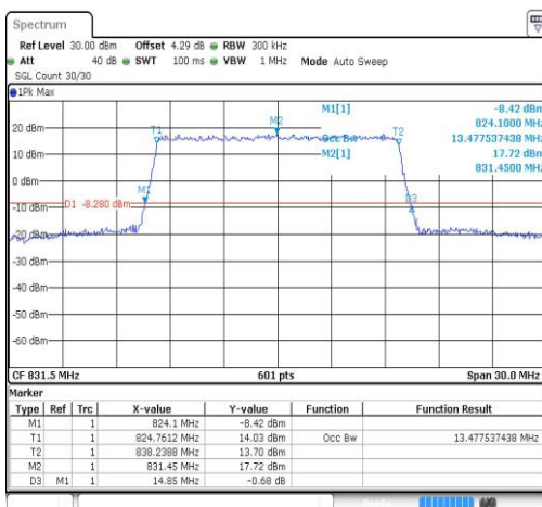
Band26-15MHz-QPSK-26865-75RB#0-13.478
