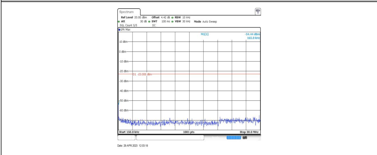
Band26-15MHz-QPSK-26865-1RB#0-Range2:0.15~30MHz
