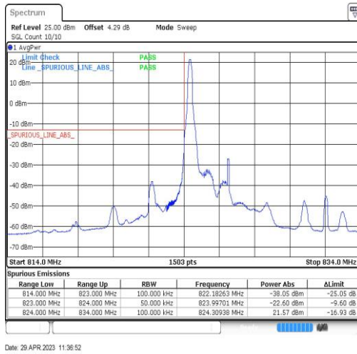
Band26-5MHz-QPSK-26815-1RB#0
