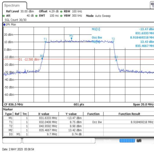
Band26-10MHz-64QAM-26915-50RB#0-8.918
