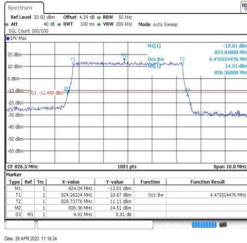
Band26-5MHz-QPSK-26815-25RB#0-4.476
