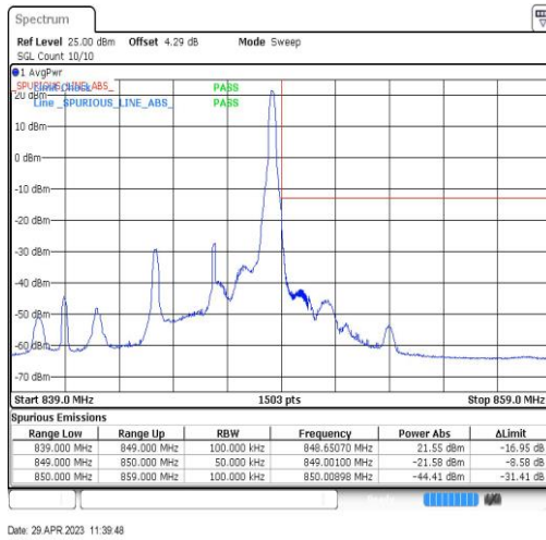
Band26-5MHz-QPSK-27015-1RB#24
