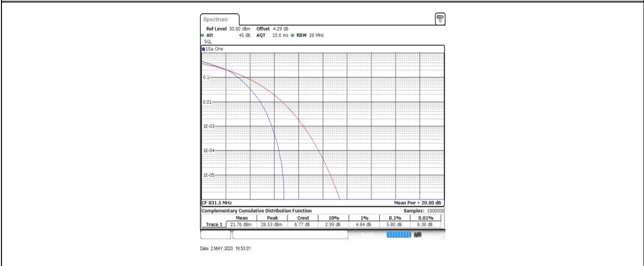
Band26-15MHz-16QAM-26865-75RB#0
