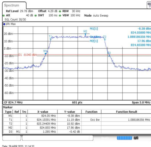
Band26-1.4MHz-QPSK-26797-6RB#0-1.088
