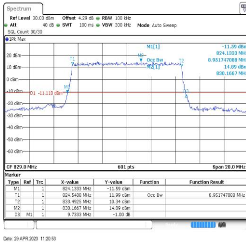
Band26-10MHz-QPSK-26840-50RB#0-8.952
