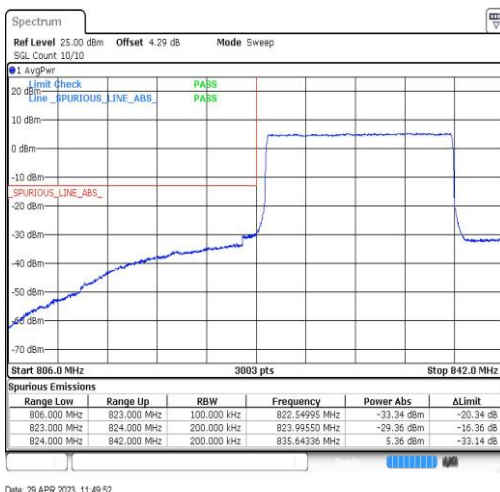
Band26-15MHz-QPSK-26865-75RB#0
