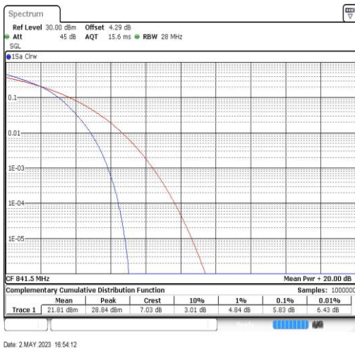
Band26-15MHz-16QAM-26965-75RB#0
