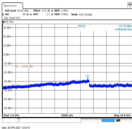
Band26-15MHz-QPSK-26915-1RB#0-Range4:1000~10000MHz
