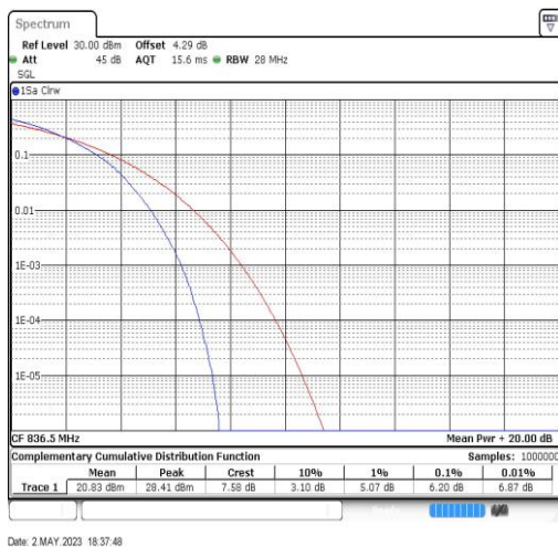
Band26-15MHz-64QAM-26915-75RB#0
