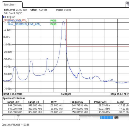
Band26-3MHz-QPSK-27025-1RB#14
