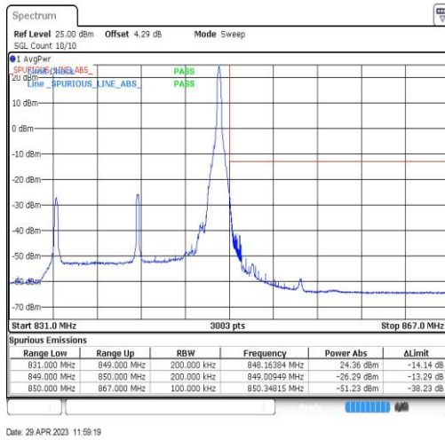
Band26-15MHz-QPSK-26965-1RB#74
