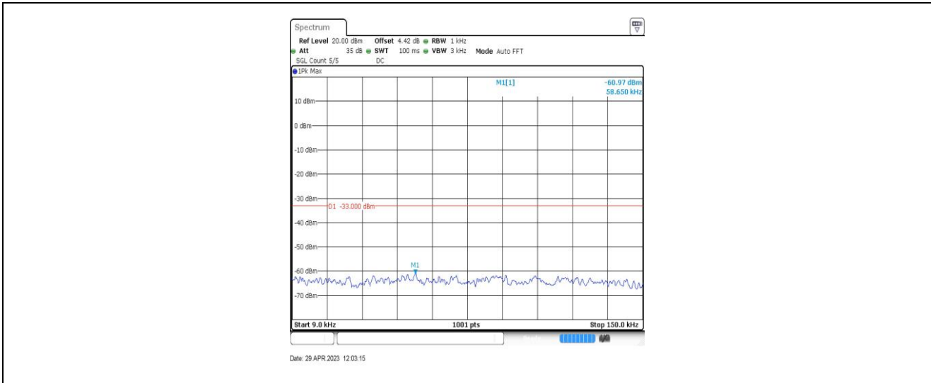
Band26-15MHz-QPSK-26865-1RB#0-Range1:0.009~0.15MHz
