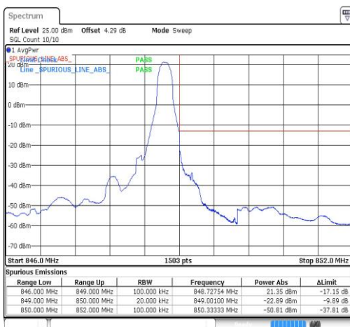
Band26-1.4MHz-QPSK-27033-1RB#5
