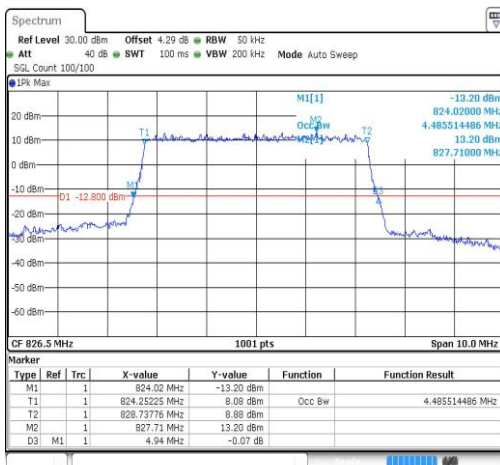
Band26-5MHz-64QAM-26815-25RB#0-4.486
