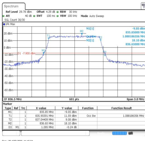
Band26-1.4MHz-QPSK-26915-6RB#0-1.088
