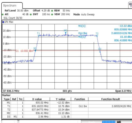
Band26-3MHz-64QAM-26915-15RB#0-2.686
