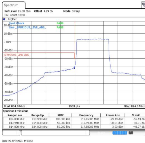
Band26-5MHz-QPSK-26715-25RB#0
