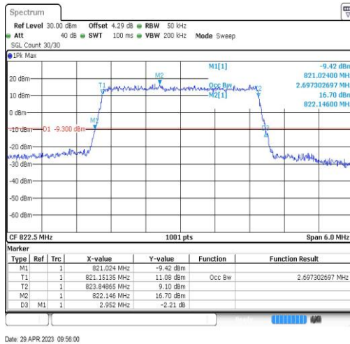
Band26-3MHz-QPSK-26775-15RB#0-2.697
