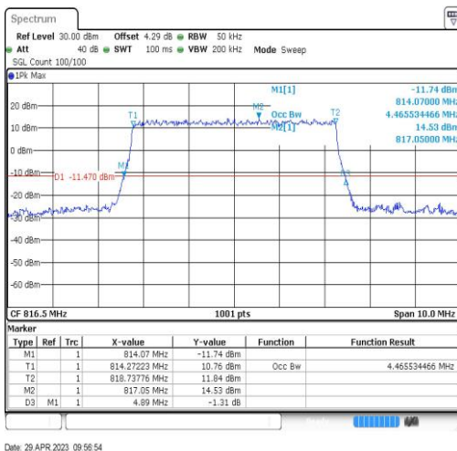
Band26-5MHz-QPSK-26715-25RB#0-4.466
