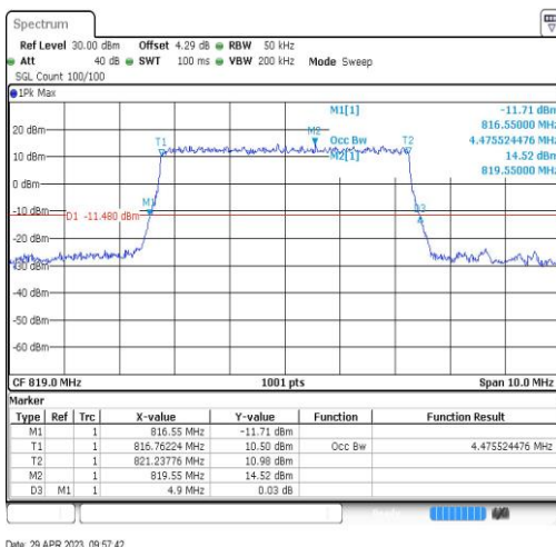
Band26-5MHz-QPSK-26740-25RB#0-4.476
