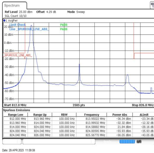
Band26-10MHz-QPSK-26740-1RB#0
