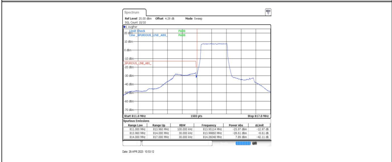
Band26-1.4MHz-QPSK-26697-6RB#0
