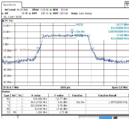
Band26-1.4MHz-QPSK-26697-6RB#0-2.97
