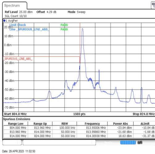
Band26-5MHz-QPSK-26715-1RB#0
