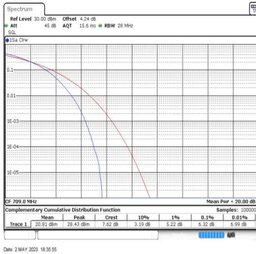
Band17-10MHz-64QAM-23780-50RB#0
