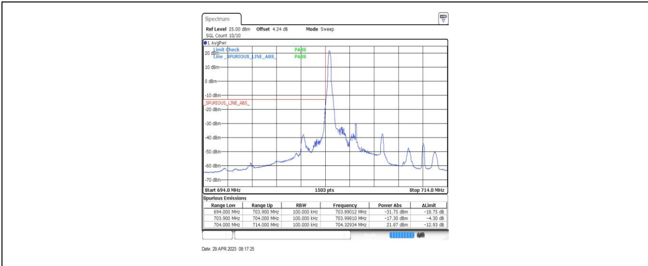
Band17-5MHz-QPSK-23755-1RB#0
