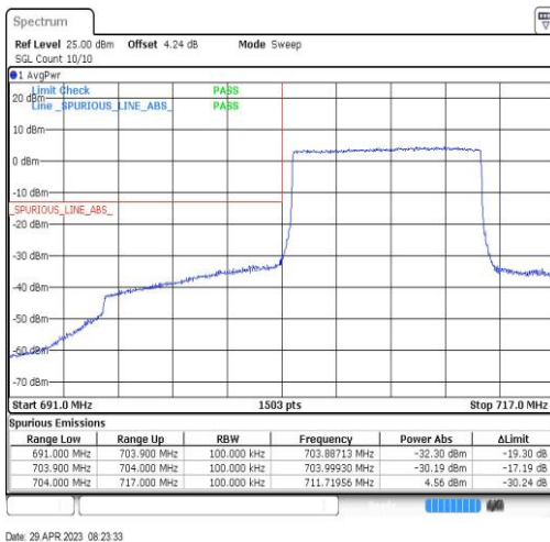
Band17-10MHz-QPSK-23780-50RB#0
