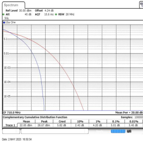
Band17-10MHz-QPSK-23790-50RB#0
