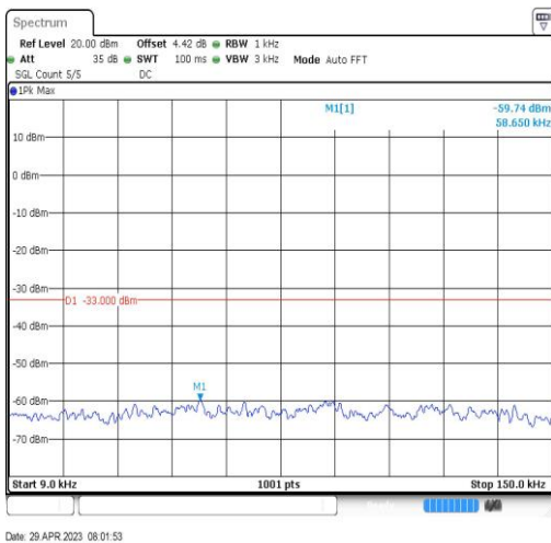
Band17-10MHz-QPSK-23800-1RB#0-Range1:0.009~0.15MHz
