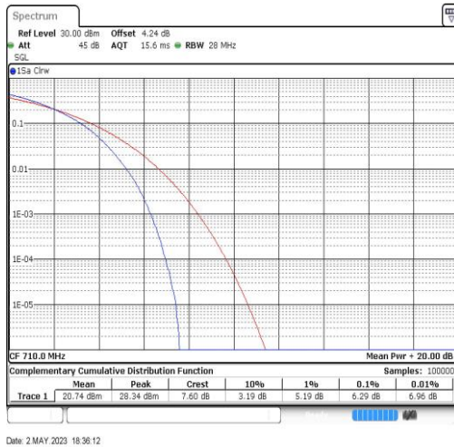
Band17-10MHz-64QAM-23790-50RB#0
