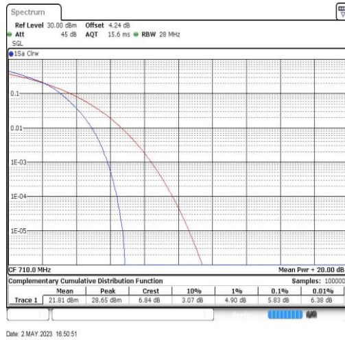
Band17-10MHz-16QAM-23790-50RB#0
