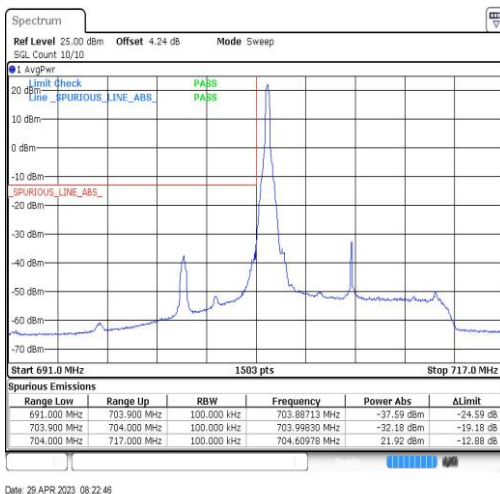
Band17-10MHz-QPSK-23780-1RB#0
