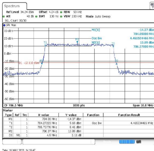
Band17-5MHz-QPSK-23755-25RB#0-9.9
