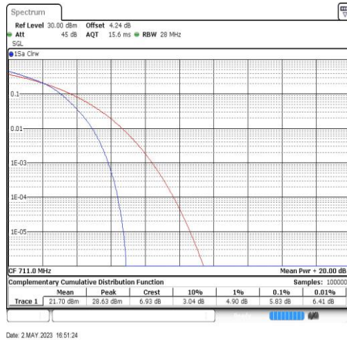
Band17-10MHz-16QAM-23800-50RB#0
