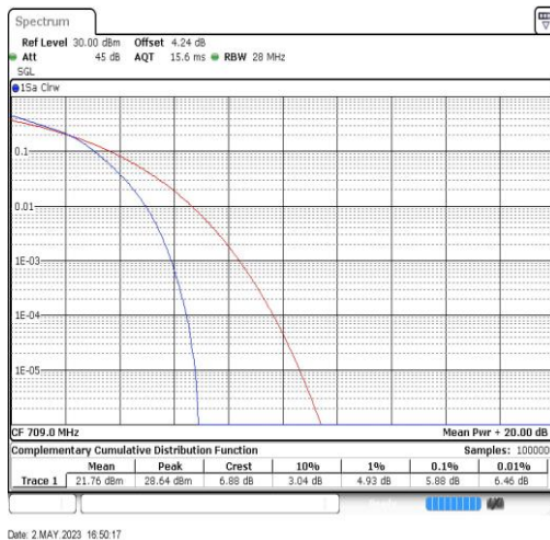
Band17-10MHz-16QAM-23780-50RB#0
