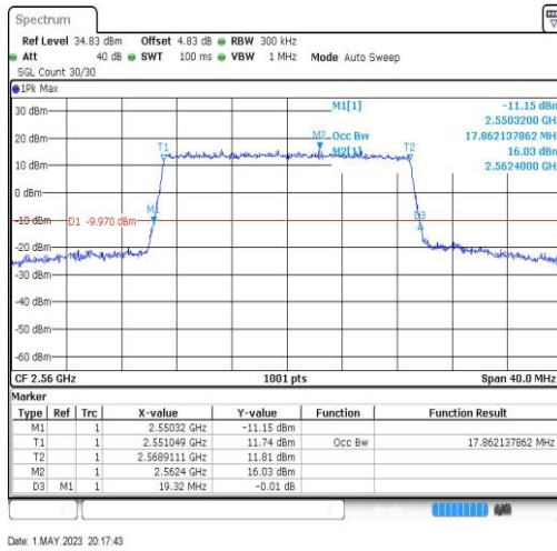
Band7-20MHz-64QAM-21350-100RB#0-17.862
