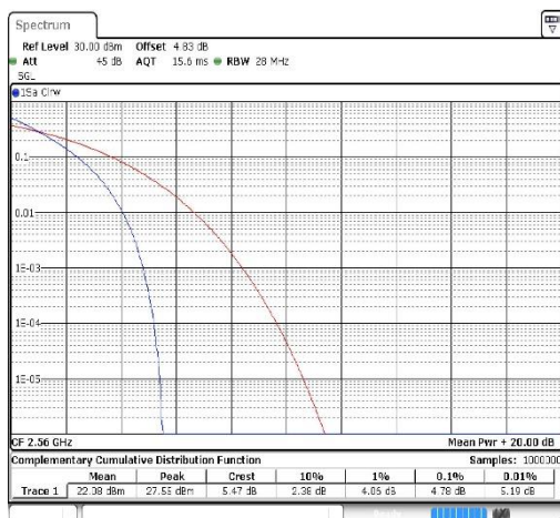
Band7-20MHz-QPSK-21350-100RB#0
