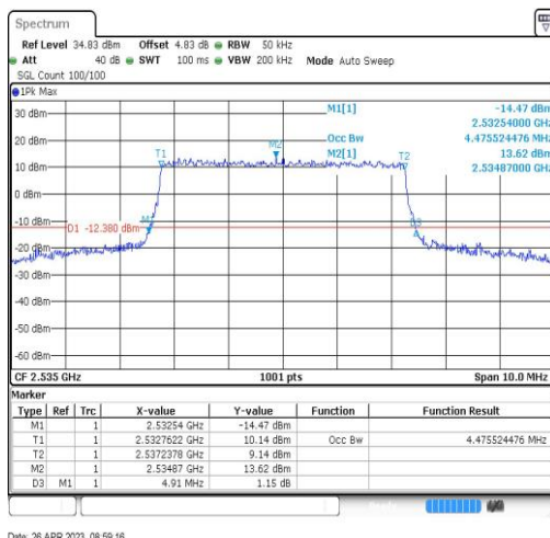
Band7-5MHz-QPSK-21100-25RB#0-4.476
