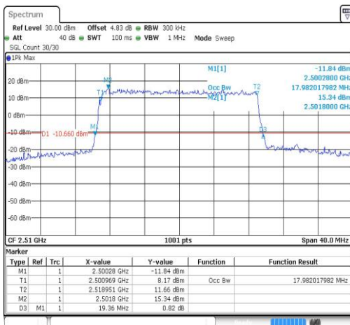
Band7-20MHz-QPSK-20850-100RB#0-17.982
