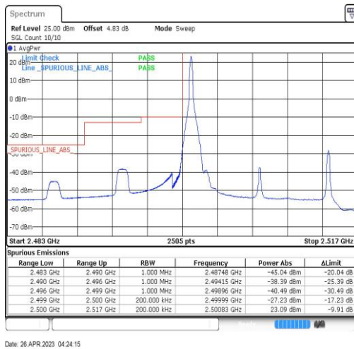
Band7-15MHz-QPSK-20825-1RB#0
