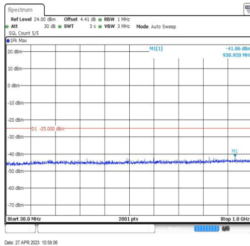
Band7-20MHz-QPSK-21100-1RB#0-Range3:30~1000MHz
