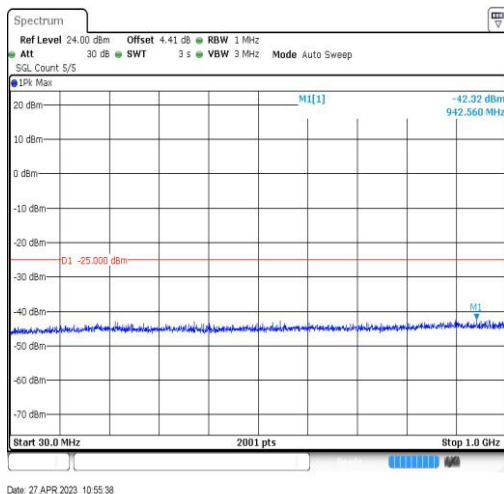
Band7-20MHz-QPSK-20850-1RB#0-Range3:30~1000MHz
