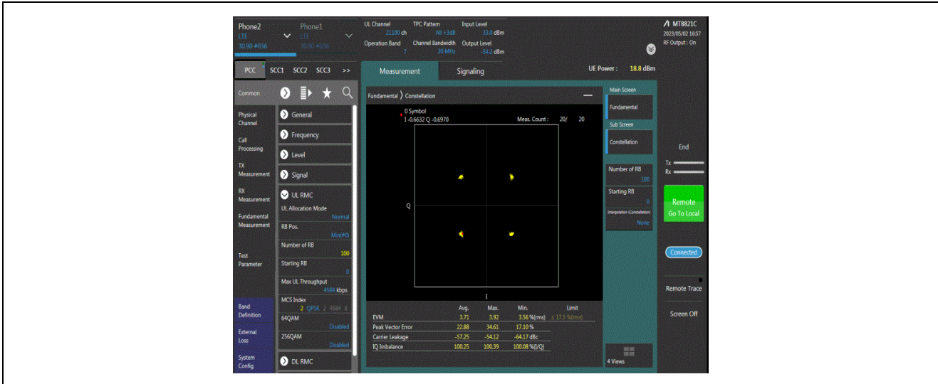
Band7-20MHz-QPSK-21100-100RB#0
