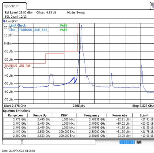
Band7-20MHz-QPSK-20850-1RB#0
