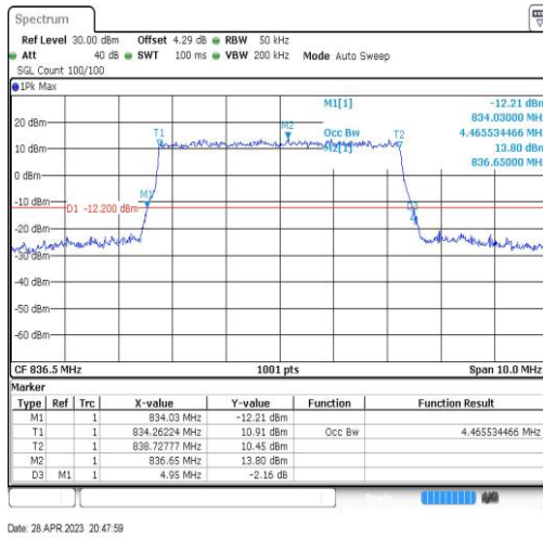
Band5-5MHz-16QAM-20525-25RB#0-4.466
