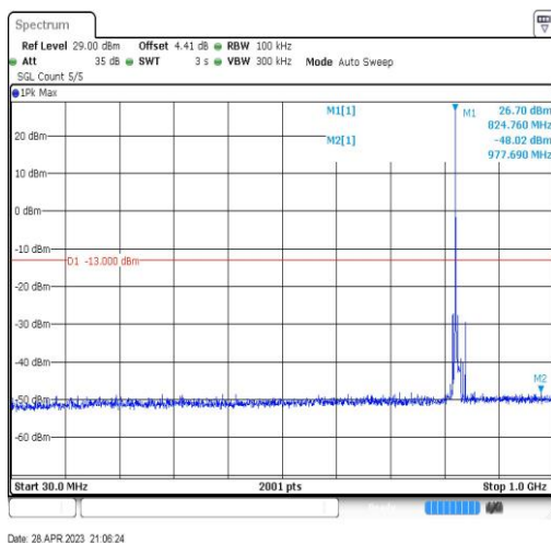
Band5-10MHz-QPSK-20450-1RB#0-Range3:30~1000MHz
