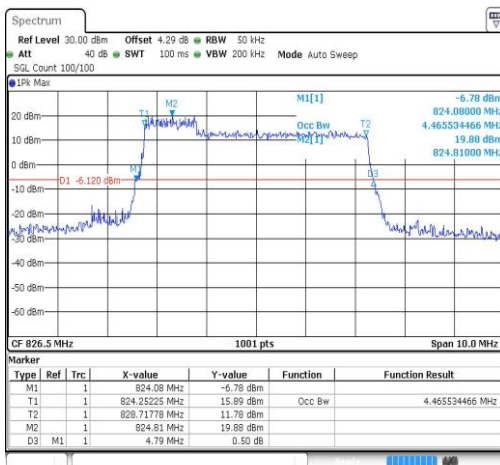
Band5-5MHz-QPSK-20425-25RB#0-4.466
