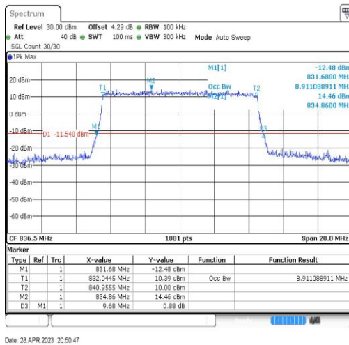
Band5-10MHz-16QAM-20525-50RB#0-8.911
