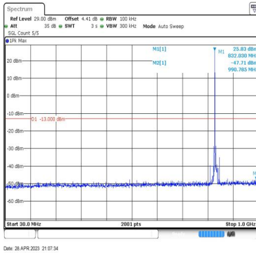
Band5-10MHz-QPSK-20525-1RB#0-Range3:30~1000MHz
