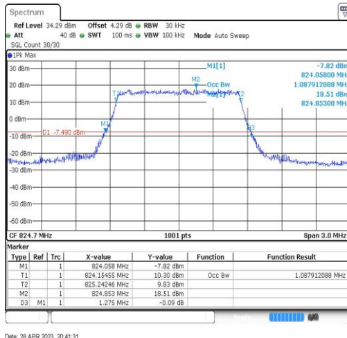
Band5-1.4MHz-QPSK-20407-6RB#0-1.088
