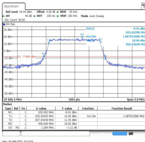
Band5-1.4MHz-QPSK-20525-6RB#0-1.088
