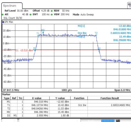
Band5-3MHz-64QAM-20525-15RB#0-2.685
