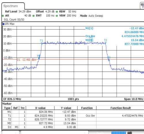
Band5-5MHz-64QAM-20425-25RB#0-4.476
