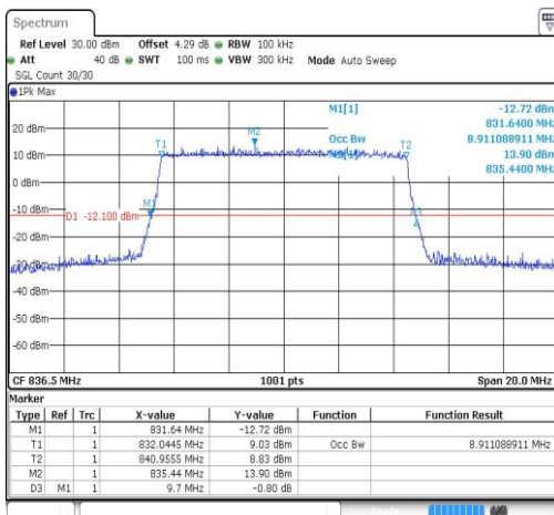
Band5-10MHz-64QAM-20525-50RB#0-8.911
