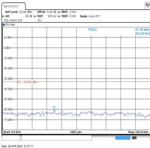
Band5-10MHz-QPSK-20525-1RB#0-Range1:0.009~0.15MHz
