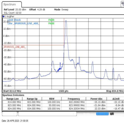
Band5-5MHz-QPSK-20425-1RB#0
