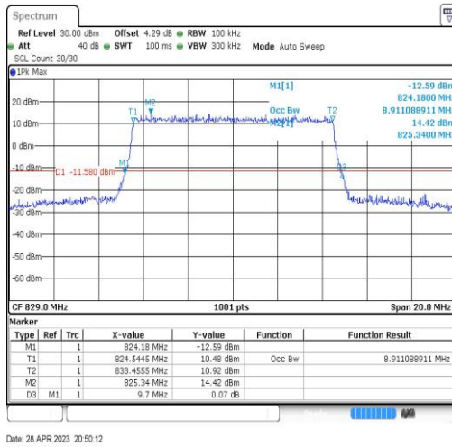
Band5-10MHz-16QAM-20450-50RB#0-8.911
