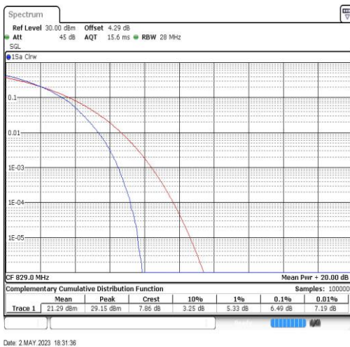
Band5-10MHz-64QAM-20450-50RB#0
