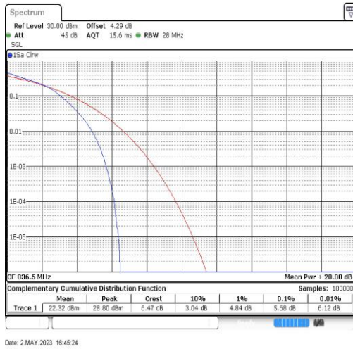
Band5-10MHz-16QAM-20525-50RB#0
