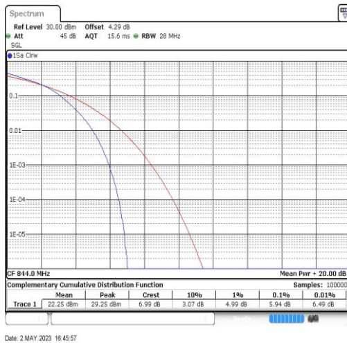
Band5-10MHz-16QAM-20600-50RB#0
