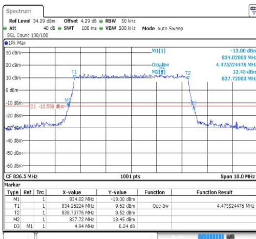
Band5-5MHz-64QAM-20425-25RB#0-4.476
