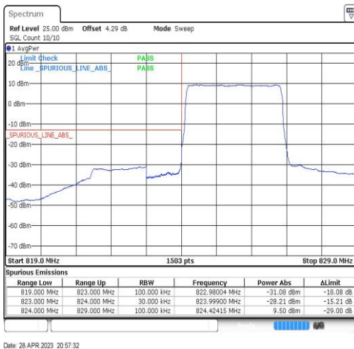
Band5-3MHz-QPSK-20415-15RB#0
