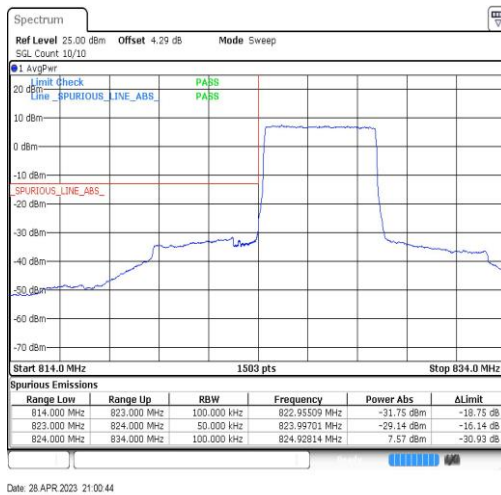
Band5-5MHz-QPSK-20425-25RB#0
