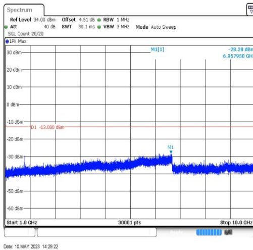
GSM850-190-5-1000~10000MHz-6957.95
