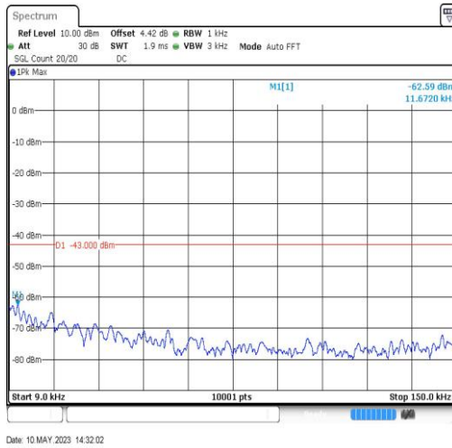
GSM1900-512-0-0.009~0.15MHz-0.01
