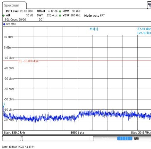
EGPRS850-128-8-0.15~30MHz-0.17
