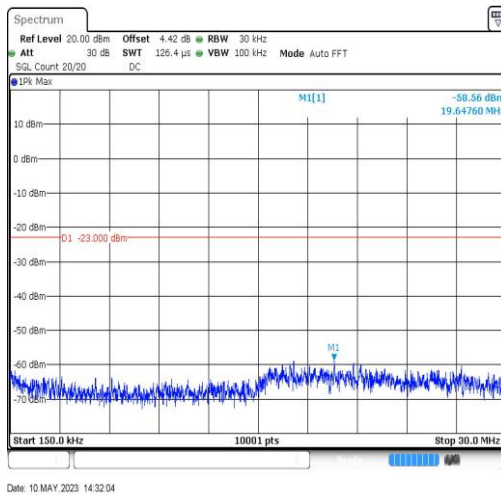
GSM1900-512-0-0.15~30MHz-19.65
