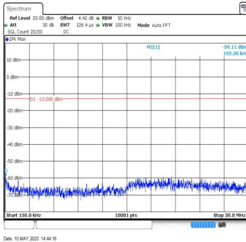
EGPRS850-190-8-0.15~30MHz-0.19
