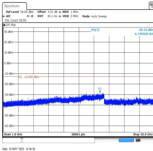
EGPRS850-190-8-1000~10000MHz-6748.26
