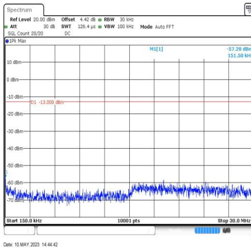
EGPRS850-251-8-0.15~30MHz-0.15
