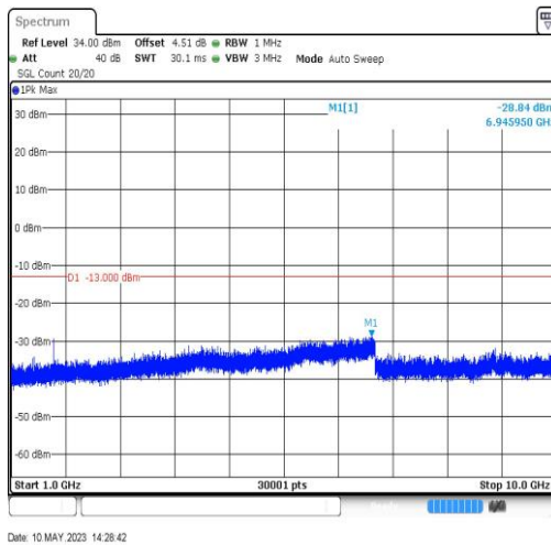
GSM850-128-5-1000~10000MHz-6945.95
