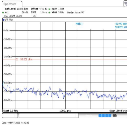
EGPRS850-128-8-0.009~0.15MHz-0.01
