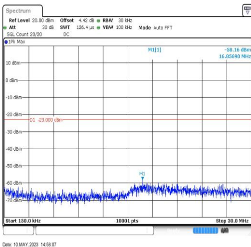
EGPRS1900-512-2-0.15~30MHz-16.86
