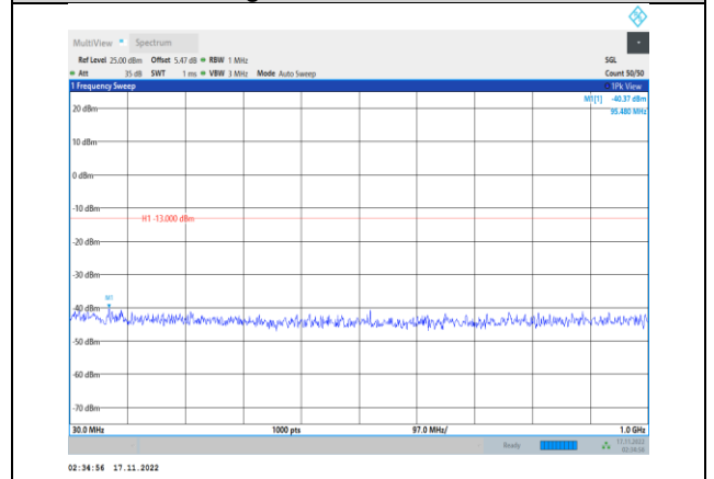
Band66-5MHz-64QAM-132647-1RB#0- Range1:30~1000MHz
