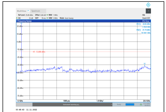
Band66-10MHz-QPSK-132322-1RB#0- Range2:1000~20000MHz
