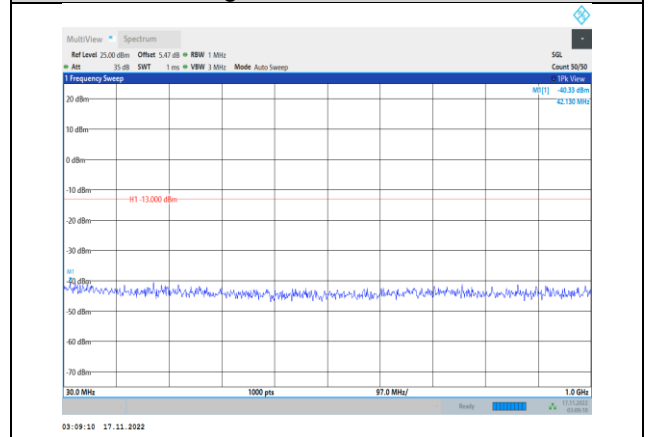
Band66-3MHz-64QAM-132657-1RB#0- Range1:30~1000MHz
