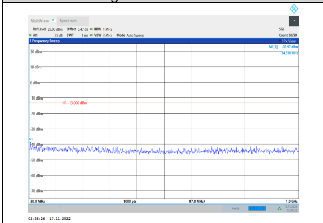
Band66-5MHz-64QAM-132322-1RB#0- Range1:30~1000MHz
