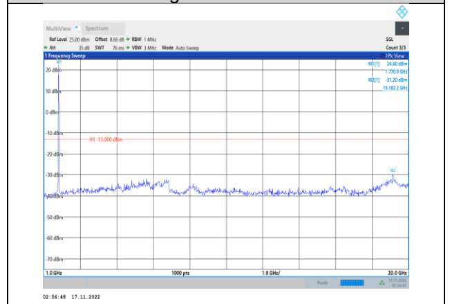
Band66-20MHz-64QAM-132572-1RB#0- Range2:1000~20000MHz
