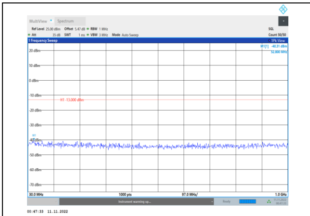
Band66-10MHz-QPSK-132022-1RB#0- Range1:30~1000MHz
