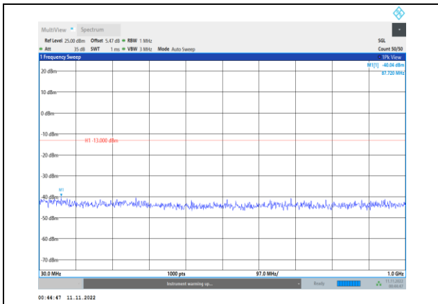
Band66-15MHz-16QAM-132047-1RB#0- Range1:30~1000MHz
