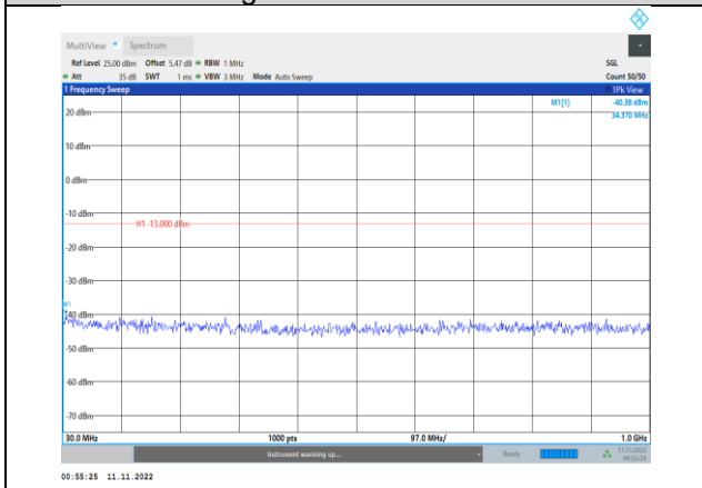
Band66-3MHz-QPSK-132322-1RB#0- Range1:30~1000MHz
