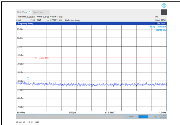
Band66-3MHz-64QAM-131987-1RB#0- Range1:30~1000MHz
