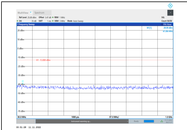
Band66-5MHz-16QAM-131997-1RB#0- Range1:30~1000MHz
