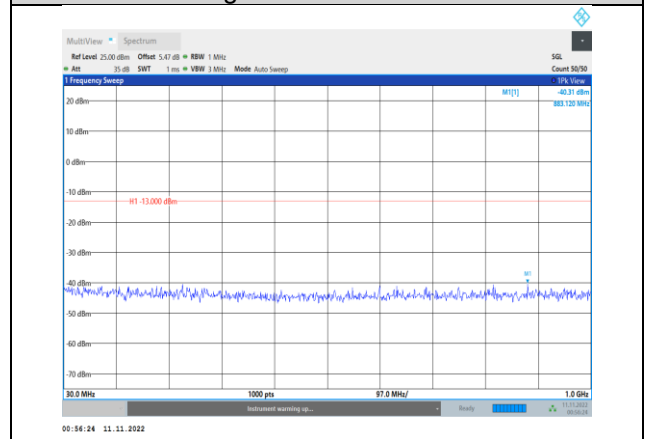
Band66-3MHz-QPSK-132657-1RB#0- Range1:30~1000MHz
