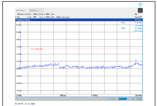
Band66-1.4MHz-16QAM-132322-1RB#0- Range2:1000~20000MHz
