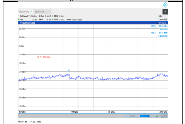
Band66-3MHz-64QAM-132657-1RB#0- Range2:1000~20000MHz
