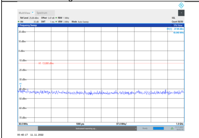
Band66-15MHz-QPSK-132322-1RB#0- Range1:30~1000MHz
