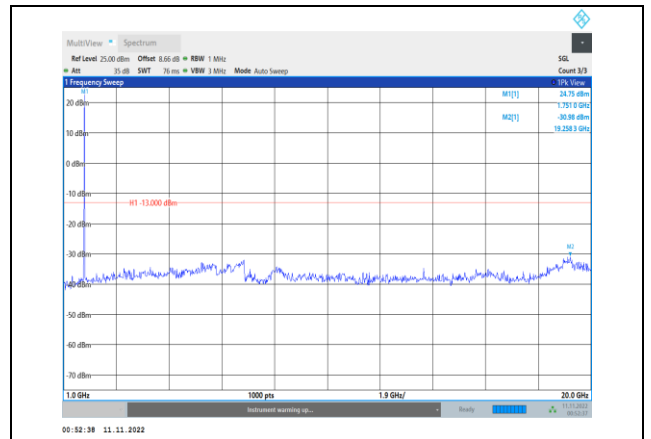
Band66-5MHz-16QAM-132322-1RB#0- Range2:1000~20000MHz
