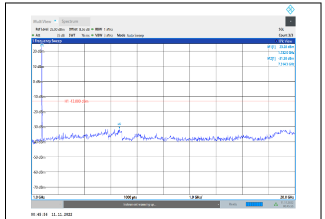
Band66-15MHz-16QAM-132322-1RB#0- Range2:1000~20000MHz
