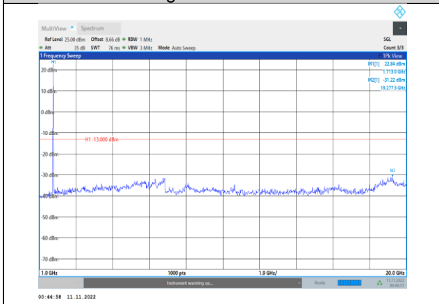
Band66-15MHz-16QAM-132047-1RB#0- Range2:1000~20000MHz
