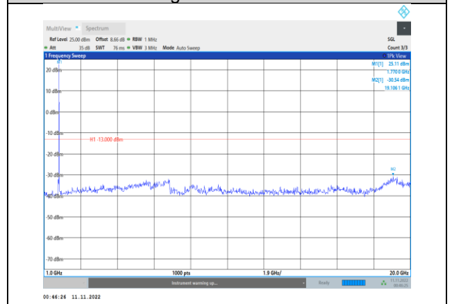
Band66-15MHz-QPSK-132597-1RB#0- Range2:1000~20000MHz
