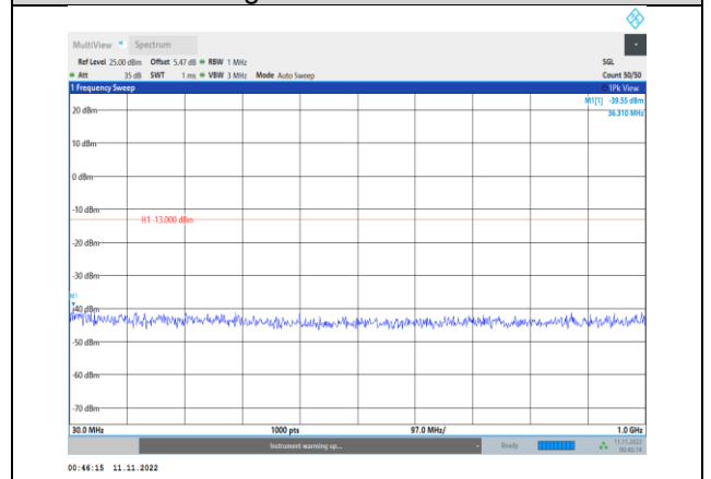
Band66-15MHz-QPSK-132597-1RB#0- Range1:30~1000MHz
