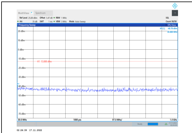
Band66-1.4MHz-64QAM-131979-1RB#0- Range1:30~1000MHz
