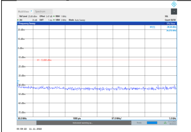
Band66-20MHz-16QAM-132322-1RB#0- Range1:30~1000MHz
