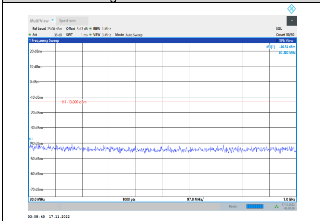
Band66-3MHz-64QAM-132322-1RB#0- Range1:30~1000MHz
