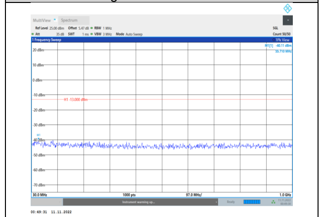
Band66-10MHz-QPSK-132622-1RB#0- Range1:30~1000MHz
