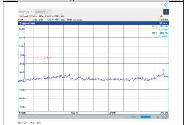
Band66-5MHz-64QAM-132647-1RB#0- Range2:1000~20000MHz
