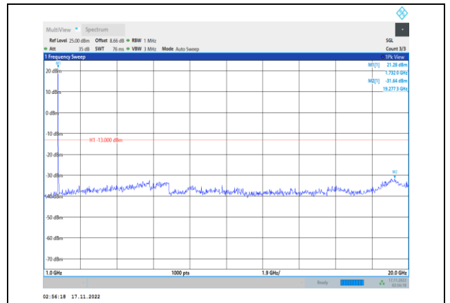
Band66-20MHz-64QAM-132322-1RB#0- Range2:1000~20000MHz
