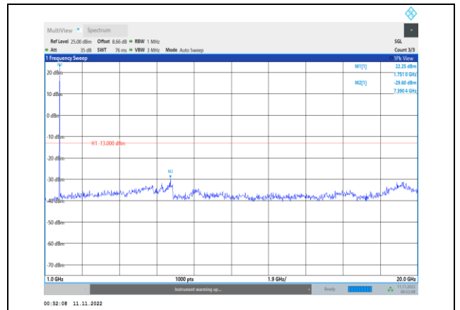
Band66-5MHz-QPSK-132322-1RB#0- Range2:1000~20000MHz
