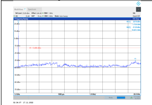
Band66-5MHz-64QAM-131997-1RB#0- Range2:1000~20000MHz
