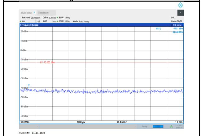
Band66-1.4MHz-16QAM-132665-1RB#0- Range1:30~1000MHz
