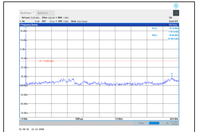
Band66-1.4MHz-QPSK-132322-1RB#0- Range2:1000~20000MHz
