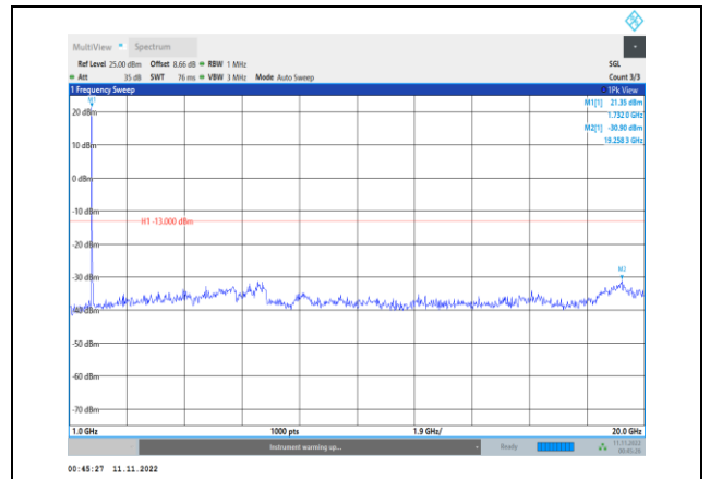
Band66-15MHz-QPSK-132322-1RB#0- Range2:1000~20000MHz
