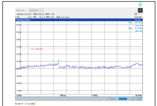
Band66-5MHz-64QAM-132322-1RB#0- Range2:1000~20000MHz
