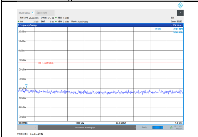
Band66-3MHz-16QAM-132322-1RB#0- Range1:30~1000MHz
