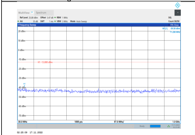
Band66-1.4MHz-64QAM-132322-1RB#0- Range1:30~1000MHz
