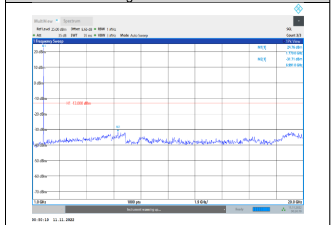
Band66-10MHz-16QAM-132622-1RB#0- Range2:1000~20000MHz
