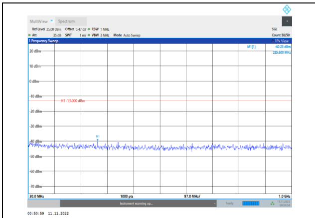
Band66-5MHz-QPSK-131997-1RB#0- Range1:30~1000MHz
