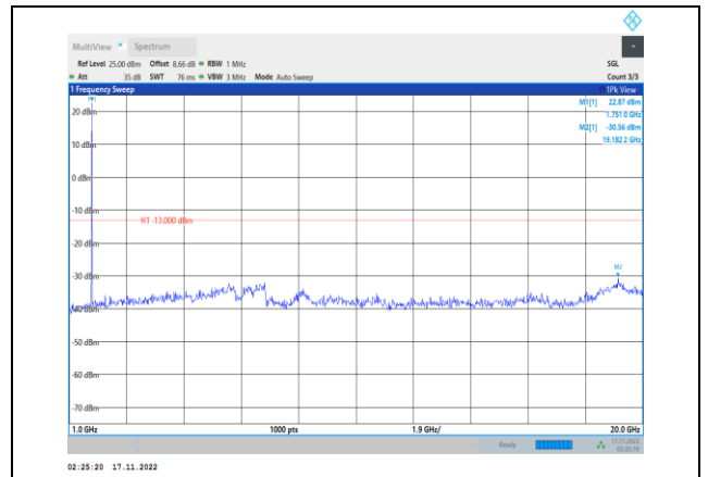
Band66-1.4MHz-64QAM-132322-1RB#0- Range2:1000~20000MHz
