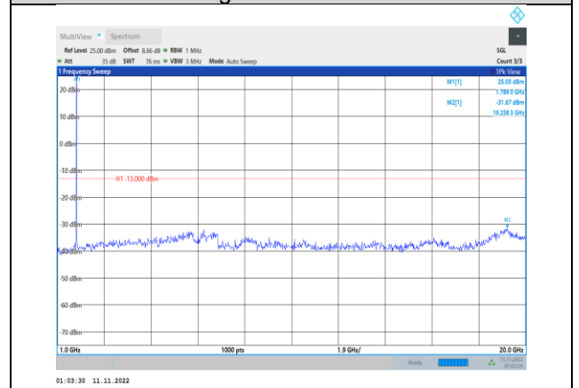
Band66-1.4MHz-QPSK-132665-1RB#0- Range2:1000~20000MHz
