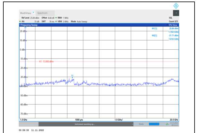
Band66-20MHz-16QAM-132322-1RB#0- Range2:1000~20000MHz
