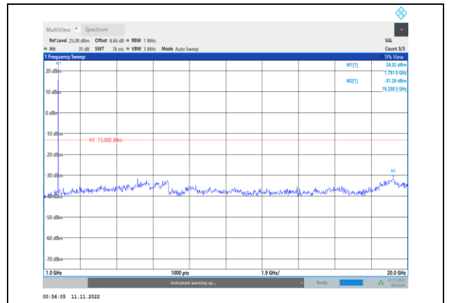
Band66-3MHz-16QAM-132322-1RB#0- Range2:1000~20000MHz
