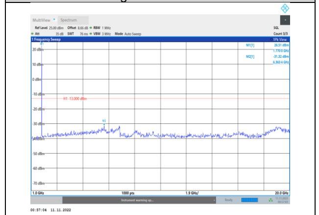
Band66-3MHz-16QAM-132657-1RB#0- Range2:1000~20000MHz
