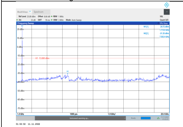
Band66-1.4MHz-16QAM-131979-1RB#0- Range2:1000~20000MHz
