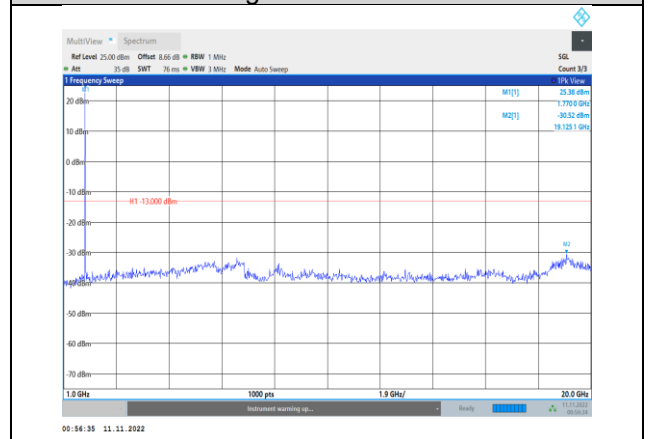
Band66-3MHz-QPSK-132657-1RB#0- Range2:1000~20000MHz
