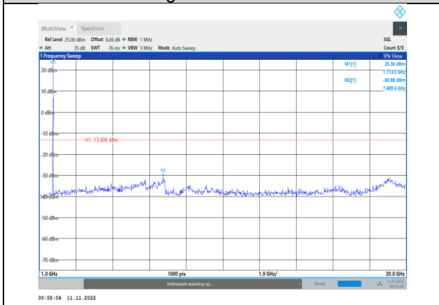
Band66-3MHz-16QAM-131987-1RB#0- Range2:1000~20000MHz
