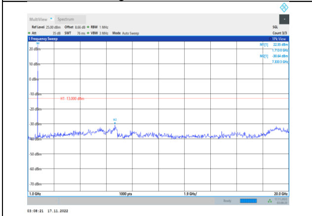
Band66-3MHz-64QAM-131987-1RB#0- Range2:1000~20000MHz
