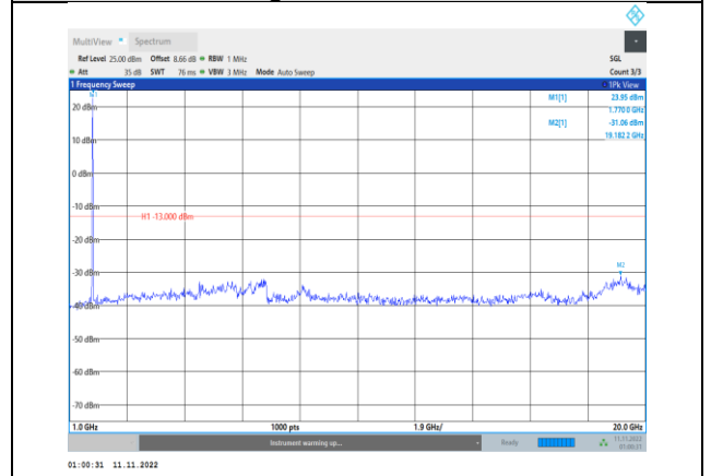
Band66-20MHz-16QAM-132572-1RB#0- Range2:1000~20000MHz
