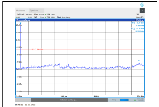
Band66-10MHz-16QAM-132322-1RB#0- Range2:1000~20000MHz
