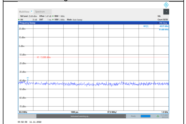
Band66-5MHz-QPSK-132647-1RB#0- Range1:30~1000MHz
