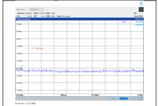
Band66-1.4MHz-QPSK-132665-1RB#0- Range1:30~1000MHz
