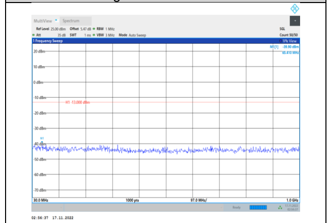
Band66-20MHz-64QAM-132572-1RB#0- Range1:30~1000MHz
