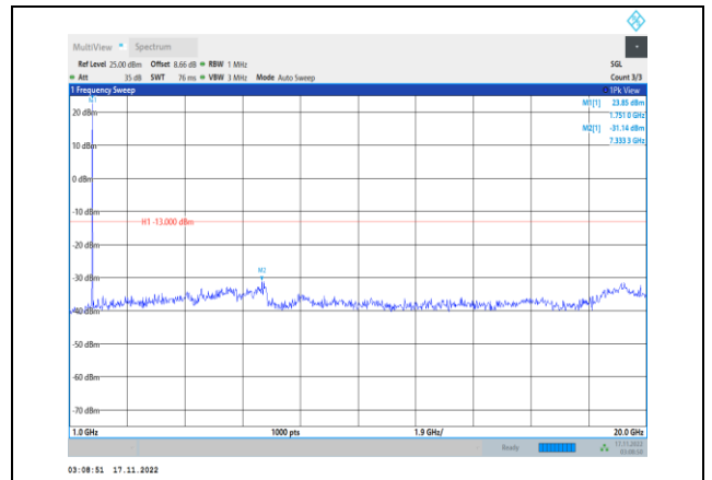
Band66-3MHz-64QAM-132322-1RB#0- Range2:1000~20000MHz
