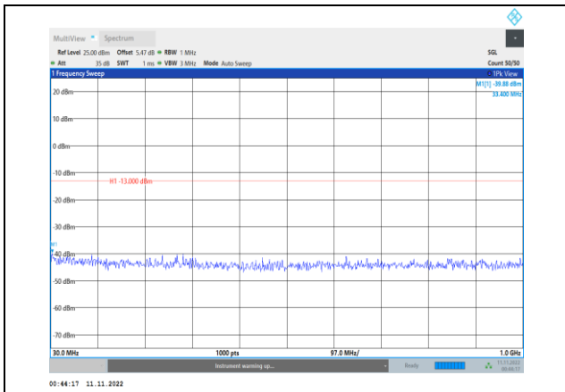
Band66-15MHz-QPSK-132047-1RB#0- Range1:30~1000MHz
