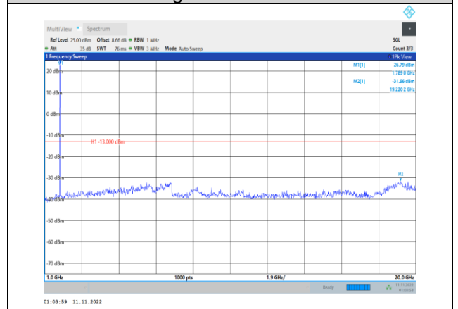
Band66-1.4MHz-16QAM-132665-1RB#0- Range2:1000~20000MHz
