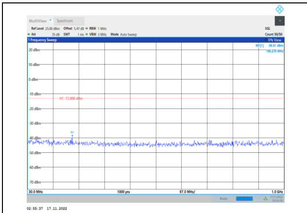
Band66-20MHz-64QAM-132072-1RB#0- Range1:30~1000MHz
