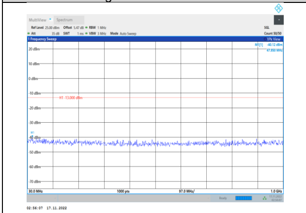
Band66-20MHz-64QAM-132322-1RB#0- Range1:30~1000MHz
