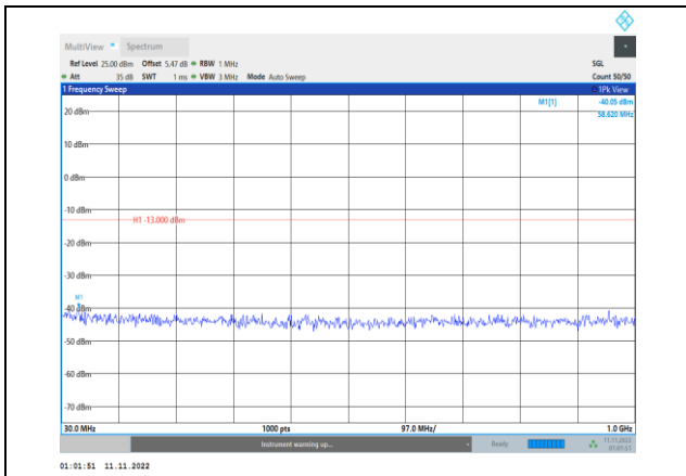
Band66-1.4MHz-16QAM-131979-1RB#0- Range1:30~1000MHz
