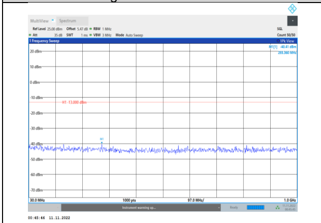
Band66-15MHz-16QAM-132322-1RB#0- Range1:30~1000MHz
