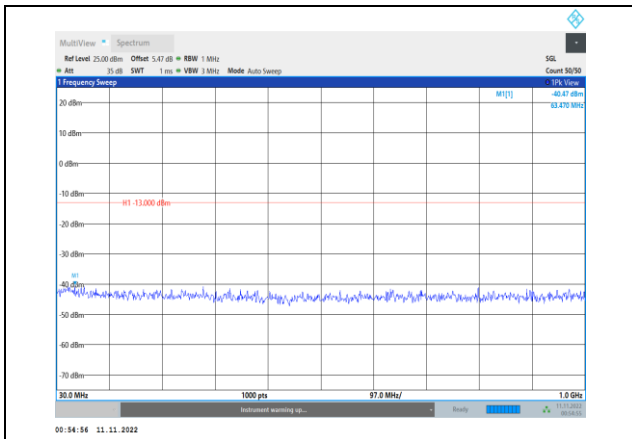
Band66-3MHz-16QAM-131987-1RB#0- Range1:30~1000MHz
