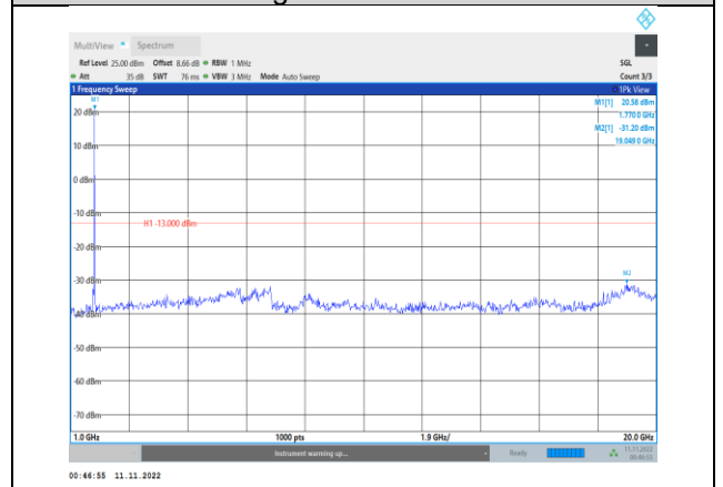
Band66-15MHz-16QAM-132597-1RB#0- Range2:1000~20000MHz
