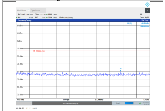
Band66-3MHz-16QAM-132657-1RB#0- Range1:30~1000MHz
