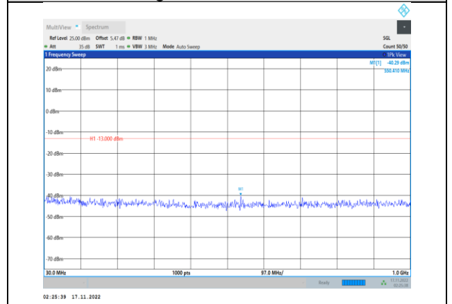
Band66-1.4MHz-64QAM-132665-1RB#0- Range1:30~1000MHz
