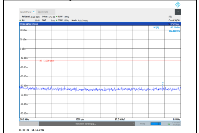
Band66-20MHz-16QAM-132572-1RB#0- Range1:30~1000MHz
