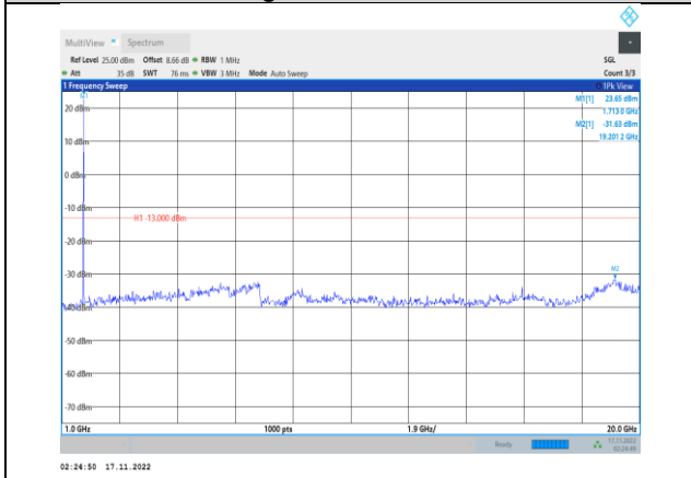
Band66-1.4MHz-64QAM-131979-1RB#0- Range2:1000~20000MHz
