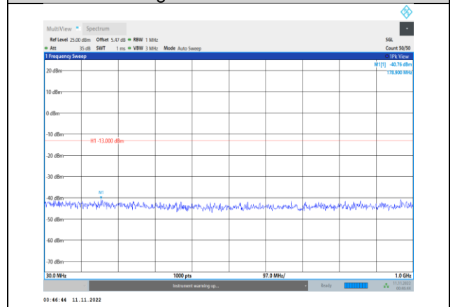
Band66-15MHz-16QAM-132597-1RB#0- Range1:30~1000MHz
