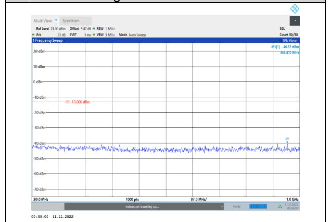
Band66-10MHz-16QAM-132622-1RB#0- Range1:30~1000MHz
