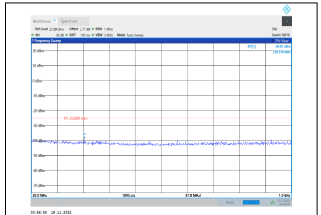
Band38-20MHz-16QAM-38000-1RB#0- Range1:30~1000MHz
