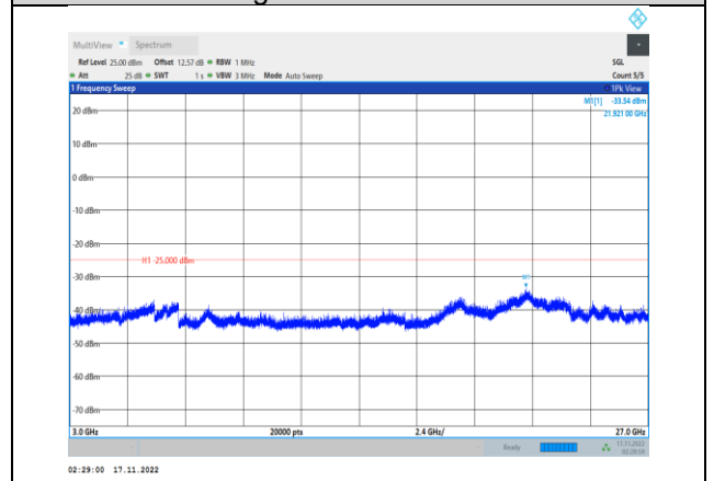
Band41-20MHz-64QAM-40140-1RB#0- Range3:3000~27000MHz
