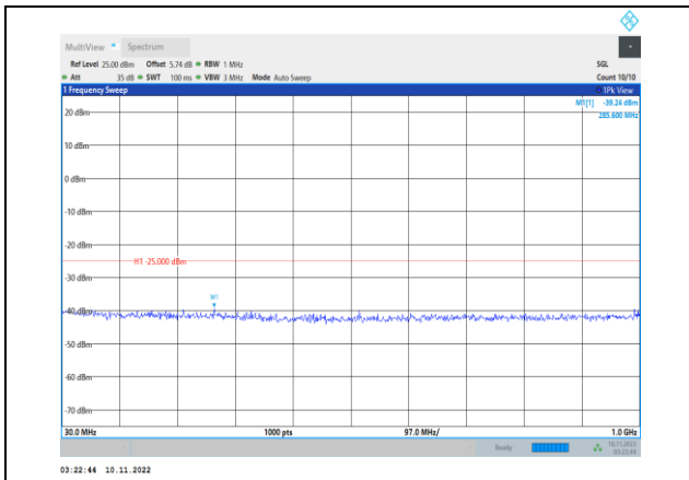
Band41-15MHz-QPSK-40115-1RB#0- Range1:30~1000MHz
