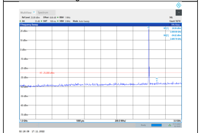
Band41-5MHz-64QAM-40640-1RB#0- Range2:1000~3000MHz
