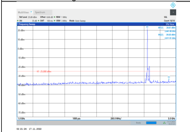
Band41-15MHz-64QAM-41165-1RB#0- Range2:1000~3000MHz
