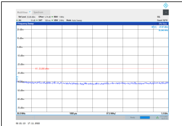
Band41-15MHz-64QAM-41165-1RB#0- Range1:30~1000MHz
