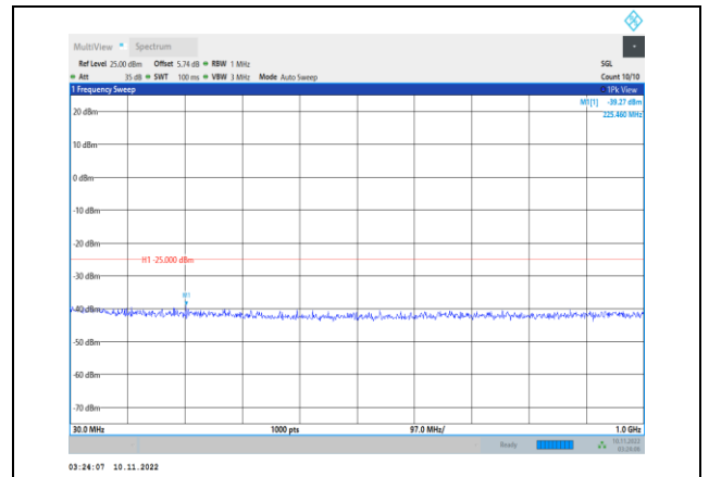
Band41-15MHz-QPSK-40640-1RB#0- Range1:30~1000MHz
