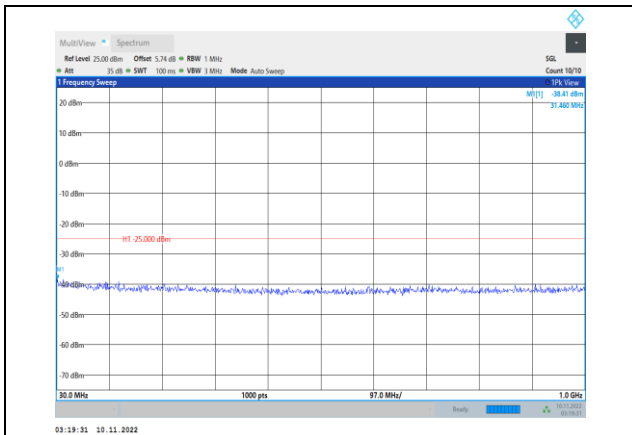
Band41-20MHz-QPSK-40640-1RB#0- Range1:30~1000MHz
