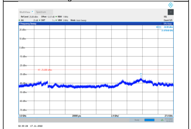
Band41-20MHz-64QAM-41140-1RB#0- Range3:3000~27000MHz
