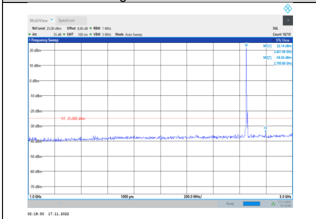
Band41-5MHz-64QAM-41215-1RB#0- Range2:1000~3000MHz
