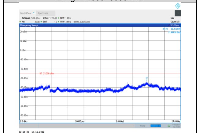
Band41-5MHz-64QAM-40640-1RB#0- Range3:3000~27000MHz
