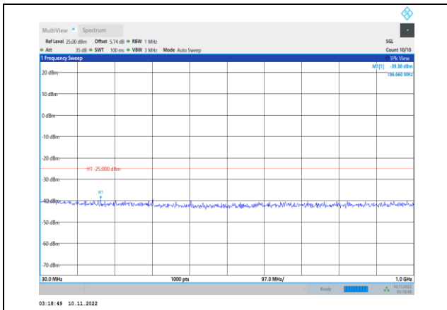
Band41-20MHz-16QAM-40140-1RB#0- Range1:30~1000MHz
