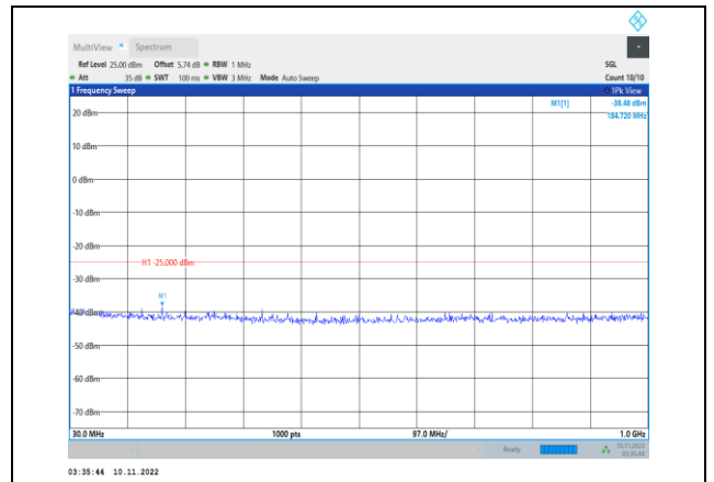
Band41-5MHz-16QAM-41215-1RB#0- Range1:30~1000MHz
