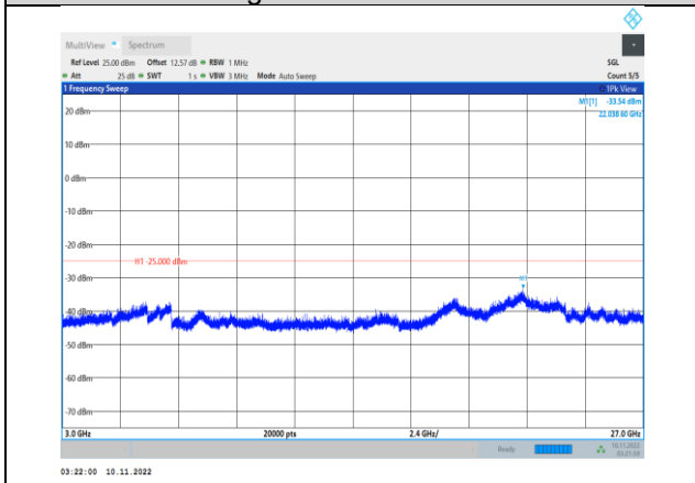
Band41-20MHz-16QAM-41140-1RB#0- Range3:3000~27000MHz
