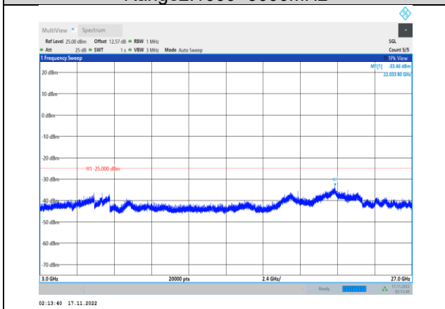
Band41-10MHz-64QAM-40640-1RB#0- Range3:3000~27000MHz
