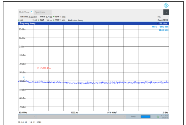
Band41-15MHz-16QAM-41165-1RB#0- Range1:30~1000MHz
