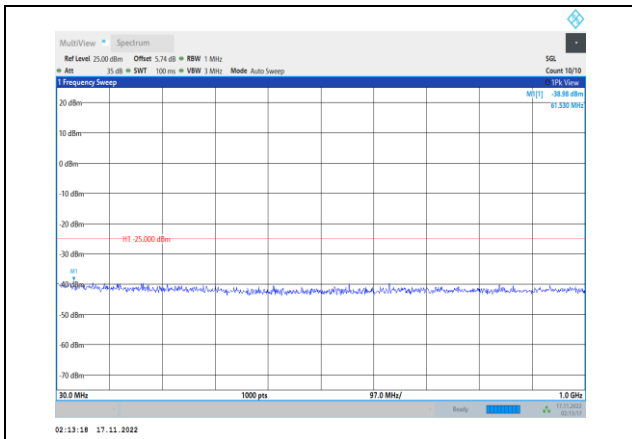
Band41-10MHz-64QAM-40640-1RB#0- Range1:30~1000MHz
