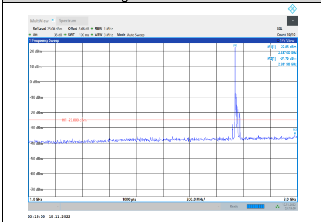
Band41-20MHz-16QAM-40140-1RB#0- Range2:1000~3000MHz
