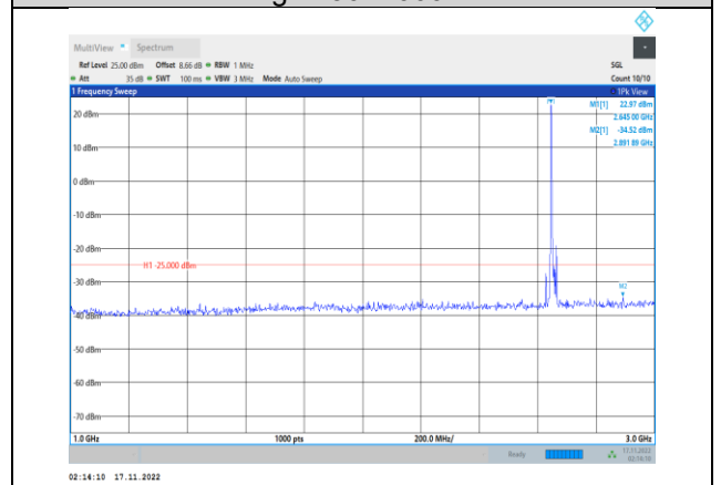
Band41-10MHz-64QAM-41190-1RB#0- Range2:1000~3000MHz
