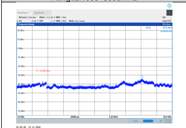
Band38-20MHz-16QAM-37850-1RB#0- Range3:3000~26500MHz
