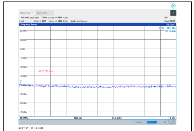
Band41-10MHz-QPSK-40090-1RB#0- Range1:30~1000MHz
