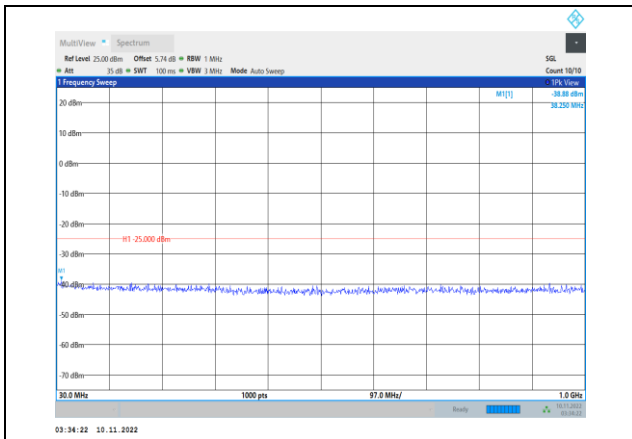
Band41-5MHz-16QAM-40640-1RB#0- Range1:30~1000MHz
