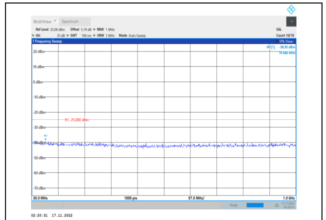
Band41-15MHz-64QAM-40640-1RB#0- Range1:30~1000MHz
