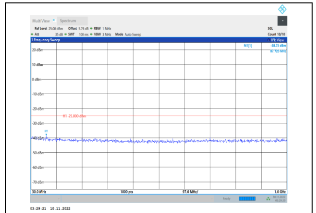
Band41-10MHz-16QAM-40640-1RB#0- Range1:30~1000MHz
