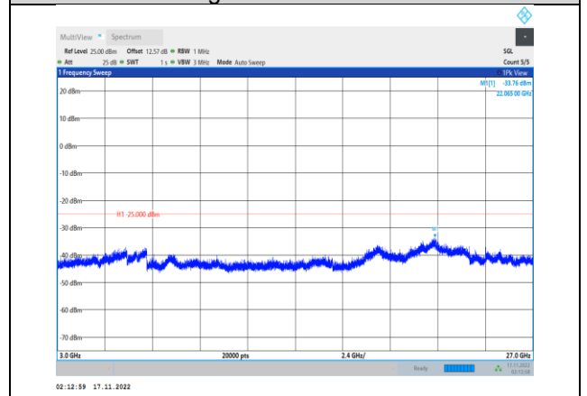
Band41-10MHz-64QAM-40090-1RB#0- Range3:3000~27000MHz
