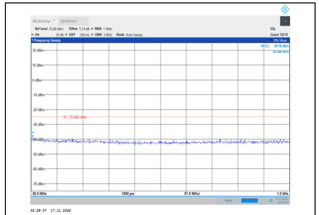
Band41-20MHz-64QAM-40140-1RB#0- Range1:30~1000MHz
