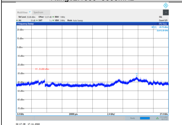
Band41-5MHz-64QAM-40065-1RB#0- Range3:3000~27000MHz
