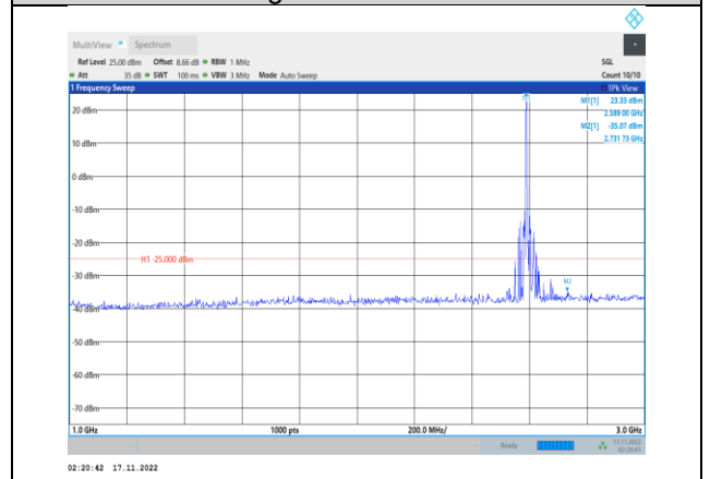
Band41-15MHz-64QAM-40640-1RB#0- Range2:1000~3000MHz
