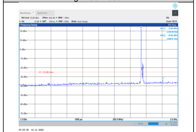
Band41-15MHz-16QAM-40115-1RB#0- Range2:1000~3000MHz
