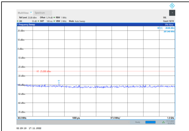
Band41-20MHz-64QAM-40640-1RB#0- Range1:30~1000MHz
