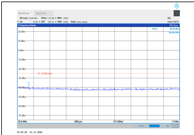
Band41-10MHz-16QAM-41190-1RB#0- Range1:30~1000MHz
