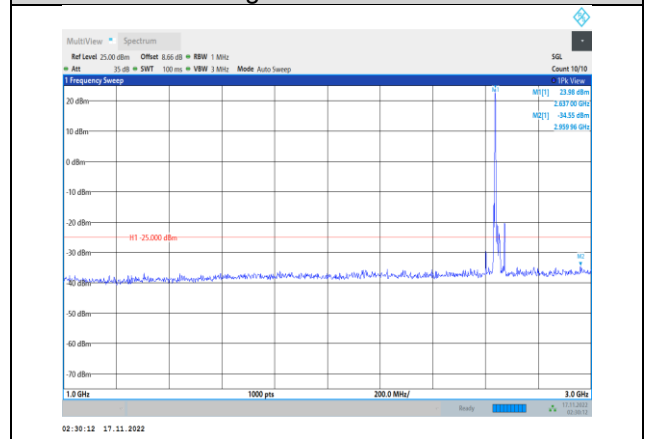
Band41-20MHz-64QAM-41140-1RB#0- Range2:1000~3000MHz
