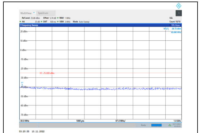
Band41-20MHz-QPSK-41140-1RB#0- Range1:30~1000MHz
