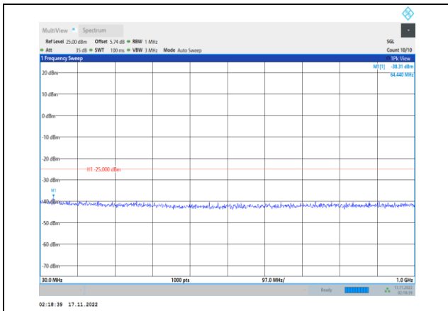
Band41-5MHz-64QAM-41215-1RB#0- Range1:30~1000MHz
