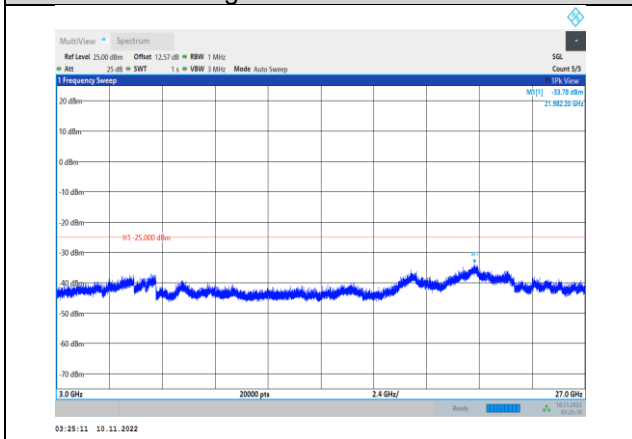
Band41-15MHz-16QAM-40640-1RB#0- Range3:3000~27000MHz
