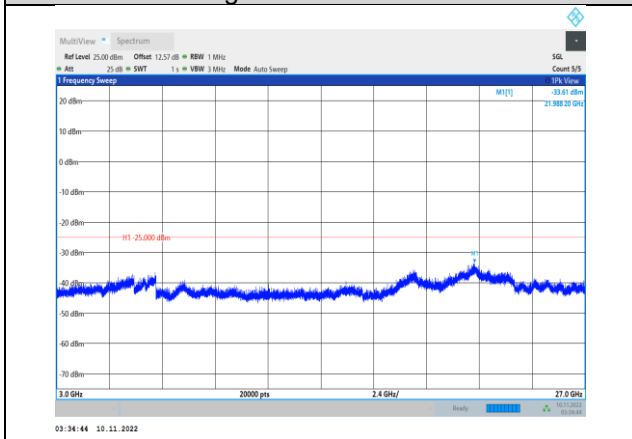
Band41-5MHz-16QAM-40640-1RB#0- Range3:3000~27000MHz
