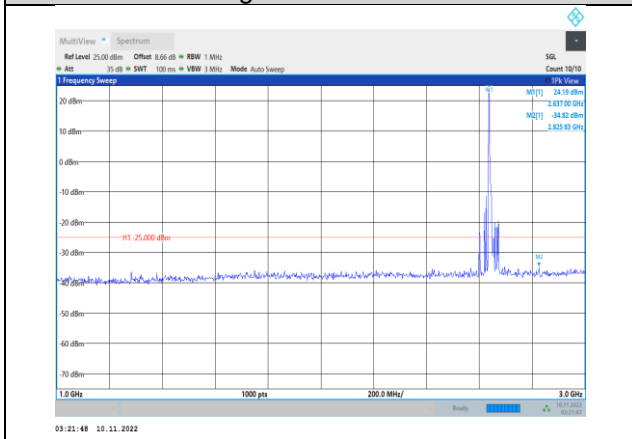
Band41-20MHz-16QAM-41140-1RB#0- Range2:1000~3000MHz
