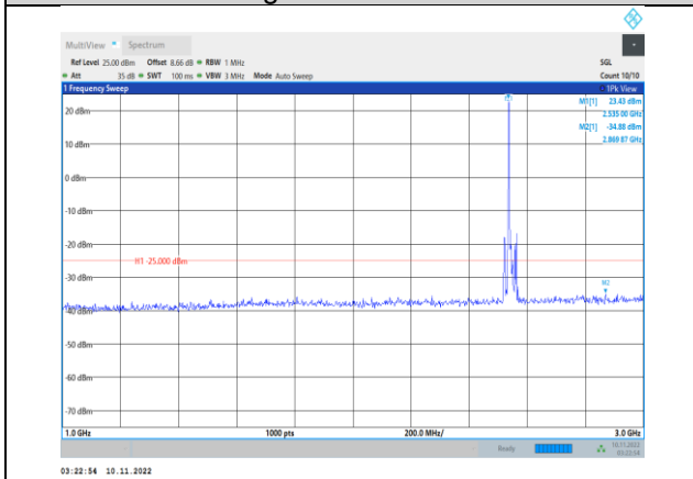
Band41-15MHz-QPSK-40115-1RB#0- Range2:1000~3000MHz
