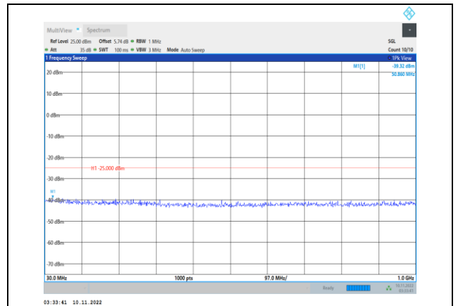
Band41-5MHz-QPSK-40640-1RB#0- Range1:30~1000MHz
