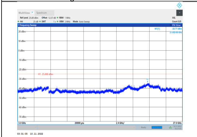
Band41-10MHz-16QAM-41190-1RB#0- Range3:3000~27000MHz
