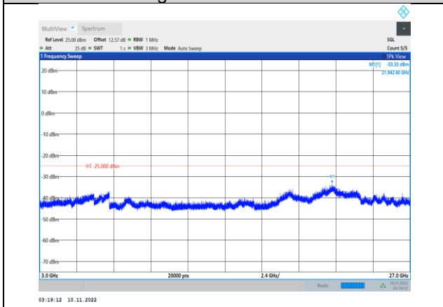
Band41-20MHz-16QAM-40140-1RB#0- Range3:3000~27000MHz
