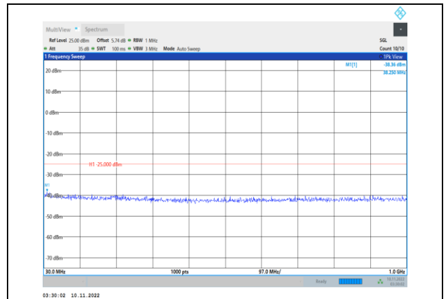
Band41-10MHz-QPSK-41190-1RB#0- Range1:30~1000MHz
