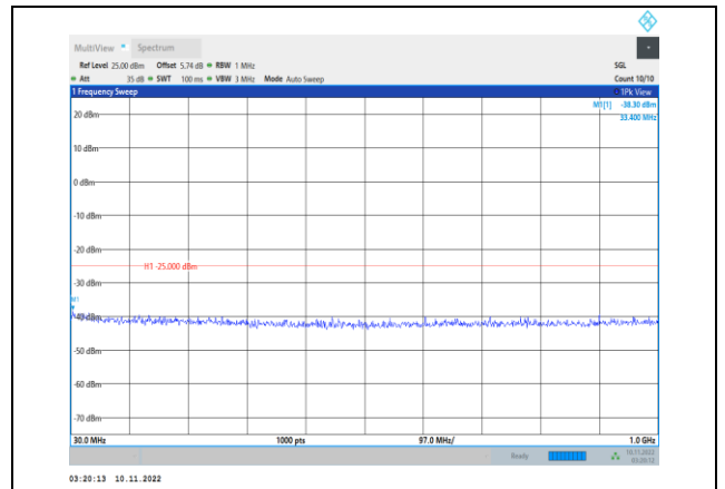
Band41-20MHz-16QAM-40640-1RB#0- Range1:30~1000MHz
