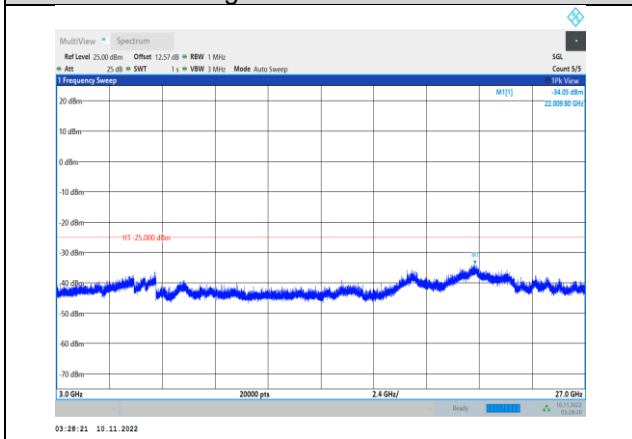
Band41-10MHz-16QAM-40090-1RB#0- Range3:3000~27000MHz
