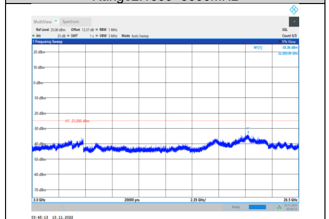
Band38-20MHz-16QAM-38000-1RB#0- Range3:3000~26500MHz
