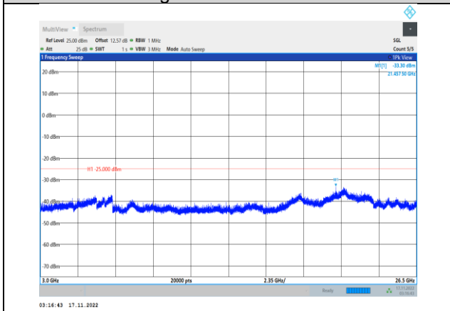
Band38-15MHz-64QAM-38175-1RB#0-Range3:3000~26500MHz
