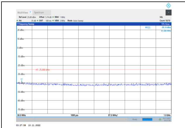
Band41-10MHz-16QAM-40090-1RB#0- Range1:30~1000MHz
