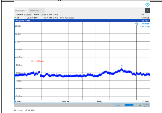
Band41-5MHz-64QAM-41215-1RB#0- Range3:3000~27000MHz
