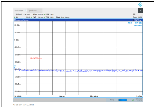
Band41-15MHz-QPSK-41165-1RB#0- Range1:30~1000MHz
