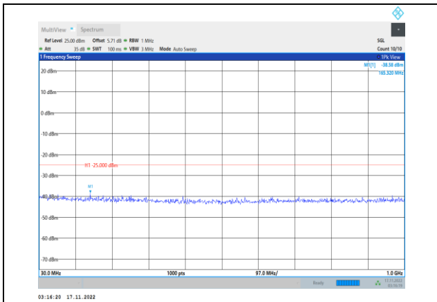
Band38-15MHz-64QAM-38175-1RB#0-Range1:30~1000MHz
