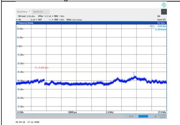
Band41-15MHz-64QAM-40115-1RB#0- Range3:3000~27000MHz
