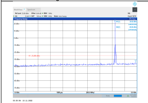
Band41-10MHz-16QAM-41190-1RB#0- Range2:1000~3000MHz
