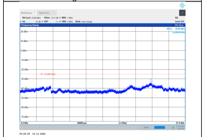
Band41-15MHz-16QAM-41165-1RB#0- Range3:3000~27000MHz
