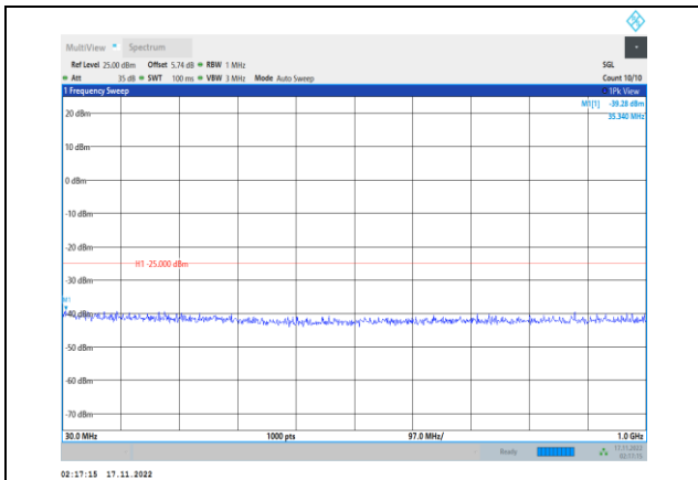
Band41-5MHz-64QAM-40065-1RB#0- Range1:30~1000MHz
