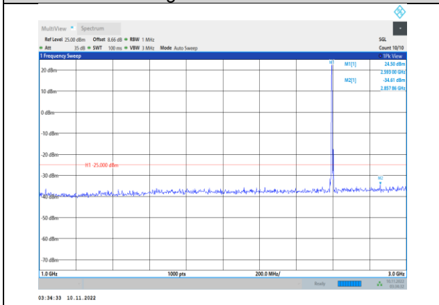
Band41-5MHz-16QAM-40640-1RB#0- Range2:1000~3000MHz
