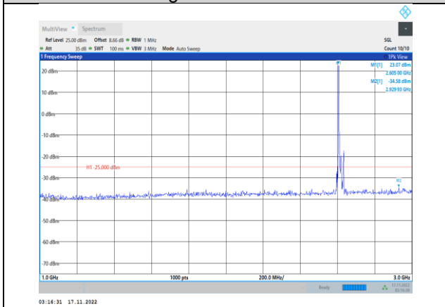
Band38-15MHz-64QAM-38175-1RB#0-Range2:1000~3000MHz
