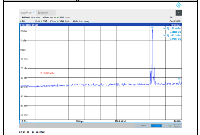
Band41-15MHz-16QAM-41165-1RB#0- Range2:1000~3000MHz
