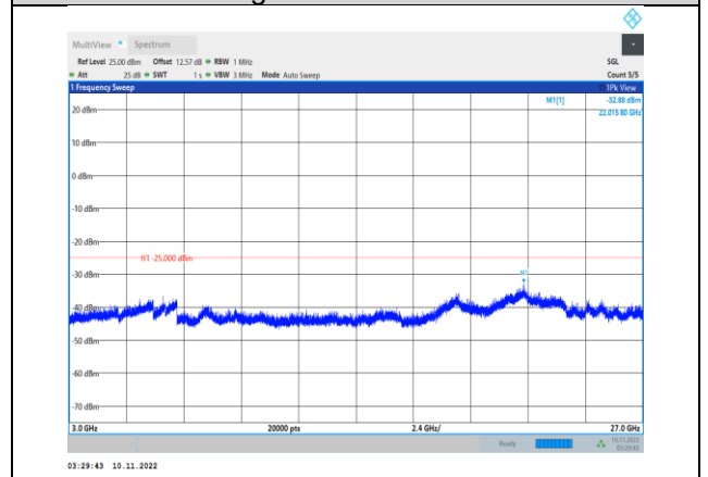
Band41-10MHz-16QAM-40640-1RB#0- Range3:3000~27000MHz
