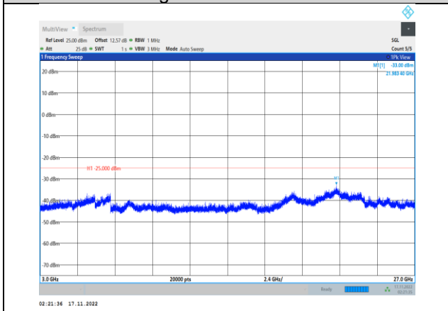
Band41-15MHz-64QAM-41165-1RB#0- Range3:3000~27000MHz
