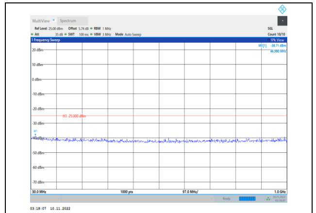
Band41-20MHz-QPSK-40140-1RB#0- Range1:30~1000MHz
