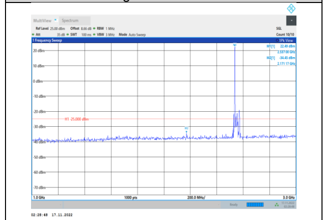
Band41-20MHz-64QAM-40140-1RB#0- Range2:1000~3000MHz
