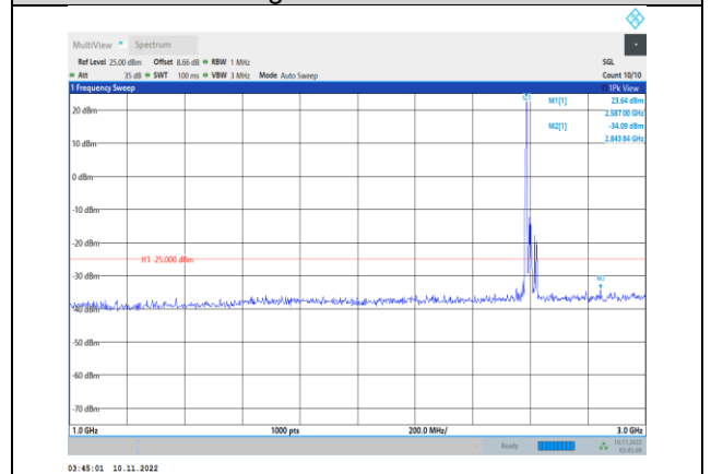
Band38-20MHz-16QAM-38000-1RB#0- Range2:1000~3000MHz
