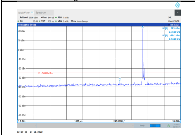
Band41-15MHz-64QAM-40115-1RB#0- Range2:1000~3000MHz
