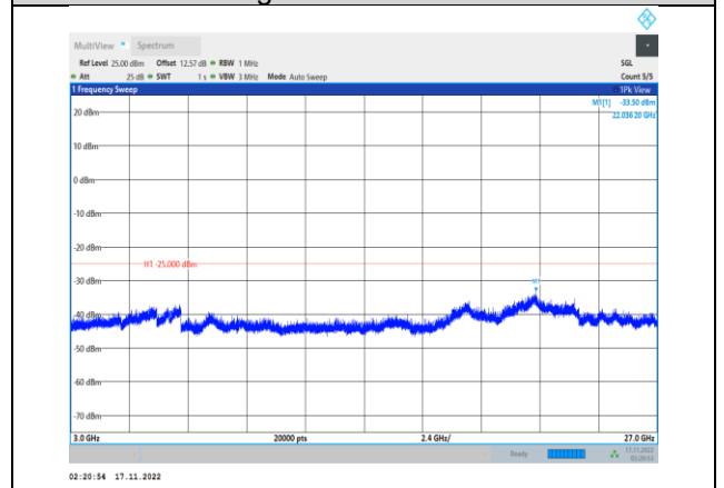
Band41-15MHz-64QAM-40640-1RB#0- Range3:3000~27000MHz
