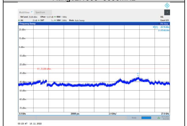
Band41-15MHz-16QAM-40115-1RB#0- Range3:3000~27000MHz
