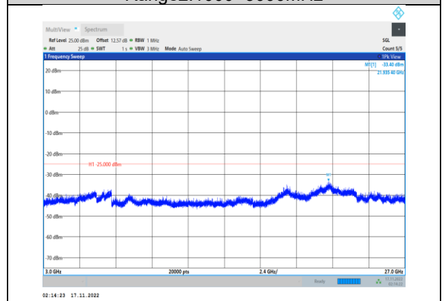
Band41-10MHz-64QAM-41190-1RB#0- Range3:3000~27000MHz
