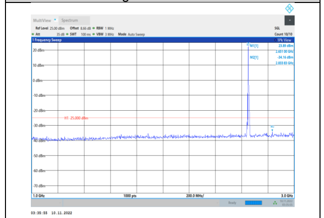
Band41-5MHz-16QAM-41215-1RB#0- Range2:1000~3000MHz
