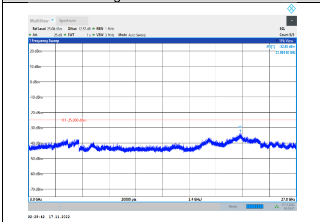
Band41-20MHz-64QAM-40640-1RB#0- Range3:3000~27000MHz
