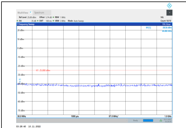
Band41-10MHz-QPSK-40640-1RB#0- Range1:30~1000MHz
