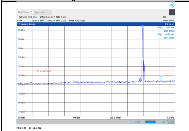
Band41-15MHz-16QAM-40640-1RB#0- Range2:1000~3000MHz
