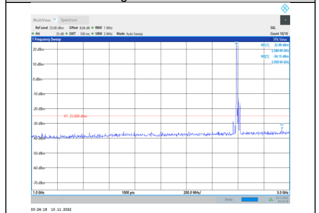
Band41-15MHz-QPSK-40640-1RB#0- Range2:1000~3000MHz
