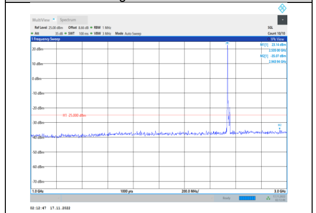
Band41-10MHz-64QAM-40090-1RB#0- Range2:1000~3000MHz
