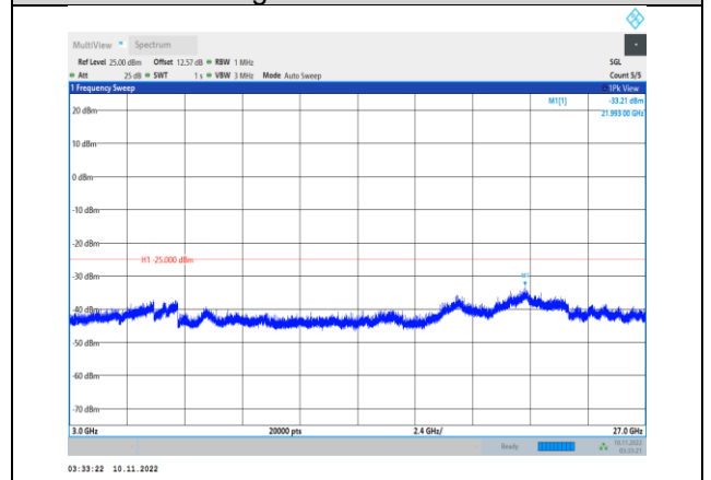
Band41-5MHz-16QAM-40065-1RB#0- Range3:3000~27000MHz
