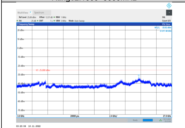
Band41-15MHz-QPSK-40115-1RB#0- Range3:3000~27000MHz
