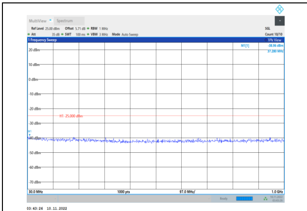
Band38-20MHz-16QAM-37850-1RB#0- Range1:30~1000MHz
