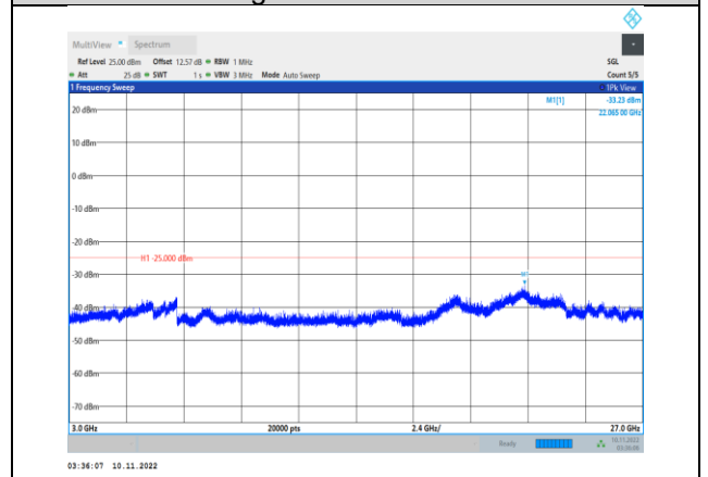
Band41-5MHz-16QAM-41215-1RB#0- Range3:3000~27000MHz
