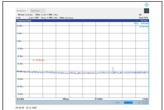
Band41-15MHz-16QAM-40115-1RB#0- Range1:30~1000MHz
