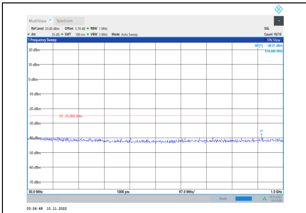
Band41-15MHz-16QAM-40640-1RB#0- Range1:30~1000MHz
