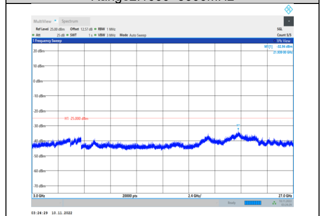
Band41-15MHz-QPSK-40640-1RB#0- Range3:3000~27000MHz
