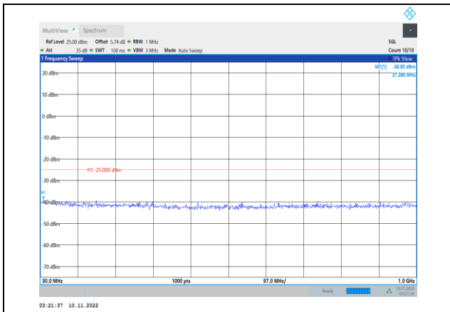
Band41-20MHz-16QAM-41140-1RB#0- Range1:30~1000MHz
