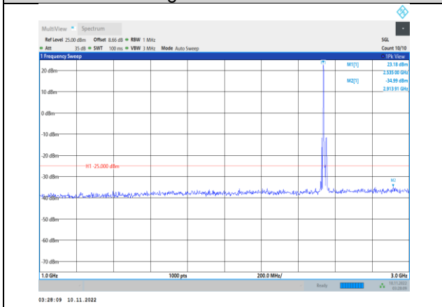
Band41-10MHz-16QAM-40090-1RB#0- Range2:1000~3000MHz
