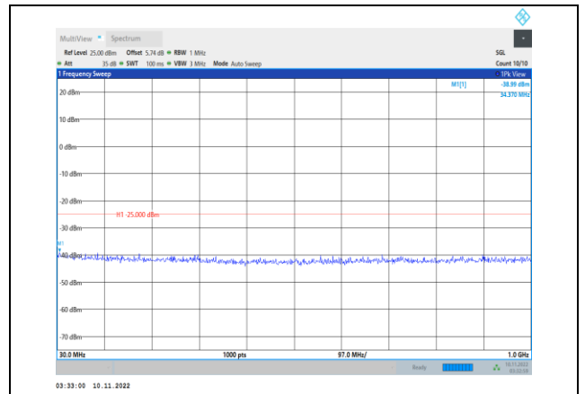
Band41-5MHz-16QAM-40065-1RB#0- Range1:30~1000MHz
