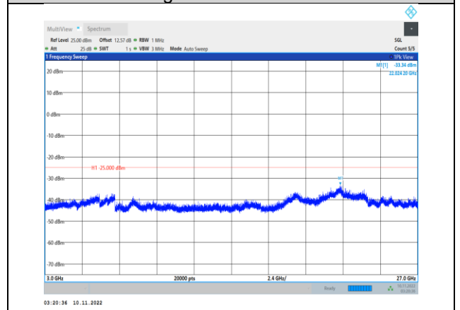
Band41-20MHz-16QAM-40640-1RB#0- Range3:3000~27000MHz
