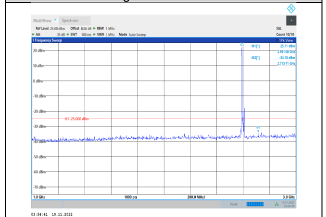
Band38-10MHz-16QAM-38000-1RB#0- Range2:1000~3000MHz
