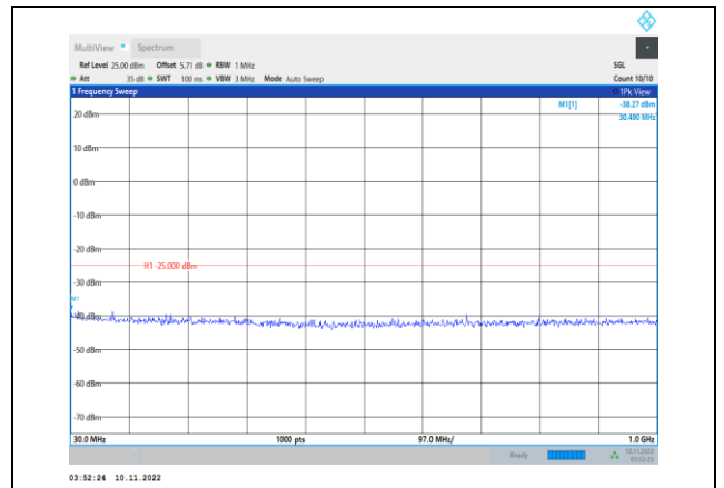
Band38-10MHz-QPSK-37800-1RB#0- Range1:30~1000MHz
