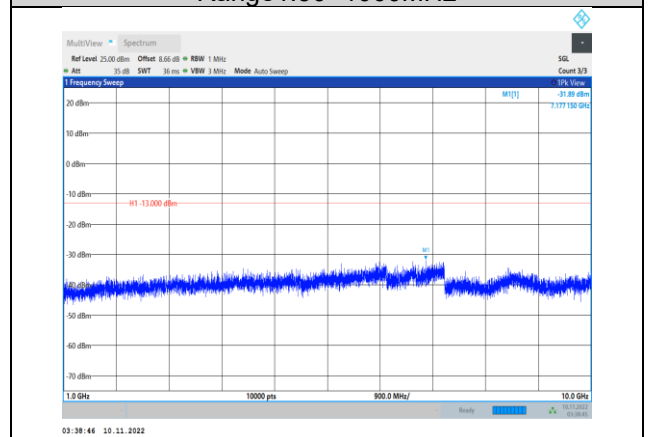
Band26-15MHz-QPSK-26915-1RB#0- Range2:1000~10000MHz
