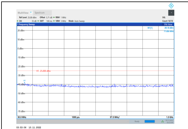
Band38-10MHz-16QAM-37800-1RB#0- Range1:30~1000MHz
