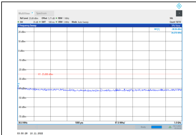
Band38-15MHz-QPSK-38175-1RB#0- Range1:30~1000MHz
