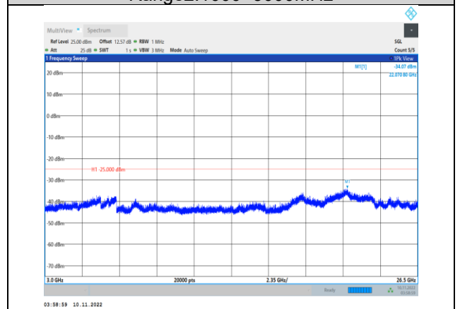
Band38-5MHz-QPSK-38000-1RB#0- Range3:3000~26500MHz
