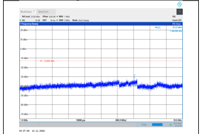
Band26-15MHz-16QAM-26865-1RB#0- Range2:1000~10000MHz
