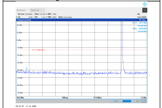
Band26-10MHz-64QAM-26740-1RB#0- Range1:30~1000MHz
