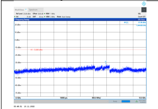
Band26-3MHz-16QAM-26705-1RB#0- Range2:1000~10000MHz
