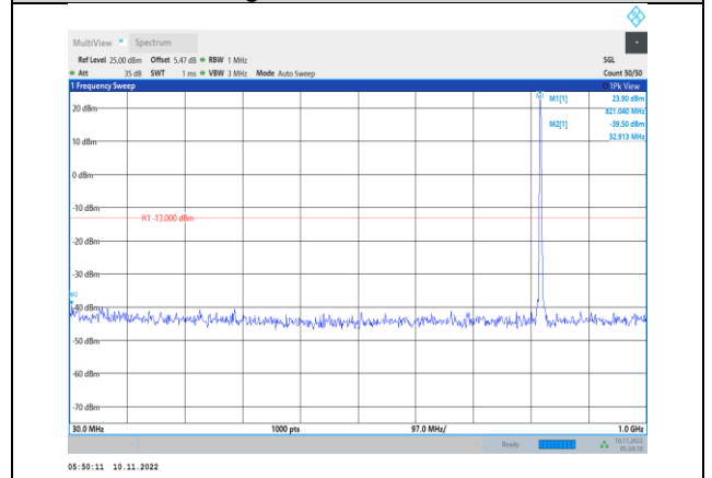
Band26-3MHz-QPSK-26775-1RB#0- Range1:30~1000MHz
