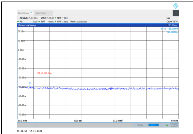
Band38-5MHz-64QAM-38225-1RB#0- Range1:30~1000MHz
