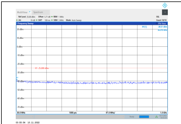
Band38-10MHz-16QAM-38200-1RB#0- Range1:30~1000MHz
