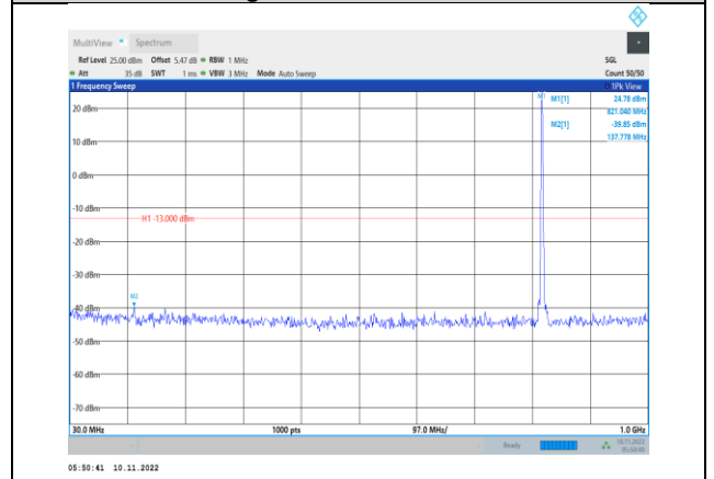
Band26-3MHz-16QAM-26775-1RB#0- Range1:30~1000MHz
