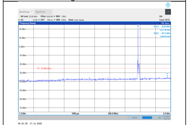
Band38-10MHz-64QAM-37800-1RB#0- Range2:1000~3000MHz
