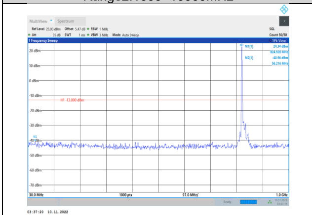
Band26-15MHz-QPSK-26865-1RB#0- Range1:30~1000MHz
