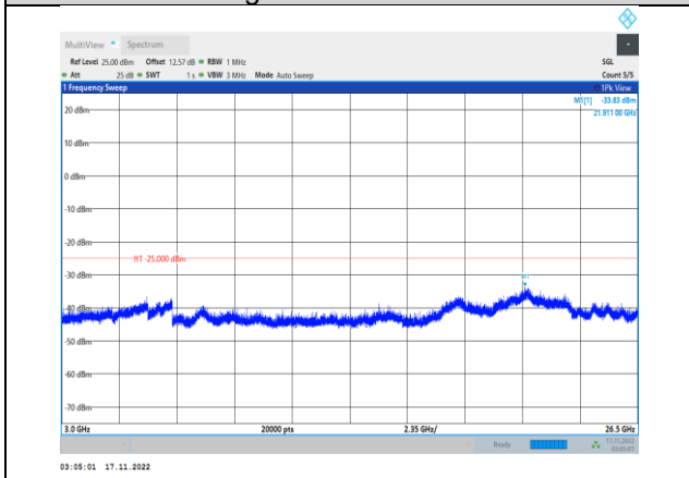
Band38-5MHz-64QAM-38225-1RB#0- Range3:3000~26500MHz
