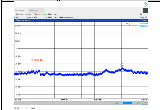
Band38-10MHz-16QAM-38200-1RB#0- Range3:3000~26500MHz
