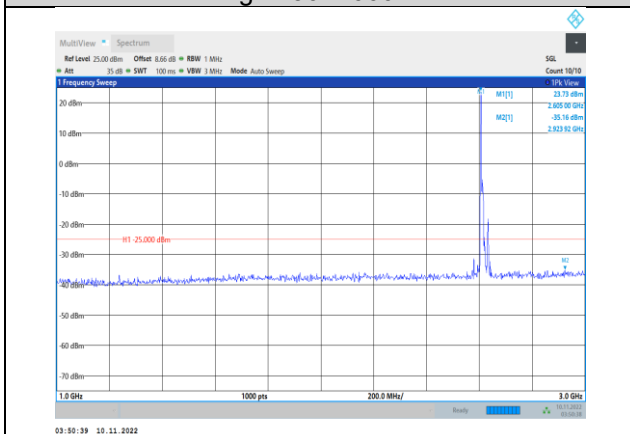
Band38-15MHz-QPSK-38175-1RB#0- Range2:1000~3000MHz
