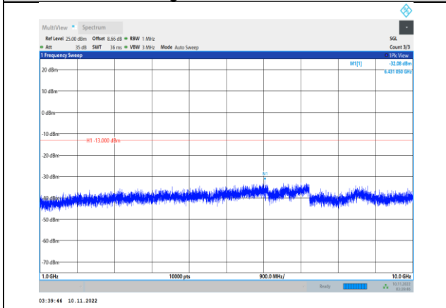
Band26-15MHz-QPSK-26965-1RB#0- Range2:1000~10000MHz
