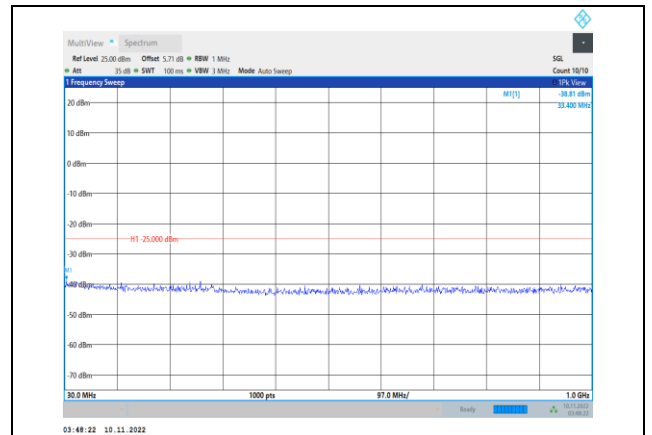
Band38-15MHz-16QAM-37825-1RB#0- Range1:30~1000MHz
