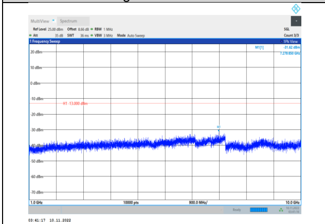
Band26-15MHz-QPSK-26765-1RB#0- Range2:1000~10000MHz
