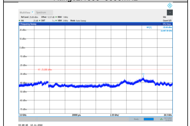
Band38-15MHz-16QAM-37825-1RB#0- Range3:3000~26500MHz
