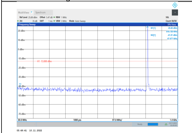
Band26-3MHz-16QAM-26740-1RB#0- Range1:30~1000MHz
