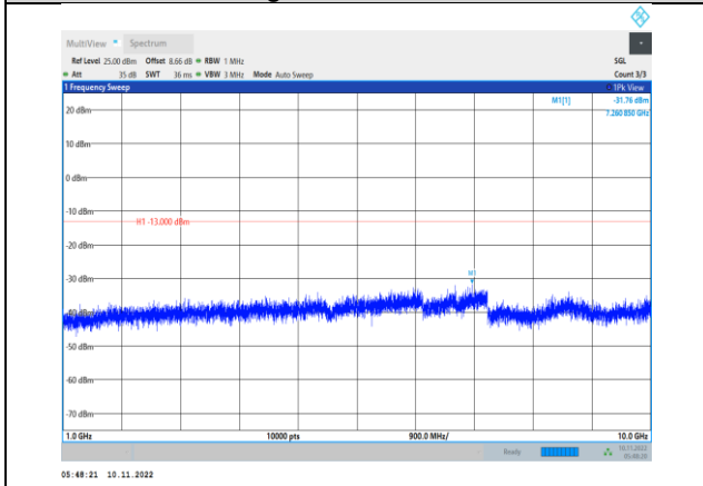
Band26-3MHz-QPSK-26705-1RB#0- Range2:1000~10000MHz
