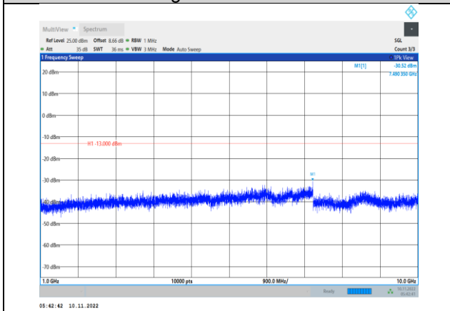
Band26-10MHz-QPSK-26740-1RB#0- Range2:1000~10000MHz
