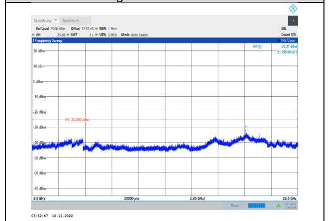
Band38-10MHz-QPSK-37800-1RB#0- Range3:3000~26500MHz
