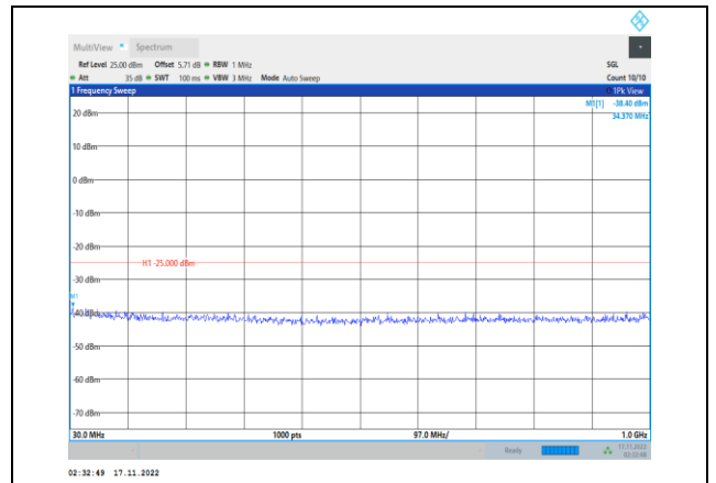
Band38-10MHz-64QAM-38200-1RB#0-Range1:30~1000MHz
