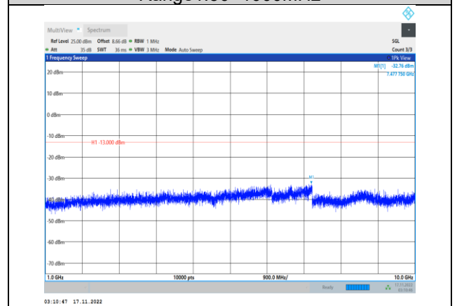
Band26-10MHz-64QAM-26740-1RB#0- Range2:1000~10000MHz
