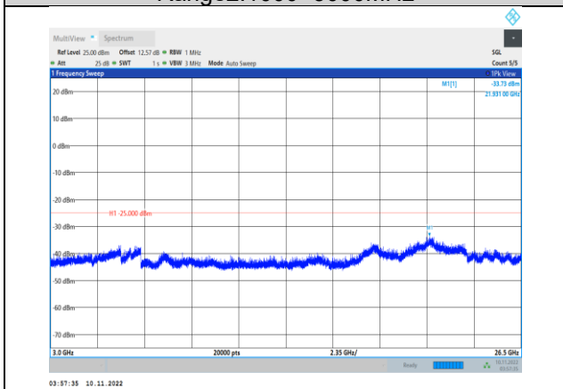
Band38-5MHz-QPSK-37775-1RB#0- Range3:3000~26500MHz
