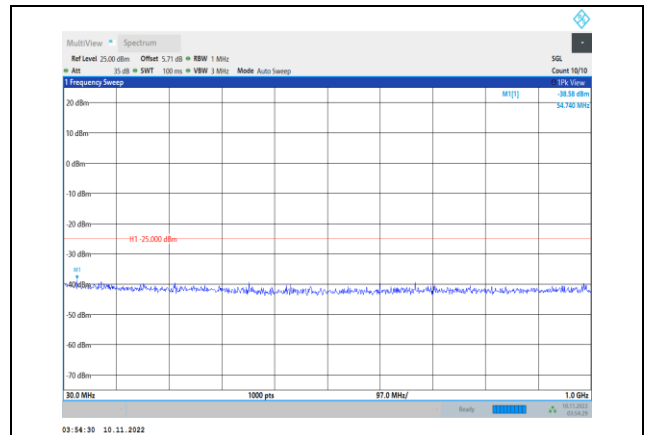
Band38-10MHz-16QAM-38000-1RB#0- Range1:30~1000MHz
