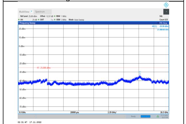
Band38-10MHz-64QAM-37800-1RB#0- Range3:3000~26500MHz
