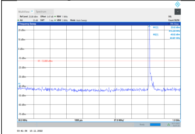
Band26-15MHz-16QAM-26765-1RB#0- Range1:30~1000MHz
