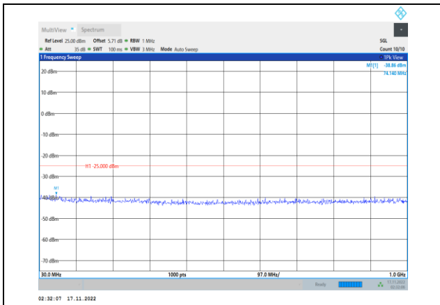
Band38-10MHz-64QAM-38000-1RB#0-Range1:30~1000MHz
