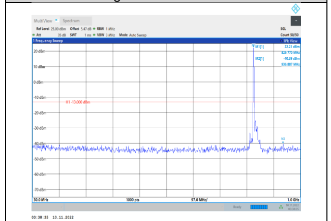
Band26-15MHz-QPSK-26915-1RB#0- Range1:30~1000MHz
