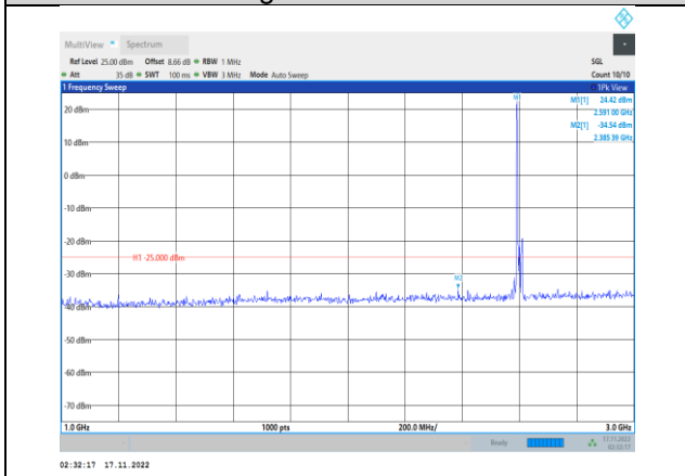
Band38-10MHz-64QAM-38000-1RB#0-Range2:1000~3000MHz
