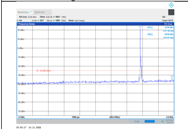
Band38-10MHz-16QAM-37800-1RB#0- Range2:1000~3000MHz
