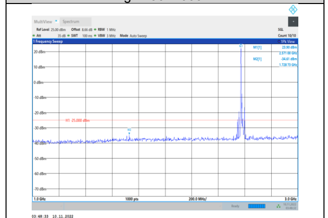
Band38-15MHz-16QAM-37825-1RB#0- Range2:1000~3000MHz
