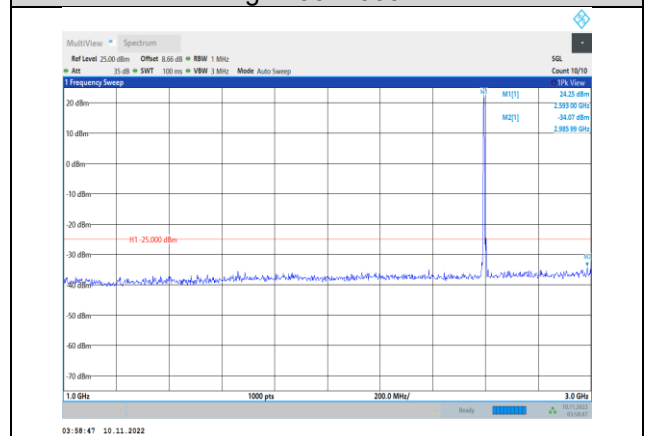
Band38-5MHz-QPSK-38000-1RB#0- Range2:1000~3000MHz
