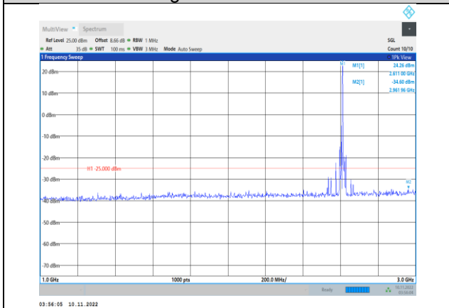
Band38-10MHz-16QAM-38200-1RB#0- Range2:1000~3000MHz
