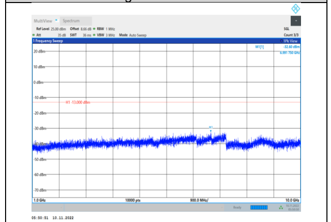
Band26-3MHz-16QAM-26775-1RB#0- Range2:1000~10000MHz
