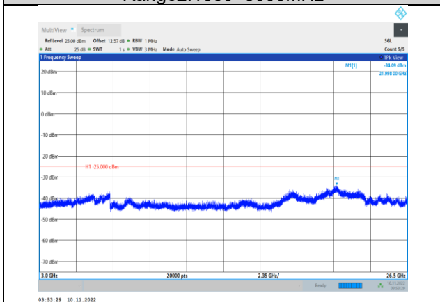
Band38-10MHz-16QAM-37800-1RB#0- Range3:3000~26500MHz
