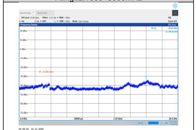
Band38-10MHz-16QAM-38000-1RB#0- Range3:3000~26500MHz
