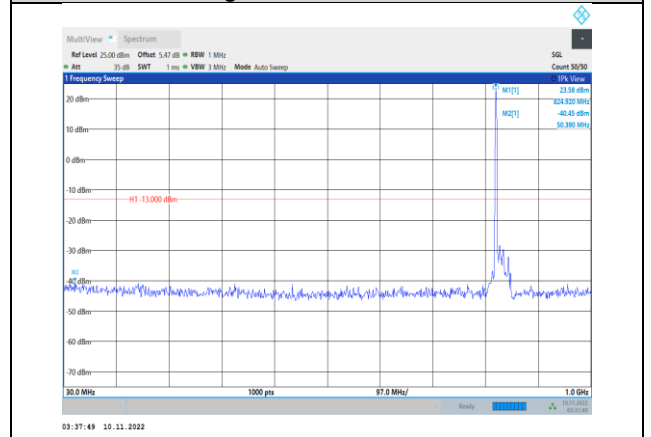
Band26-15MHz-16QAM-26865-1RB#0- Range1:30~1000MHz
