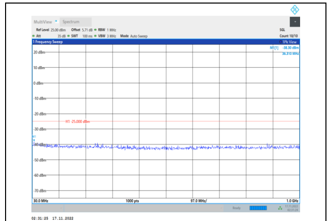
Band38-10MHz-64QAM-37800-1RB#0- Range1:30~1000MHz
