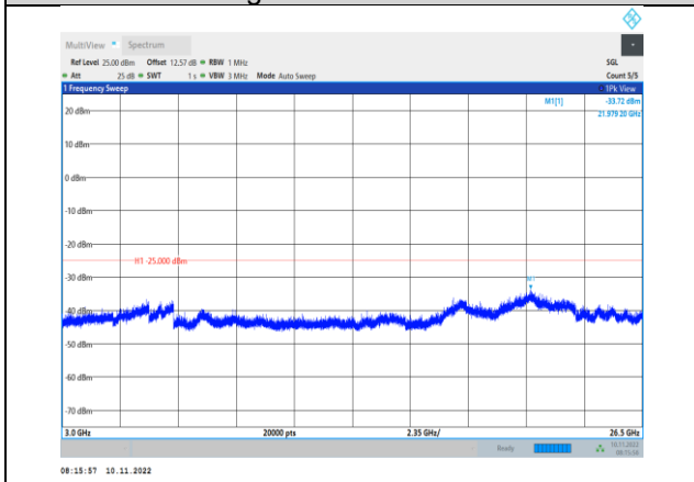
Band7-15MHz-16QAM-20825-1RB#0- Range3:3000~26500MHz
