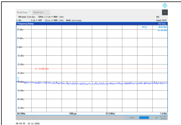
Band7-5MHz-QPSK-20775-1RB#0- Range1:30~1000MHz
