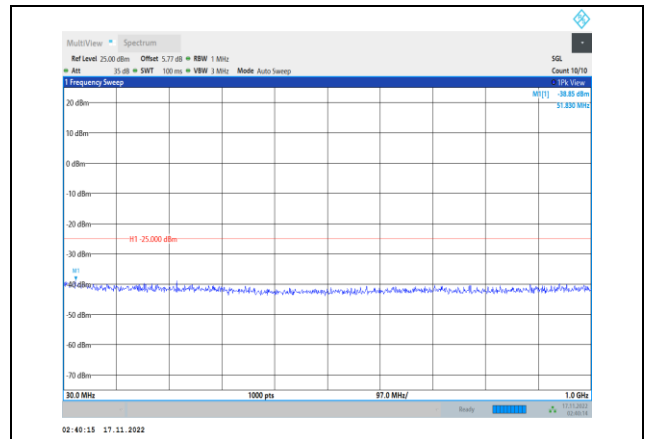
Band7-15MHz-64QAM-20825-1RB#0- Range1:30~1000MHz
