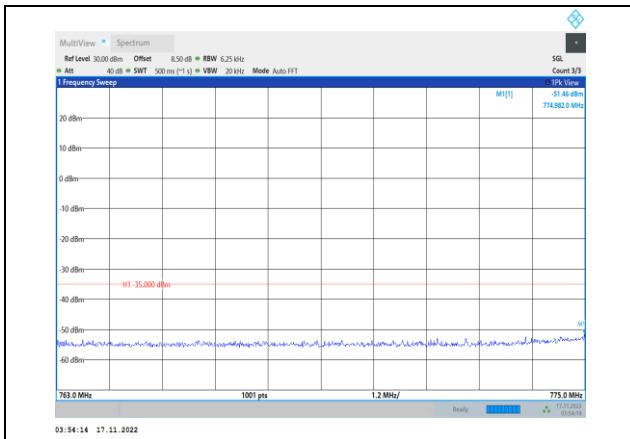
Band13-5MHz-64QAM-23230-1RB#0- Range3:763~775MHz
