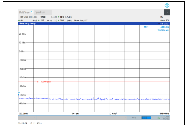
Band13-10MHz-64QAM-23230-1RB#0- Range4:793~805MHz
