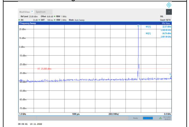
Band7-5MHz-16QAM-21425-1RB#0- Range2:1000~3000MHz
