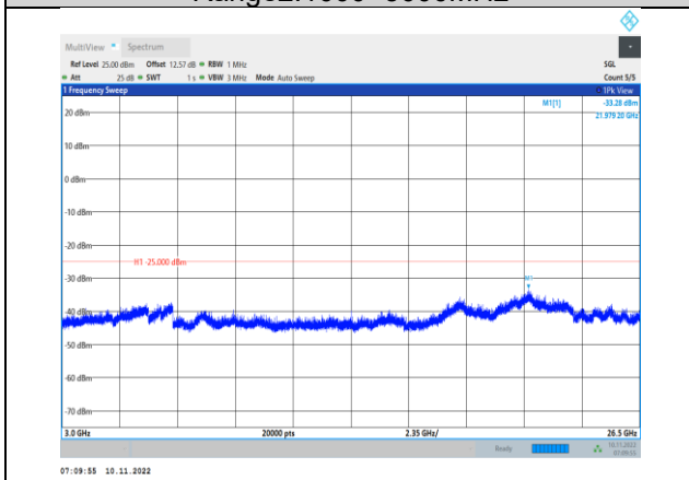
Band7-20MHz-16QAM-21100-1RB#0- Range3:3000~26500MHz
