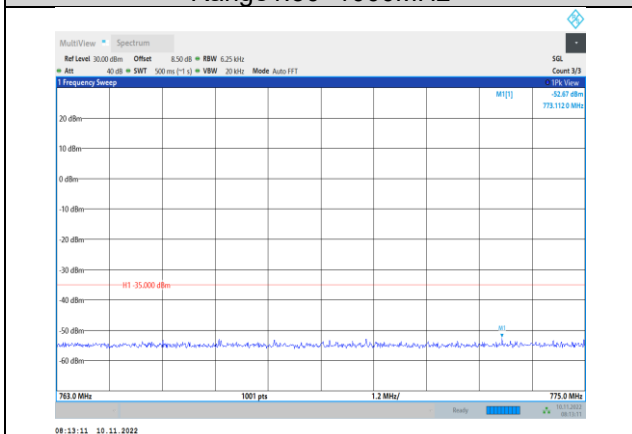
Band13-5MHz-16QAM-23255-1RB#0- Range3:763~775MHz
