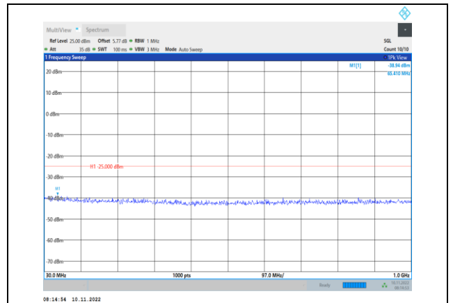
Band7-15MHz-QPSK-20825-1RB#0- Range1:30~1000MHz
