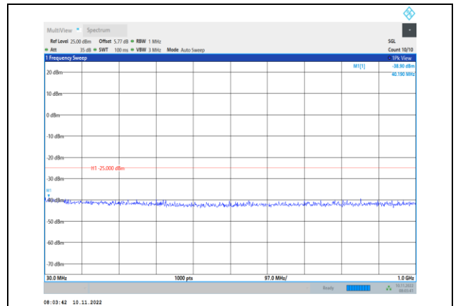
Band7-5MHz-16QAM-20775-1RB#0- Range1:30~1000MHz
