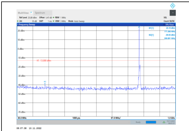
Band13-5MHz-QPSK-23205-1RB#0- Range1:30~1000MHz
