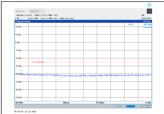
Band7-5MHz-16QAM-21100-1RB#0- Range1:30~1000MHz
