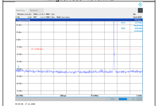
Band13-5MHz-64QAM-23230-1RB#0- Range1:30~1000MHz
