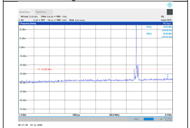
Band7-15MHz-16QAM-21100-1RB#0- Range2:1000~3000MHz
