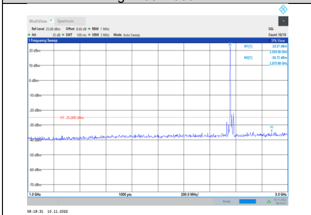
Band7-15MHz-16QAM-21375-1RB#0- Range2:1000~3000MHz
