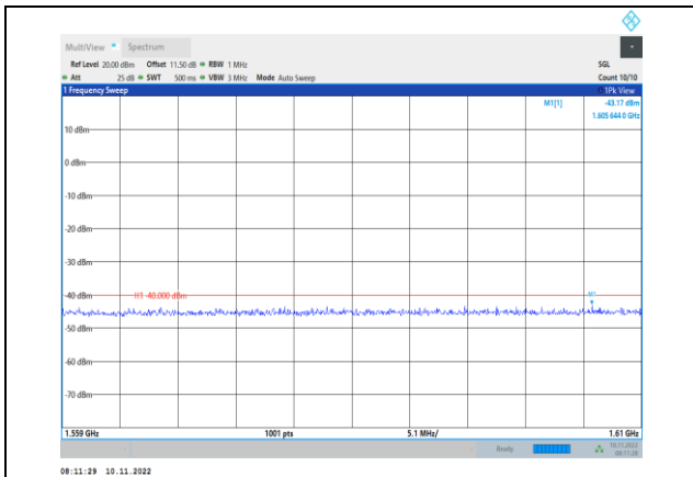
Band13-5MHz-16QAM-23230-1RB#0- Range5:1559~1610MHz
