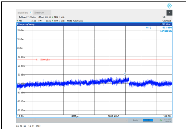
Band13-5MHz-16QAM-23205-1RB#0- Range2:1000~10000MHz
