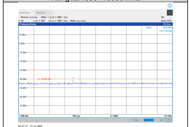
Band13-10MHz-64QAM-23230-1RB#0- Range5:1559~1610MHz
