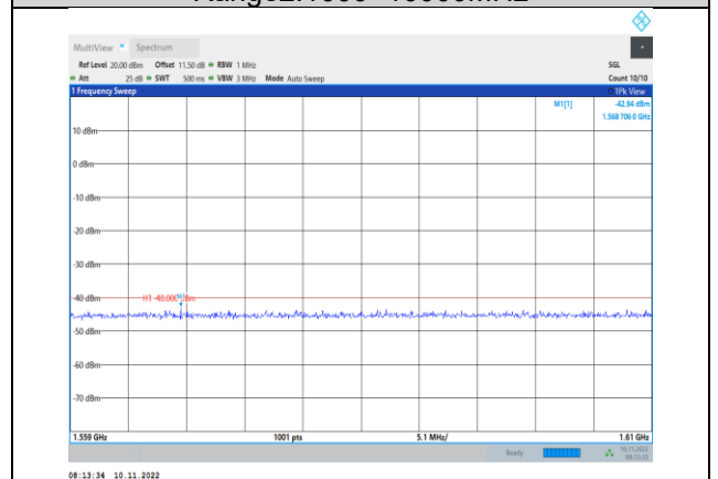
Band13-5MHz-16QAM-23255-1RB#0- Range5:1559~1610MHz
