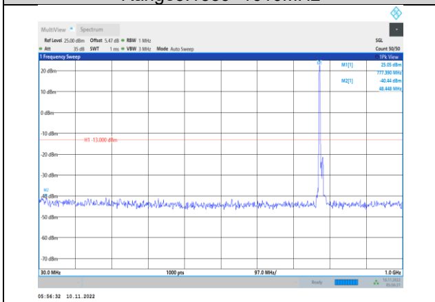
Band13-10MHz-16QAM-23230-1RB#0- Range1:30~1000MHz
