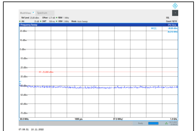
Band7-20MHz-QPSK-21100-1RB#0- Range1:30~1000MHz
