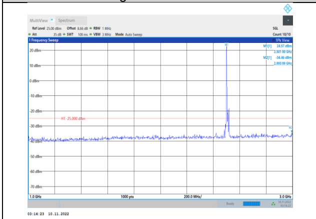
Band7-10MHz-16QAM-20800-1RB#0- Range2:1000~3000MHz
