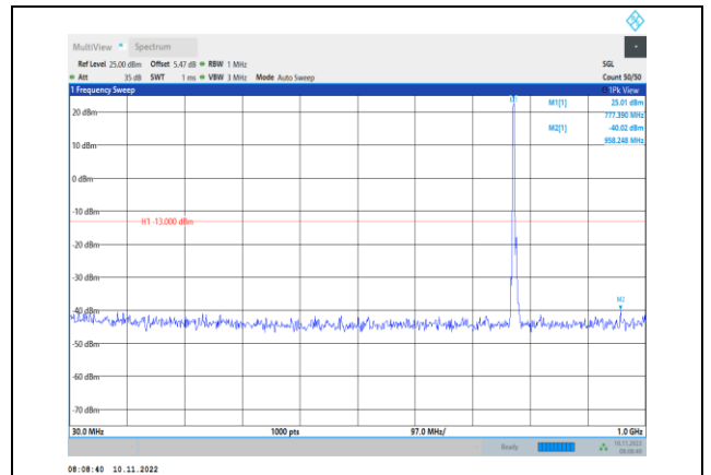
Band13-5MHz-16QAM-23205-1RB#0-Range1:30~1000MHz
