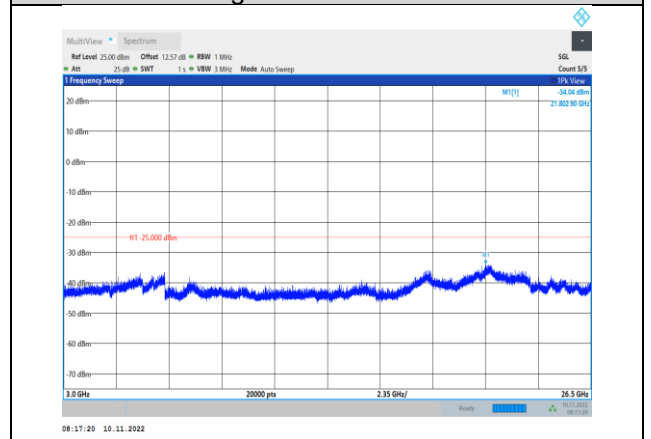
Band7-15MHz-16QAM-21100-1RB#0- Range3:3000~26500MHz
