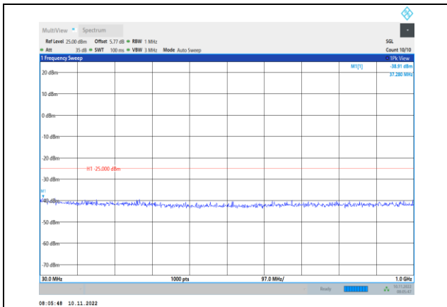
Band7-5MHz-QPSK-21425-1RB#0- Range1:30~1000MHz
