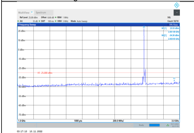
Band7-10MHz-16QAM-21400-1RB#0- Range2:1000~3000MHz
