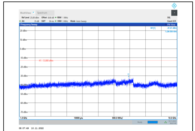
Band13-5MHz-QPSK-23205-1RB#0- Range2:1000~10000MHz
