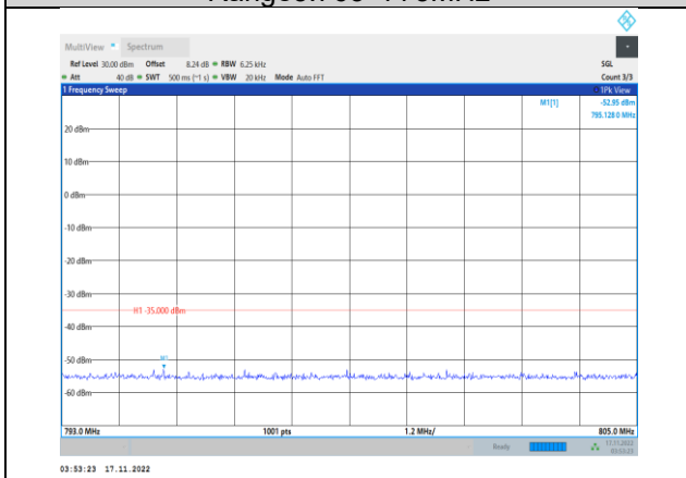
Band13-5MHz-64QAM-23205-1RB#0- Range4:793~805MHz
