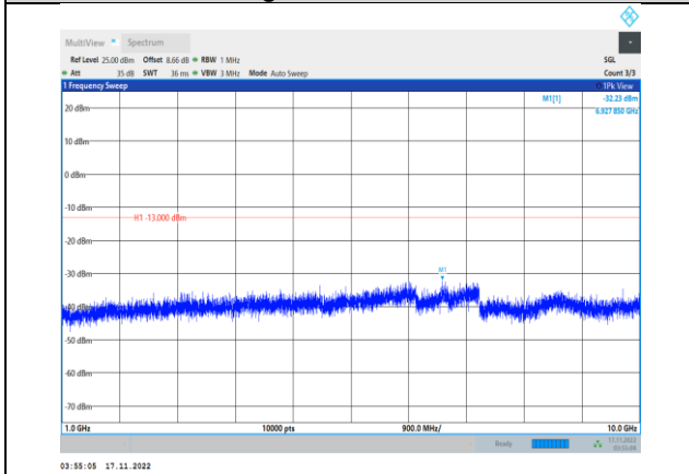
Band13-5MHz-64QAM-23255-1RB#0- Range2:1000~10000MHz
