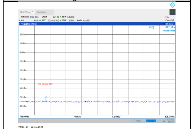
Band13-5MHz-16QAM-23230-1RB#0- Range4:793~805MHz
