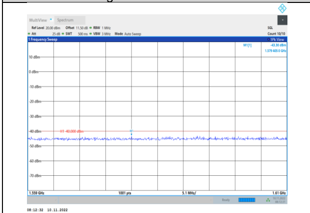
Band13-5MHz-QPSK-23255-1RB#0-Range5:1559~1610MHz
