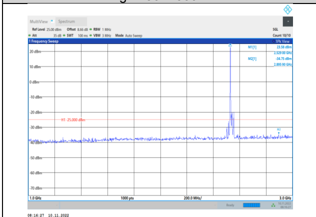
Band7-15MHz-QPSK-21100-1RB#0- Range2:1000~3000MHz
