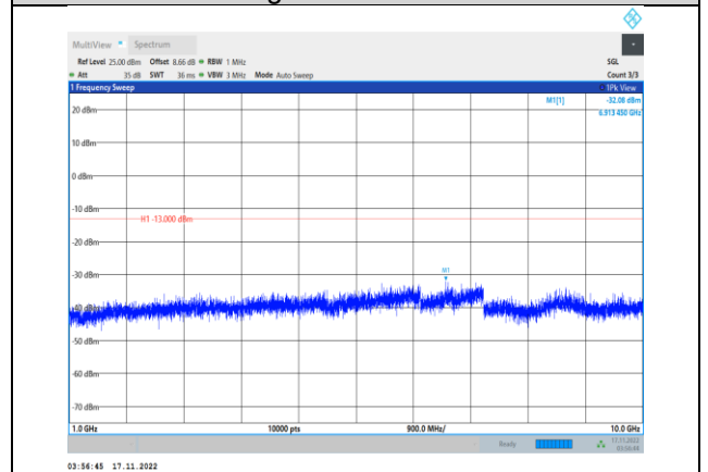
Band13-10MHz-64QAM-23230-1RB#0- Range2:1000~10000MHz
