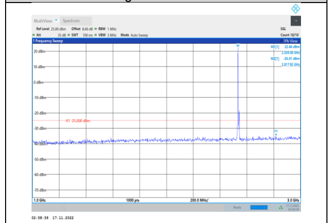
Band7-5MHz-64QAM-21100-1RB#0- Range2:1000~3000MHz
