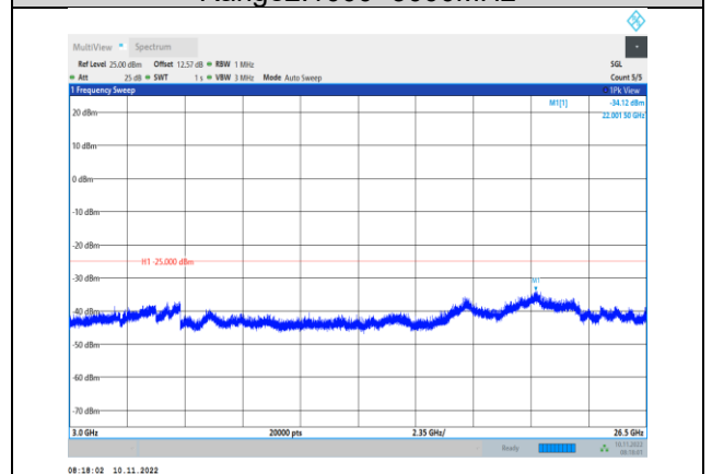
Band7-15MHz-QPSK-21375-1RB#0- Range3:3000~26500MHz
