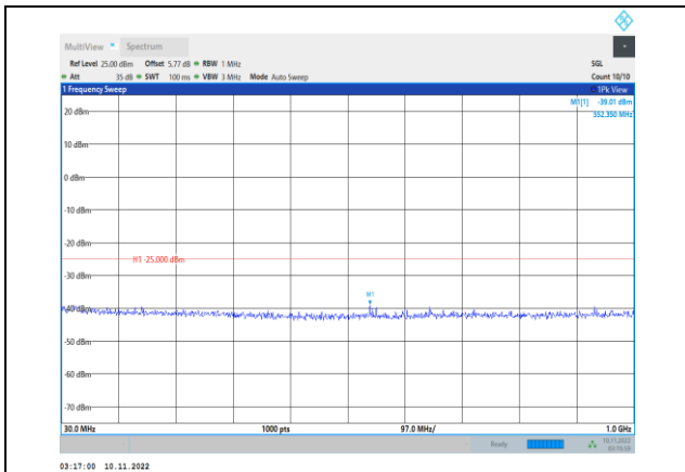
Band7-10MHz-16QAM-21400-1RB#0- Range1:30~1000MHz
