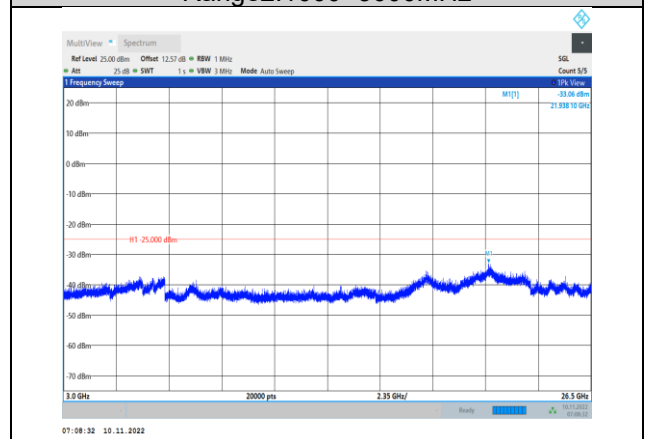
Band7-20MHz-16QAM-20850-1RB#0-Range3:3000~26500MHz
