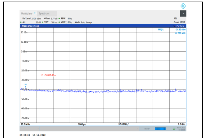
Band7-20MHz-16QAM-20850-1RB#0-Range1:30~1000MHz
