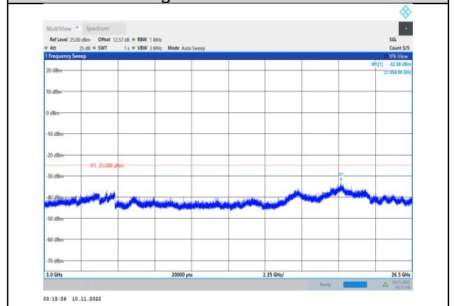
Band7-10MHz-16QAM-21100-1RB#0- Range3:3000~26500MHz
