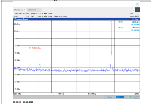
Band13-5MHz-16QAM-23230-1RB#0- Range1:30~1000MHz
