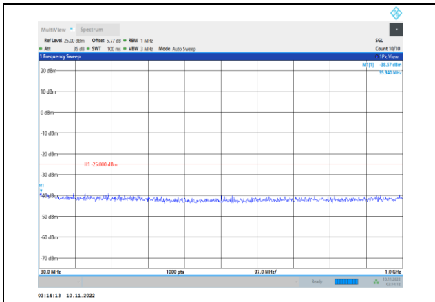
Band7-10MHz-16QAM-20800-1RB#0- Range1:30~1000MHz
