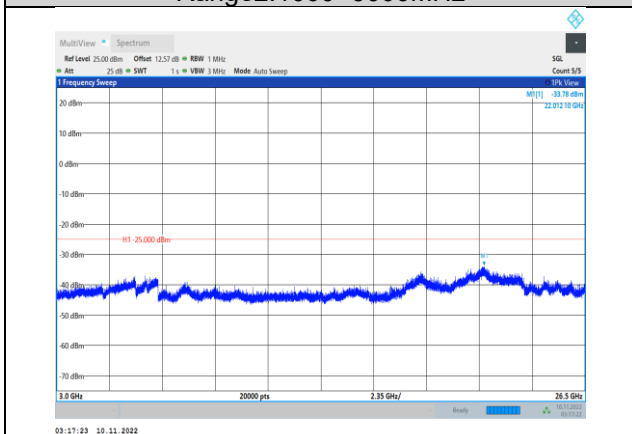
Band7-10MHz-16QAM-21400-1RB#0- Range3:3000~26500MHz
