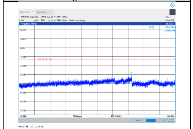
Band13-5MHz-16QAM-23230-1RB#0- Range2:1000~10000MHz
