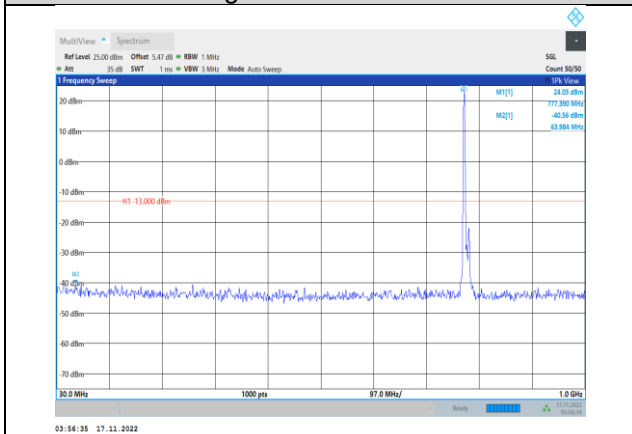
Band13-10MHz-64QAM-23230-1RB#0- Range1:30~1000MHz
