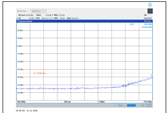
Band13-10MHz-16QAM-23230-1RB#0- Range3:763~775MHz
