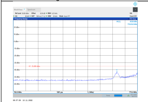
Band13-5MHz-QPSK-23205-1RB#0- Range3:763~775MHz
