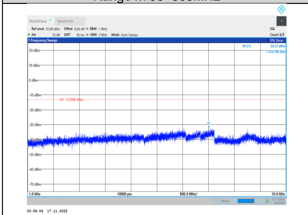
Band13-5MHz-64QAM-23230-1RB#0- Range2:1000~10000MHz
