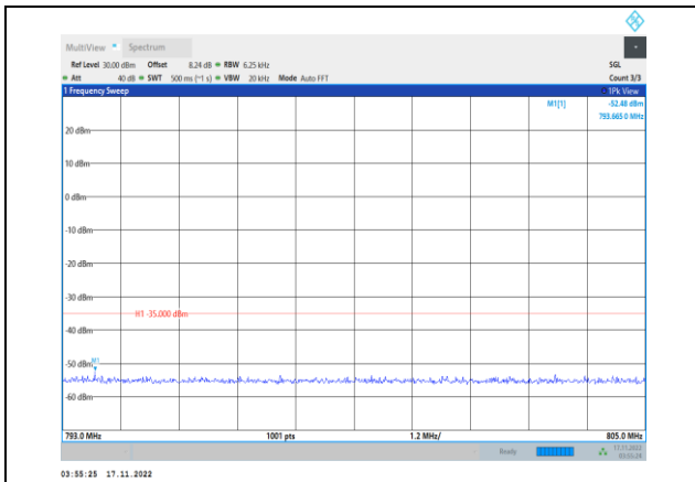
Band13-5MHz-64QAM-23255-1RB#0- Range4:793~805MHz
