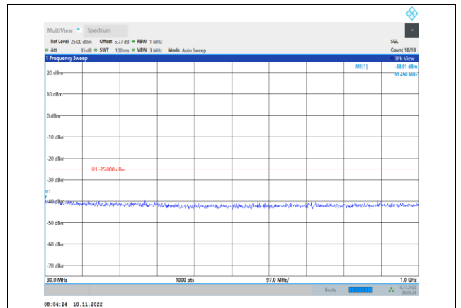
Band7-5MHz-QPSK-21100-1RB#0- Range1:30~1000MHz
