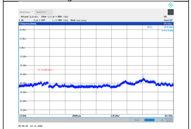
Band7-5MHz-16QAM-21425-1RB#0- Range3:3000~26500MHz
