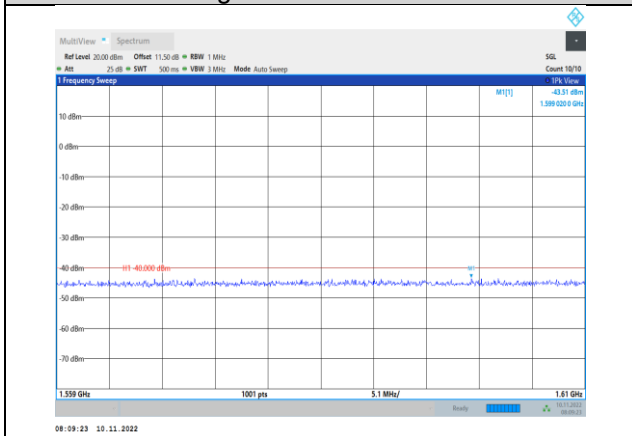
Band13-5MHz-16QAM-23205-1RB#0- Range5:1559~1610MHz
