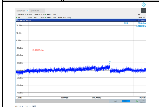
Band13-5MHz-16QAM-23255-1RB#0- Range2:1000~10000MHz
