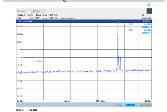
Band7-20MHz-16QAM-20850-1RB#0-Range2:1000~3000MHz
