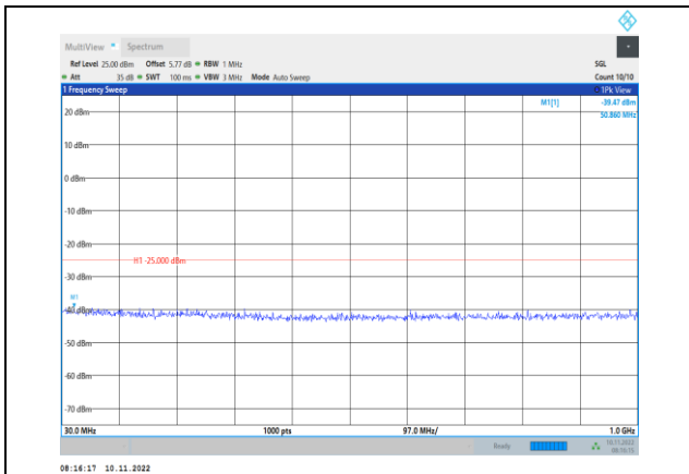
Band7-15MHz-QPSK-21100-1RB#0- Range1:30~1000MHz
