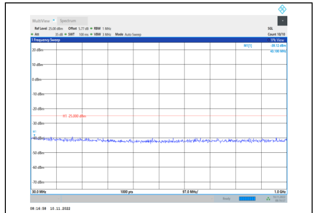
Band7-15MHz-16QAM-21100-1RB#0- Range1:30~1000MHz
