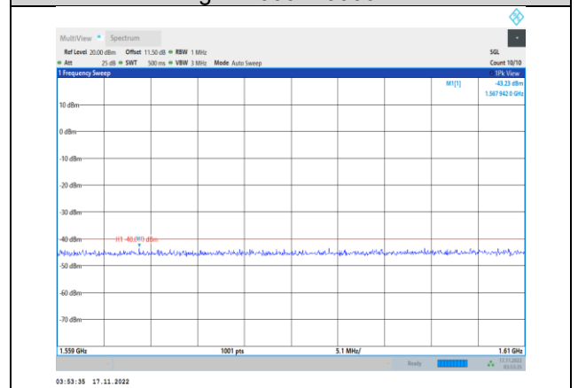
Band13-5MHz-64QAM-23205-1RB#0- Range5:1559~1610MHz
