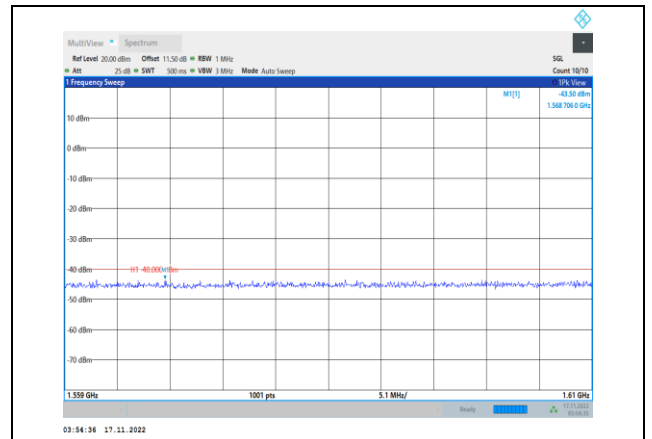
Band13-5MHz-64QAM-23230-1RB#0- Range5:1559~1610MHz
