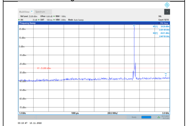
Band7-10MHz-16QAM-21100-1RB#0- Range2:1000~3000MHz
