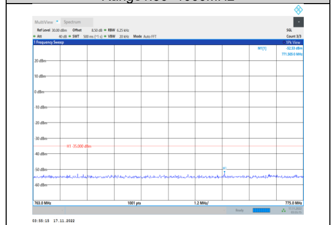
Band13-5MHz-64QAM-23255-1RB#0- Range3:763~775MHz
