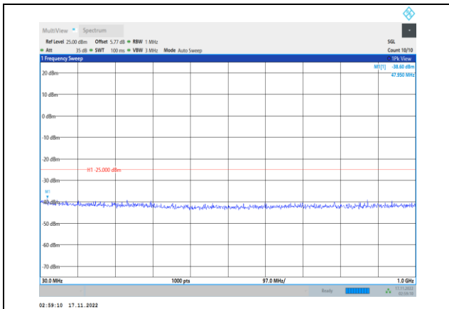
Band7-5MHz-64QAM-21425-1RB#0- Range1:30~1000MHz
