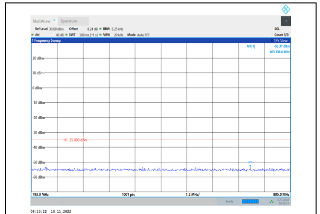
Band13-5MHz-16QAM-23255-1RB#0- Range4:793~805MHz
