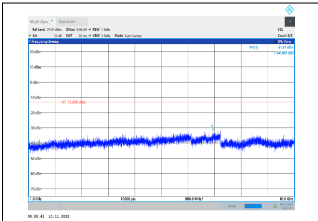
Band13-10MHz-QPSK-23230-1RB#0- Range2:1000~10000MHz
