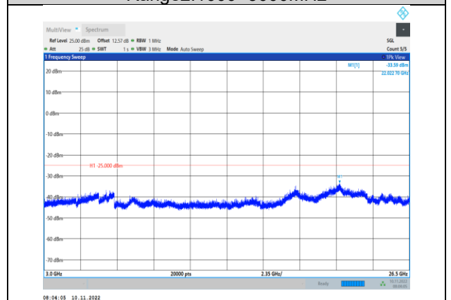
Band7-5MHz-16QAM-20775-1RB#0- Range3:3000~26500MHz
