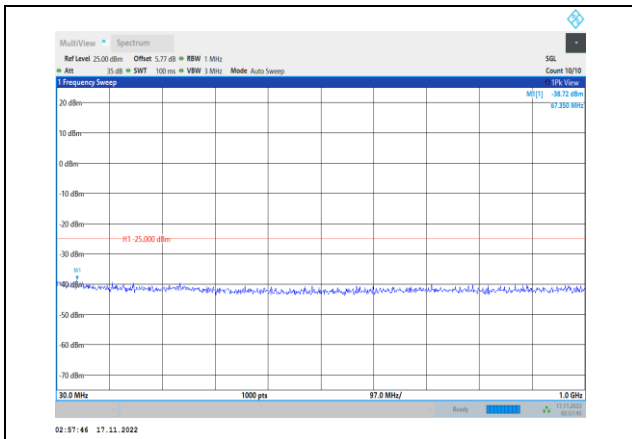
Band7-5MHz-64QAM-20775-1RB#0- Range1:30~1000MHz
