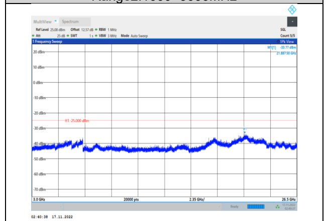
Band7-15MHz-64QAM-20825-1RB#0- Range3:3000~26500MHz
