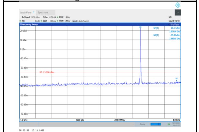
Band7-5MHz-16QAM-20775-1RB#0- Range2:1000~3000MHz
