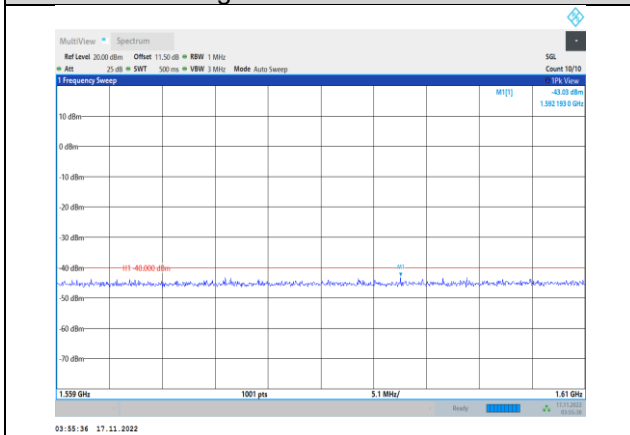
Band13-5MHz-64QAM-23255-1RB#0- Range5:1559~1610MHz
