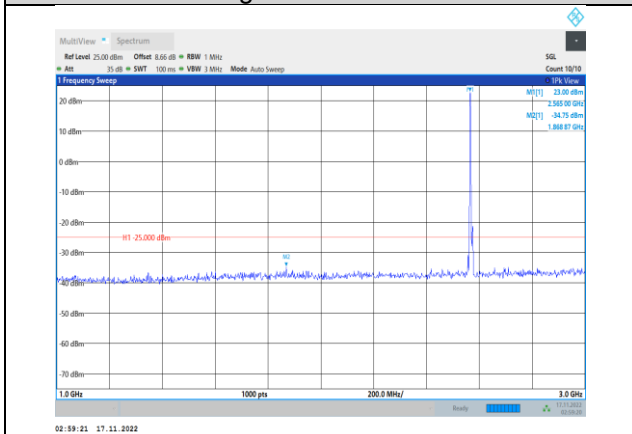
Band7-5MHz-64QAM-21425-1RB#0- Range2:1000~3000MHz
