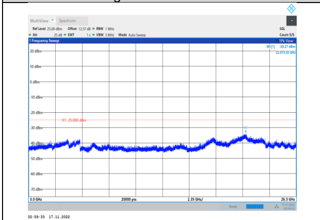
Band7-5MHz-64QAM-21425-1RB#0- Range3:3000~26500MHz
