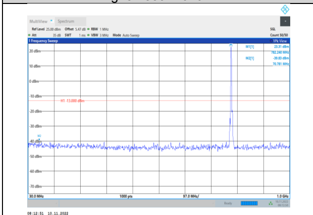
Band13-5MHz-16QAM-23255-1RB#0- Range1:30~1000MHz
