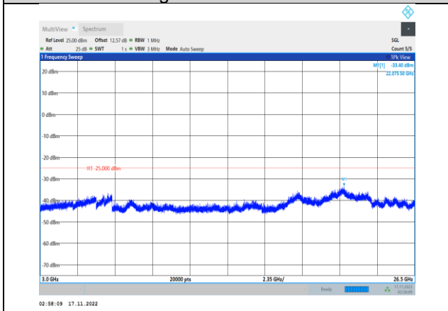
Band7-5MHz-64QAM-20775-1RB#0- Range3:3000~26500MHz
