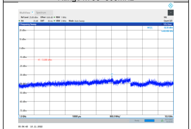
Band13-10MHz-16QAM-23230-1RB#0- Range2:1000~10000MHz
