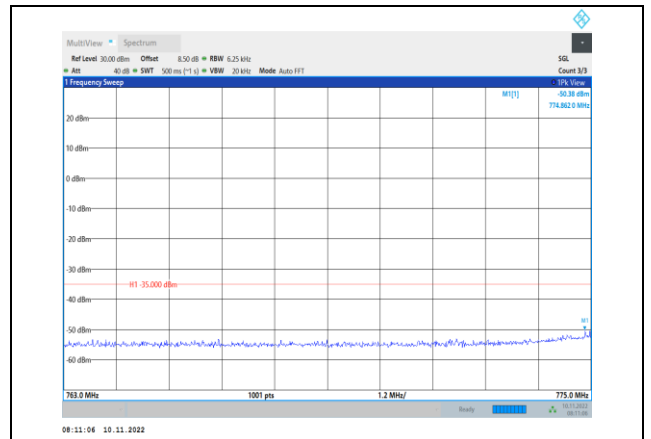
Band13-5MHz-16QAM-23230-1RB#0- Range3:763~775MHz
