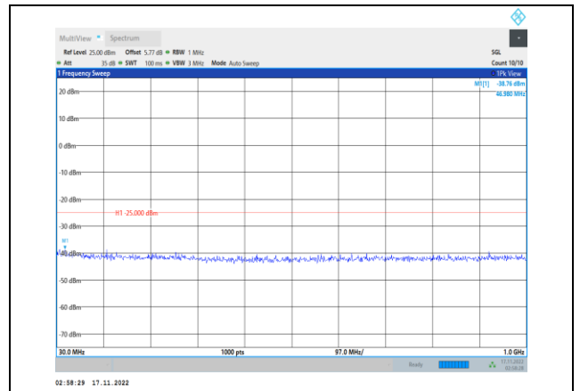
Band7-5MHz-64QAM-21100-1RB#0- Range1:30~1000MHz
