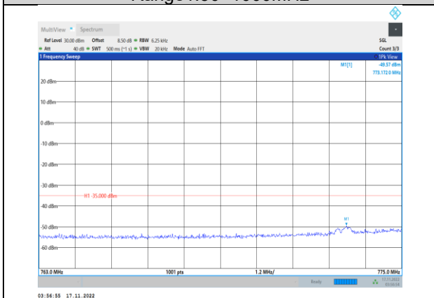
Band13-10MHz-64QAM-23230-1RB#0- Range3:763~775MHz
