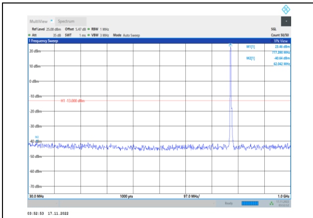
Band13-5MHz-64QAM-23205-1RB#0- Range1:30~1000MHz
