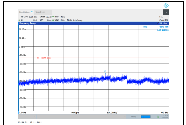
Band13-5MHz-64QAM-23205-1RB#0- Range2:1000~10000MHz
