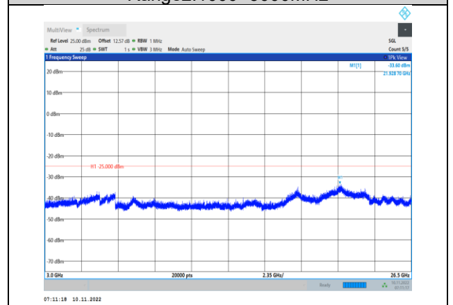
Band7-20MHz-16QAM-21350-1RB#0- Range3:3000~26500MHz
