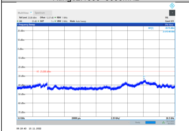
Band7-15MHz-16QAM-21375-1RB#0- Range3:3000~26500MHz
