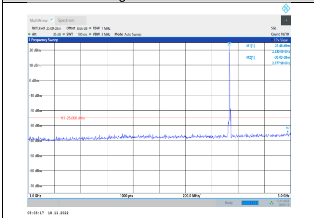
Band7-5MHz-16QAM-21100-1RB#0- Range2:1000~3000MHz
