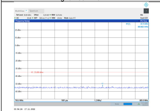
Band13-5MHz-64QAM-23230-1RB#0- Range4:793~805MHz
