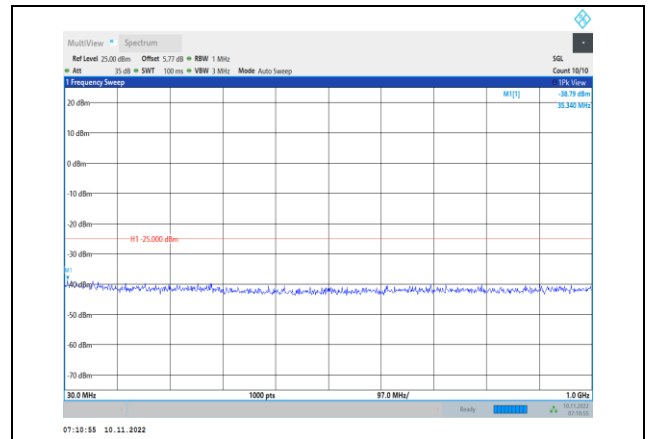
Band7-20MHz-16QAM-21350-1RB#0- Range1:30~1000MHz
