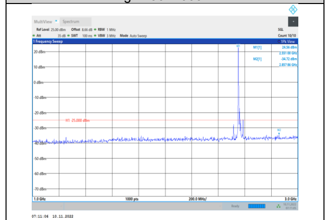
Band7-20MHz-16QAM-21350-1RB#0- Range2:1000~3000MHz
