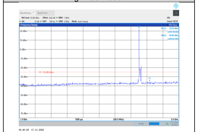
Band7-15MHz-64QAM-20825-1RB#0- Range2:1000~3000MHz
