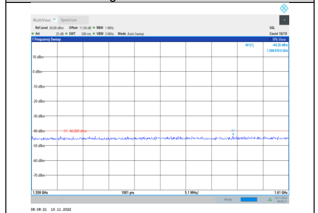
Band13-5MHz-QPSK-23205-1RB#0- Range5:1559~1610MHz
