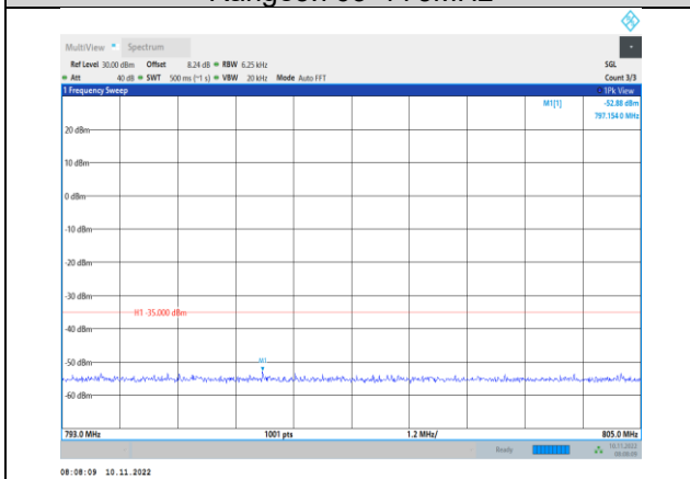
Band13-5MHz-QPSK-23205-1RB#0- Range4:793~805MHz
