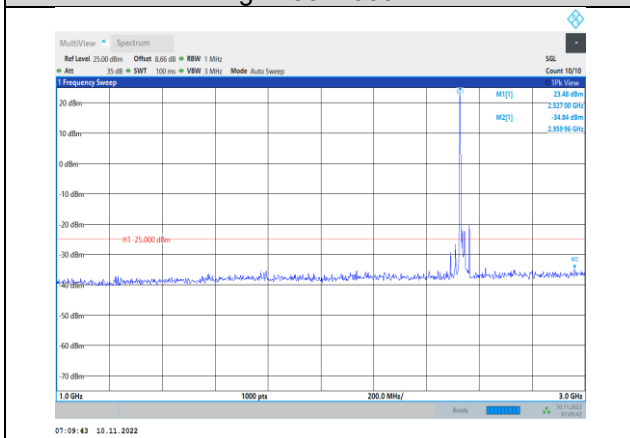
Band7-20MHz-16QAM-21100-1RB#0- Range2:1000~3000MHz
