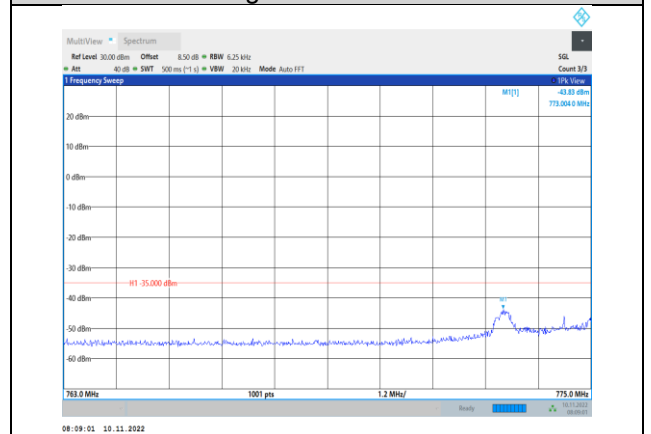
Band13-5MHz-16QAM-23205-1RB#0-Range3:763~775MHz
