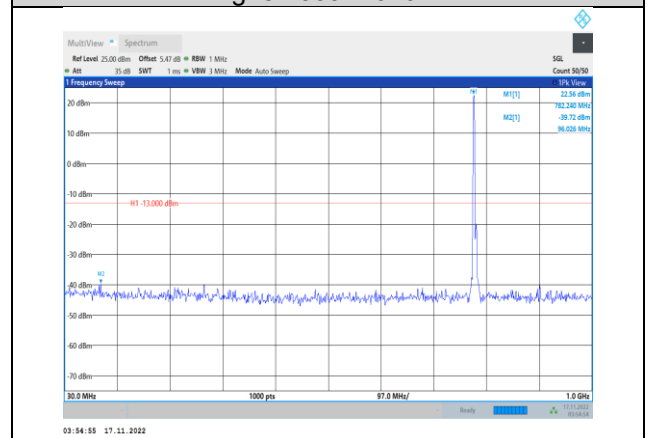
Band13-5MHz-64QAM-23255-1RB#0- Range1:30~1000MHz
