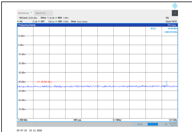
Band13-10MHz-16QAM-23230-1RB#0- Range5:1559~1610MHz
