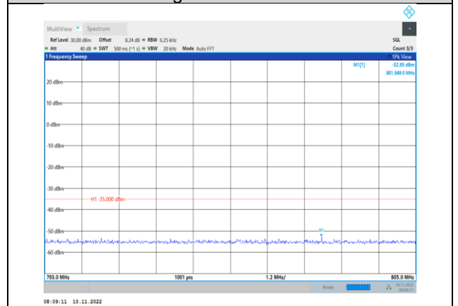
Band13-5MHz-16QAM-23205-1RB#0-Range4:793~805MHz
