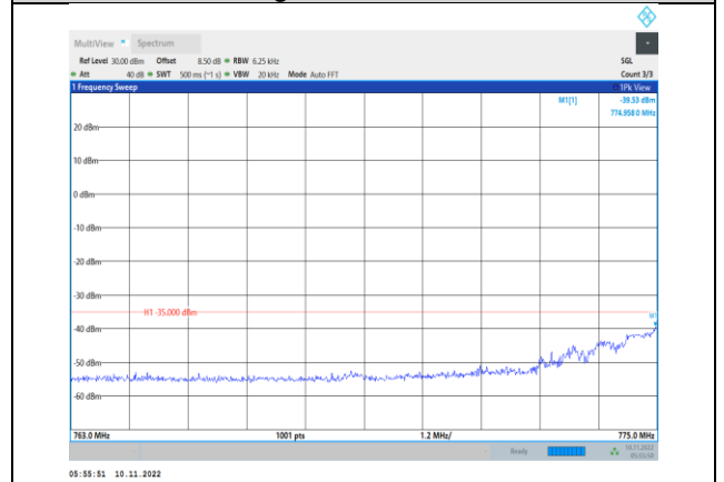
Band13-10MHz-QPSK-23230-1RB#0- Range3:763~775MHz
