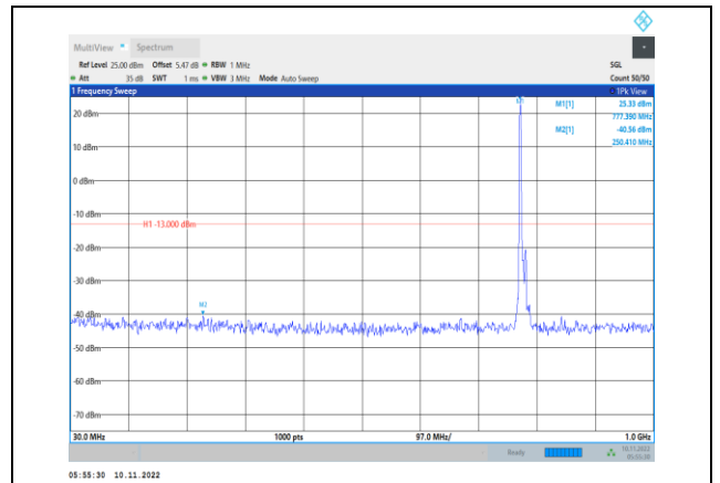
Band13-10MHz-QPSK-23230-1RB#0- Range1:30~1000MHz
