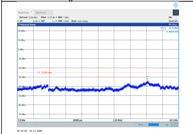
Band7-10MHz-16QAM-20800-1RB#0- Range3:3000~26500MHz
