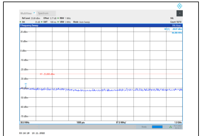
Band7-10MHz-QPSK-21400-1RB#0- Range1:30~1000MHz
