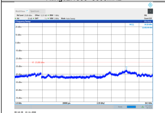
Band7-15MHz-QPSK-21100-1RB#0- Range3:3000~26500MHz
