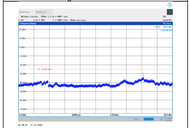
Band7-5MHz-64QAM-21100-1RB#0- Range3:3000~26500MHz
