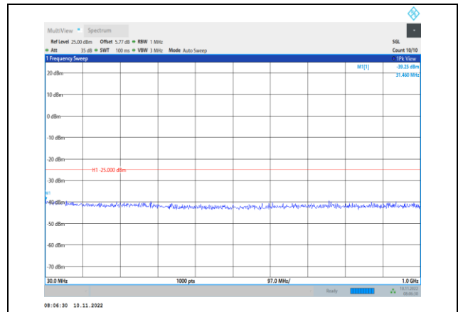
Band7-5MHz-16QAM-21425-1RB#0- Range1:30~1000MHz
