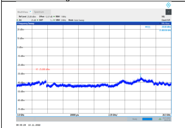
Band7-5MHz-16QAM-21100-1RB#0- Range3:3000~26500MHz
