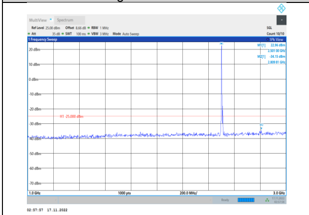
Band7-5MHz-64QAM-20775-1RB#0- Range2:1000~3000MHz
