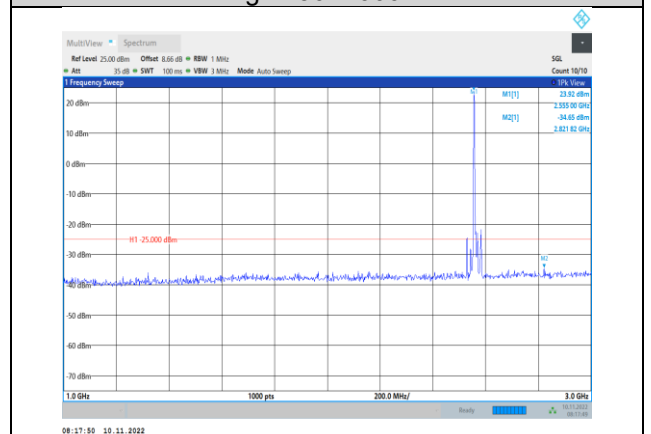
Band7-15MHz-QPSK-21375-1RB#0- Range2:1000~3000MHz
