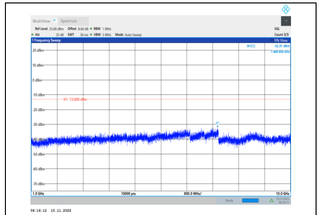
Band5-1.4MHz-16QAM-20525-1RB#0- Range2:1000~10000MHz
