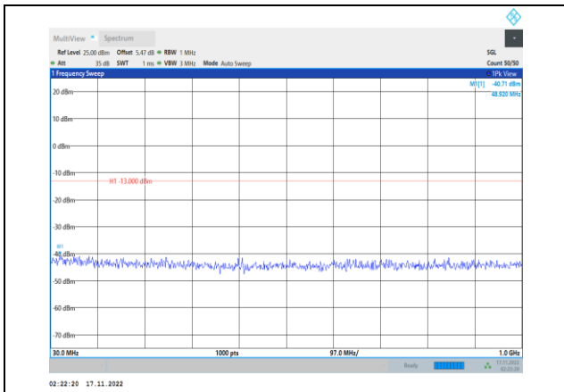
Band4-5MHz-64QAM-19975-1RB#0- Range1:30~1000MHz
