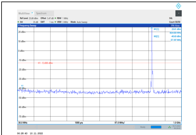
Band5-3MHz-16QAM-20415-1RB#0- Range1:30~1000MHz
