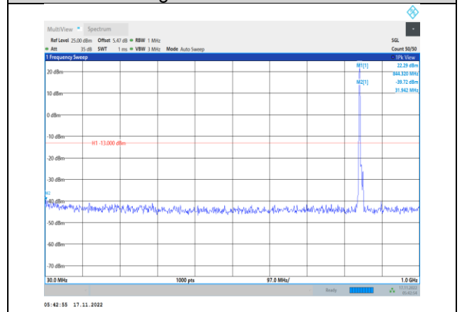
Band5-5MHz-64QAM-20625-1RB#0- Range1:30~1000MHz
