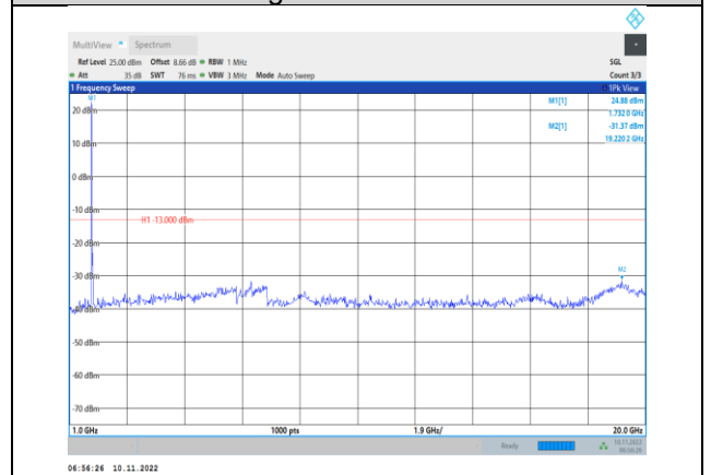
Band4-20MHz-16QAM-20300-1RB#0- Range2:1000~20000MHz
