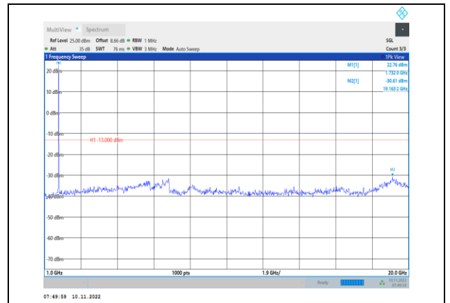
Band4-10MHz-16QAM-20175-1RB#0- Range2:1000~20000MHz
