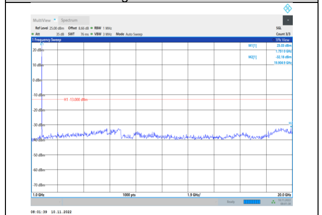
Band4-5MHz-16QAM-20375-1RB#0- Range2:1000~20000MHz
