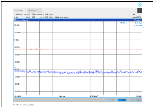
Band4-10MHz-16QAM-20000-1RB#0- Range1:30~1000MHz
