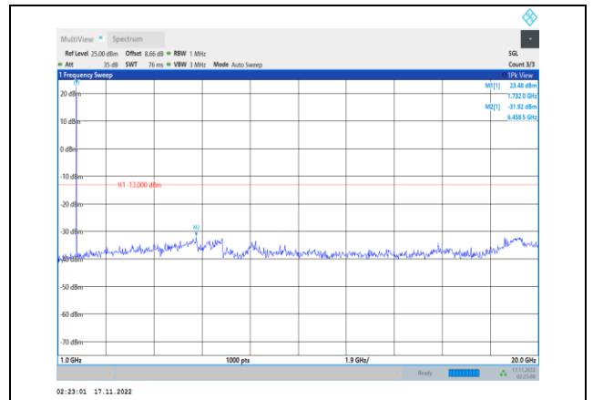
Band4-5MHz-64QAM-20175-1RB#0- Range2:1000~20000MHz
