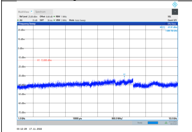
Band5-3MHz-64QAM-20415-1RB#0- Range2:1000~10000MHz
