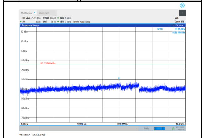
Band5-5MHz-16QAM-20625-1RB#0- Range2:1000~10000MHz
