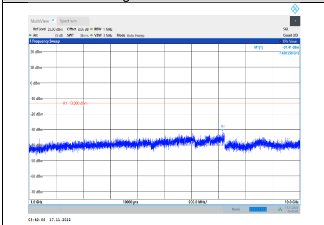
Band5-5MHz-64QAM-20425-1RB#0- Range2:1000~10000MHz
