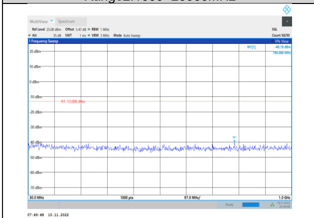
Band4-10MHz-16QAM-20175-1RB#0- Range1:30~1000MHz
