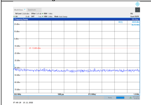
Band4-10MHz-QPSK-20175-1RB#0-Range1:30~1000MHz
