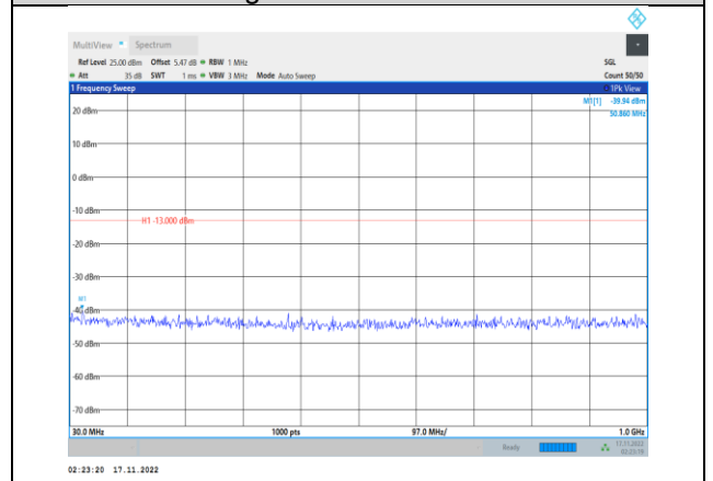
Band4-5MHz-64QAM-20375-1RB#0- Range1:30~1000MHz
