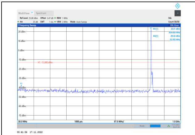
Band5-5MHz-64QAM-20425-1RB#0- Range1:30~1000MHz
