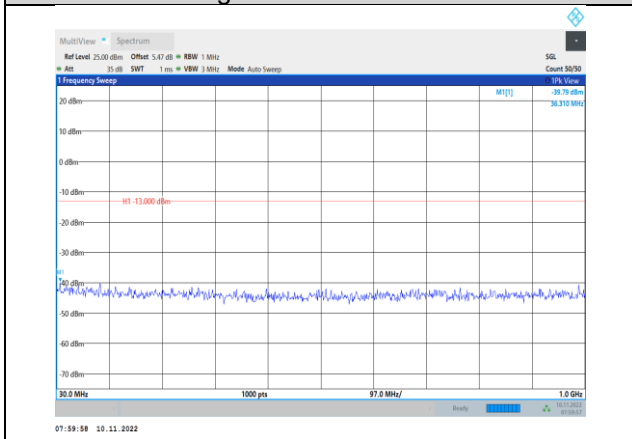
Band4-5MHz-QPSK-20175-1RB#0- Range1:30~1000MHz
