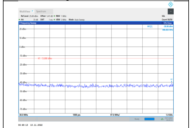
Band4-15MHz-QPSK-20325-1RB#0-Range1:30~1000MHz
