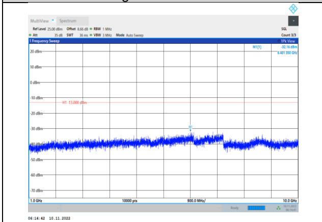
Band5-1.4MHz-QPSK-20407-1RB#0- Range2:1000~10000MHz
