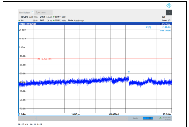
Band5-10MHz-16QAM-20525-1RB#0- Range2:1000~10000MHz
