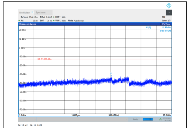
Band5-1.4MHz-QPSK-20525-1RB#0- Range2:1000~10000MHz
