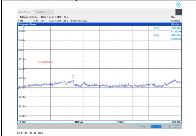
Band4-15MHz-16QAM-20025-1RB#0- Range2:1000~20000MHz
