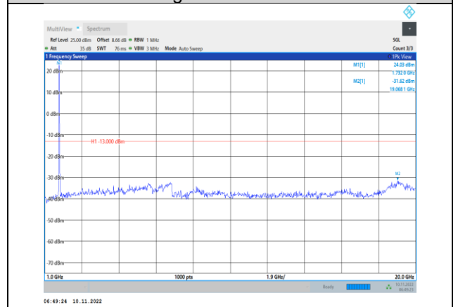
Band4-15MHz-QPSK-20325-1RB#0-Range2:1000~20000MHz
