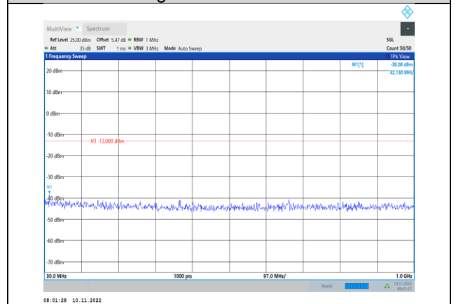
Band4-5MHz-16QAM-20375-1RB#0- Range1:30~1000MHz
