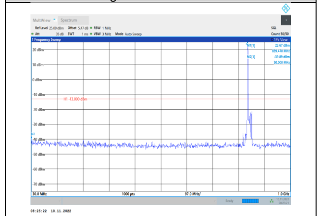
Band5-10MHz-QPSK-20600-1RB#0-Range1:30~1000MHz
