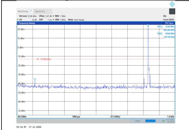
Band5-3MHz-64QAM-20525-1RB#0- Range1:30~1000MHz
