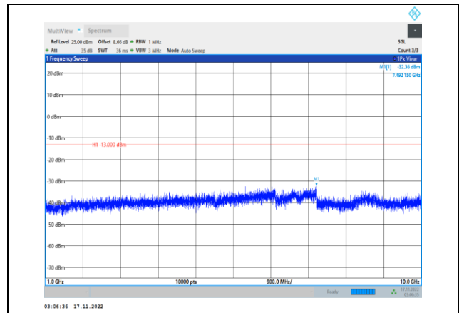
Band5-10MHz-64QAM-20525-1RB#0- Range2:1000~10000MHz
