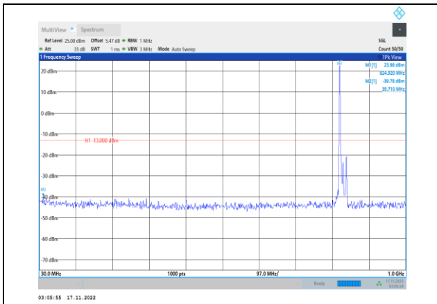
Band5-10MHz-64QAM-20450-1RB#0- Range1:30~1000MHz
