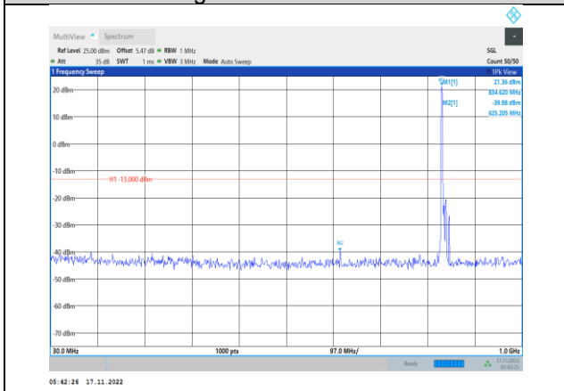
Band5-5MHz-64QAM-20525-1RB#0- Range1:30~1000MHz
