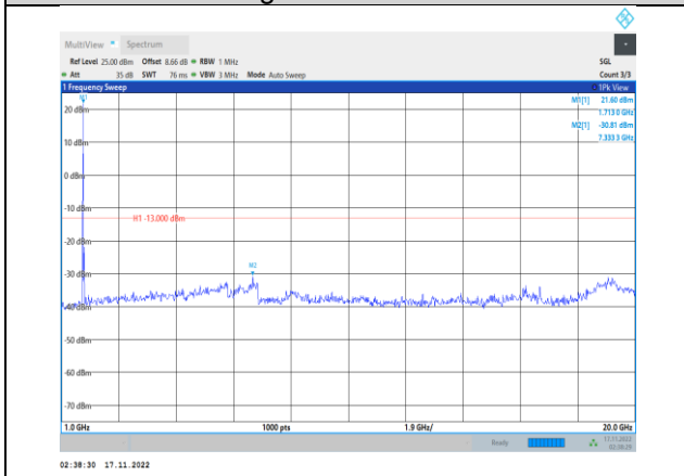
Band4-20MHz-64QAM-20050-1RB#0- Range2:1000~20000MHz
