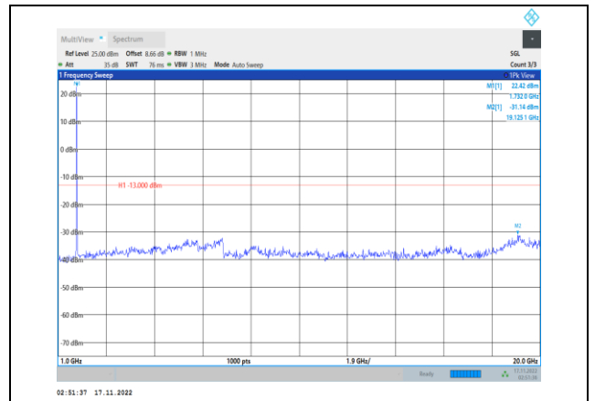
Band4-10MHz-64QAM-20175-1RB#0- Range2:1000~20000MHz
