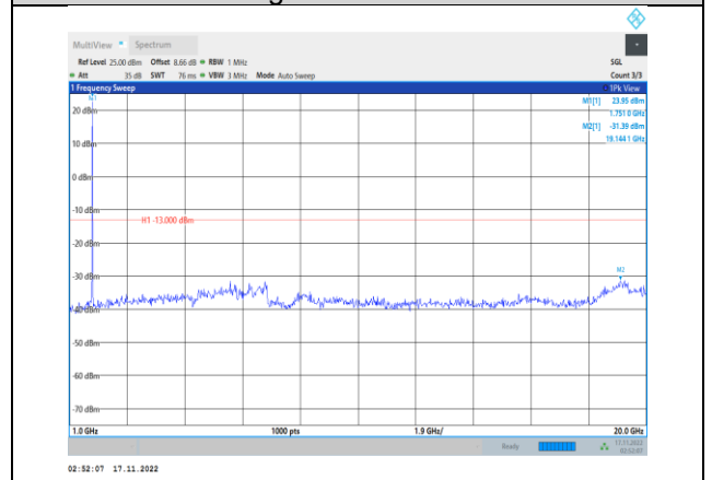
Band4-10MHz-64QAM-20350-1RB#0- Range2:1000~20000MHz
