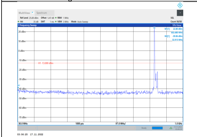
Band5-10MHz-64QAM-20525-1RB#0- Range1:30~1000MHz
