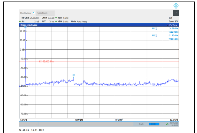
Band4-15MHz-QPSK-20175-1RB#0-Range2:1000~20000MHz
