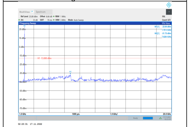
Band4-5MHz-64QAM-20375-1RB#0- Range2:1000~20000MHz
