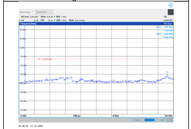
Band4-20MHz-64QAM-20300-1RB#0- Range2:1000~20000MHz
