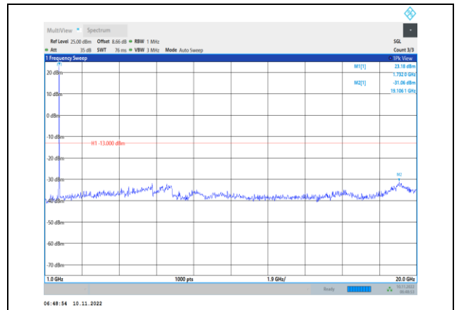
Band4-15MHz-16QAM-20175-1RB#0- Range2:1000~20000MHz
