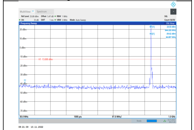
Band5-5MHz-QPSK-20625-1RB#0- Range1:30~1000MHz
