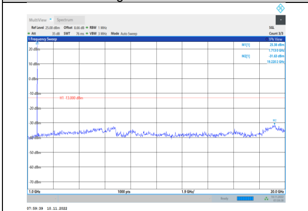
Band4-5MHz-16QAM-19975-1RB#0- Range2:1000~20000MHz
