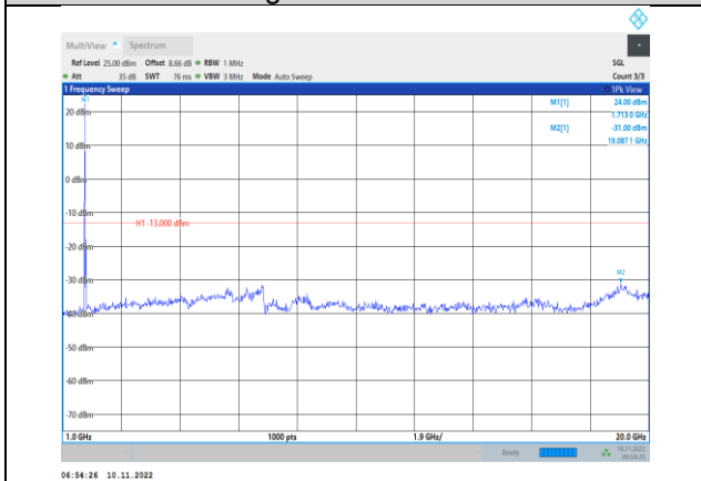
Band4-20MHz-16QAM-20050-1RB#0- Range2:1000~20000MHz
