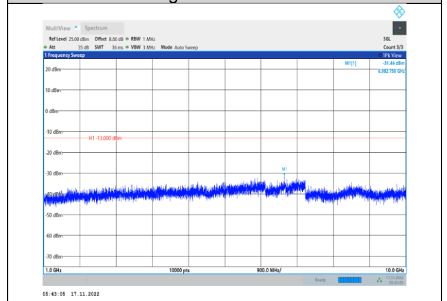
Band5-5MHz-64QAM-20625-1RB#0- Range2:1000~10000MHz
