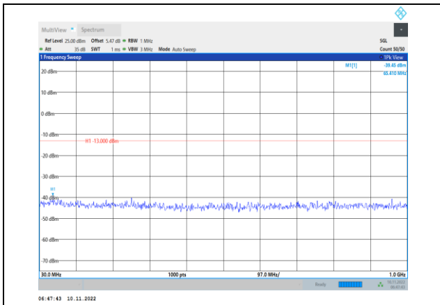
Band4-15MHz-16QAM-20025-1RB#0- Range1:30~1000MHz
