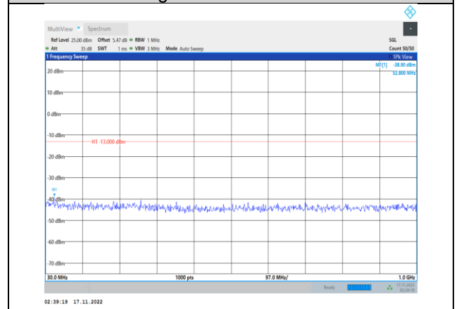
Band4-20MHz-64QAM-20300-1RB#0- Range1:30~1000MHz
