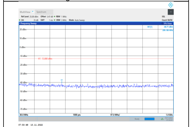
Band4-10MHz-16QAM-20350-1RB#0- Range1:30~1000MHz
