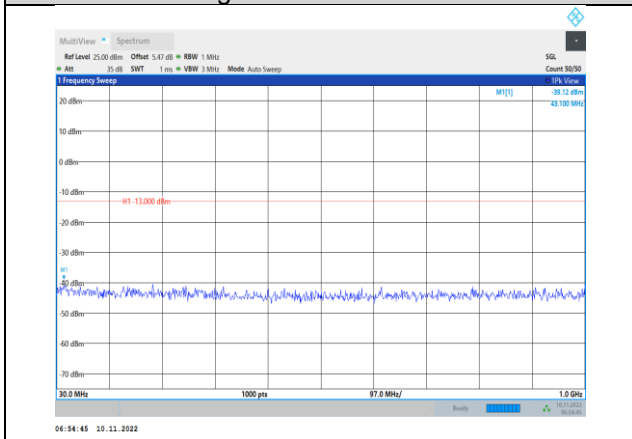
Band4-20MHz-QPSK-20175-1RB#0- Range1:30~1000MHz
