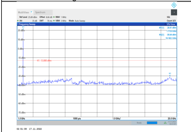
Band4-10MHz-64QAM-20000-1RB#0- Range2:1000~20000MHz
