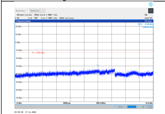
Band5-10MHz-64QAM-20450-1RB#0- Range2:1000~10000MHz
