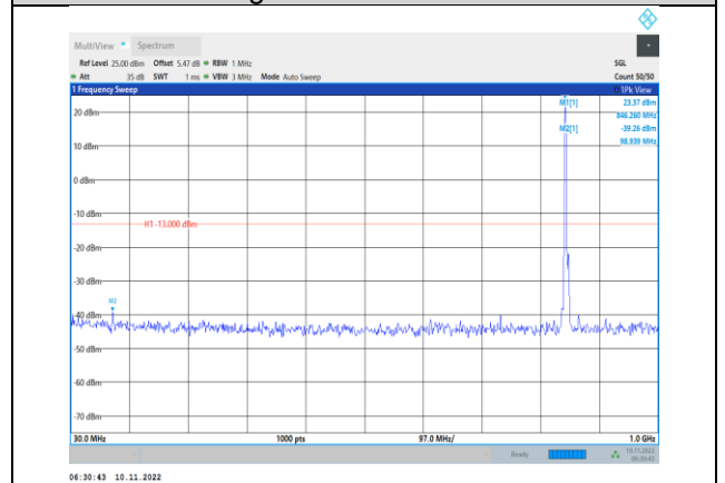
Band5-3MHz-16QAM-20635-1RB#0- Range1:30~1000MHz
