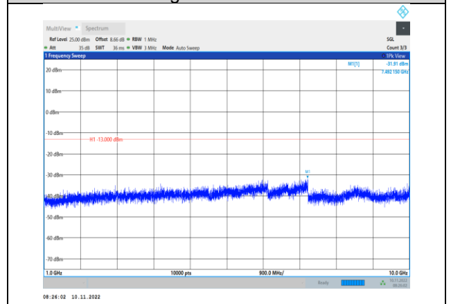
Band5-10MHz-16QAM-20600-1RB#0- Range2:1000~10000MHz
