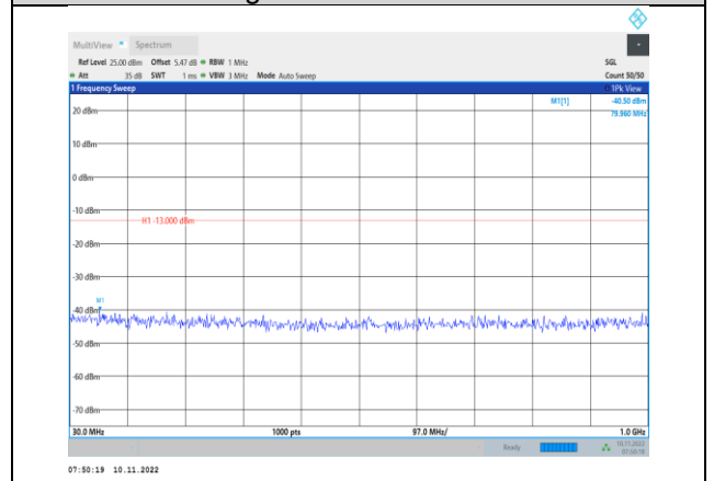
Band4-10MHz-QPSK-20350-1RB#0-Range1:30~1000MHz
