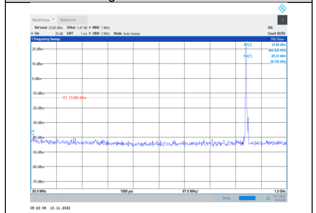
Band5-5MHz-16QAM-20625-1RB#0- Range1:30~1000MHz
