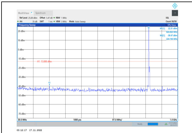
Band5-3MHz-64QAM-20415-1RB#0- Range1:30~1000MHz
