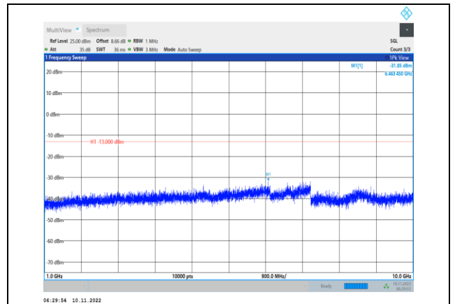
Band5-3MHz-16QAM-20525-1RB#0- Range2:1000~10000MHz
