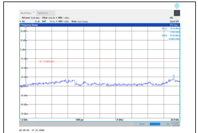
Band4-20MHz-64QAM-20175-1RB#0- Range2:1000~20000MHz
