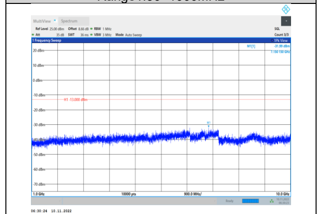
Band5-3MHz-QPSK-20635-1RB#0- Range2:1000~10000MHz
