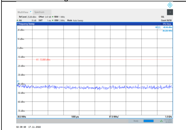
Band4-20MHz-64QAM-20175-1RB#0- Range1:30~1000MHz
