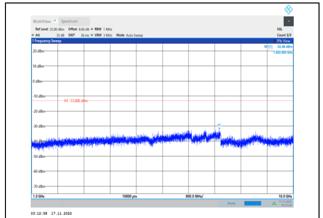
Band5-3MHz-64QAM-20525-1RB#0- Range2:1000~10000MHz
