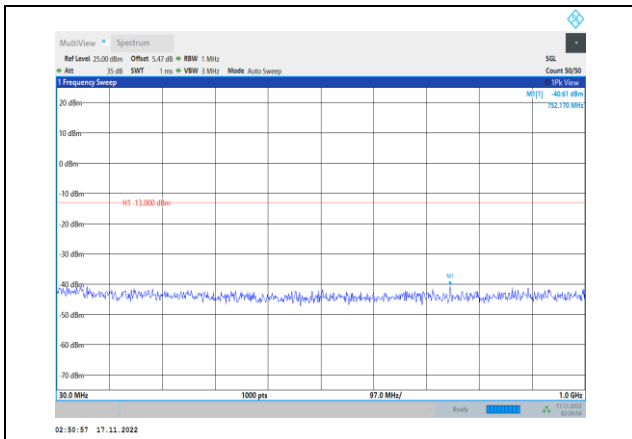
Band4-10MHz-64QAM-20000-1RB#0- Range1:30~1000MHz
