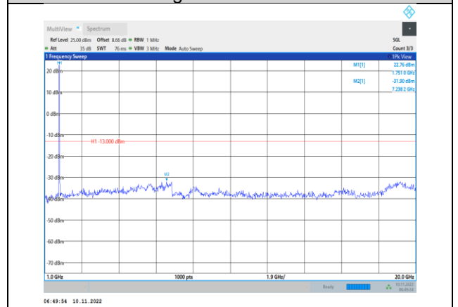
Band4-15MHz-16QAM-20325-1RB#0- Range2:1000~20000MHz
