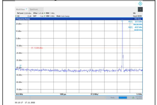
Band5-3MHz-64QAM-20635-1RB#0- Range1:30~1000MHz
