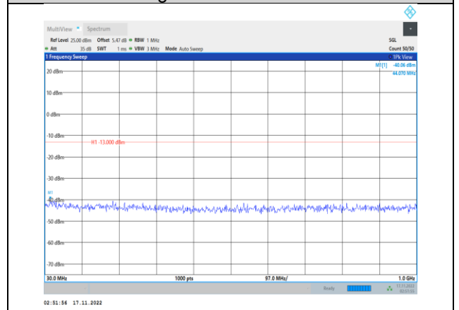
Band4-10MHz-64QAM-20350-1RB#0- Range1:30~1000MHz
