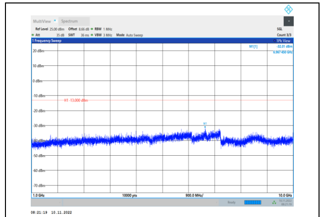
Band5-5MHz-16QAM-20525-1RB#0- Range2:1000~10000MHz
