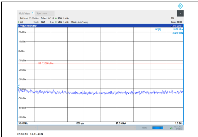
Band4-5MHz-QPSK-19975-1RB#0- Range1:30~1000MHz
