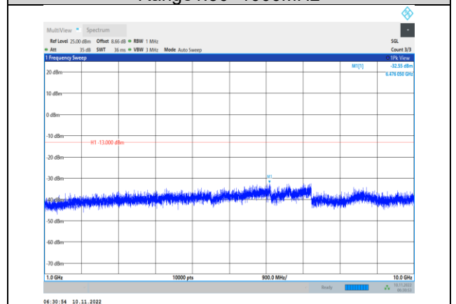
Band5-3MHz-16QAM-20635-1RB#0- Range2:1000~10000MHz
