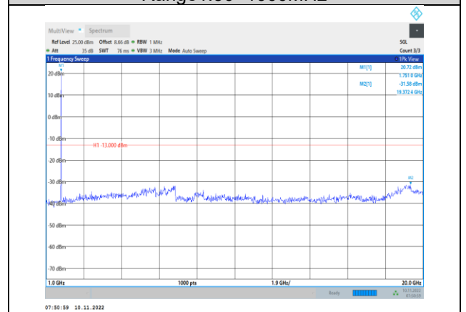
Band4-10MHz-16QAM-20350-1RB#0- Range2:1000~20000MHz
