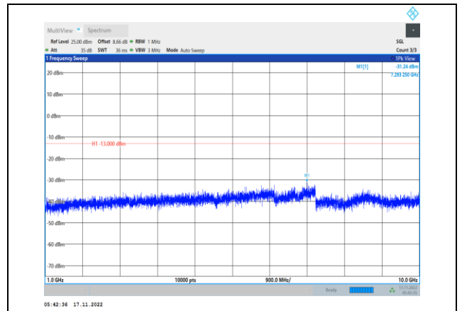
Band5-5MHz-64QAM-20525-1RB#0- Range2:1000~10000MHz
