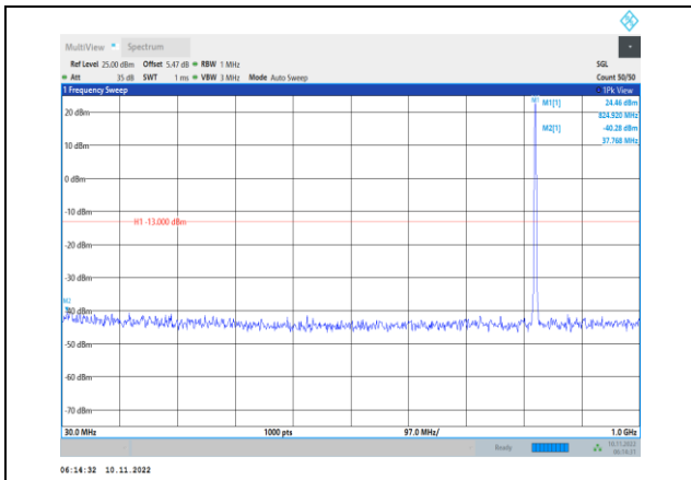
Band5-1.4MHz-QPSK-20407-1RB#0- Range1:30~1000MHz
