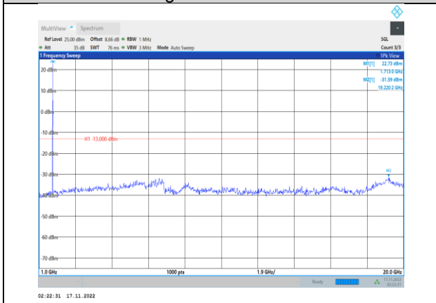
Band4-5MHz-64QAM-19975-1RB#0- Range2:1000~20000MHz
