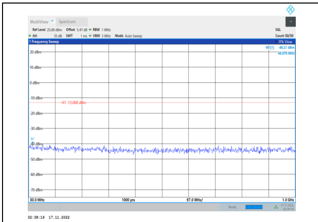
Band4-20MHz-64QAM-20050-1RB#0- Range1:30~1000MHz
