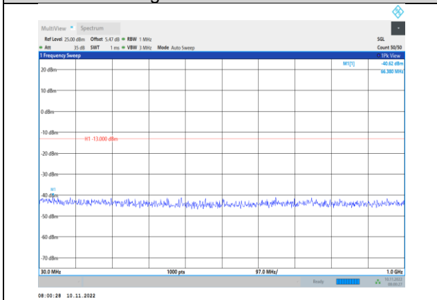
Band4-5MHz-16QAM-20175-1RB#0- Range1:30~1000MHz
