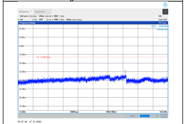
Band5-10MHz-64QAM-20600-1RB#0- Range2:1000~10000MHz
