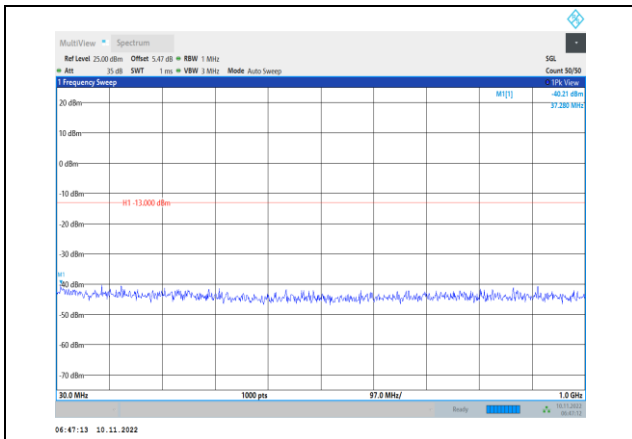
Band4-15MHz-QPSK-20025-1RB#0-Range1:30~1000MHz
