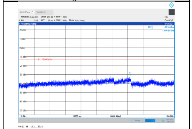
Band5-5MHz-QPSK-20625-1RB#0- Range2:1000~10000MHz
