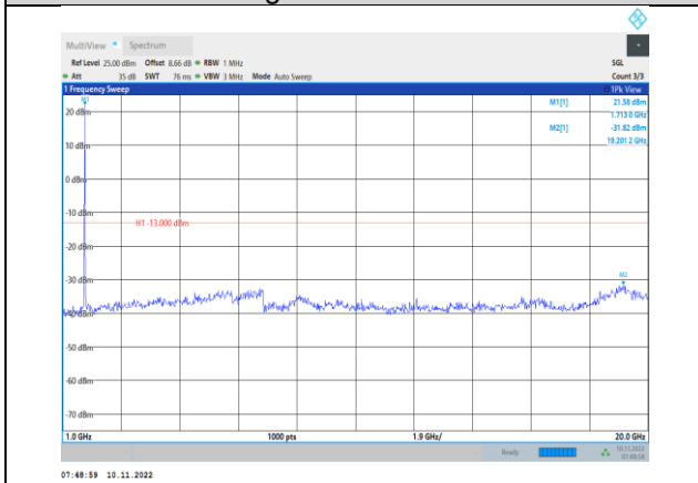
Band4-10MHz-16QAM-20000-1RB#0- Range2:1000~20000MHz
