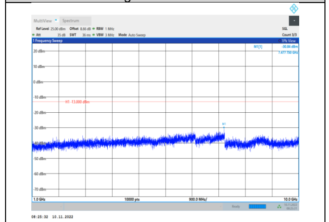
Band5-10MHz-QPSK-20600-1RB#0-Range2:1000~10000MHz
