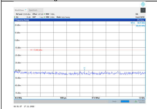
Band4-10MHz-64QAM-20175-1RB#0- Range1:30~1000MHz
