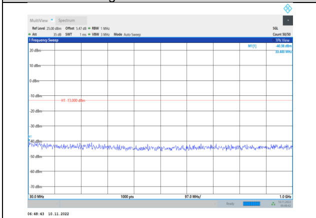
Band4-15MHz-16QAM-20175-1RB#0- Range1:30~1000MHz
