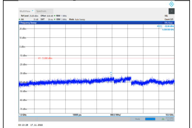
Band5-3MHz-64QAM-20635-1RB#0- Range2:1000~10000MHz
