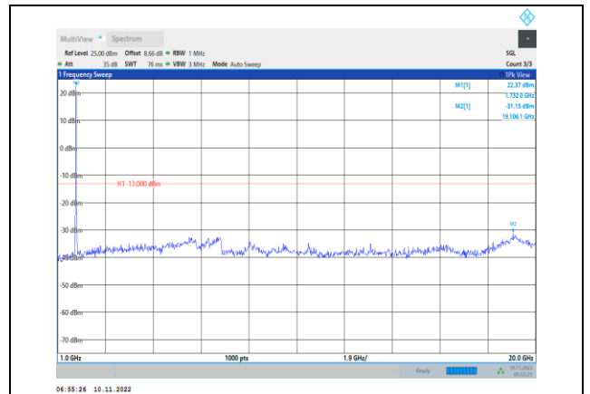
Band4-20MHz-16QAM-20175-1RB#0- Range2:1000~20000MHz
