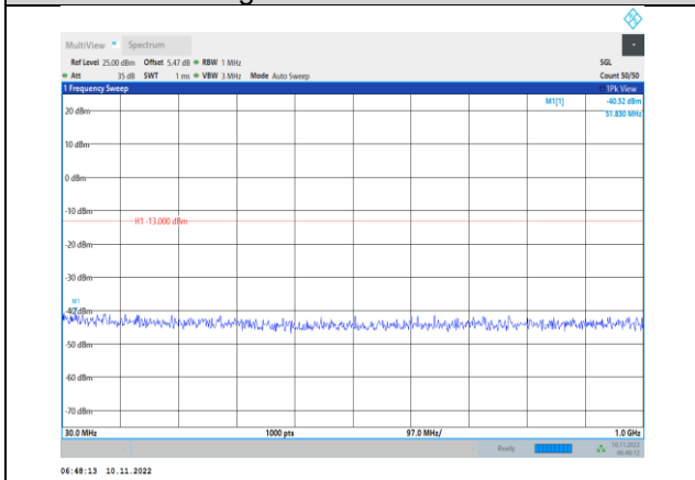
Band4-15MHz-QPSK-20175-1RB#0-Range1:30~1000MHz
