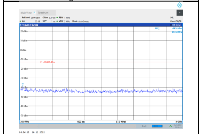
Band4-20MHz-16QAM-20300-1RB#0- Range1:30~1000MHz
