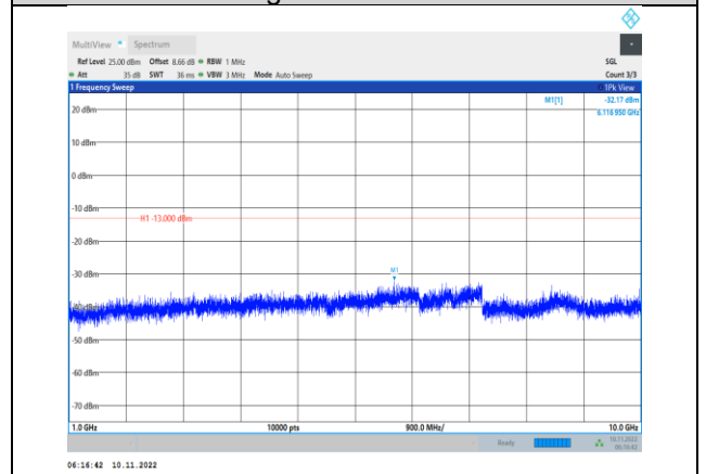
Band5-1.4MHz-QPSK-20643-1RB#0- Range2:1000~10000MHz
