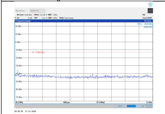
Band4-5MHz-64QAM-20175-1RB#0- Range1:30~1000MHz
