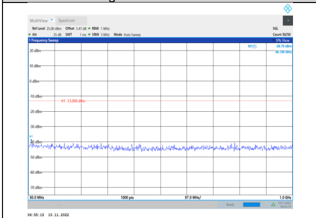
Band4-20MHz-16QAM-20175-1RB#0- Range1:30~1000MHz
