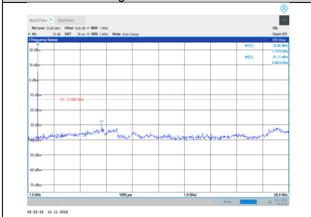
Band4-1.4MHz-16QAM-19957-1RB#0- Range2:1000~20000MHz
