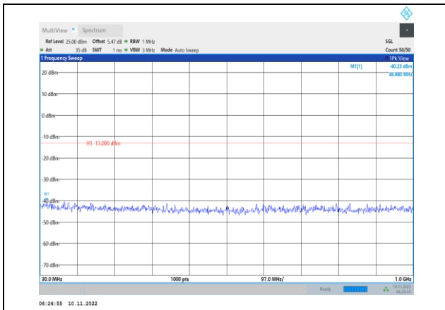
Band4-1.4MHz-16QAM-19957-1RB#0- Range1:30~1000MHz
