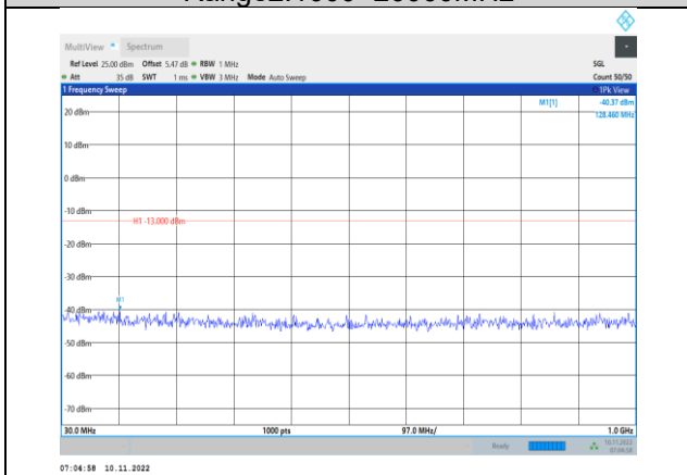
Band2-10MHz-QPSK-18900-1RB#0- Range1:30~1000MHz
