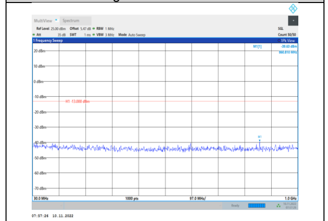
Band2-15MHz-QPSK-19125-1RB#0-Range1:30~1000MHz
