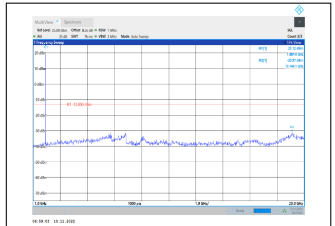
Band2-1.4MHz-16QAM-18900-1RB#0- Range2:1000~20000MHz
