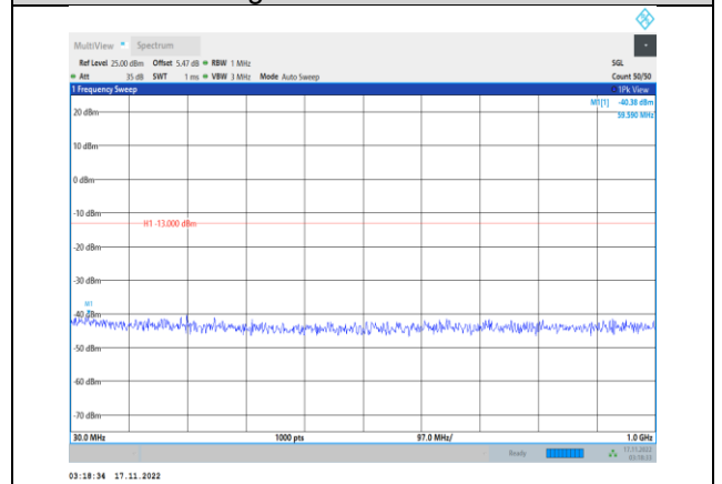
Band2-20MHz-64QAM-19100-1RB#0- Range1:30~1000MHz
