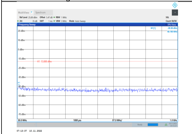
Band2-3MHz-QPSK-18900-1RB#0- Range1:30~1000MHz
