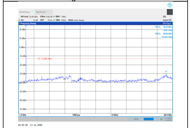
Band2-15MHz-64QAM-19125-1RB#0- Range2:1000~20000MHz
