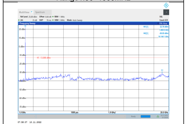
Band2-15MHz-16QAM-19125-1RB#0- Range2:1000~20000MHz
