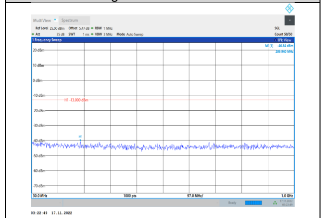
Band2-10MHz-64QAM-19150-1RB#0- Range1:30~1000MHz
