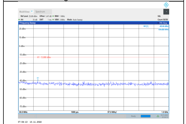
Band2-20MHz-16QAM-19100-1RB#0- Range1:30~1000MHz
