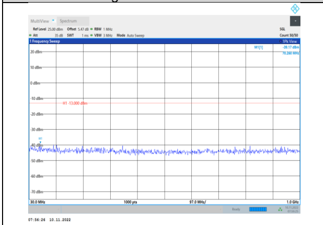
Band2-15MHz-QPSK-18900-1RB#0-Range1:30~1000MHz
