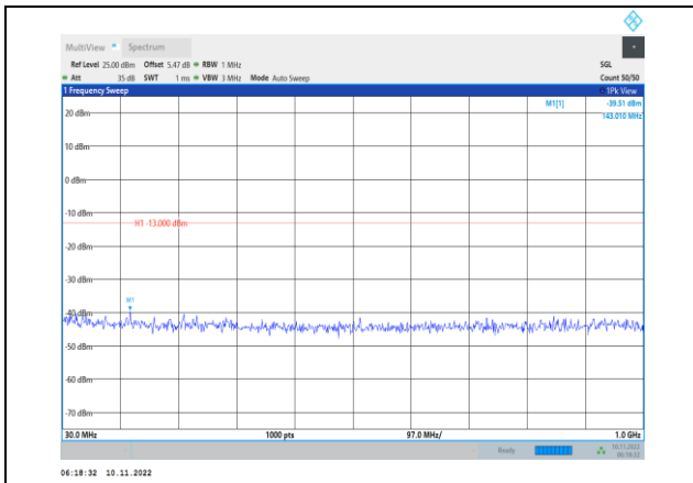
Band2-5MHz-QPSK-18625-1RB#0- Range1:30~1000MHz
