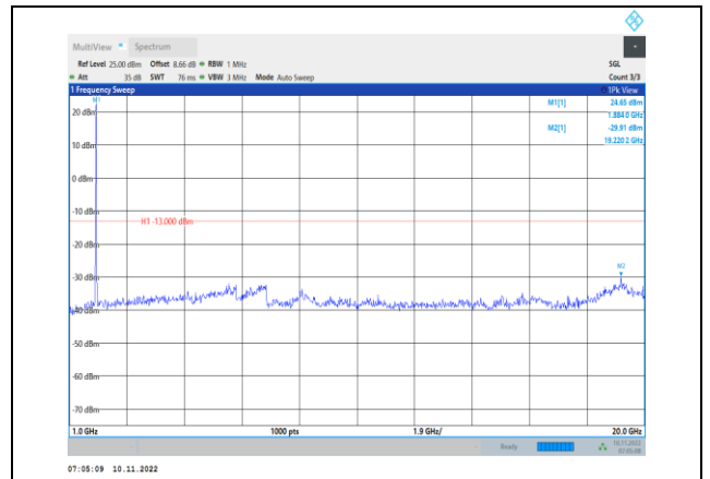
Band2-10MHz-QPSK-18900-1RB#0- Range2:1000~20000MHz
