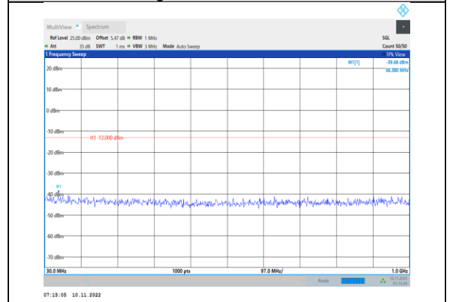
Band2-3MHz-16QAM-19185-1RB#0- Range1:30~1000MHz
