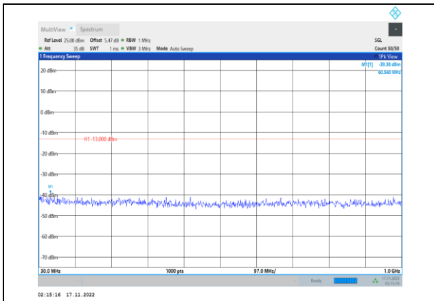
Band4-3MHz-64QAM-19965-1RB#0- Range1:30~1000MHz
