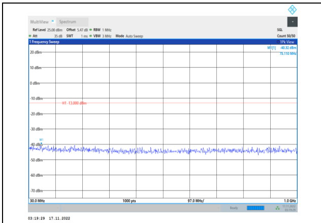
Band2-15MHz-64QAM-18675-1RB#0- Range1:30~1000MHz
