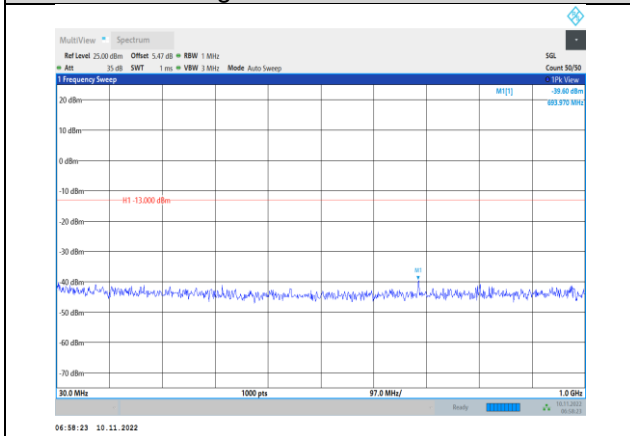
Band2-1.4MHz-QPSK-18900-1RB#0- Range1:30~1000MHz
