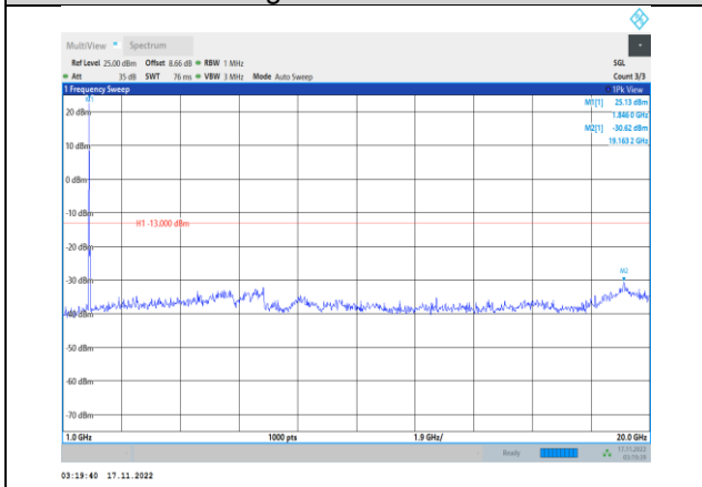
Band2-15MHz-64QAM-18675-1RB#0- Range2:1000~20000MHz
