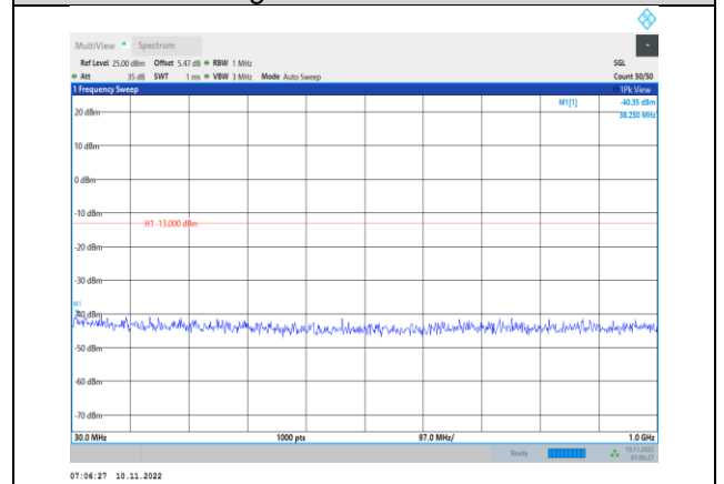
Band2-10MHz-16QAM-19150-1RB#0- Range1:30~1000MHz
