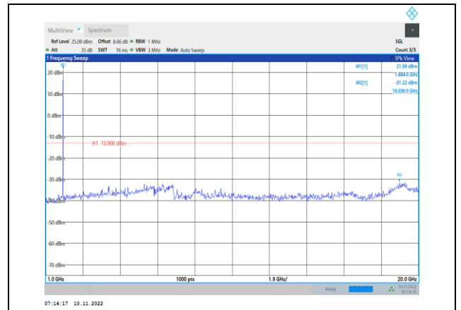
Band2-3MHz-16QAM-18900-1RB#0- Range2:1000~20000MHz
