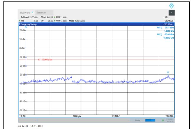
Band2-5MHz-64QAM-18900-1RB#0- Range2:1000~20000MHz
