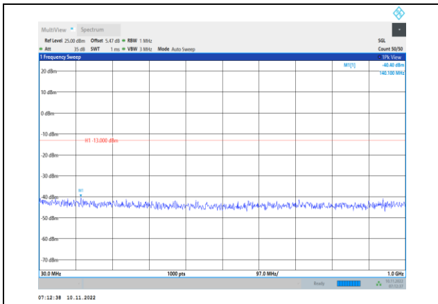
Band2-3MHz-QPSK-18615-1RB#0- Range1:30~1000MHz
