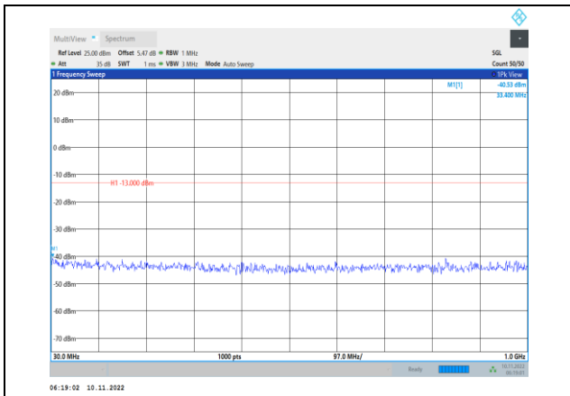
Band2-5MHz-16QAM-18625-1RB#0- Range1:30~1000MHz
