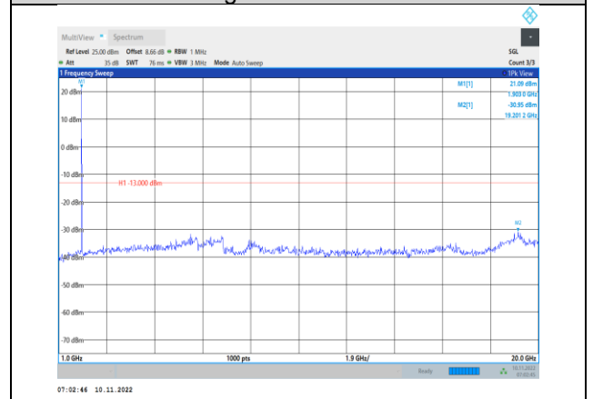
Band2-1.4MHz-16QAM-19193-1RB#0- Range2:1000~20000MHz
