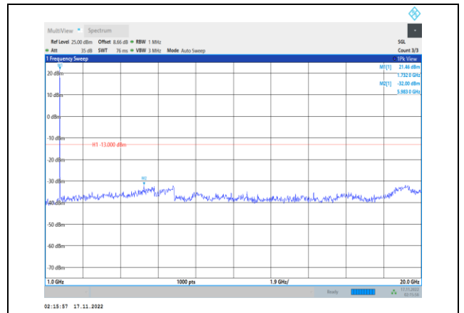
Band4-3MHz-64QAM-20175-1RB#0- Range2:1000~20000MHz
