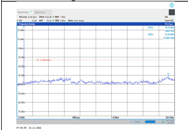
Band2-10MHz-16QAM-18650-1RB#0- Range2:1000~20000MHz
