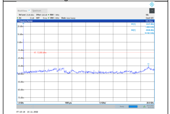
Band2-3MHz-16QAM-19185-1RB#0- Range2:1000~20000MHz
