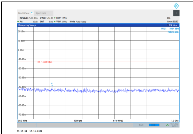
Band2-20MHz-64QAM-18700-1RB#0- Range1:30~1000MHz
