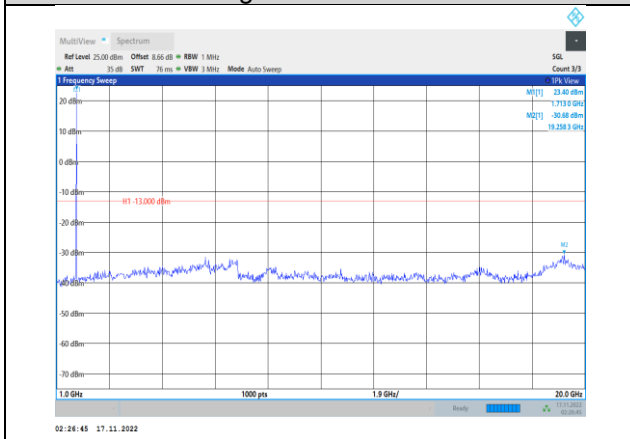
Band4-1.4MHz-64QAM-19957-1RB#0- Range2:1000~20000MHz
