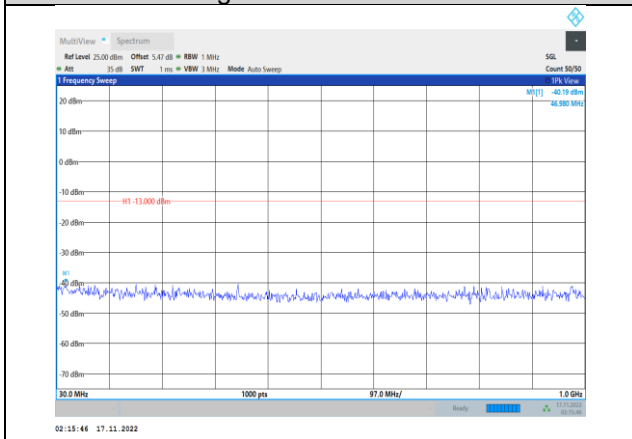
Band4-3MHz-64QAM-20175-1RB#0- Range1:30~1000MHz
