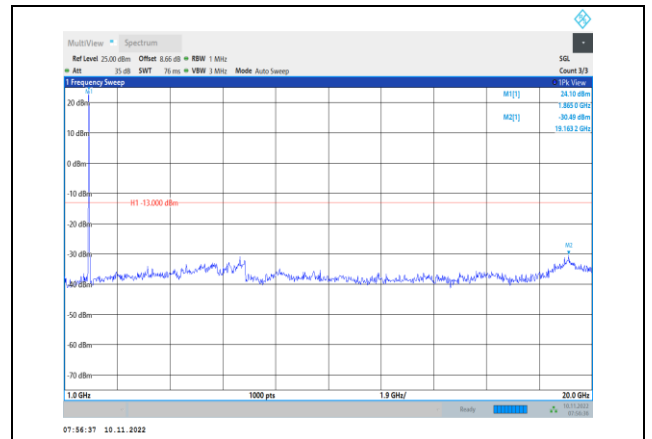
Band2-15MHz-QPSK-18900-1RB#0-Range2:1000~20000MHz
