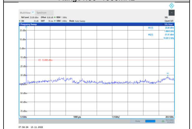
Band2-20MHz-16QAM-19100-1RB#0- Range2:1000~20000MHz
