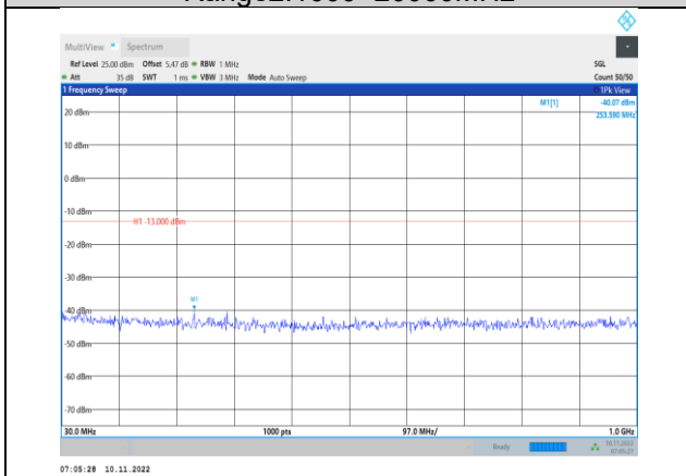
Band2-10MHz-16QAM-18900-1RB#0- Range1:30~1000MHz
