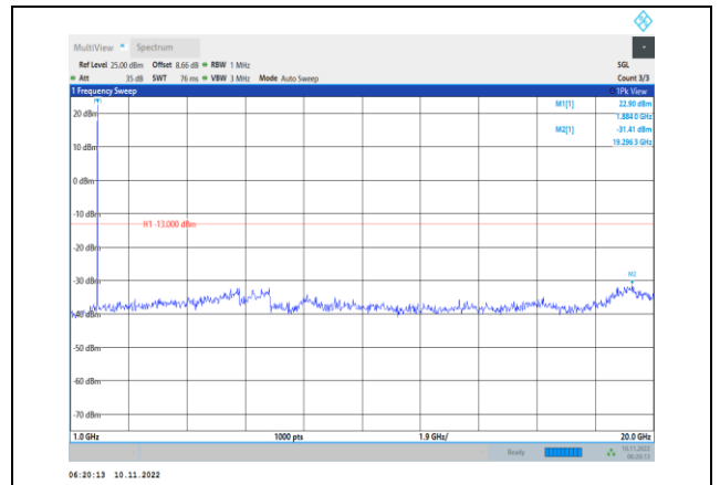
Band2-5MHz-16QAM-18900-1RB#0- Range2:1000~20000MHz
