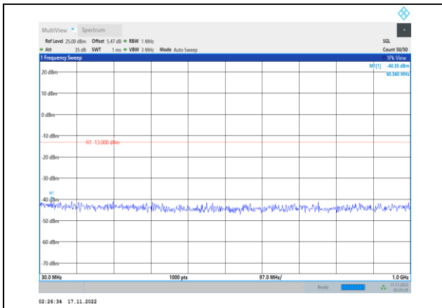
Band4-1.4MHz-64QAM-19957-1RB#0- Range1:30~1000MHz
