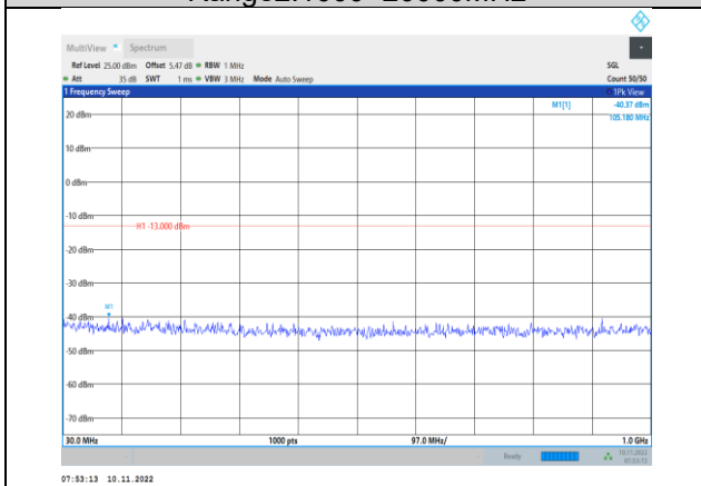
Band2-20MHz-16QAM-18900-1RB#0- Range1:30~1000MHz
