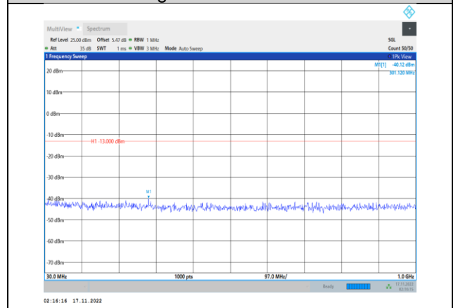
Band4-3MHz-64QAM-20385-1RB#0- Range1:30~1000MHz
