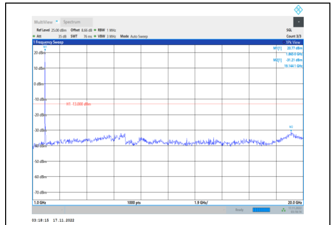
Band2-20MHz-64QAM-18900-1RB#0- Range2:1000~20000MHz
