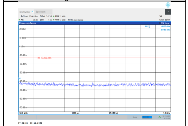
Band2-1.4MHz-16QAM-19193-1RB#0- Range1:30~1000MHz
