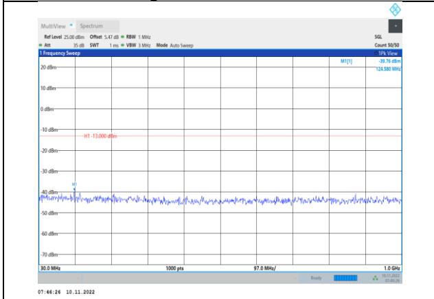
Band4-3MHz-16QAM-20175-1RB#0- Range1:30~1000MHz
