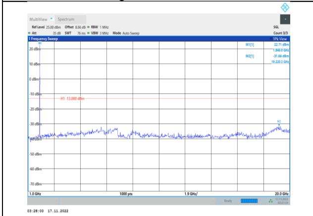
Band2-1.4MHz-64QAM-18607-1RB#0- Range2:1000~20000MHz
