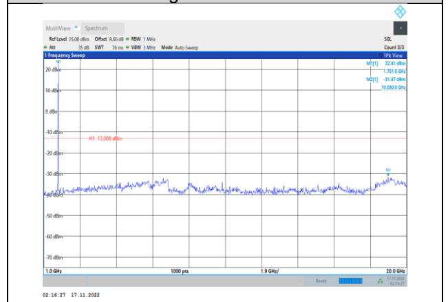
Band4-3MHz-64QAM-20385-1RB#0- Range2:1000~20000MHz
