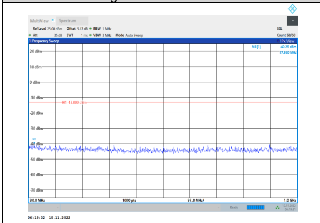
Band2-5MHz-QPSK-18900-1RB#0- Range1:30~1000MHz
