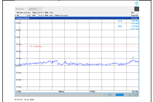
Band4-3MHz-16QAM-20385-1RB#0- Range2:1000~20000MHz
