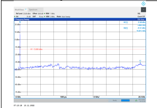
Band2-3MHz-16QAM-18615-1RB#0- Range2:1000~20000MHz
