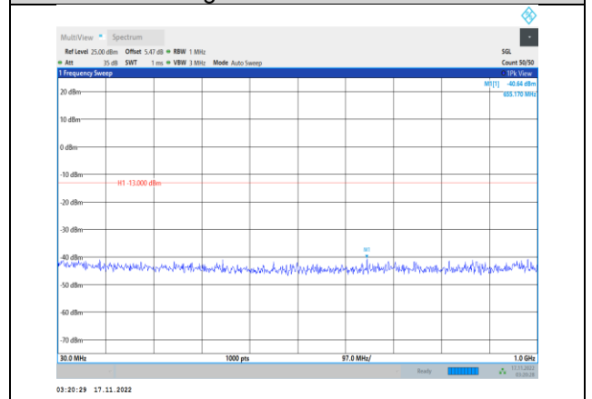
Band2-15MHz-64QAM-19125-1RB#0- Range1:30~1000MHz
