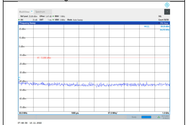
Band4-3MHz-QPSK-20385-1RB#0- Range1:30~1000MHz
