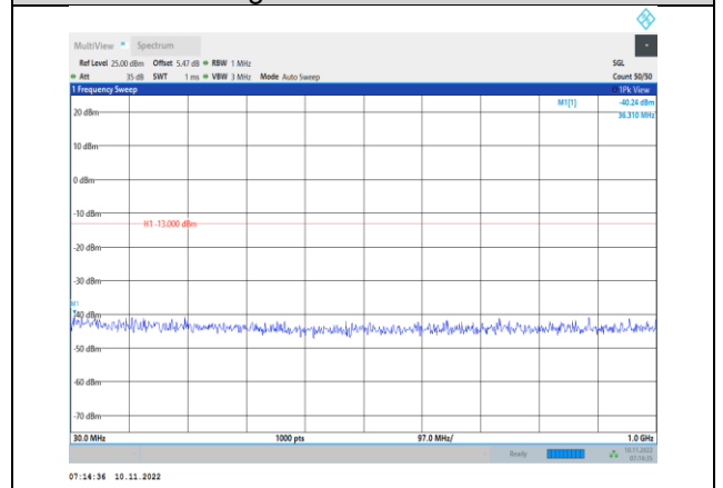
Band2-3MHz-QPSK-19185-1RB#0- Range1:30~1000MHz
