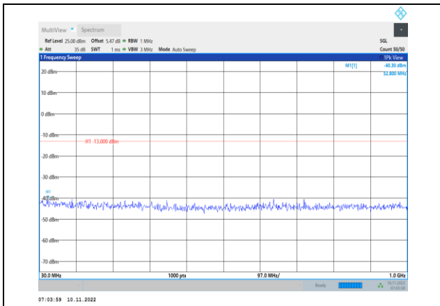
Band2-10MHz-QPSK-18650-1RB#0- Range1:30~1000MHz
