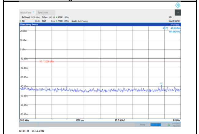
Band4-1.4MHz-64QAM-20393-1RB#0- Range1:30~1000MHz
