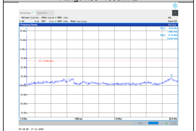
Band2-20MHz-64QAM-19100-1RB#0- Range2:1000~20000MHz
