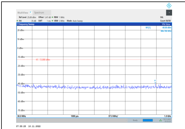
Band2-15MHz-QPSK-18675-1RB#0-Range1:30~1000MHz
