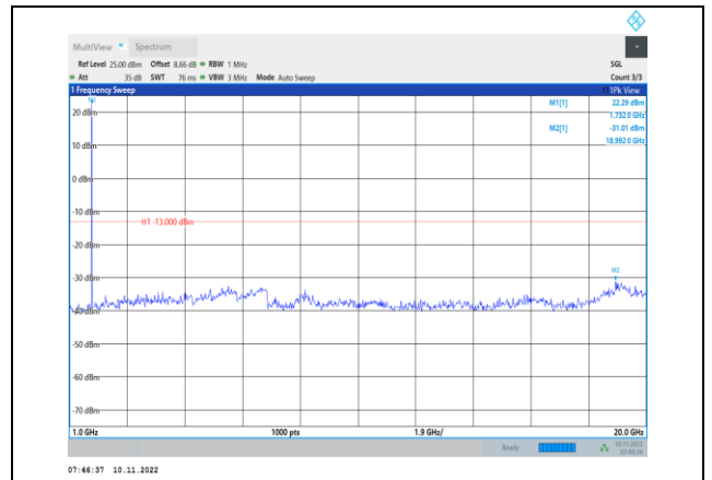
Band4-3MHz-16QAM-20175-1RB#0- Range2:1000~20000MHz
