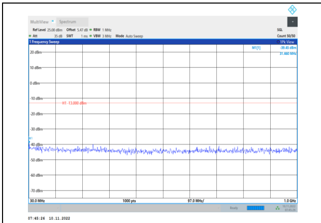
Band4-3MHz-16QAM-19965-1RB#0- Range1:30~1000MHz
