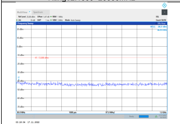
Band2-20MHz-64QAM-18900-1RB#0- Range1:30~1000MHz
