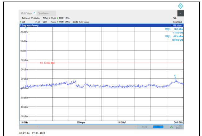
Band4-1.4MHz-64QAM-20175-1RB#0- Range2:1000~20000MHz
