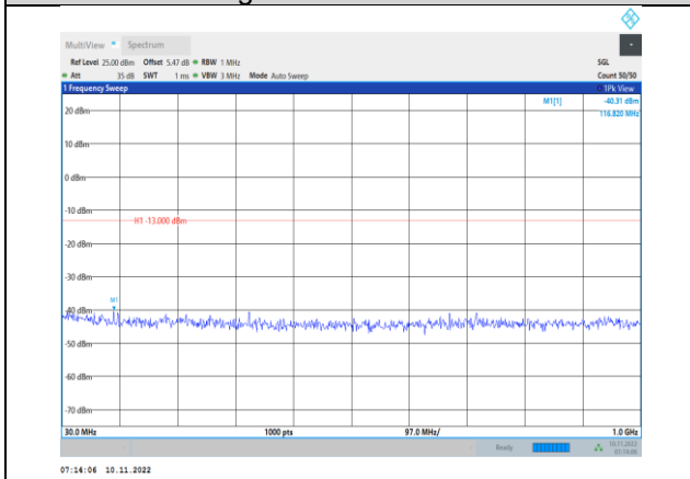
Band2-3MHz-16QAM-18900-1RB#0- Range1:30~1000MHz
