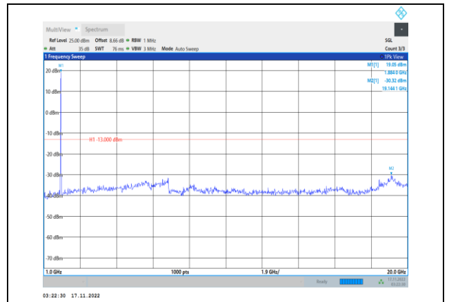
Band2-10MHz-64QAM-18900-1RB#0- Range2:1000~20000MHz
