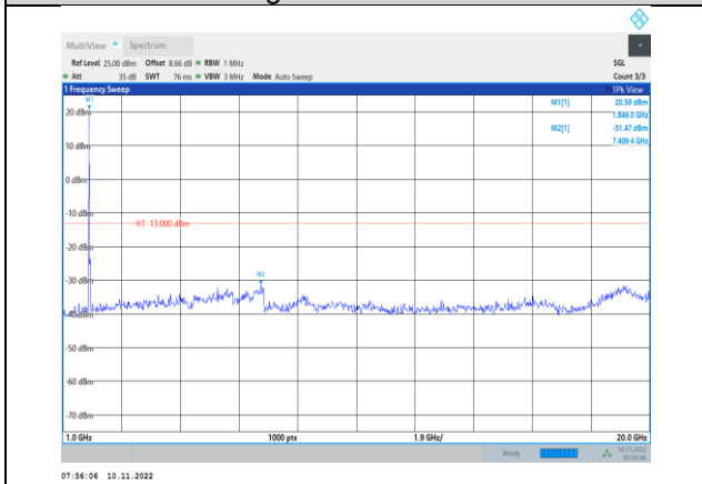
Band2-15MHz-16QAM-18675-1RB#0- Range2:1000~20000MHz
