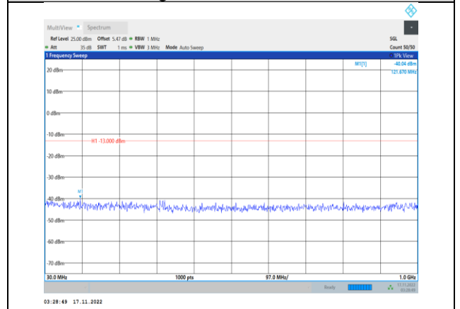
Band2-1.4MHz-64QAM-19193-1RB#0- Range1:30~1000MHz
