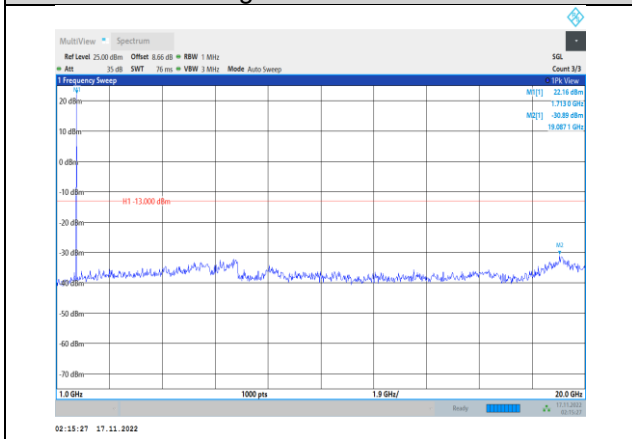
Band4-3MHz-64QAM-19965-1RB#0- Range2:1000~20000MHz
