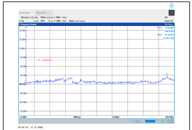
Band2-15MHz-64QAM-18900-1RB#0- Range2:1000~20000MHz
