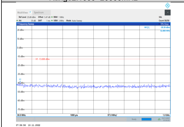
Band2-15MHz-16QAM-18900-1RB#0- Range1:30~1000MHz
