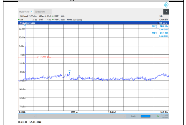
Band2-10MHz-64QAM-19150-1RB#0- Range2:1000~20000MHz
