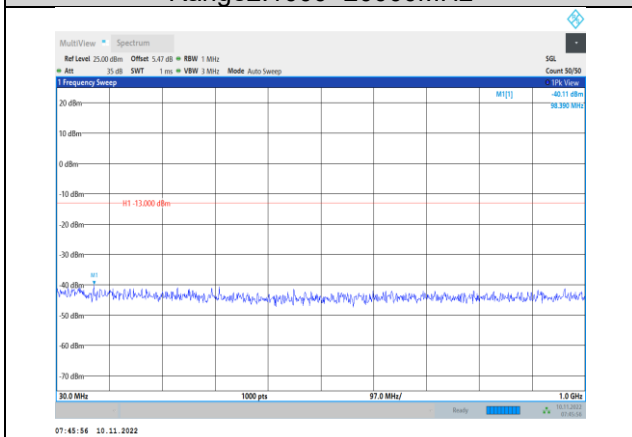
Band4-3MHz-QPSK-20175-1RB#0- Range1:30~1000MHz
