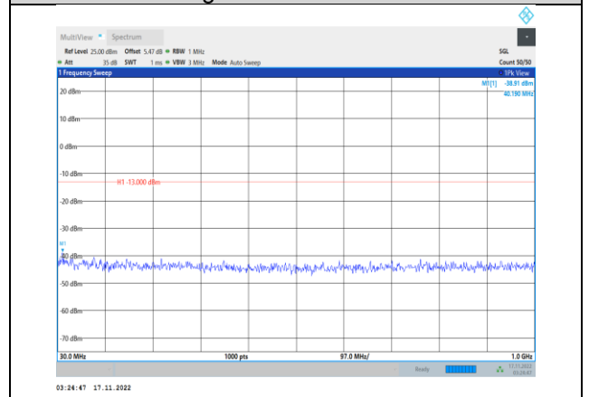
Band2-5MHz-64QAM-19175-1RB#0- Range1:30~1000MHz
