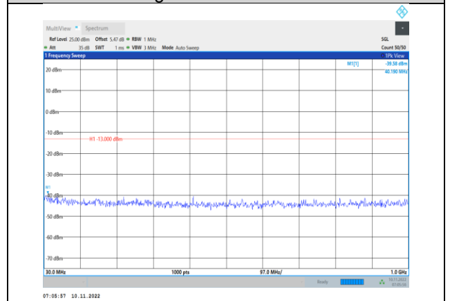
Band2-10MHz-QPSK-19150-1RB#0- Range1:30~1000MHz
