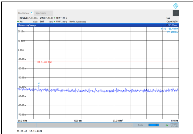
Band2-5MHz-64QAM-18625-1RB#0- Range1:30~1000MHz
