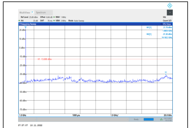
Band2-15MHz-16QAM-18900-1RB#0- Range2:1000~20000MHz
