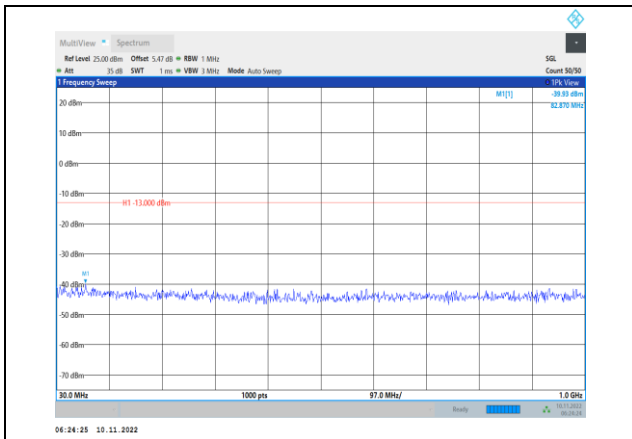
Band4-1.4MHz-QPSK-19957-1RB#0-Range1:30~1000MHz
