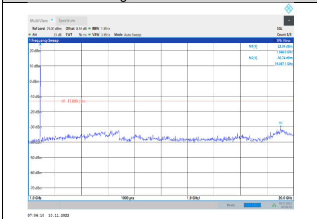
Band2-10MHz-QPSK-18650-1RB#0- Range2:1000~20000MHz
