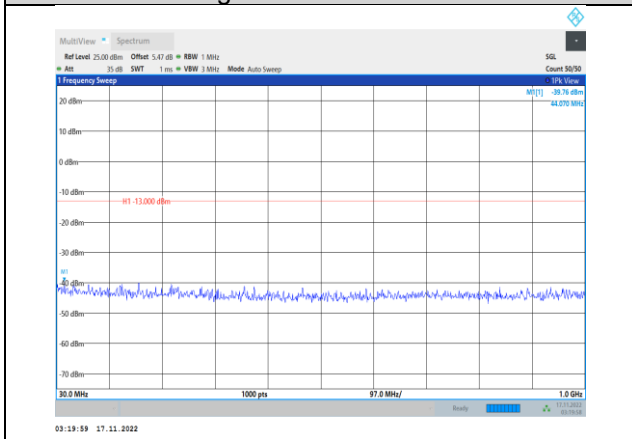
Band2-15MHz-64QAM-18900-1RB#0- Range1:30~1000MHz
