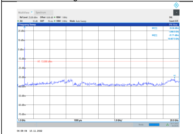
Band2-1.4MHz-16QAM-18607-1RB#0- Range2:1000~20000MHz
