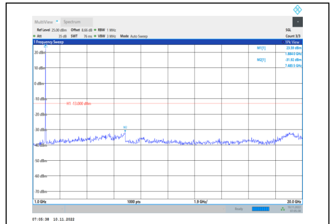
Band2-10MHz-16QAM-18900-1RB#0- Range2:1000~20000MHz
