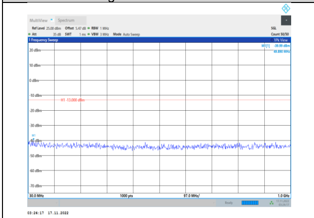
Band2-5MHz-64QAM-18900-1RB#0- Range1:30~1000MHz
