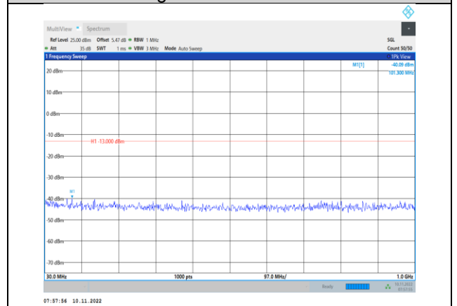
Band2-15MHz-16QAM-19125-1RB#0- Range1:30~1000MHz
