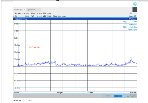
Band2-10MHz-64QAM-18650-1RB#0- Range2:1000~20000MHz
