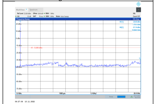
Band4-1.4MHz-16QAM-20393-1RB#0- Range2:1000~20000MHz
