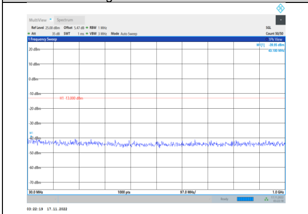
Band2-10MHz-64QAM-18900-1RB#0- Range1:30~1000MHz
