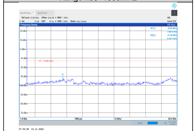
Band2-10MHz-16QAM-19150-1RB#0- Range2:1000~20000MHz
