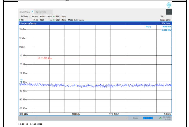
Band4-1.4MHz-16QAM-20393-1RB#0- Range1:30~1000MHz
