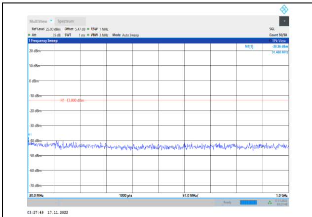
Band2-1.4MHz-64QAM-18607-1RB#0- Range1:30~1000MHz
