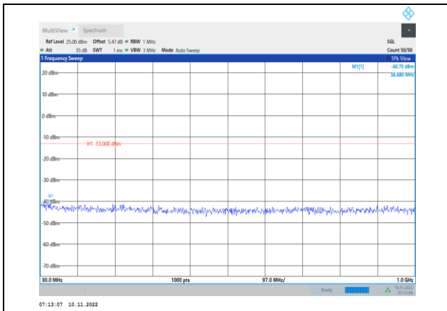
Band2-3MHz-16QAM-18615-1RB#0- Range1:30~1000MHz
