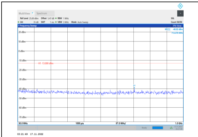
Band2-10MHz-64QAM-18650-1RB#0- Range1:30~1000MHz
