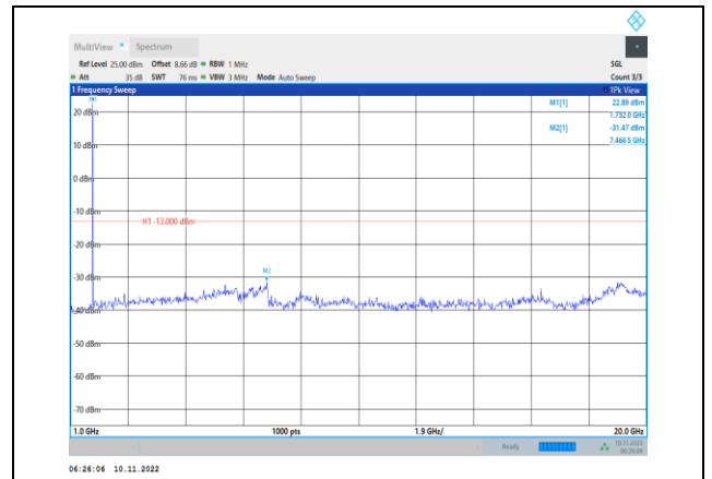
Band4-1.4MHz-16QAM-20175-1RB#0- Range2:1000~20000MHz
