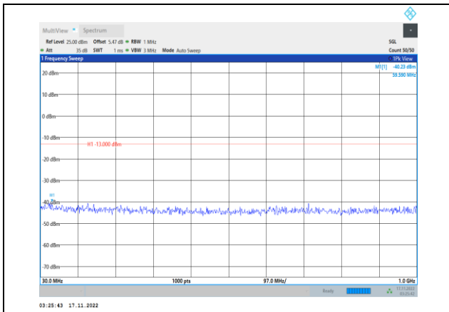
Band2-3MHz-64QAM-18615-1RB#0-Range1:30~1000MHz
