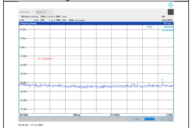
Band2-3MHz-64QAM-19185-1RB#0-Range1:30~1000MHz
