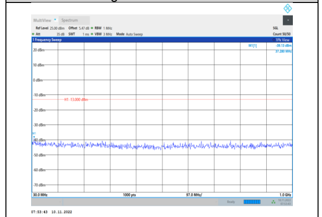
Band2-20MHz-QPSK-19100-1RB#0-Range1:30~1000MHz
