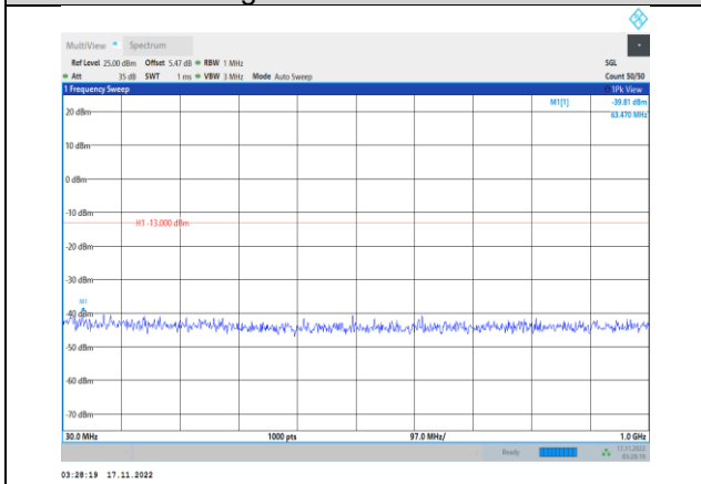
Band2-1.4MHz-64QAM-18900-1RB#0- Range1:30~1000MHz
