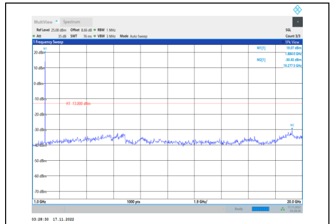
Band2-1.4MHz-64QAM-18900-1RB#0- Range2:1000~20000MHz
