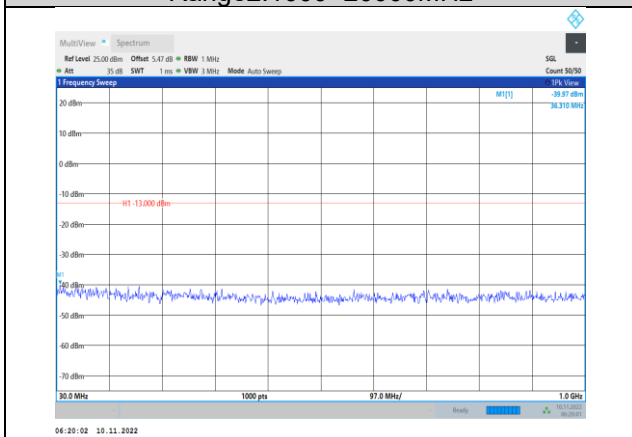
Band2-5MHz-16QAM-18900-1RB#0- Range1:30~1000MHz
