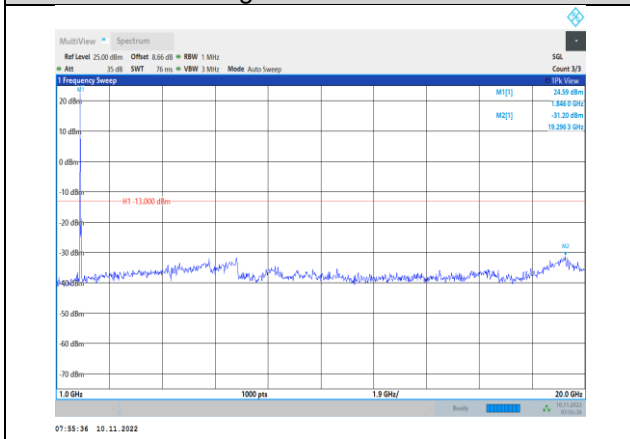
Band2-15MHz-QPSK-18675-1RB#0-Range2:1000~20000MHz
