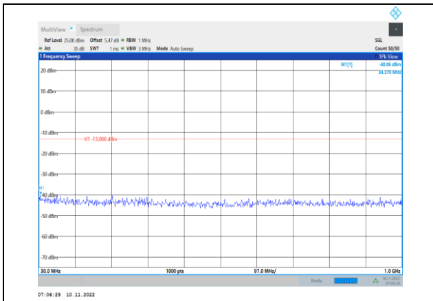
Band2-10MHz-16QAM-18650-1RB#0- Range1:30~1000MHz
