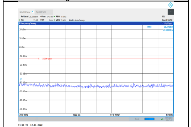
Band2-5MHz-16QAM-19175-1RB#0- Range1:30~1000MHz
