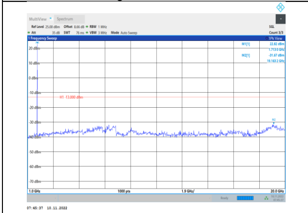
Band4-3MHz-16QAM-19965-1RB#0- Range2:1000~20000MHz
