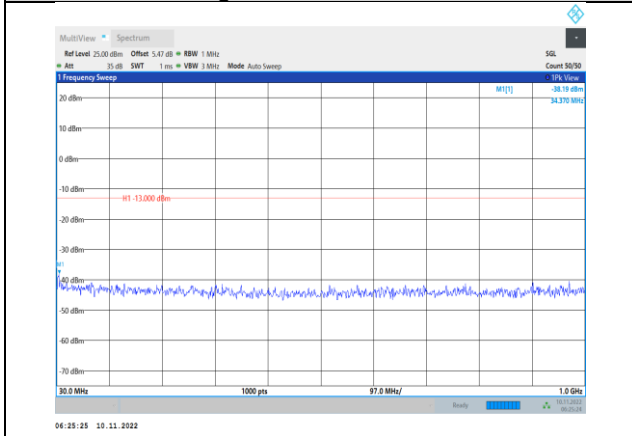
Band4-1.4MHz-QPSK-20175-1RB#0-Range1:30~1000MHz
