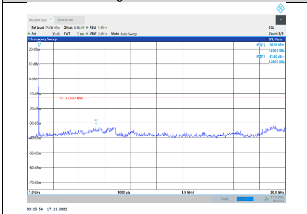
Band2-3MHz-64QAM-18615-1RB#0-Range2:1000~20000MHz
