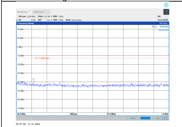
Band4-1.4MHz-64QAM-20175-1RB#0- Range1:30~1000MHz
