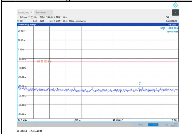
Band2-3MHz-64QAM-18900-1RB#0-Range1:30~1000MHz
