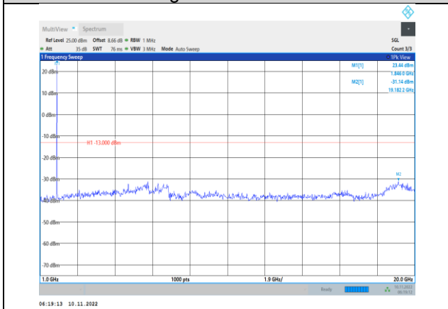
Band2-5MHz-16QAM-18625-1RB#0- Range2:1000~20000MHz
