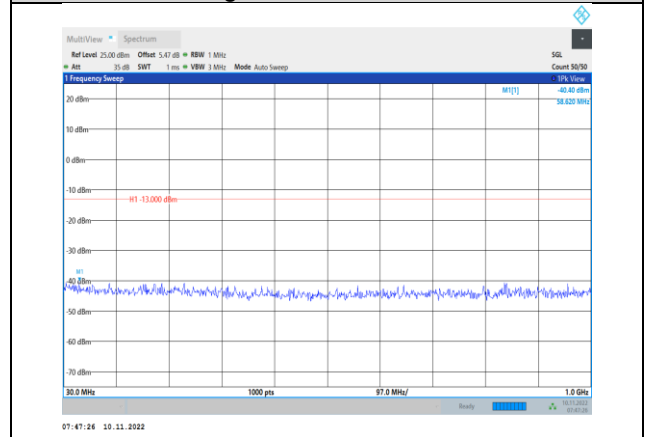
Band4-3MHz-16QAM-20385-1RB#0- Range1:30~1000MHz
