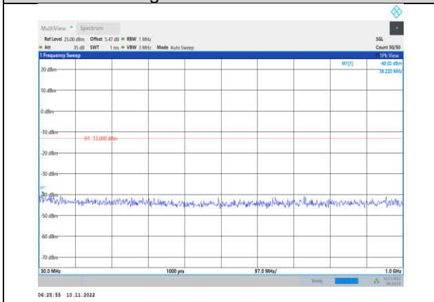
Band4-1.4MHz-16QAM-20175-1RB#0- Range1:30~1000MHz
