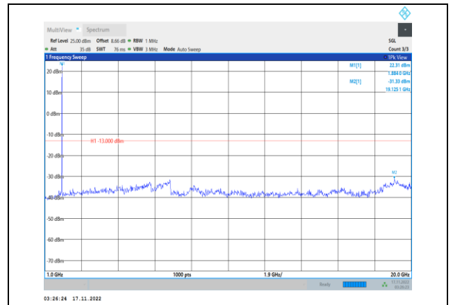
Band2-3MHz-64QAM-18900-1RB#0-Range2:1000~20000MHz
