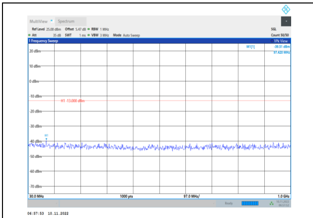
Band2-1.4MHz-16QAM-18607-1RB#0- Range1:30~1000MHz
