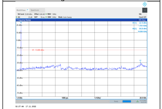
Band4-1.4MHz-64QAM-20393-1RB#0- Range2:1000~20000MHz
