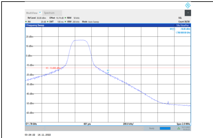
Band66-5MHz-64QAM-132647-1RB#24
