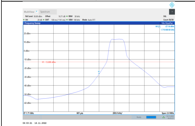
Band66-3MHz-64QAM-131987-1RB#0
