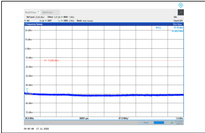
Band2-9262-30~1000MHz
