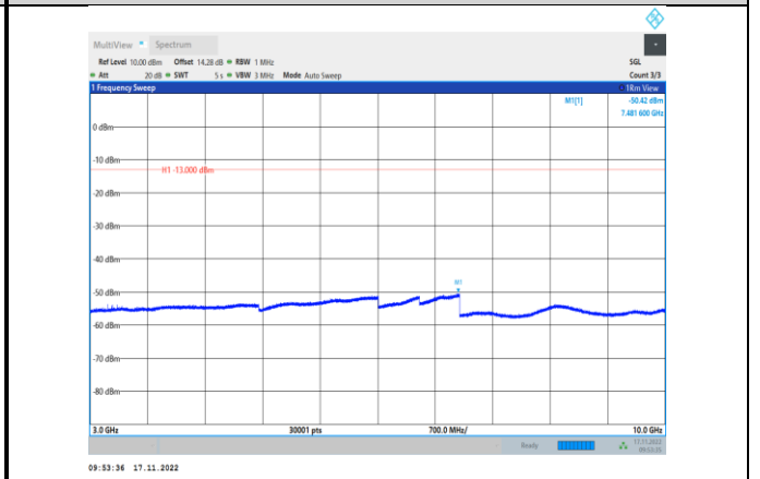
Band5-4182-3000~10000MHz
