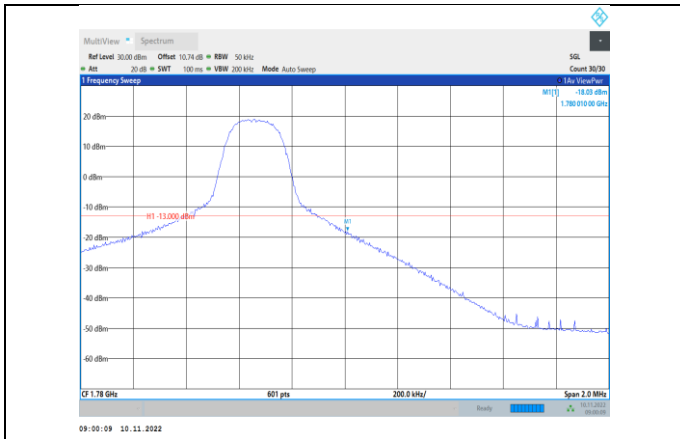
Band66-5MHz-QPSK-132647-1RB#24
