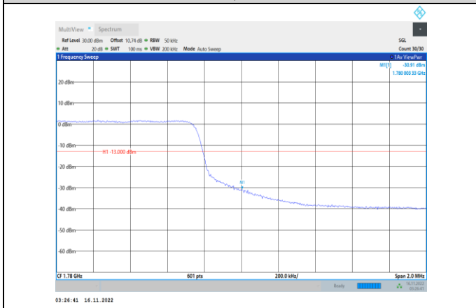
Band66-5MHz-64QAM-132647-25RB#0
