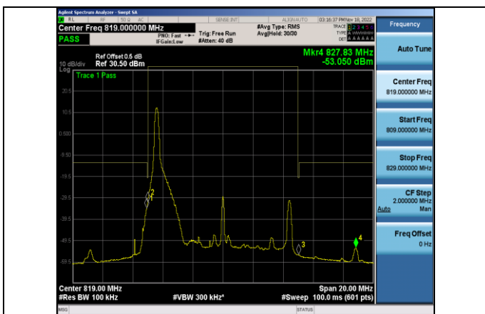
Band26-10MHz-QPSK-26740 Left-1RB#0
