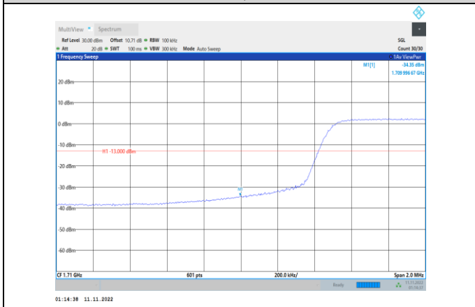
Band66-10MHz-16QAM-132022-50RB#0
