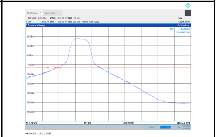
Band66-5MHz-16QAM-132647-1RB#24
