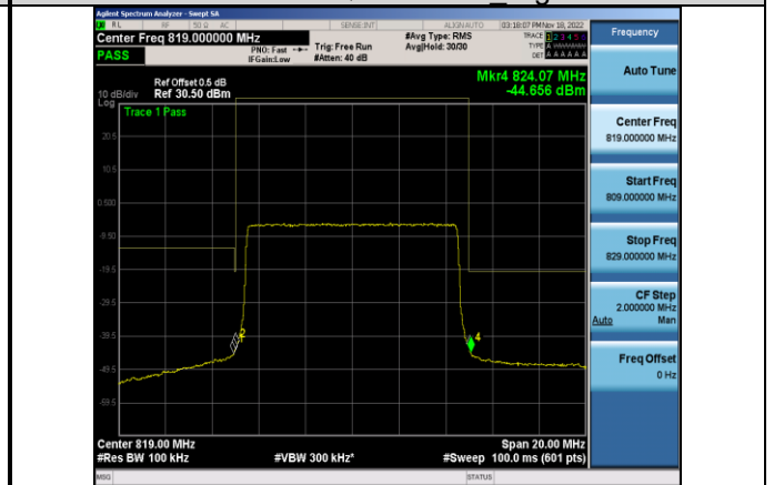
Band26-10MHz-16QAM-26740 Right-50RB#0
