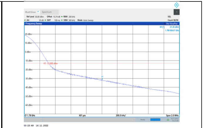
Band66-20MHz-64QAM-132572-1RB#99
