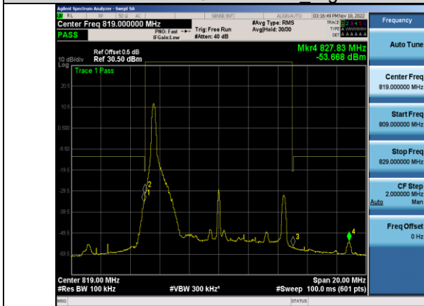
Band26-10MHz-16QAM-26740 Left-1RB#0
