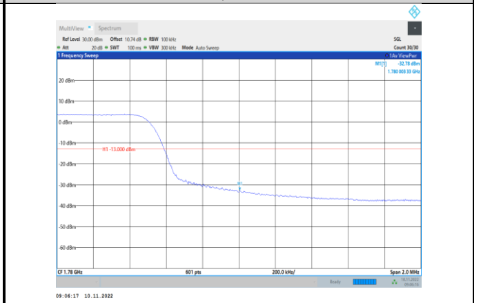
Band66-10MHz-QPSK-132622-50RB#0
