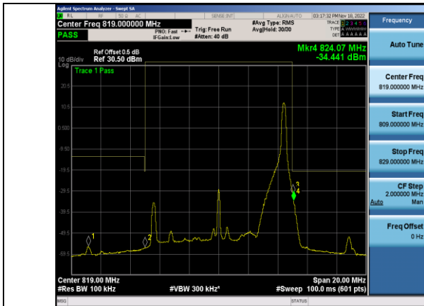
Band26-10MHz-QPSK-26740 Right-1RB#49
