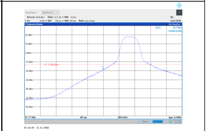
Band66-5MHz-QPSK-131997-1RB#0
