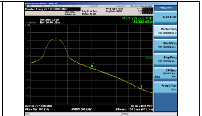
Band13-10MHz-QPSK-23230 Right-1RB#49
