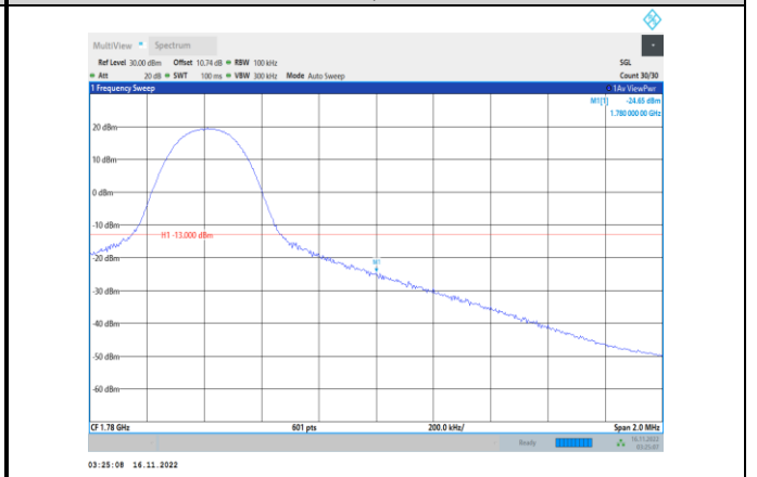
Band66-10MHz-64QAM-132622-1RB#49
