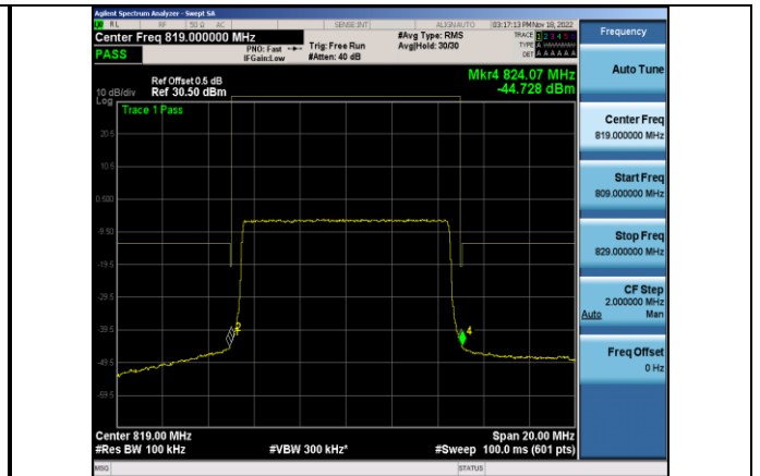
Band26-10MHz-16QAM-26740 Left-50RB#0
