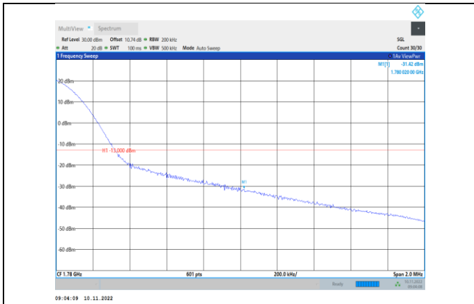
Band66-20MHz-16QAM-132572-1RB#99
