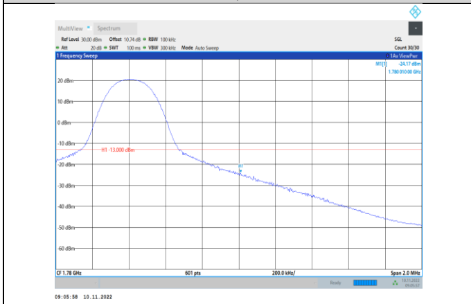
Band66-10MHz-16QAM-132622-1RB#49
