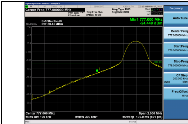
Band13-10MHz-QPSK-23230 Left-1RB#0
