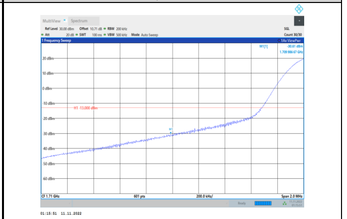
Band66-20MHz-16QAM-132072-1RB#0
