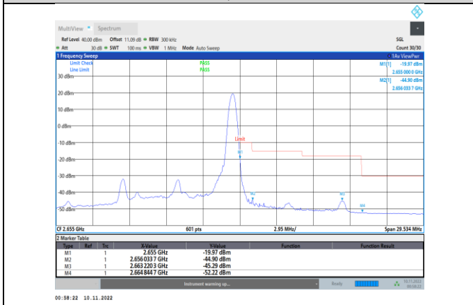
Band41-10MHz-QPSK-41190-1RB#49
