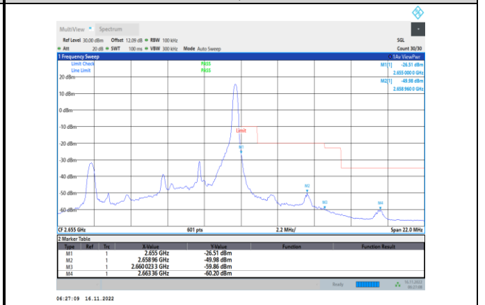
Band41-5MHz-64QAM-41215-1RB#24
