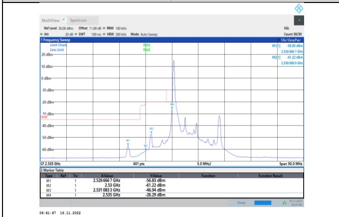
Band41-5MHz-64QAM-40065-1RB#0
