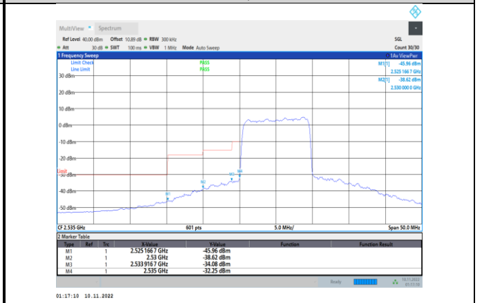
Band41-10MHz-16QAM-40090-50RB#0
