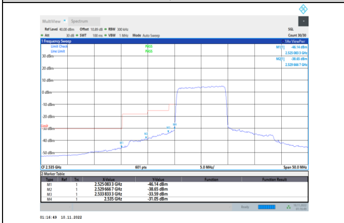
Band41-10MHz-QPSK-40090-50RB#0
