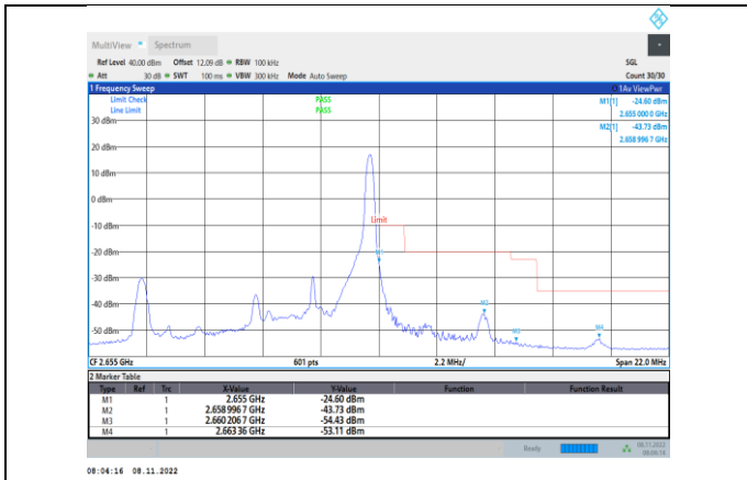
Band41-5MHz-16QAM-41215-1RB#24
