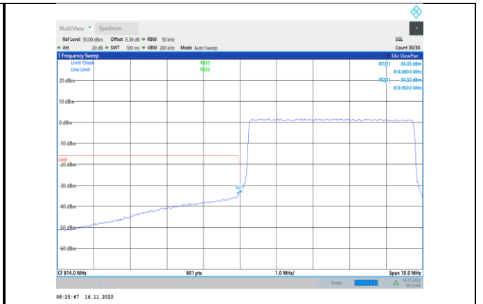
Band26-5MHz-64QAM-26715-25RB#0
