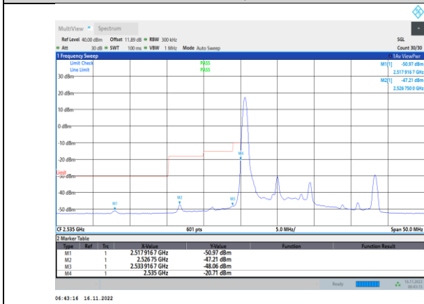
Band41-10MHz-64QAM-40090-1RB#0
