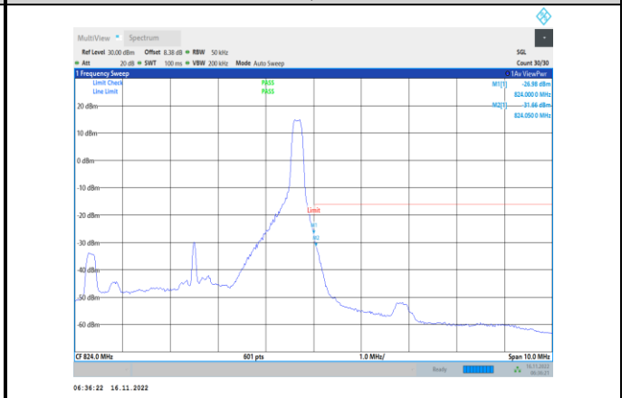
Band26-5MHz-64QAM-26765-1RB#24
