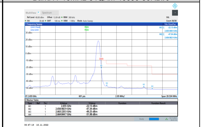
Band41-10MHz-64QAM-41190-1RB#49
