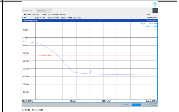
Band26-15MHz-QPSK-26965-75RB#0
