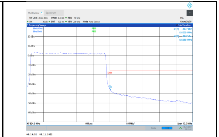
Band26-5MHz-QPSK-26765-25RB#0
