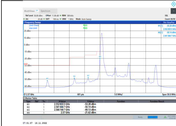
Band38-10MHz-64QAM-37800-1RB#0
