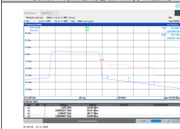
Band41-10MHz-16QAM-41190-50RB#0
