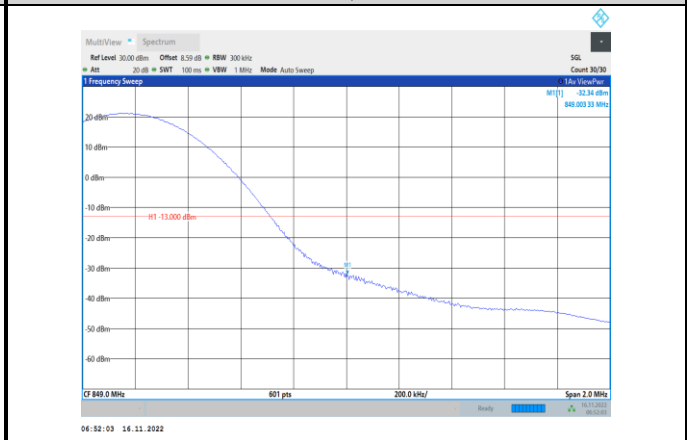
Band26-15MHz-64QAM-26965-1RB#74
