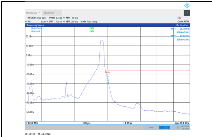
Band26-5MHz-16QAM-26765-1RB#24
