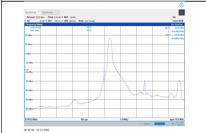
Band26-5MHz-64QAM-26715-1RB#0
