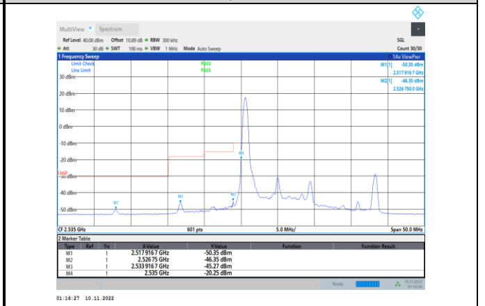
Band41-10MHz-16QAM-40090-1RB#0
