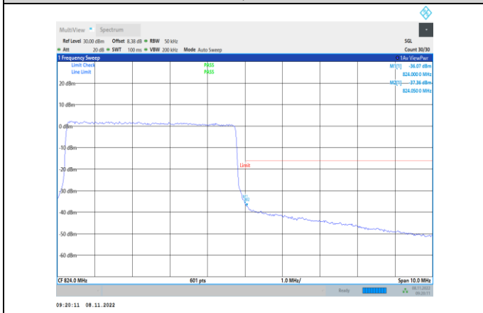
Band26-5MHz-16QAM-26765-25RB#0
