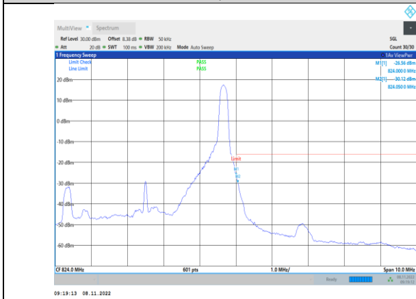
Band26-5MHz-QPSK-26765-1RB#24
