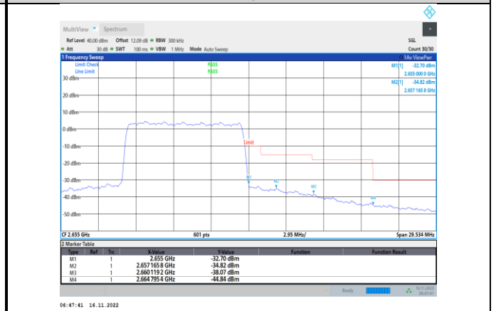
Band41-10MHz-64QAM-41190-50RB#0
