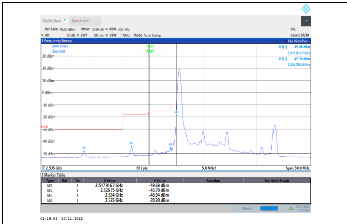
Band41-10MHz-QPSK-40090-1RB#0
