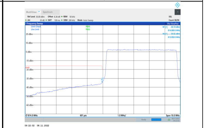
Band26-5MHz-16QAM-26715-25RB#0
