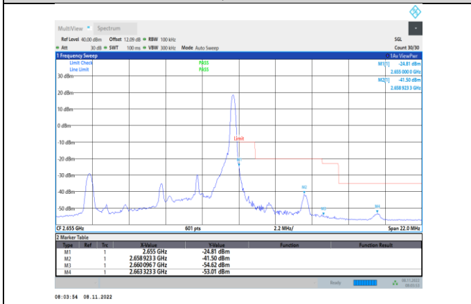
Band41-5MHz-QPSK-41215-1RB#24
