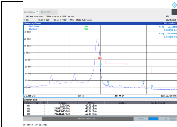
Band41-10MHz-16QAM-41190-1RB#49
