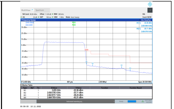
Band41-10MHz-QPSK-41190-50RB#0
