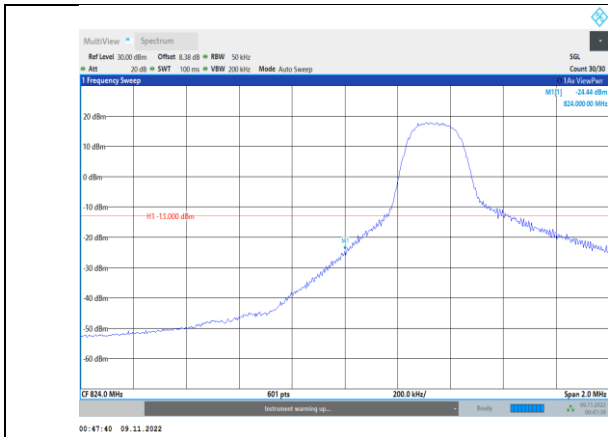
Band5-5MHz-QPSK-20425-1RB#0
