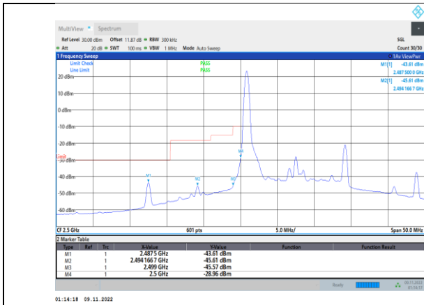
Band7-15MHz-QPSK-20825-1RB#0
