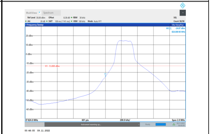
Band5-3MHz-16QAM-20415-1RB#0
