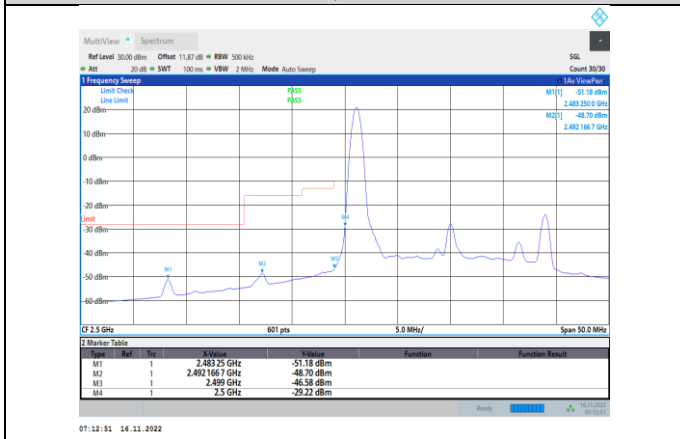
Band7-20MHz-64QAM-20850-1RB#0
