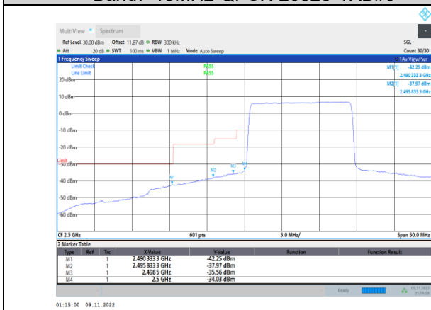
Band7-15MHz-QPSK-20825-75RB#0
