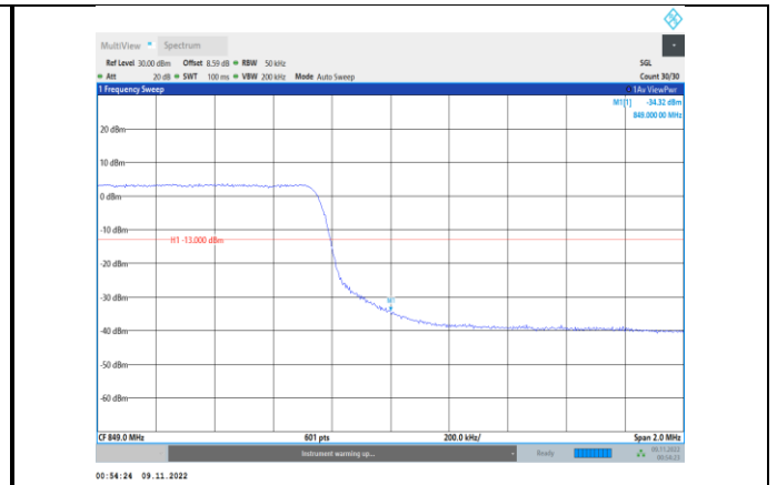
Band5-5MHz-QPSK-20625-25RB#0
