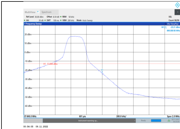
Band5-5MHz-16QAM-20625-1RB#24
