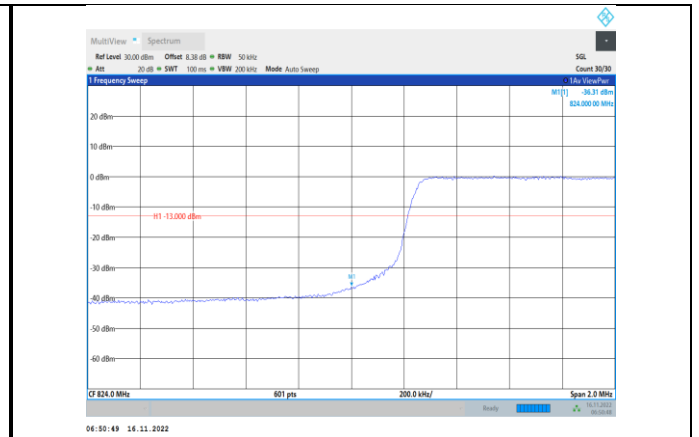
Band5-5MHz-64QAM-20425-25RB#0
