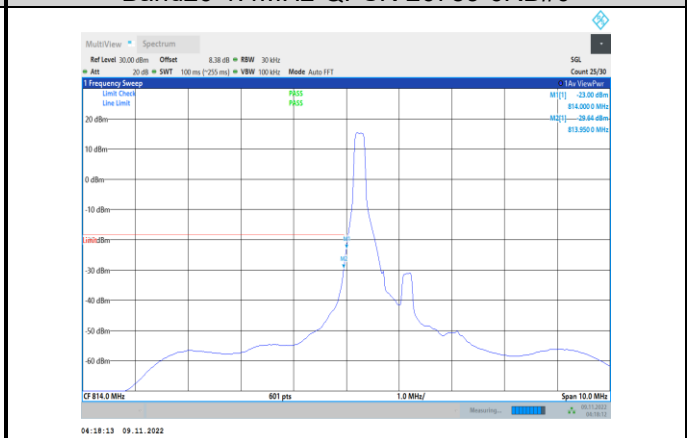
Band26-1.4MHz-16QAM-26697-1RB#0
