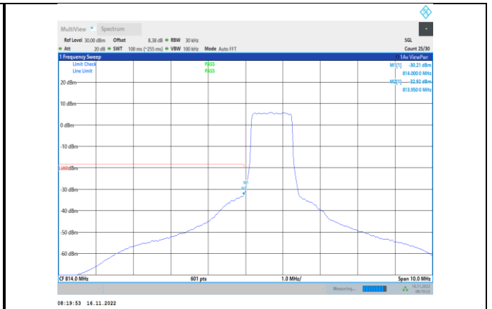
Band26-1.4MHz-64QAM-26697-6RB#0
