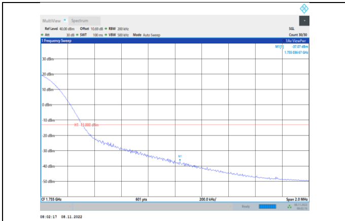
Band4-20MHz-16QAM-20300-1RB#99
