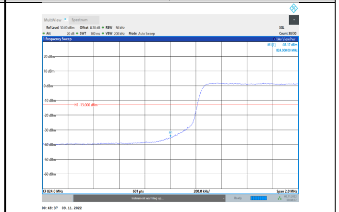
Band5-5MHz-16QAM-20425-25RB#0
