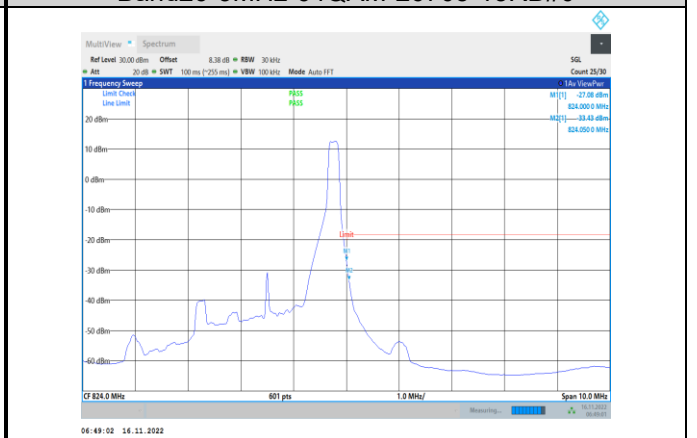
Band26-3MHz-64QAM-26775-1RB#14
