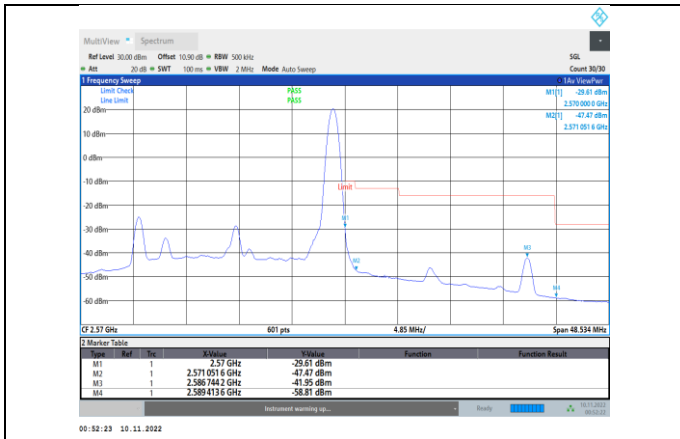
Band7-20MHz-16QAM-21350-1RB#99
