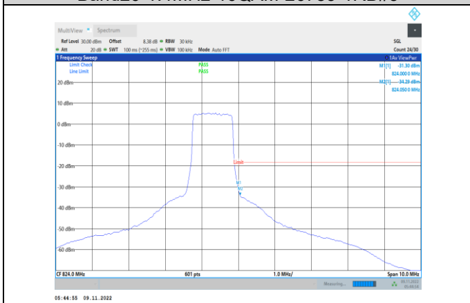
Band26-1.4MHz-16QAM-26783-6RB#0
