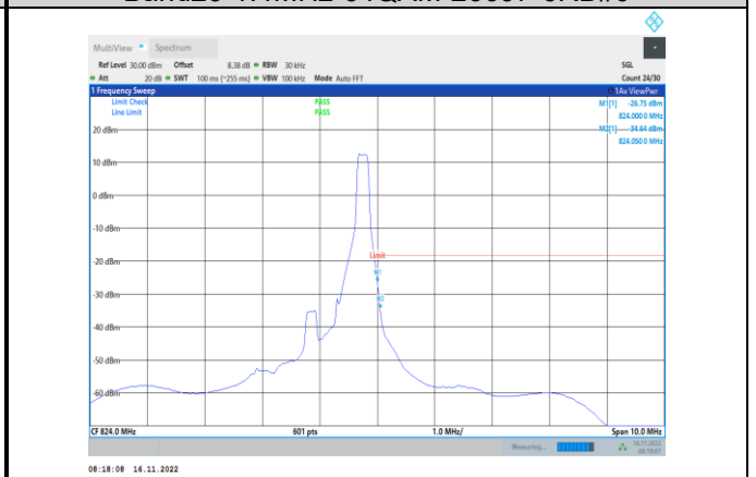
Band26-1.4MHz-64QAM-26783-1RB#5
