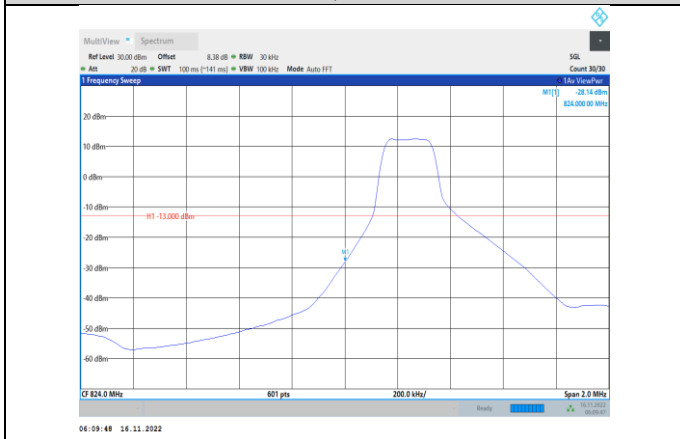
Band5-3MHz-64QAM-20415-1RB#0
