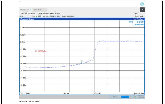
Band13-5MHz-64QAM-23205-25RB#0
