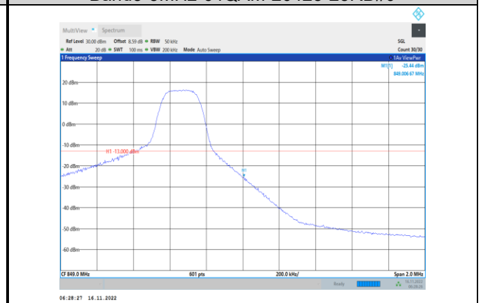
Band5-5MHz-64QAM-20625-1RB#24
