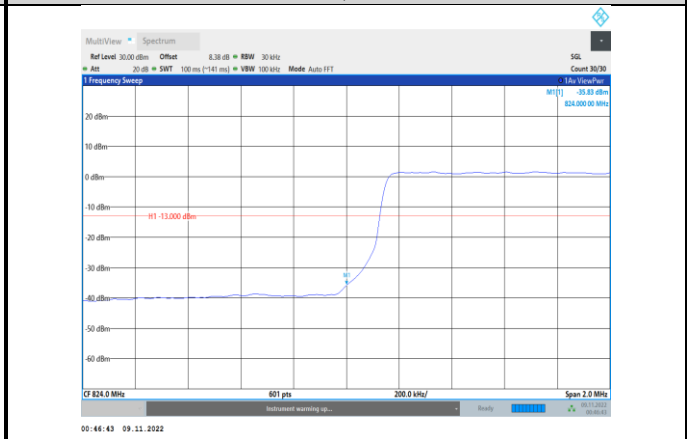
Band5-3MHz-16QAM-20415-15RB#0
