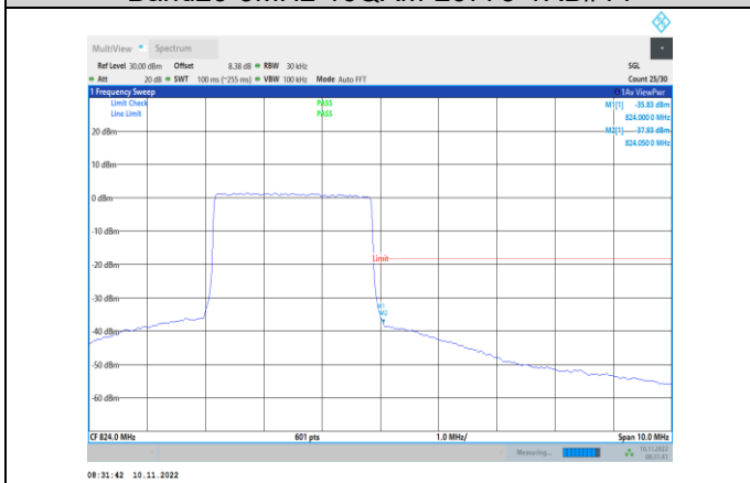
Band26-3MHz-16QAM-26775-15RB#0
