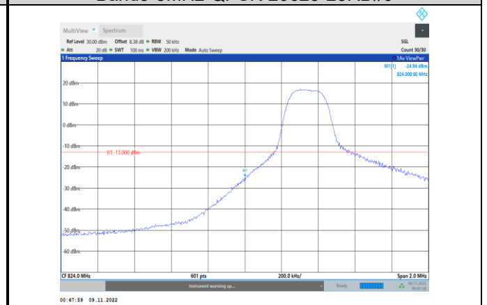
Band5-5MHz-16QAM-20425-1RB#0
