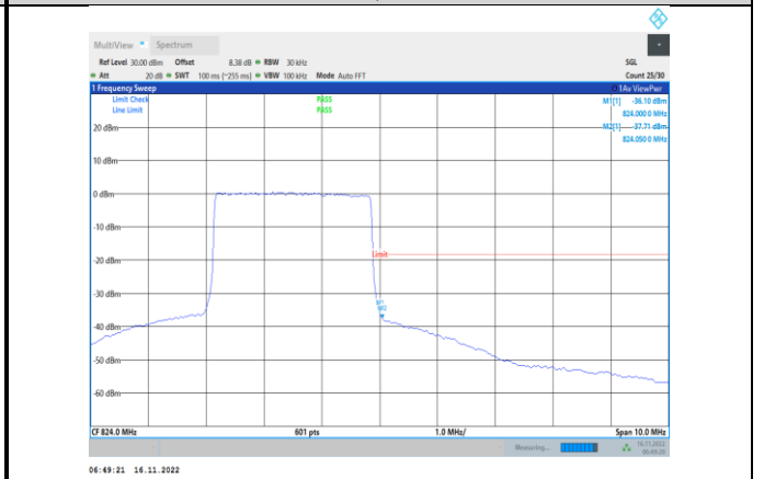
Band26-3MHz-64QAM-26775-15RB#0
