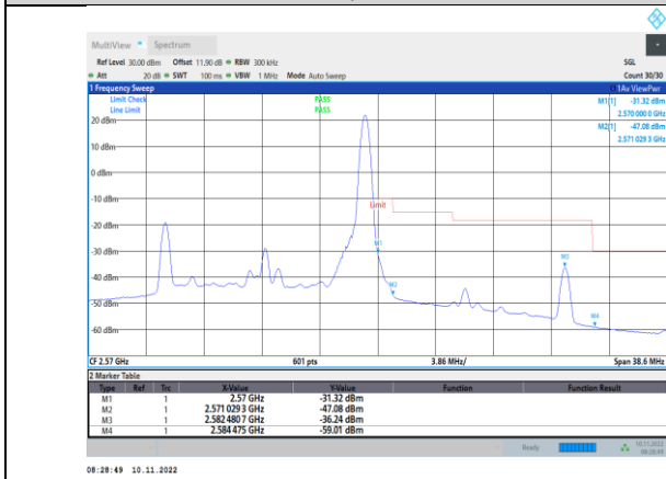
Band7-15MHz-QPSK-21375-1RB#74
