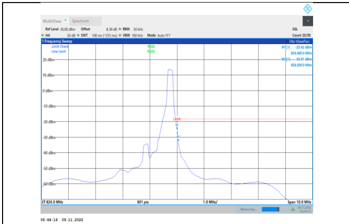
Band26-1.4MHz-16QAM-26783-1RB#5
