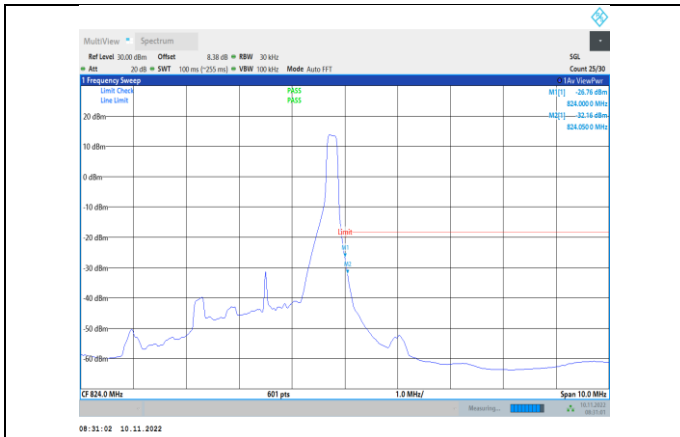
Band26-3MHz-16QAM-26775-1RB#14
