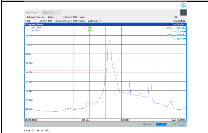
Band26-3MHz-64QAM-26705-1RB#0
