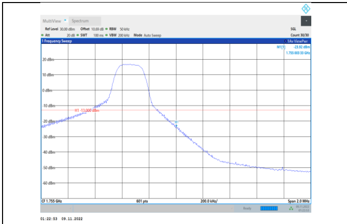
Band4-5MHz-16QAM-20375-1RB#24
