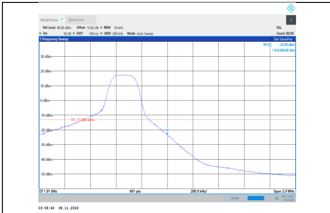
Band2-5MHz-16QAM-19175-1RB#24
