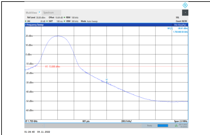
Band4-10MHz-16QAM-20350-1RB#49
