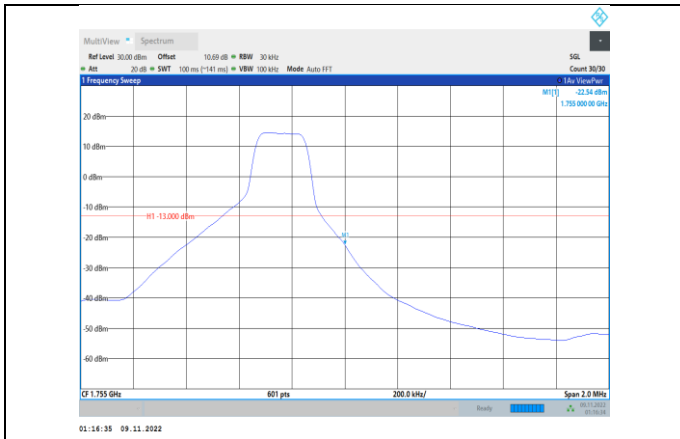
Band4-3MHz-16QAM-20385-1RB#14
