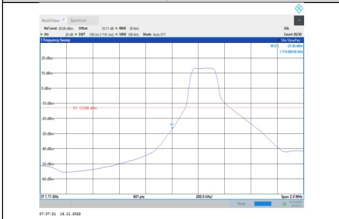
Band4-3MHz-64QAM-19965-1RB#0
