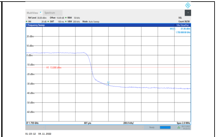
Band4-5MHz-QPSK-20375-25RB#0
