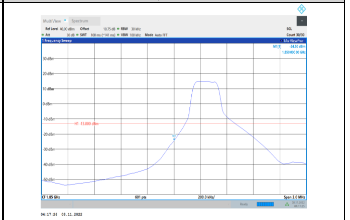
Band2-3MHz-16QAM-18615-1RB#0
