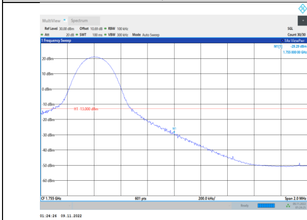
Band4-10MHz-QPSK-20350-1RB#49
