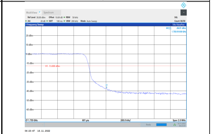
Band4-5MHz-64QAM-20375-25RB#0
