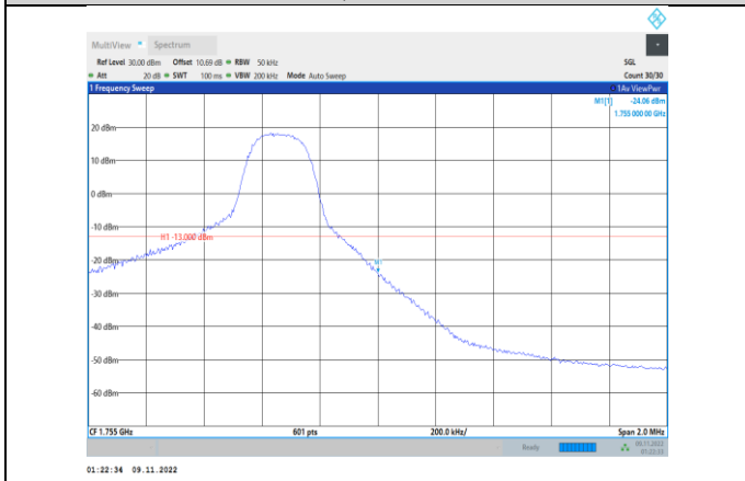
Band4-5MHz-QPSK-20375-1RB#24
