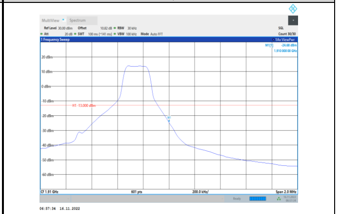
Band2-1.4MHz-64QAM-19193-1RB#5
