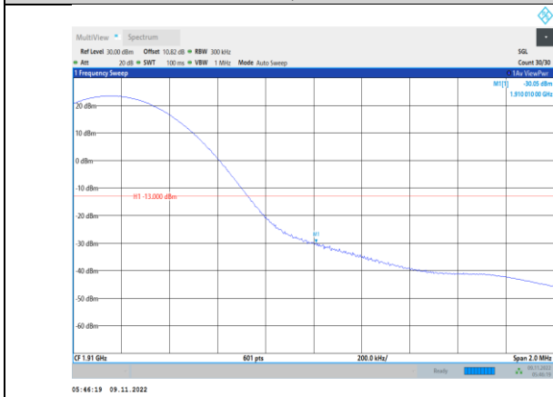
Band2-15MHz-QPSK-19125-1RB#74
