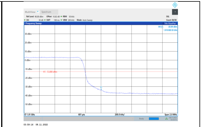
Band2-5MHz-QPSK-19175-25RB#0
