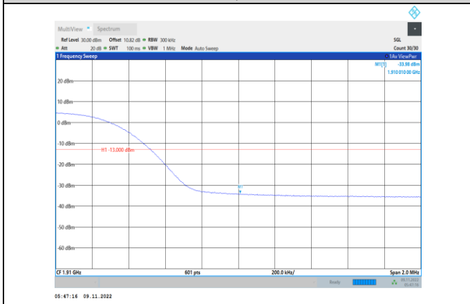
Band2-15MHz-16QAM-19125-75RB#0
