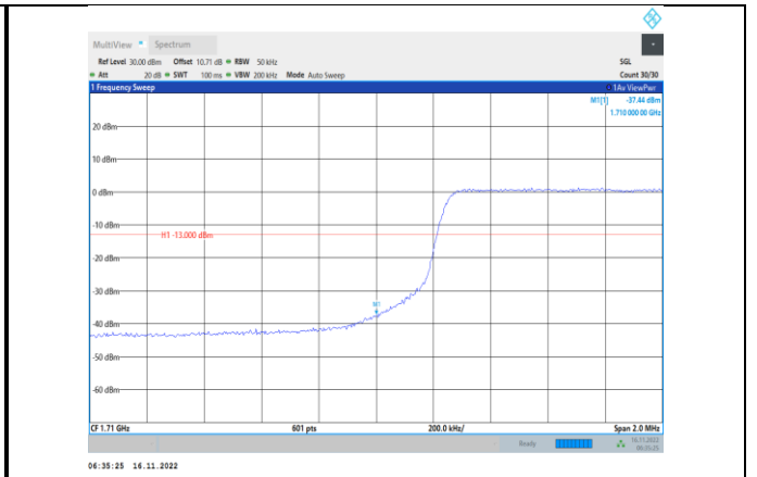
Band4-5MHz-64QAM-19975-25RB#0
