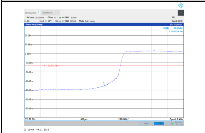
Band4-5MHz-QPSK-19975-25RB#0
