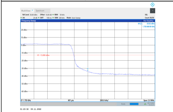
Band4-5MHz-16QAM-20375-25RB#0
