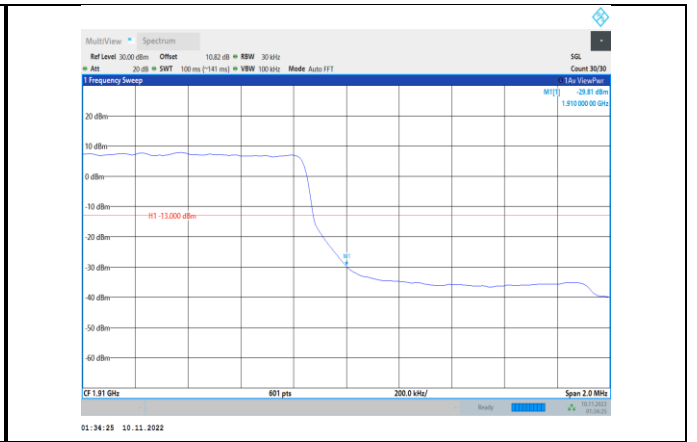
Band2-1.4MHz-QPSK-19193-6RB#0
