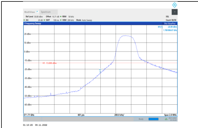
Band4-5MHz-QPSK-19975-1RB#0
