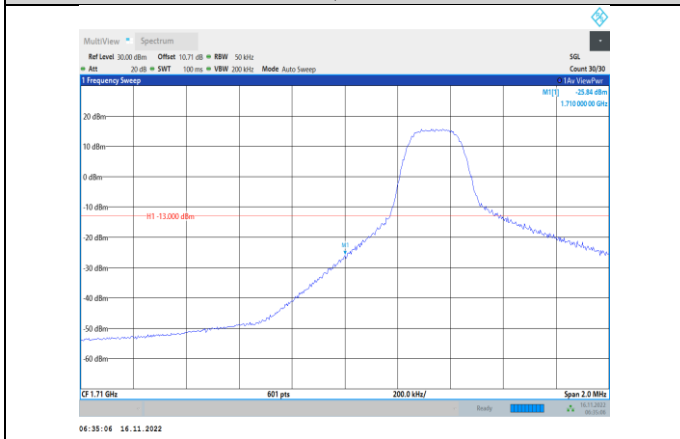
Band4-5MHz-64QAM-19975-1RB#0
