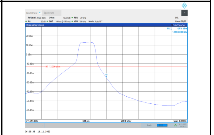
Band4-3MHz-64QAM-20385-1RB#14
