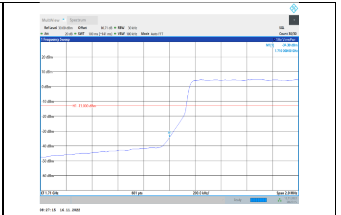
Band4-1.4MHz-64QAM-19957-6RB#0
