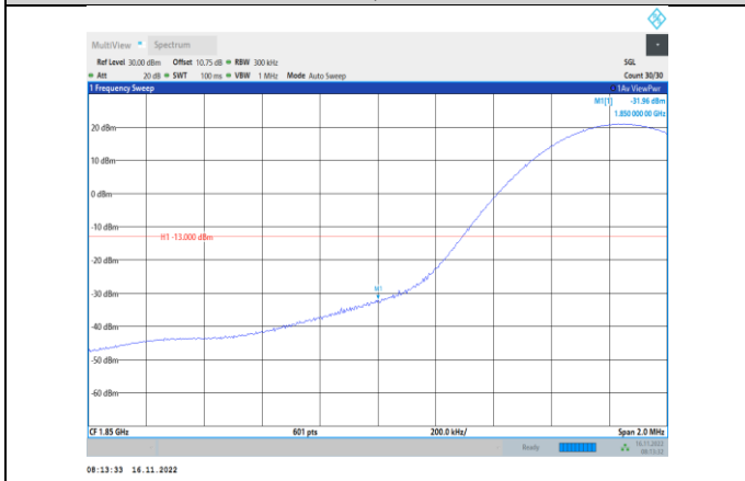
Band2-15MHz-64QAM-18675-1RB#0
