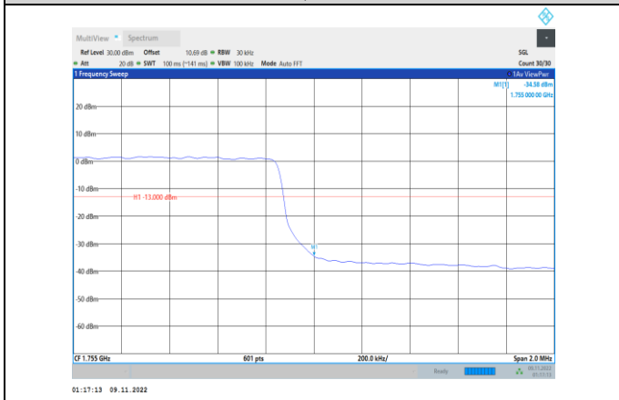
Band4-3MHz-16QAM-20385-15RB#0
