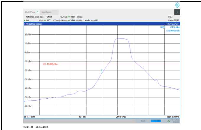
Band4-1.4MHz-QPSK-19957-1RB#0
