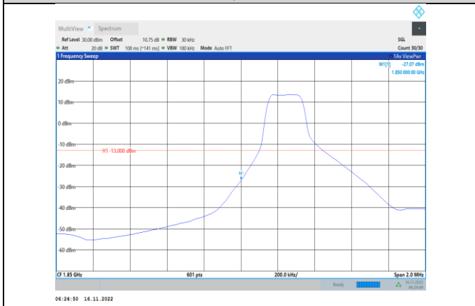
Band2-3MHz-64QAM-18615-1RB#0
