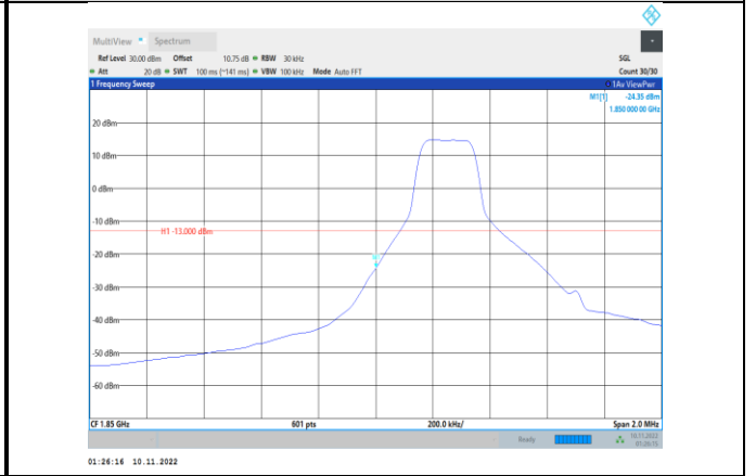
Band2-1.4MHz-16QAM-18607-1RB#0
