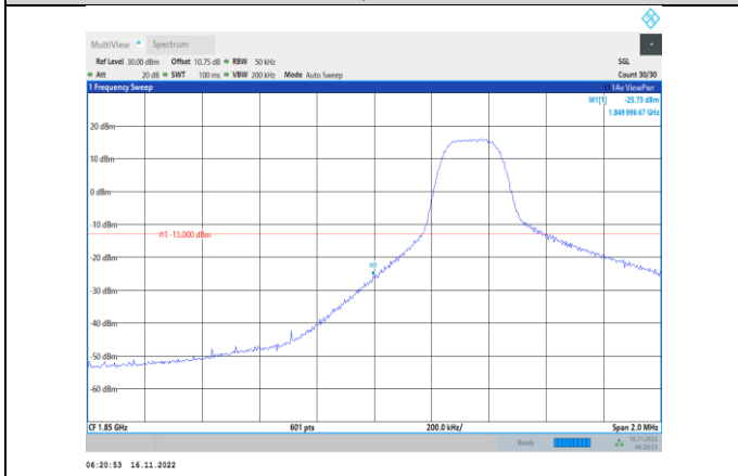
Band2-5MHz-64QAM-18625-1RB#0
