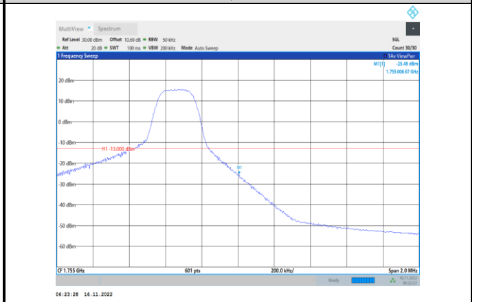
Band4-5MHz-64QAM-20375-1RB#24
