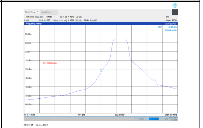
Band4-1.4MHz-16QAM-19957-1RB#0
