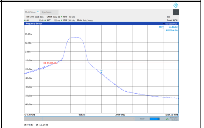
Band2-5MHz-64QAM-19175-1RB#24
