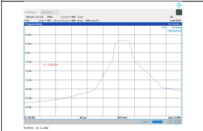
Band2-1.4MHz-64QAM-18607-1RB#0
