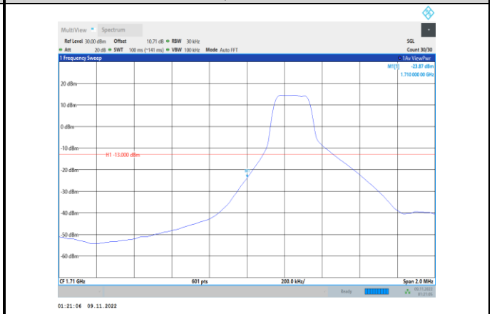
Band4-3MHz-16QAM-19965-1RB#0
