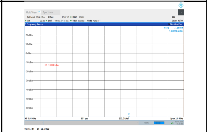
Band2-3MHz-64QAM-19185-15RB#0
