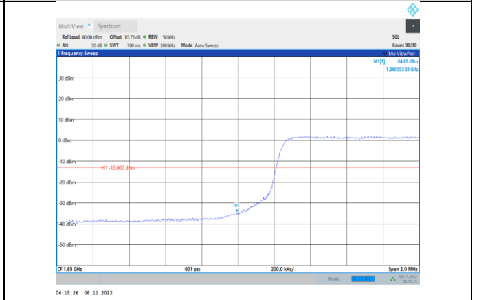
Band2-5MHz-16QAM-18625-25RB#0
