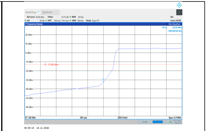
Band2-1.4MHz-64QAM-18607-6RB#0
