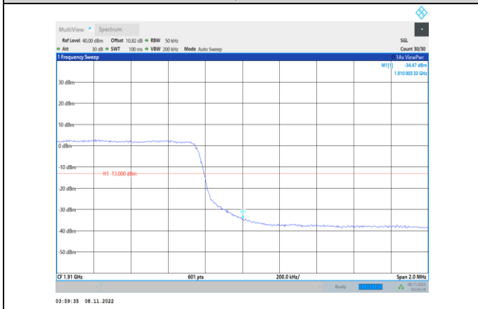
Band2-5MHz-16QAM-19175-25RB#0
