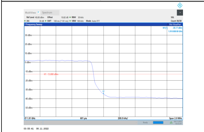
Band2-3MHz-16QAM-19185-15RB#0
