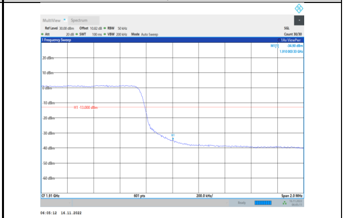
Band2-5MHz-64QAM-19175-25RB#0
