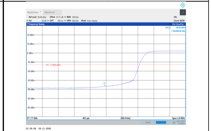
Band4-10MHz-16QAM-20000-50RB#0
