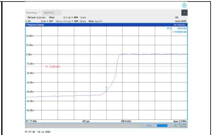
Band4-3MHz-64QAM-19965-15RB#0
