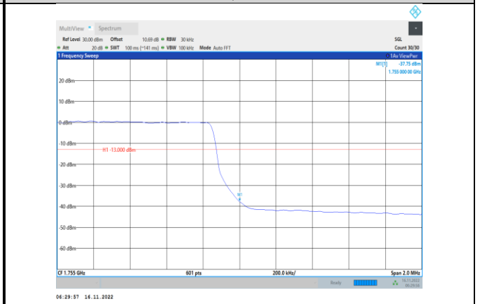
Band4-3MHz-64QAM-20385-15RB#0
