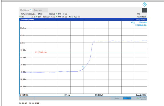
Band4-3MHz-QPSK-19965-15RB#0
