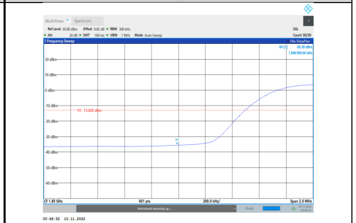
Band2-15MHz-16QAM-18675-75RB#0
