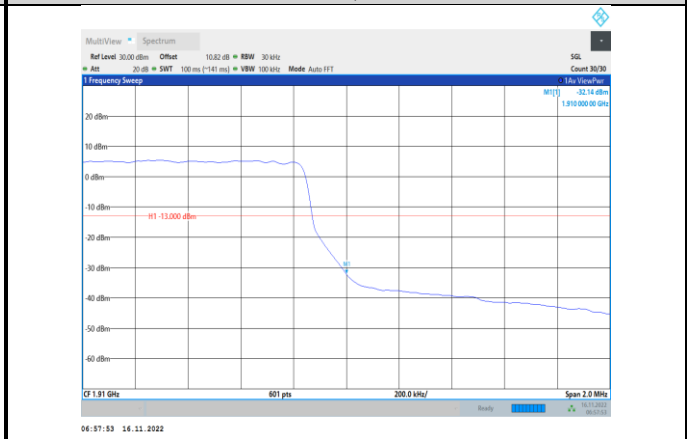
Band2-1.4MHz-64QAM-19193-6RB#0
