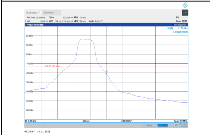
Band2-1.4MHz-QPSK-19193-1RB#5
