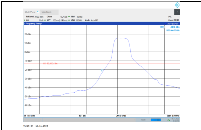
Band2-1.4MHz-QPSK-18607-1RB#0
