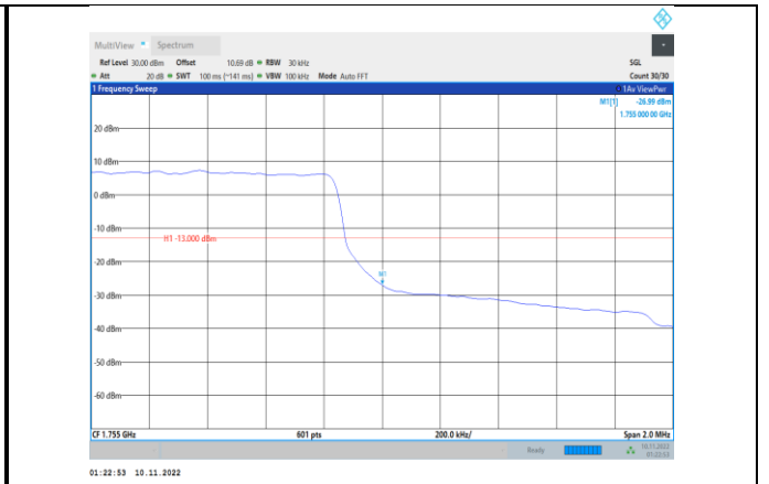
Band4-1.4MHz-QPSK-20393-6RB#0
