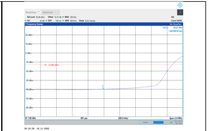
Band2-20MHz-64QAM-18700-100RB#0
