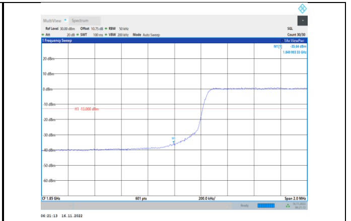
Band2-5MHz-64QAM-18625-25RB#0
