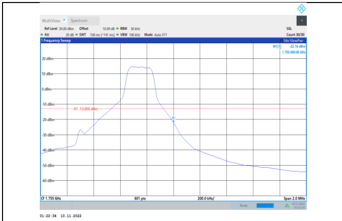
Band4-1.4MHz-16QAM-20393-1RB#5
