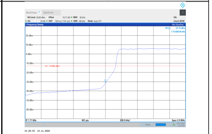
Band4-1.4MHz-16QAM-19957-6RB#0
