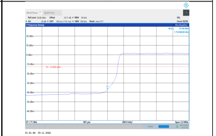
Band4-3MHz-16QAM-19965-15RB#0
