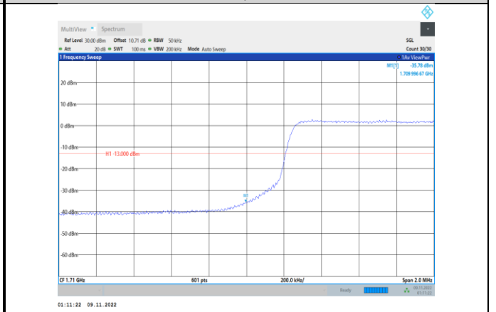
Band4-5MHz-16QAM-19975-25RB#0
