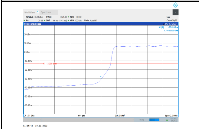
Band4-1.4MHz-QPSK-19957-6RB#0
