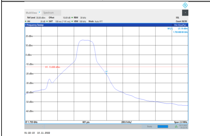
Band4-1.4MHz-QPSK-20393-1RB#5
