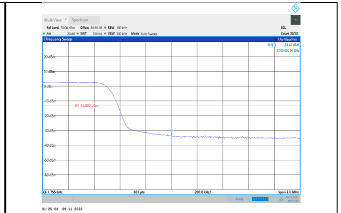
Band4-10MHz-QPSK-20350-50RB#0
