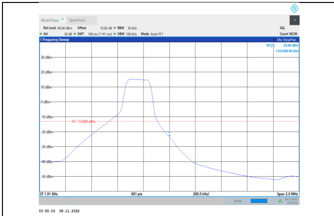
Band2-3MHz-16QAM-19185-1RB#14
