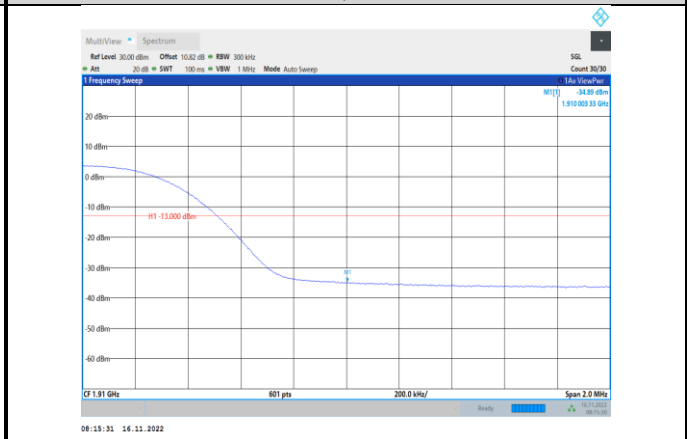
Band2-15MHz-64QAM-19125-75RB#0
