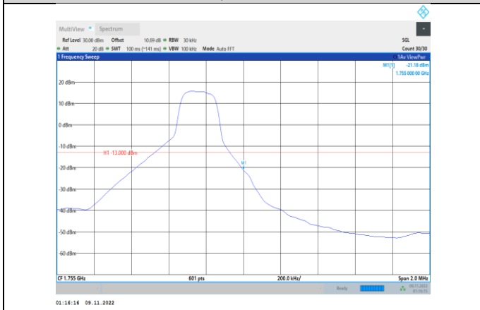
Band4-3MHz-QPSK-20385-1RB#14
