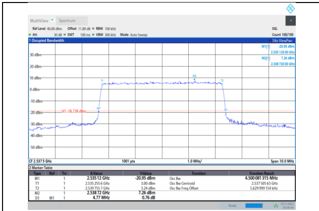
Band41-5MHz-64QAM-40065-25RB#0
