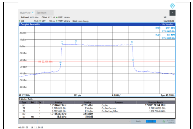
Band66-20MHz-64QAM-132072-100RB#0
