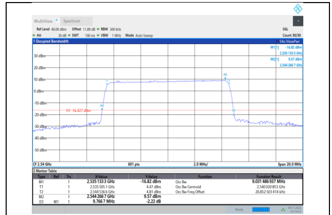
Band41-10MHz-QPSK-40090-50RB#0
