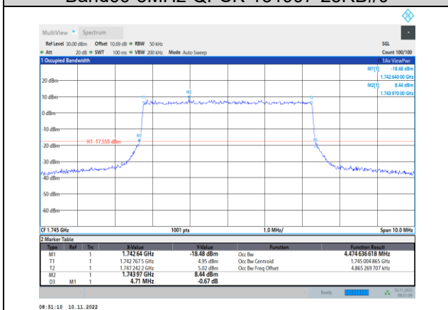
Band66-5MHz-QPSK-132322-25RB#0
