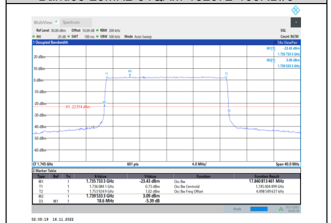
Band66-20MHz-64QAM-132322-100RB#0
