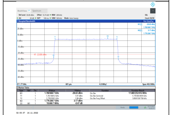
Band66-20MHz-64QAM-132572-100RB#0
