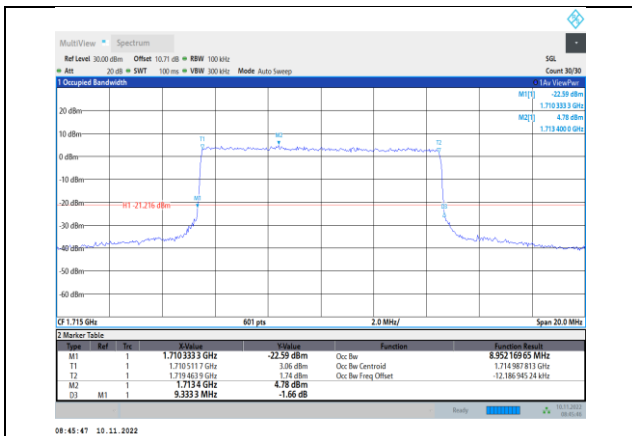
Band66-10MHz-16QAM-132022-50RB#0
