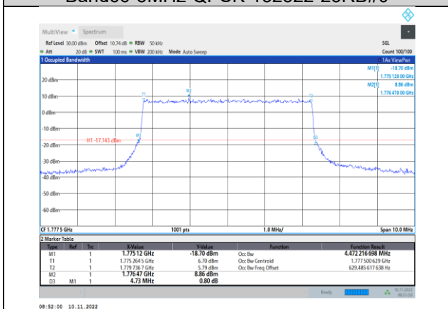
Band66-5MHz-QPSK-132647-25RB#0
