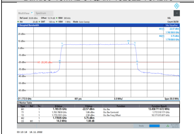
Band66-15MHz-64QAM-132597-75RB#0
