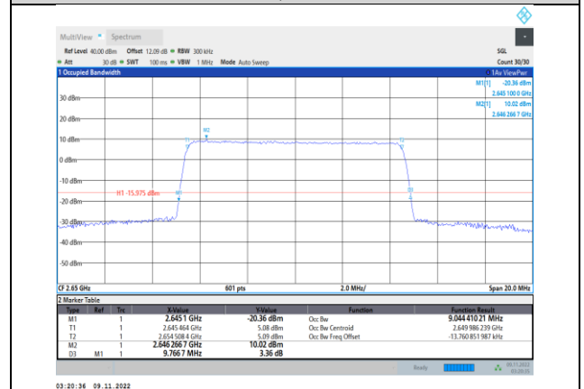
Band41-10MHz-QPSK-41190-50RB#0
