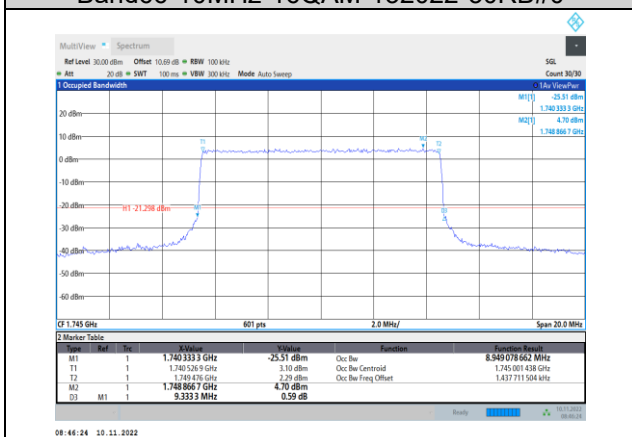
Band66-10MHz-16QAM-132322-50RB#0
