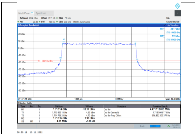
Band66-5MHz-QPSK-131997-25RB#0
