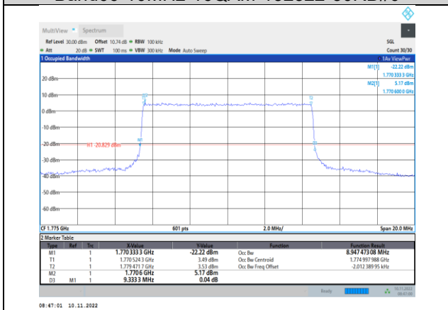
Band66-10MHz-16QAM-132622-50RB#0
