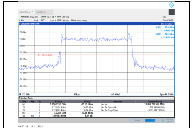
Band66-20MHz-QPSK-132072-100RB#0
