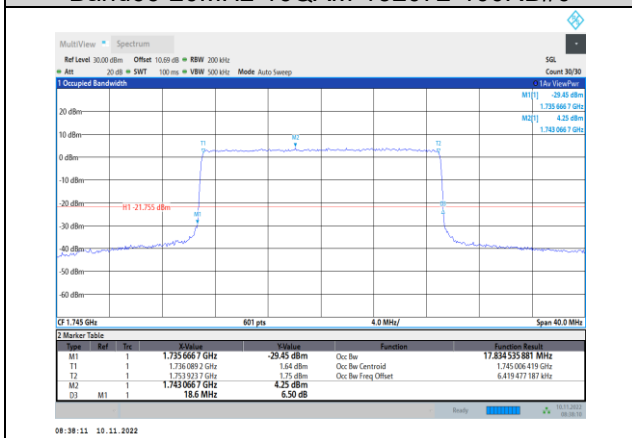
Band66-20MHz-16QAM-132322-100RB#0
