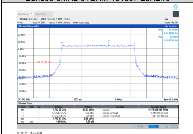
Band66-5MHz-64QAM-132322-25RB#0
