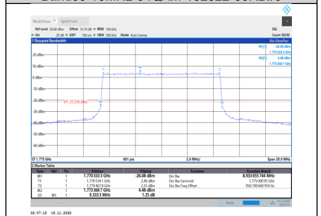
Band66-10MHz-64QAM-132622-50RB#0
