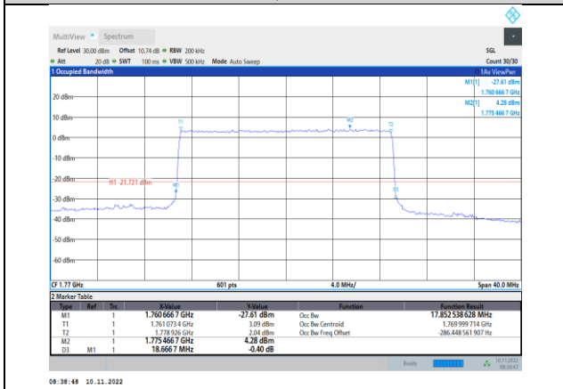
Band66-20MHz-16QAM-132572-100RB#0
