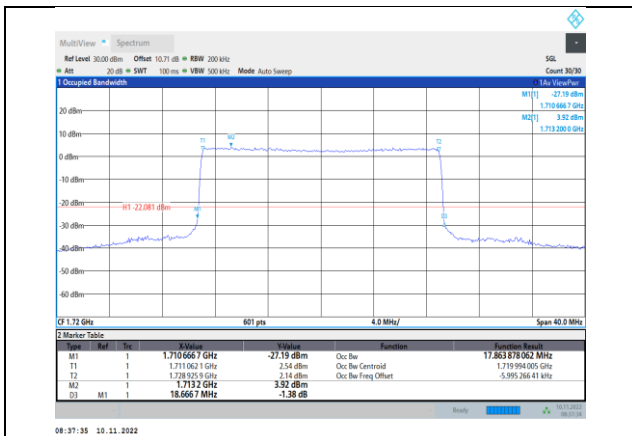
Band66-20MHz-16QAM-132072-100RB#0
