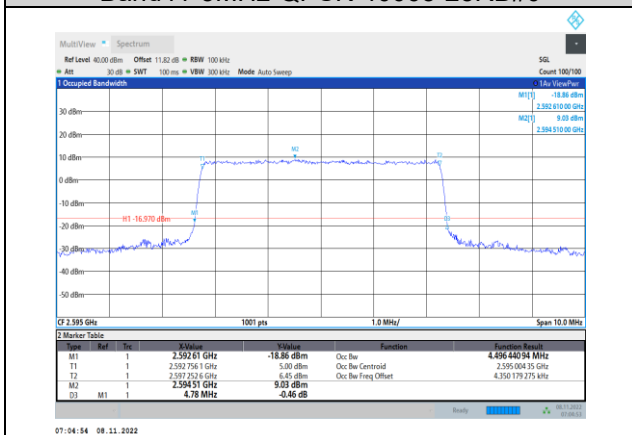
Band41-5MHz-QPSK-40640-25RB#0
