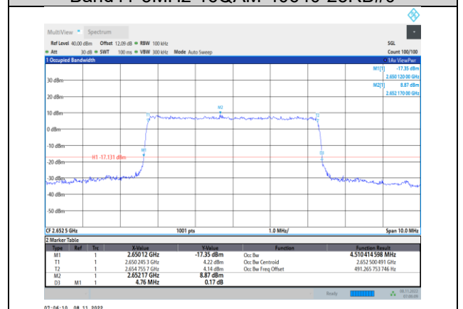
Band41-5MHz-16QAM-41215-25RB#0
