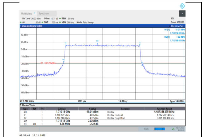
Band66-5MHz-16QAM-131997-25RB#0
