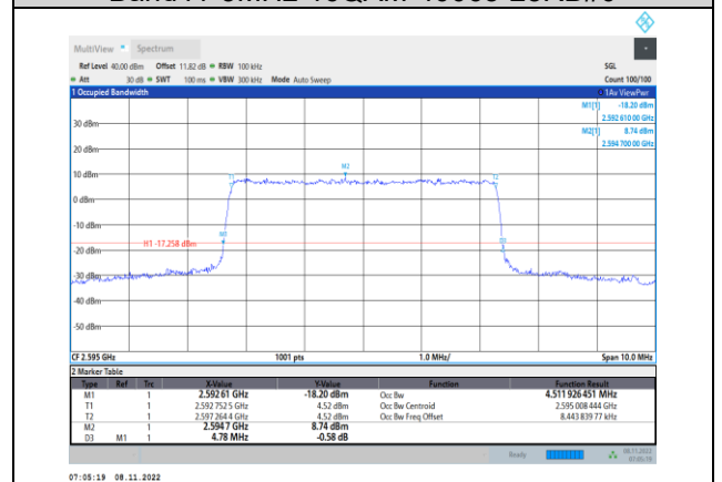
Band41-5MHz-16QAM-40640-25RB#0
