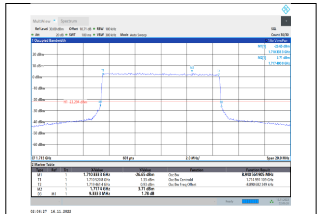
Band66-10MHz-64QAM-132022-50RB#0
