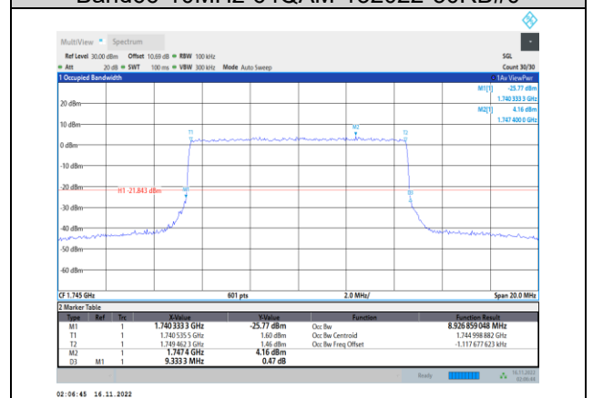
Band66-10MHz-64QAM-132322-50RB#0
