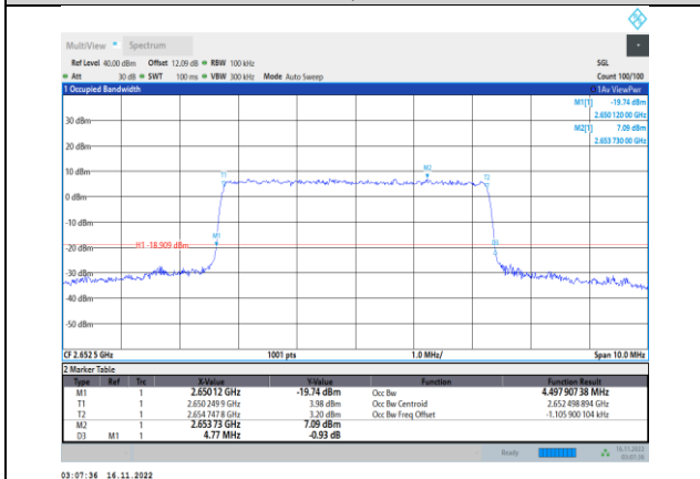
Band41-5MHz-64QAM-41215-25RB#0
