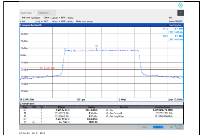
Band41-5MHz-16QAM-40065-25RB#0
