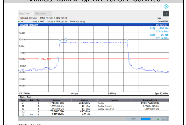
Band66-10MHz-QPSK-132622-50RB#0
