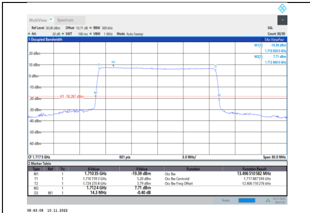
Band66-15MHz-QPSK-132047-75RB#0
