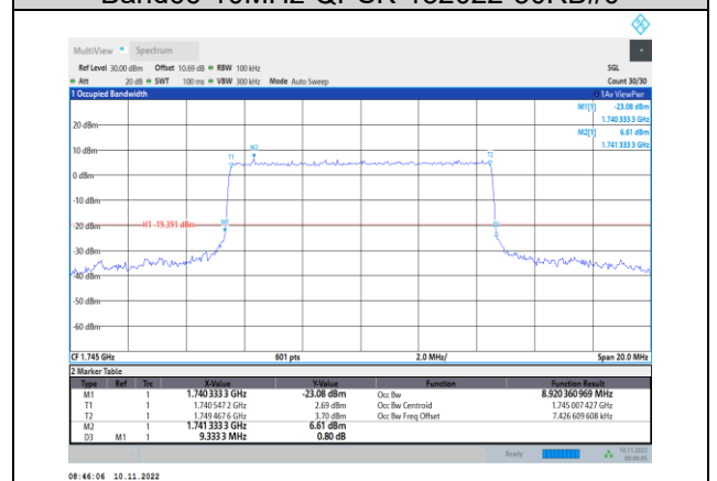
Band66-10MHz-QPSK-132322-50RB#0
