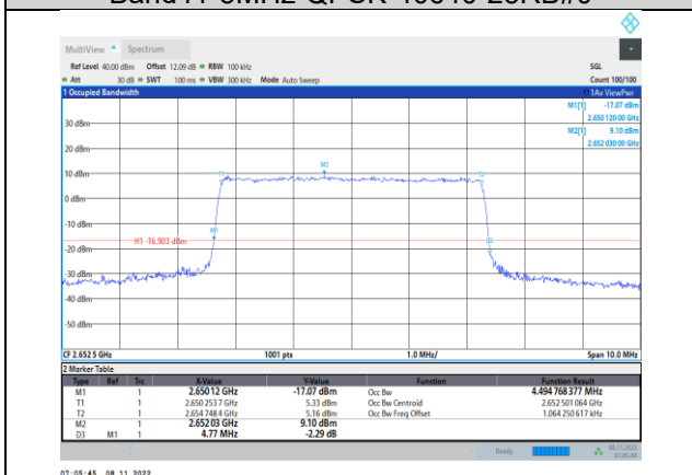
Band41-5MHz-QPSK-41215-25RB#0
