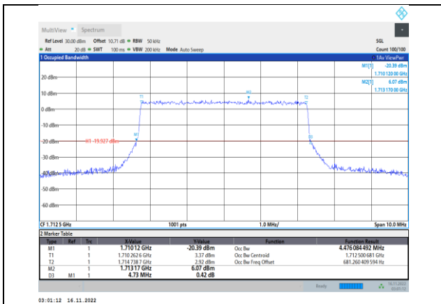
Band66-5MHz-64QAM-131997-25RB#0
