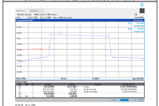
Band26-15MHz-16QAM-26765-75RB#0
