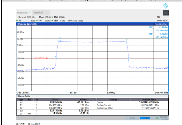
Band26-15MHz-QPSK-26865-75RB#0
