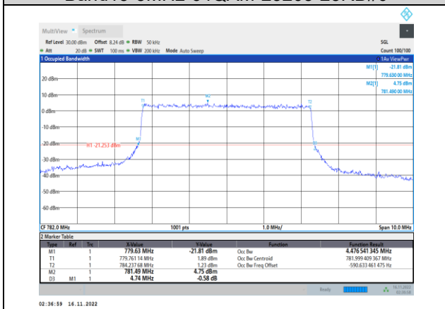
Band13-5MHz-64QAM-23230-25RB#0
