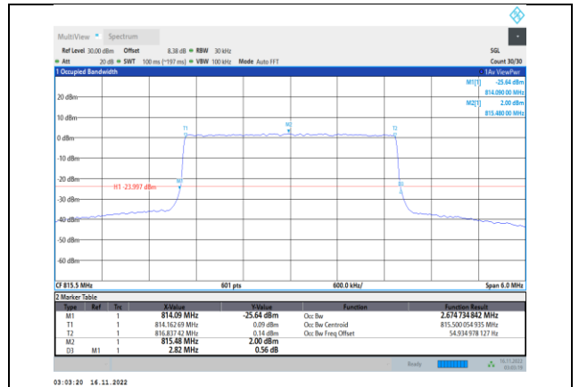
Band26-3MHz-64QAM-26705-15RB#0
