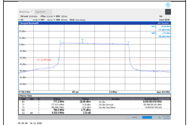
Band13-10MHz-64QAM-23230-50RB#0
