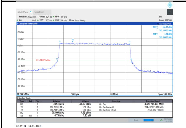
Band13-5MHz-64QAM-23255-25RB#0
