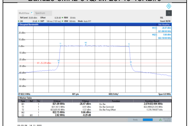
Band26-3MHz-64QAM-26775-15RB#0
