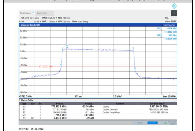
Band13-10MHz-16QAM-23230-50RB#0
