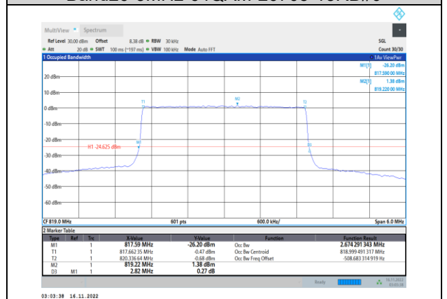
Band26-3MHz-64QAM-26740-15RB#0
