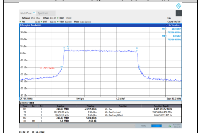
Band13-5MHz-16QAM-23255-25RB#0
