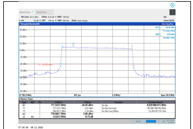
Band13-10MHz-QPSK-23230-50RB#0
