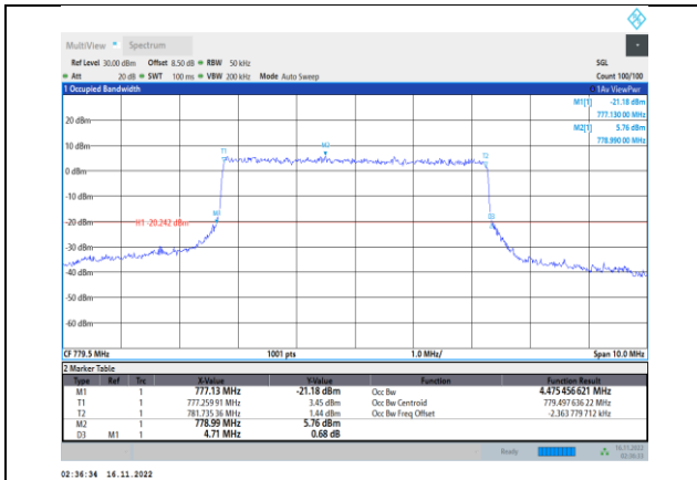
Band13-5MHz-64QAM-23205-25RB#0
