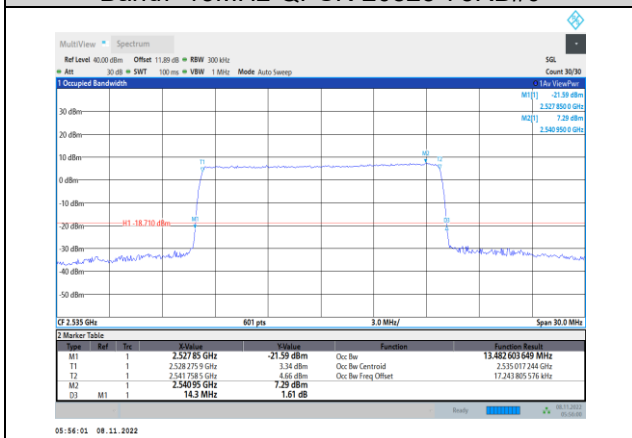
Band7-15MHz-QPSK-21100-75RB#0
