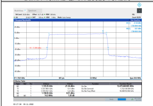
Band4-15MHz-QPSK-20175-75RB#0
