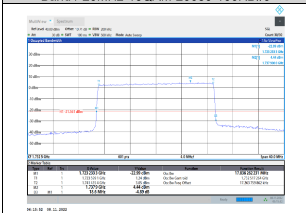
Band4-20MHz-16QAM-20175-100RB#0
