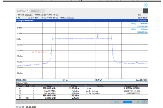
Band5-10MHz-64QAM-20525-50RB#0
