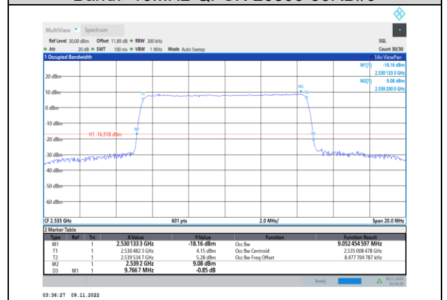
Band7-10MHz-QPSK-2100-50RB#0
