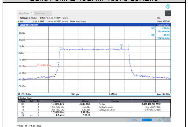
Band4-5MHz-16QAM-20175-25RB#0
