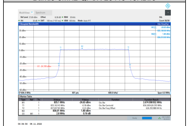
Band5-3MHz-QPSK-20525-15RB#0
