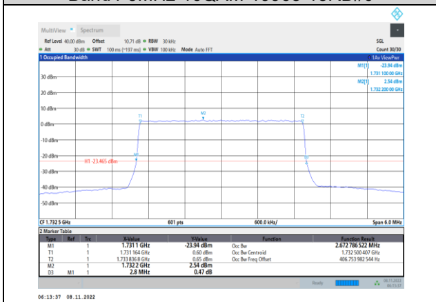
Band4-3MHz-16QAM-20175-15RB#0
