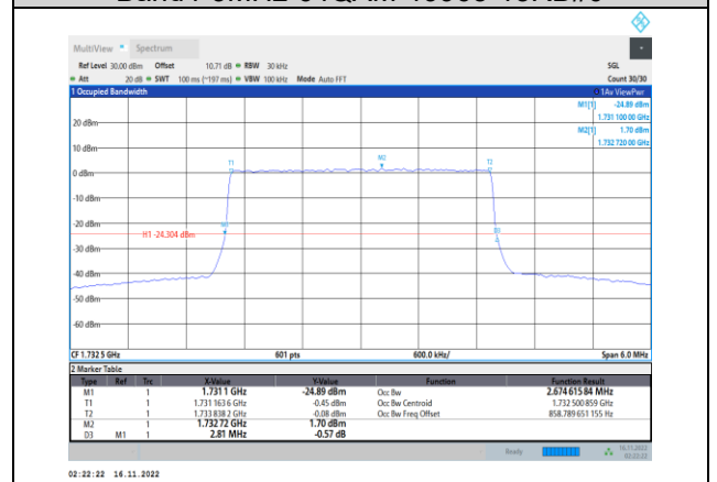
Band4-3MHz-64QAM-20175-15RB#0
