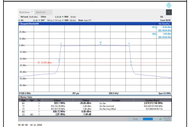
Band5-3MHz-64QAM-20525-15RB#0
