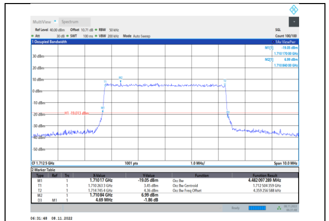
Band4-5MHz-16QAM-19975-25RB#0
