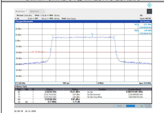
Band7-5MHz-64QAM-21100-25RB#0
