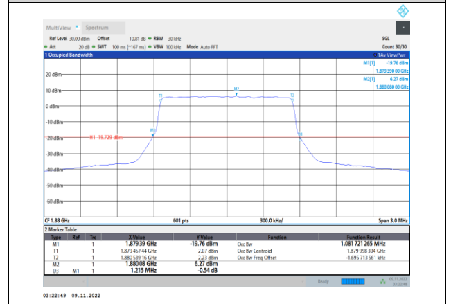
Band2-1.4MHz-16QAM-18900-6RB#0
