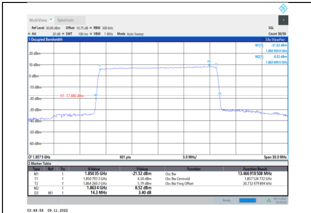
Band2-15MHz-QPSK-18675-75RB#0
