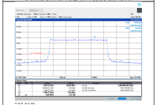
Band2-5MHz-16QAM-19175-25RB#0
