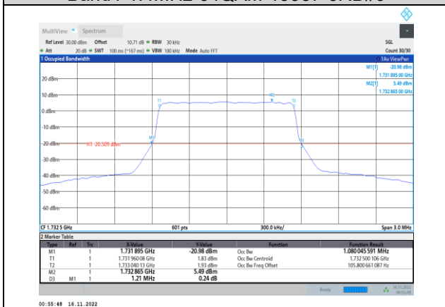
Band4-1.4MHz-64QAM-20175-6RB#0
