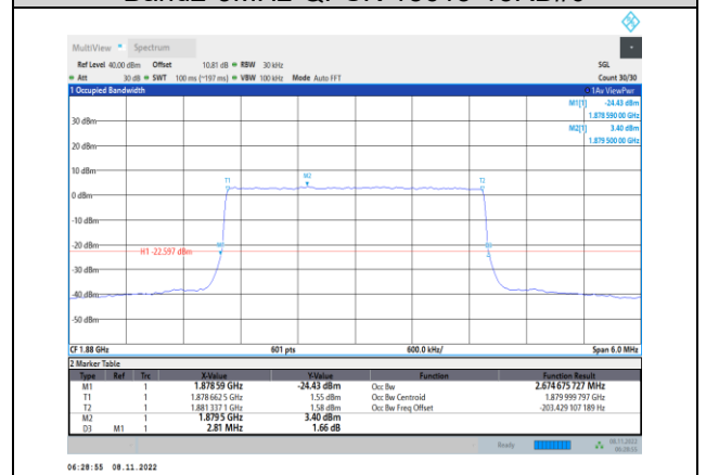
Band2-3MHz-QPSK-18900-15RB#0
