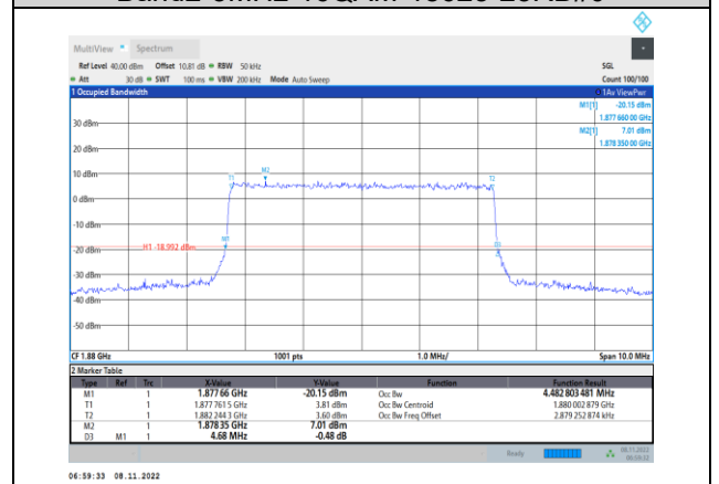
Band2-5MHz-16QAM-18900-25RB#0
