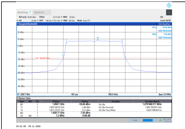
Band2-1.4MHz-QPSK-18607-6RB#0
