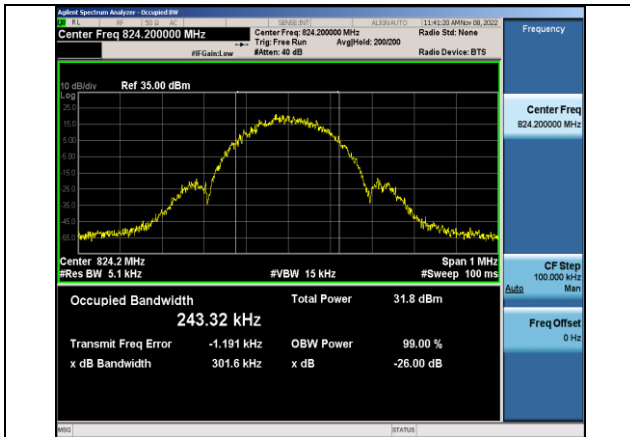
EGPRS850-128-8-0.3016
