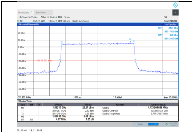
Band2-5MHz-64QAM-18625-25RB#0
