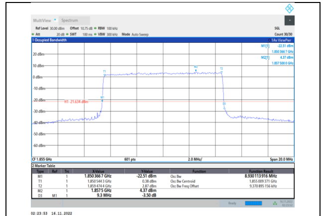
Band2-10MHz-64QAM-18650-50RB#0
