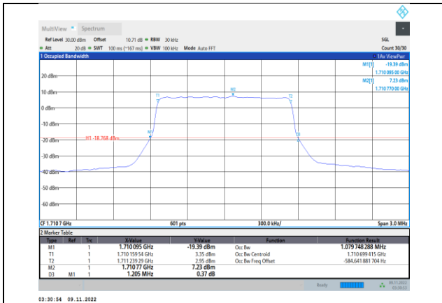
Band4-1.4MHz-QPSK-19957-6RB#0
