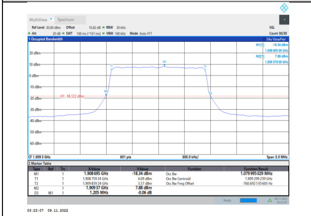
Band2-1.4MHz-QPSK-19193-6RB#0
