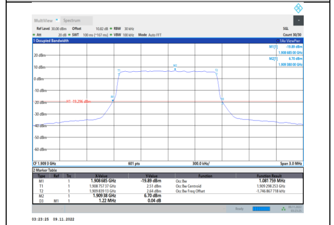
Band2-1.4MHz-16QAM-19193-6RB#0
