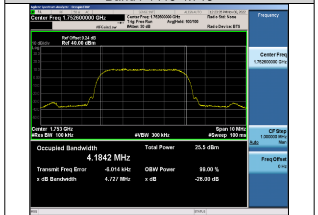
Band4-1513-4.727
