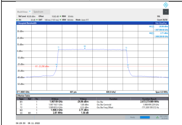
Band2-3MHz-16QAM-19185-15RB#0
