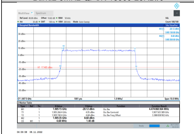
Band2-5MHz-QPSK-19175-25RB#0
