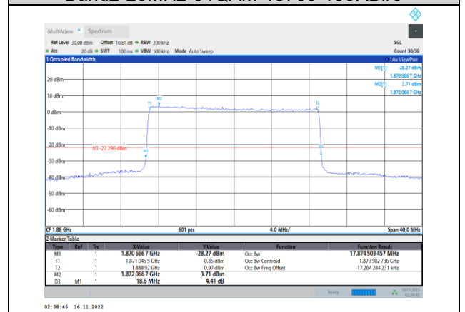
Band2-20MHz-64QAM-18900-100RB#0
