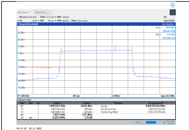
Band2-10MHz-16QAM-18650-50RB#0
