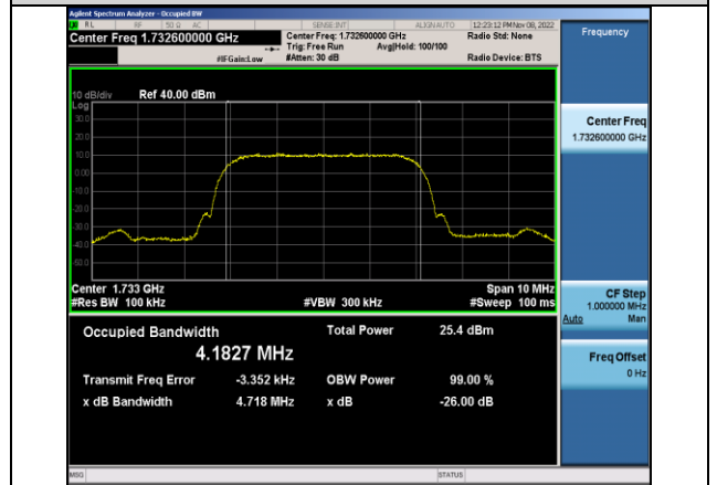
Band4-1413-4.718
