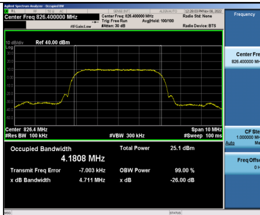
Band5-4132-4.711
