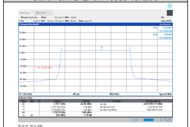
Band4-3MHz-QPSK-20175-15RB#0
