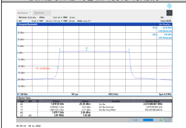
Band2-3MHz-16QAM-18900-15RB#0
