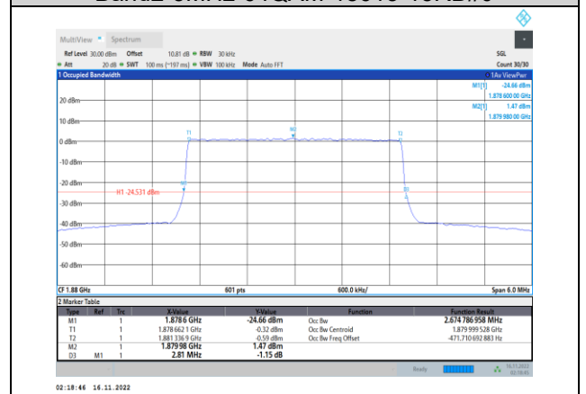
Band2-3MHz-64QAM-18900-15RB#0
