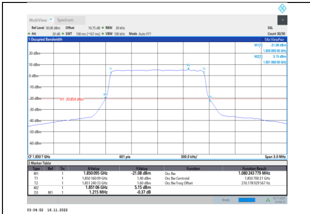
Band2-1.4MHz-64QAM-18607-6RB#0
