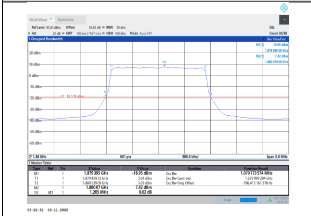
Band2-1.4MHz-QPSK-18900-6RB#0
