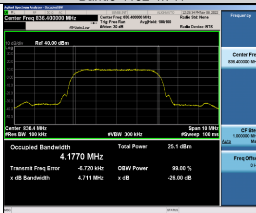
Band5-4182-4.711
