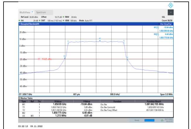
Band2-1.4MHz-16QAM-18607-6RB#0
