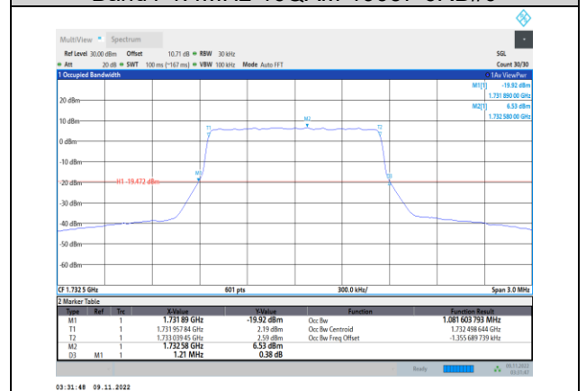
Band4-1.4MHz-16QAM-20175-6RB#0
