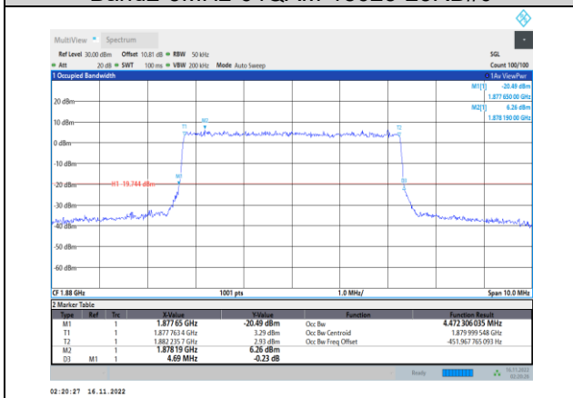
Band2-5MHz-64QAM-18900-25RB#0
