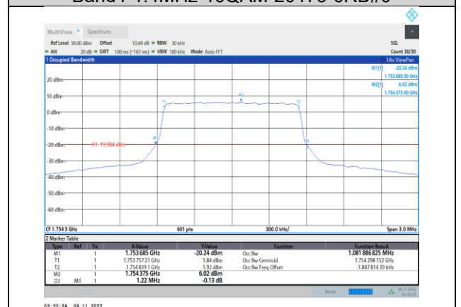
Band4-1.4MHz-16QAM-20393-6RB#0
