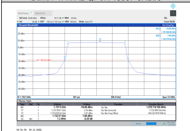
Band4-1.4MHz-QPSK-20175-6RB#0
