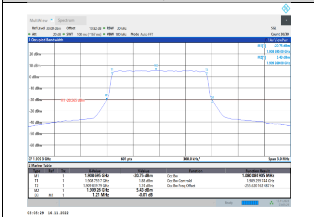
Band2-1.4MHz-64QAM-19193-6RB#0
