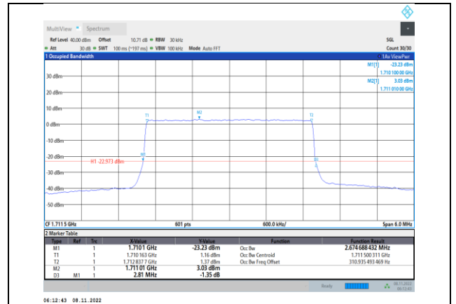
Band4-3MHz-QPSK-19965-15RB#0
