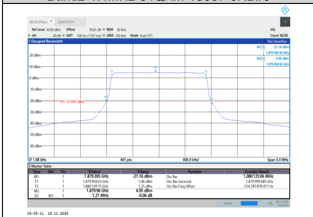
Band2-1.4MHz-64QAM-18900-6RB#0
