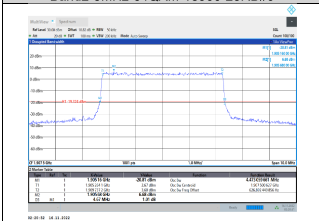
Band2-5MHz-64QAM-19175-25RB#0
