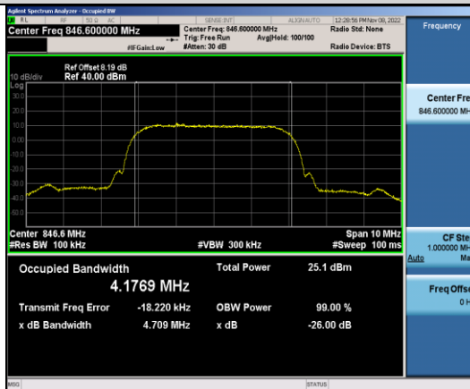
Band5-4233-4.709
