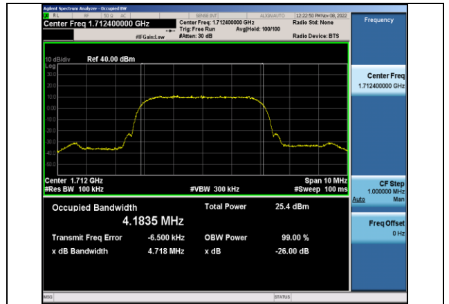
Band4-1312-4.718
