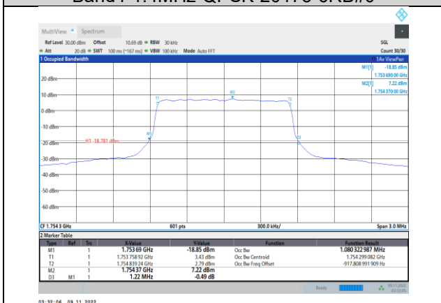
Band4-1.4MHz-QPSK-20393-6RB#0
