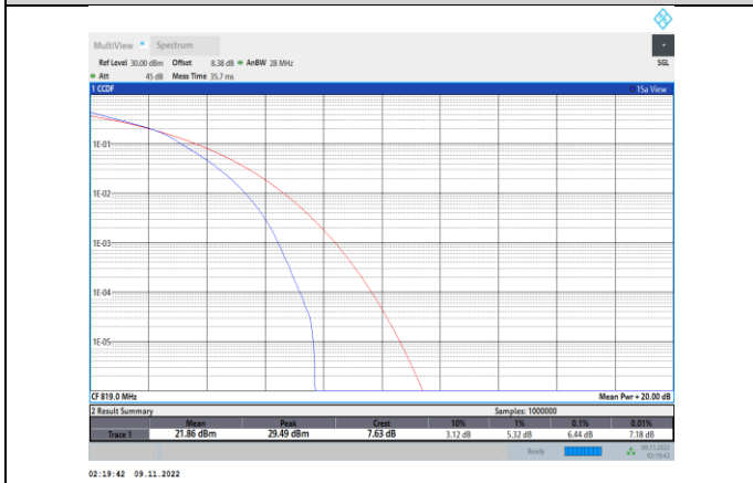
Band26-3MHz-16QAM-26740-15RB#0
