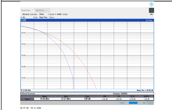
Band7-20MHz-16QAM-21100-100RB#0
