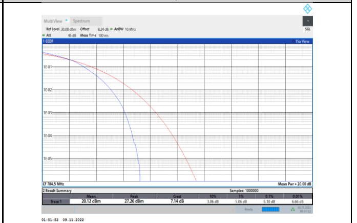
Band13-5MHz-16QAM-23255-25RB#0
