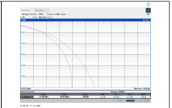
Band26-3MHz-64QAM-26705-15RB#0
