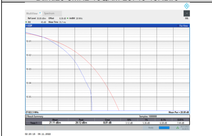
Band26-3MHz-16QAM-26775-15RB#0
