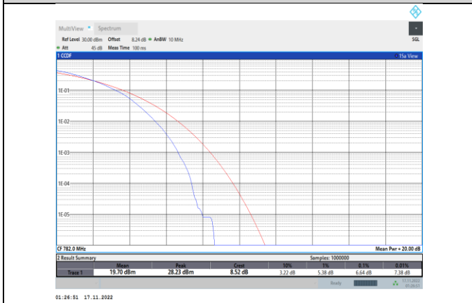
Band13-5MHz-64QAM-23230-25RB#0
