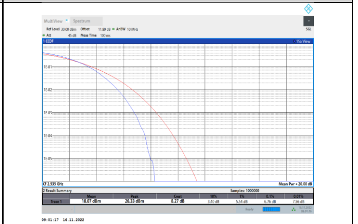
Band7-20MHz-64QAM-21100-100RB#0
