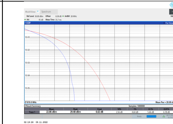
Band26-3MHz-QPSK-26740-15RB#0
