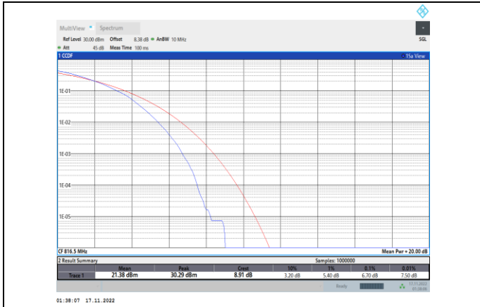
Band26-5MHz-64QAM-26715-25RB#0
