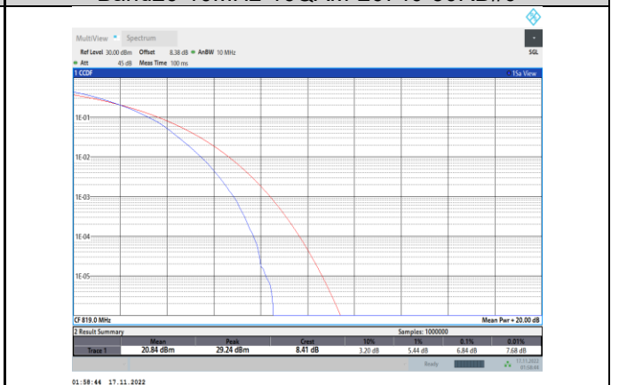
Band26-10MHz-64QAM-26740-50RB#0
