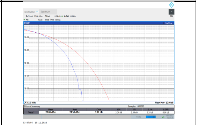
Band13-10MHz-16QAM-23230-50RB#0
