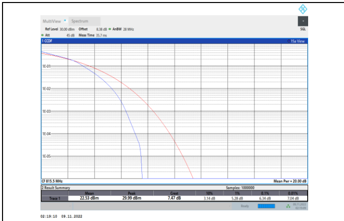
Band26-3MHz-16QAM-26705-15RB#0
