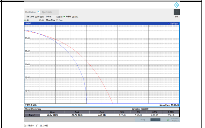
Band26-3MHz-64QAM-26740-15RB#0
