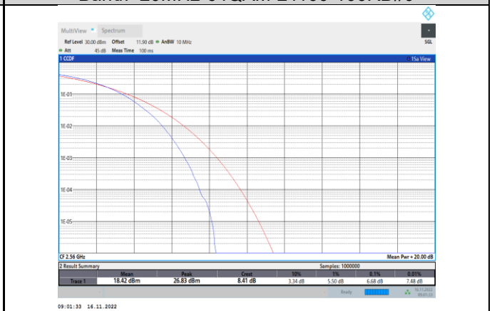
Band7-20MHz-64QAM-21350-100RB#0
