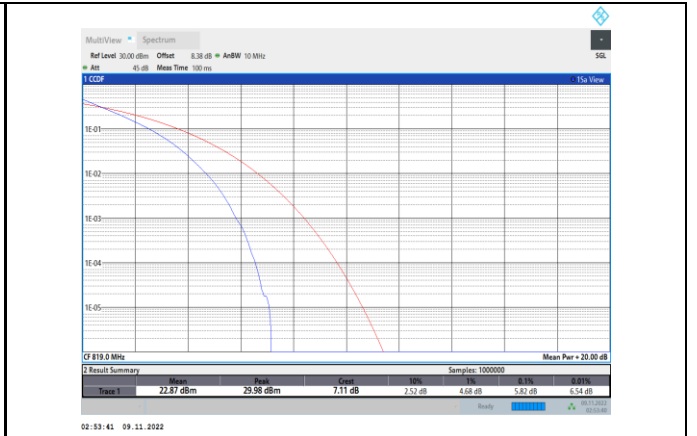
Band26-10MHz-QPSK-26740-50RB#0
