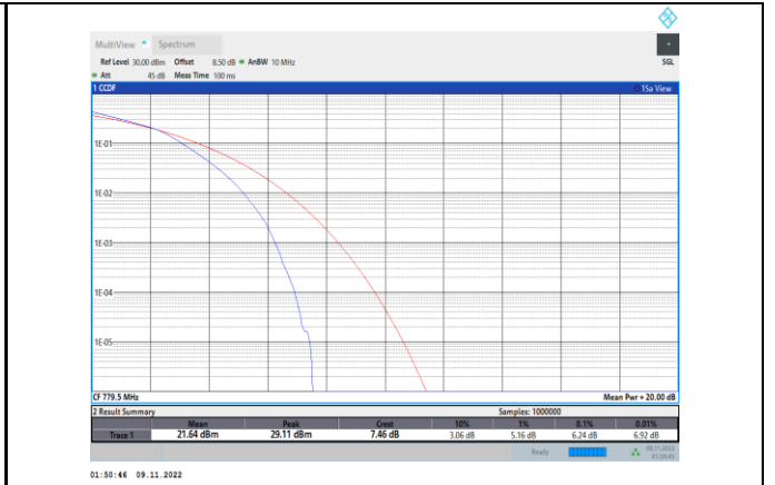
Band13-5MHz-16QAM-23205-25RB#0
