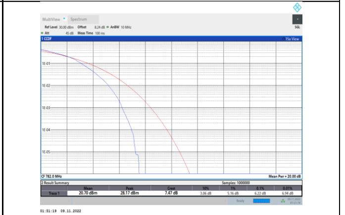
Band13-5MHz-16QAM-23230-25RB#0
