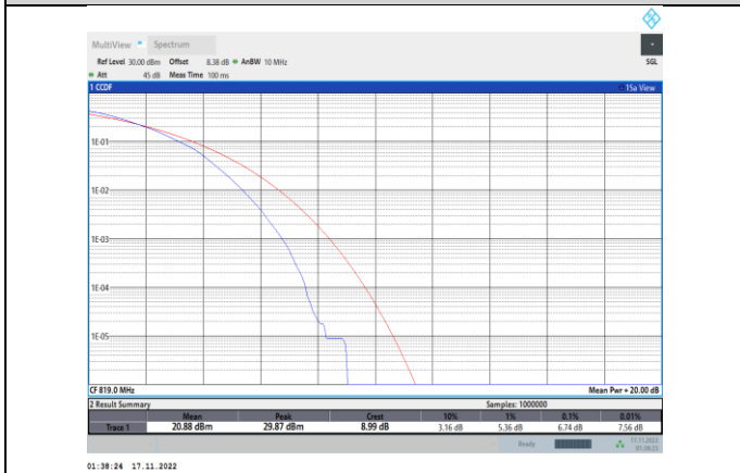
Band26-5MHz-64QAM-26740-25RB#0
