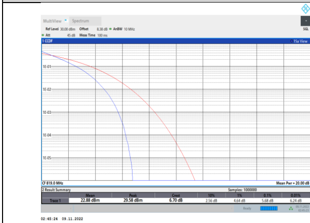
Band26-5MHz-QPSK-26740-25RB#0
