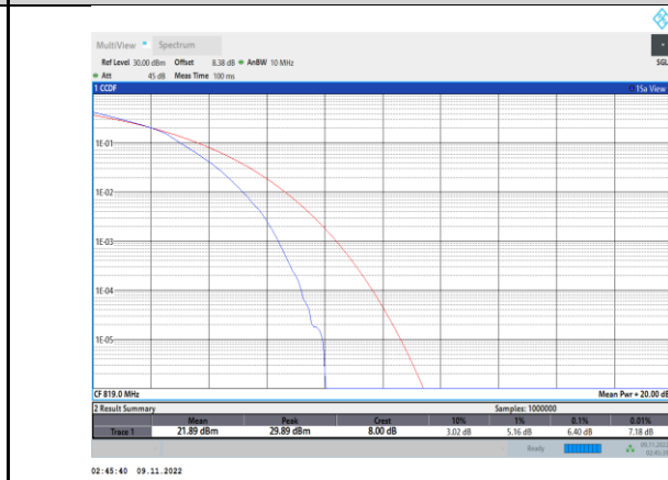
Band26-5MHz-16QAM-26740-25RB#0
