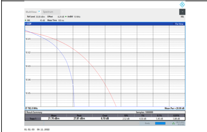
Band13-5MHz-QPSK-23230-25RB#0
