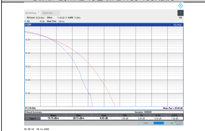
Band7-20MHz-16QAM-21350-100RB#0
