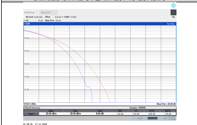
Band26-5MHz-64QAM-26765-25RB#0
