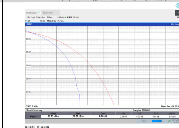
Band26-3MHz-QPSK-26775-15RB#0
