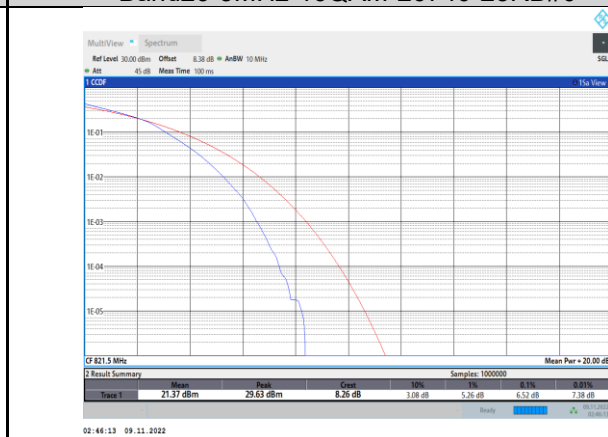
Band26-5MHz-16QAM-26765-25RB#0
