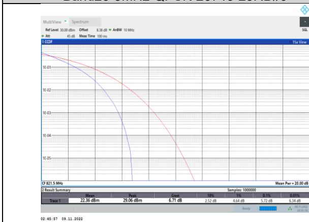
Band26-5MHz-QPSK-26765-25RB#0
