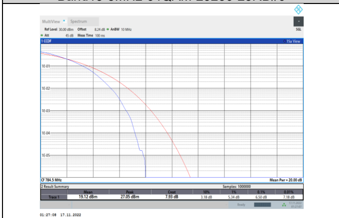
Band13-5MHz-64QAM-23255-25RB#0
