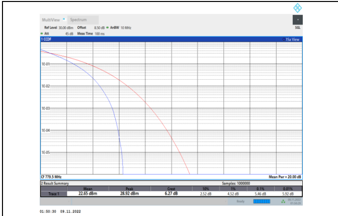
Band13-5MHz-QPSK-23205-25RB#0
