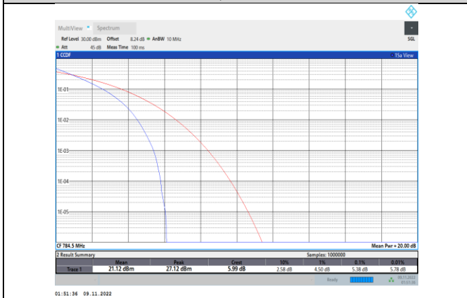
Band13-5MHz-QPSK-23255-25RB#0
