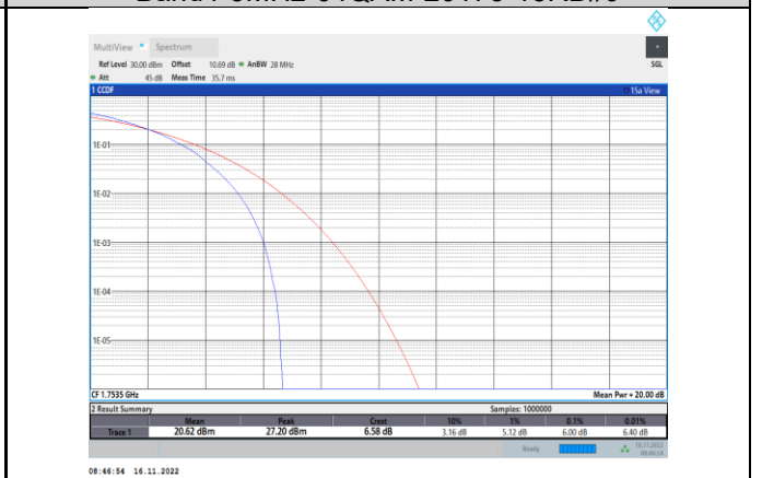
Band4-3MHz-64QAM-20385-15RB#0
