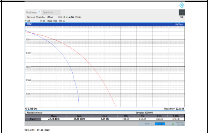
Band7-10MHz-QPSK-21100-50RB#0
