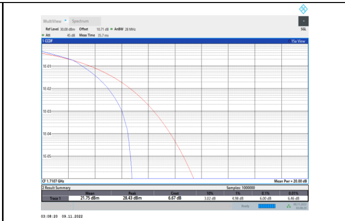
Band4-1.4MHz-16QAM-19957-6RB#0
