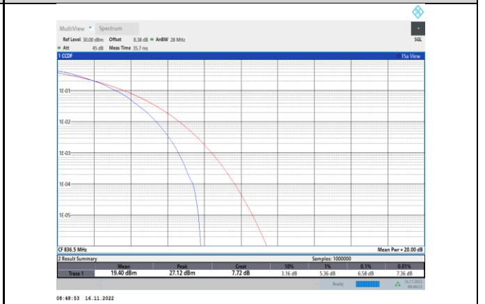
Band5-3MHz-64QAM-20525-15RB#0
