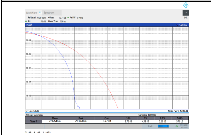
Band4-15MHz-QPSK-20175-75RB#0
