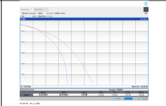
Band4-1.4MHz-16QAM-20175-6RB#0
