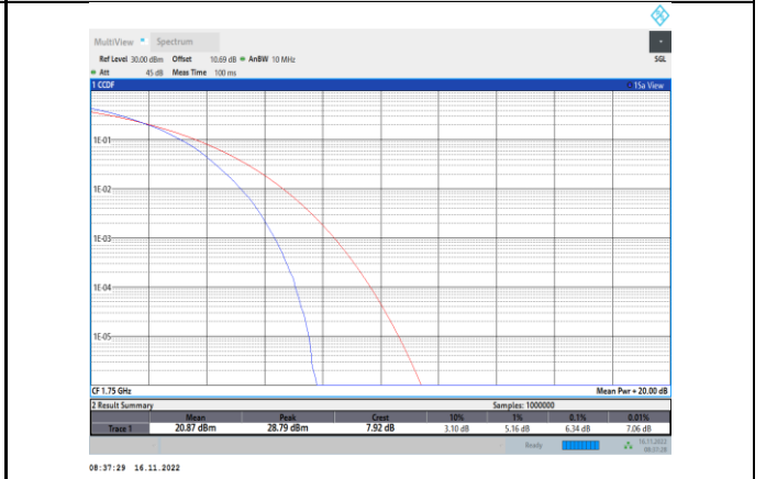
Band4-10MHz-64QAM-20350-50RB#0
