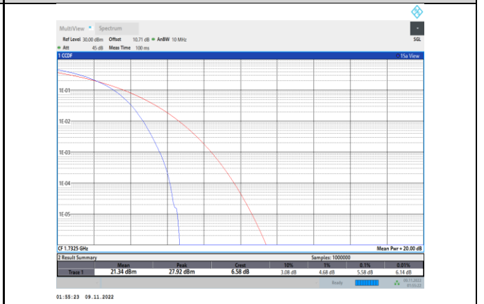
Band4-20MHz-QPSK-20175-100RB#0
