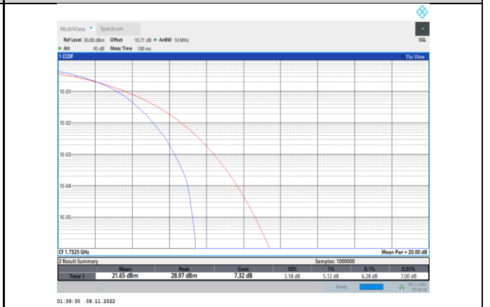
Band4-15MHz-16QAM-20175-75RB#0
