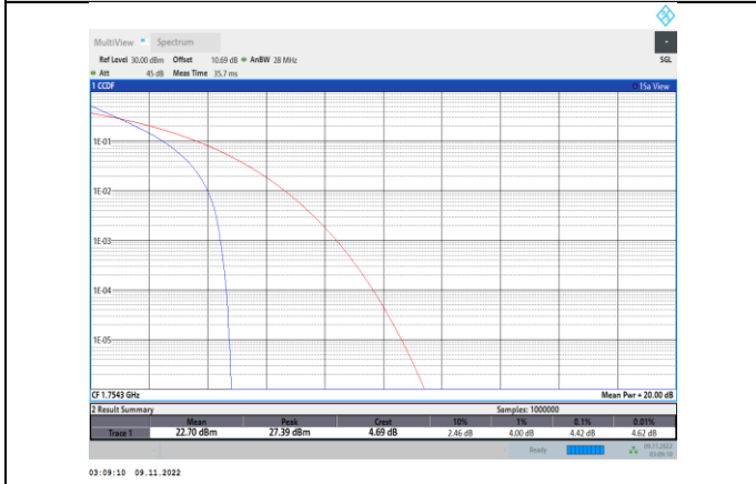
Band4-1.4MHz-QPSK-20393-6RB#0
