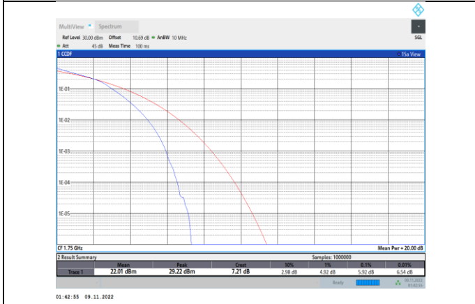
Band4-10MHz-16QAM-20350-50RB#0
