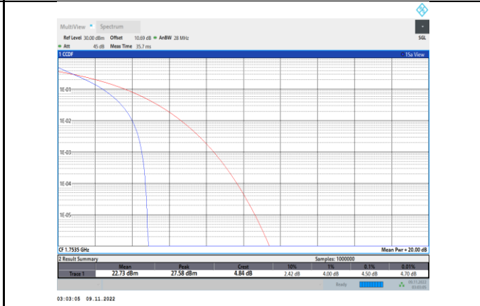
Band4-3MHz-QPSK-20385-15RB#0
