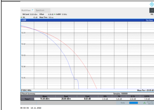
Band5-5MHz-64QAM-20525-25RB#0
