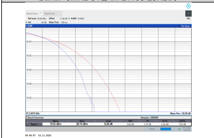
Band7-5MHz-64QAM-21425-25RB#0
