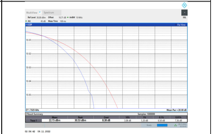
Band4-5MHz-16QAM-20175-25RB#0
