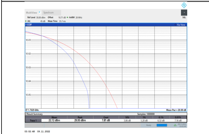
Band4-3MHz-16QAM-20175-15RB#0
