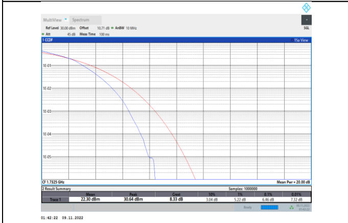
Band4-10MHz-16QAM-20175-50RB#0
