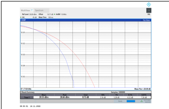
Band4-5MHz-64QAM-19975-25RB#0
