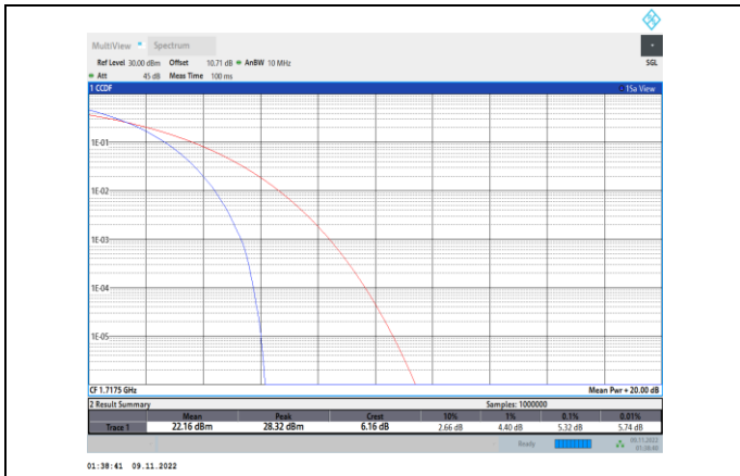
Band4-15MHz-QPSK-20025-75RB#0
