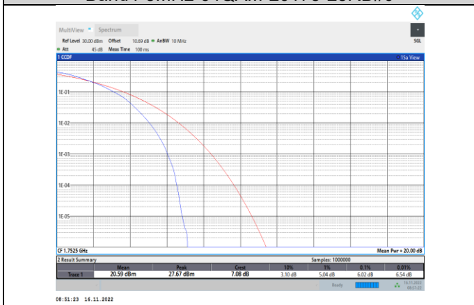
Band4-5MHz-64QAM-20375-25RB#0
