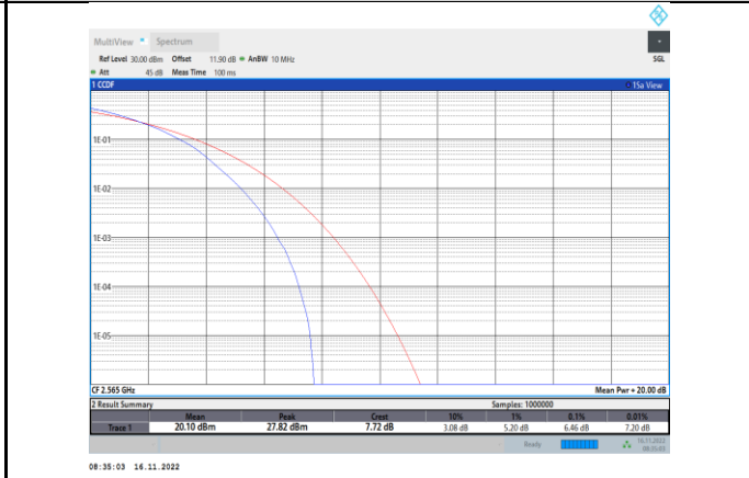
Band7-10MHz-64QAM-21400-50RB#0
