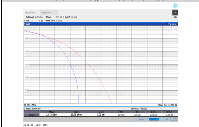
Band5-3MHz-16QAM-20635-15RB#0
