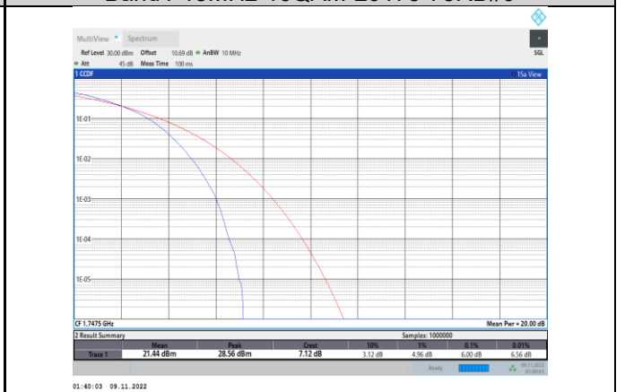
Band4-15MHz-16QAM-20325-75RB#0
