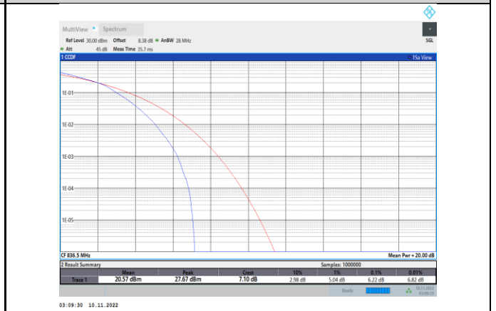
Band5-1.4MHz-16QAM-20525-6RB#0
