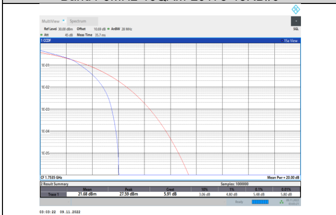
Band4-3MHz-16QAM-20385-15RB#0
