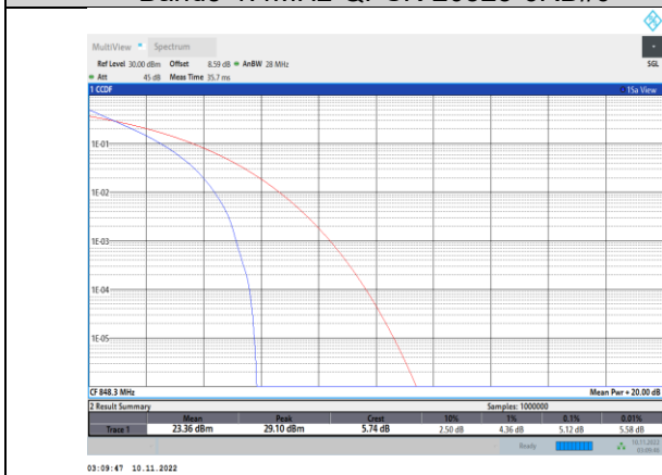
Band5-1.4MHz-QPSK-20643-6RB#0
