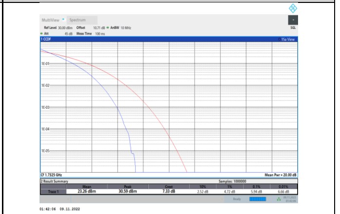
Band4-10MHz-QPSK-20175-50RB#0
