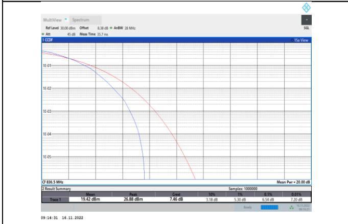
Band5-1.4MHz-64QAM-20525-6RB#0
