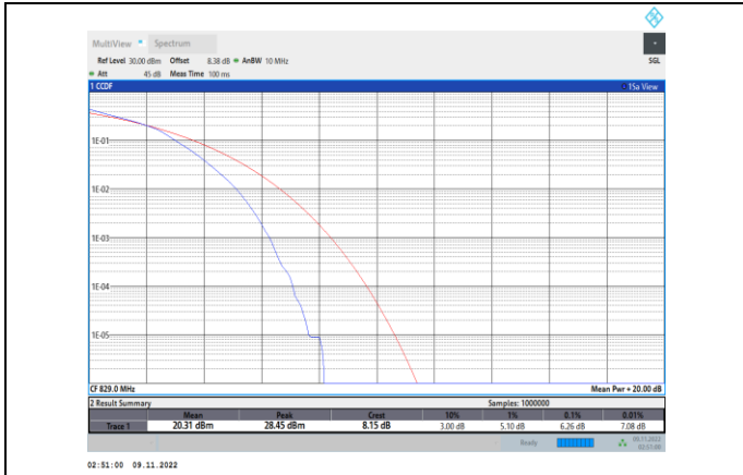
Band5-10MHz-16QAM-20450-50RB#0
