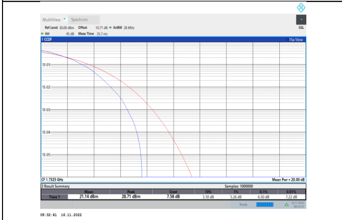
Band4-1.4MHz-64QAM-20175-6RB#0
