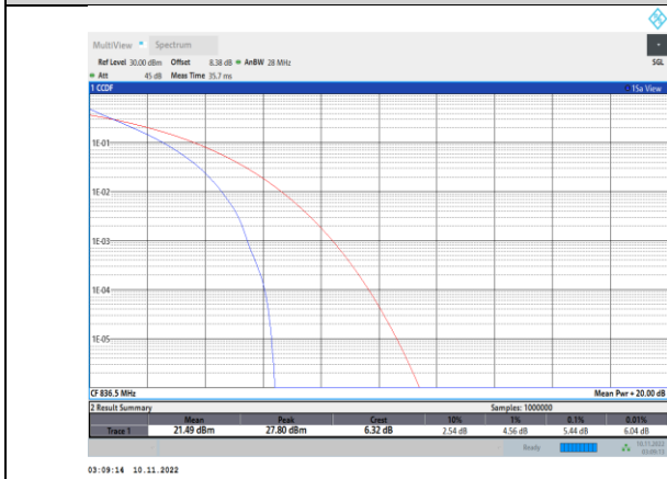
Band5-1.4MHz-QPSK-20525-6RB#0
