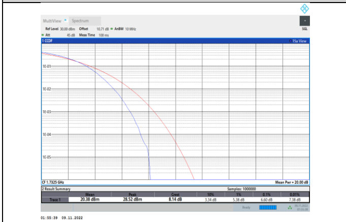
Band4-20MHz-16QAM-20175-100RB#0
