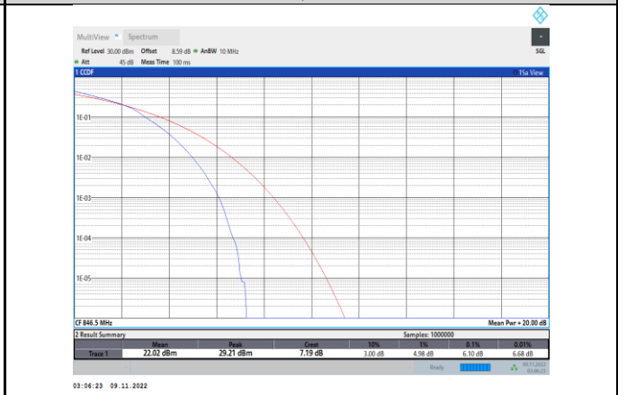
Band5-5MHz-16QAM-20625-25RB#0
