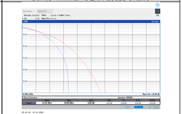
Band5-1.4MHz-16QAM-20643-6RB#0
