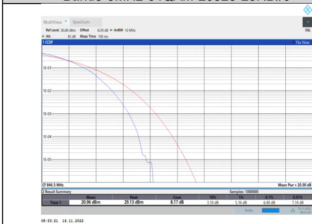
Band5-5MHz-64QAM-20625-25RB#0
