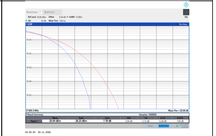
Band5-5MHz-16QAM-20525-25RB#0
