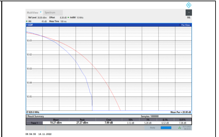
Band5-10MHz-64QAM-20450-50RB#0
