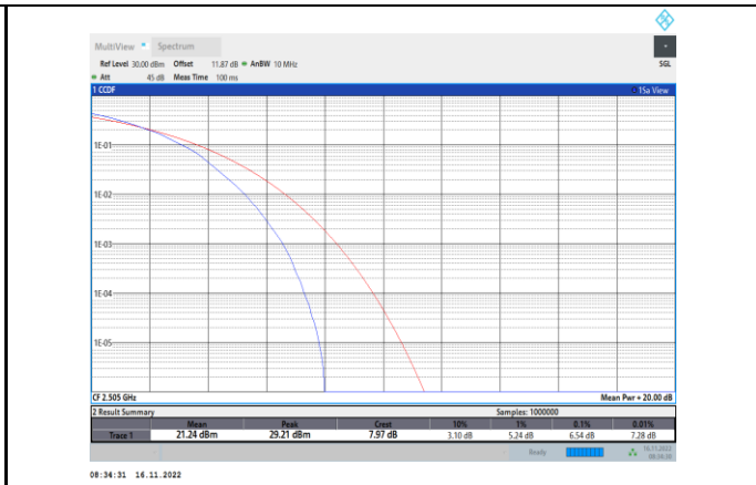
Band7-10MHz-64QAM-20800-50RB#0
