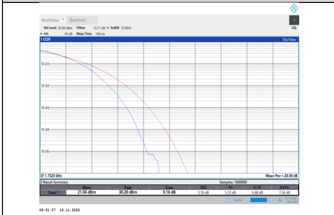
Band4-5MHz-64QAM-20175-25RB#0
