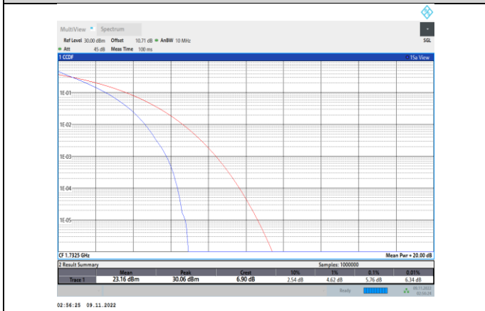
Band4-5MHz-QPSK-20175-25RB#0
