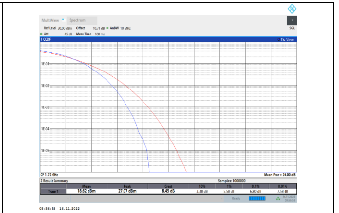
Band4-20MHz-64QAM-20050-100RB#0
