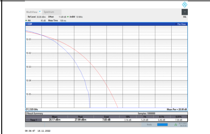
Band7-10MHz-64QAM-21100-50RB#0
