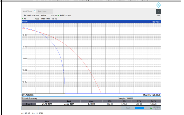
Band4-5MHz-16QAM-20375-25RB#0
