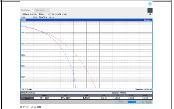
Band4-20MHz-64QAM-20175-100RB#0
