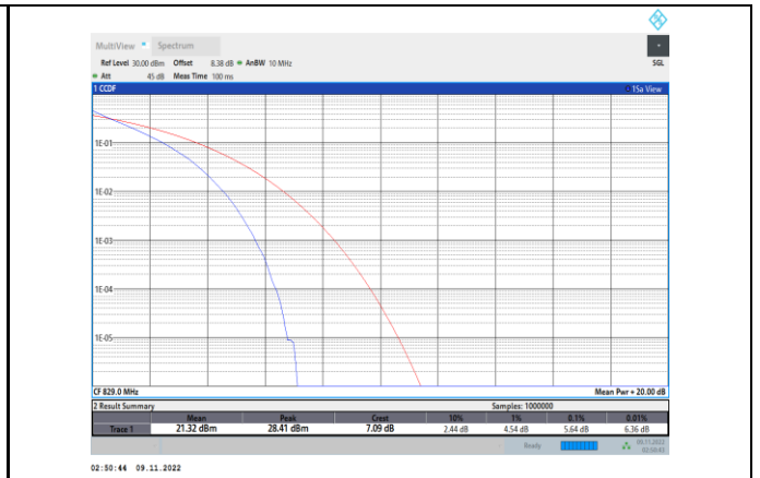
Band5-10MHz-QPSK-20450-50RB#0
