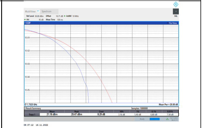
Band4-10MHz-64QAM-20175-50RB#0
