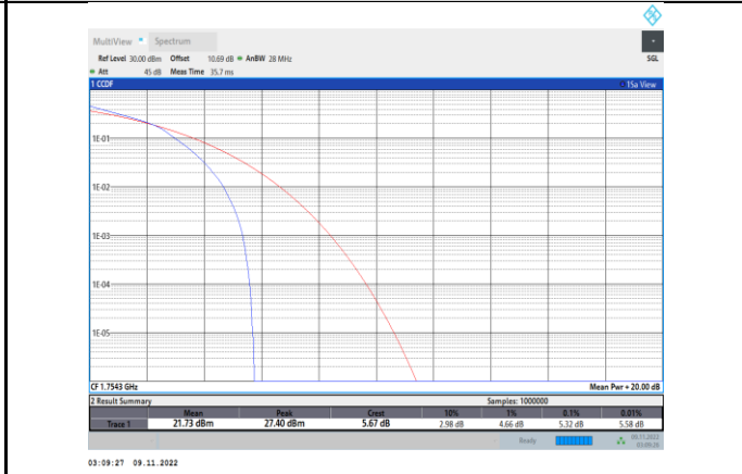
Band4-1.4MHz-16QAM-20393-6RB#0
