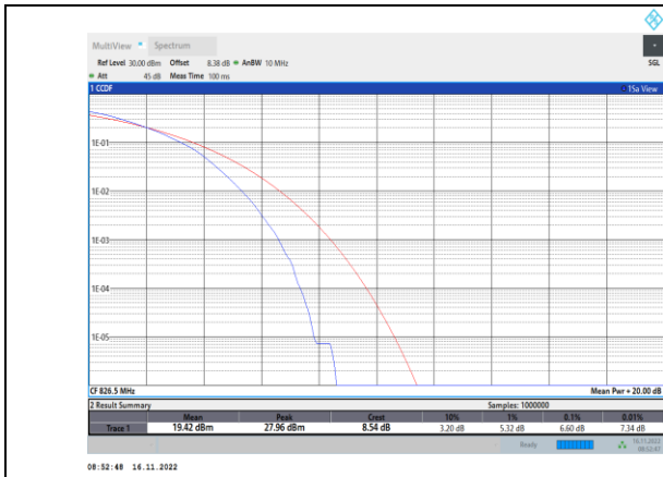
Band5-5MHz-64QAM-20425-25RB#0
