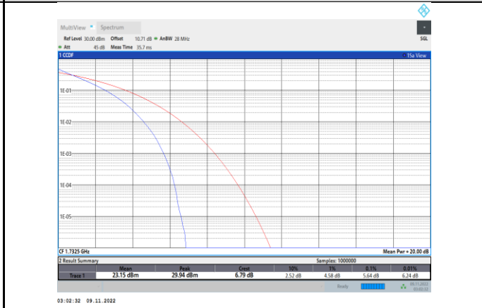
Band4-3MHz-QPSK-20175-15RB#0
