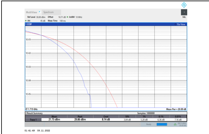
Band4-10MHz-16QAM-20000-50RB#0
