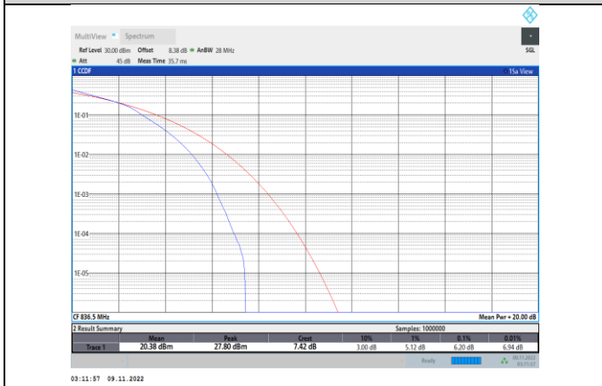
Band5-3MHz-16QAM-20525-15RB#0
