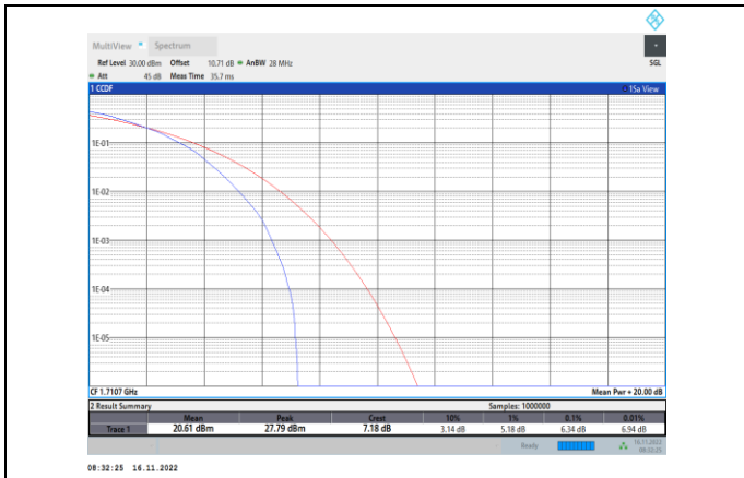
Band4-1.4MHz-64QAM-19957-6RB#0
