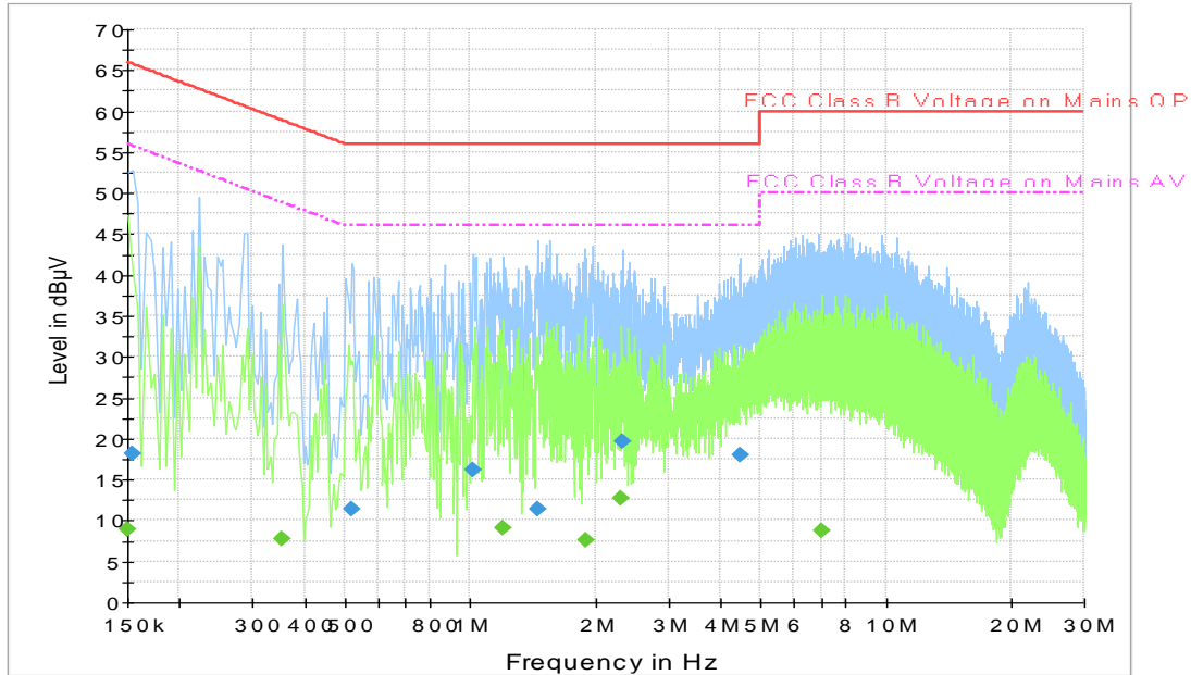
Fig.A.7.1 AC Powerline Conducted Emission-Idle
