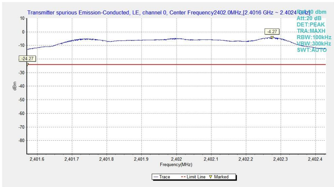
Fig.13. Transmitter Spurious Emission - Conducted: GFSK,2402MHz
